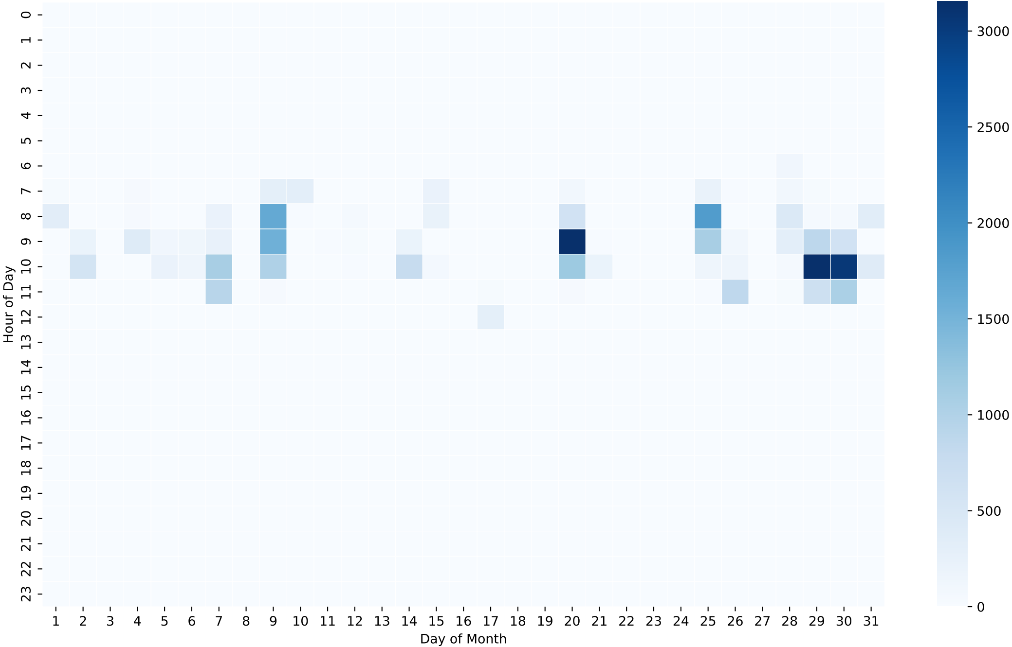
Battery Charging Power Heatmap (Wh/Hour) - 5kWh - Dec
