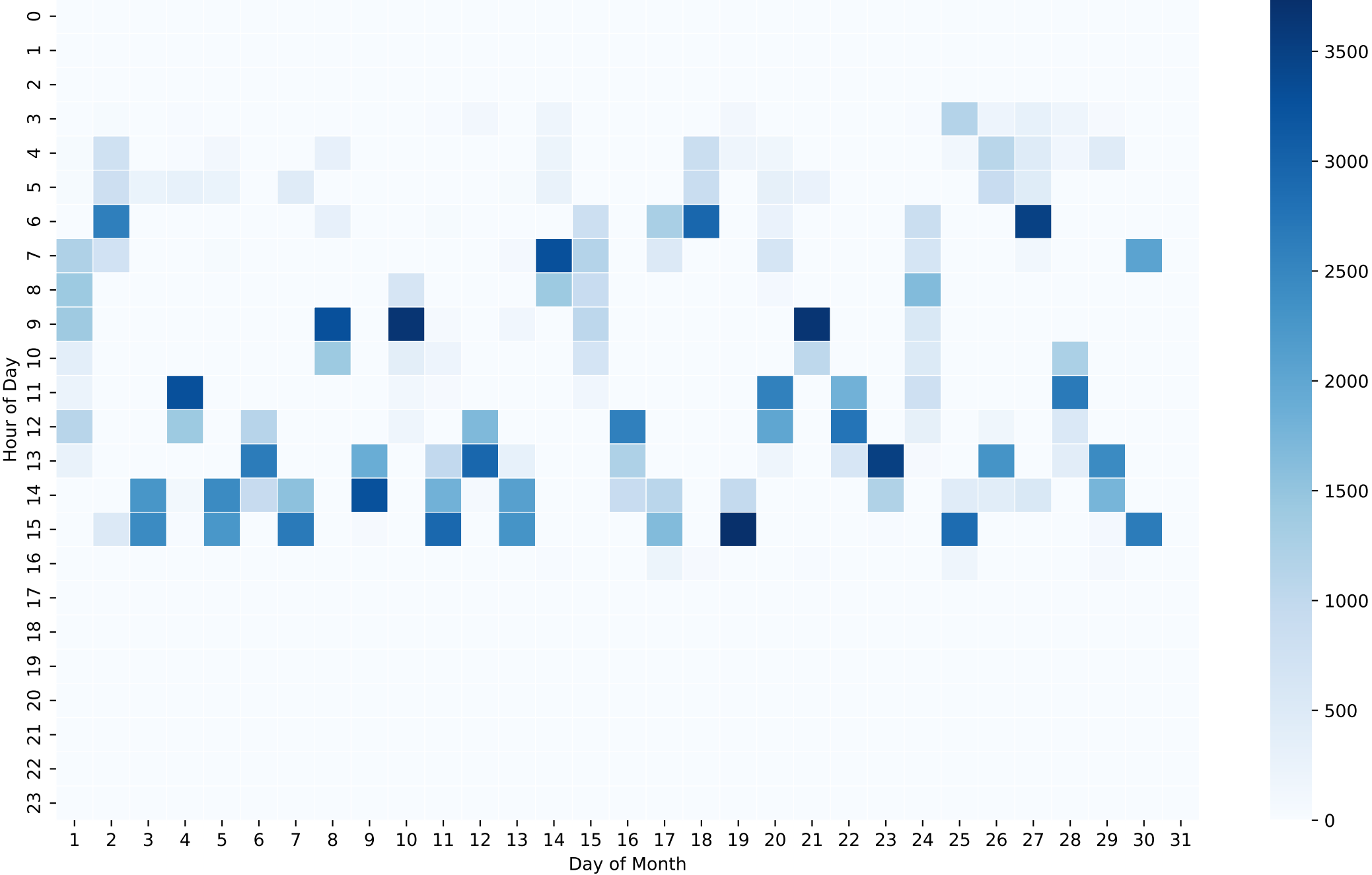
Battery Charging Power Heatmap (Wh/Hour) - 5kWh - Apr
