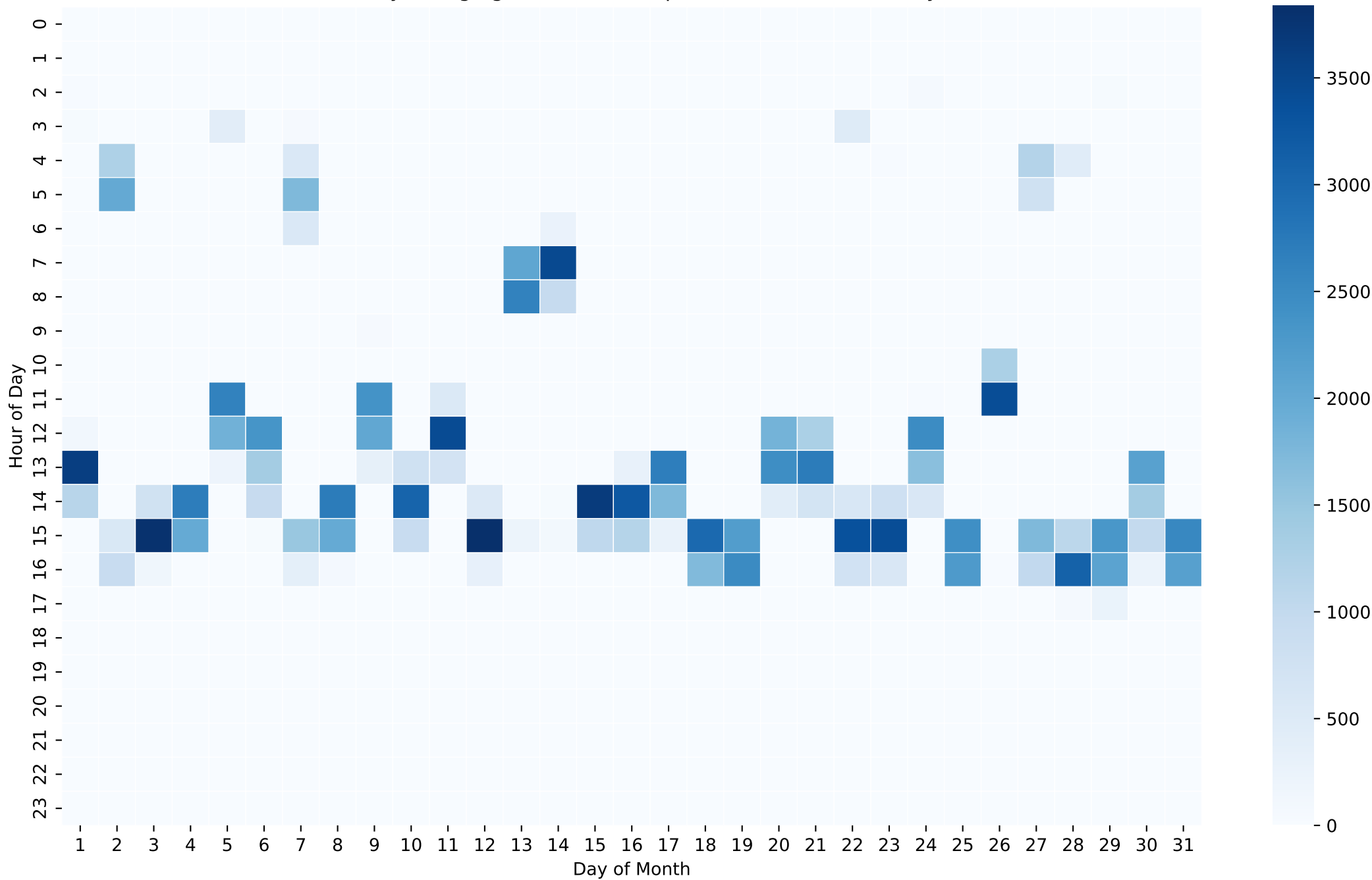
Battery Charging Power Heatmap (Wh/Hour) - 5kWh - May
