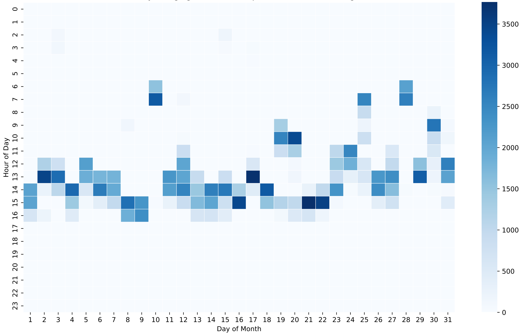
Battery Charging Power Heatmap (Wh/Hour) - 5kWh - Aug
