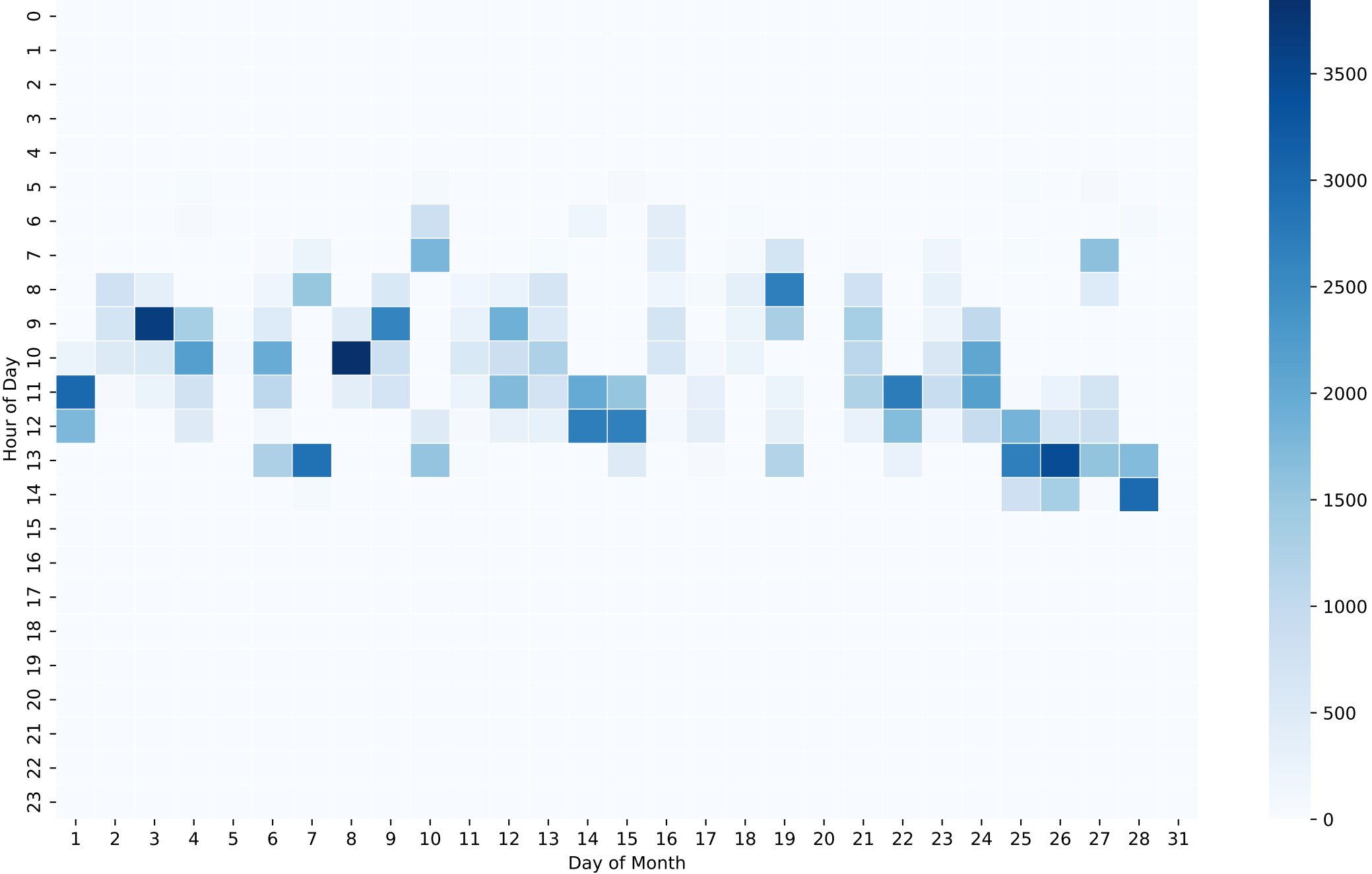
Battery Charging Power Heatmap (Wh/Hour) - 5kWh - Feb
