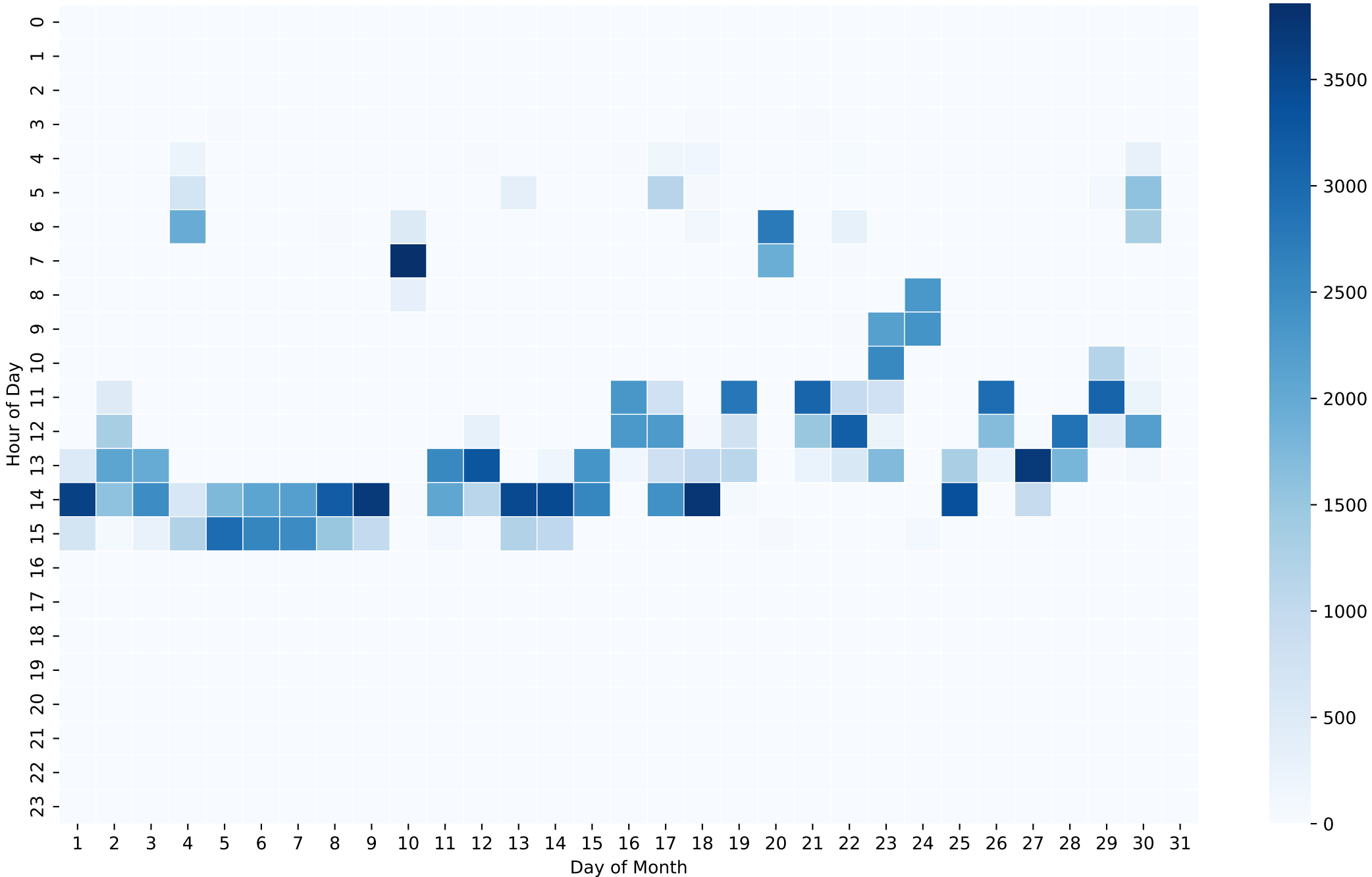
Battery Charging Power Heatmap (Wh/Hour) - 5kWh - Sep
