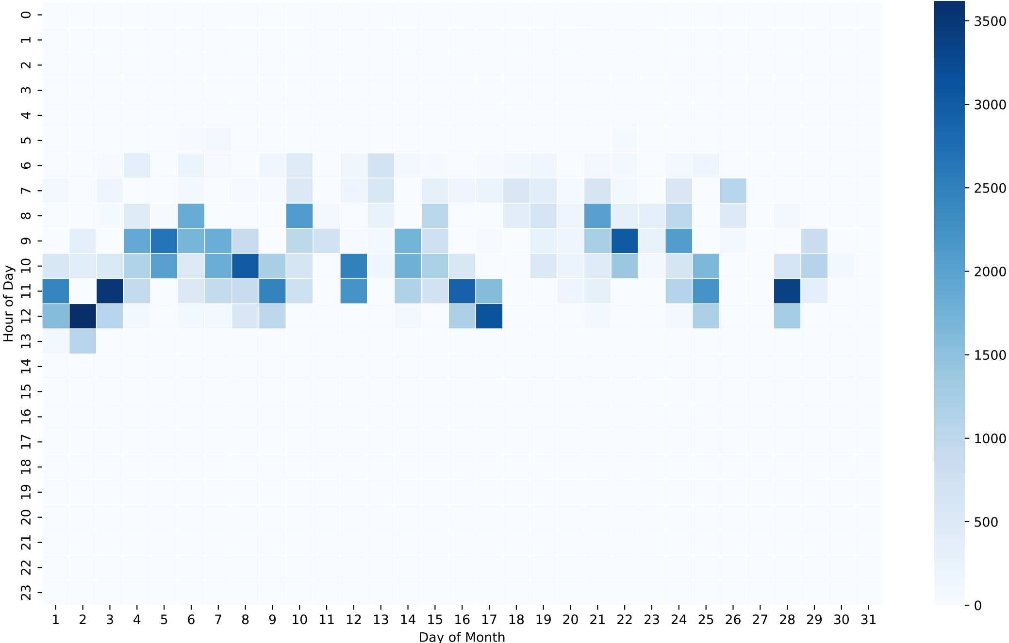
Battery Charging Power Heatmap (Wh/Hour) - 5kWh - Nov
