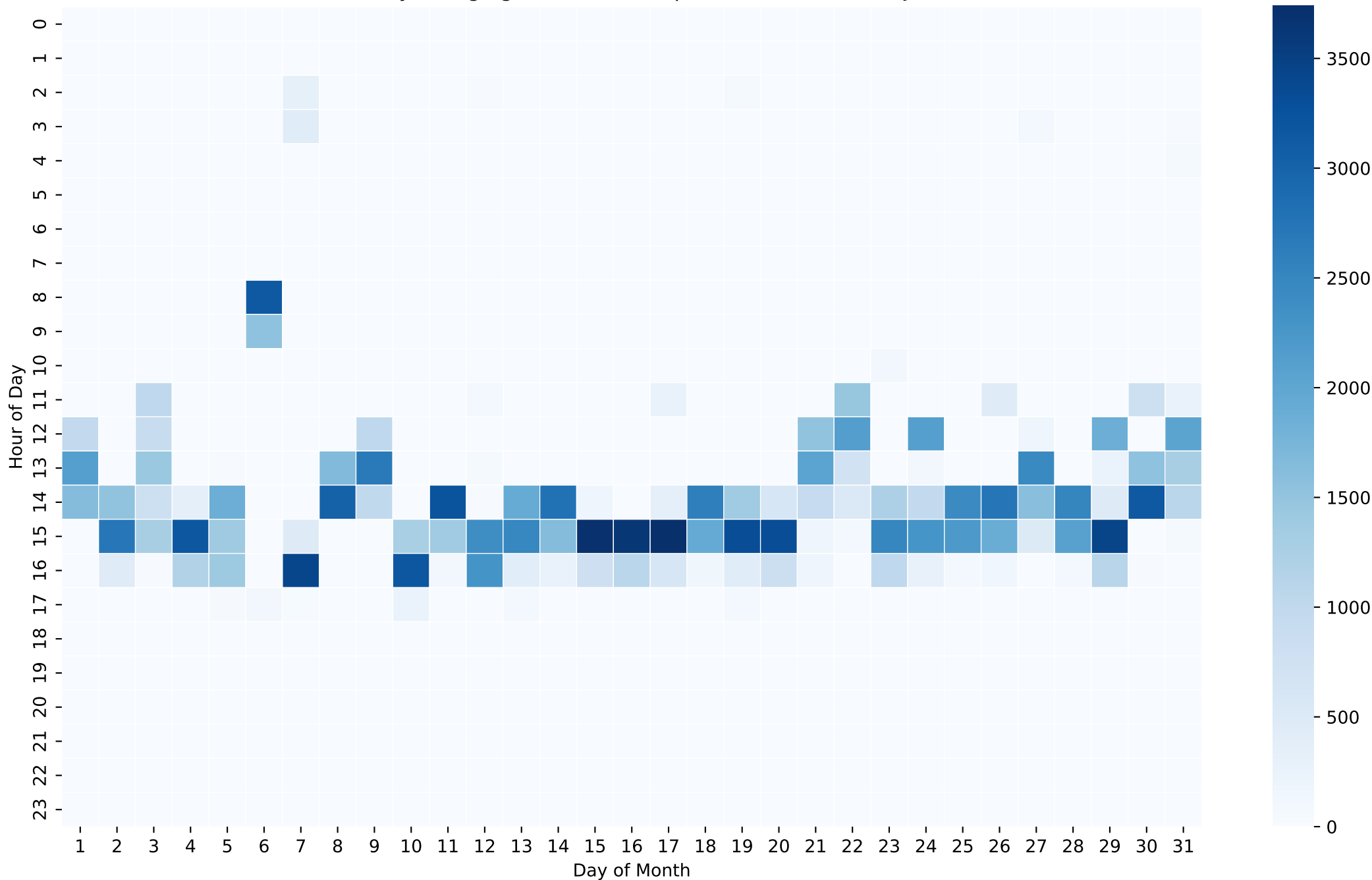
Battery Charging Power Heatmap (Wh/Hour) - 5kWh - Jul
