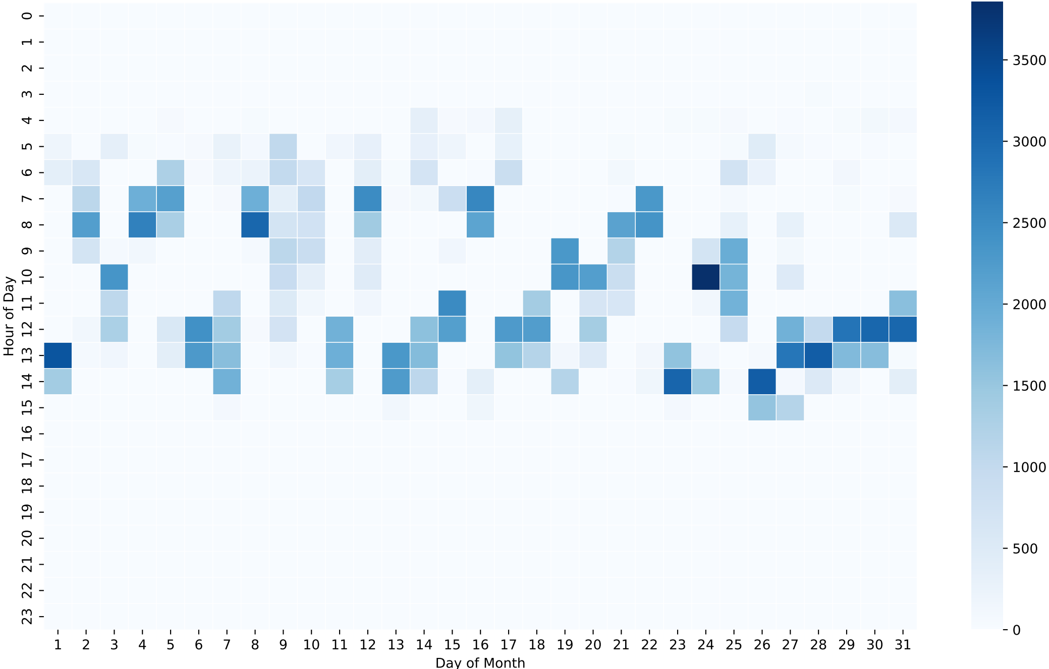
Battery Charging Power Heatmap (Wh/Hour) - 5kWh - Mar
