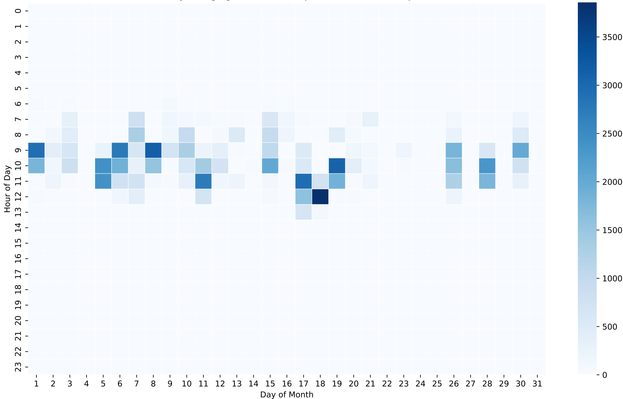
Battery Charging Power Heatmap (Wh/Hour) - 5kWh - Jan
