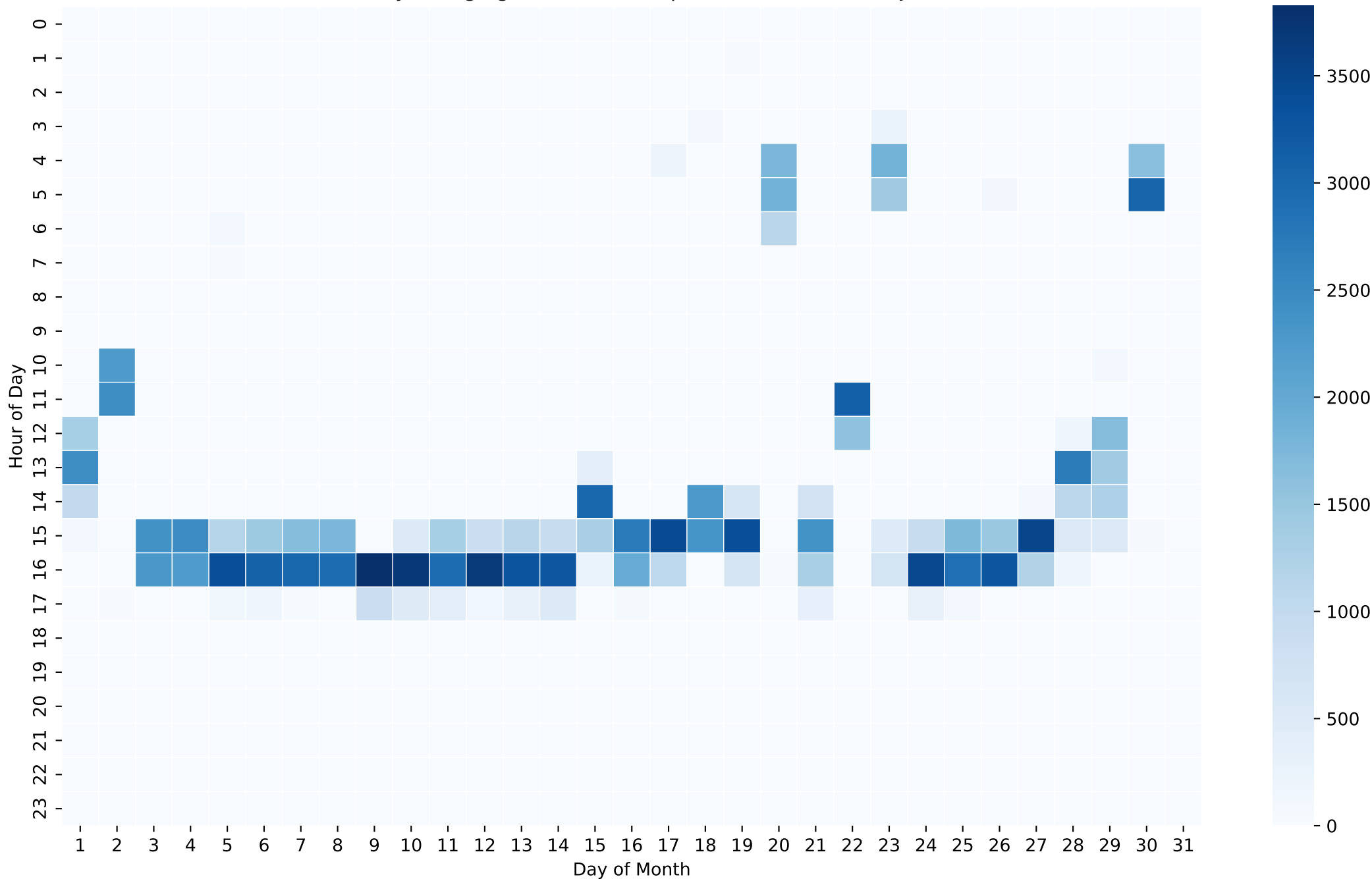
Battery Charging Power Heatmap (Wh/Hour) - 5kWh - Jun
