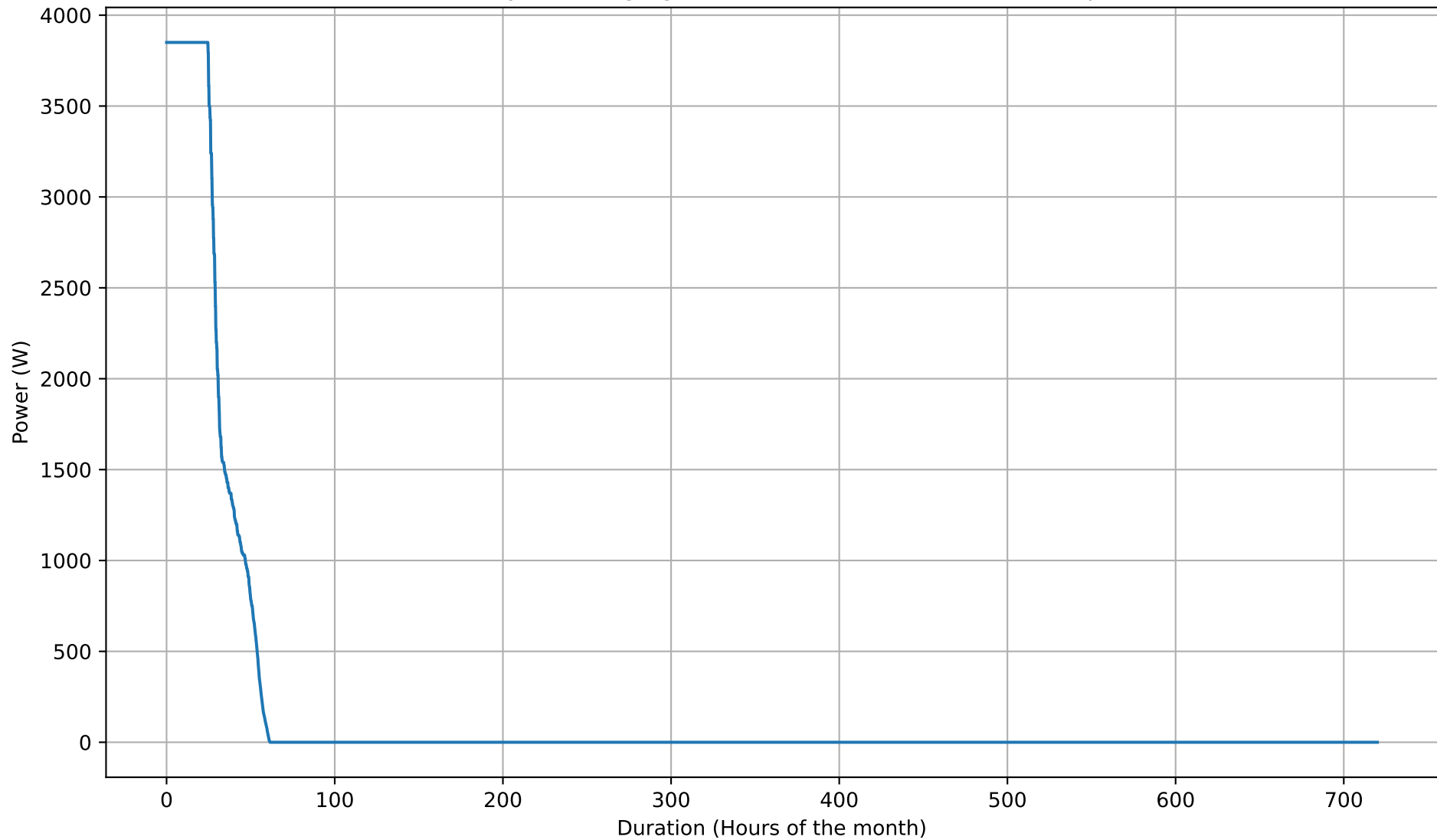
Battery Discharging Power Duration Curve - 5kWh - Apr
