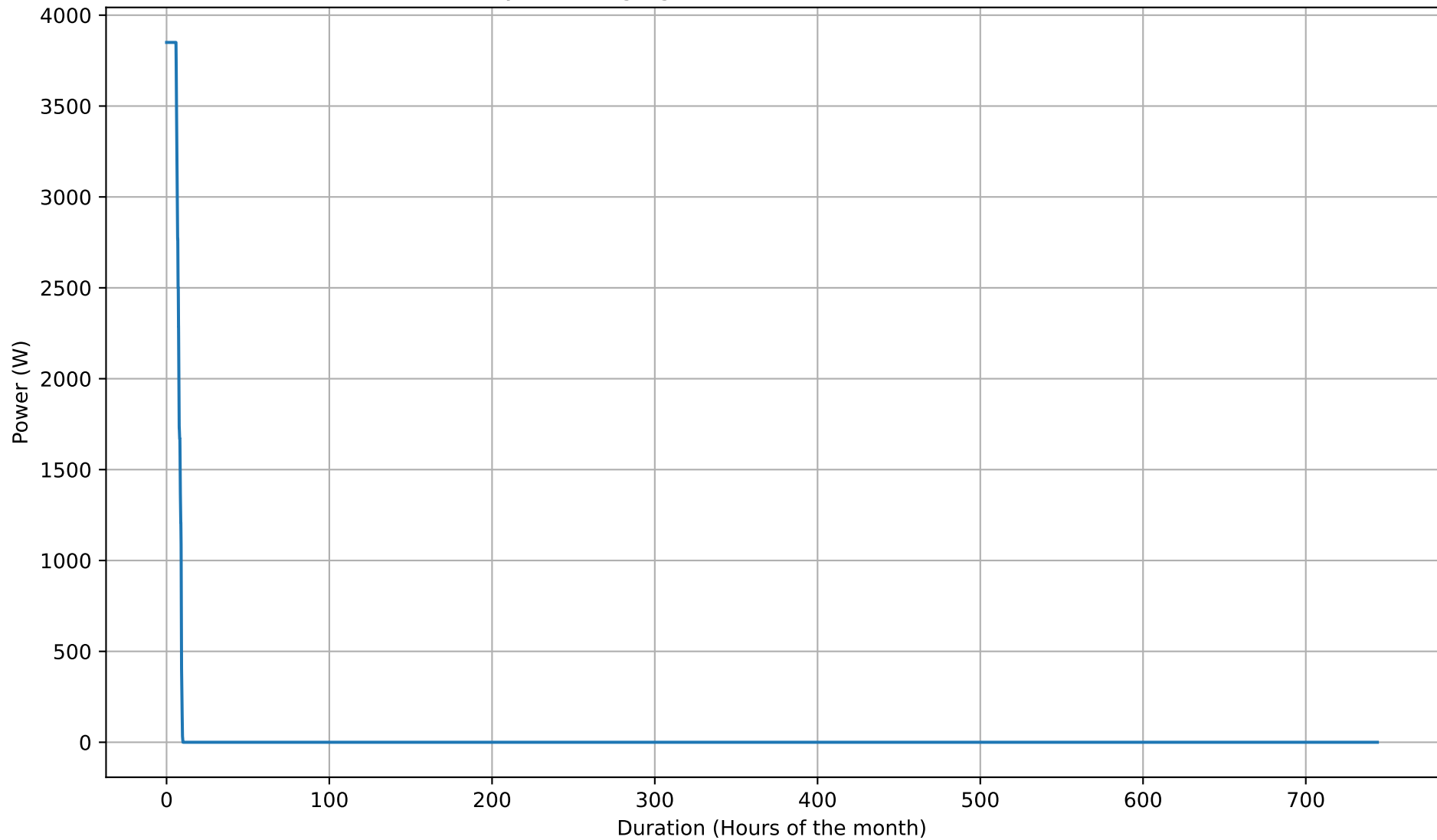
Battery Discharging Power Duration Curve - 5kWh - Dec
