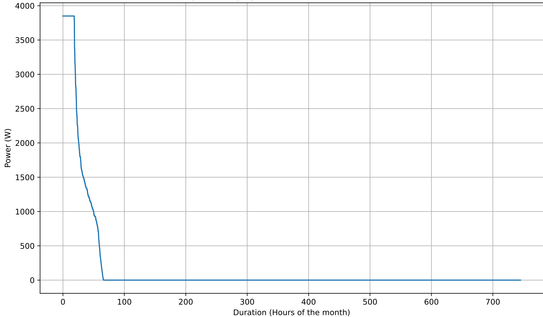
Battery Discharging Power Duration Curve - 5kWh - Oct
