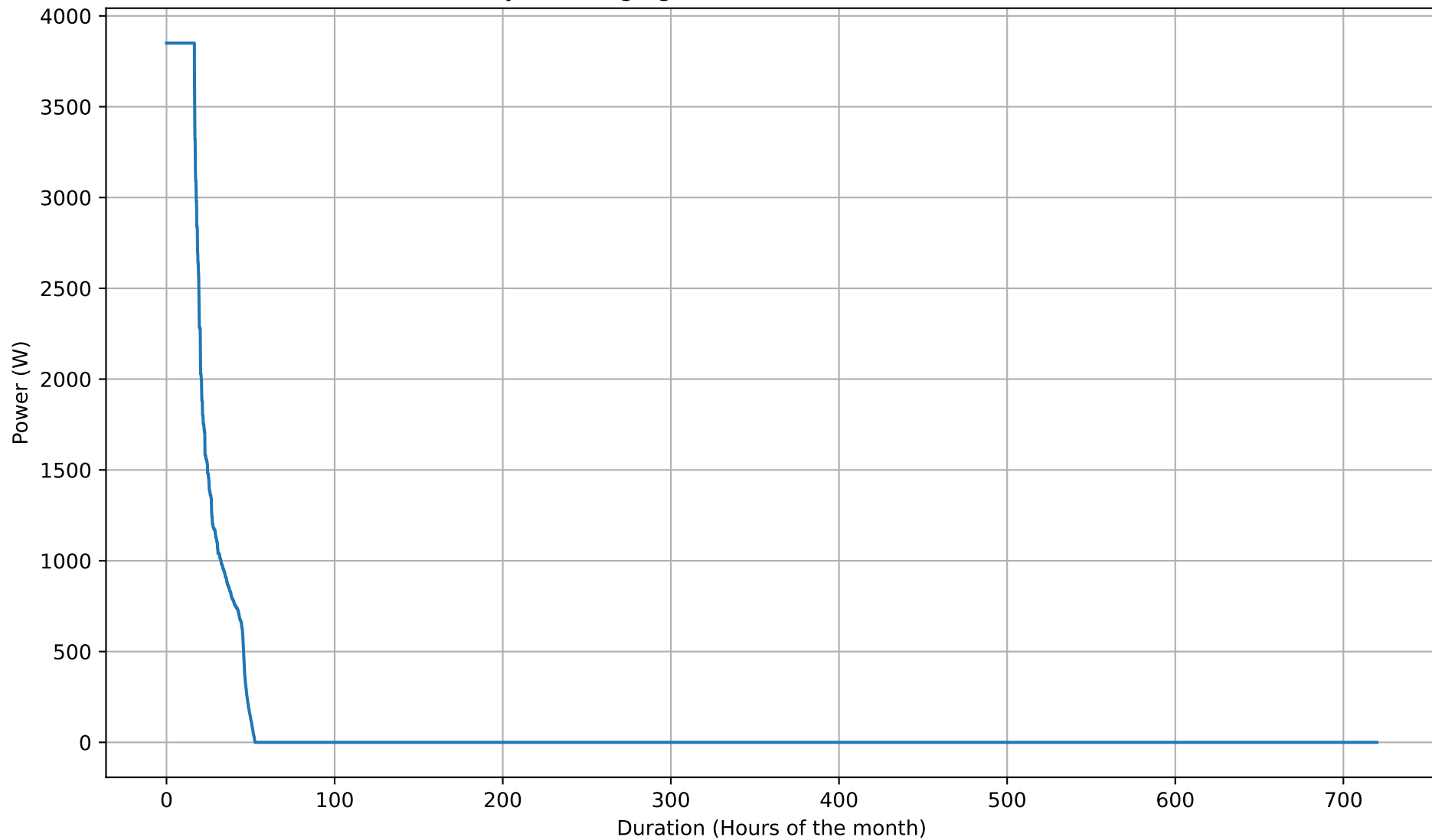
Battery Discharging Power Duration Curve - 5kWh - Nov
