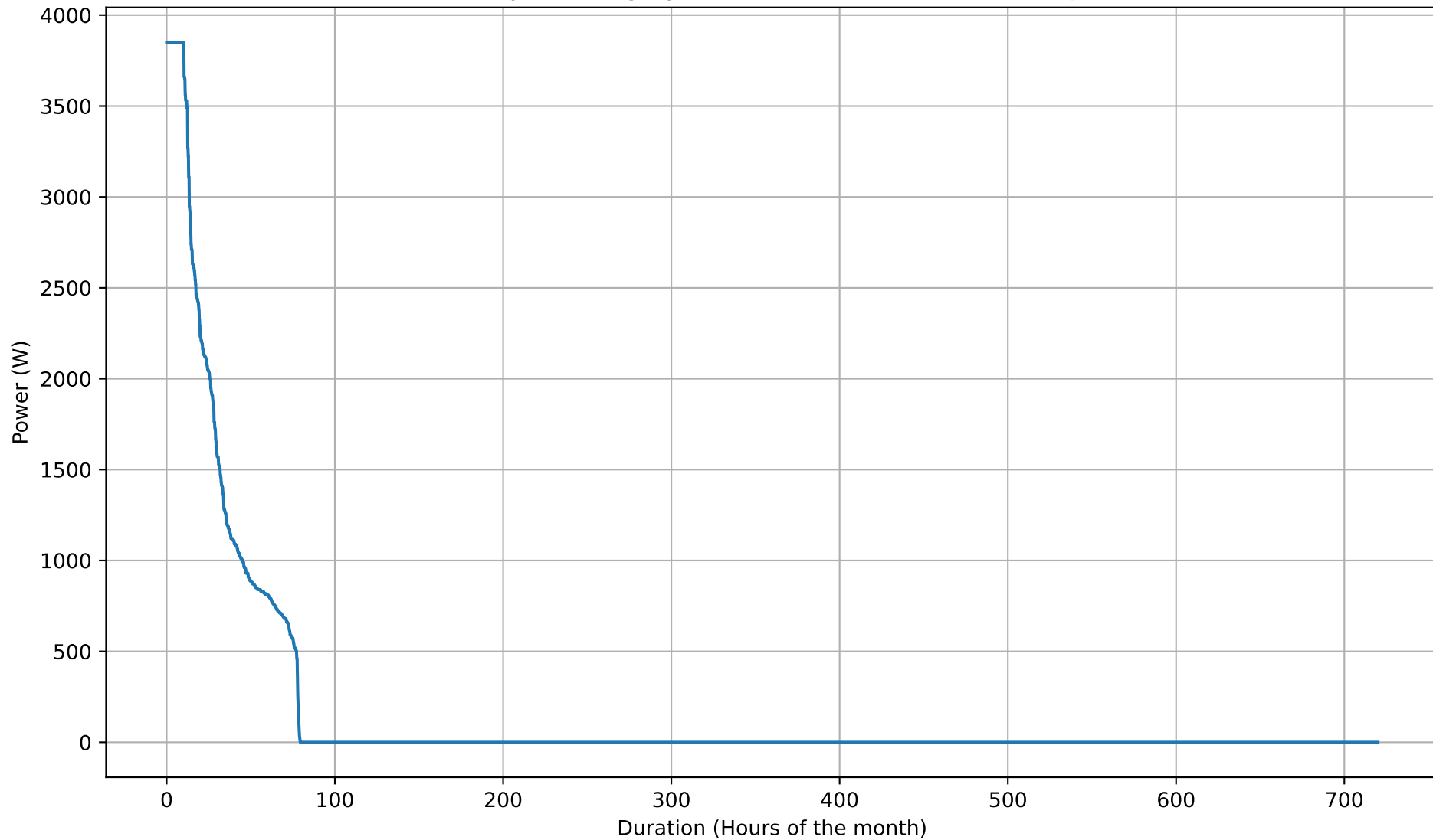
Battery Discharging Power Duration Curve - 5kWh - Jun
