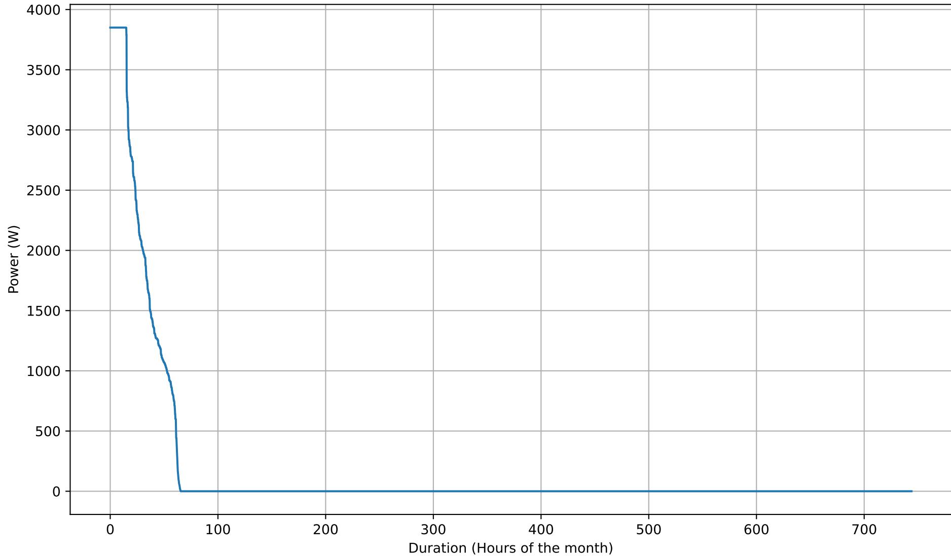
Battery Discharging Power Duration Curve - 5kWh - May
