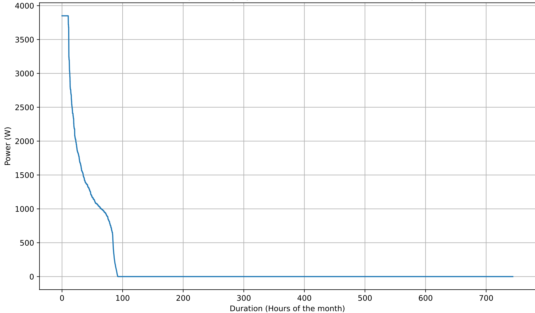
Battery Discharging Power Duration Curve - 5kWh - Aug
