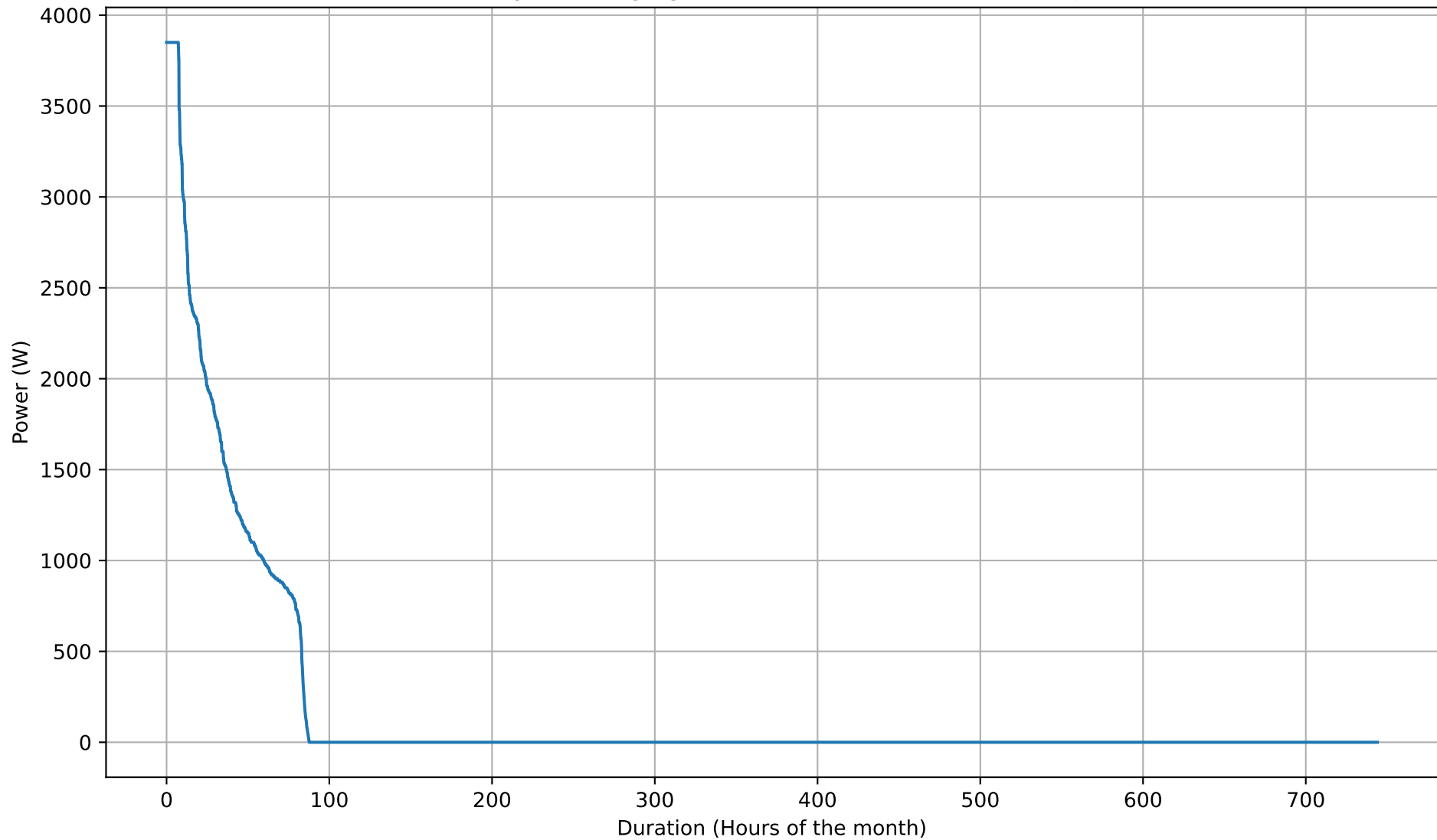
Battery Discharging Power Duration Curve - 5kWh - Jul
