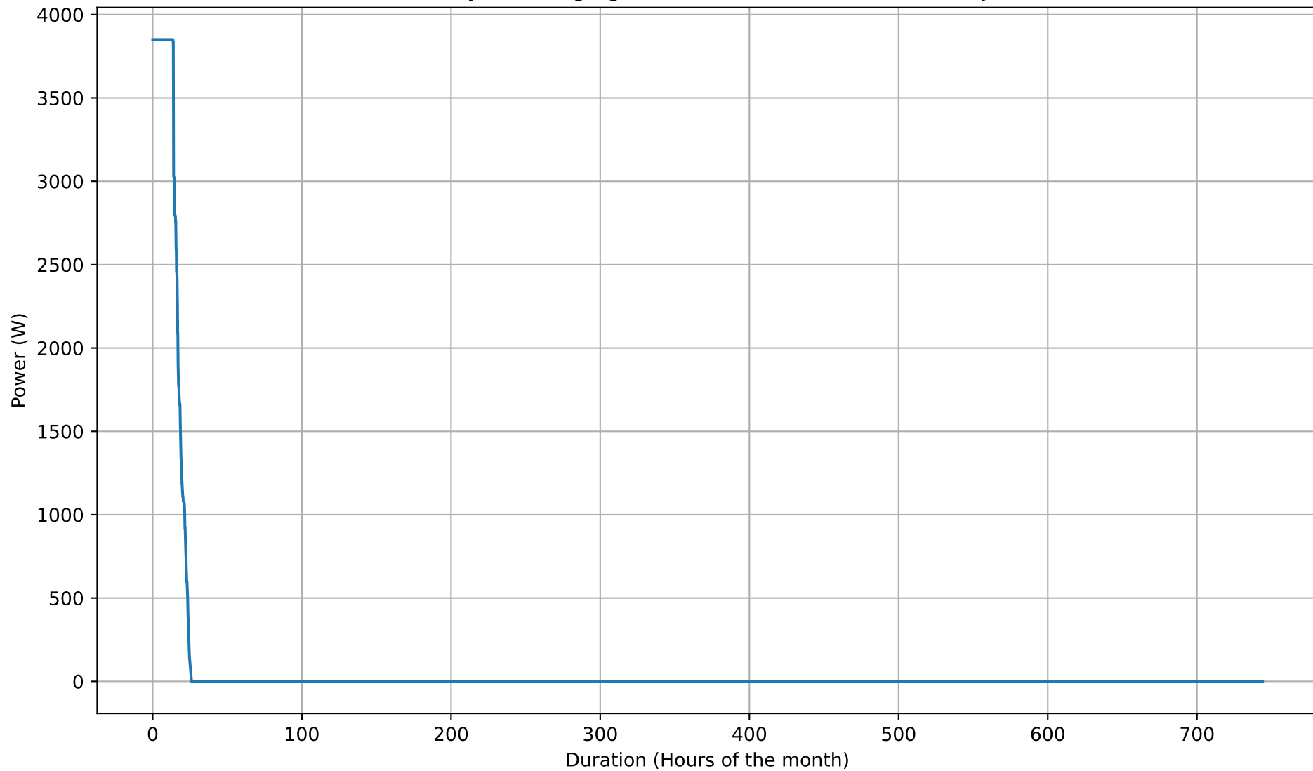
Battery Discharging Power Duration Curve - 5kWh - Jan
