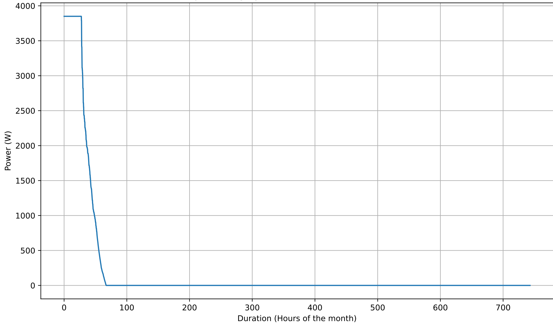
Battery Discharging Power Duration Curve - 5kWh - Mar
