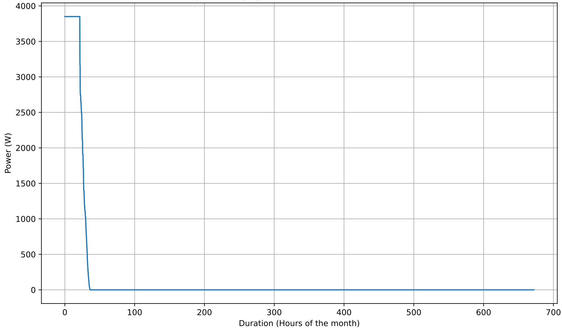
Battery Discharging Power Duration Curve - 5kWh - Feb
