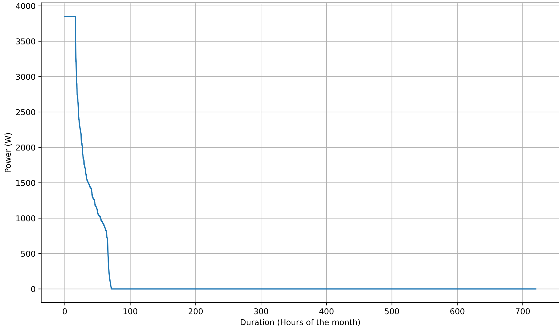
Battery Discharging Power Duration Curve - 5kWh - Sep
