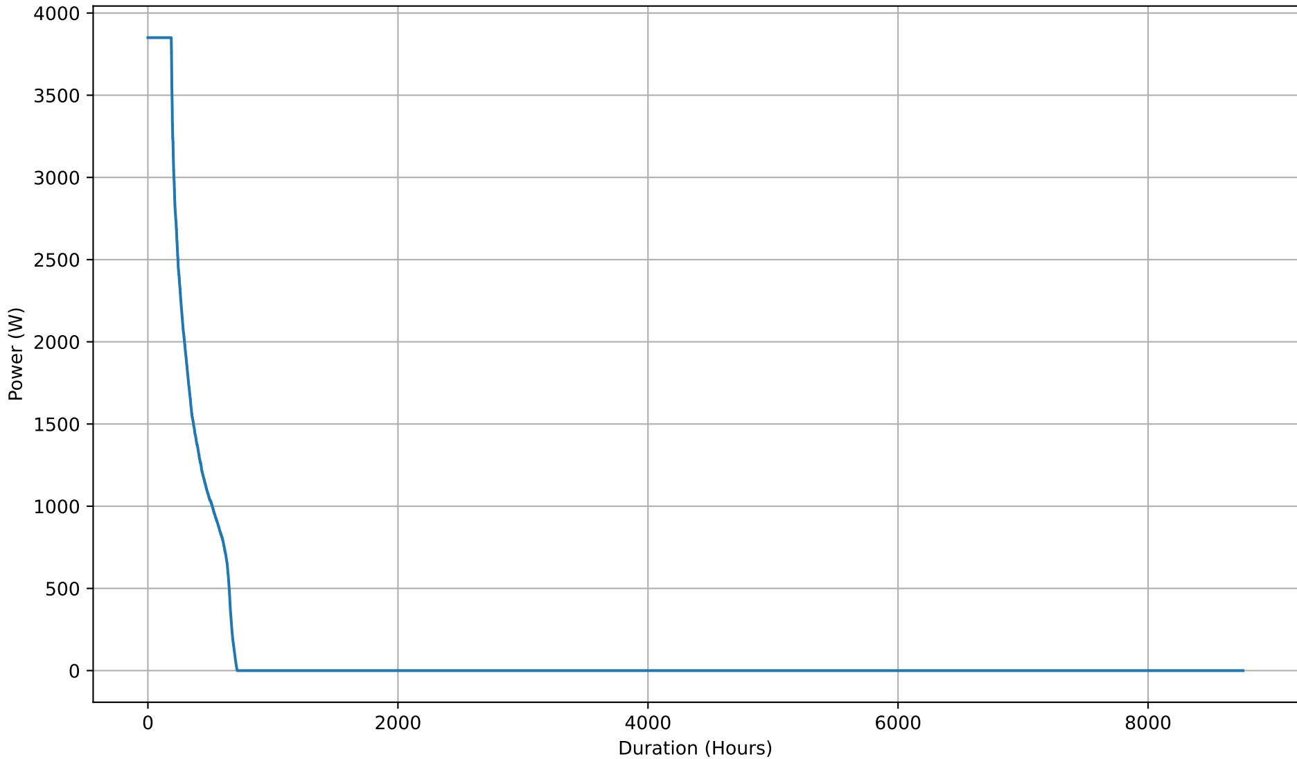
Yearly Battery Discharging Power Duration Curve - 5kWh
