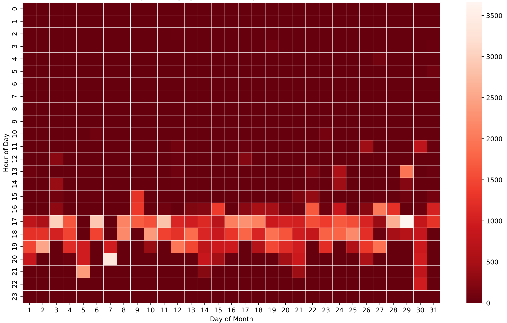
Battery Discharging Power Heatmap (Wh/Hour) - 5kWh - Jul
