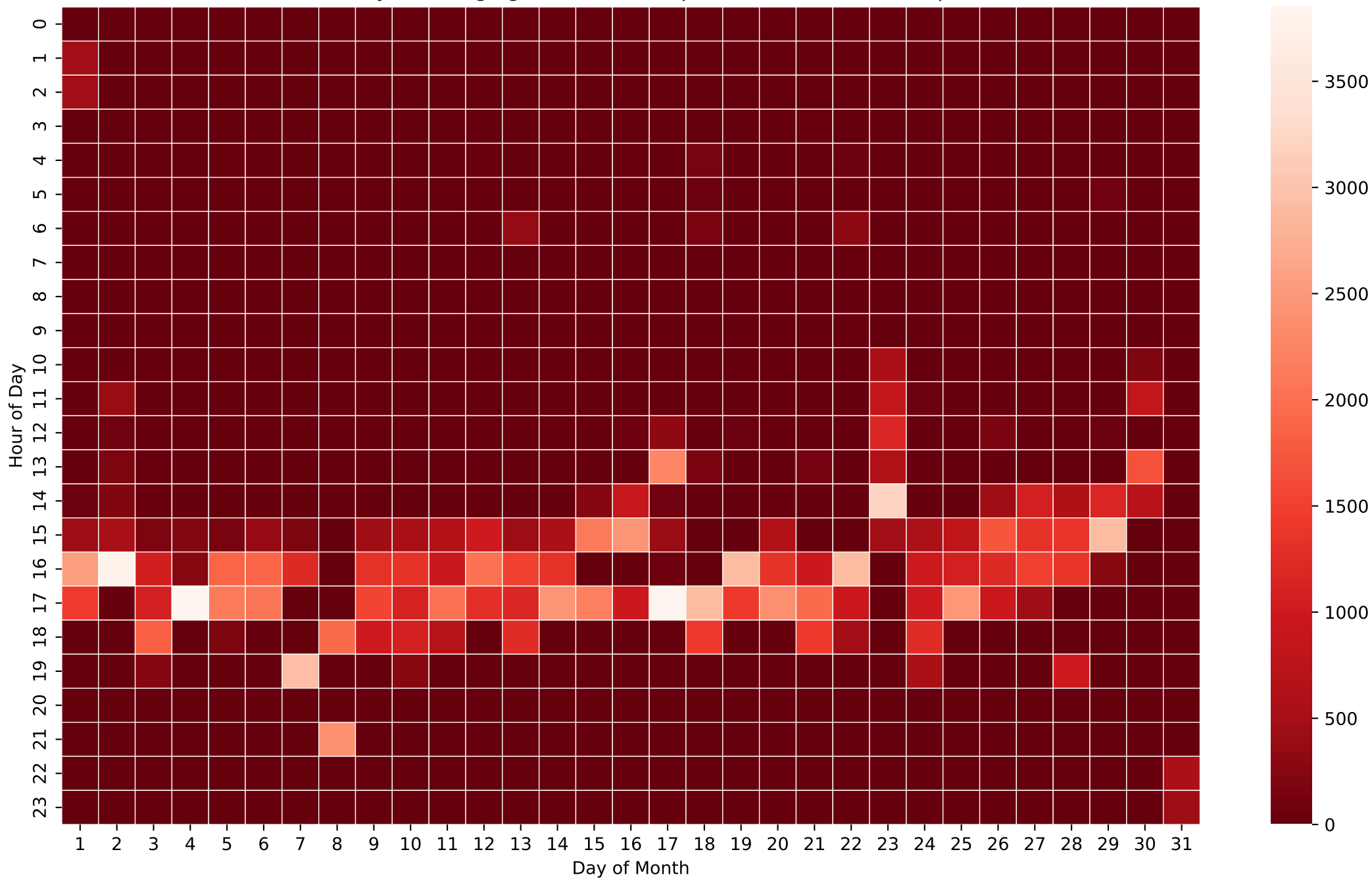
Battery Discharging Power Heatmap (Wh/Hour) - 5kWh - Sep
