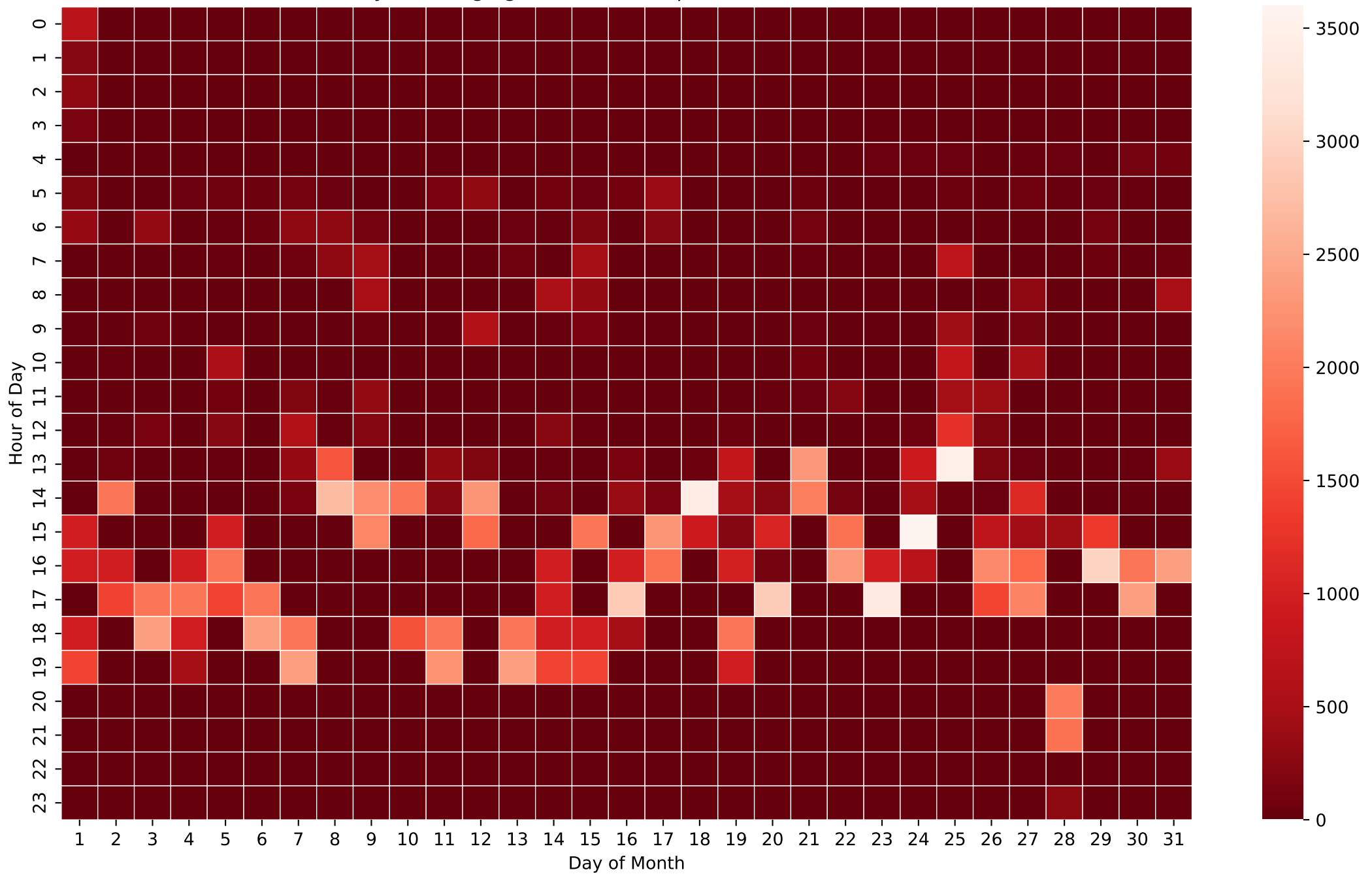
Battery Discharging Power Heatmap (Wh/Hour) - 5kWh - Mar
