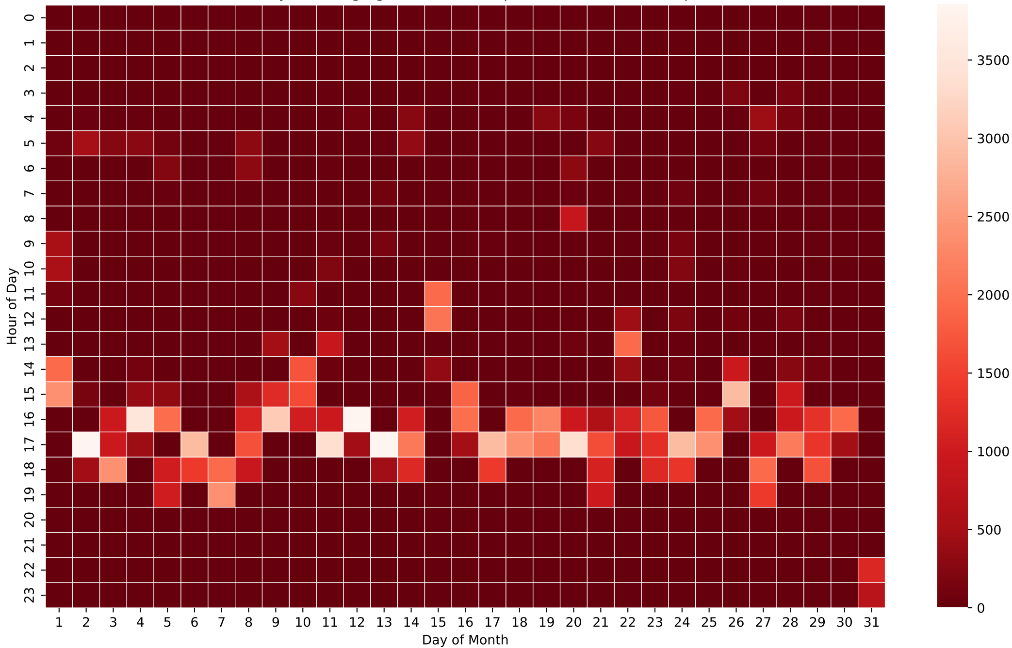
Battery Discharging Power Heatmap (Wh/Hour) - 5kWh - Apr
