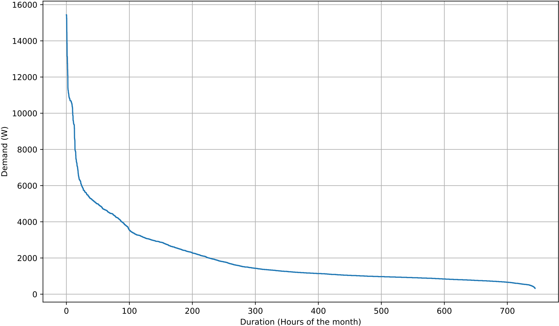
Electricity Demand Duration Curve - 5kWh - May
