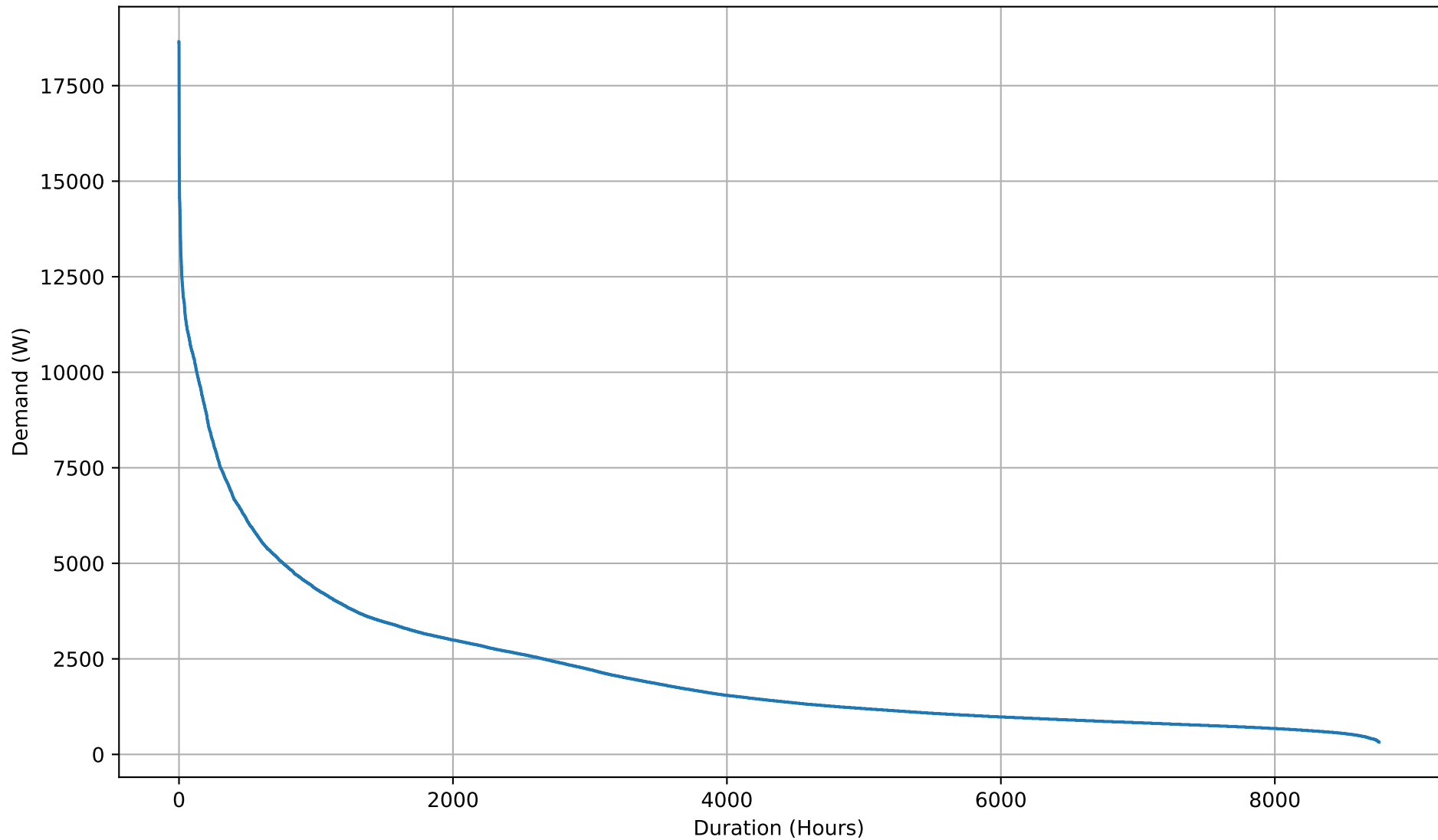
Yearly Electricity Demand Duration Curve - 5kWh
