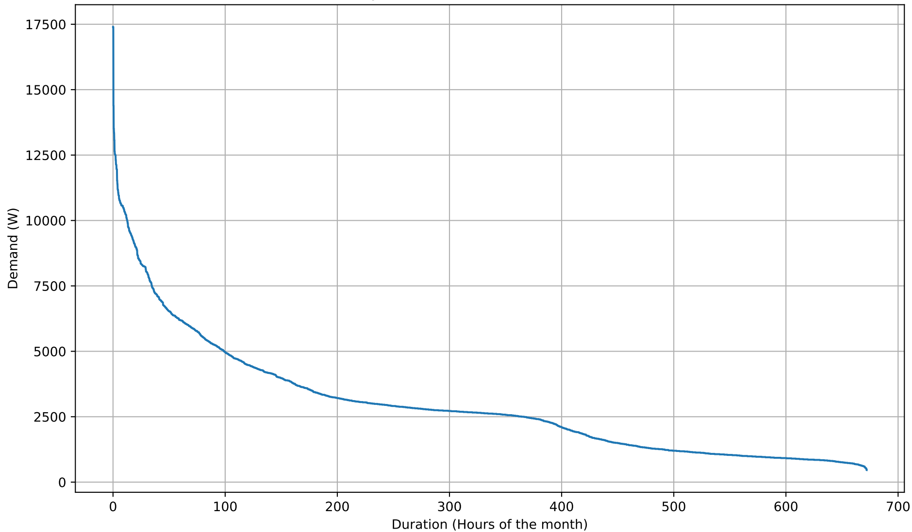
Electricity Demand Duration Curve - 5kWh - Feb
