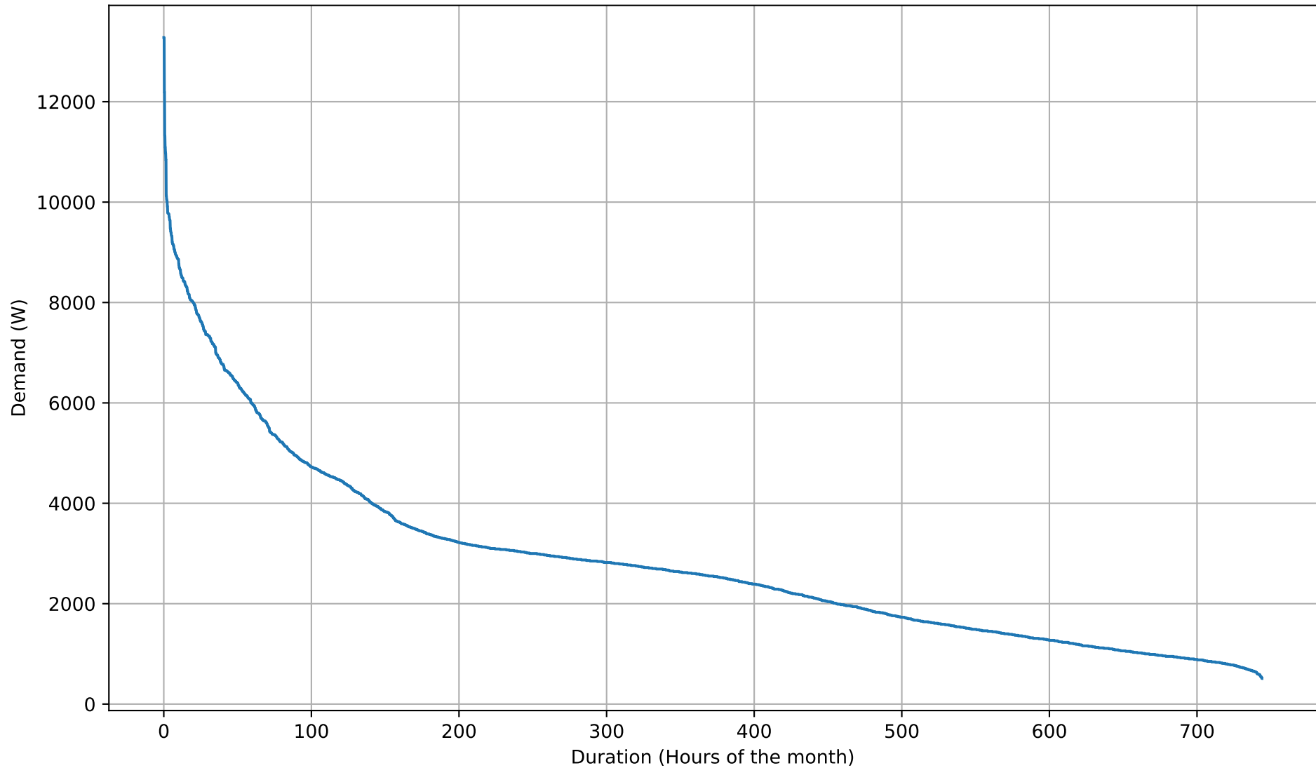
Electricity Demand Duration Curve - 5kWh - Jan
