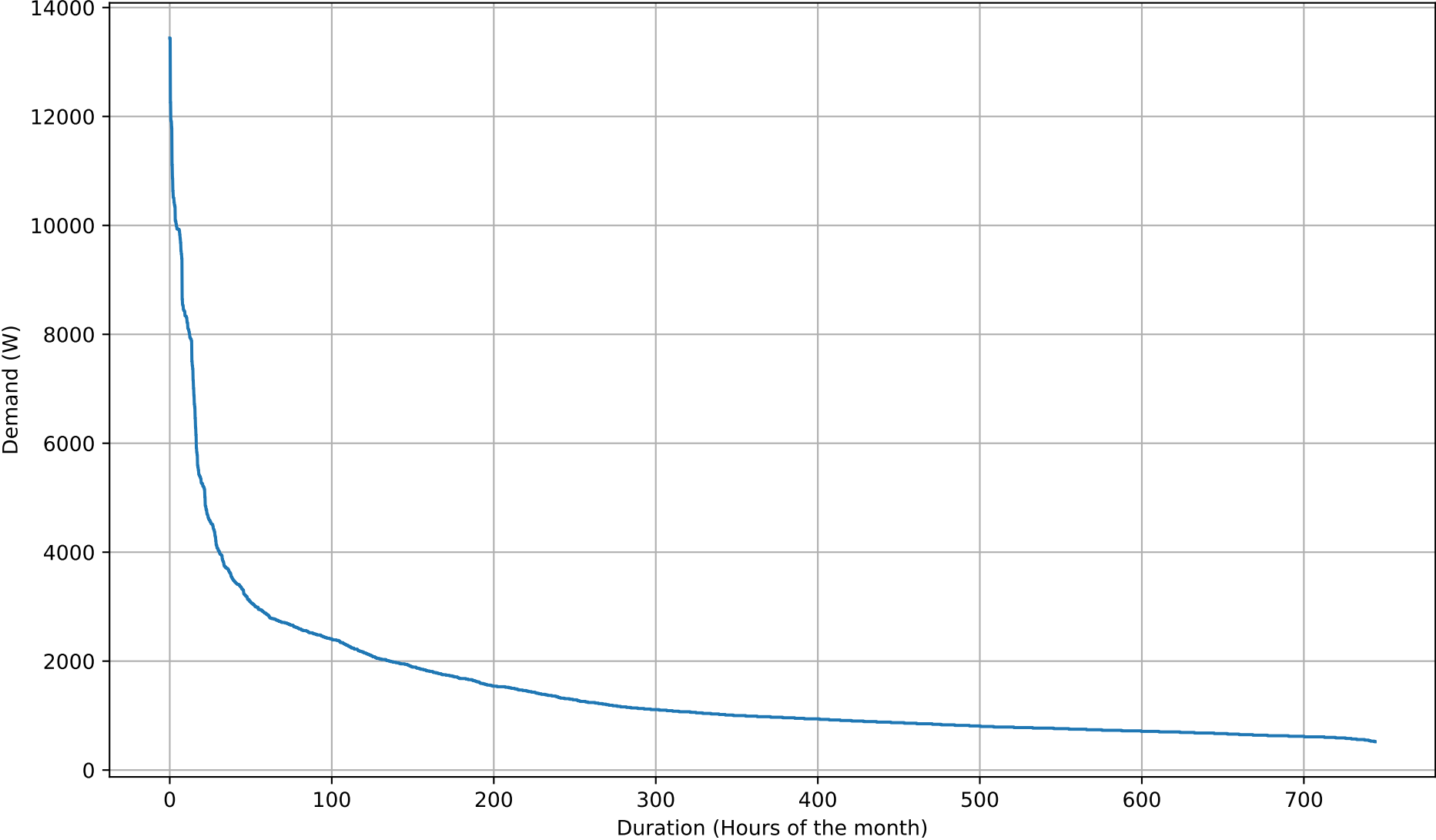
Electricity Demand Duration Curve - 5kWh - Aug
