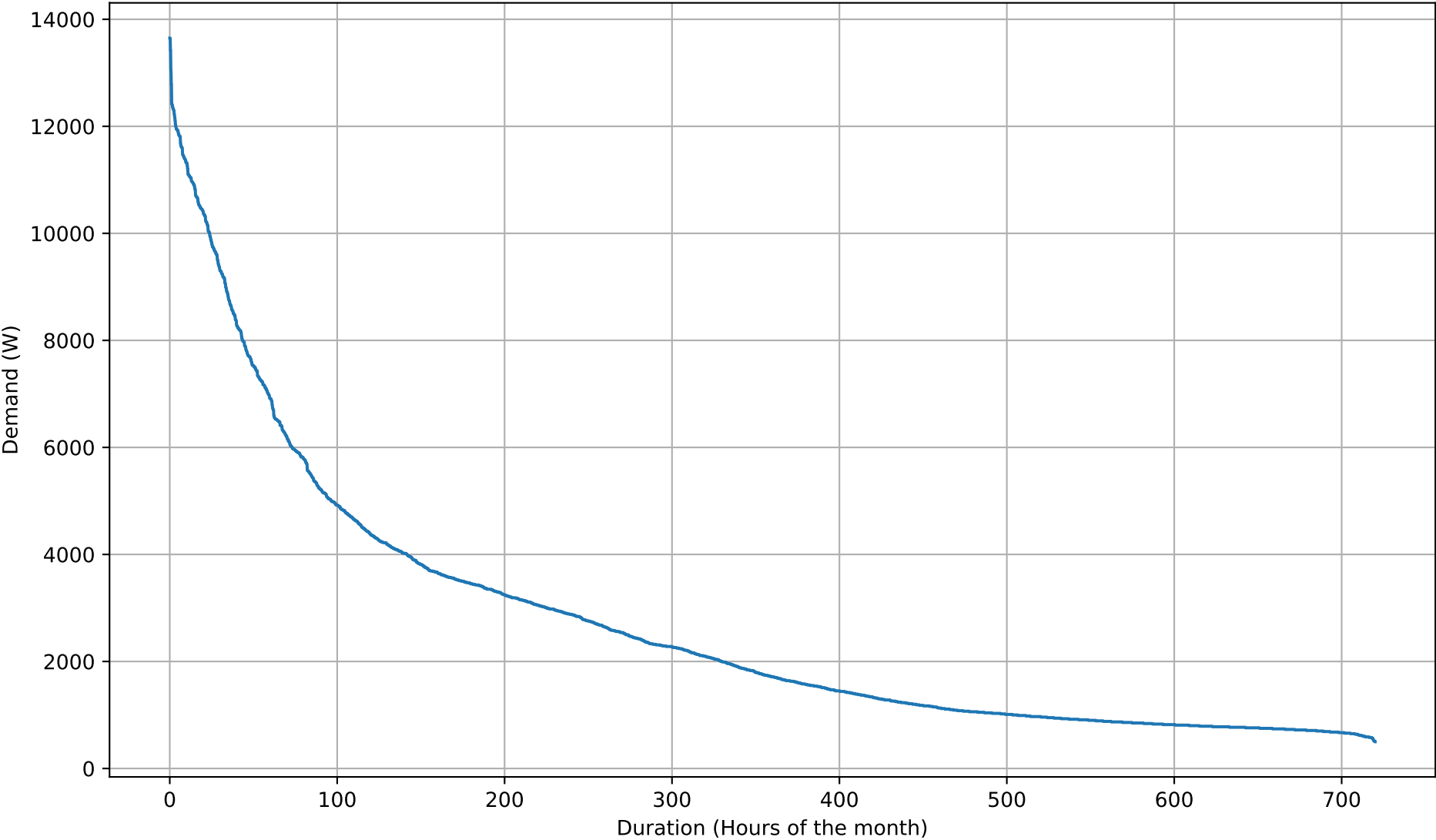
Electricity Demand Duration Curve - 5kWh - Nov
