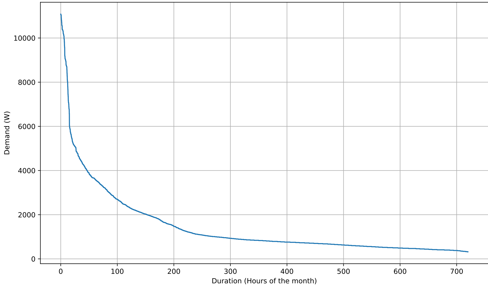
Electricity Demand Duration Curve - 5kWh - Jun
