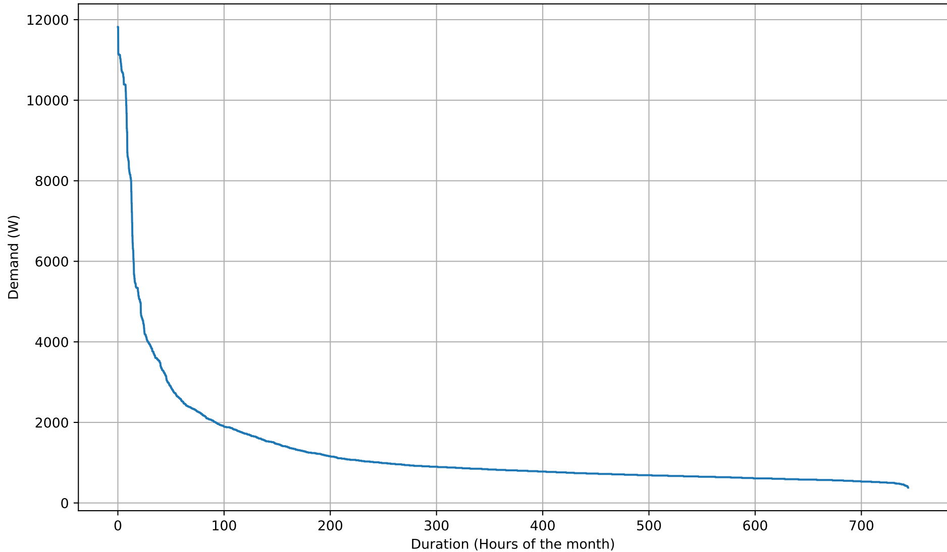
Electricity Demand Duration Curve - 5kWh - Jul
