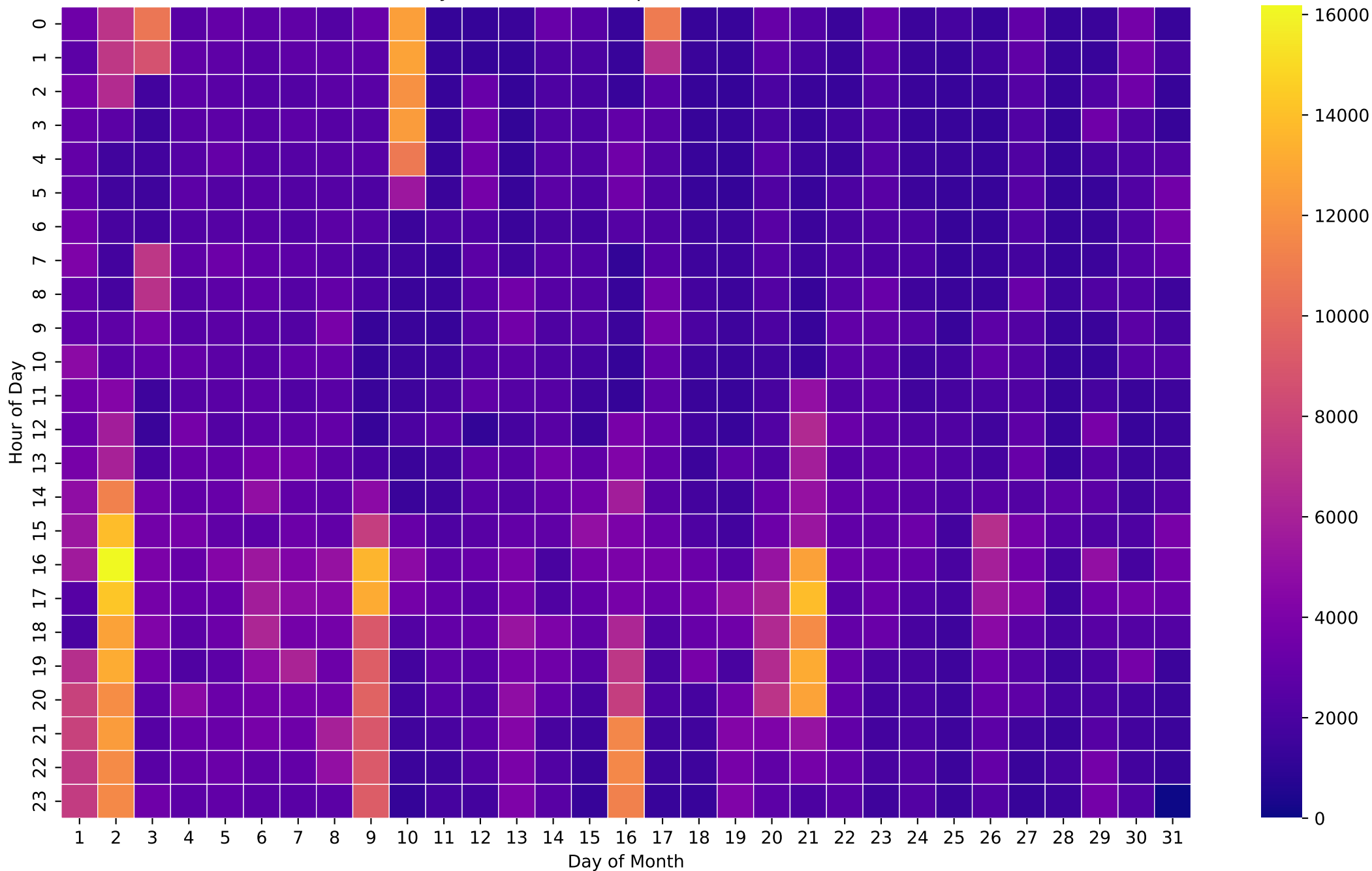
Electricity Demand Heatmap (Wh/Hour) - 5kWh - Dec
