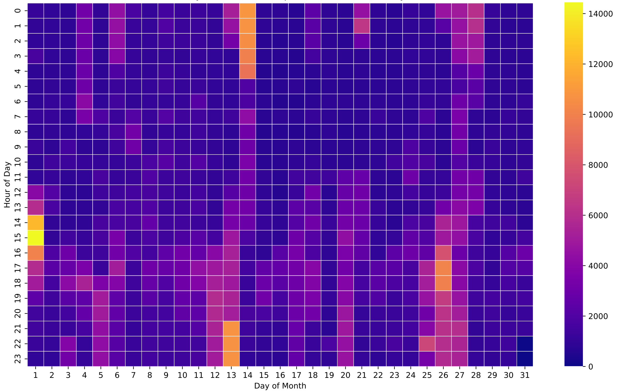
Electricity Demand Heatmap (Wh/Hour) - 5kWh - May
