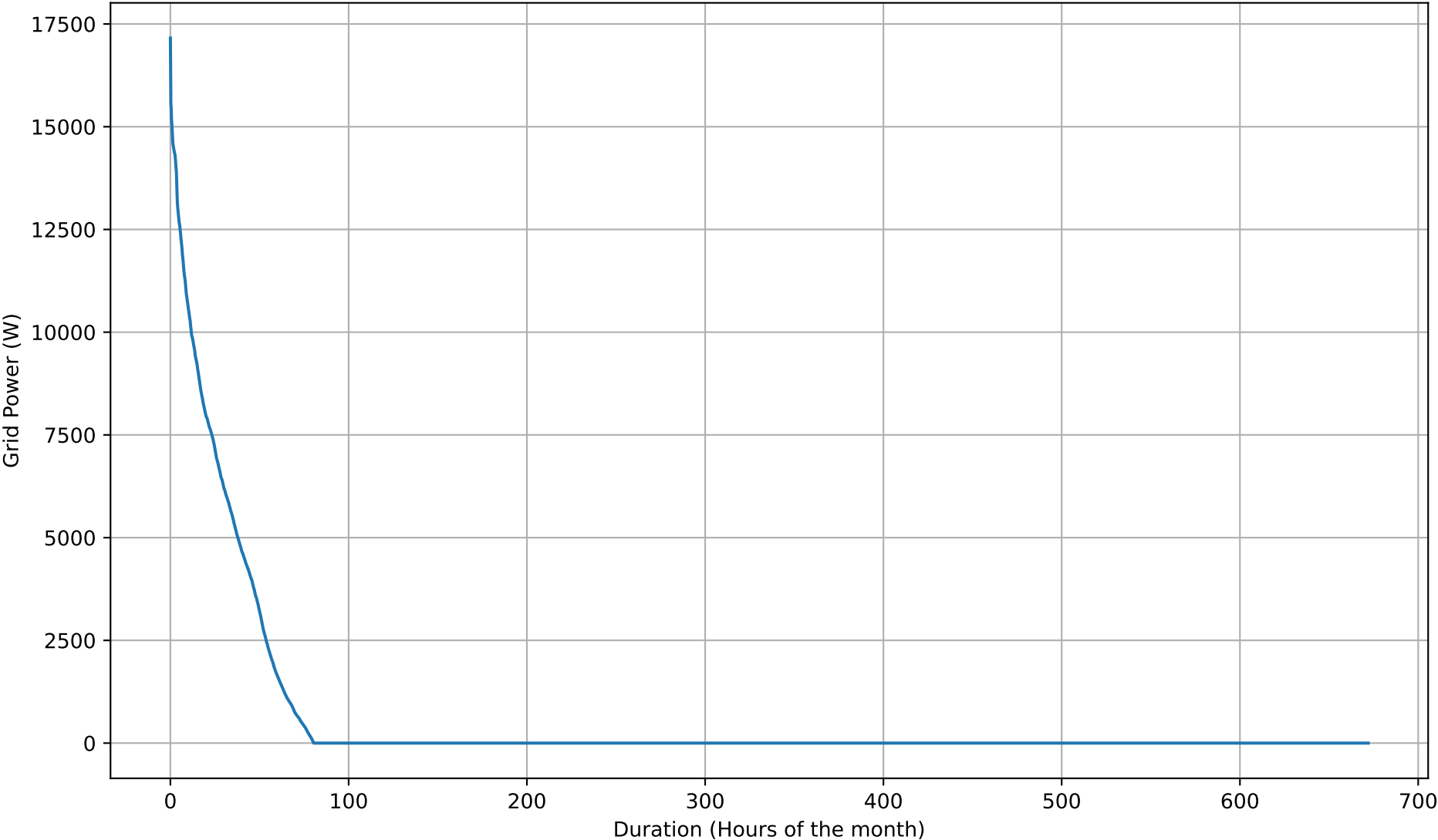
Grid Export Duration Curve - 5kWh - Feb
