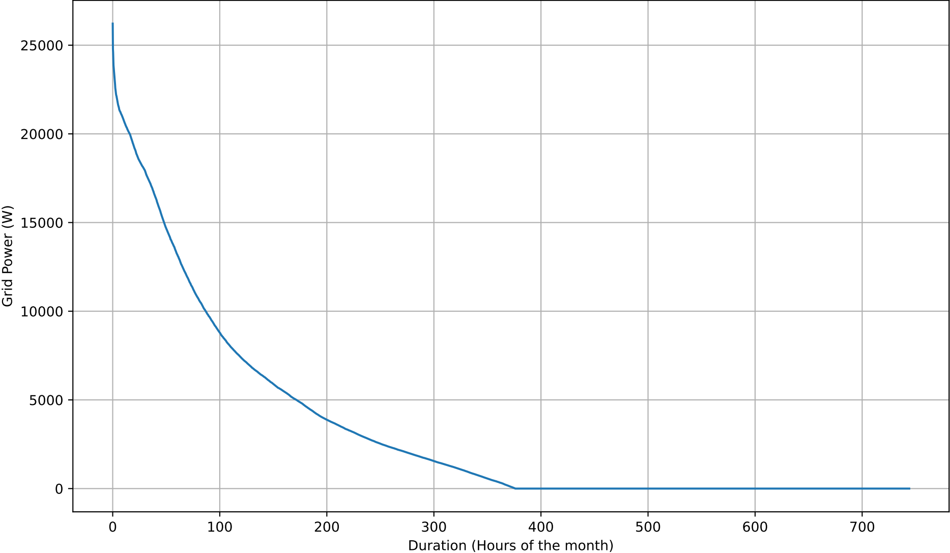
Grid Export Duration Curve - 5kWh - Jul
