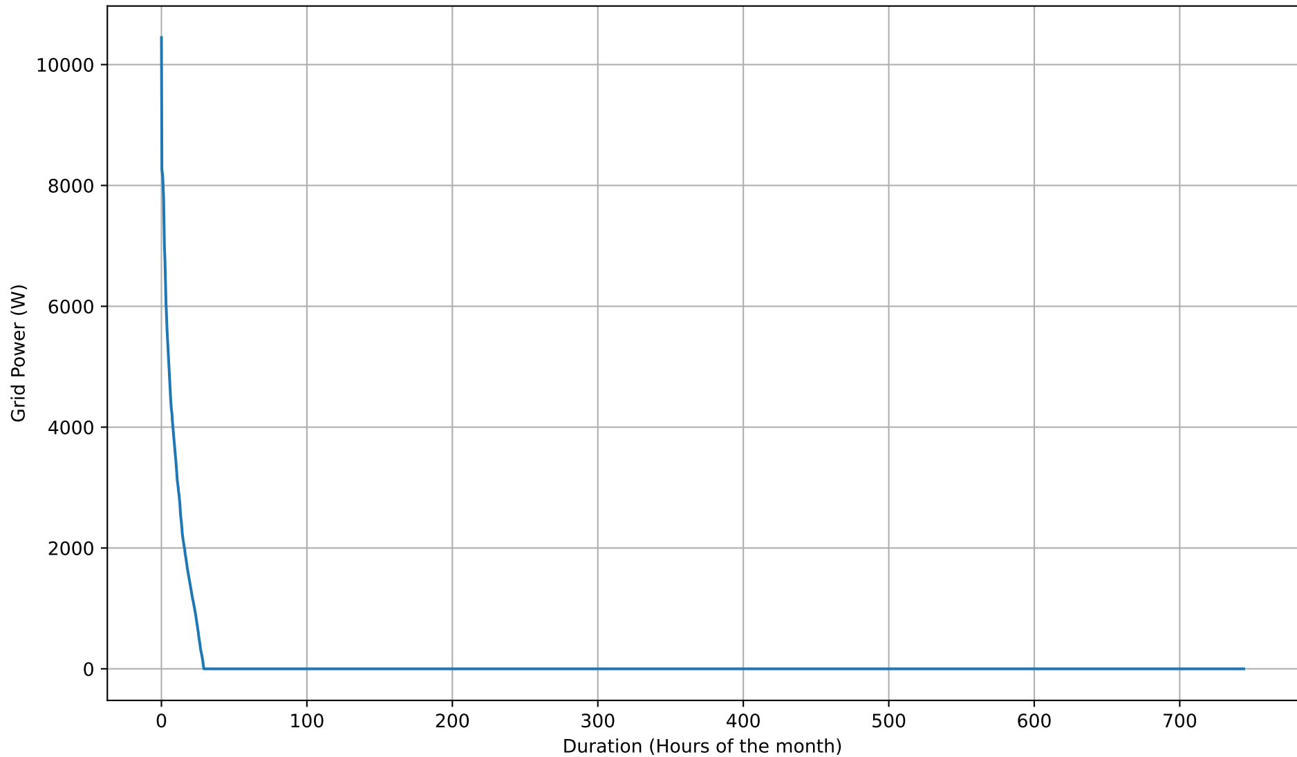
Grid Export Duration Curve - 5kWh - Jan
