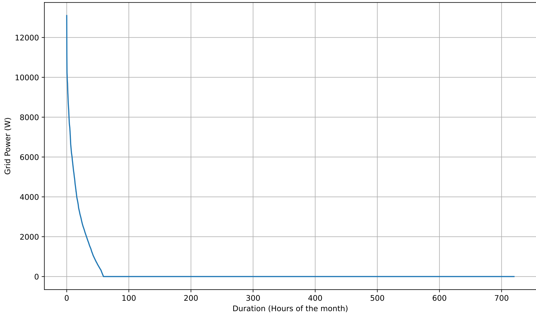
Grid Export Duration Curve - 5kWh - Nov
