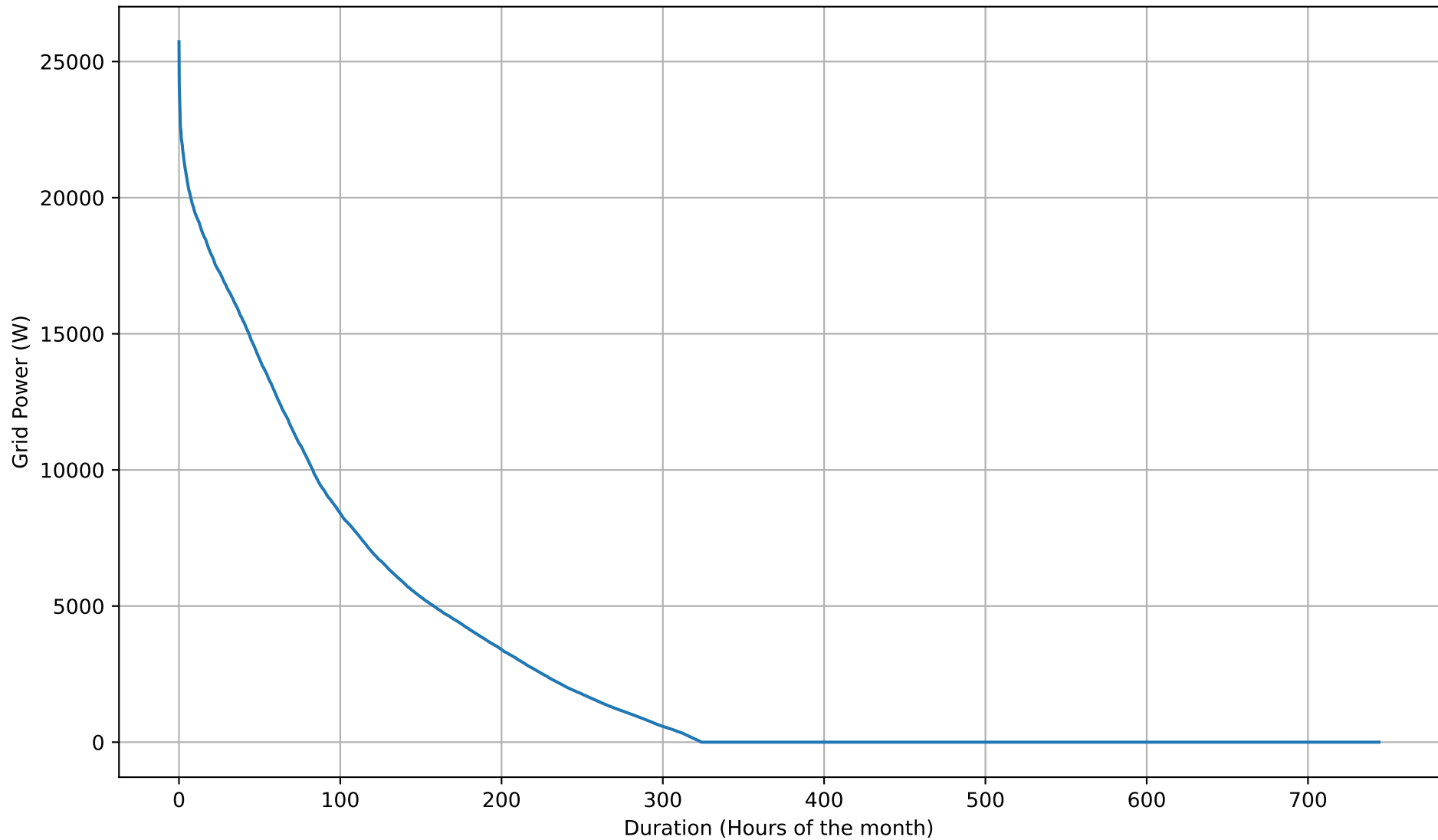
Grid Export Duration Curve - 5kWh - Aug
