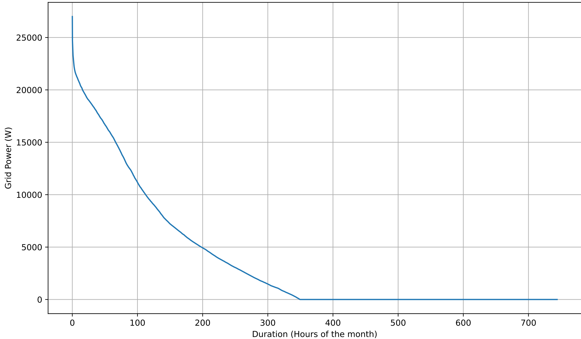
Grid Export Duration Curve - 5kWh - May
