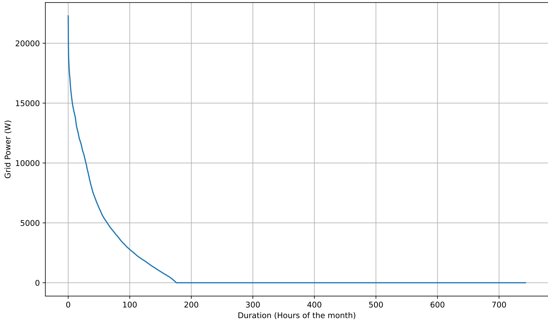
Grid Export Duration Curve - 5kWh - Mar
