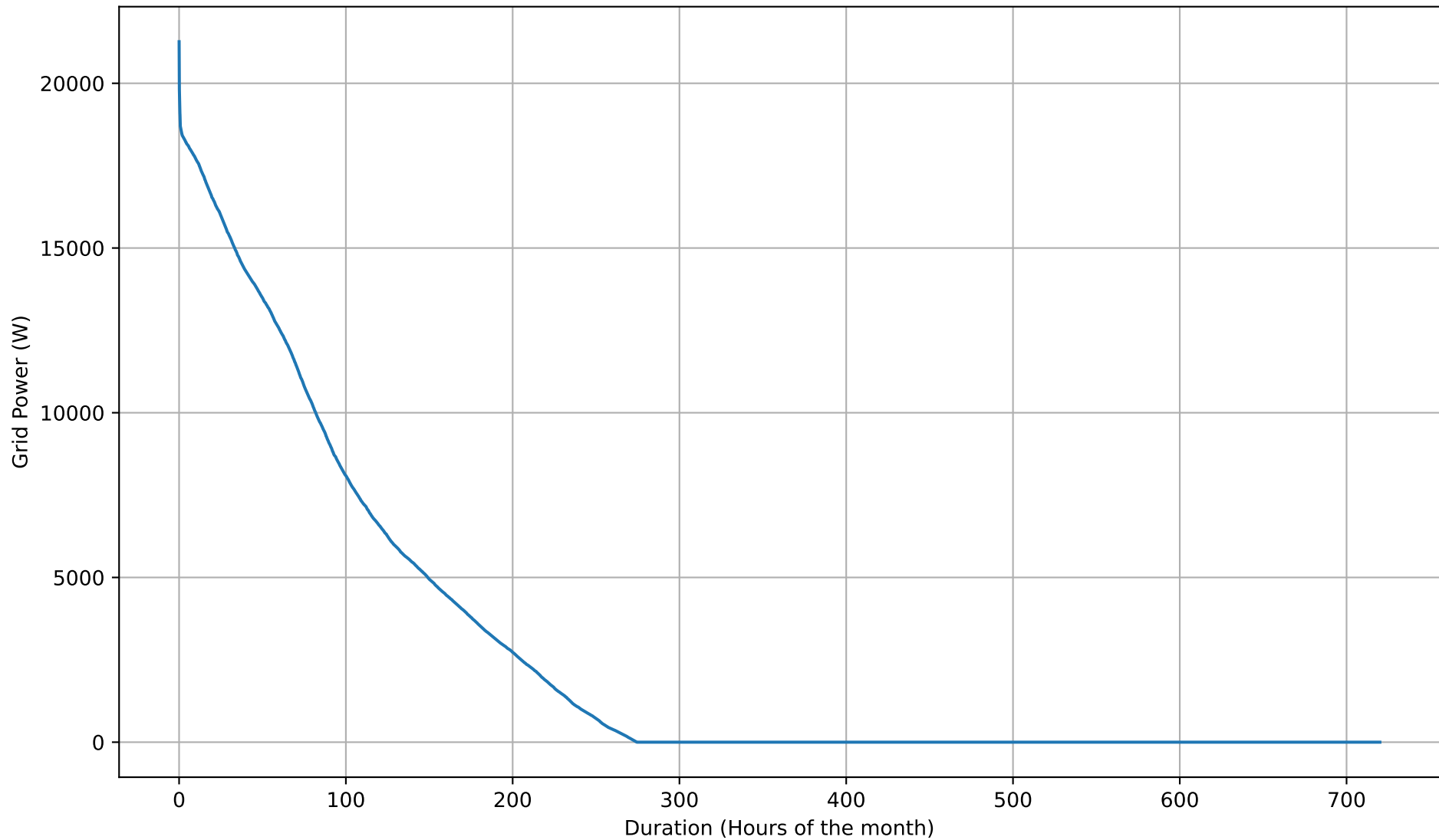
Grid Export Duration Curve - 5kWh - Sep
