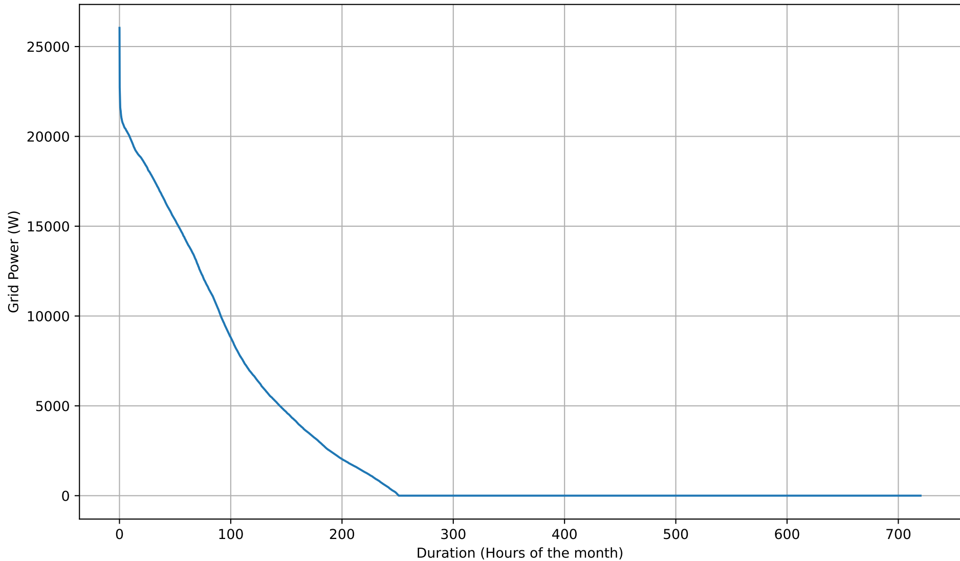
Grid Export Duration Curve - 5kWh - Apr
