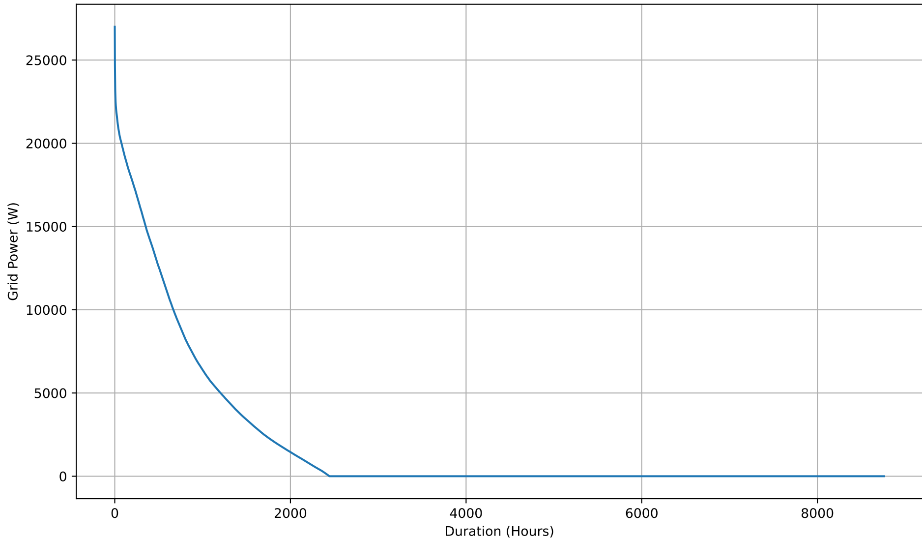
Yearly Grid Export Duration Curve - 5kWh
