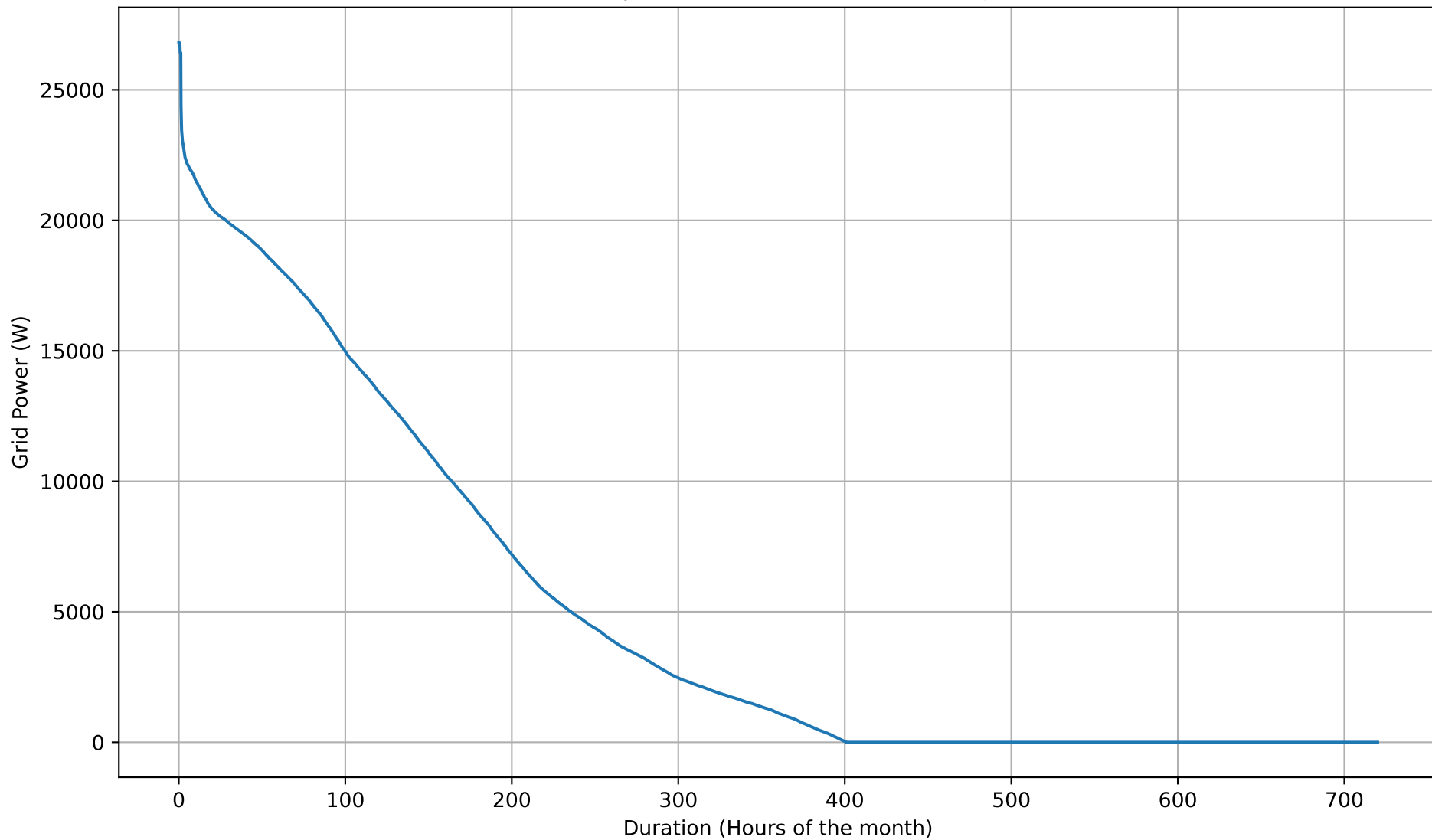
Grid Export Duration Curve - 5kWh - Jun
