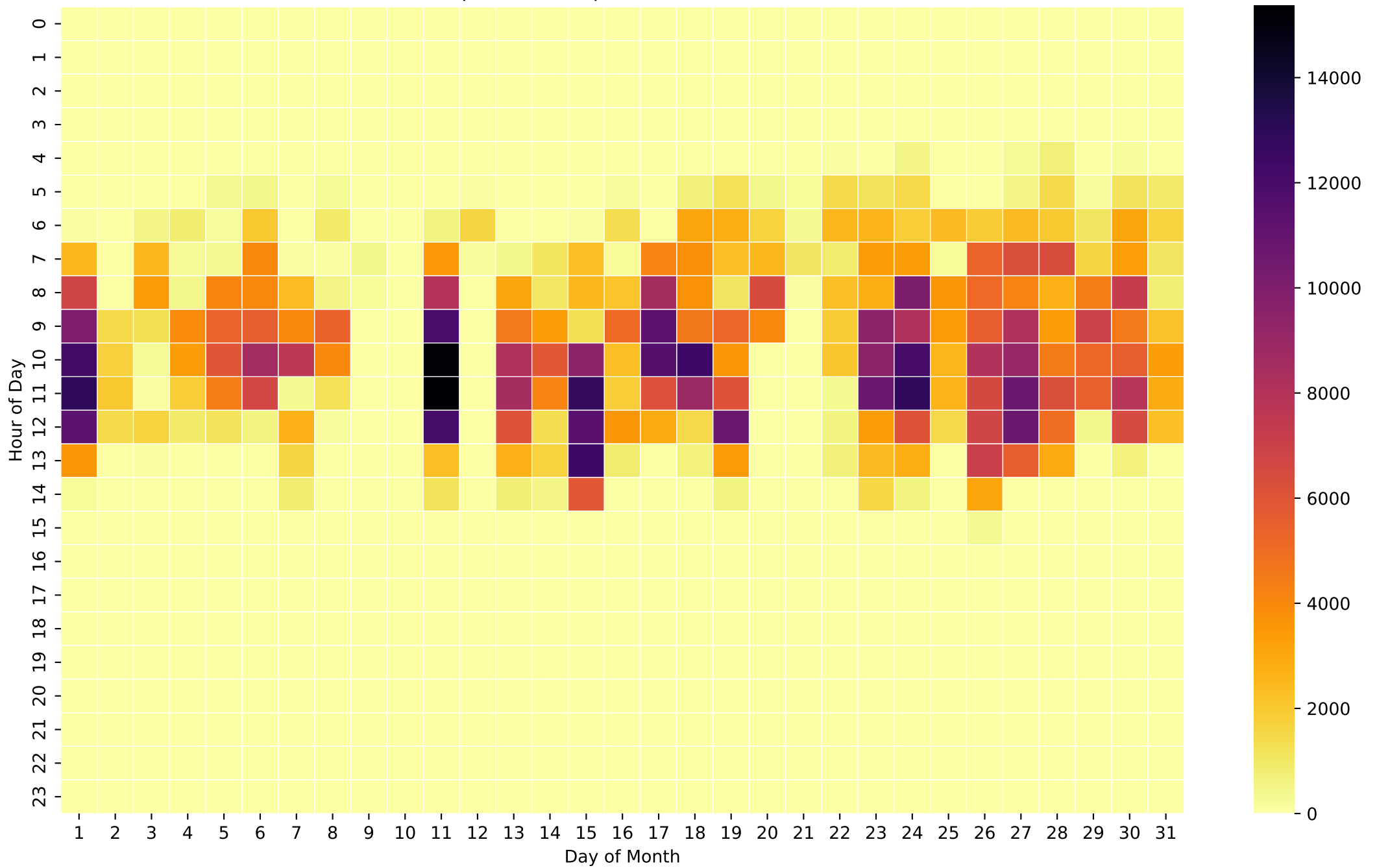
Grid Export Heatmap (Wh/Hour) - 5kWh - Mar
