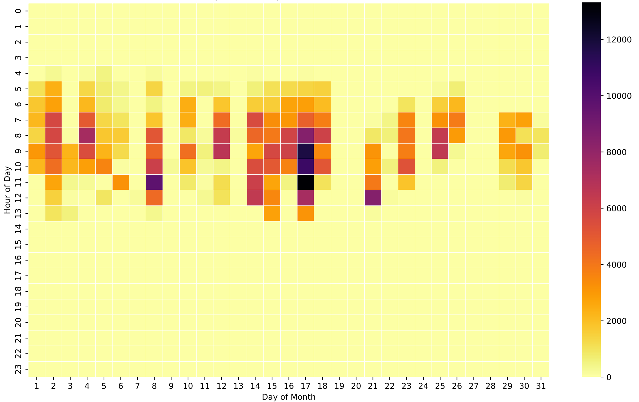
Grid Export Heatmap (Wh/Hour) - 5kWh - Oct
