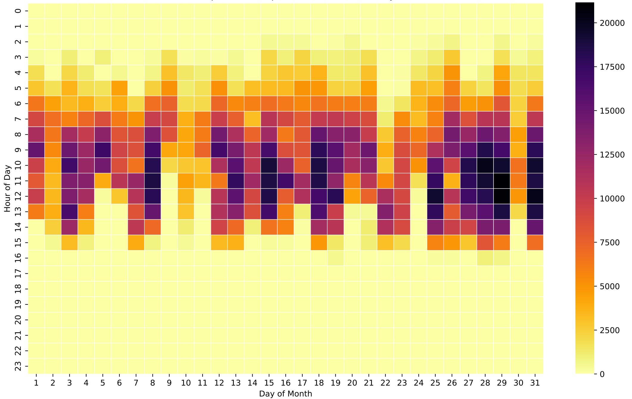
Grid Export Heatmap (Wh/Hour) - 5kWh - May
