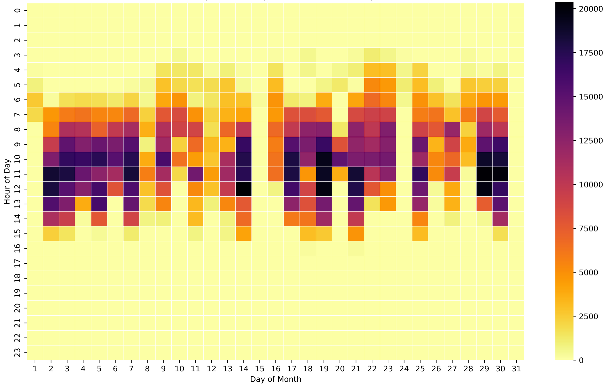
Grid Export Heatmap (Wh/Hour) - 5kWh - Apr
