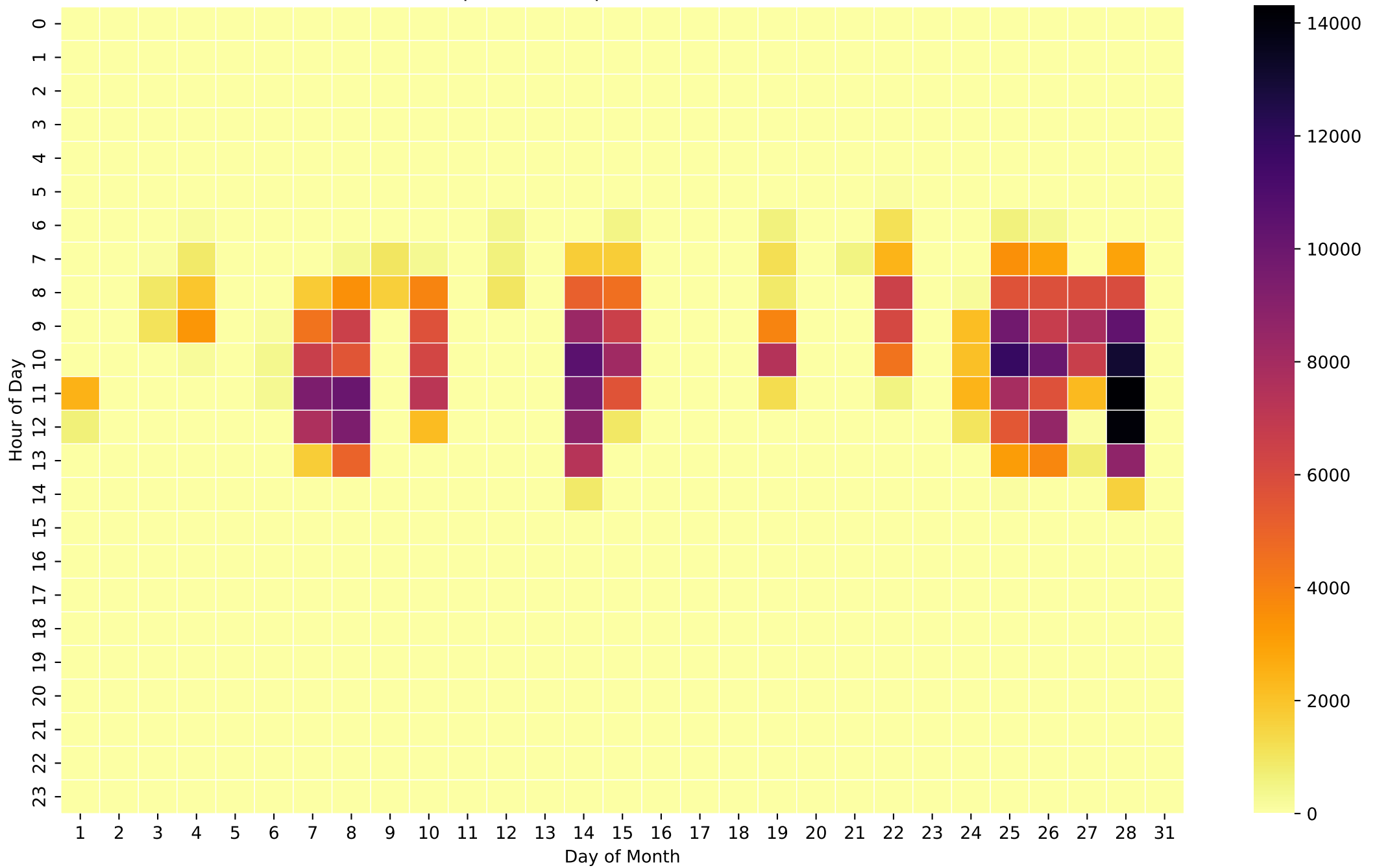
Grid Export Heatmap (Wh/Hour) - 5kWh - Feb
