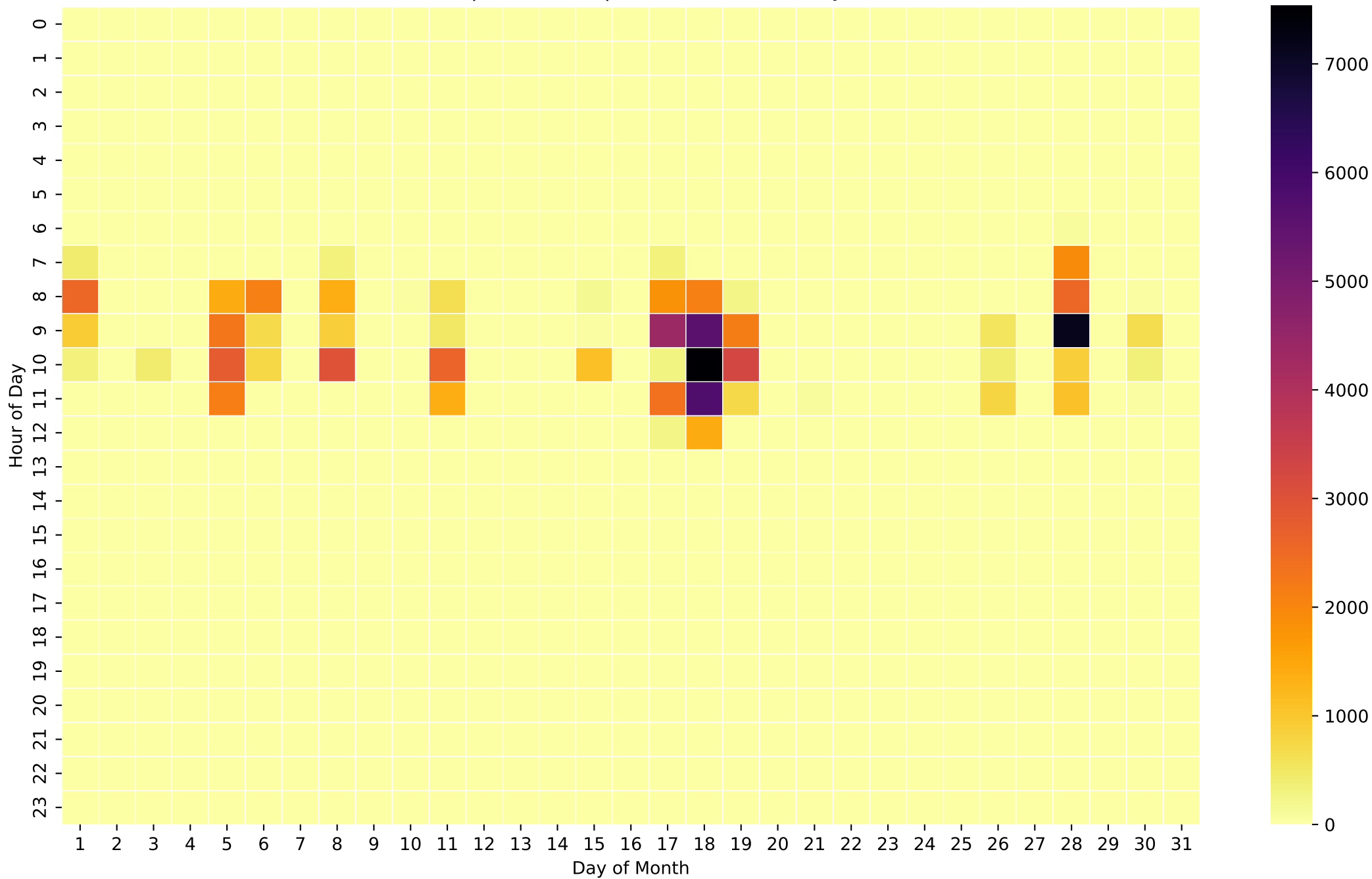
Grid Export Heatmap (Wh/Hour) - 5kWh - Jan
