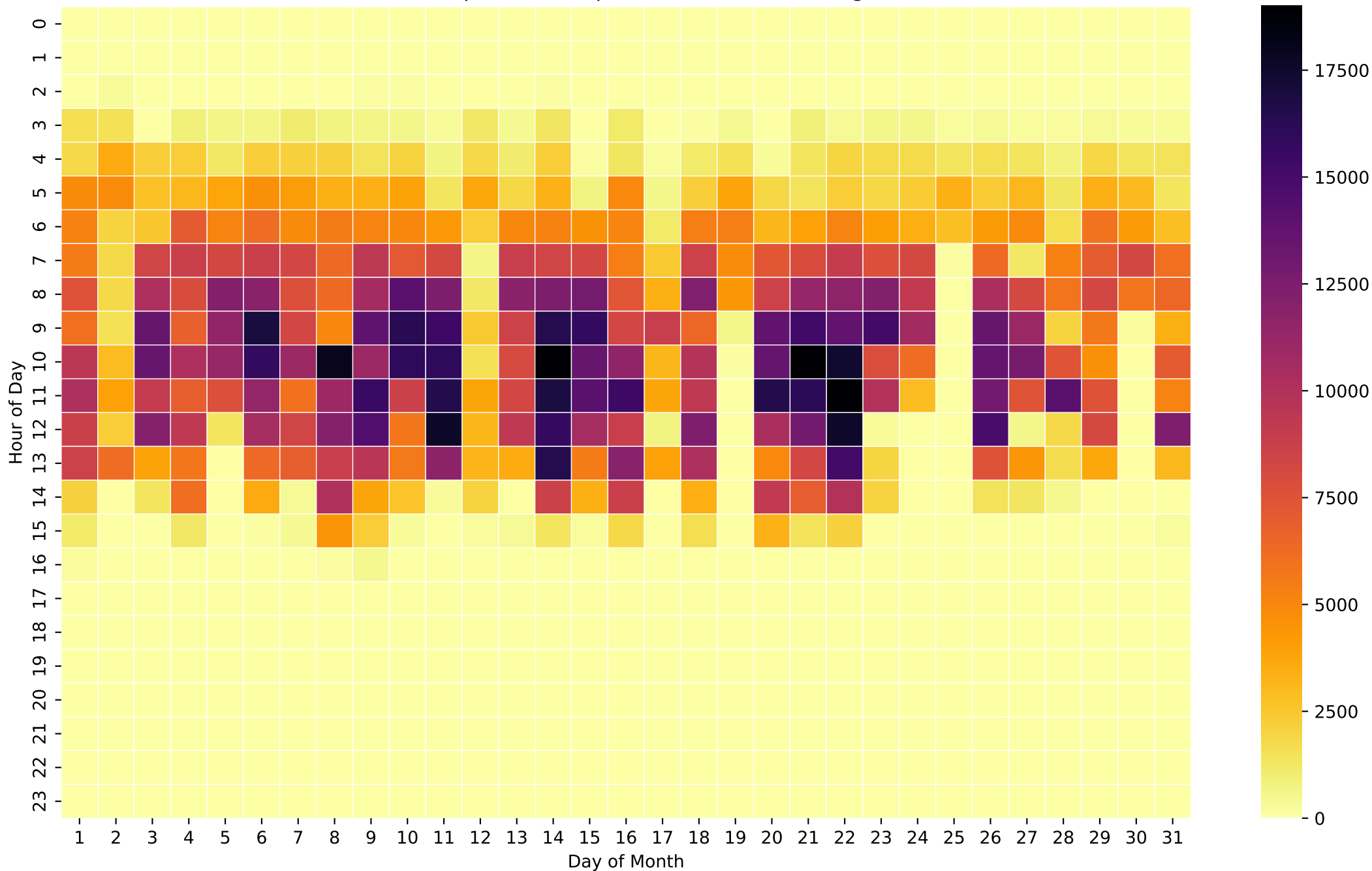
Grid Export Heatmap (Wh/Hour) - 5kWh - Aug
