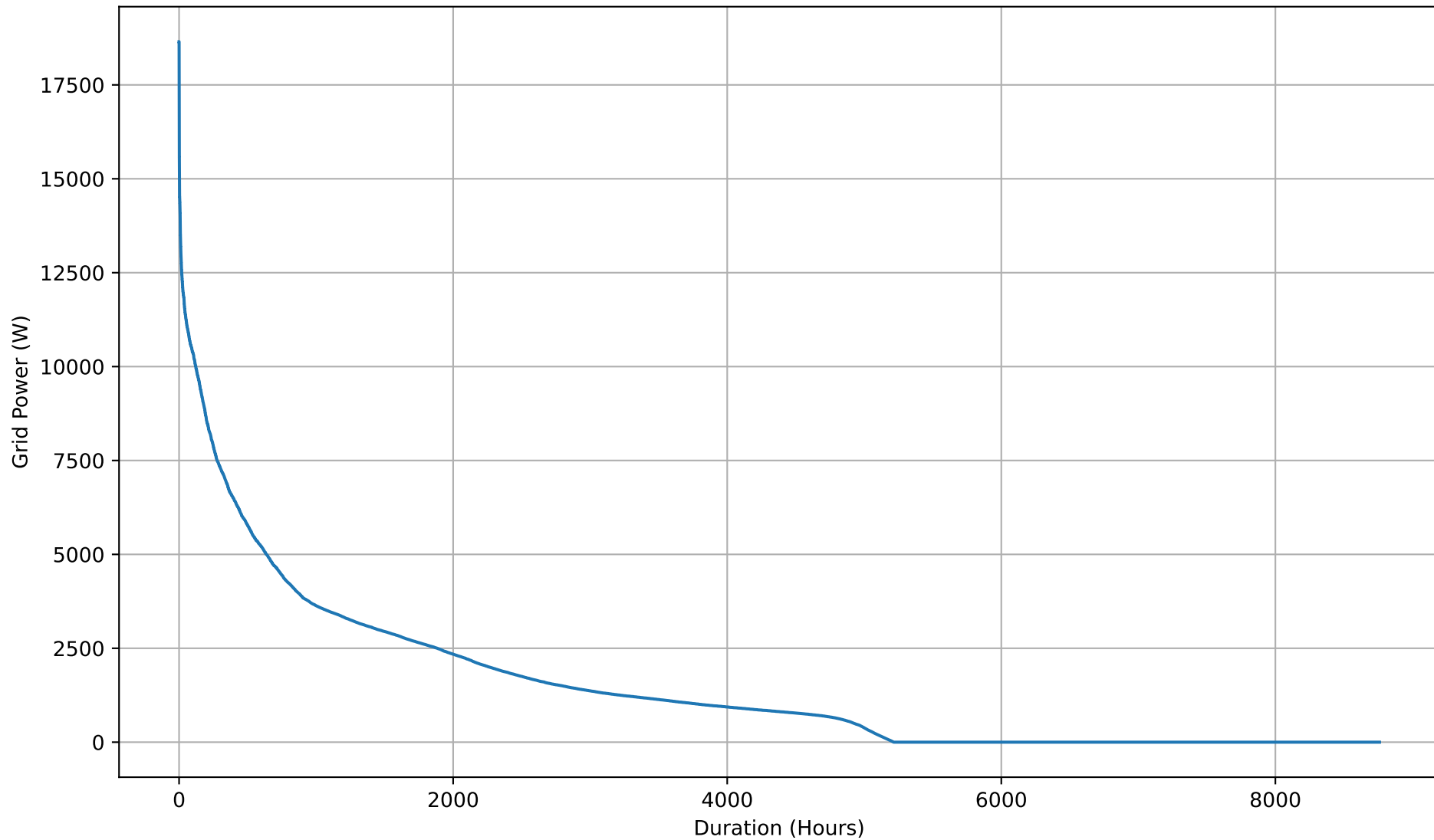
Yearly Grid Import Duration Curve - 5kWh
