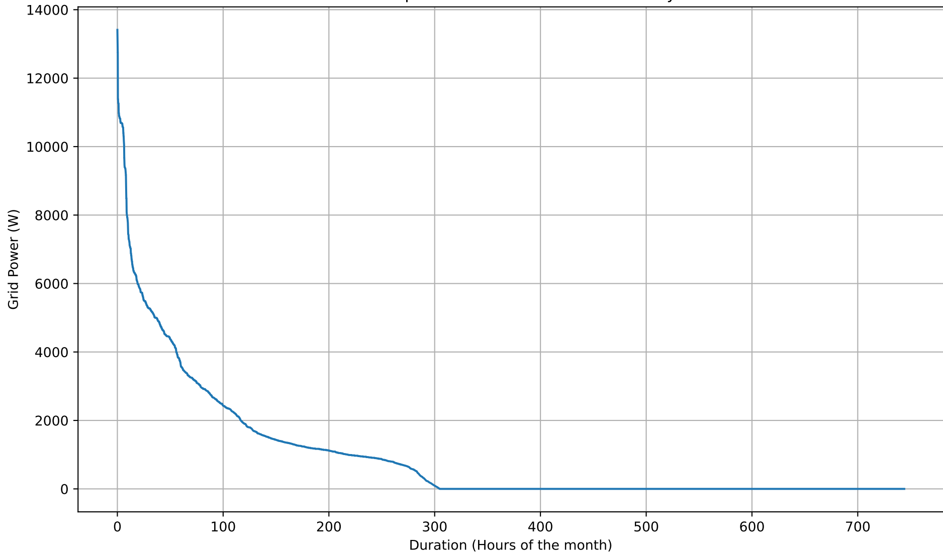
Grid Import Duration Curve - 5kWh - May
