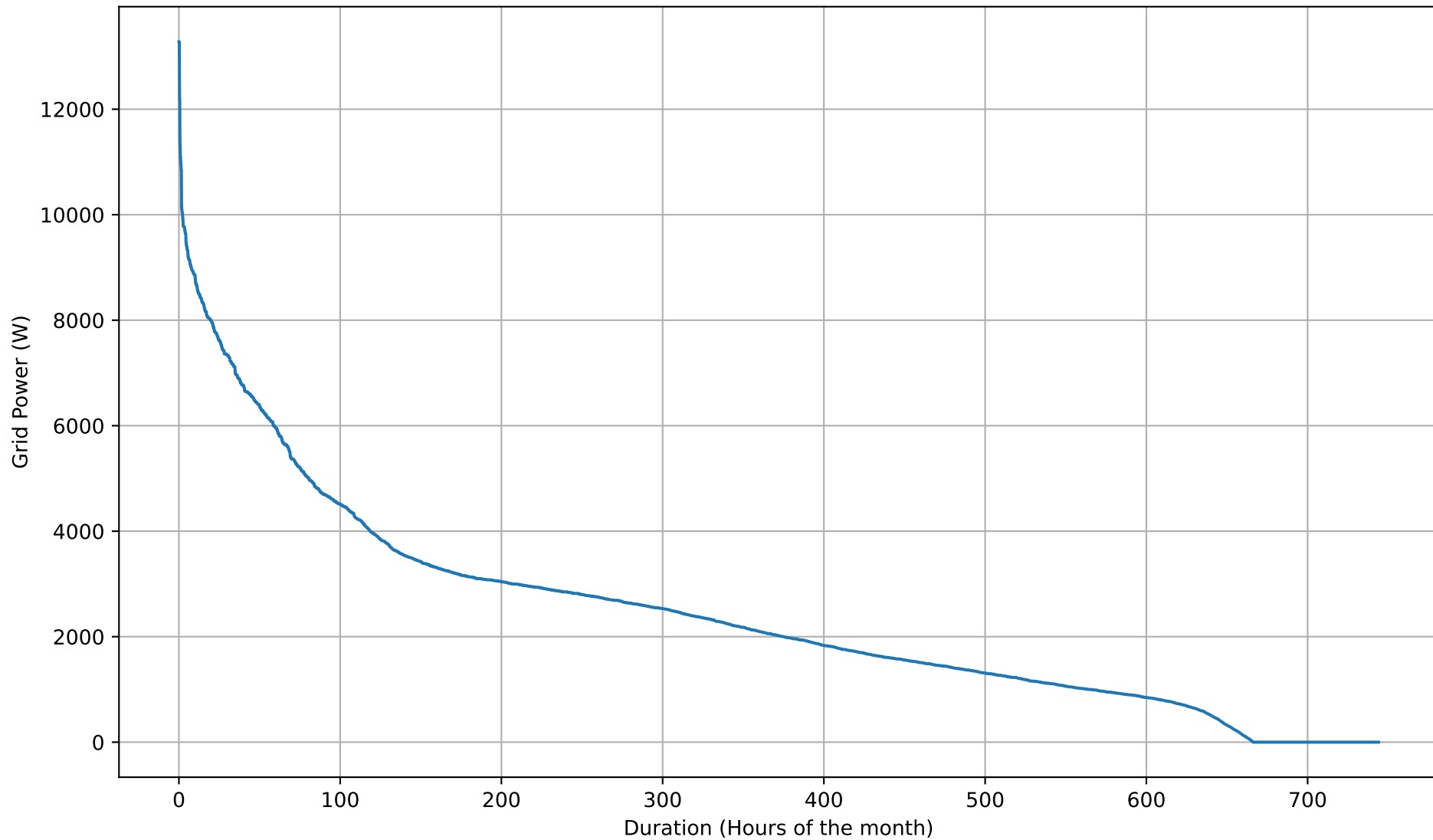
Grid Import Duration Curve - 5kWh - Jan
