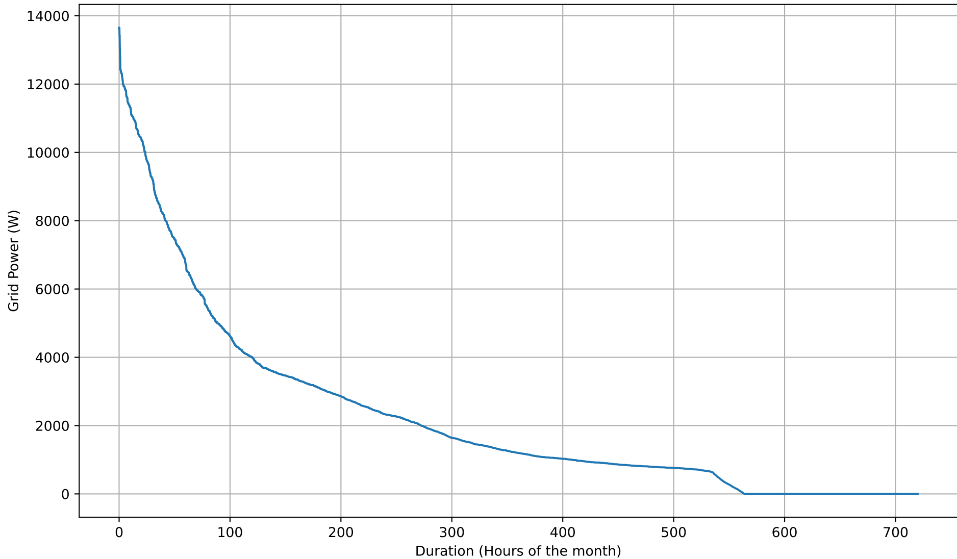
Grid Import Duration Curve - 5kWh - Nov
