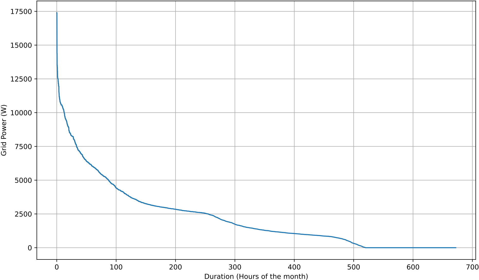
Grid Import Duration Curve - 5kWh - Feb
