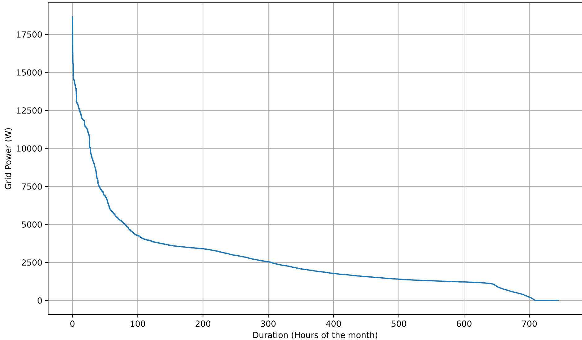
Grid Import Duration Curve - 5kWh - Dec
