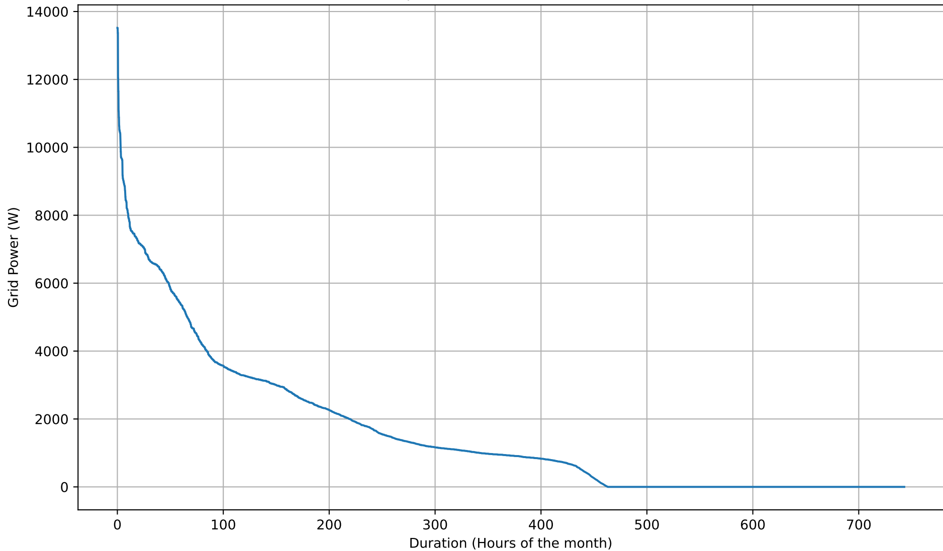
Grid Import Duration Curve - 5kWh - Mar
