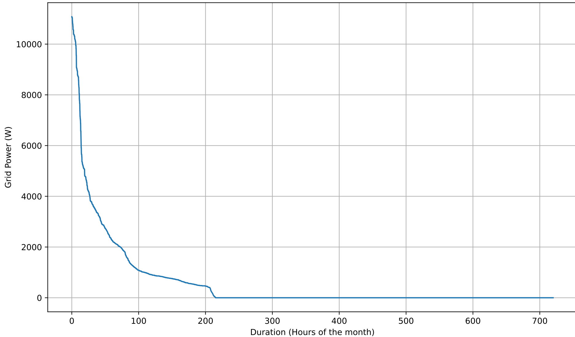
Grid Import Duration Curve - 5kWh - Jun
