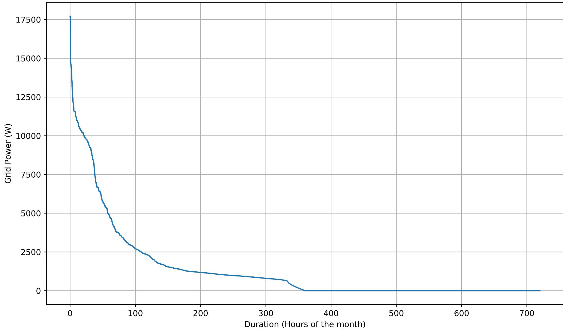
Grid Import Duration Curve - 5kWh - Sep
