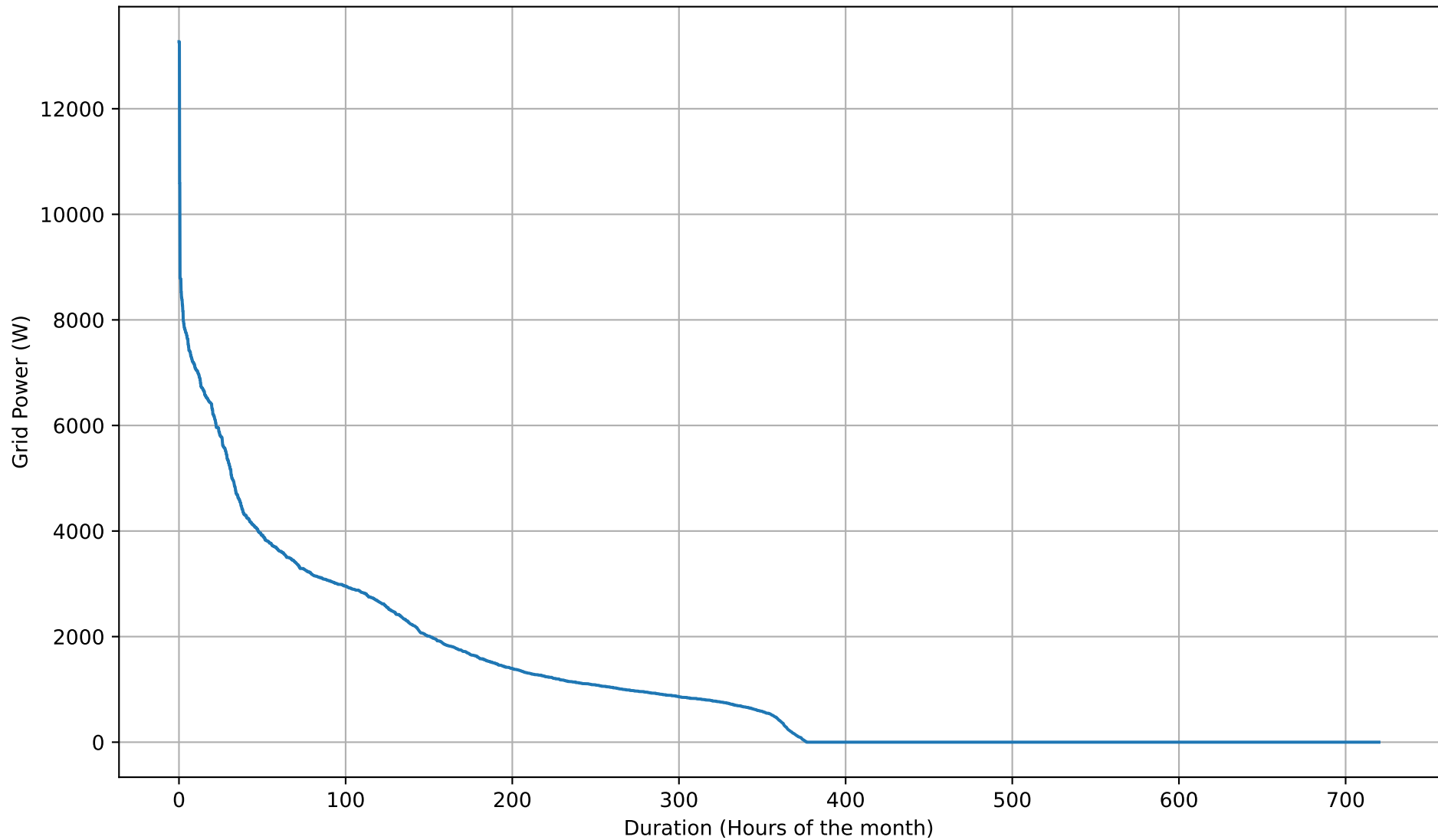
Grid Import Duration Curve - 5kWh - Apr
