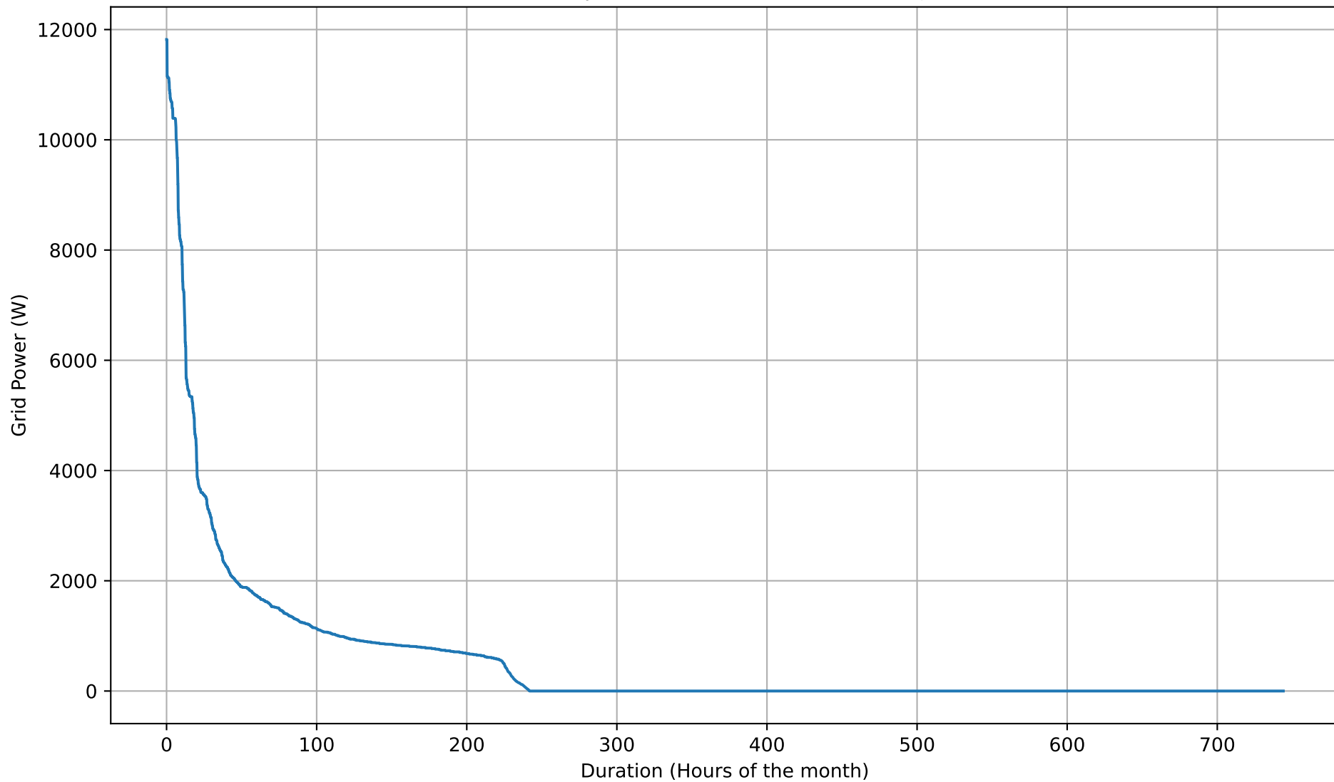
Grid Import Duration Curve - 5kWh - Jul
