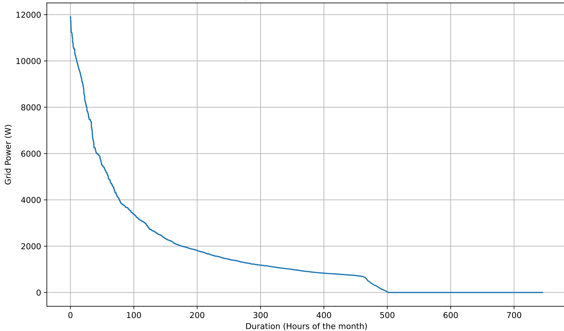
Grid Import Duration Curve - 5kWh - Oct
