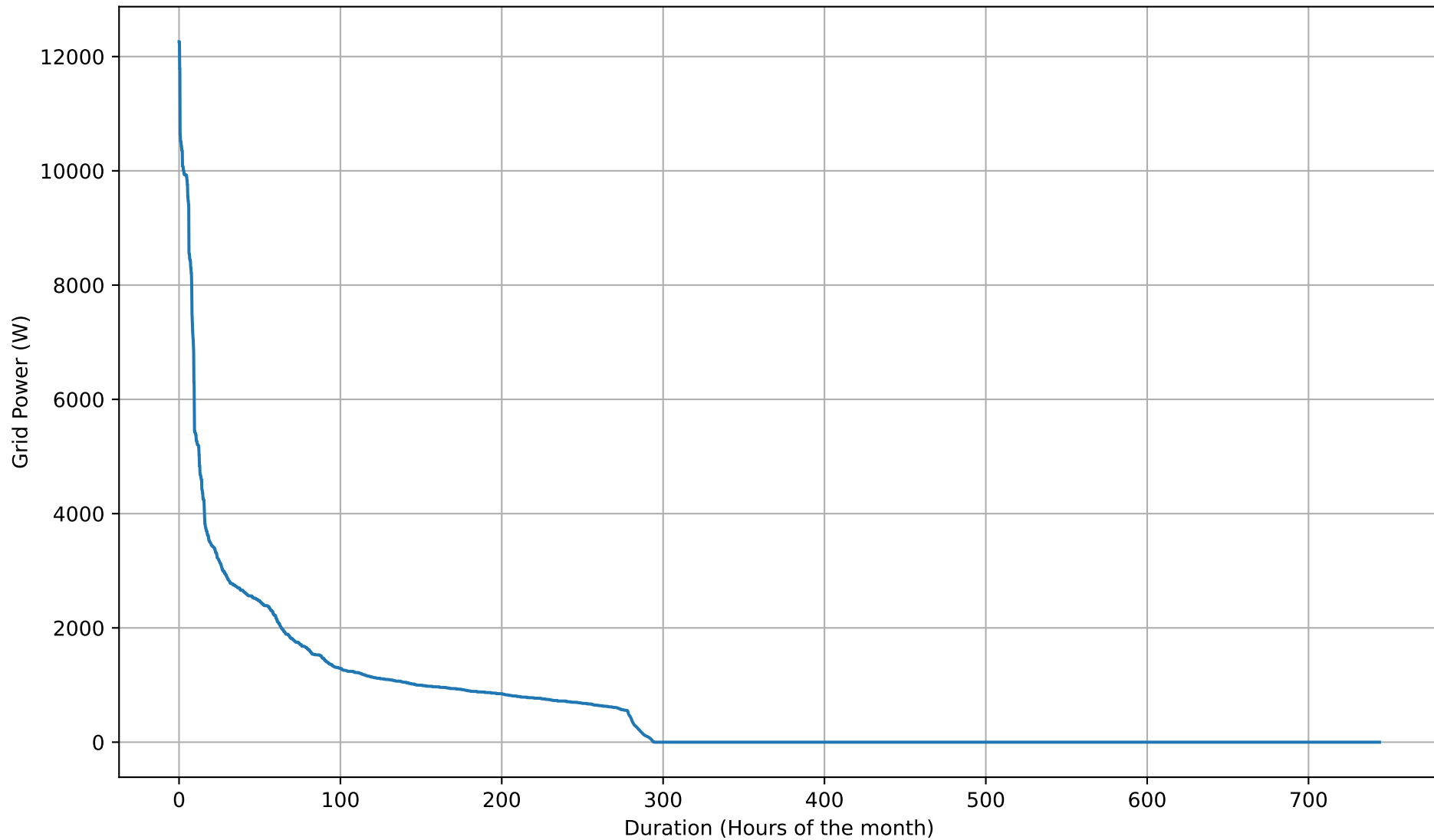
Grid Import Duration Curve - 5kWh - Aug
