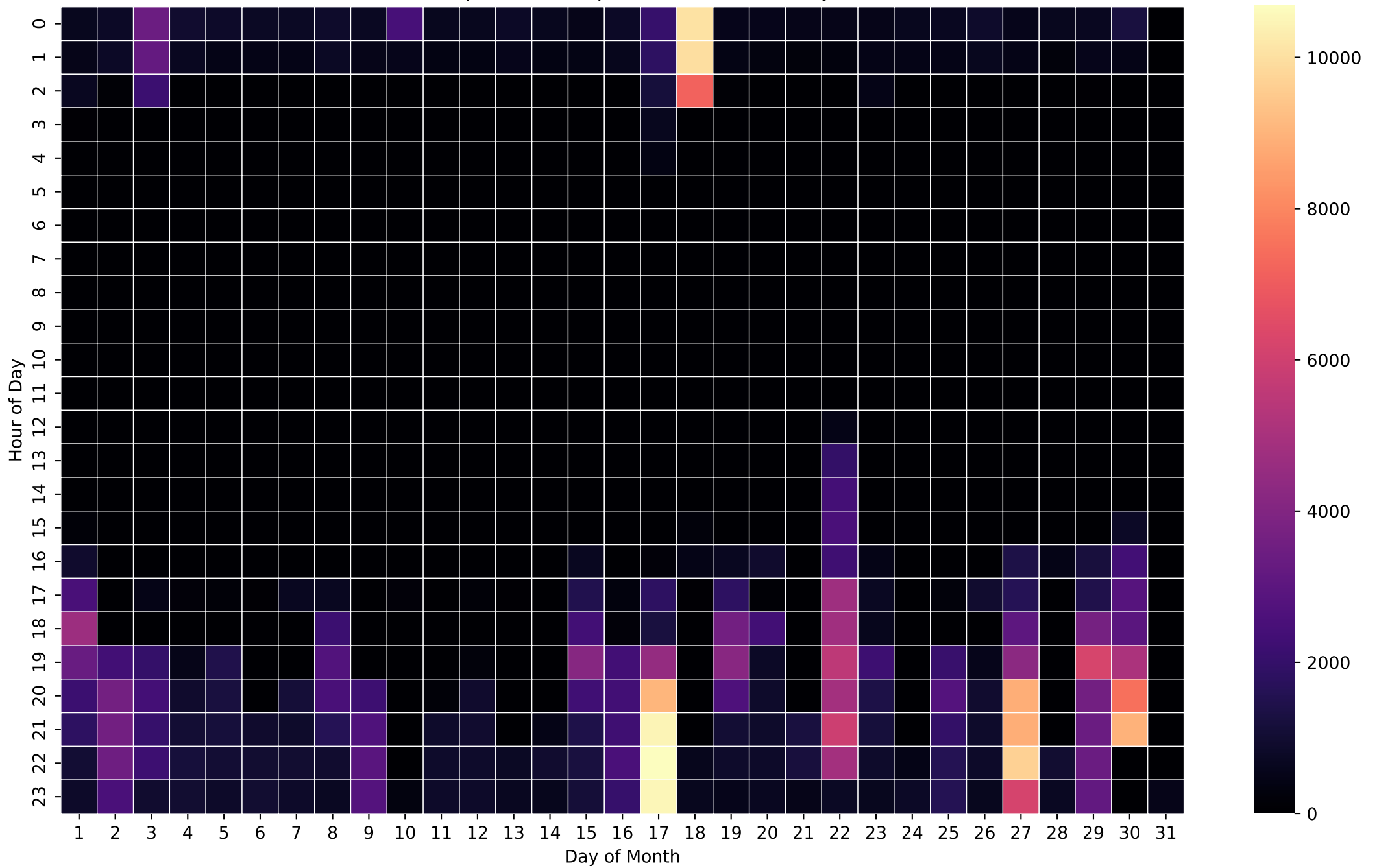
Grid Import Heatmap (Wh/Hour) - 5kWh - Jun
