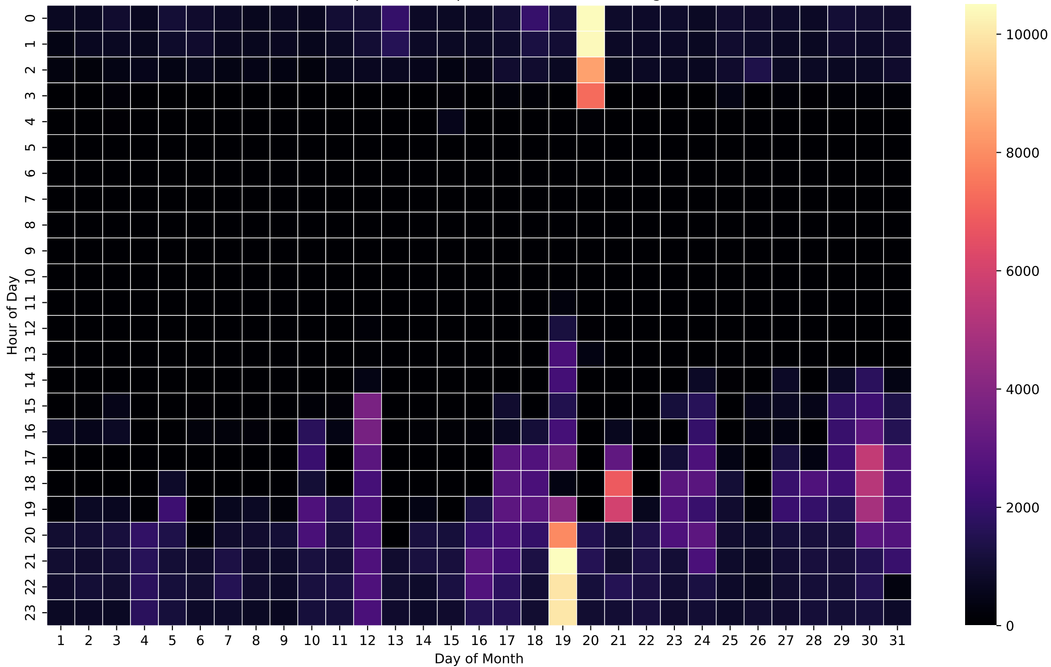
Grid Import Heatmap (Wh/Hour) - 5kWh - Aug
