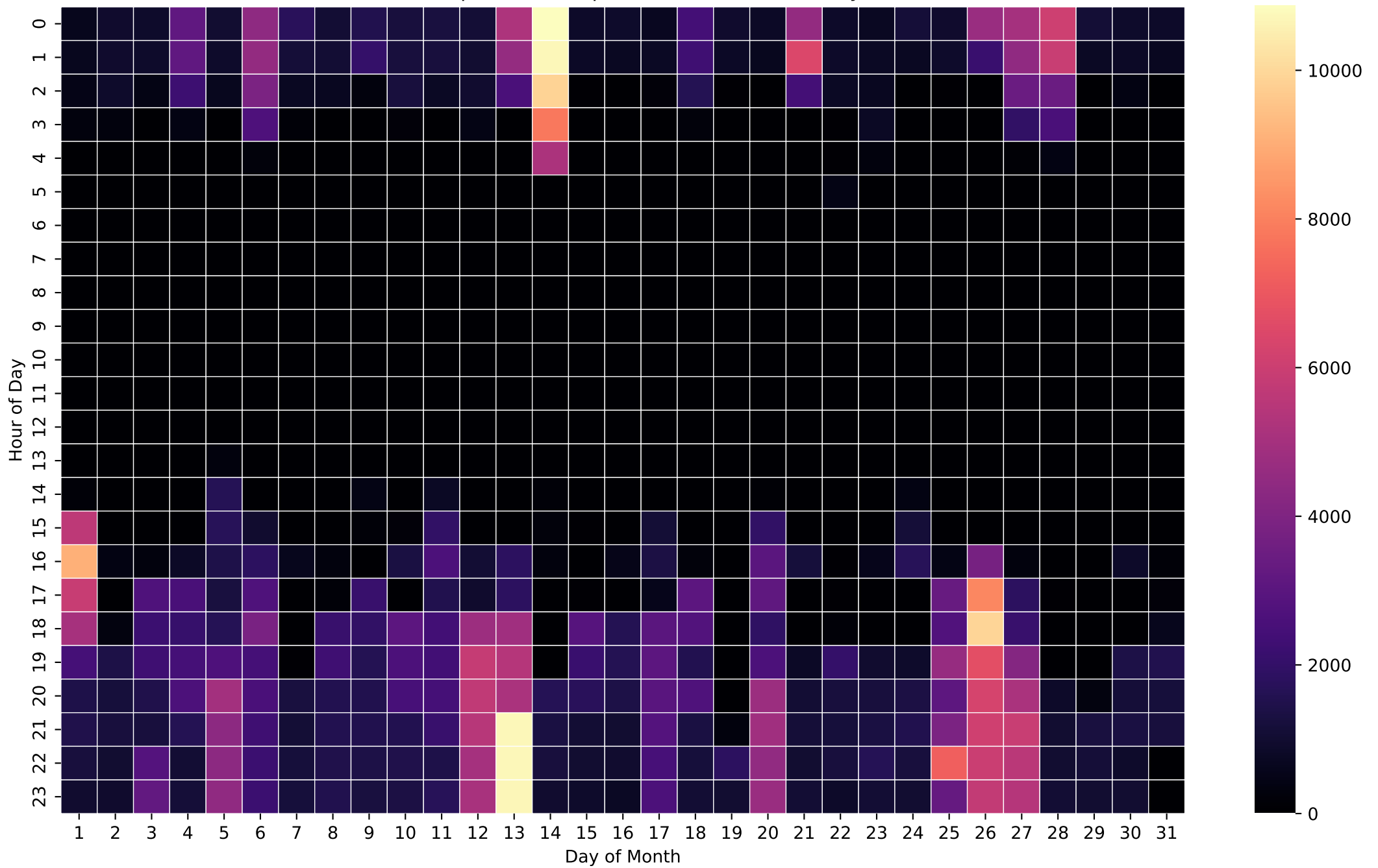
Grid Import Heatmap (Wh/Hour) - 5kWh - May
