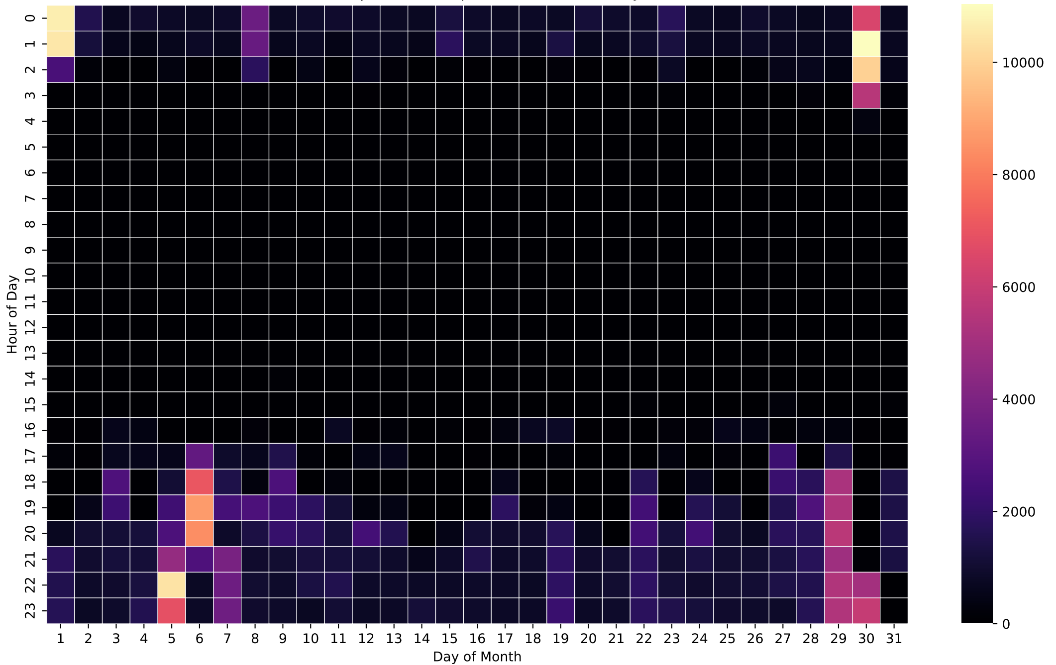
Grid Import Heatmap (Wh/Hour) - 5kWh - Jul
