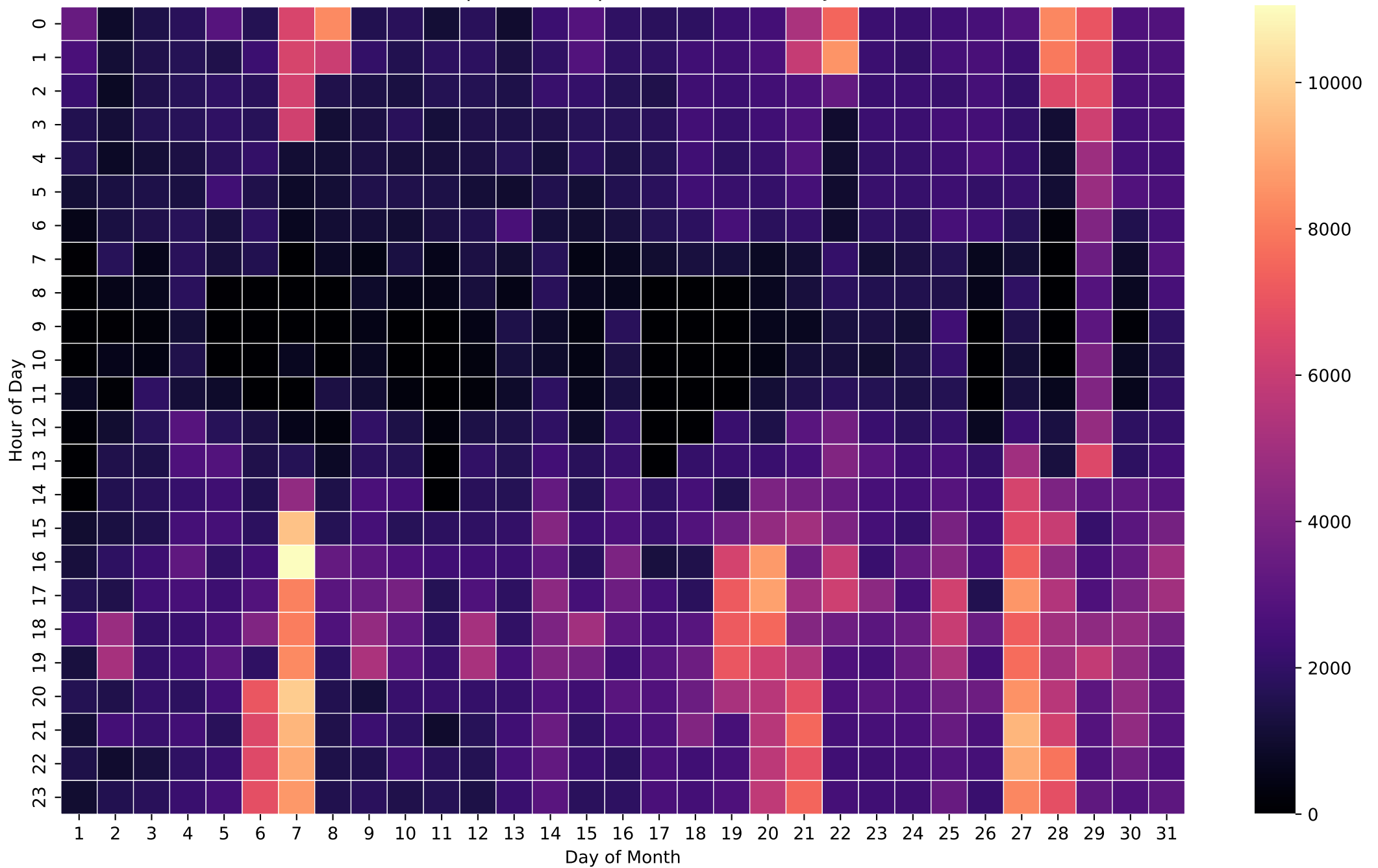
Grid Import Heatmap (Wh/Hour) - 5kWh - Jan
