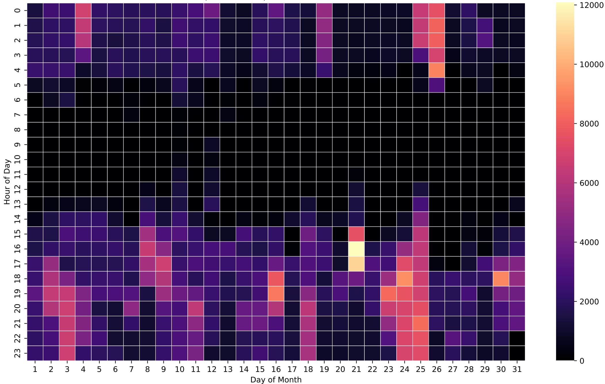
Grid Import Heatmap (Wh/Hour) - 5kWh - Mar
