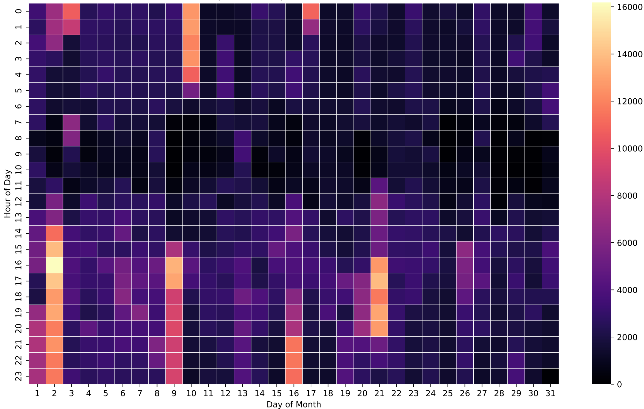
Grid Import Heatmap (Wh/Hour) - 5kWh - Dec
