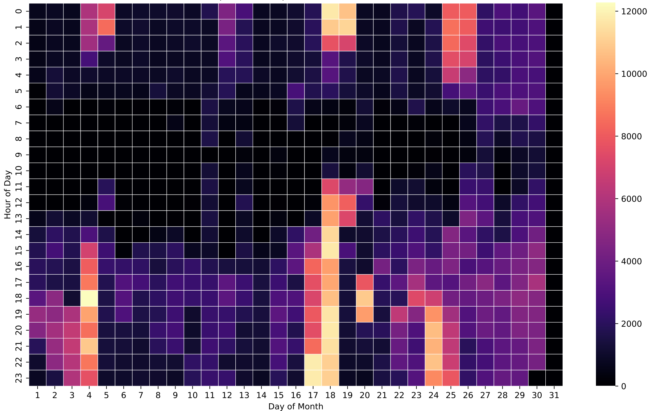
Grid Import Heatmap (Wh/Hour) - 5kWh - Nov
