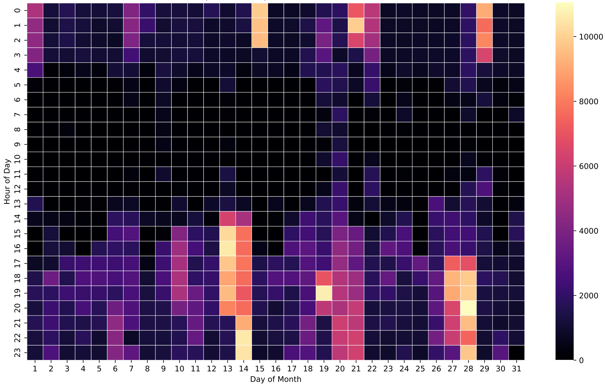
Grid Import Heatmap (Wh/Hour) - 5kWh - Oct
