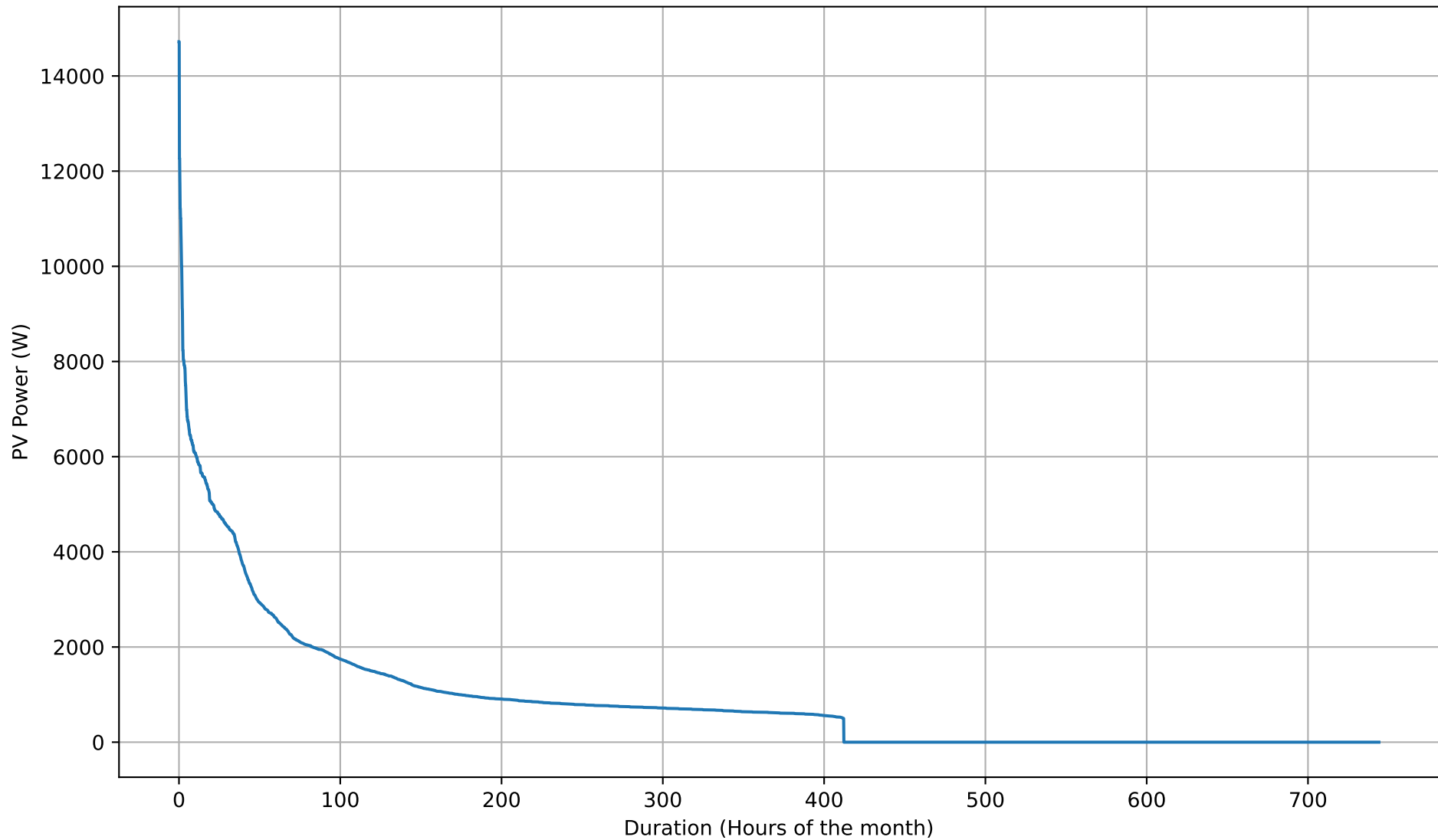
PV Self-Consumption Duration Curve - 5kWh - Aug
