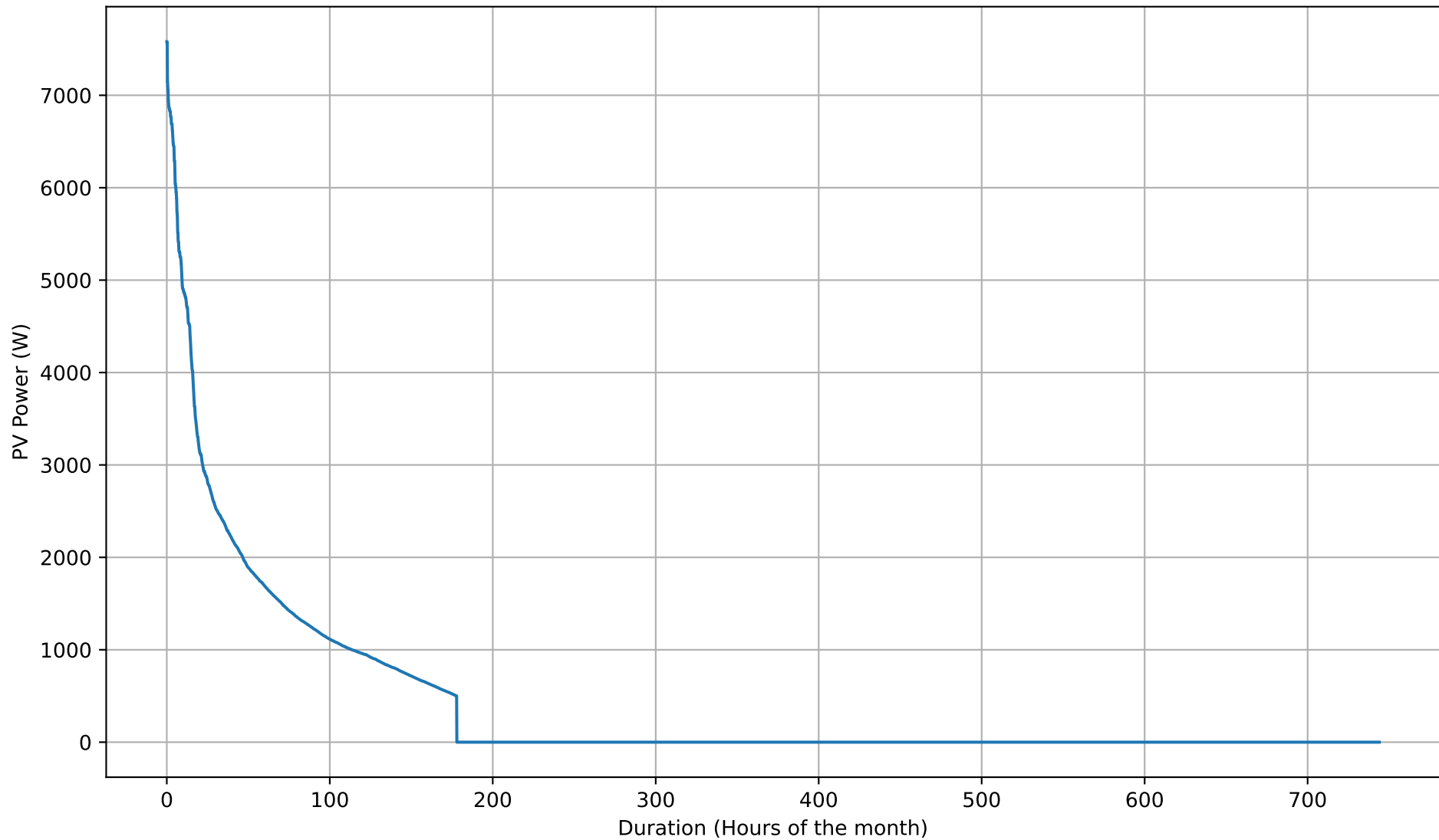
PV Self-Consumption Duration Curve - 5kWh - Jan
