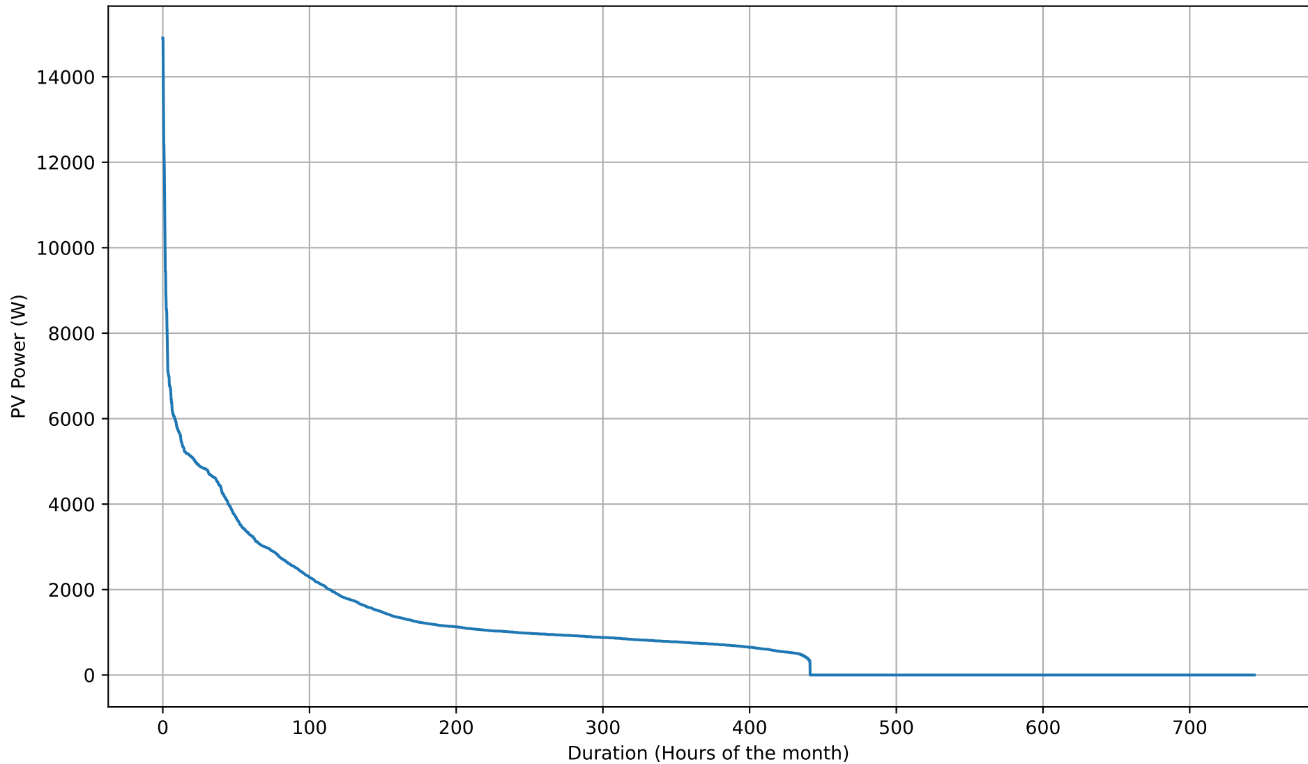
PV Self-Consumption Duration Curve - 5kWh - May
