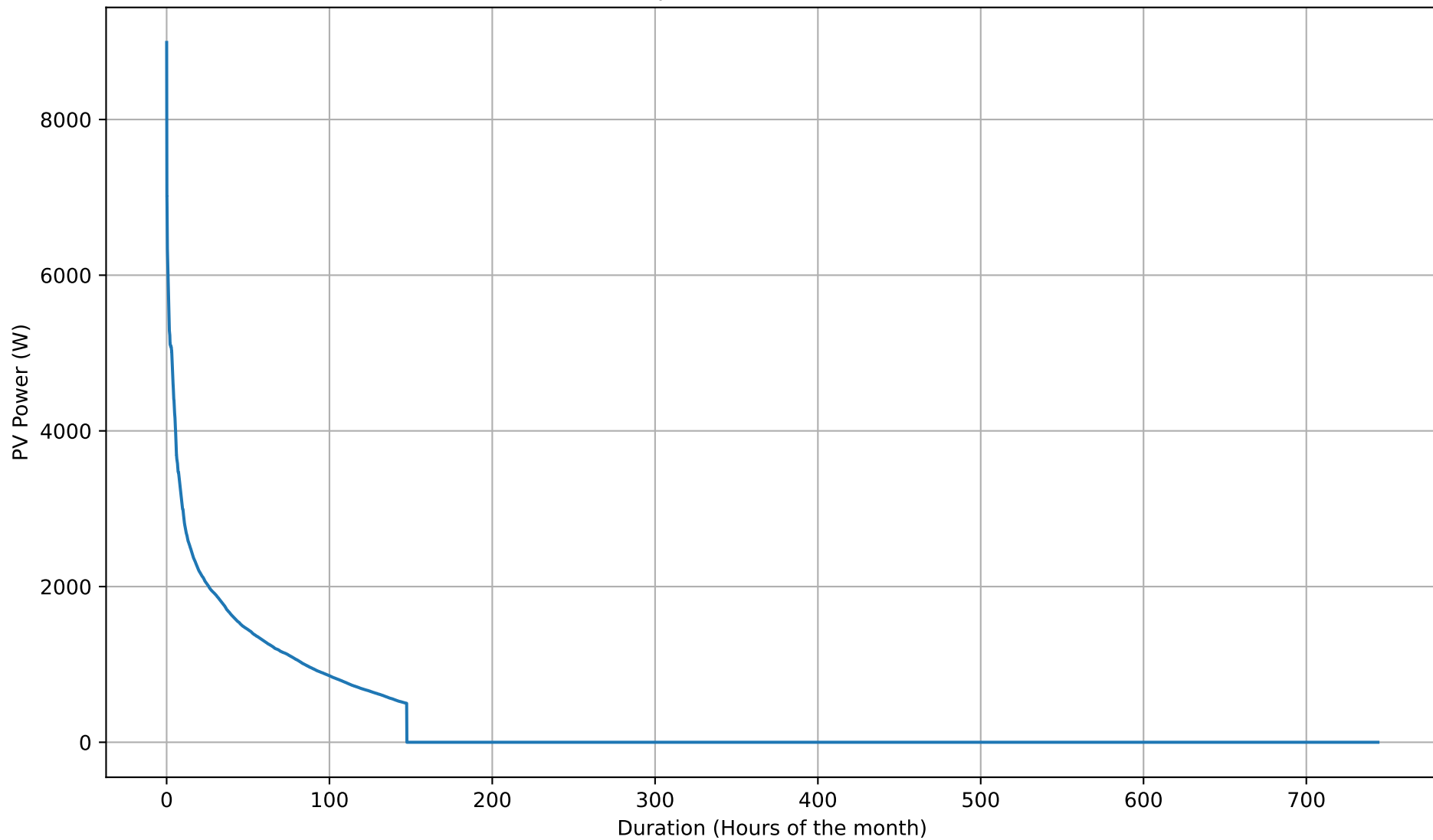
PV Self-Consumption Duration Curve - 5kWh - Dec
