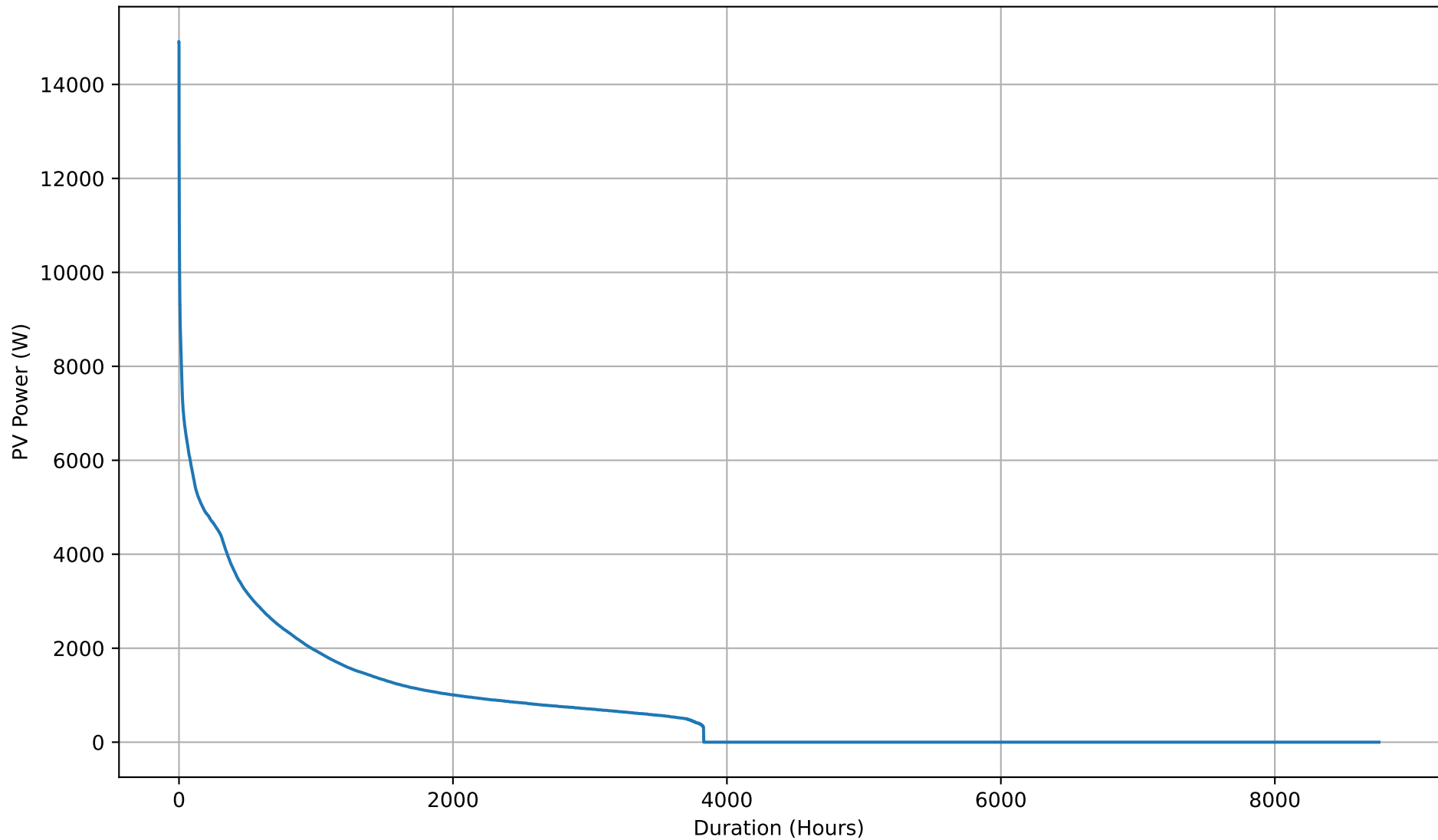
Yearly PV Self-Consumption Duration Curve - 5kWh
