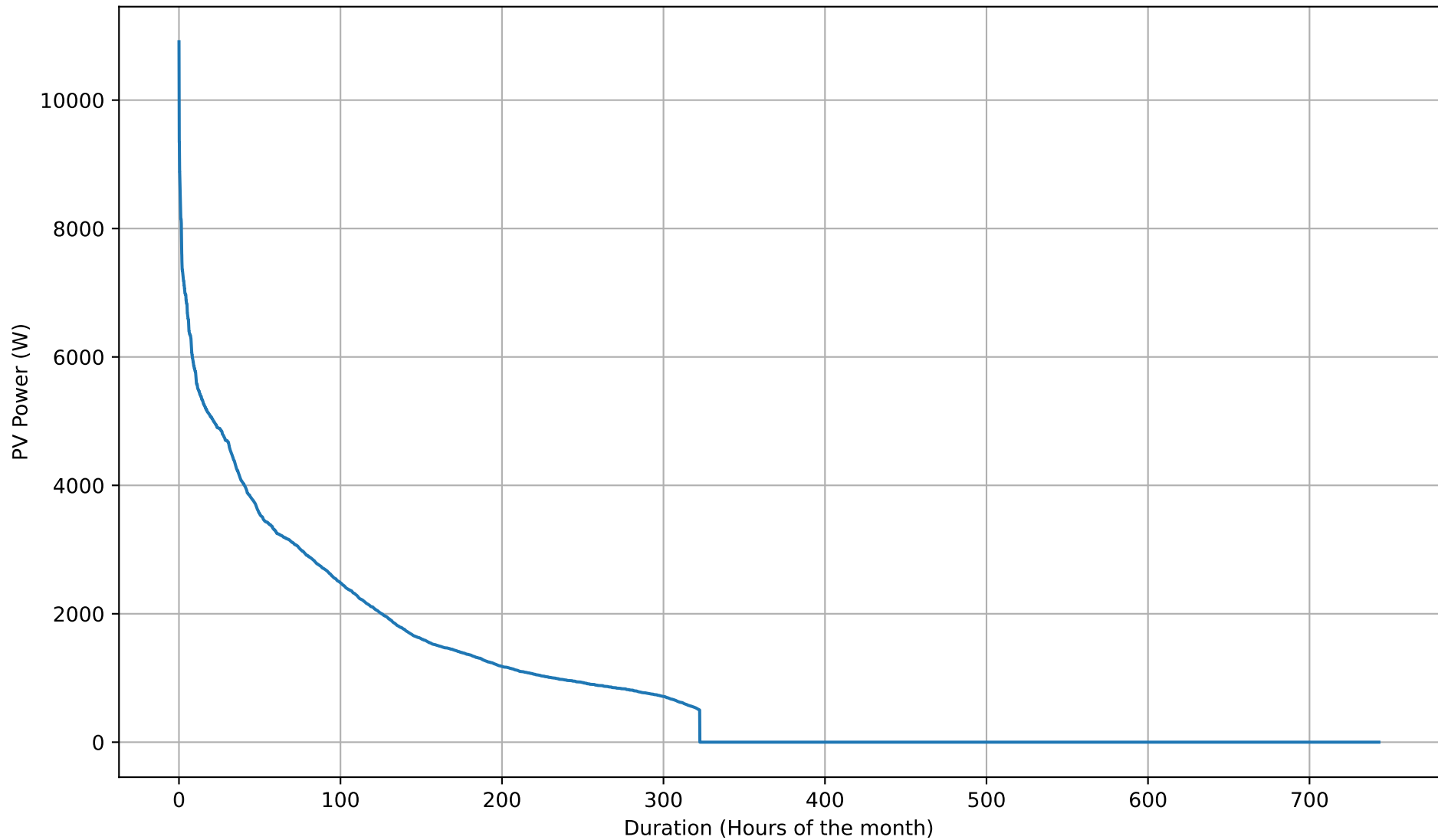
PV Self-Consumption Duration Curve - 5kWh - Mar
