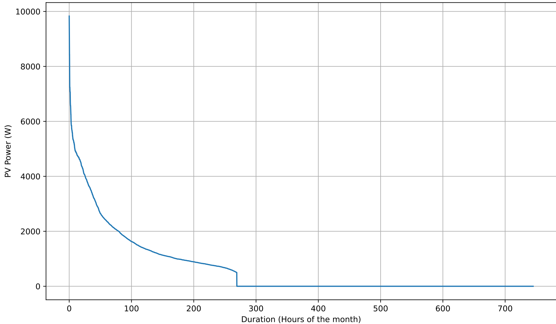
PV Self-Consumption Duration Curve - 5kWh - Oct
