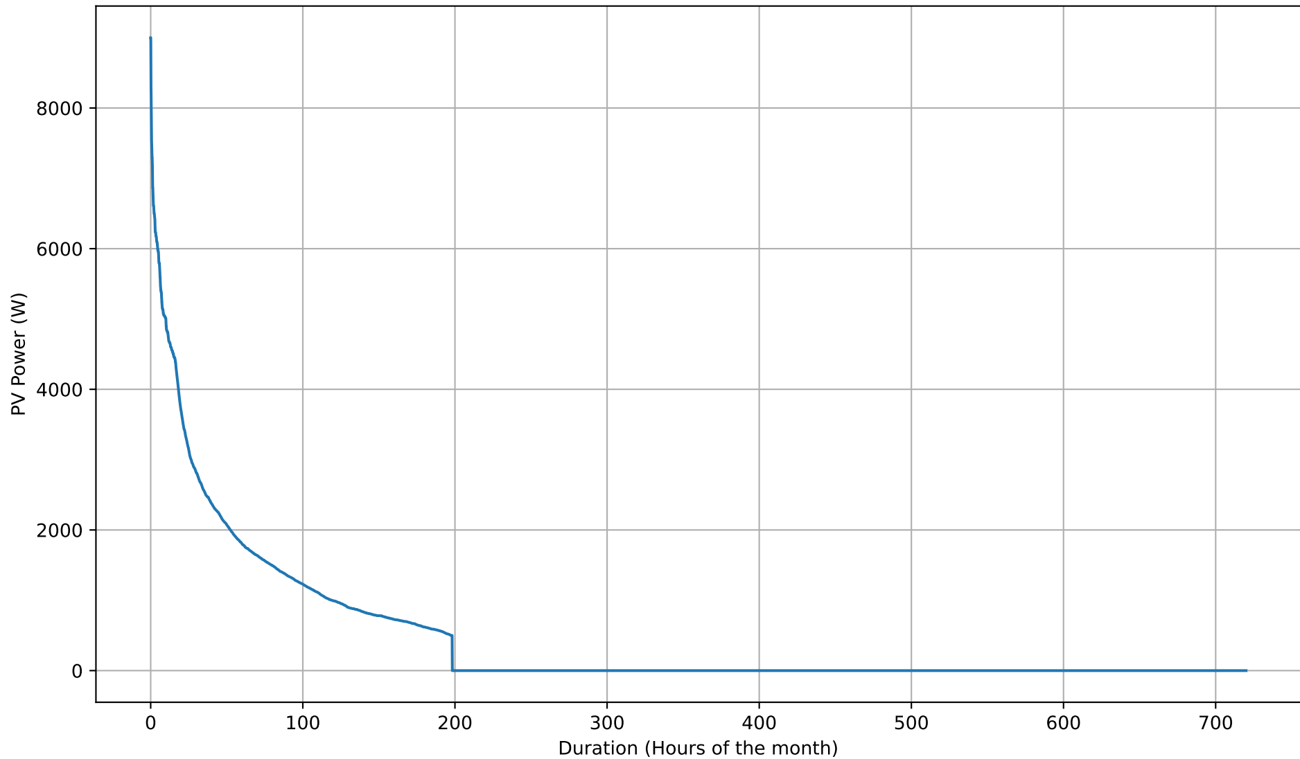
PV Self-Consumption Duration Curve - 5kWh - Nov
