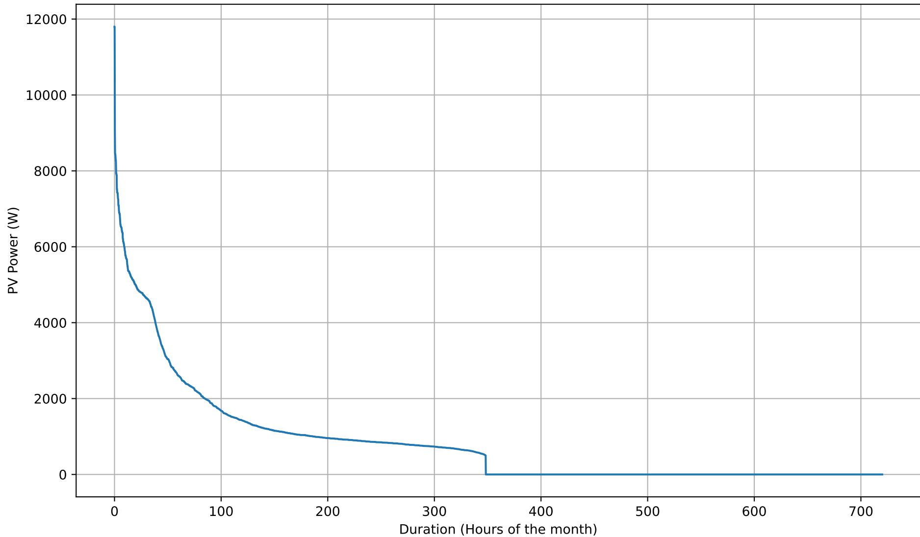
PV Self-Consumption Duration Curve - 5kWh - Sep
