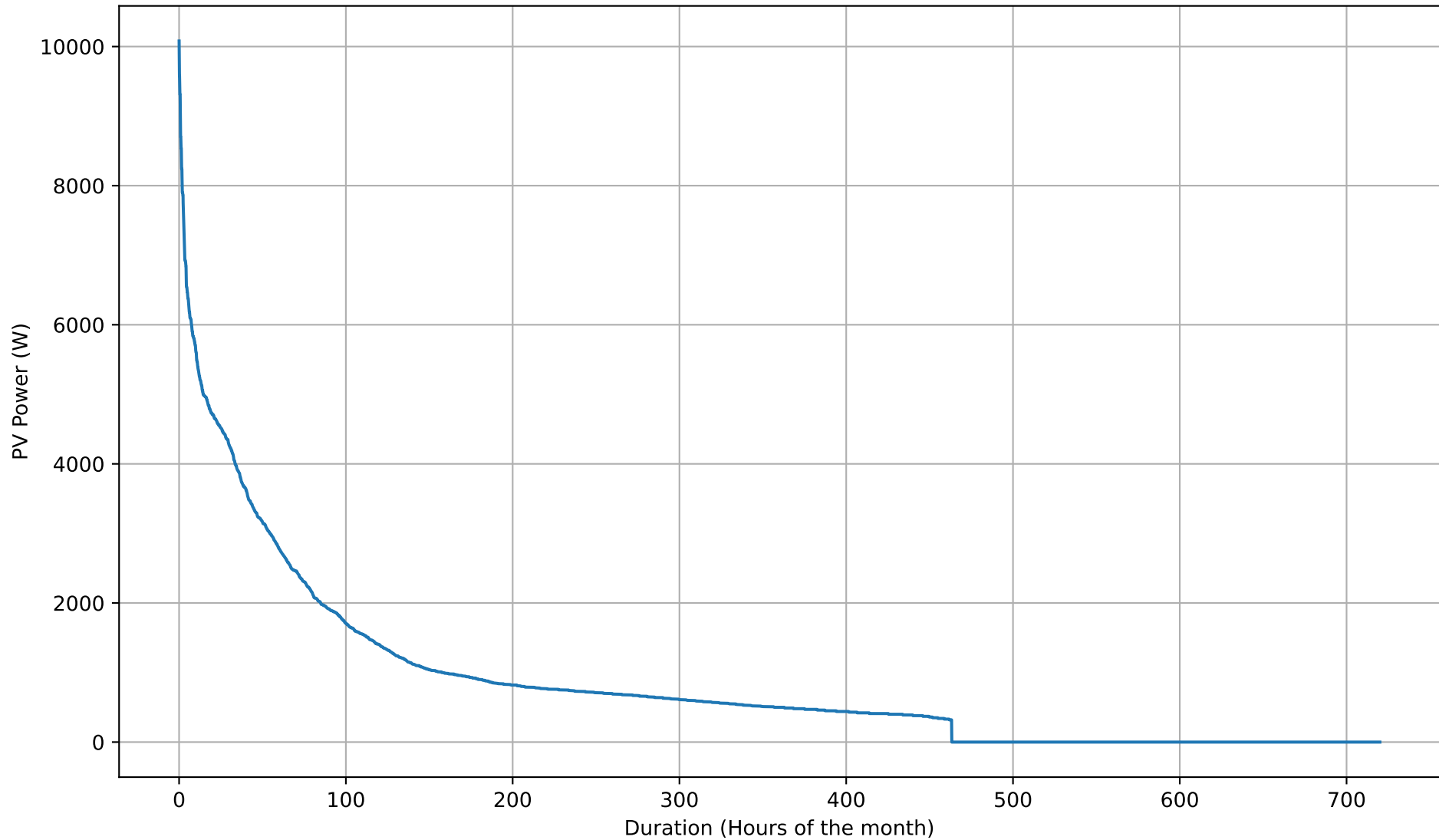
PV Self-Consumption Duration Curve - 5kWh - Jun
