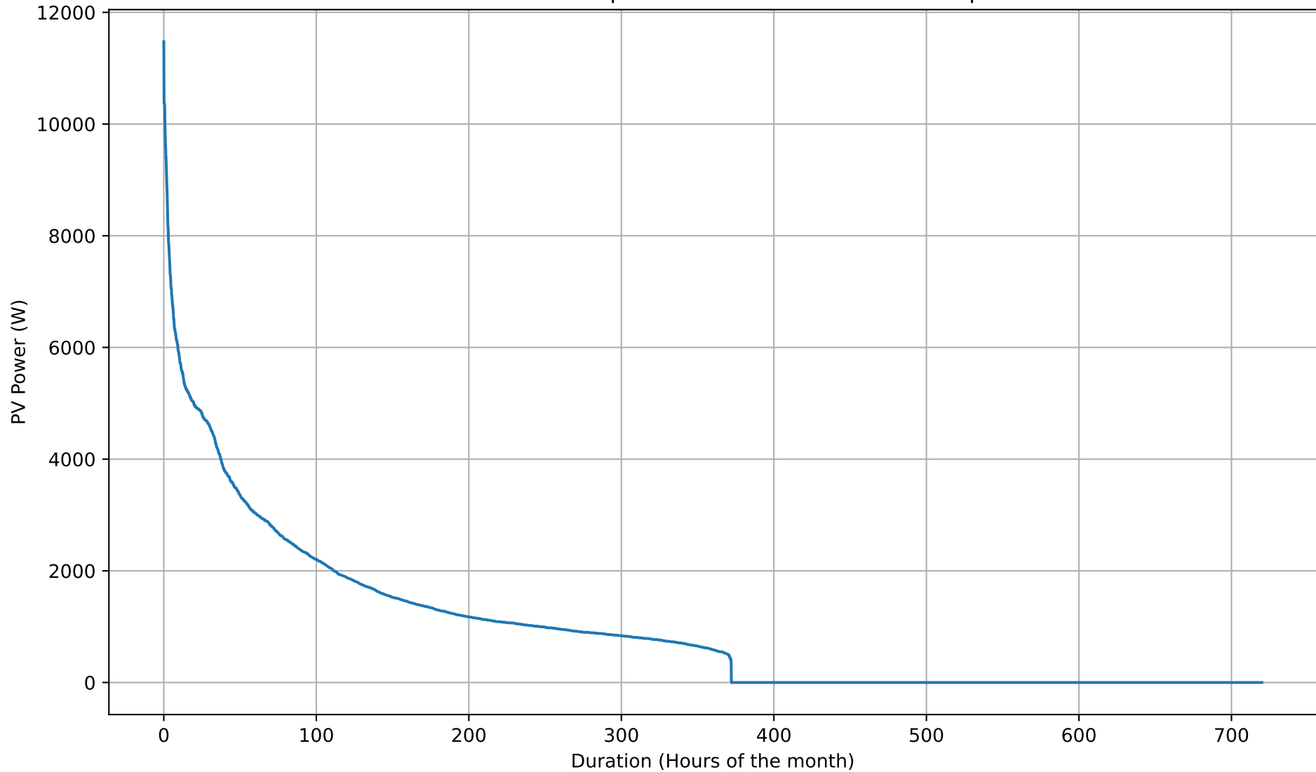
PV Self-Consumption Duration Curve - 5kWh - Apr
