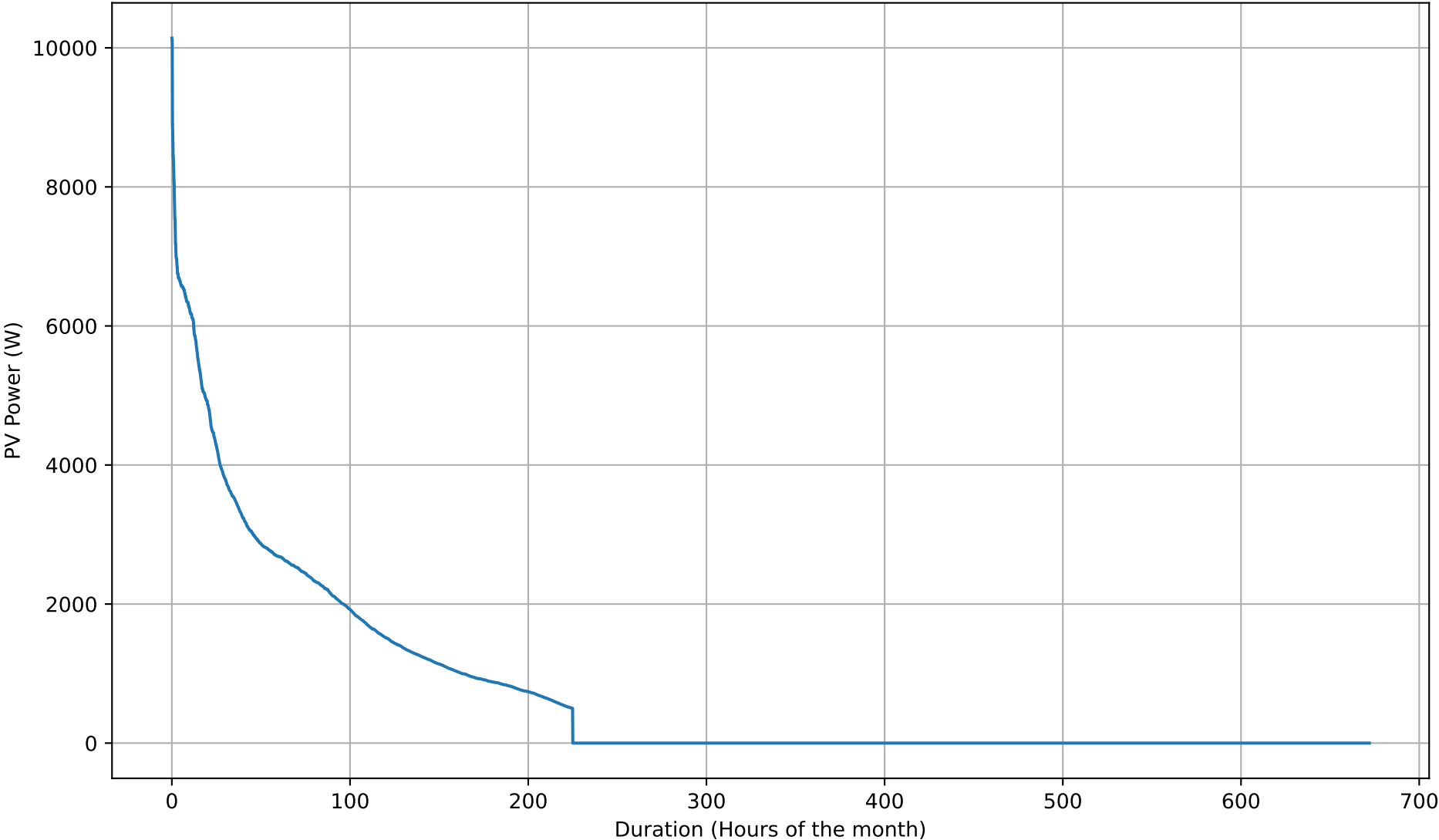
PV Self-Consumption Duration Curve - 5kWh - Feb
