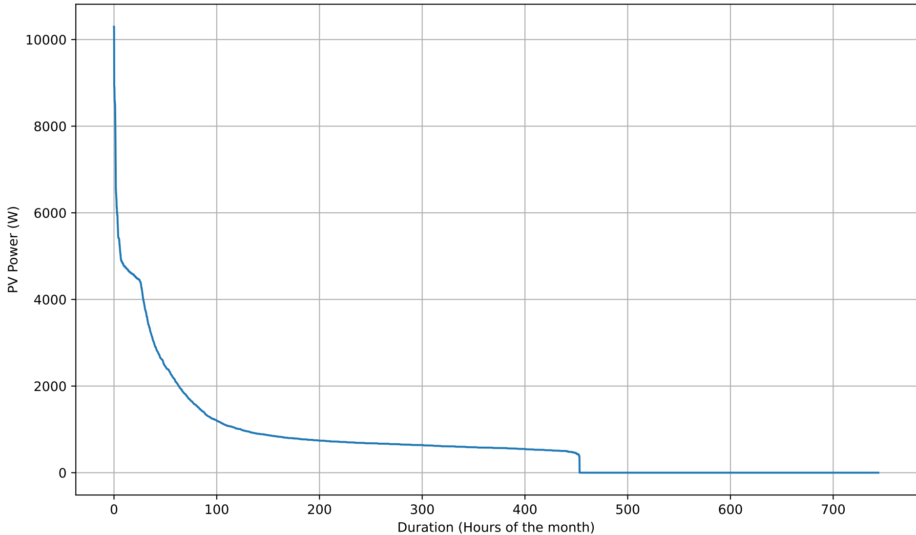
PV Self-Consumption Duration Curve - 5kWh - Jul
