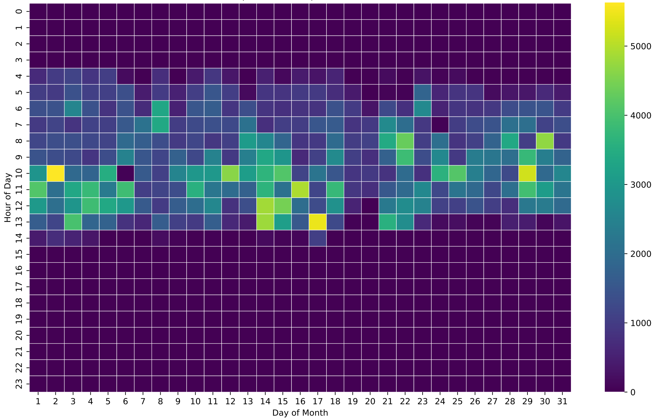
PV Self-Consumption Heatmap (Wh/Hour) - 5kWh - Oct
