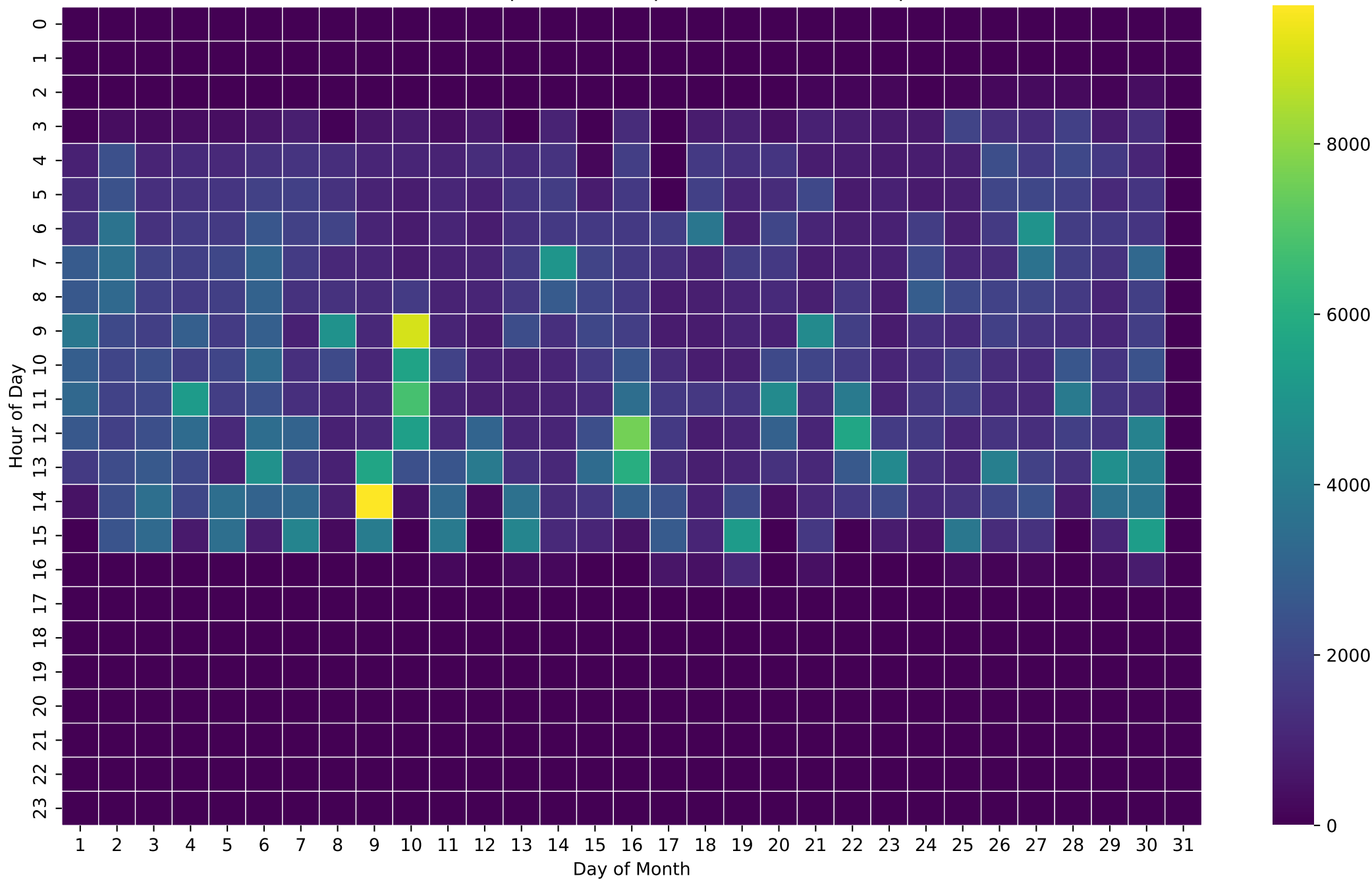
PV Self-Consumption Heatmap (Wh/Hour) - 5kWh - Apr
