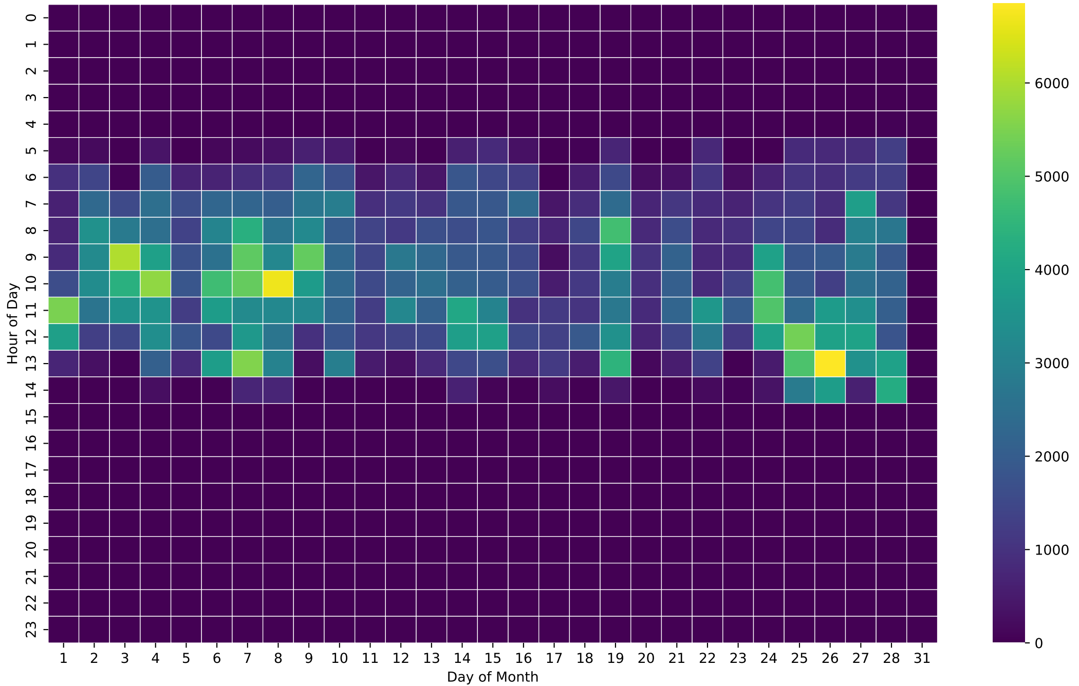
PV Self-Consumption Heatmap (Wh/Hour) - 5kWh - Feb
