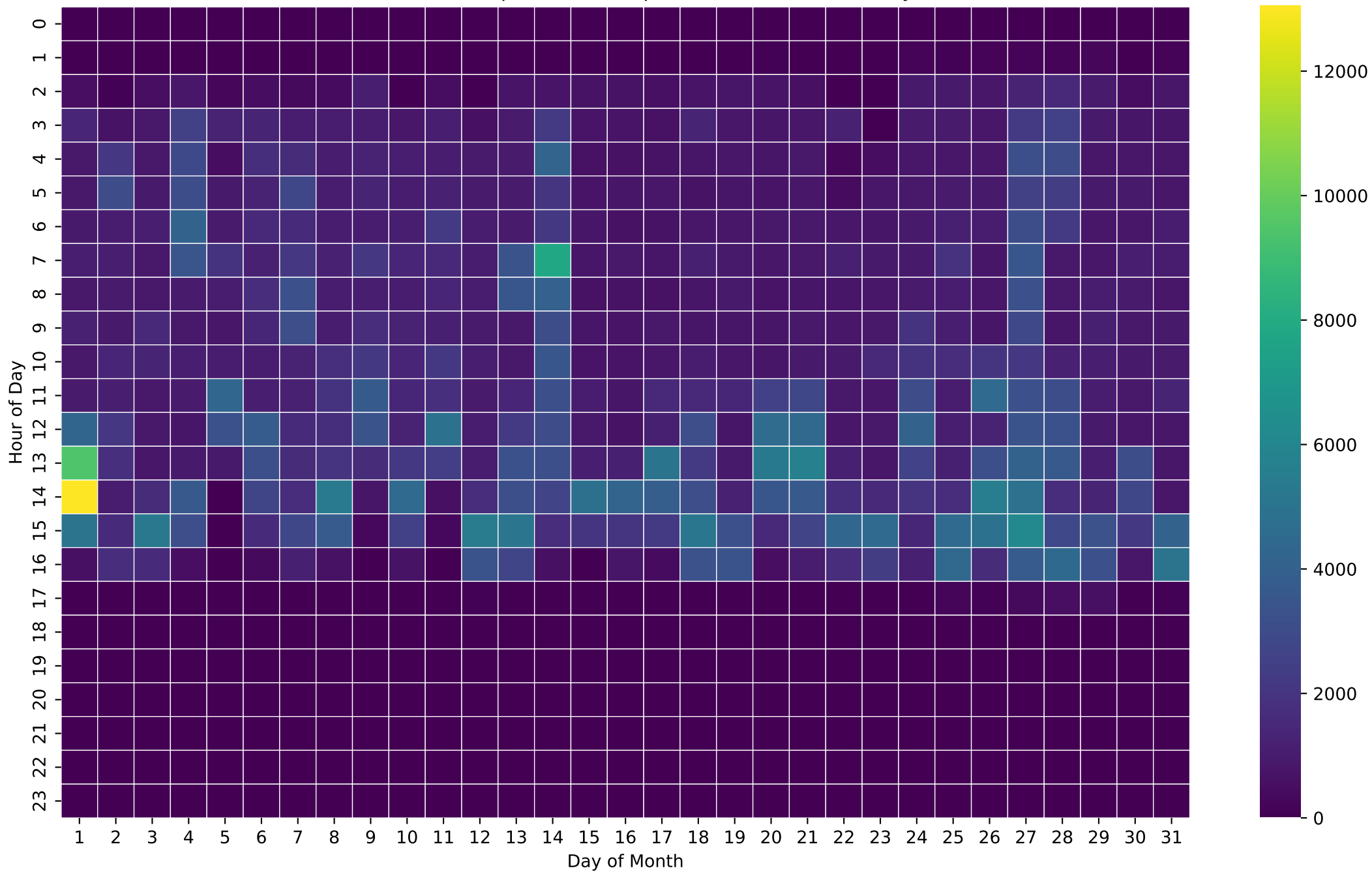
PV Self-Consumption Heatmap (Wh/Hour) - 5kWh - May
