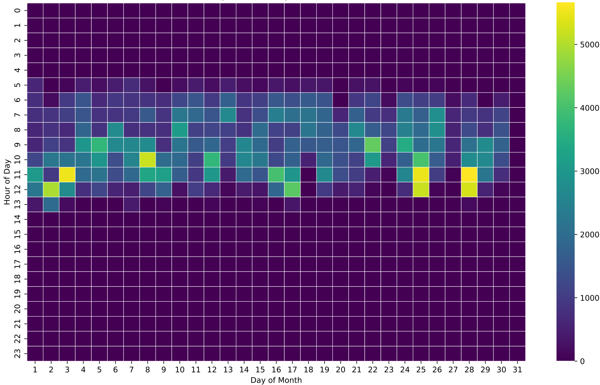
PV Self-Consumption Heatmap (Wh/Hour) - 5kWh - Nov
