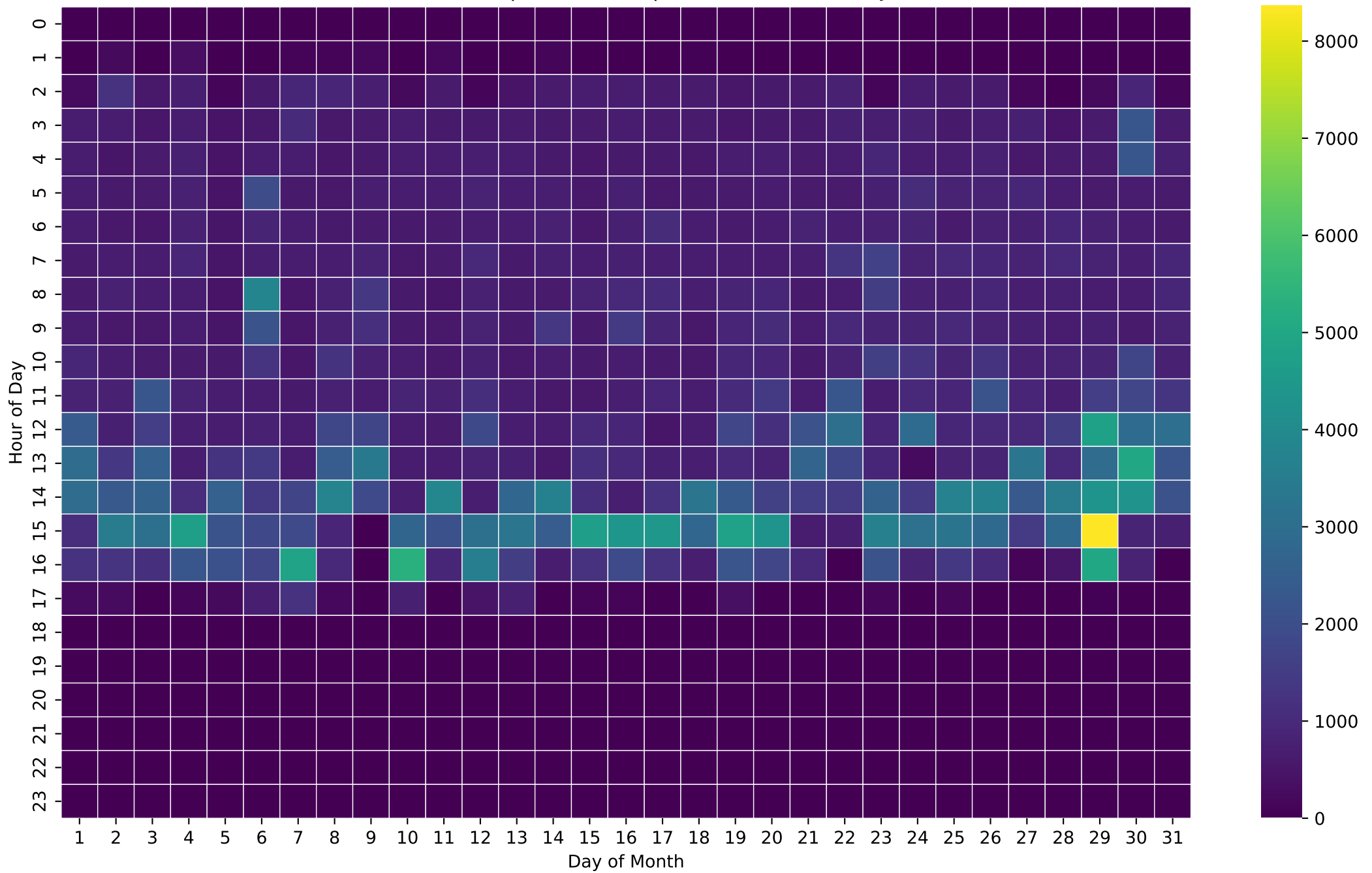
PV Self-Consumption Heatmap (Wh/Hour) - 5kWh - Jul
