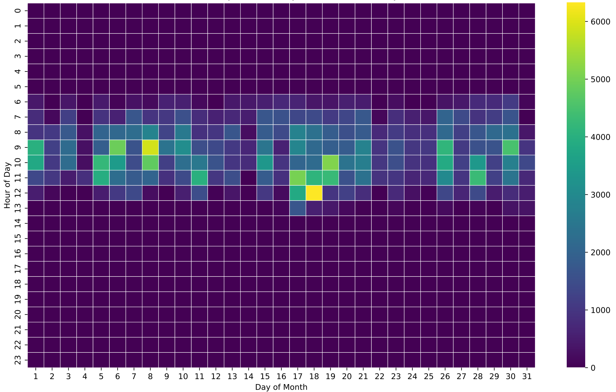
PV Self-Consumption Heatmap (Wh/Hour) - 5kWh - Jan
