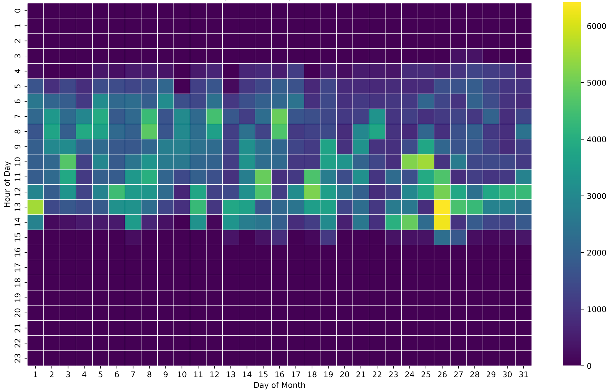
PV Self-Consumption Heatmap (Wh/Hour) - 5kWh - Mar
