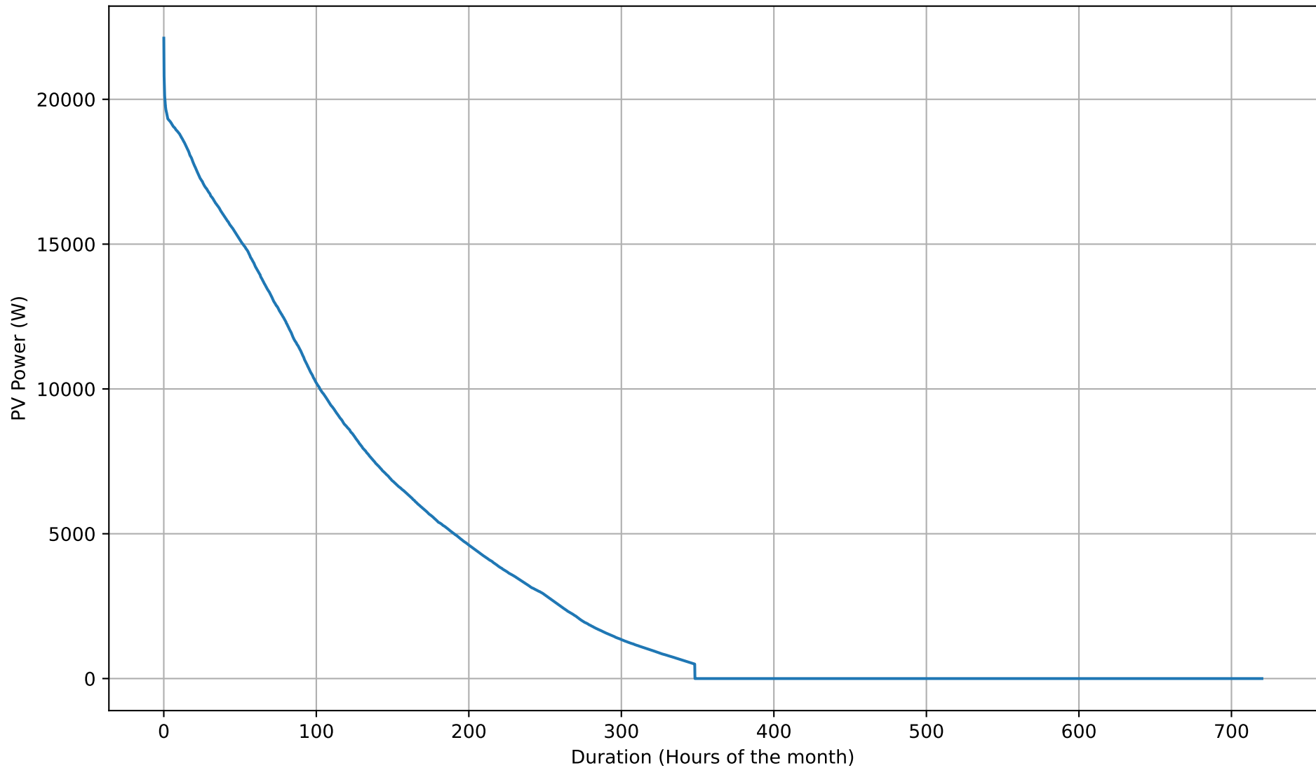
PV Production Duration Curve - 5kWh - Sep
