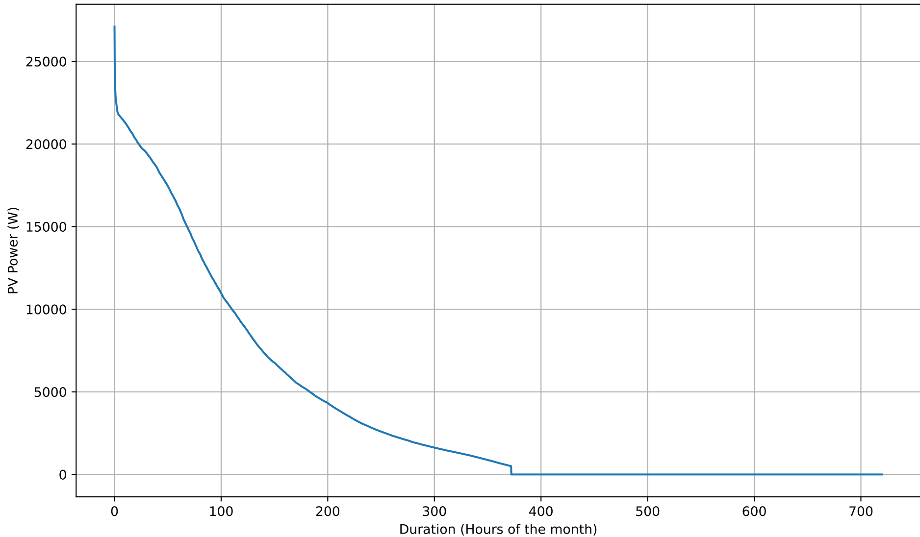
PV Production Duration Curve - 5kWh - Apr
