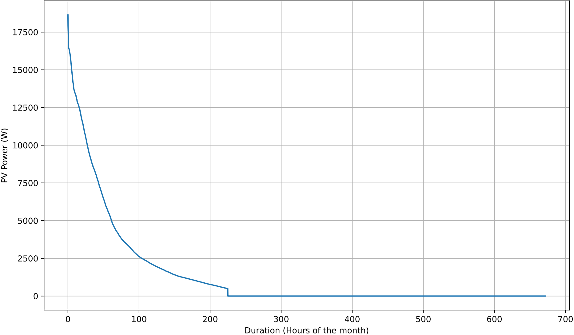
PV Production Duration Curve - 5kWh - Feb
