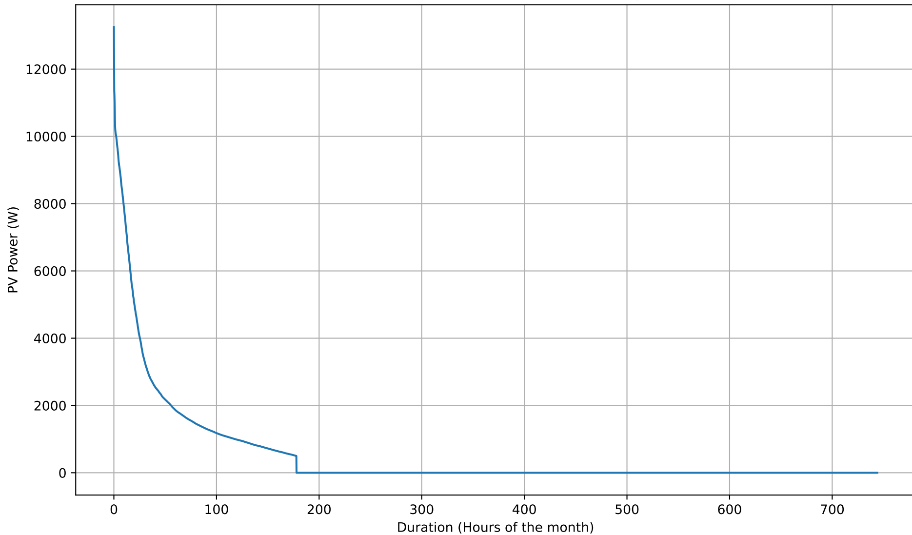
PV Production Duration Curve - 5kWh - Jan
