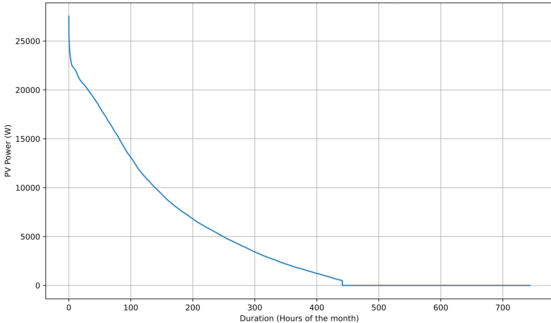
PV Production Duration Curve - 5kWh - May
