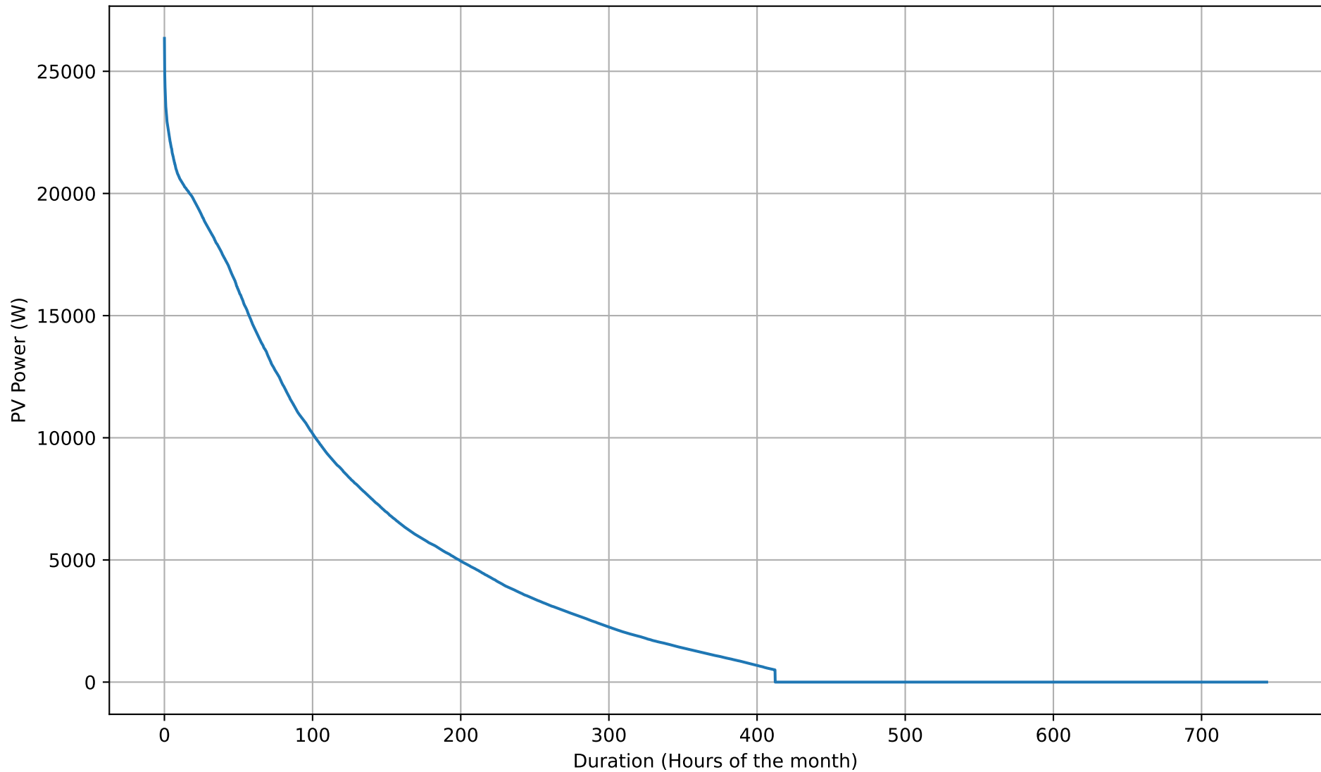
PV Production Duration Curve - 5kWh - Aug
