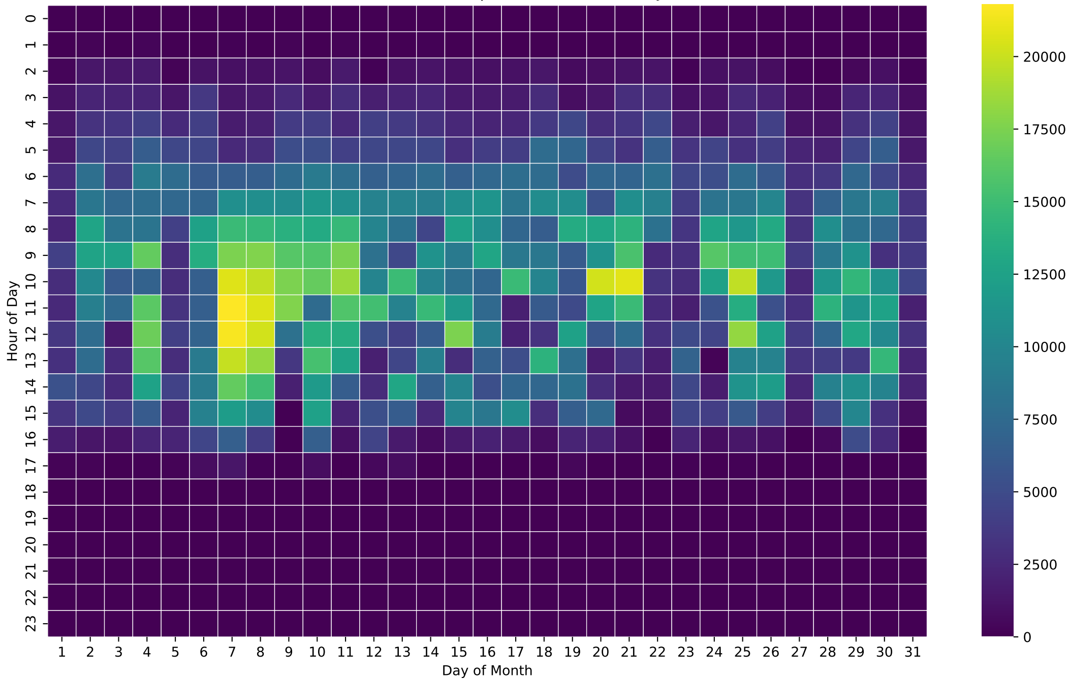
PV Production Heatmap (Wh/Hour) - 5kWh - Jul
