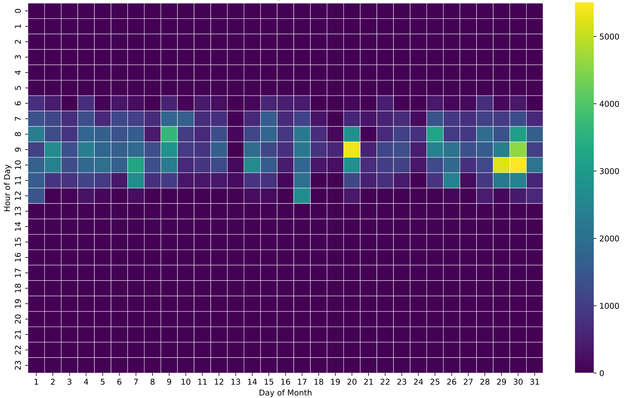
PV Production Heatmap (Wh/Hour) - 5kWh - Dec
