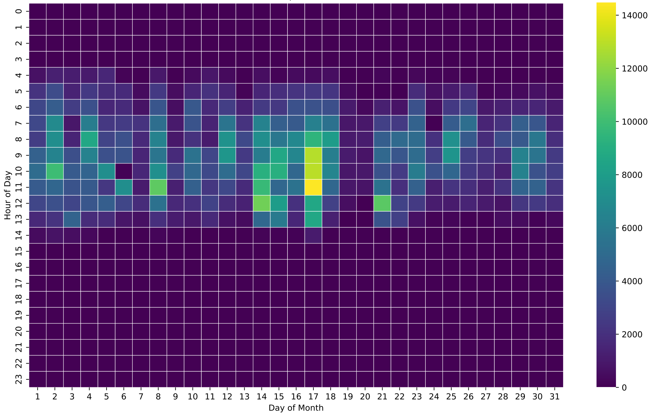
PV Production Heatmap (Wh/Hour) - 5kWh - Oct
