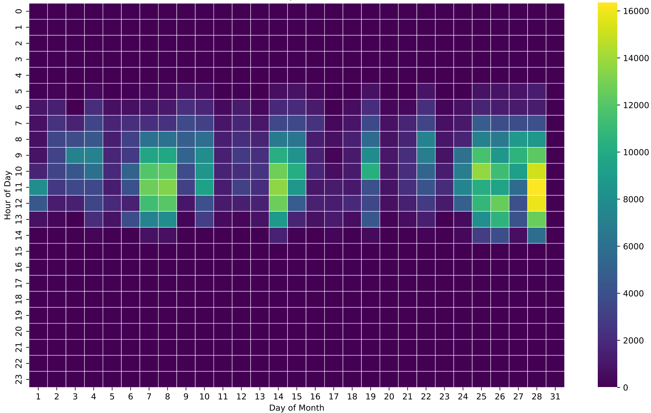
PV Production Heatmap (Wh/Hour) - 5kWh - Feb
