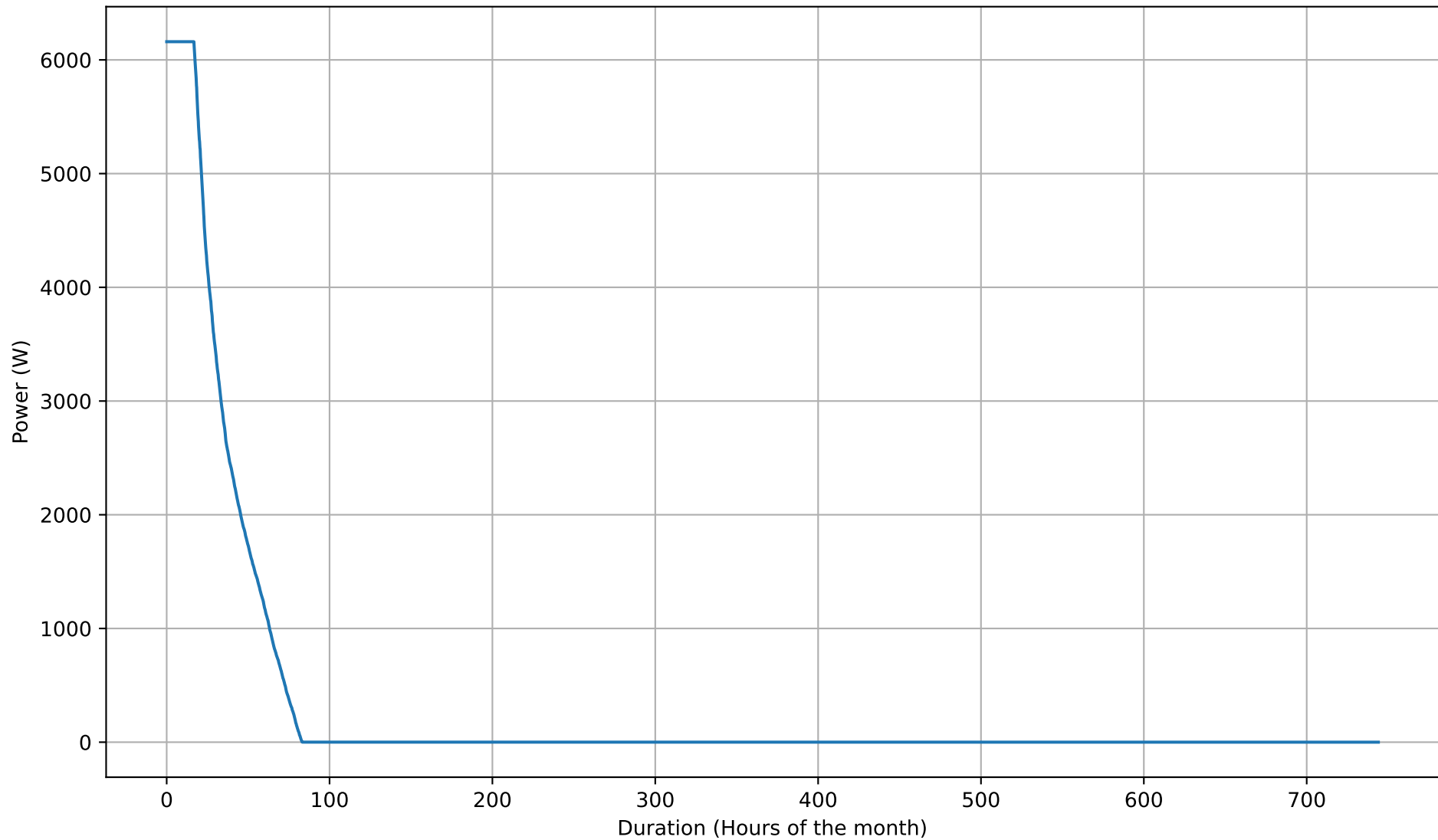
Battery Charging Power Duration Curve - 8kWh - Jul
