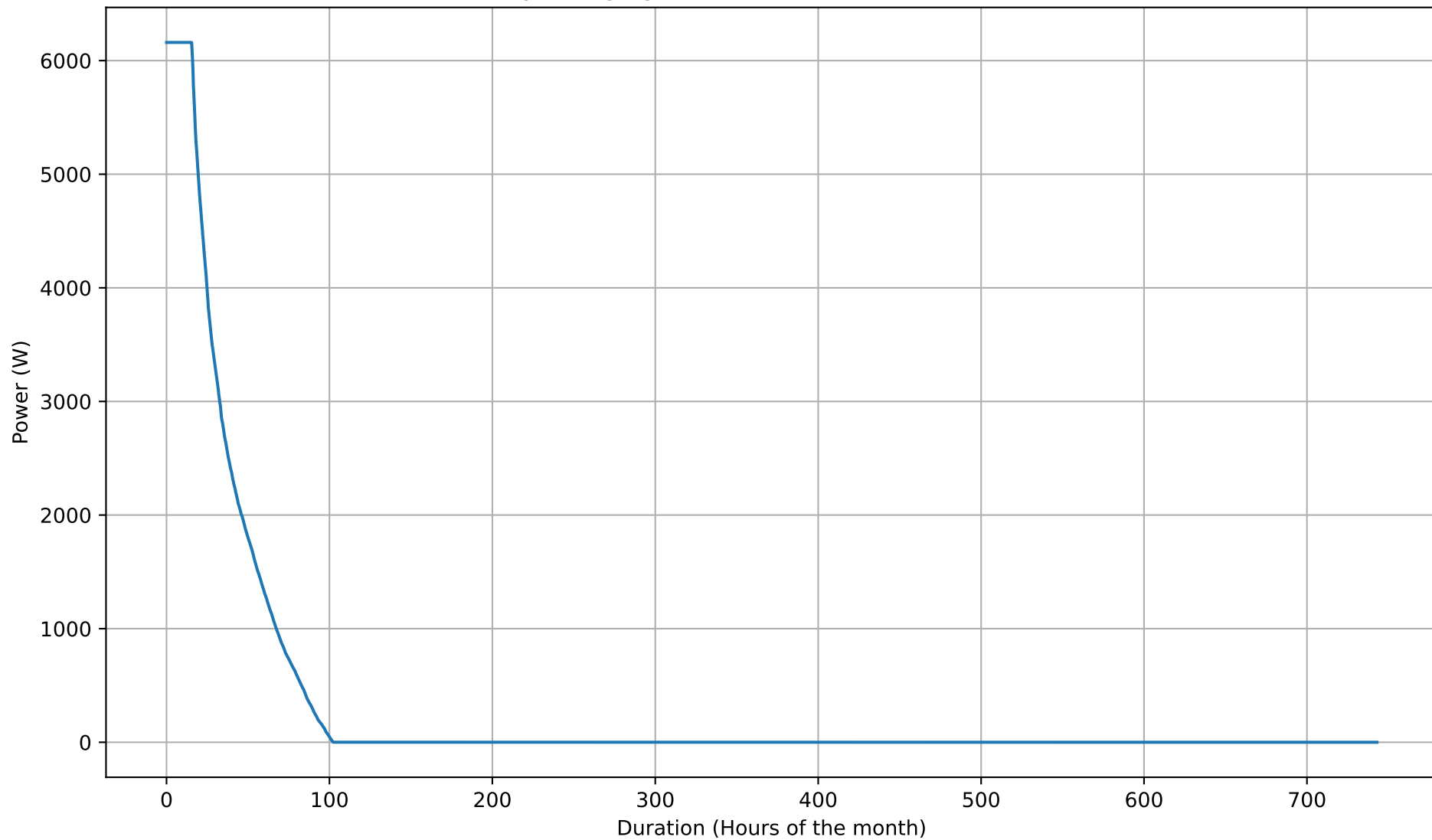
Battery Charging Power Duration Curve - 8kWh - Mar
