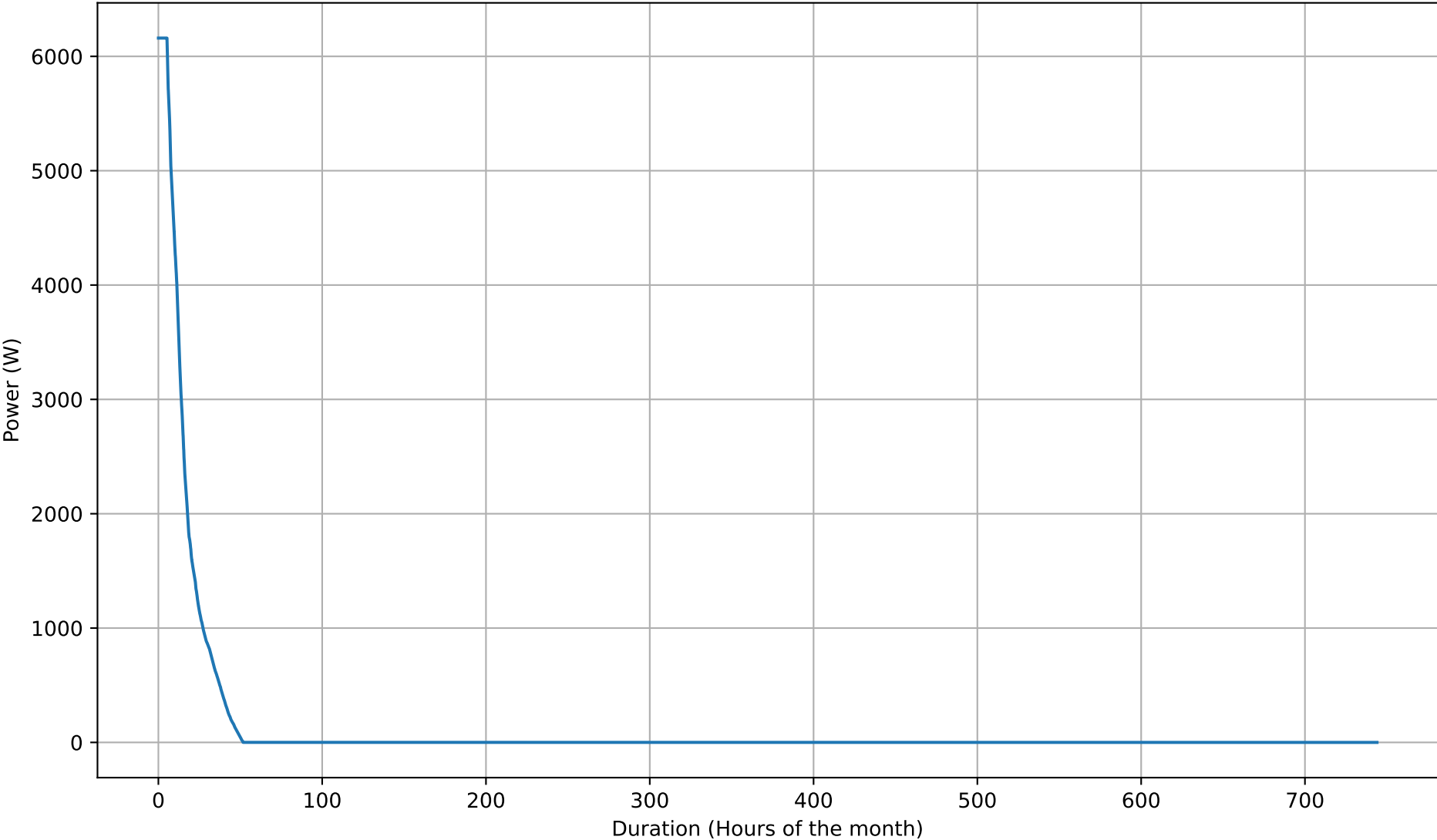
Battery Charging Power Duration Curve - 8kWh - Jan
