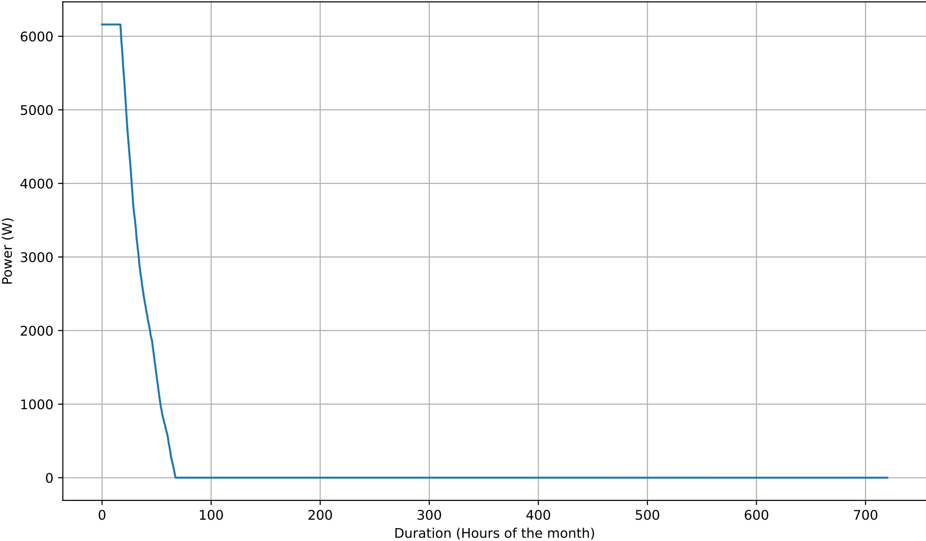
Battery Charging Power Duration Curve - 8kWh - Jun
