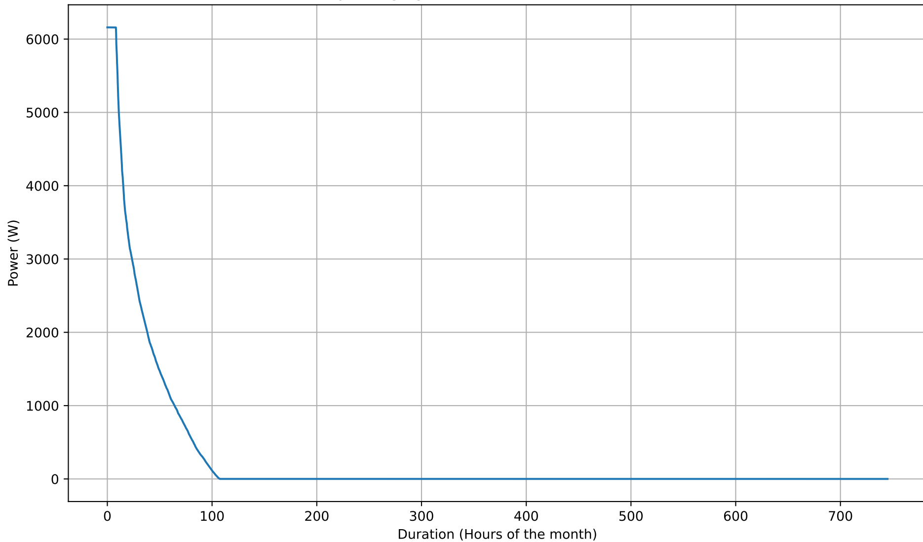
Battery Charging Power Duration Curve - 8kWh - Oct
