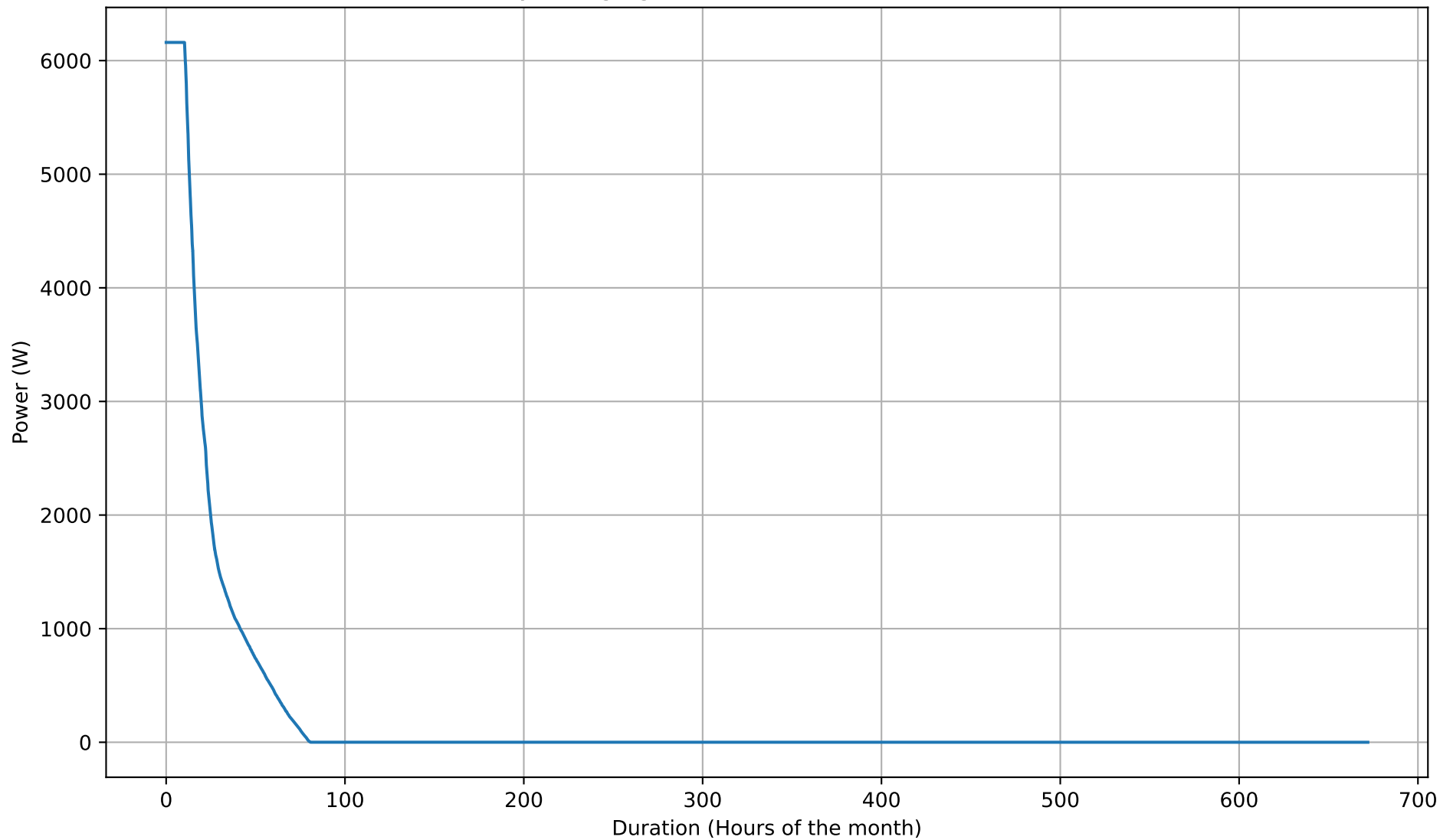
Battery Charging Power Duration Curve - 8kWh - Feb
