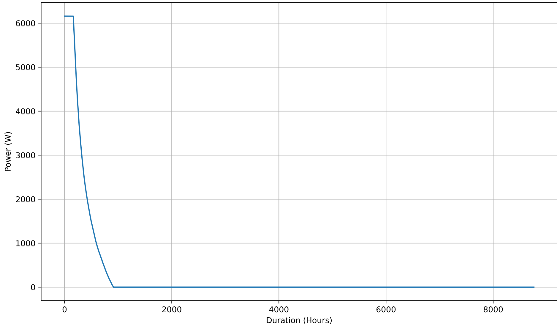
Yearly Battery Charging Power Duration Curve - 8kWh
