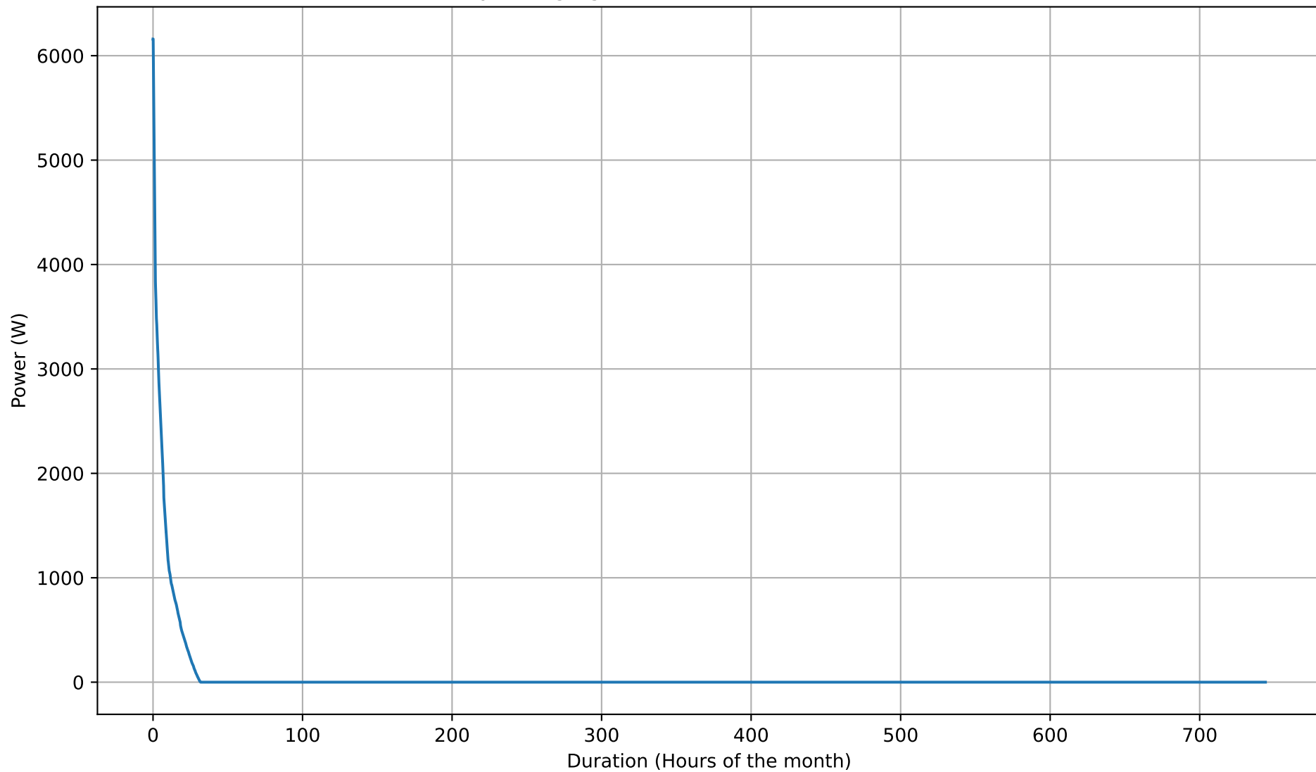
Battery Charging Power Duration Curve - 8kWh - Dec
