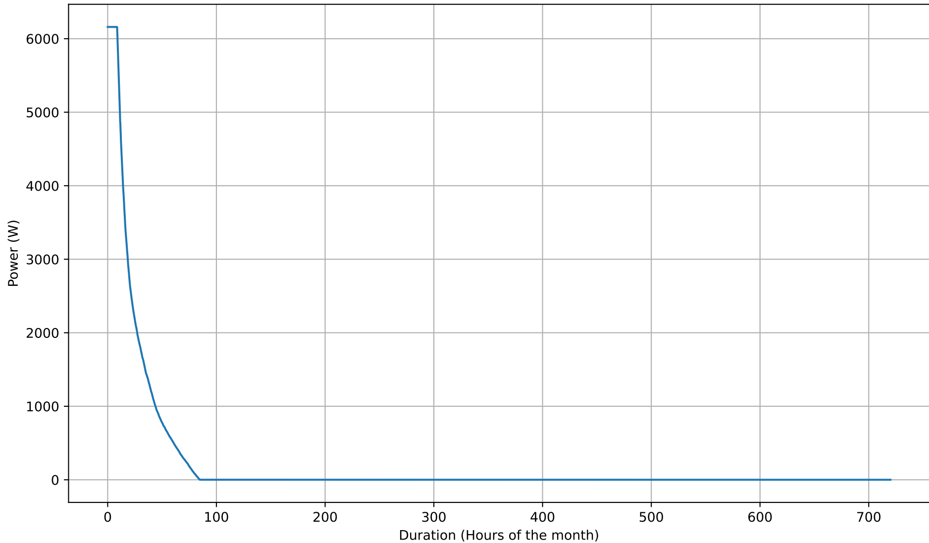
Battery Charging Power Duration Curve - 8kWh - Nov
