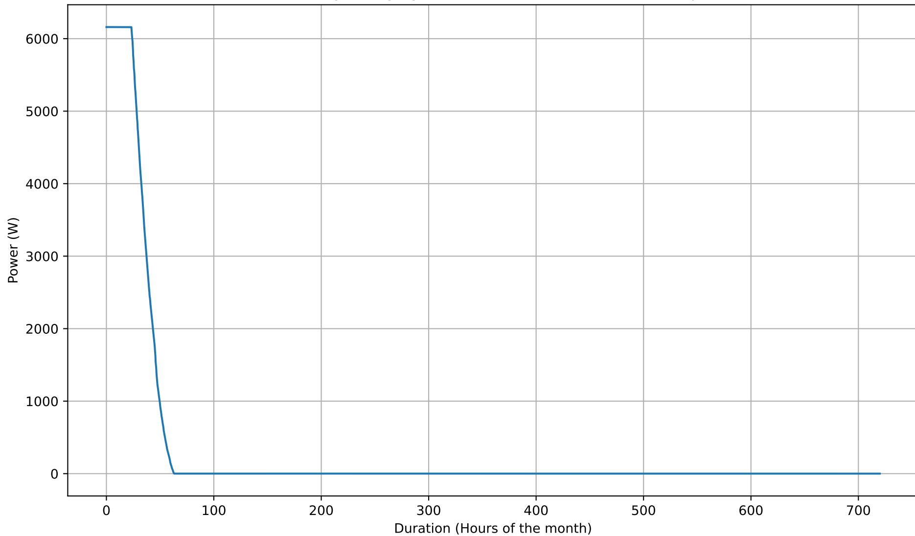
Battery Charging Power Duration Curve - 8kWh - Sep
