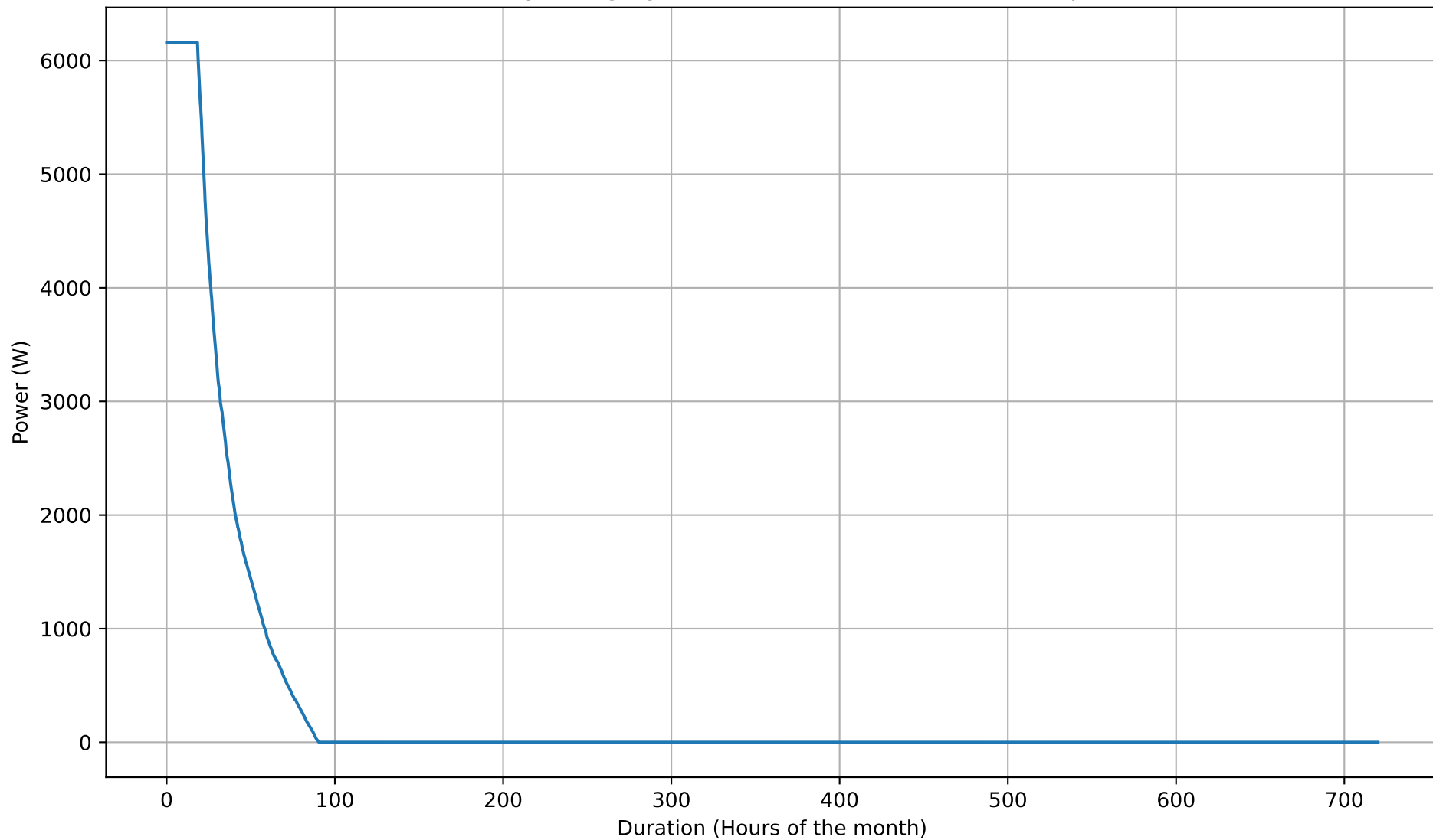
Battery Charging Power Duration Curve - 8kWh - Apr
