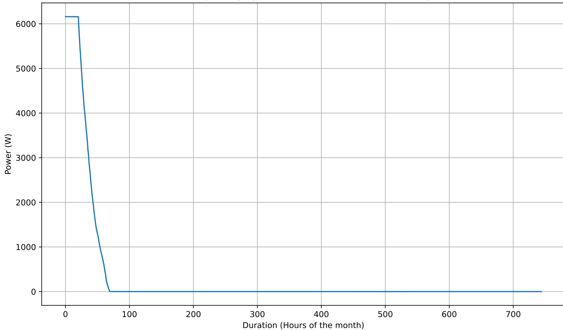
Battery Charging Power Duration Curve - 8kWh - May
