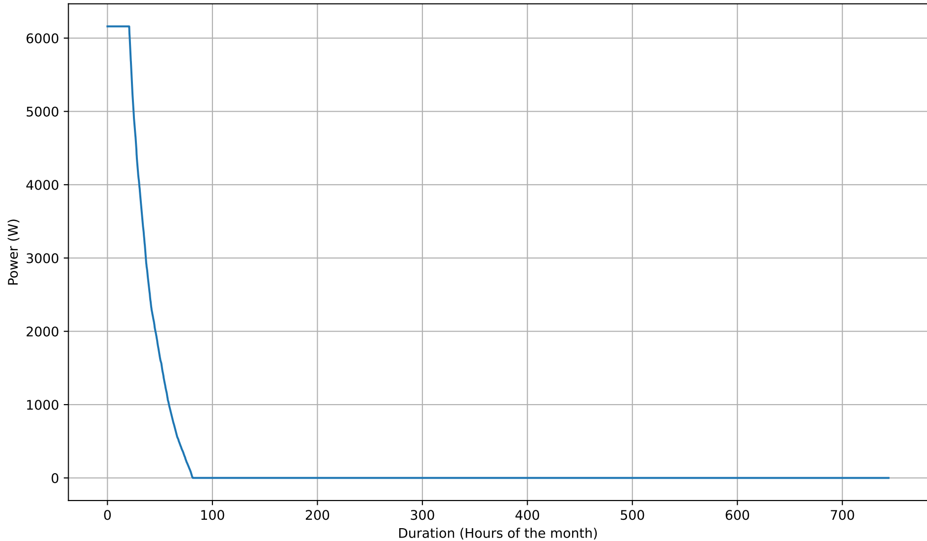
Battery Charging Power Duration Curve - 8kWh - Aug
