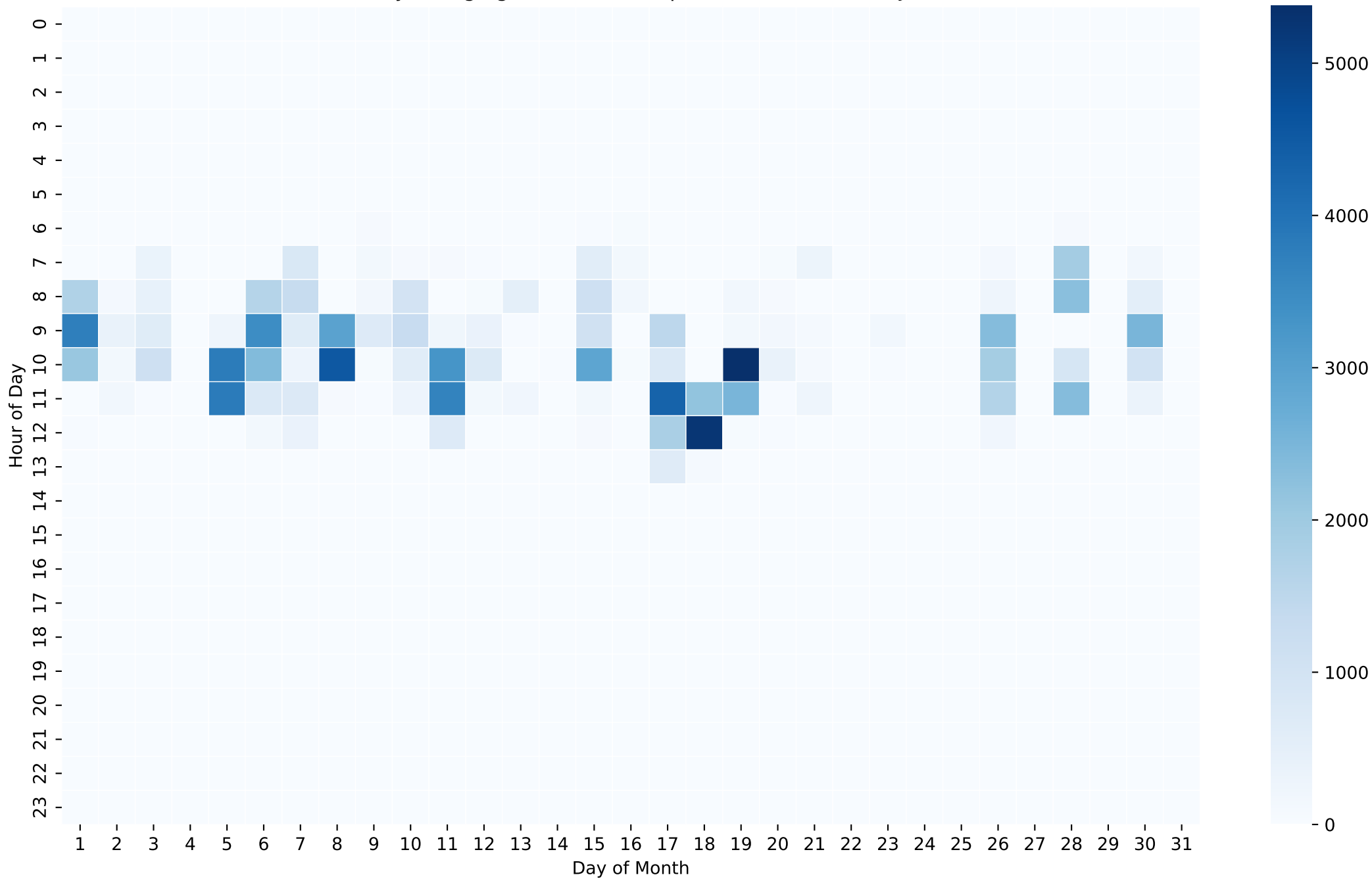
Battery Charging Power Heatmap (Wh/Hour) - 8kWh - Jan
