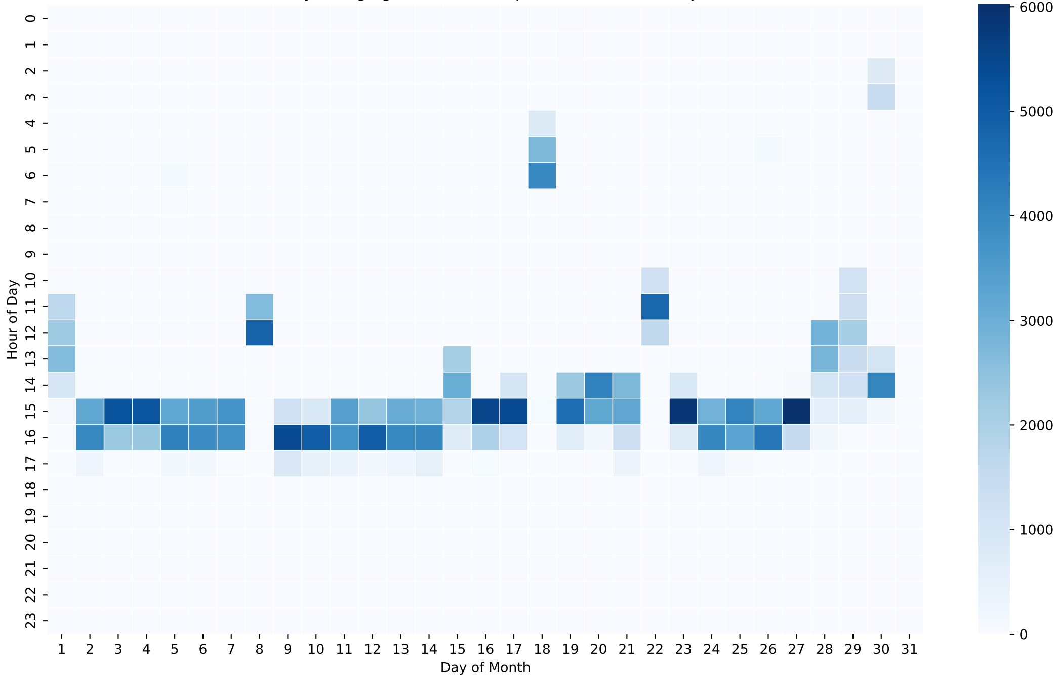
Battery Charging Power Heatmap (Wh/Hour) - 8kWh - Jun
