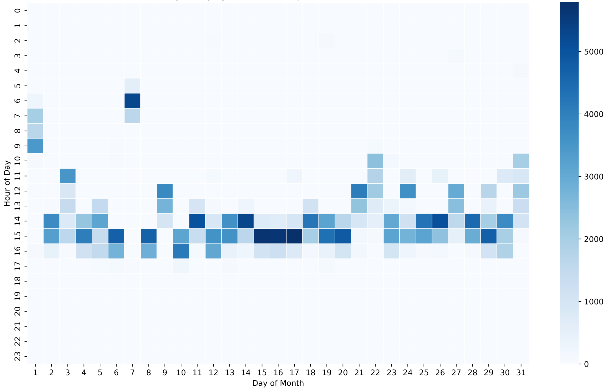
Battery Charging Power Heatmap (Wh/Hour) - 8kWh - Jul
