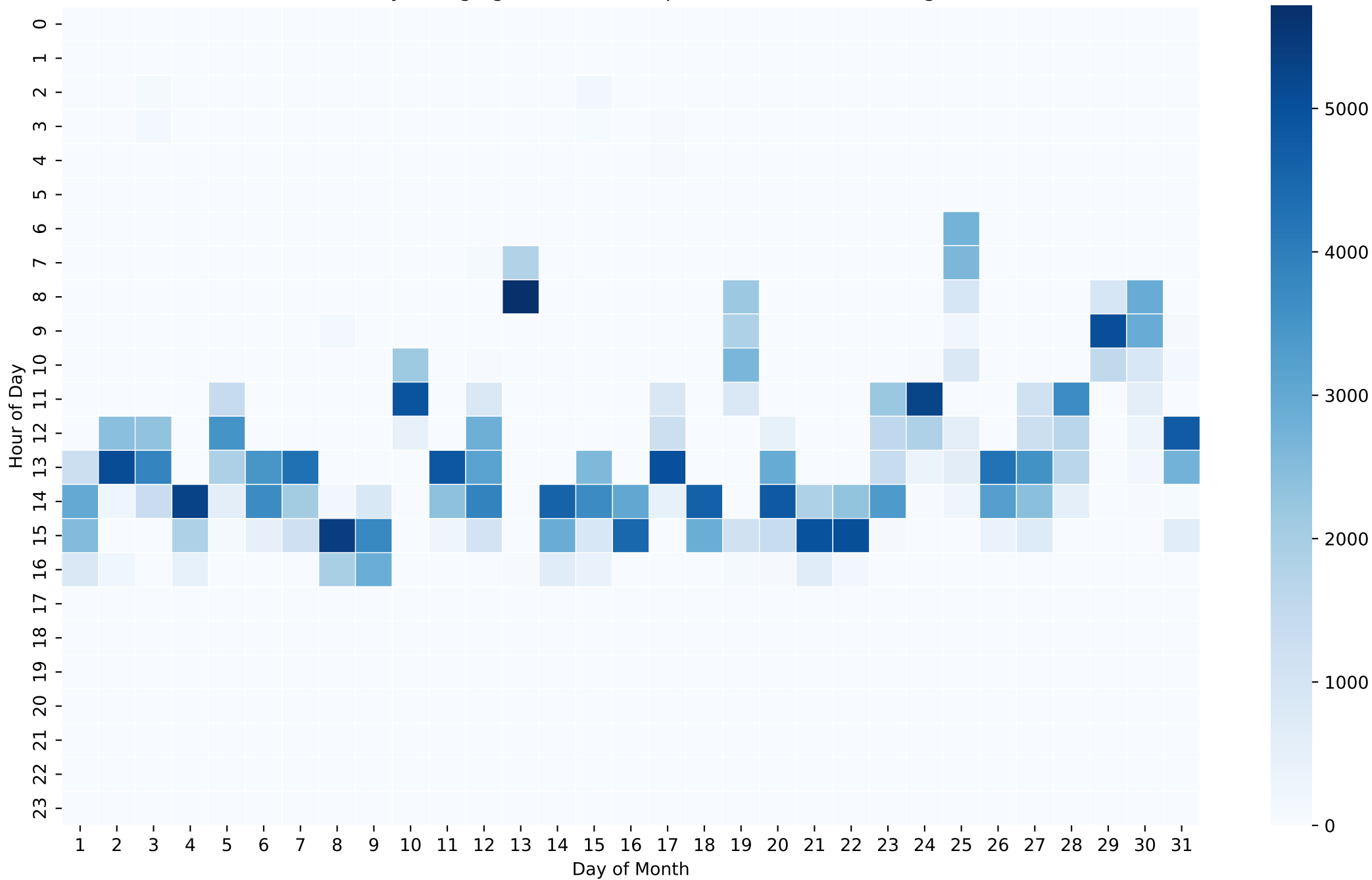
Battery Charging Power Heatmap (Wh/Hour) - 8kWh - Aug
