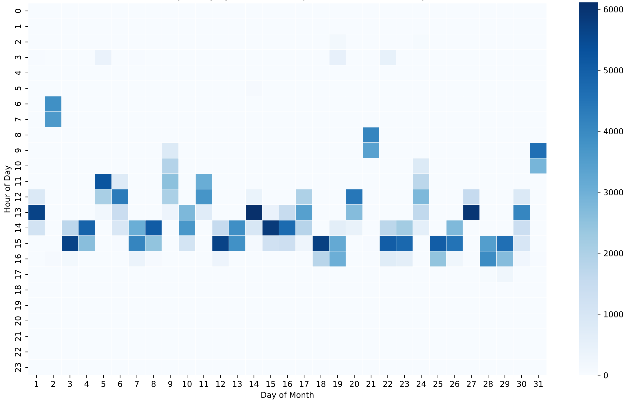
Battery Charging Power Heatmap (Wh/Hour) - 8kWh - May
