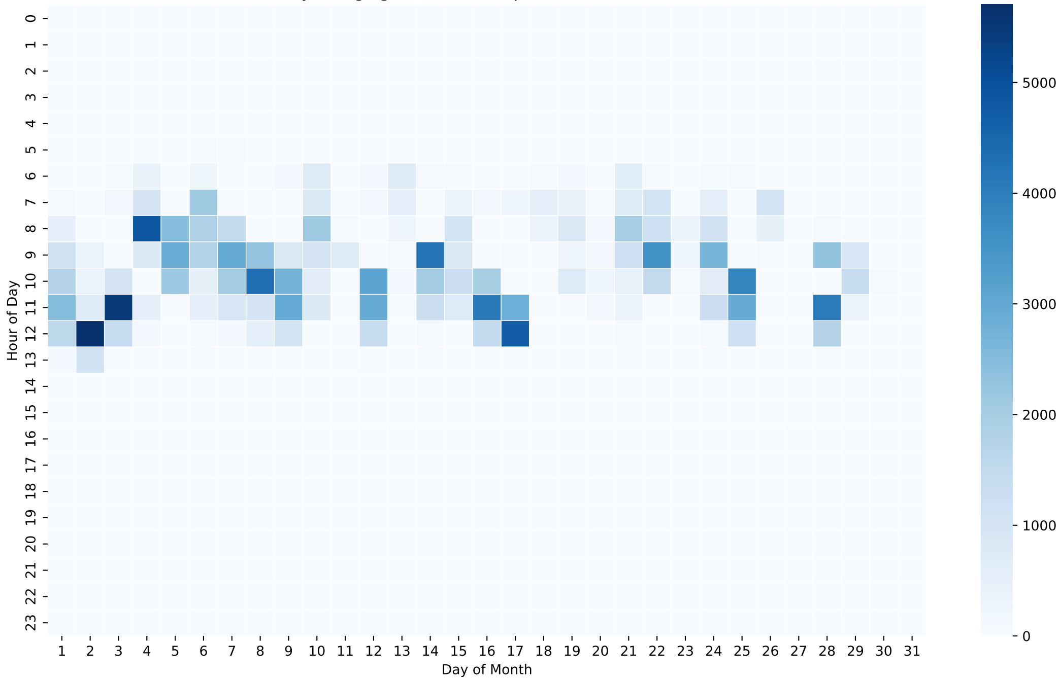
Battery Charging Power Heatmap (Wh/Hour) - 8kWh - Nov
