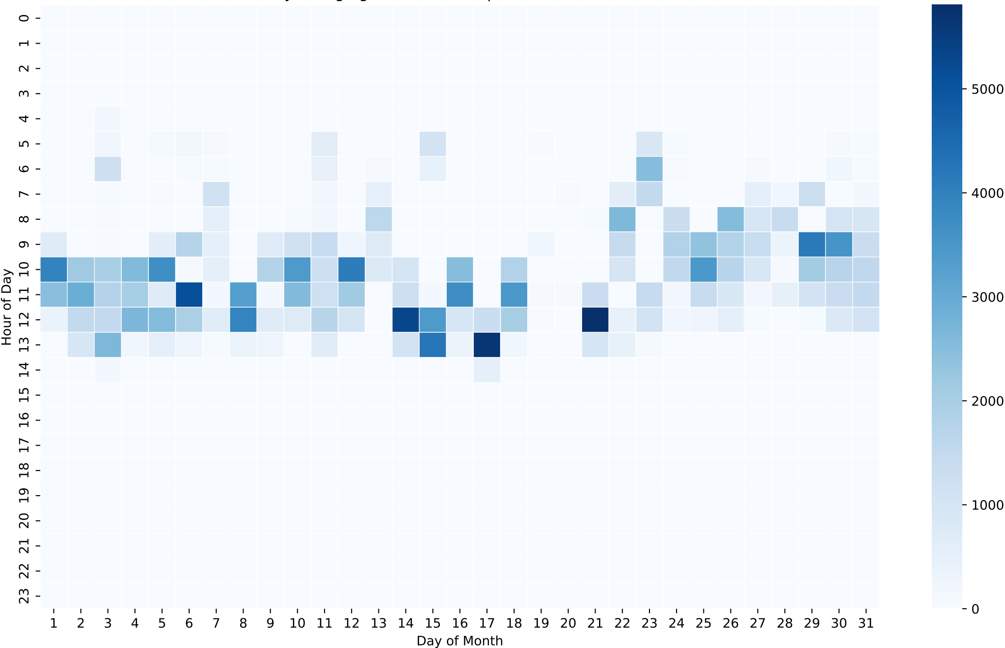
Battery Charging Power Heatmap (Wh/Hour) - 8kWh - Oct
