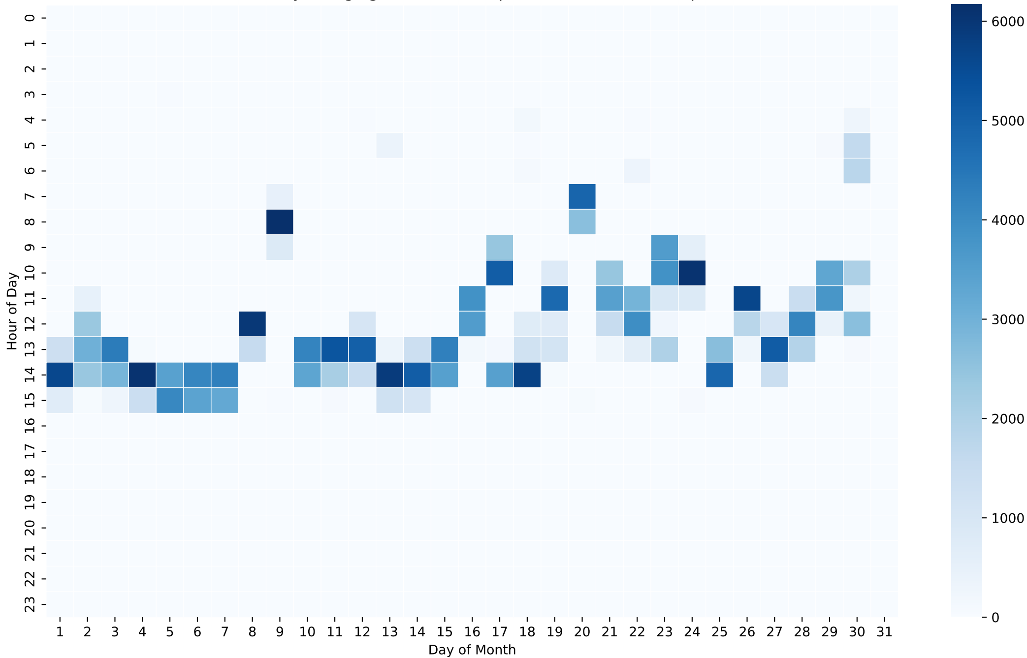
Battery Charging Power Heatmap (Wh/Hour) - 8kWh - Sep
