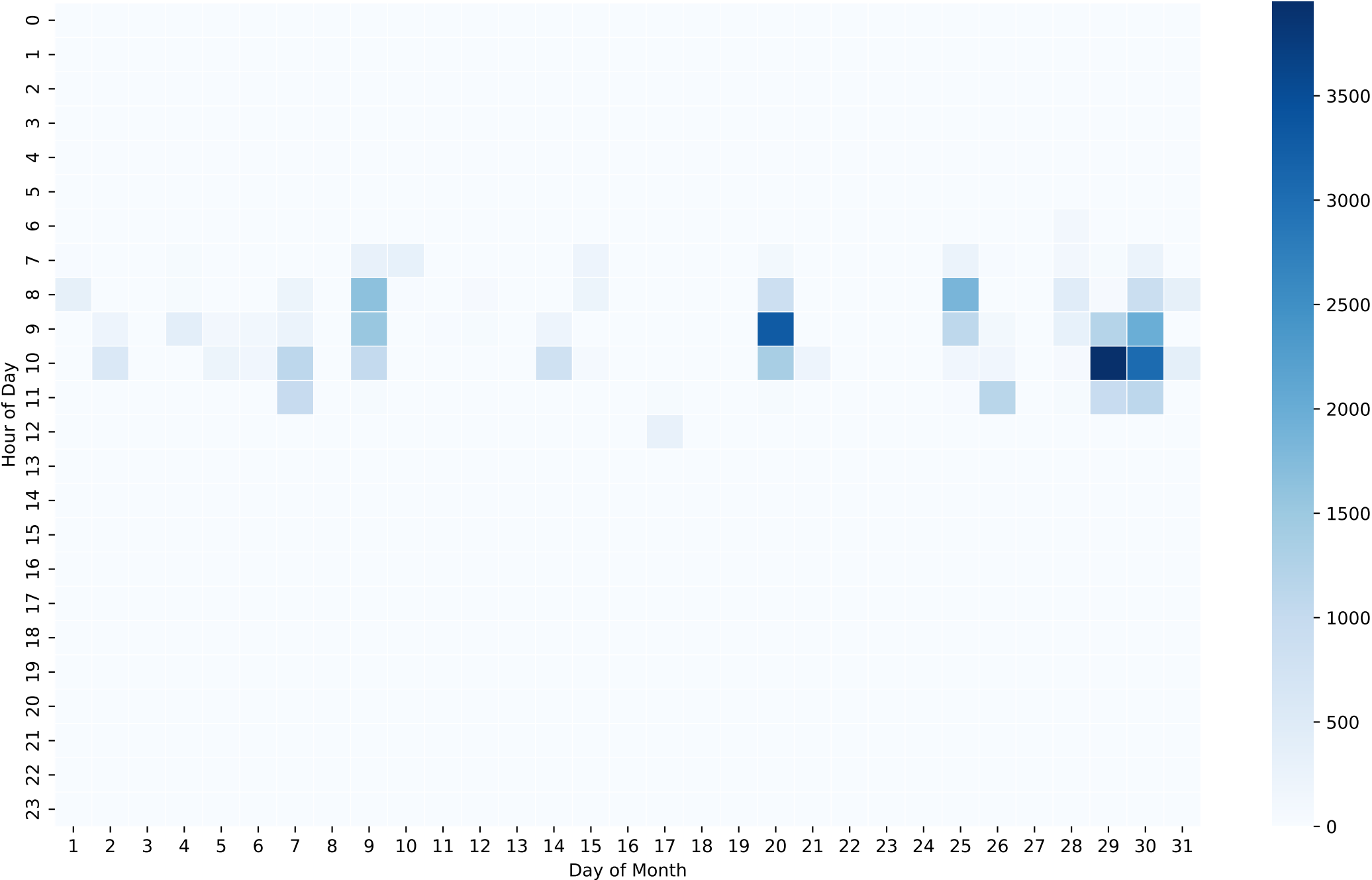
Battery Charging Power Heatmap (Wh/Hour) - 8kWh - Dec
