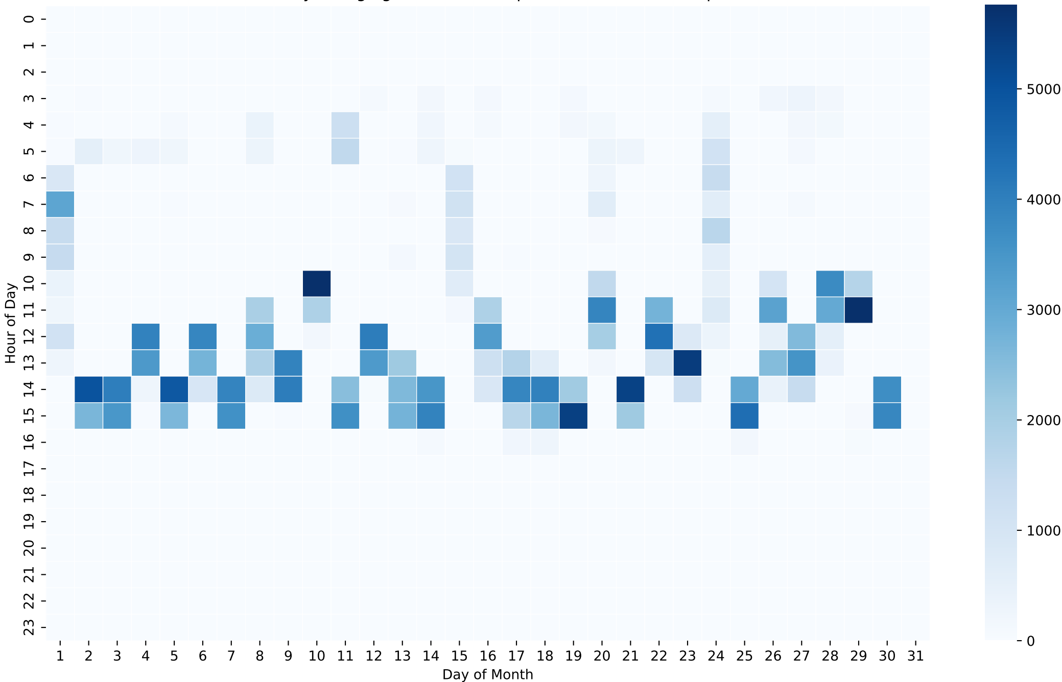
Battery Charging Power Heatmap (Wh/Hour) - 8kWh - Apr
