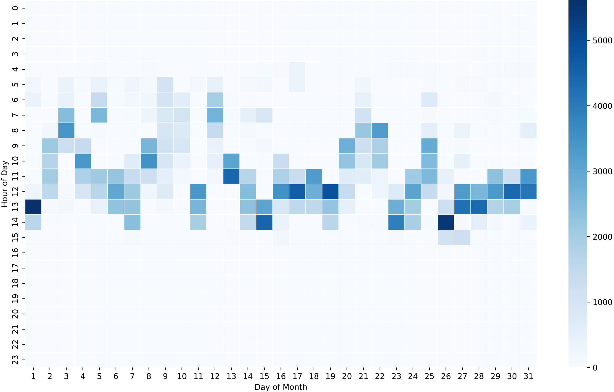
Battery Charging Power Heatmap (Wh/Hour) - 8kWh - Mar
