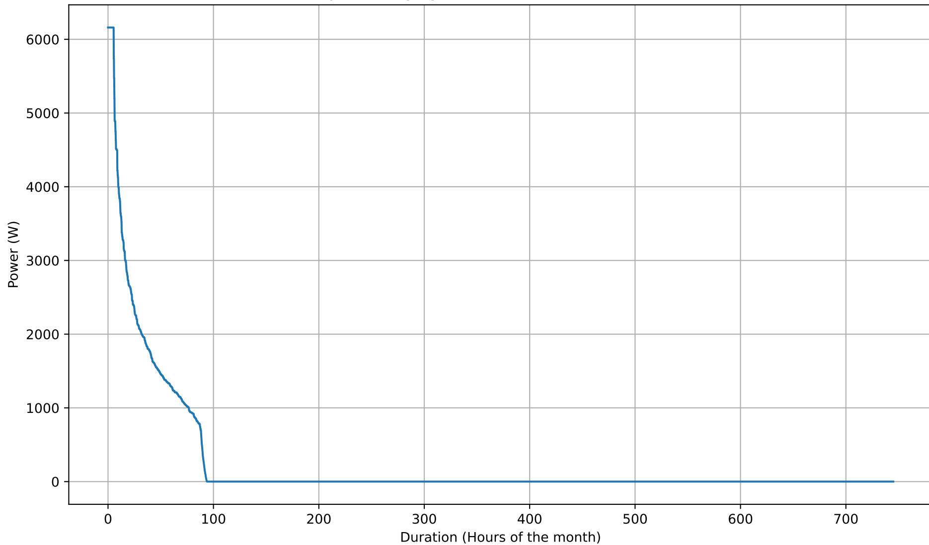
Battery Discharging Power Duration Curve - 8kWh - Oct
