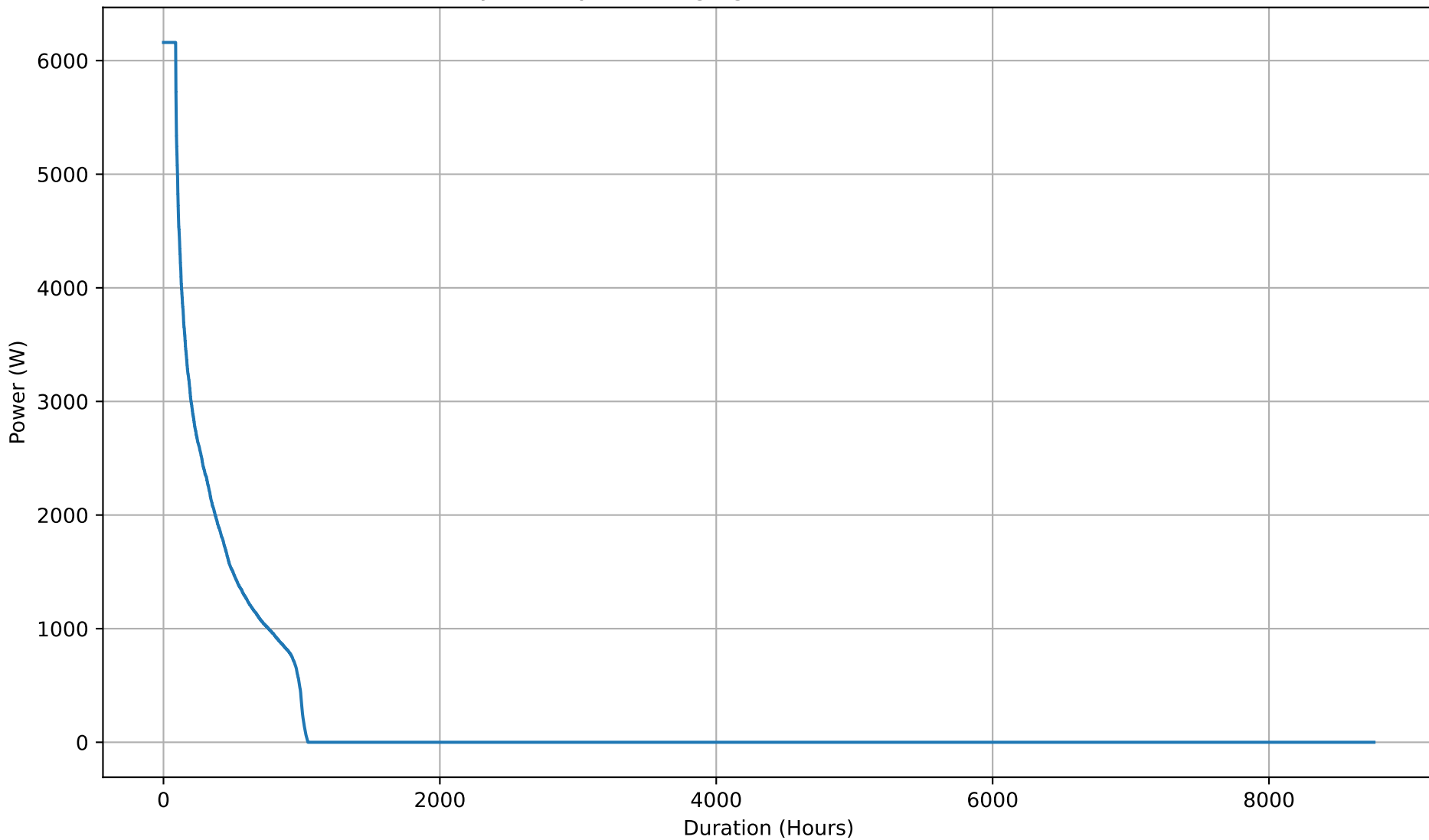
Yearly Battery Discharging Power Duration Curve - 8kWh
