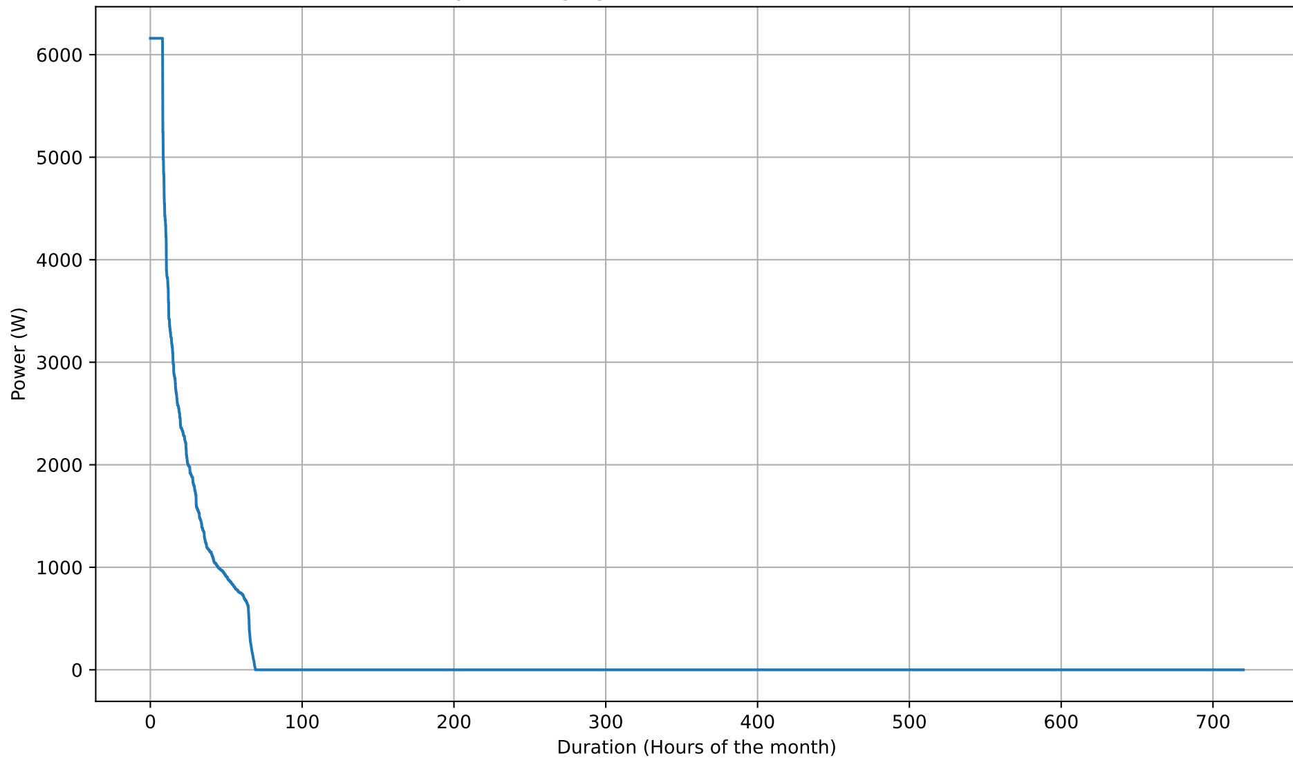
Battery Discharging Power Duration Curve - 8kWh - Nov
