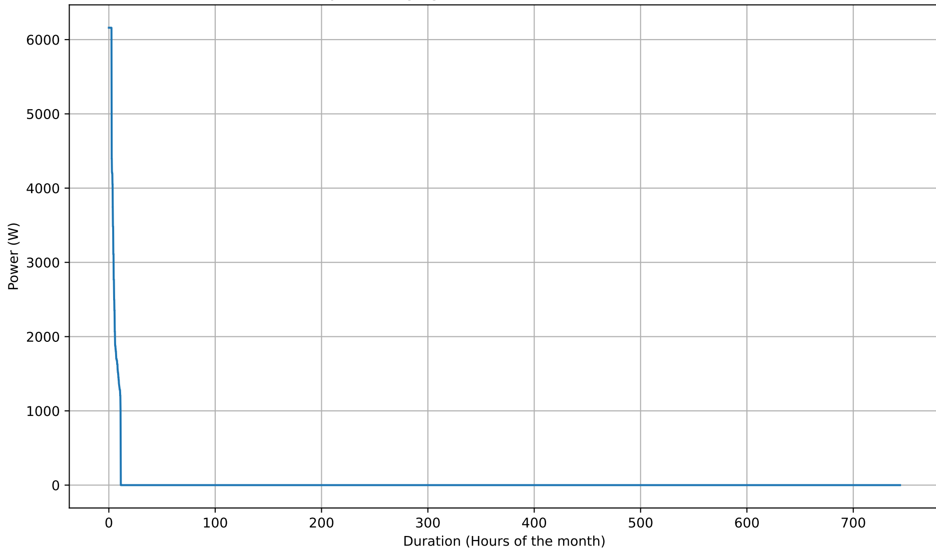
Battery Discharging Power Duration Curve - 8kWh - Dec
