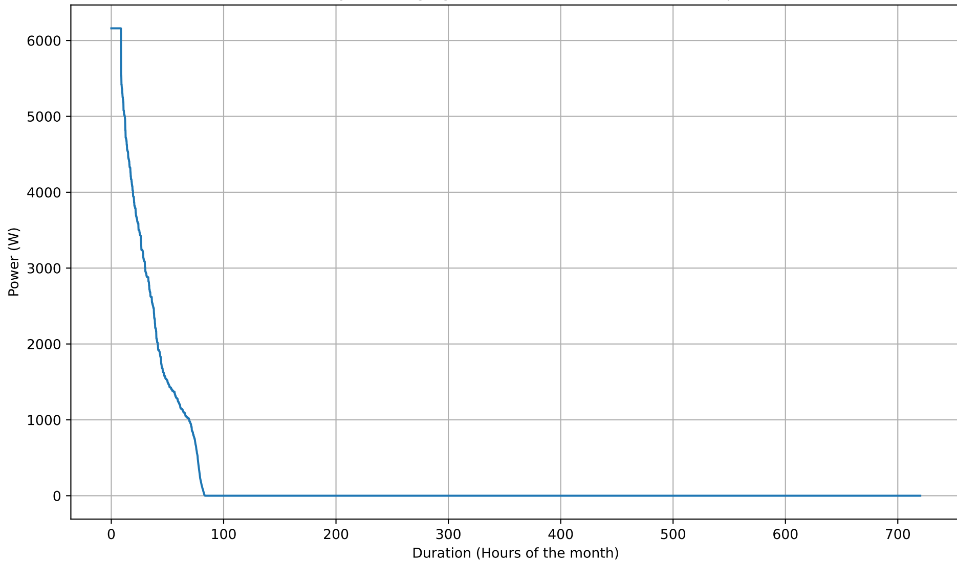
Battery Discharging Power Duration Curve - 8kWh - Apr
