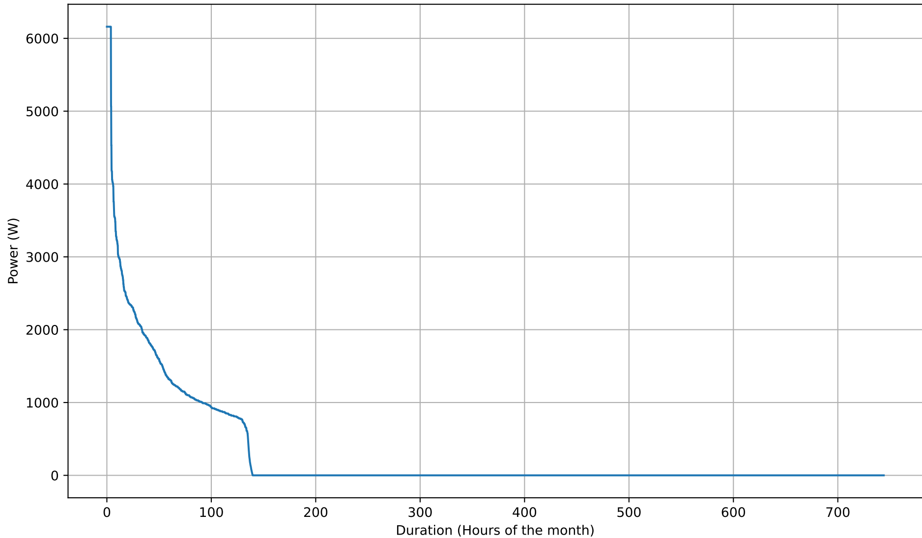
Battery Discharging Power Duration Curve - 8kWh - Jul
