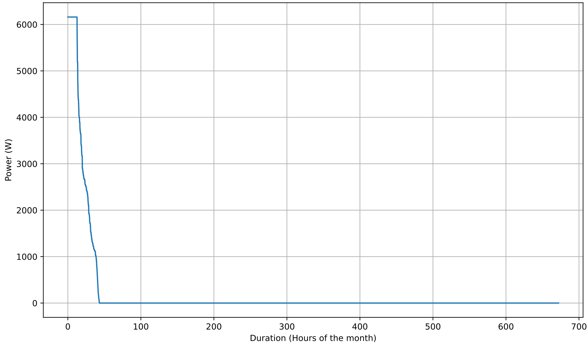
Battery Discharging Power Duration Curve - 8kWh - Feb
