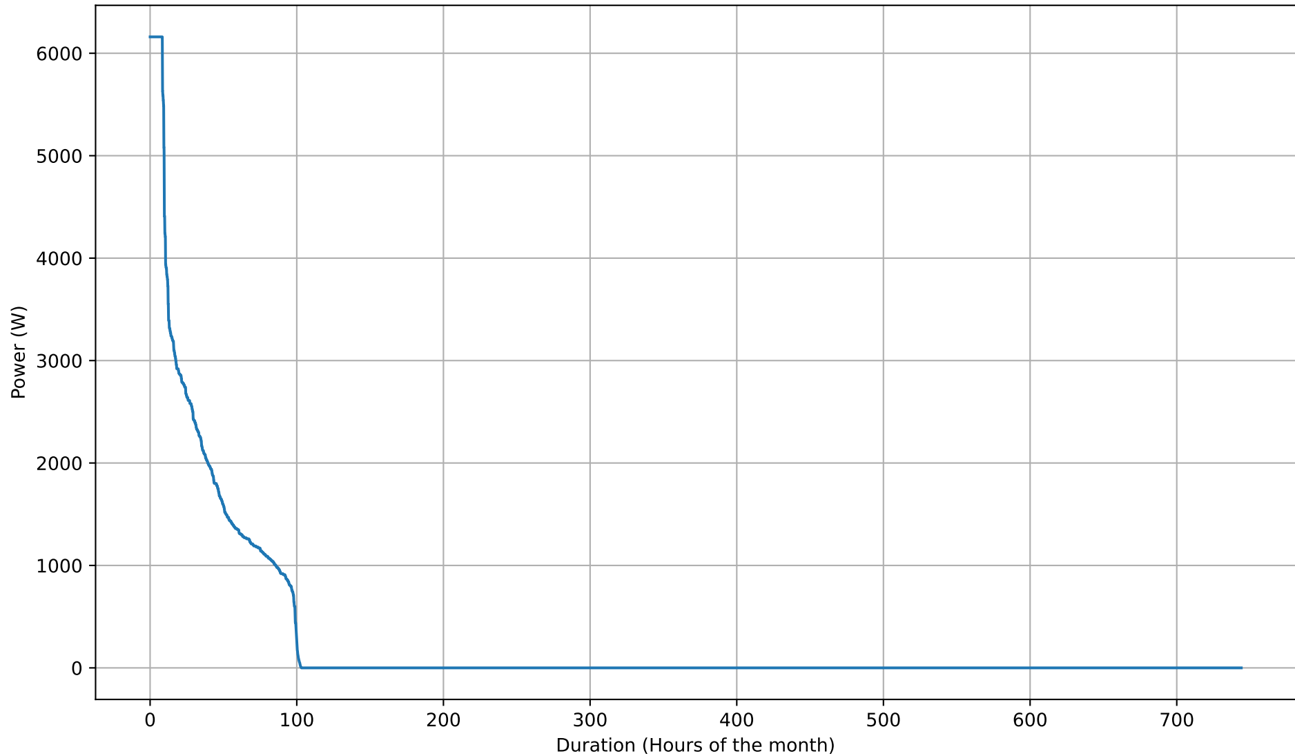
Battery Discharging Power Duration Curve - 8kWh - May
