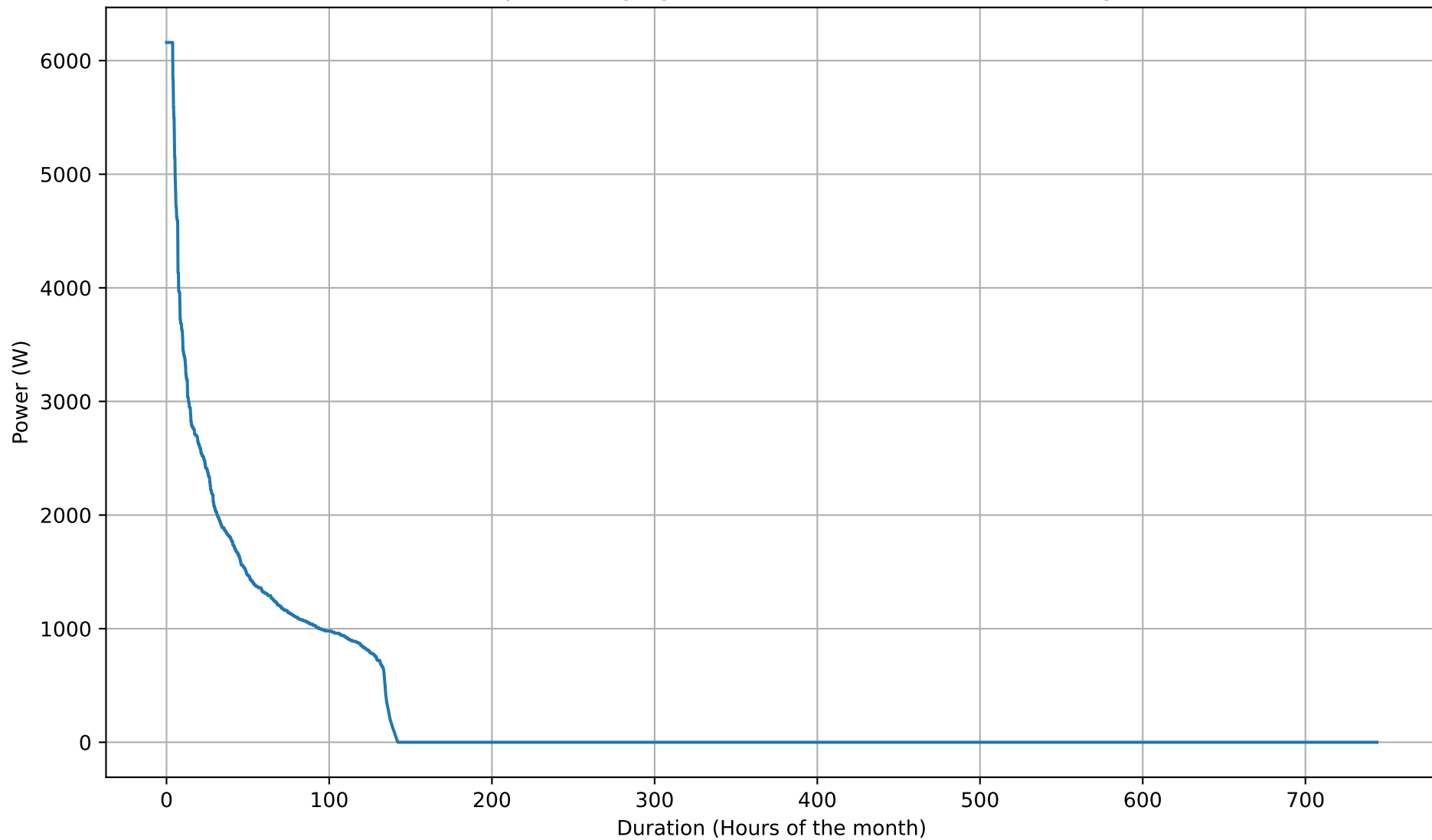
Battery Discharging Power Duration Curve - 8kWh - Aug
