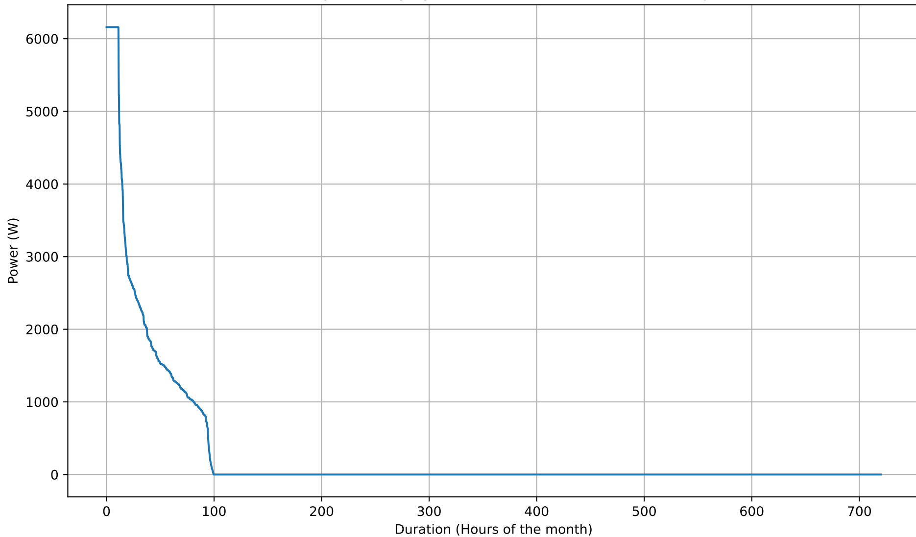
Battery Discharging Power Duration Curve - 8kWh - Sep
