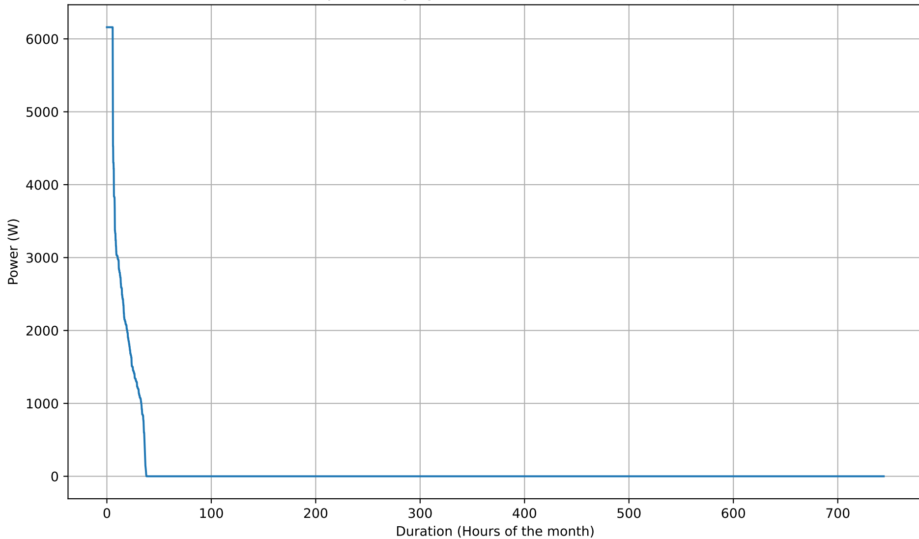
Battery Discharging Power Duration Curve - 8kWh - Jan
