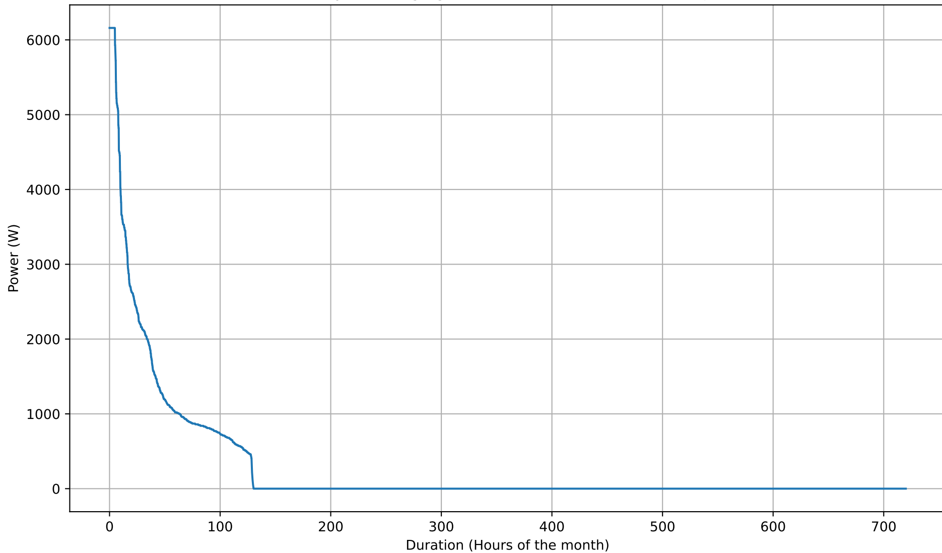
Battery Discharging Power Duration Curve - 8kWh - Jun
