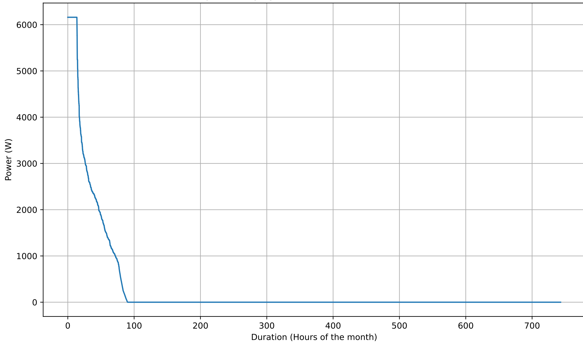
Battery Discharging Power Duration Curve - 8kWh - Mar
