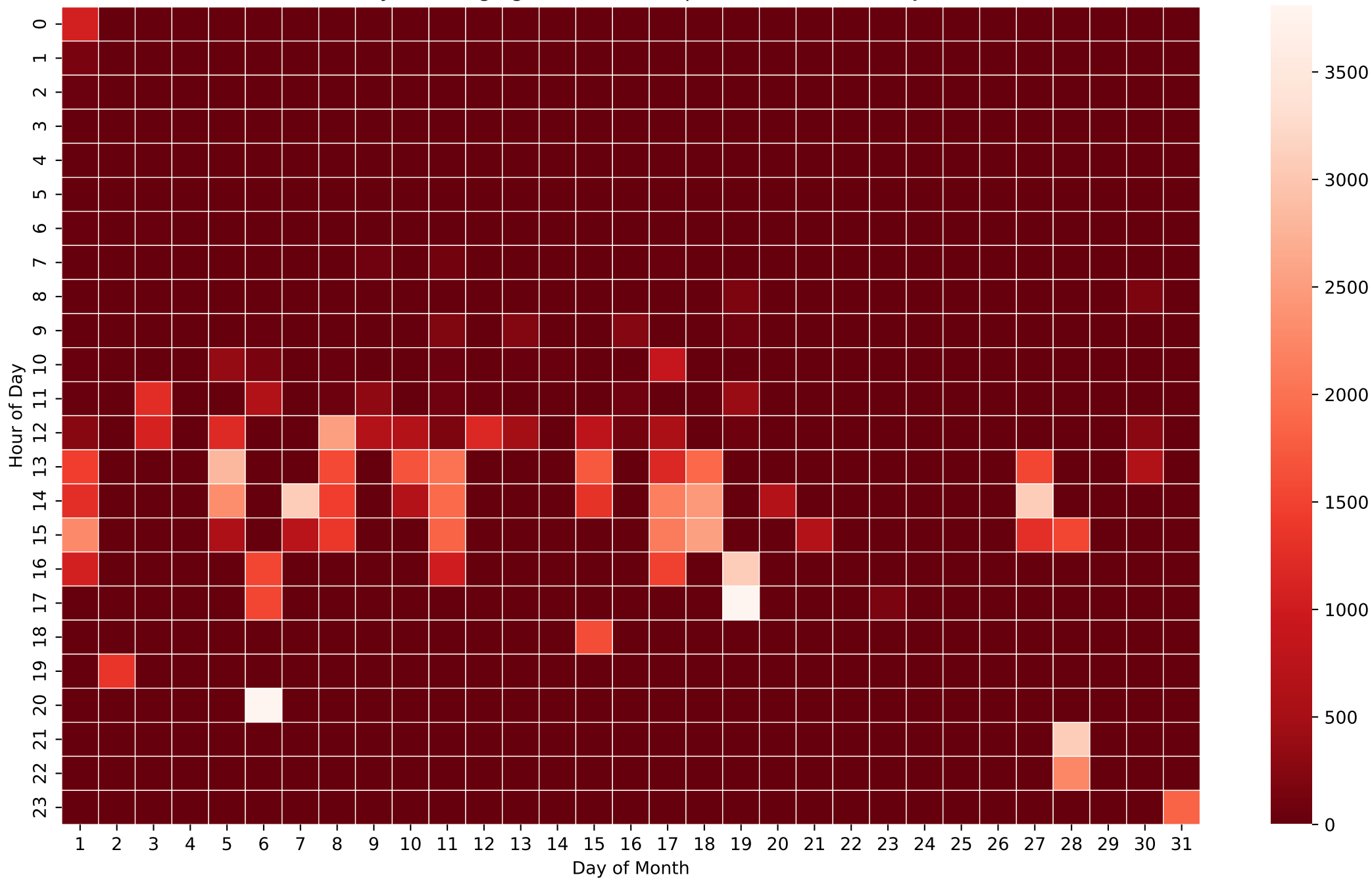
Battery Discharging Power Heatmap (Wh/Hour) - 8kWh - Jan
