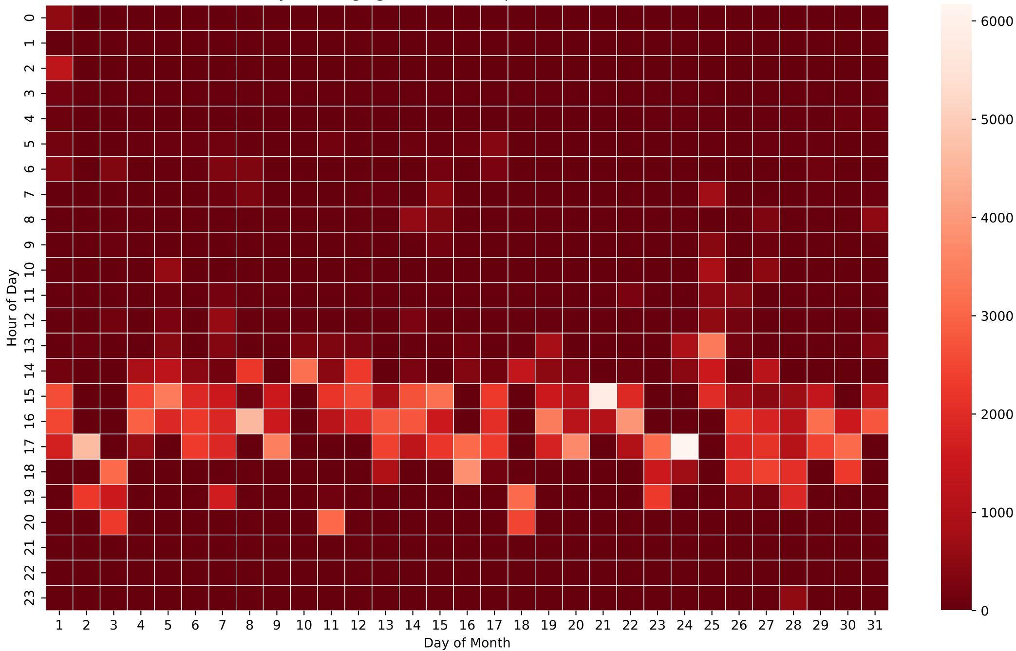
Battery Discharging Power Heatmap (Wh/Hour) - 8kWh - Mar
