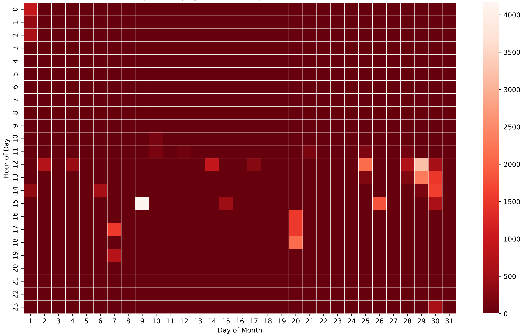
Battery Discharging Power Heatmap (Wh/Hour) - 8kWh - Dec
