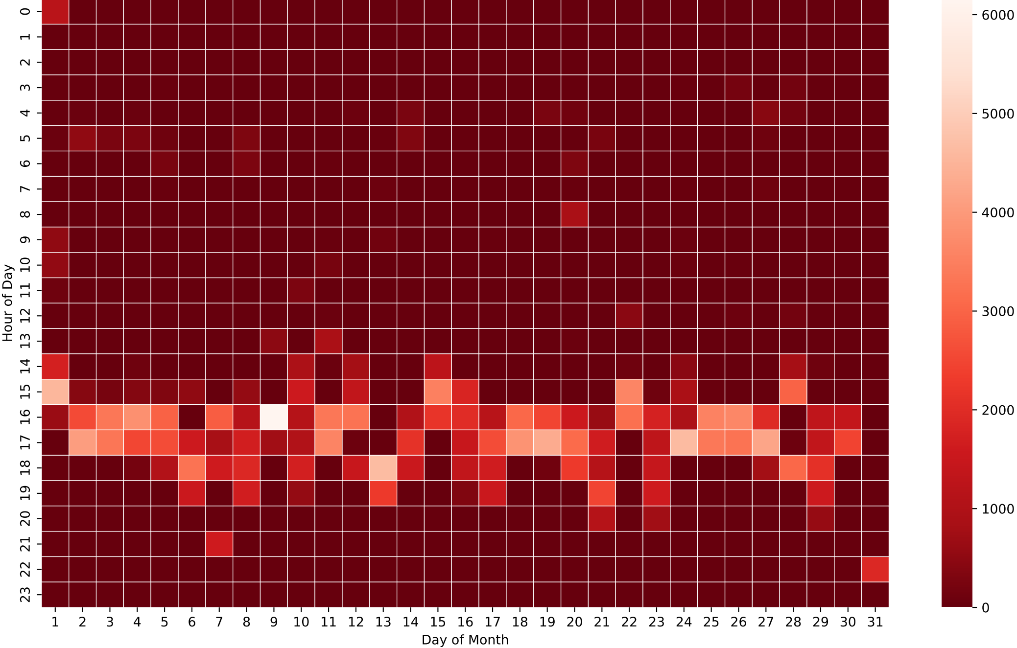
Battery Discharging Power Heatmap (Wh/Hour) - 8kWh - April
