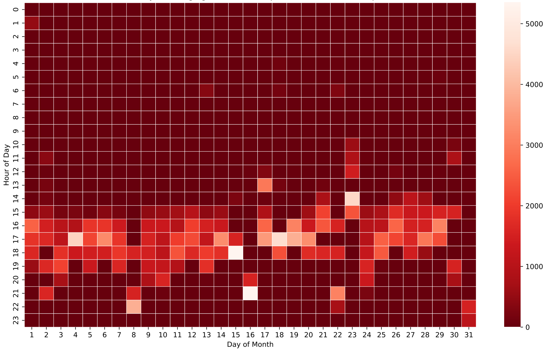
Battery Discharging Power Heatmap (Wh/Hour) - 8kWh - Sep
