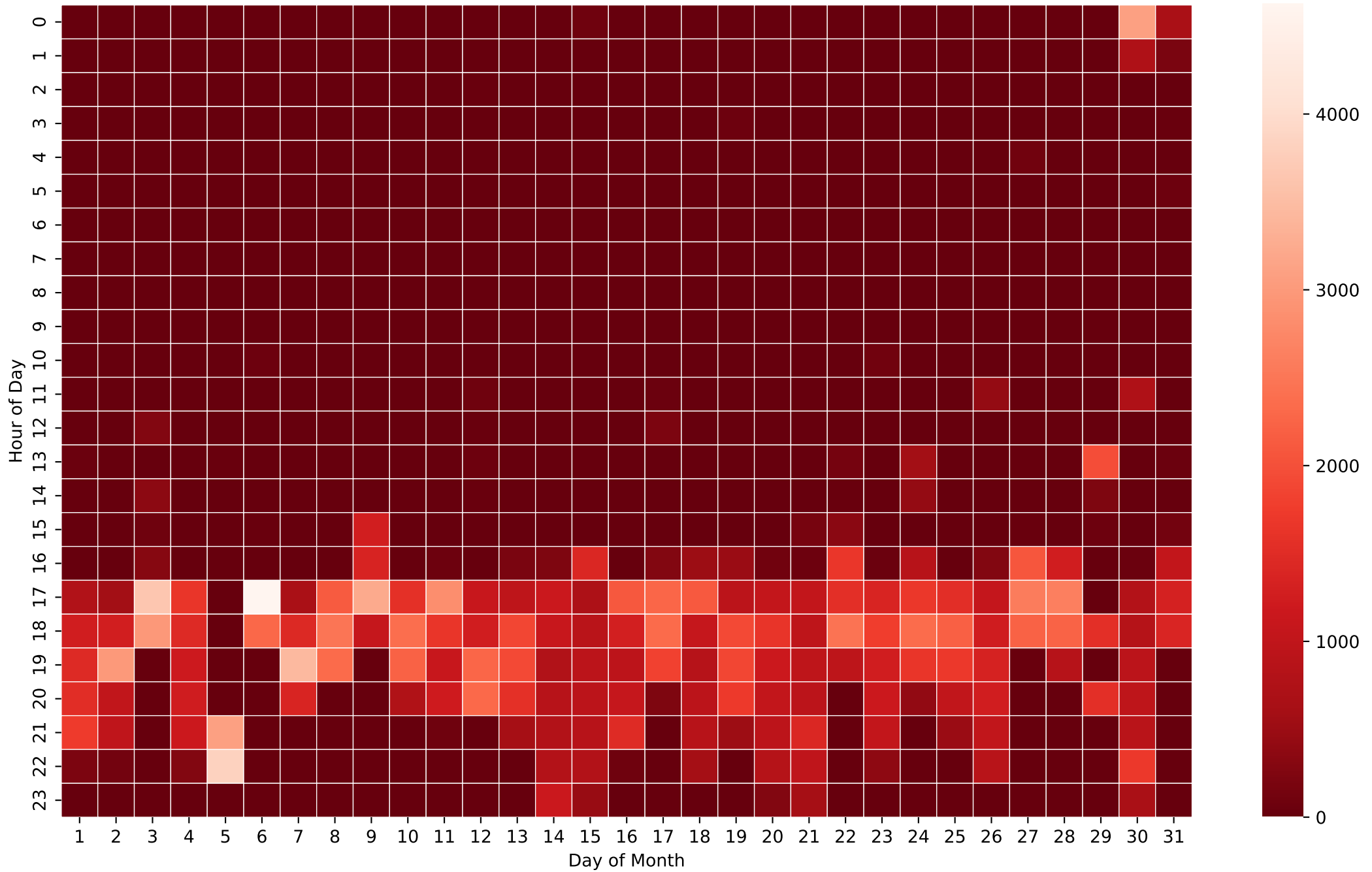
Battery Discharging Power Heatmap (Wh/Hour) - 8kWh - Jul
