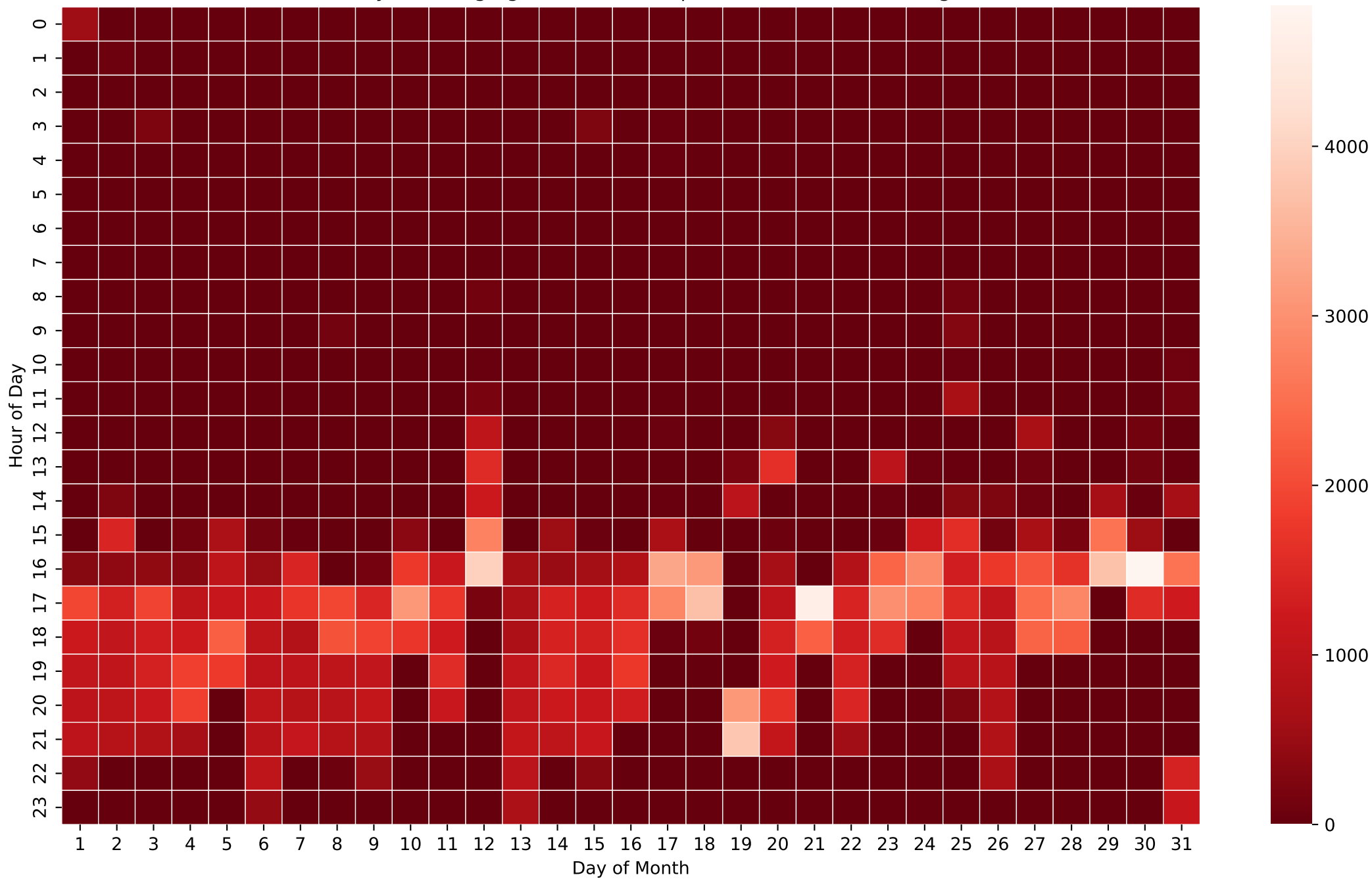
Battery Discharging Power Heatmap (Wh/Hour) - 8kWh - Aug
