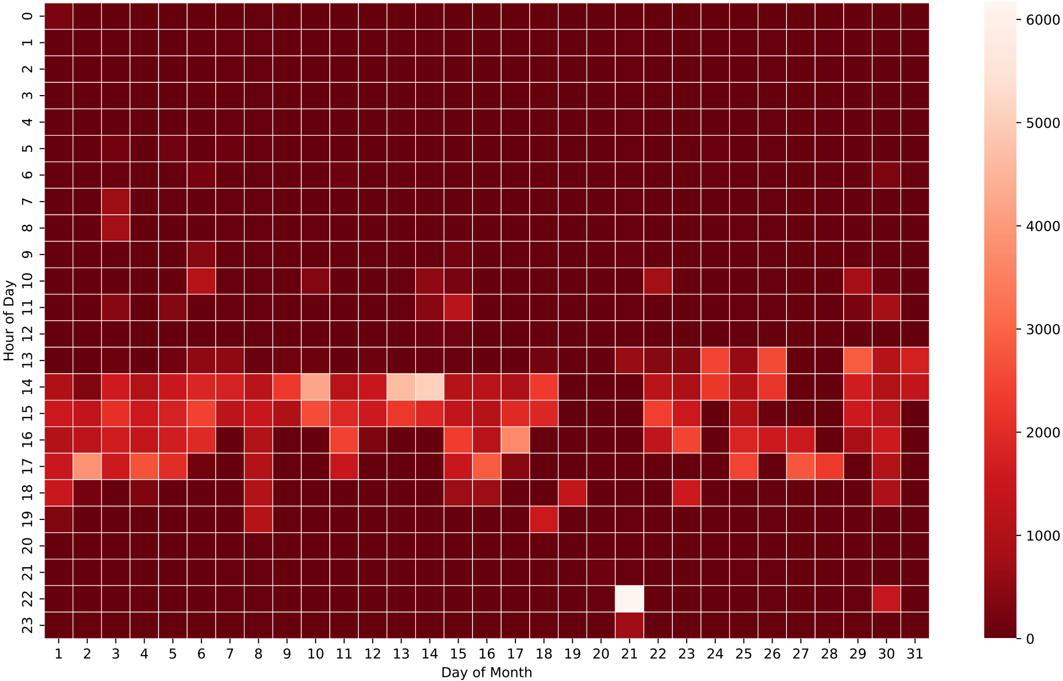
Battery Discharging Power Heatmap (Wh/Hour) - 8kWh - Oct
