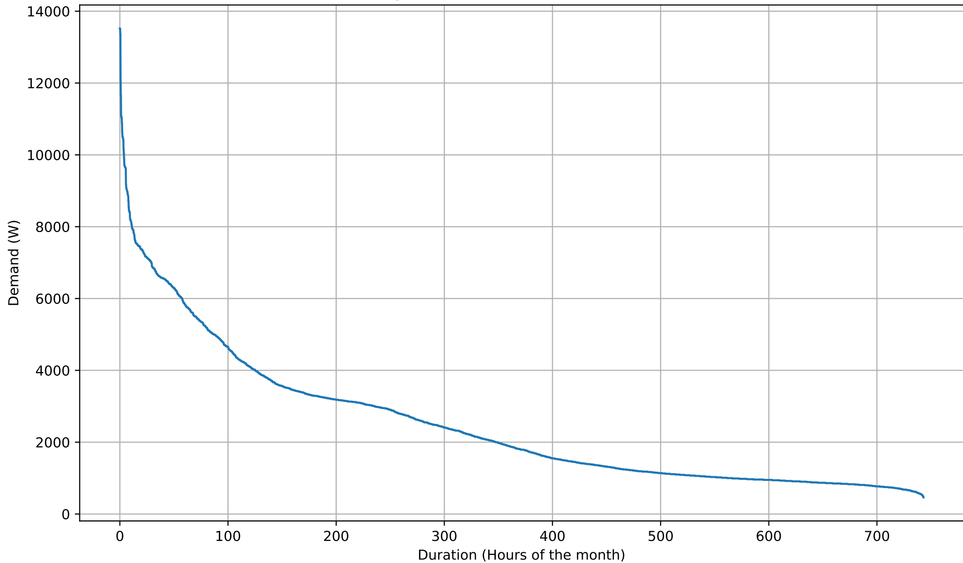
Electricity Demand Duration Curve - 8kWh - Mar
