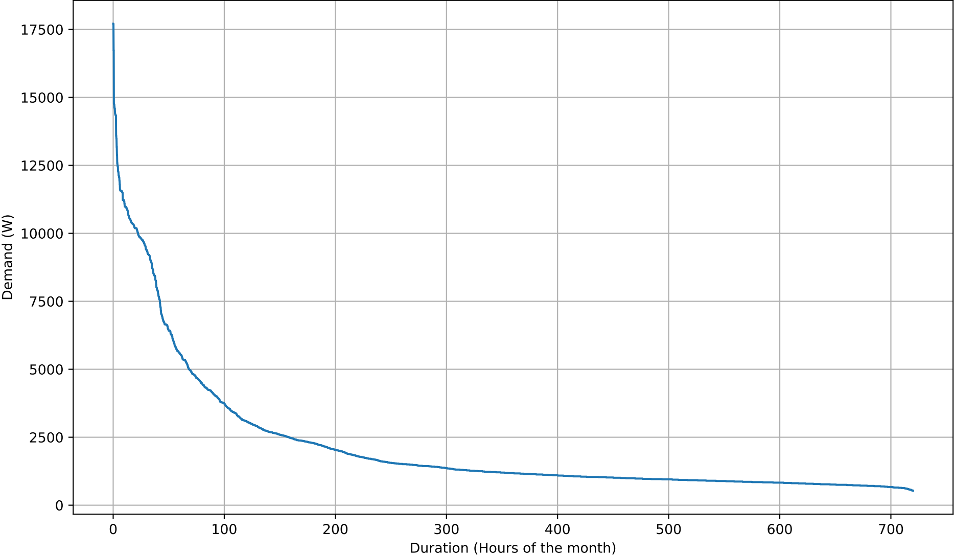
Electricity Demand Duration Curve - 8kWh - Sep
