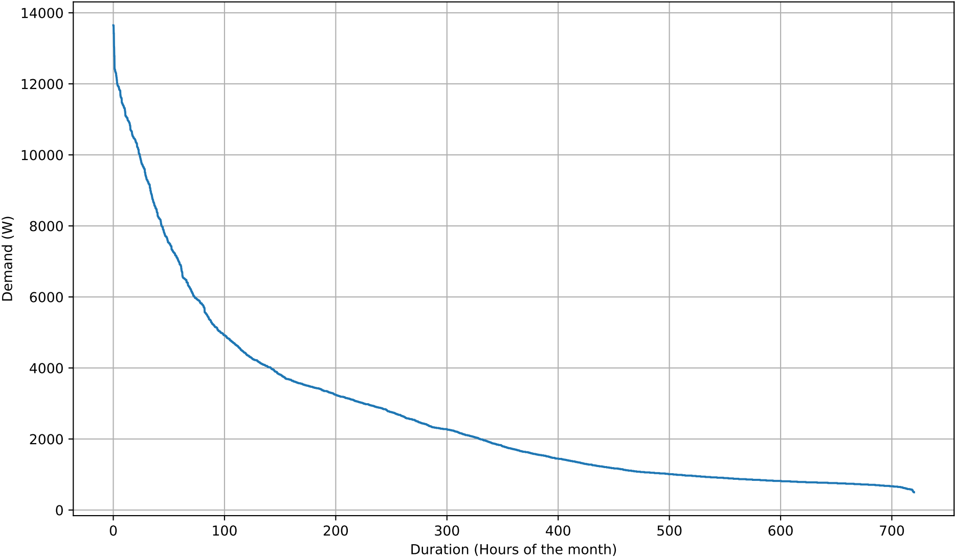
Electricity Demand Duration Curve - 8kWh - Nov
