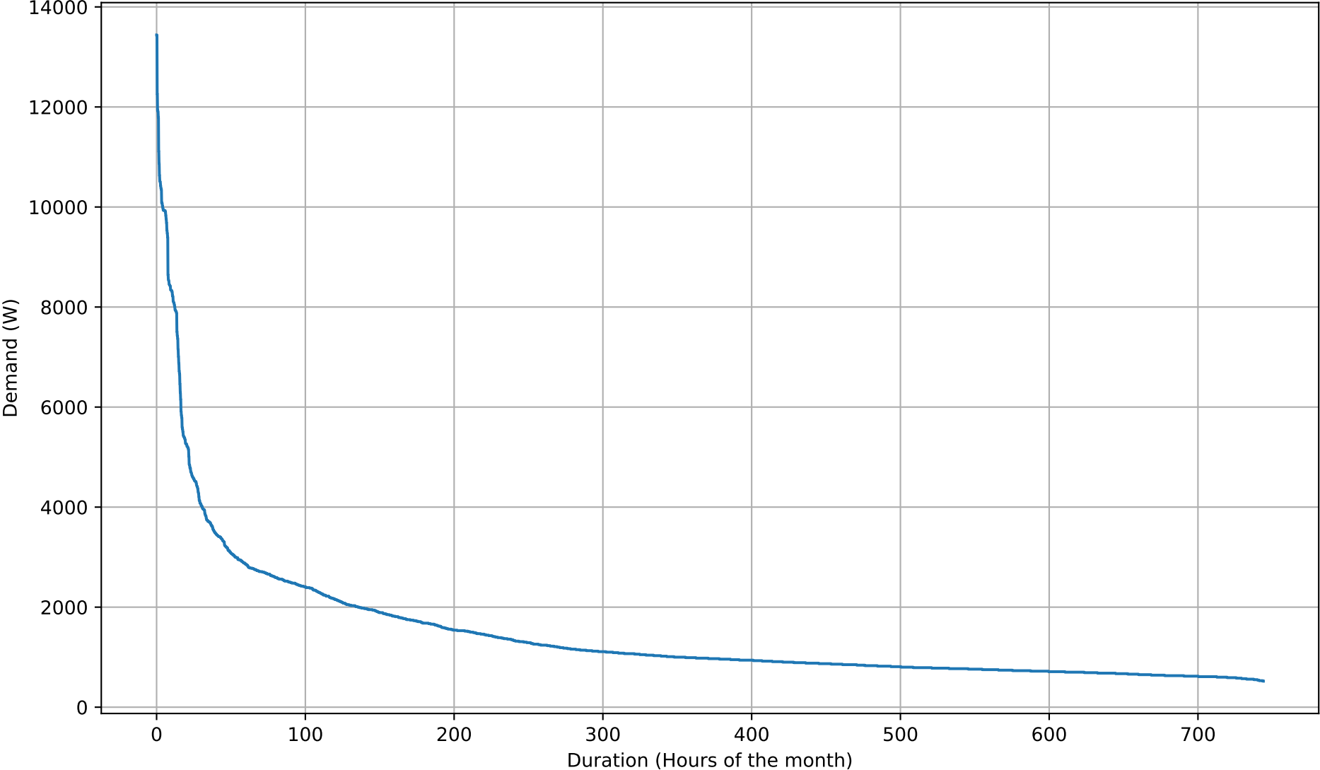
Electricity Demand Duration Curve - 8kWh - Aug
