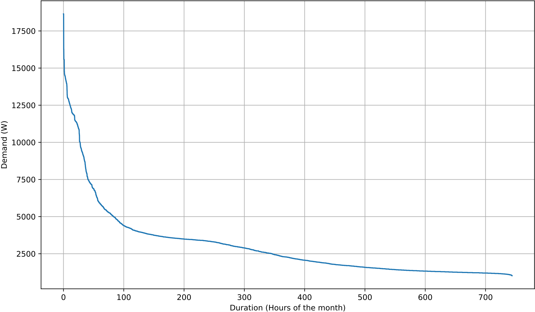
Electricity Demand Duration Curve - 8kWh - Dec
