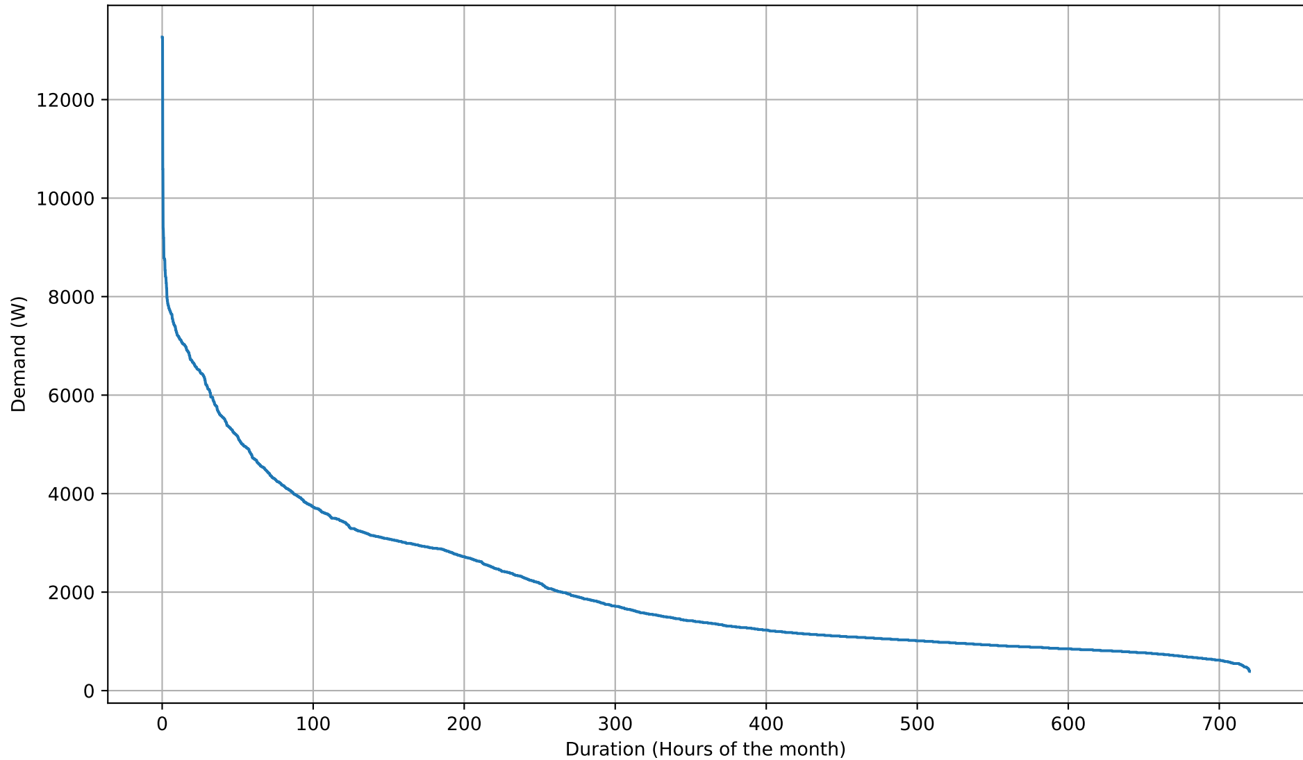
Electricity Demand Duration Curve - 8kWh - Apr
