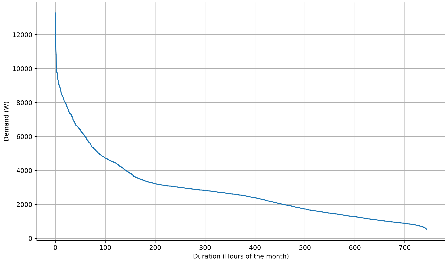
Electricity Demand Duration Curve - 8kWh - Jan
