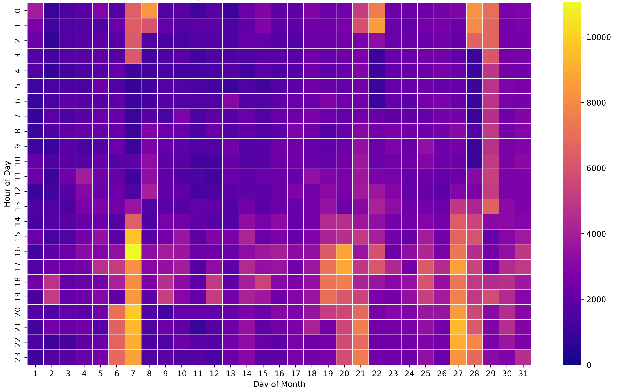
Electricity Demand Heatmap (Wh/Hour) - 8kWh - Jan
