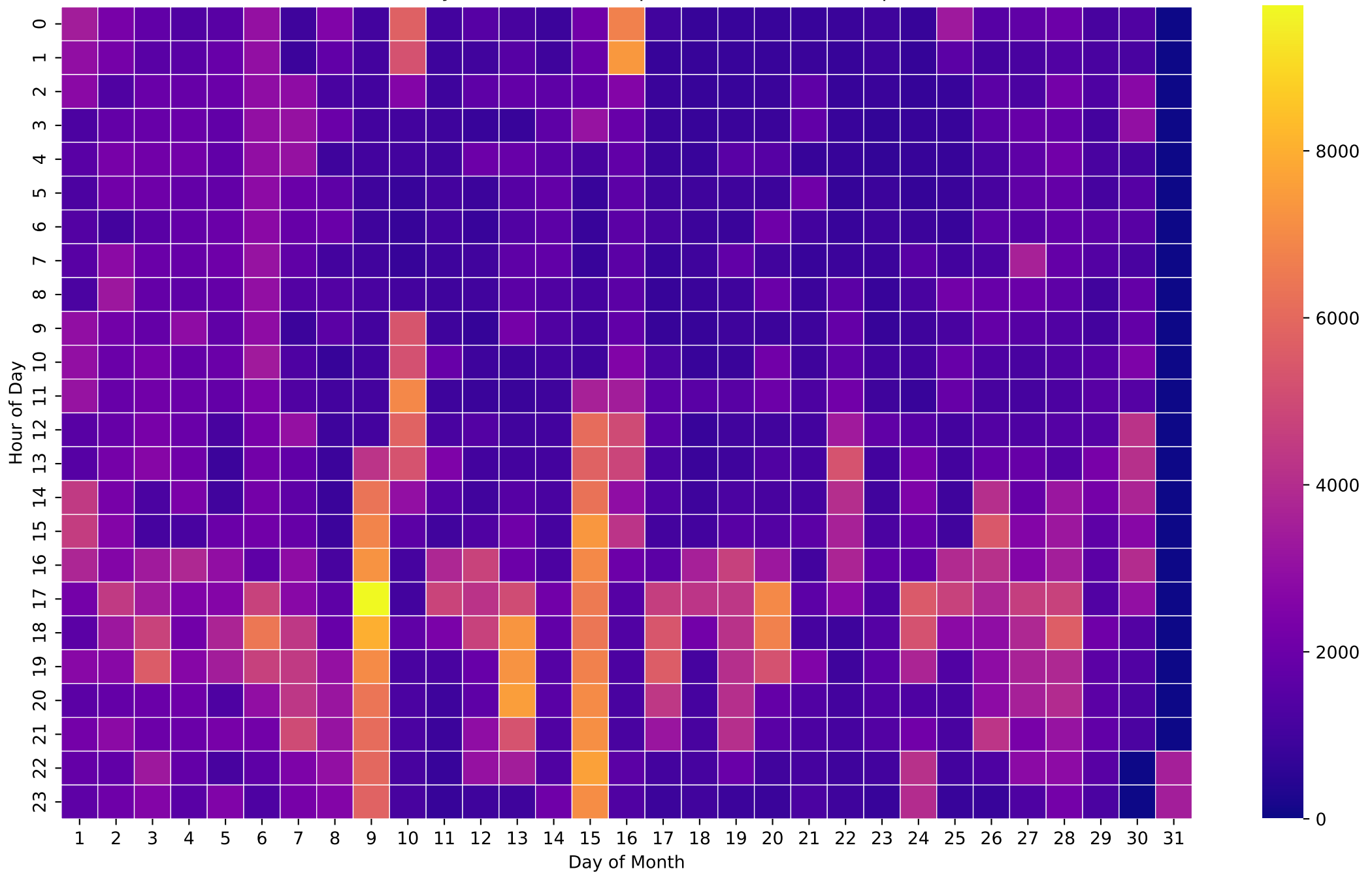
Electricity Demand Heatmap (Wh/Hour) - 8kWh - Apr
