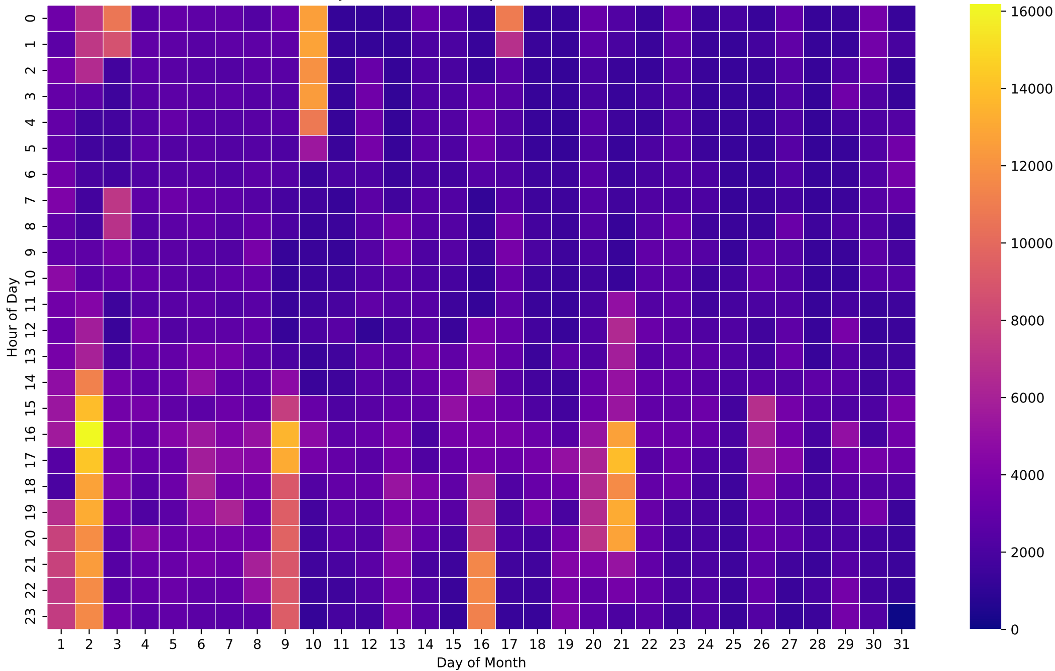
Electricity Demand Heatmap (Wh/Hour) - 8kWh - Dec
