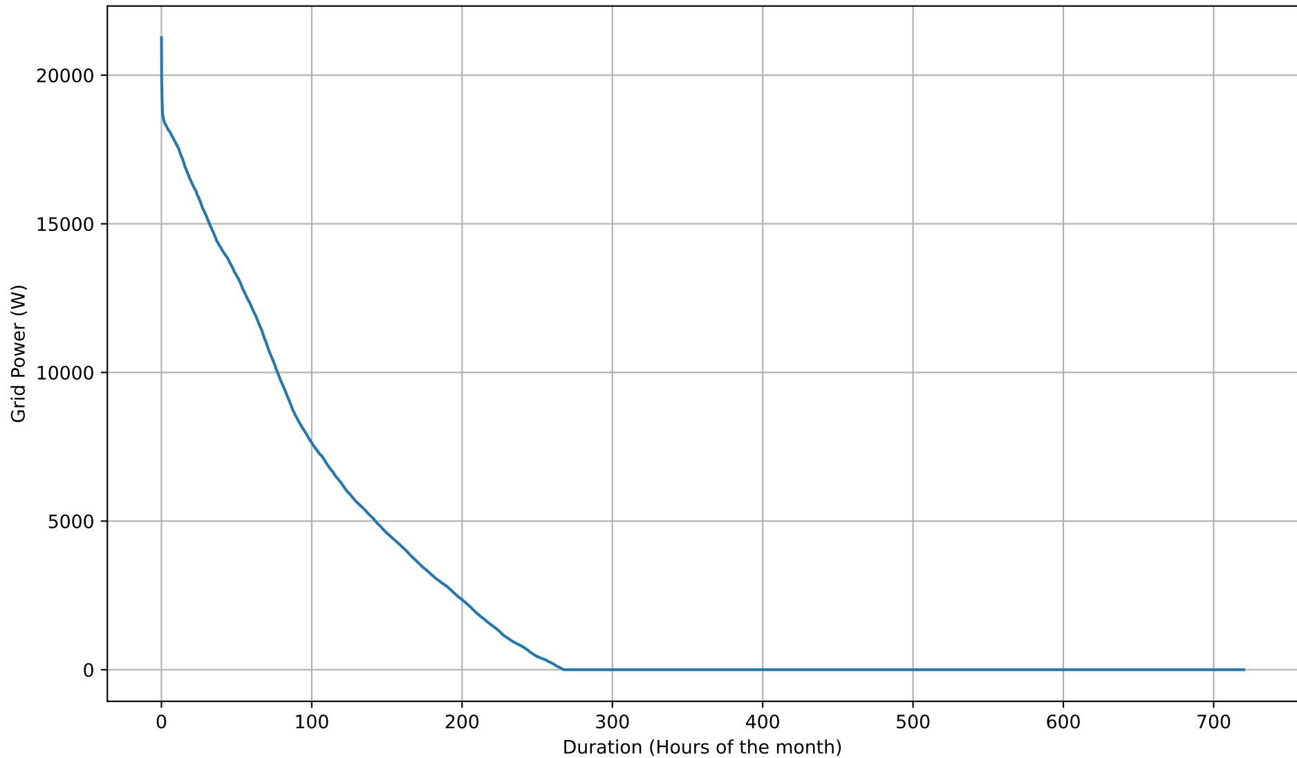
Grid Export Duration Curve - 8kWh - Sep
