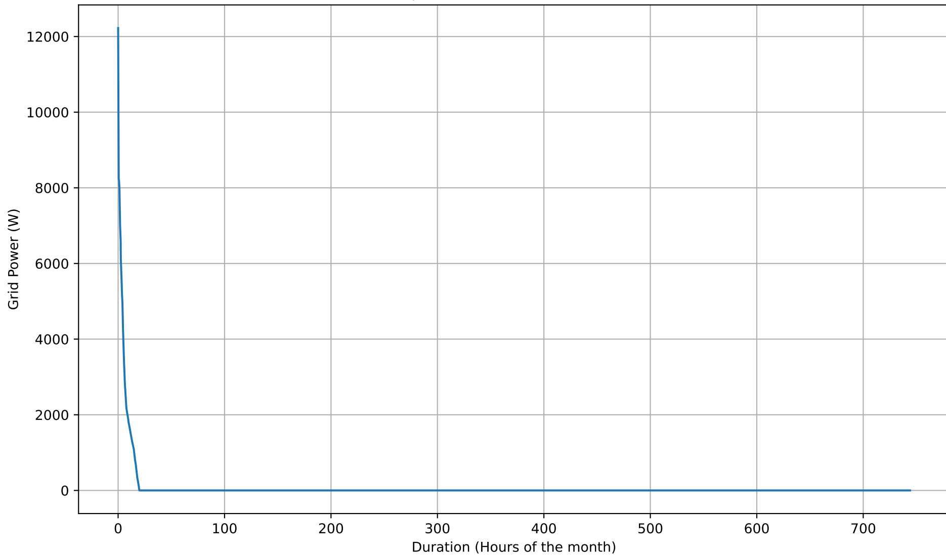
Grid Export Duration Curve - 8kWh - Jan
