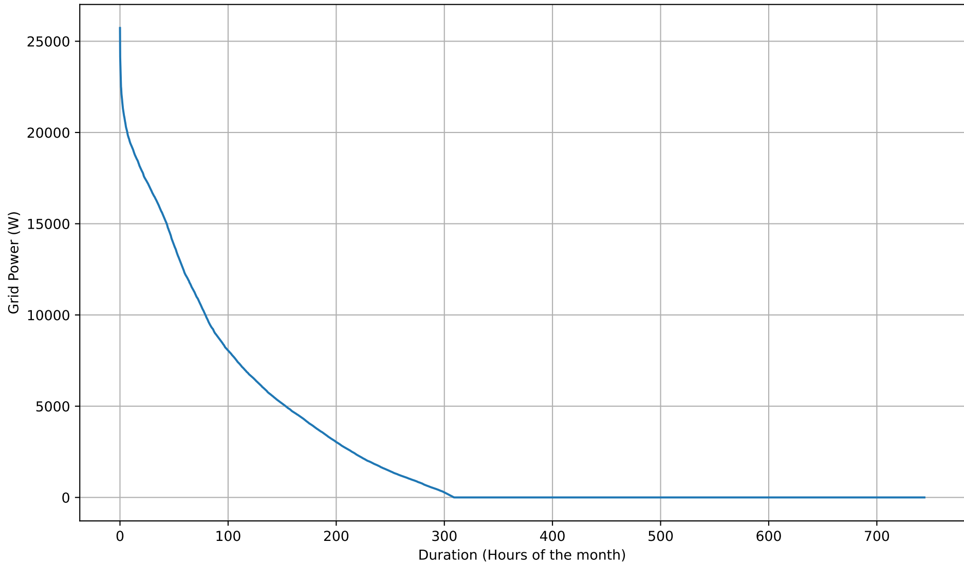
Grid Export Duration Curve - 8kWh - Aug
