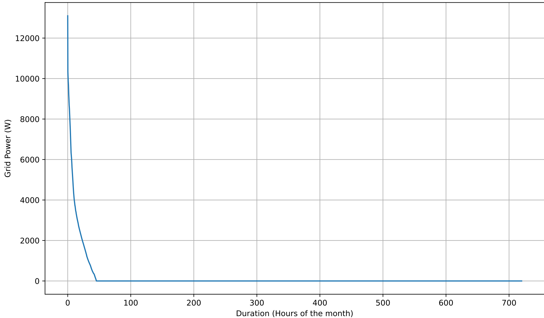
Grid Export Duration Curve - 8kWh - Nov
