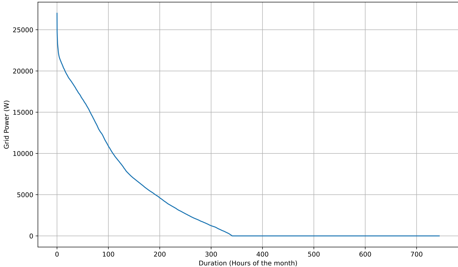
Grid Export Duration Curve - 8kWh - May
