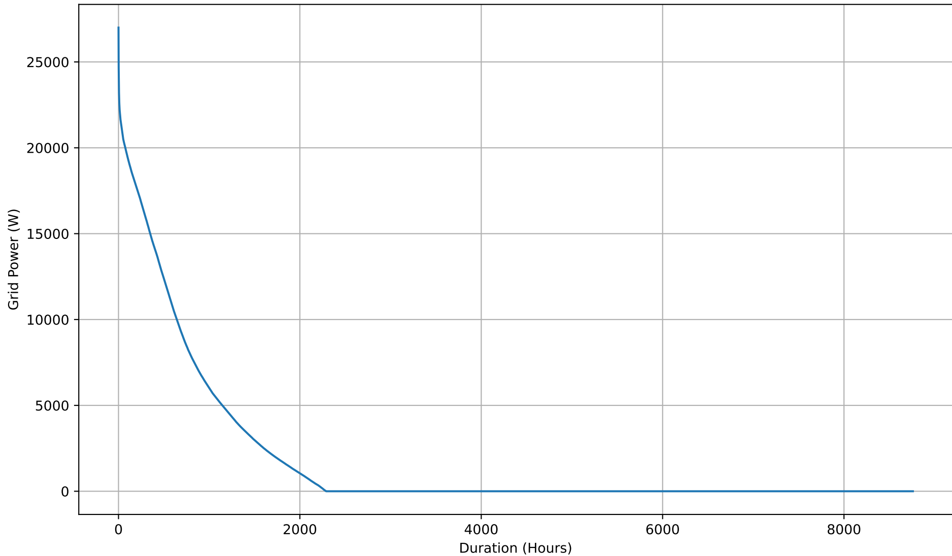
Yearly Grid Export Duration Curve - 8kWh
