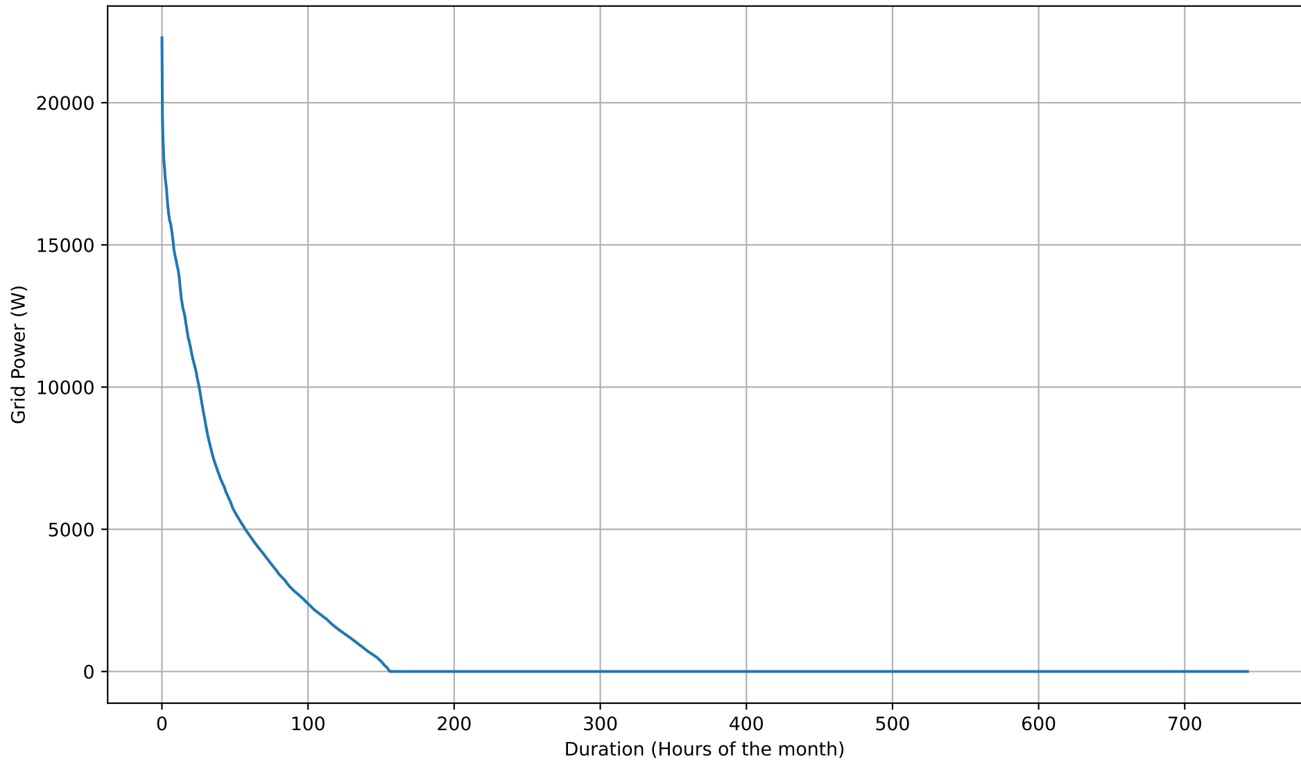
Grid Export Duration Curve - 8kWh - Mar
