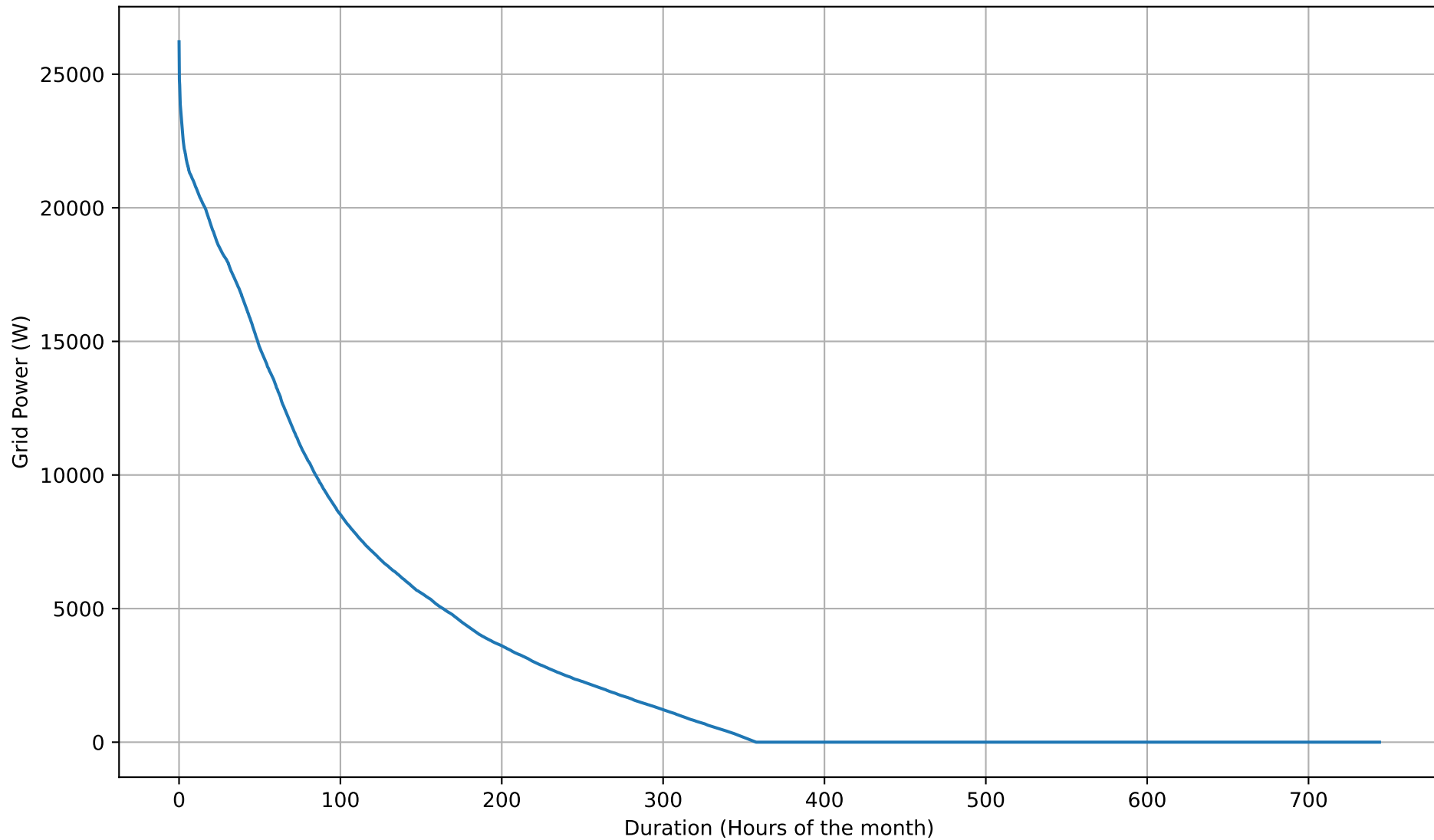
Grid Export Duration Curve - 8kWh - Jul
