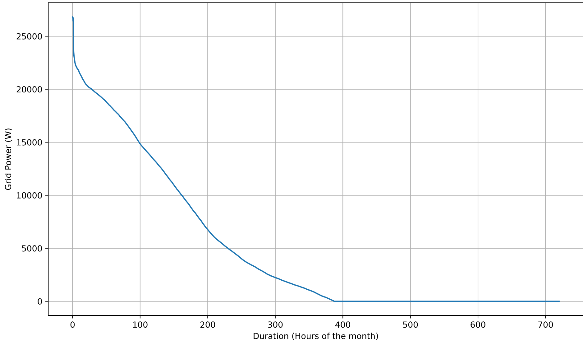
Grid Export Duration Curve - 8kWh - Jun
