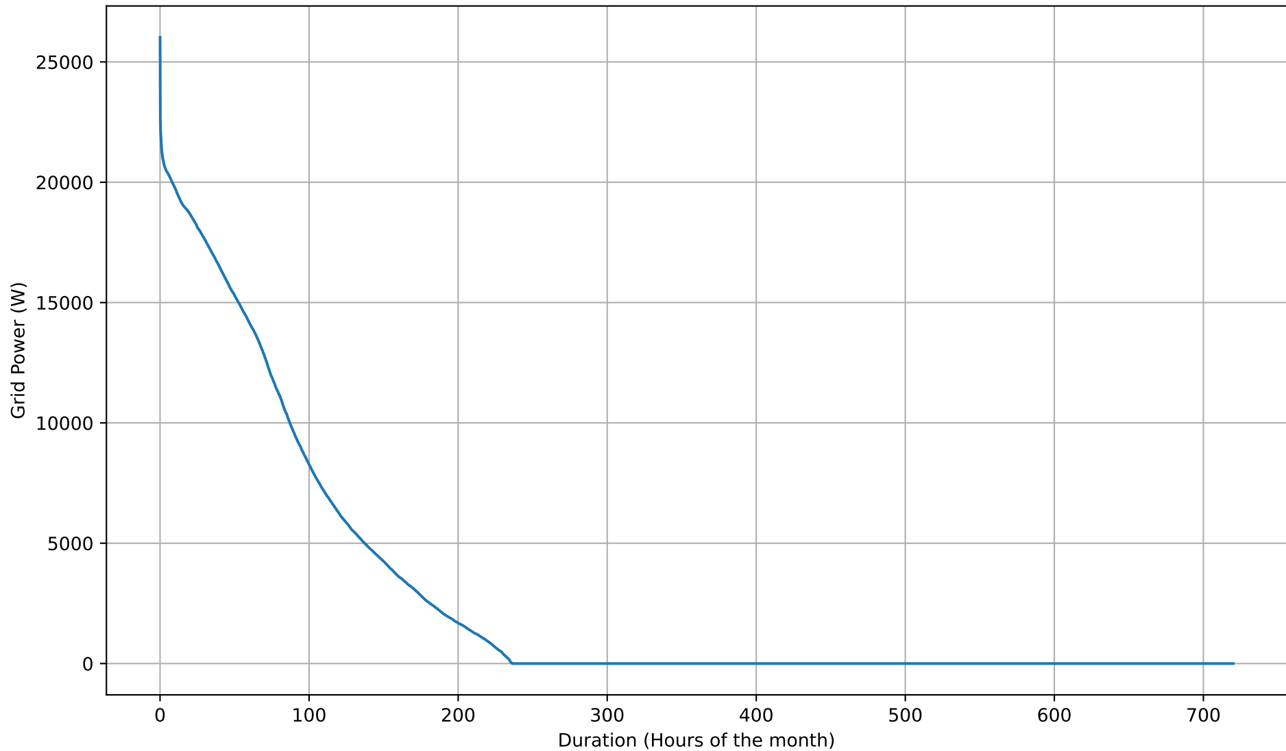
Grid Export Duration Curve - 8kWh - Apr
