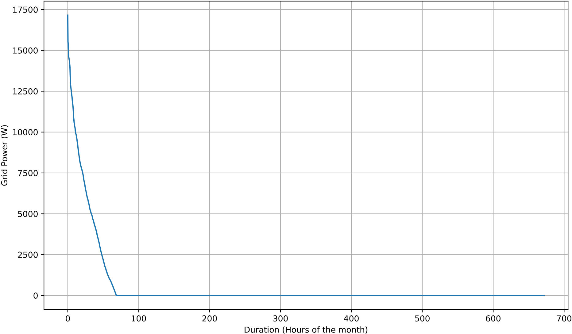
Grid Export Duration Curve - 8kWh - Feb
