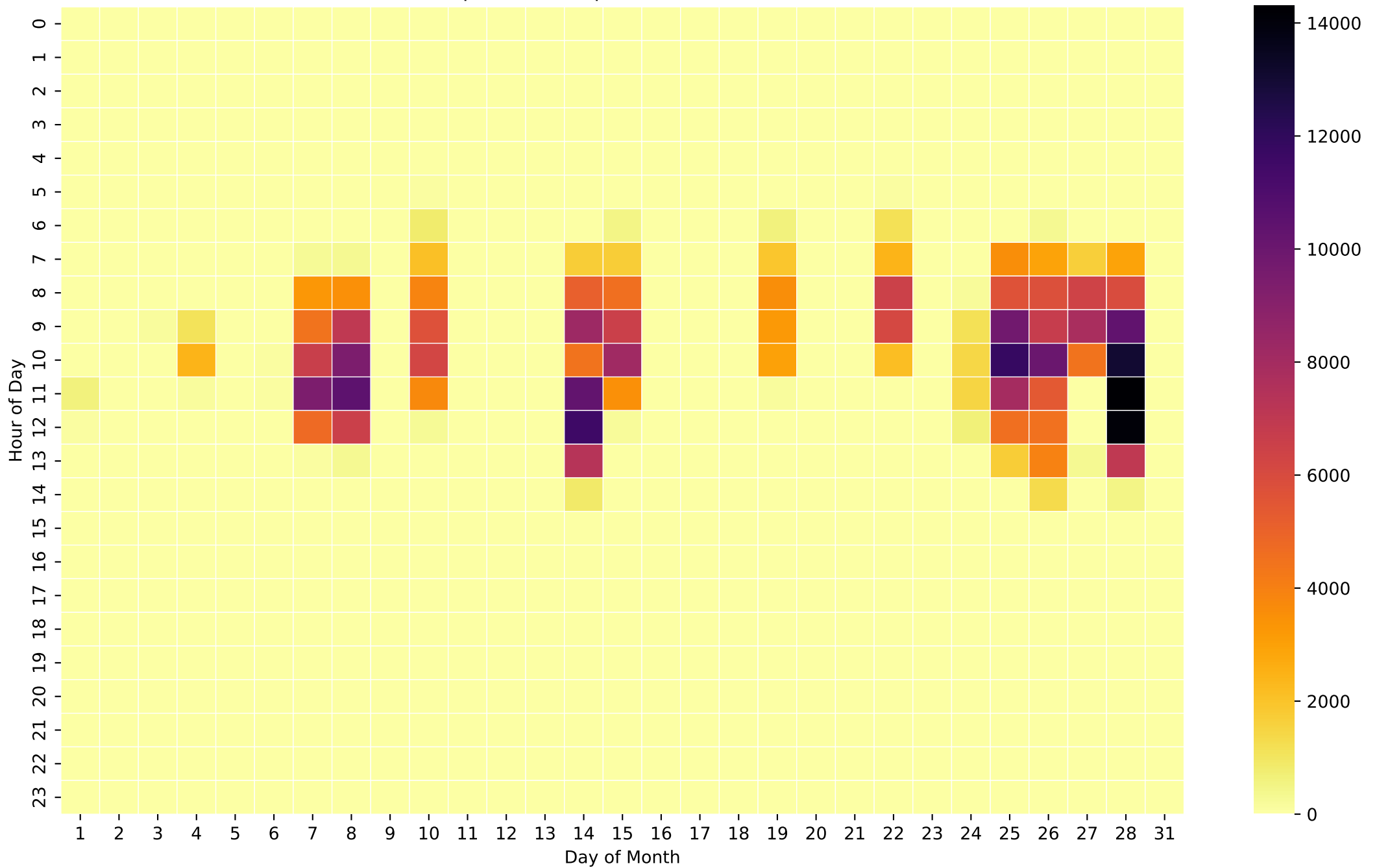
Grid Export Heatmap (Wh/Hour) - 8kWh - Feb
