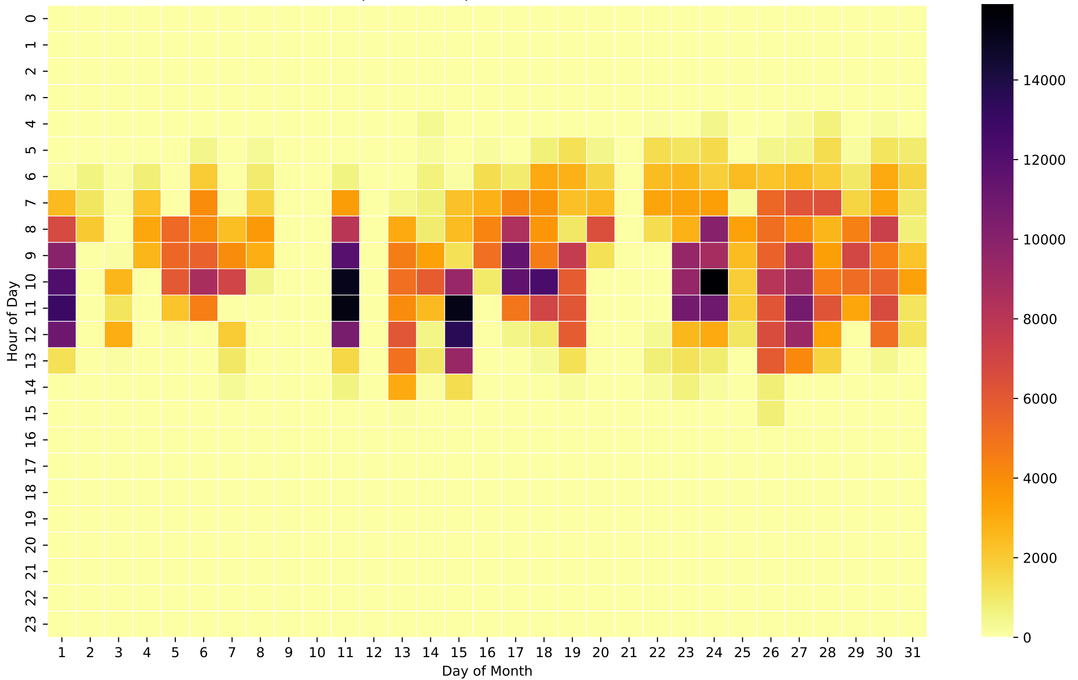
Grid Export Heatmap (Wh/Hour) - 8kWh - Mar
