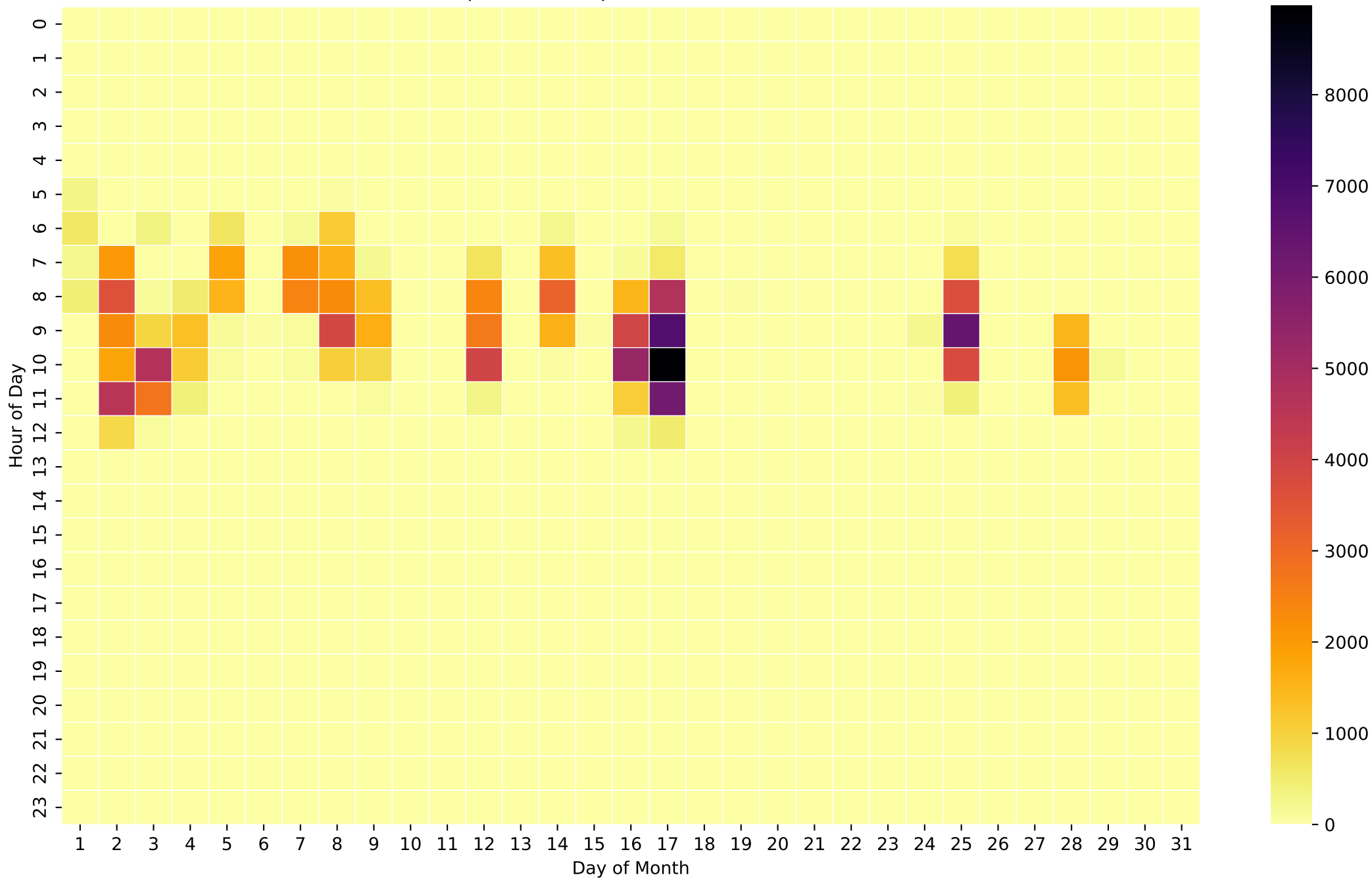
Grid Export Heatmap (Wh/Hour) - 8kWh - Nov
