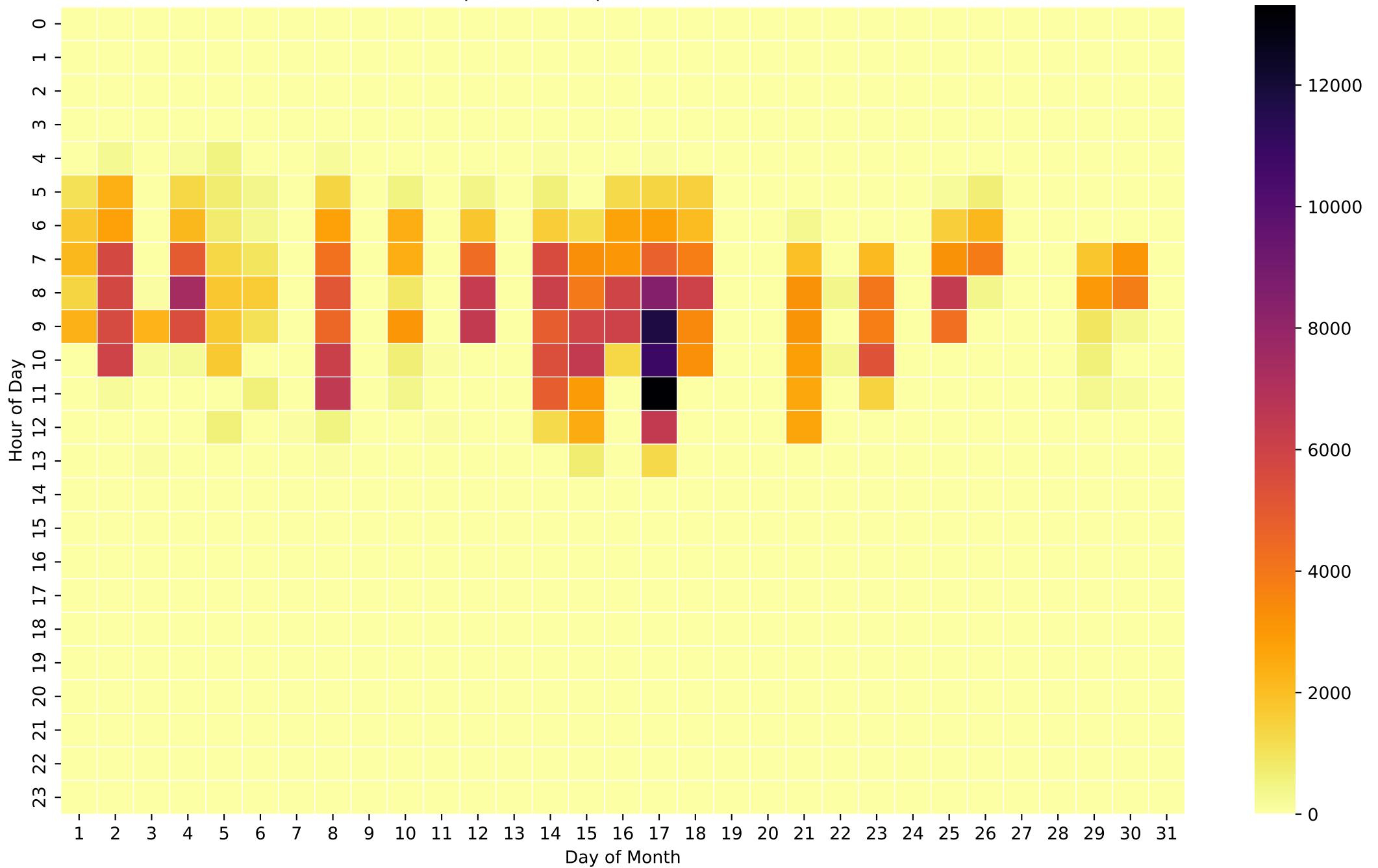
Grid Export Heatmap (Wh/Hour) - 8kWh - Oct
