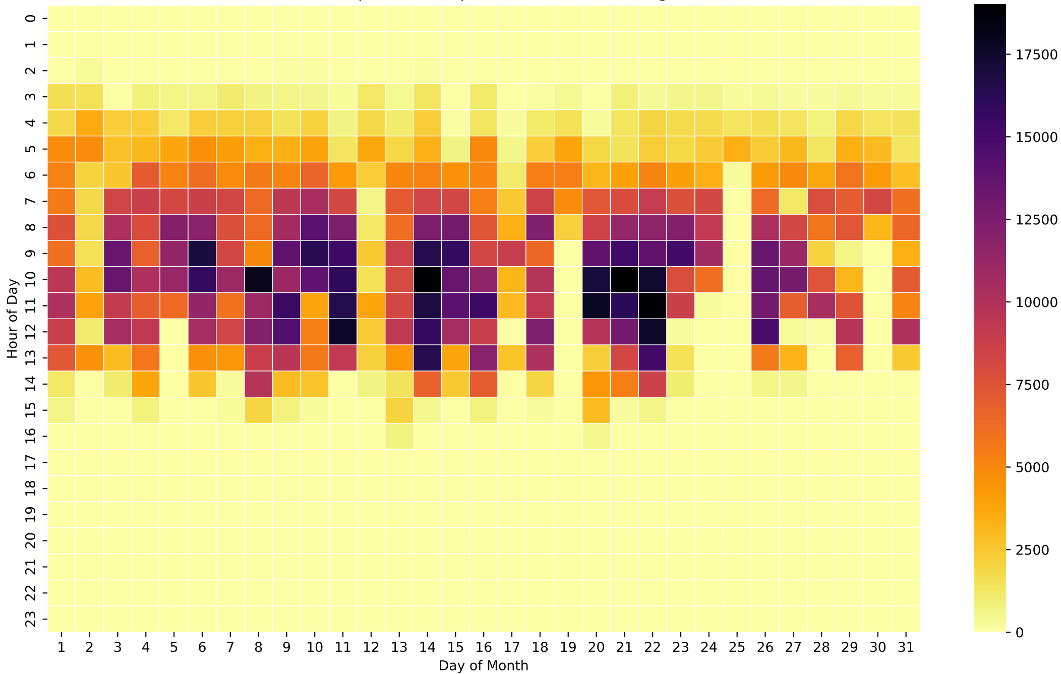
Grid Export Heatmap (Wh/Hour) - 8kWh - Aug
