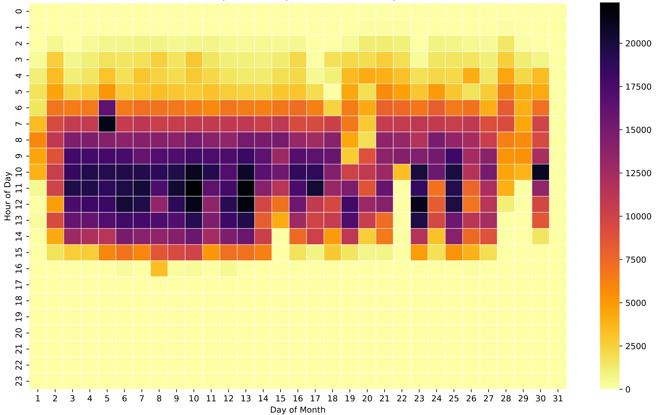
Grid Export Heatmap (Wh/Hour) - 8kWh - Jun
