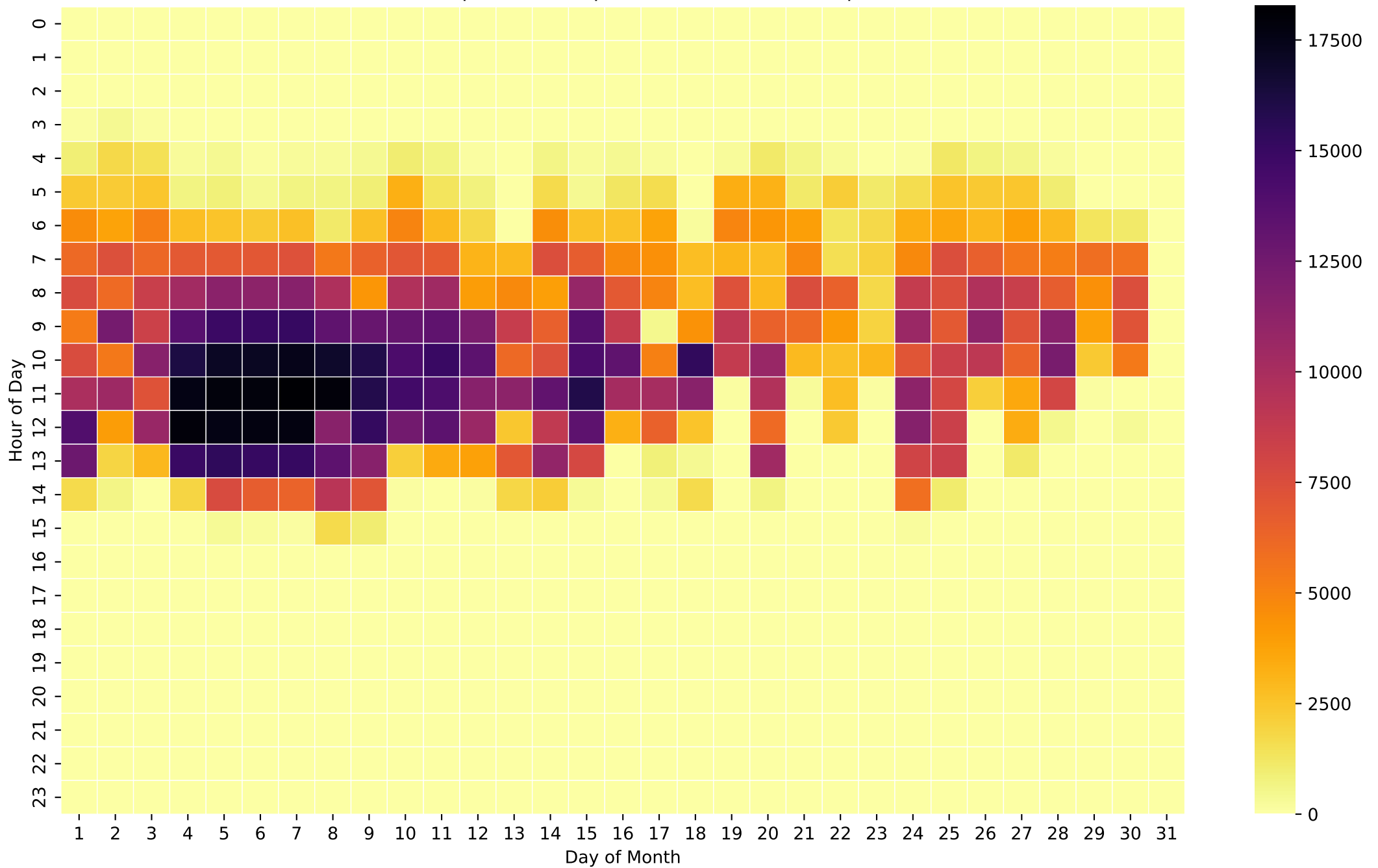
Grid Export Heatmap (Wh/Hour) - 8kWh - Sep
