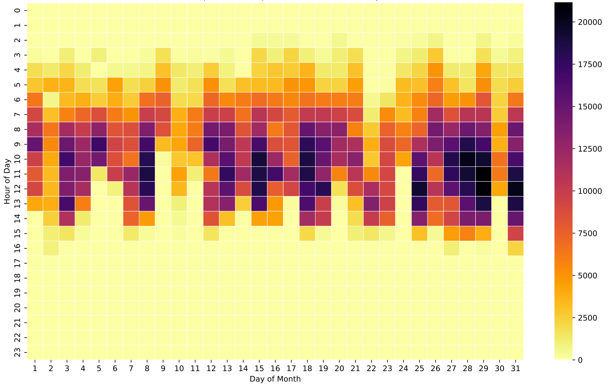
Grid Export Heatmap (Wh/Hour) - 8kWh - May
