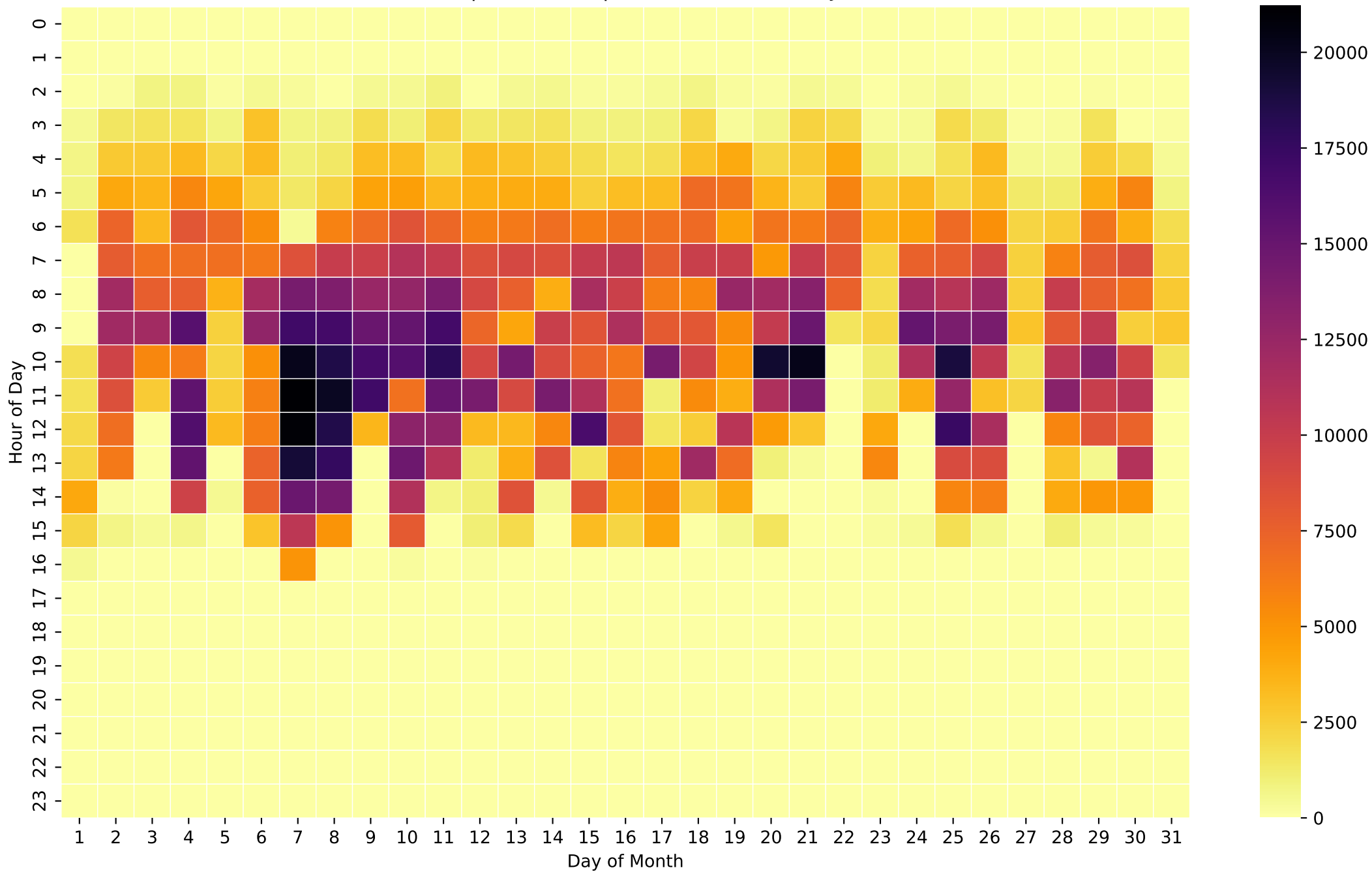
Grid Export Heatmap (Wh/Hour) - 8kWh - Jul
