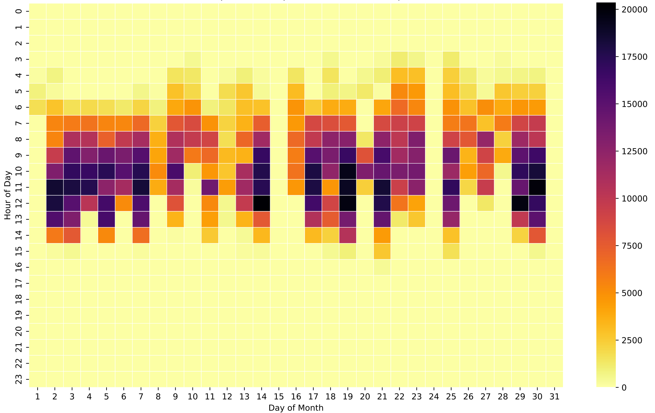
Grid Export Heatmap (Wh/Hour) - 8kWh - Apr
