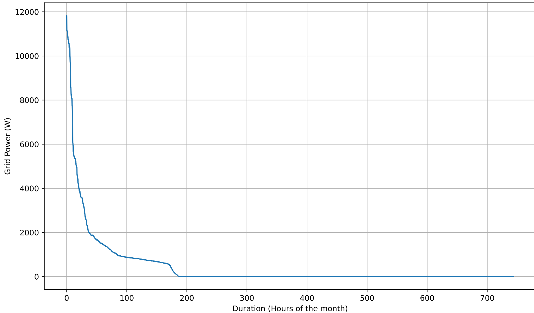
Grid Import Duration Curve - 8kWh - Jul
