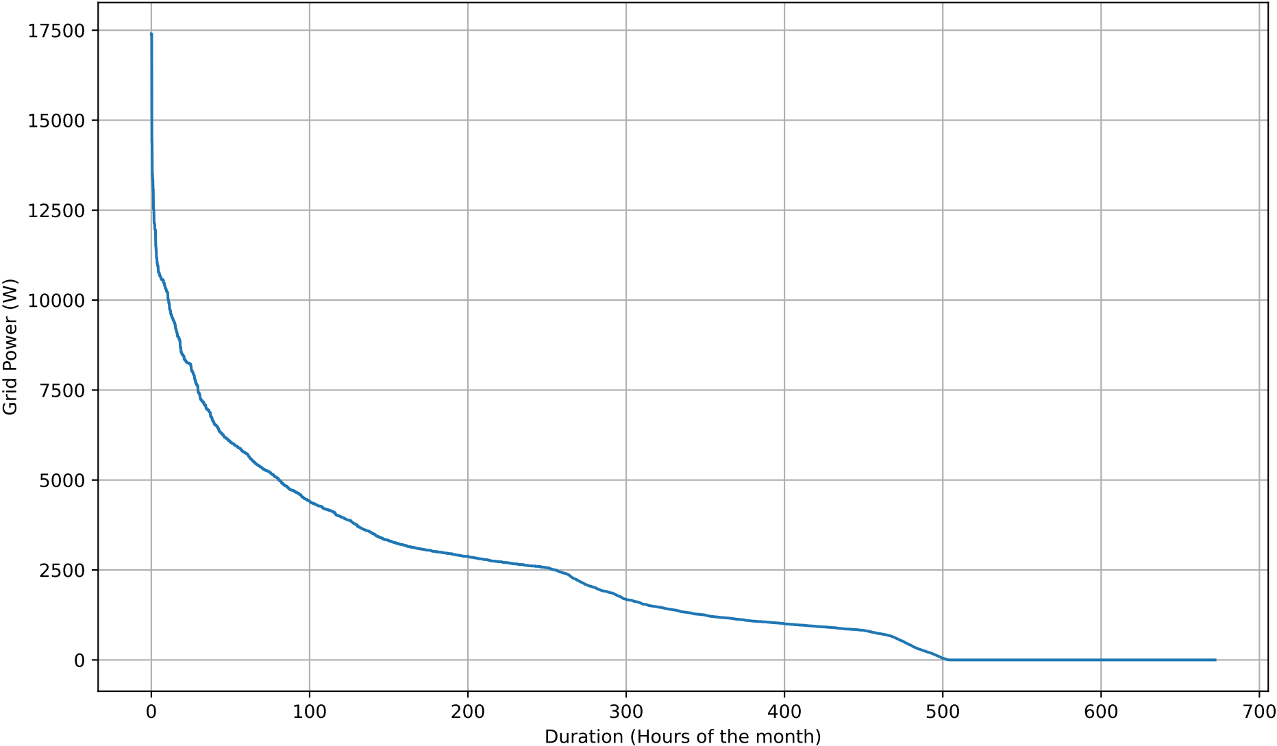
Grid Import Duration Curve - 8kWh - Feb
