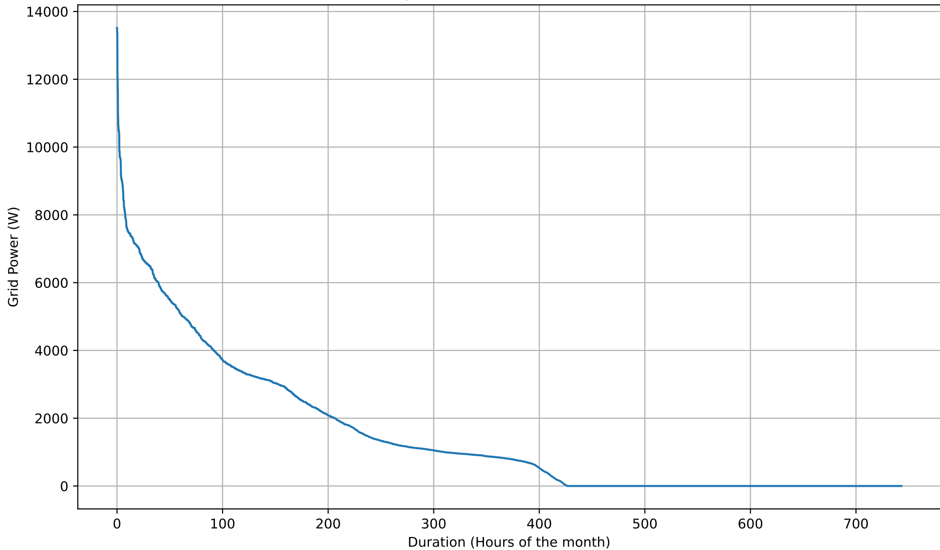
Grid Import Duration Curve - 8kWh - Mar
