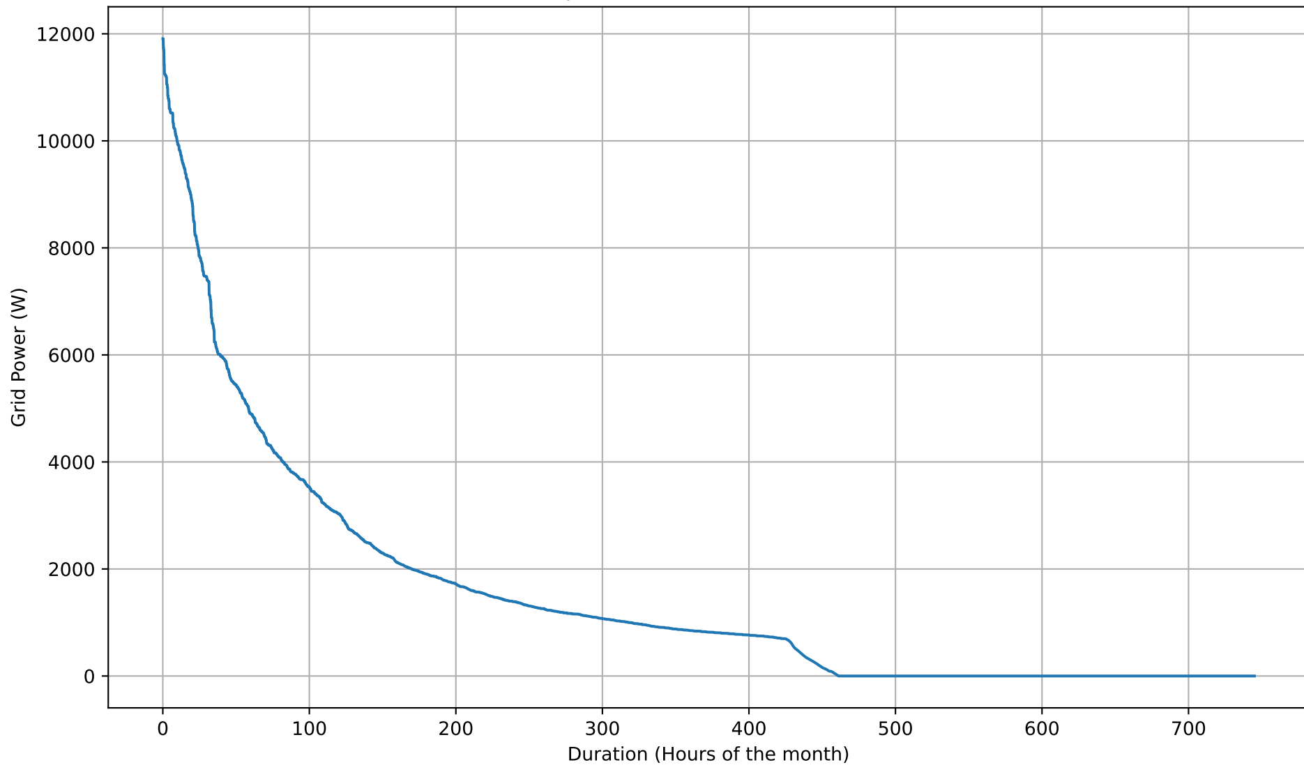
Grid Import Duration Curve - 8kWh - Oct
