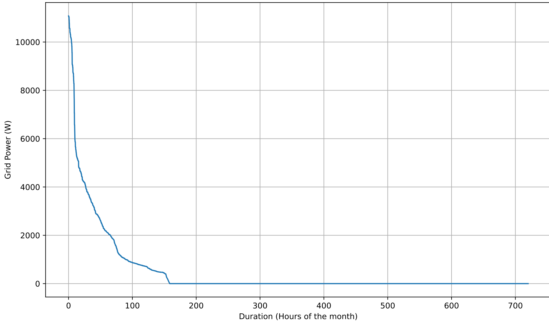
Grid Import Duration Curve - 8kWh - Jun
