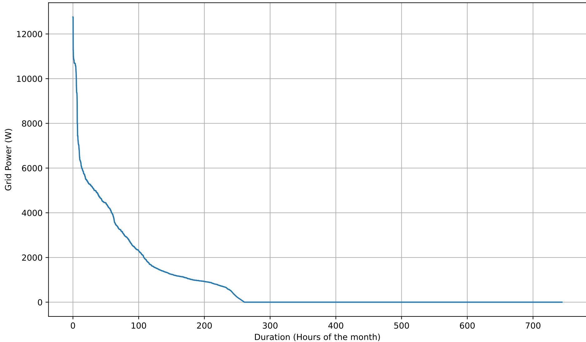
Grid Import Duration Curve - 8kWh - May
