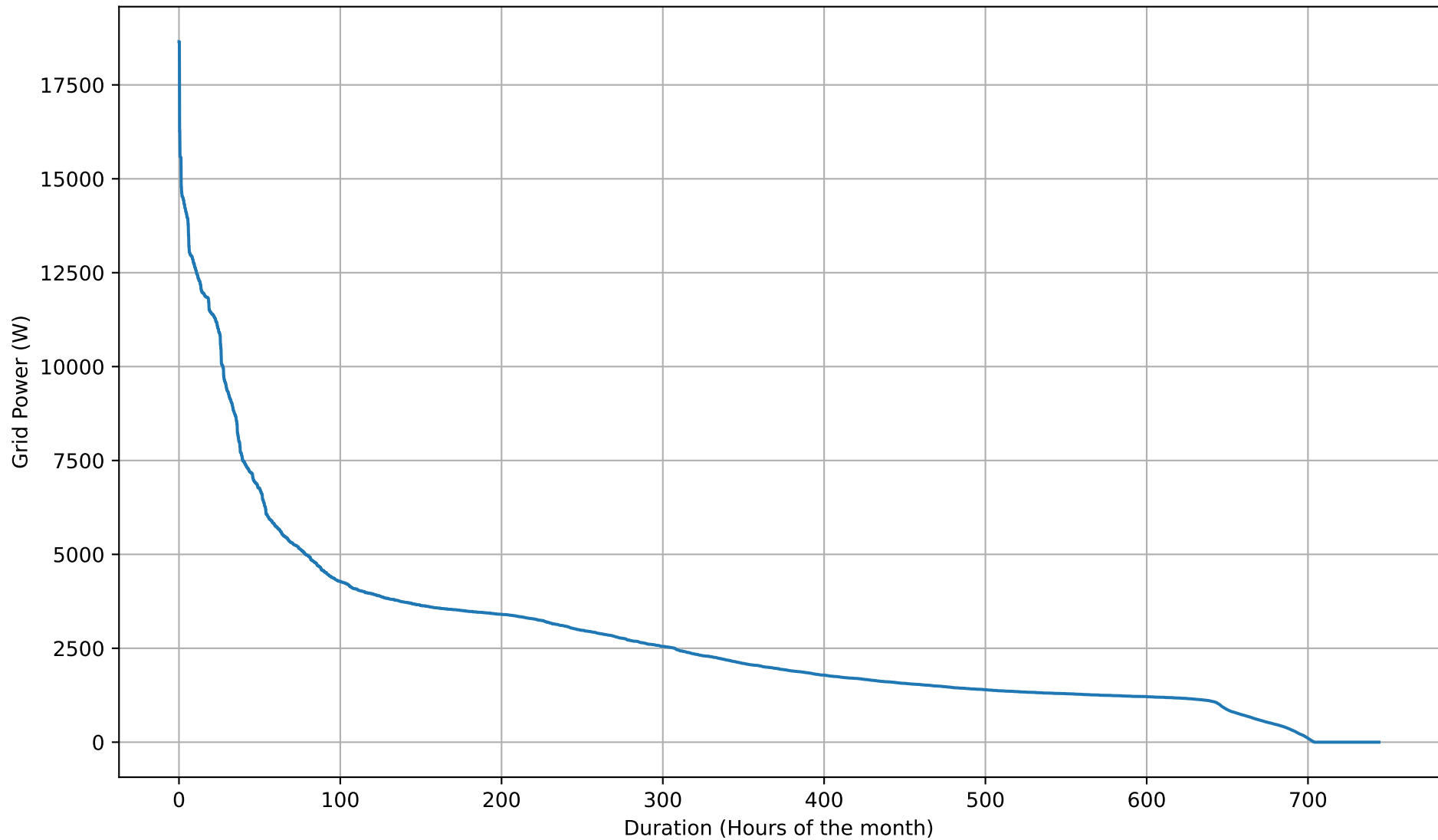
Grid Import Duration Curve - 8kWh - Dec
