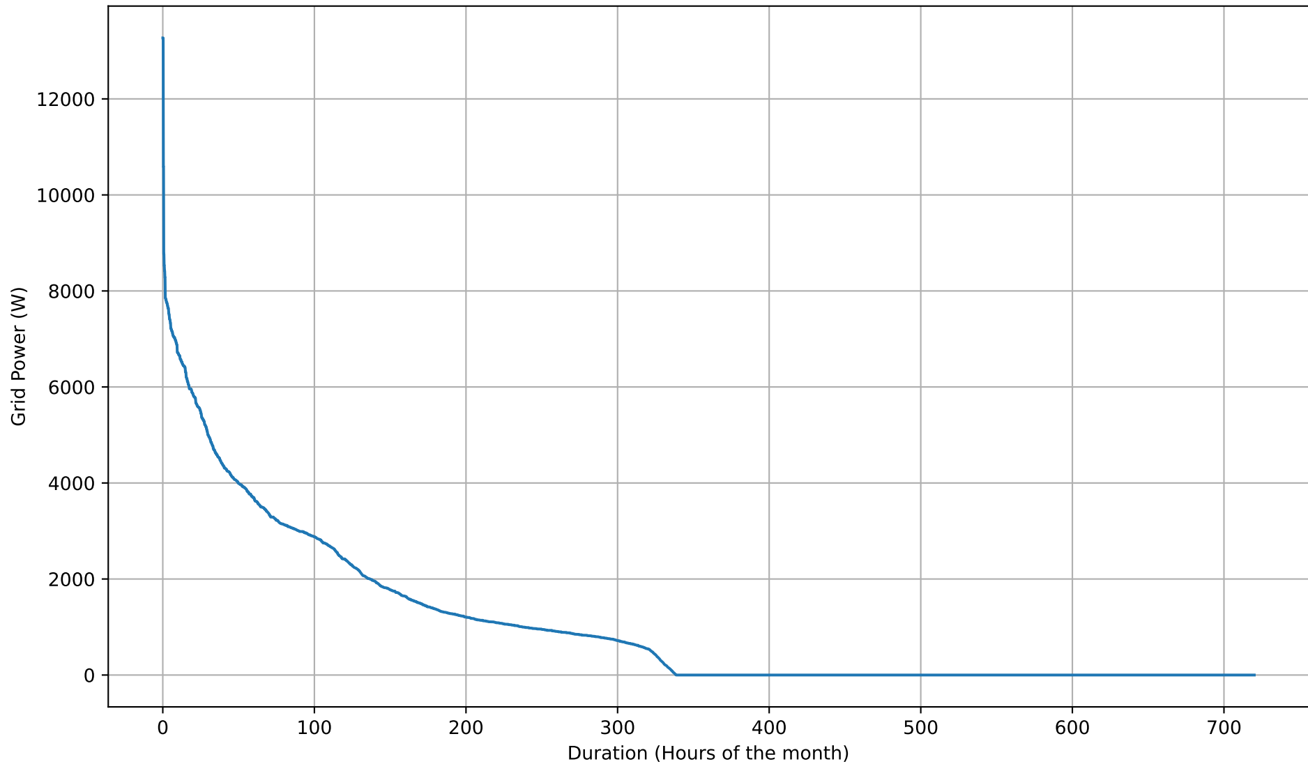
Grid Import Duration Curve - 8kWh - Apr
