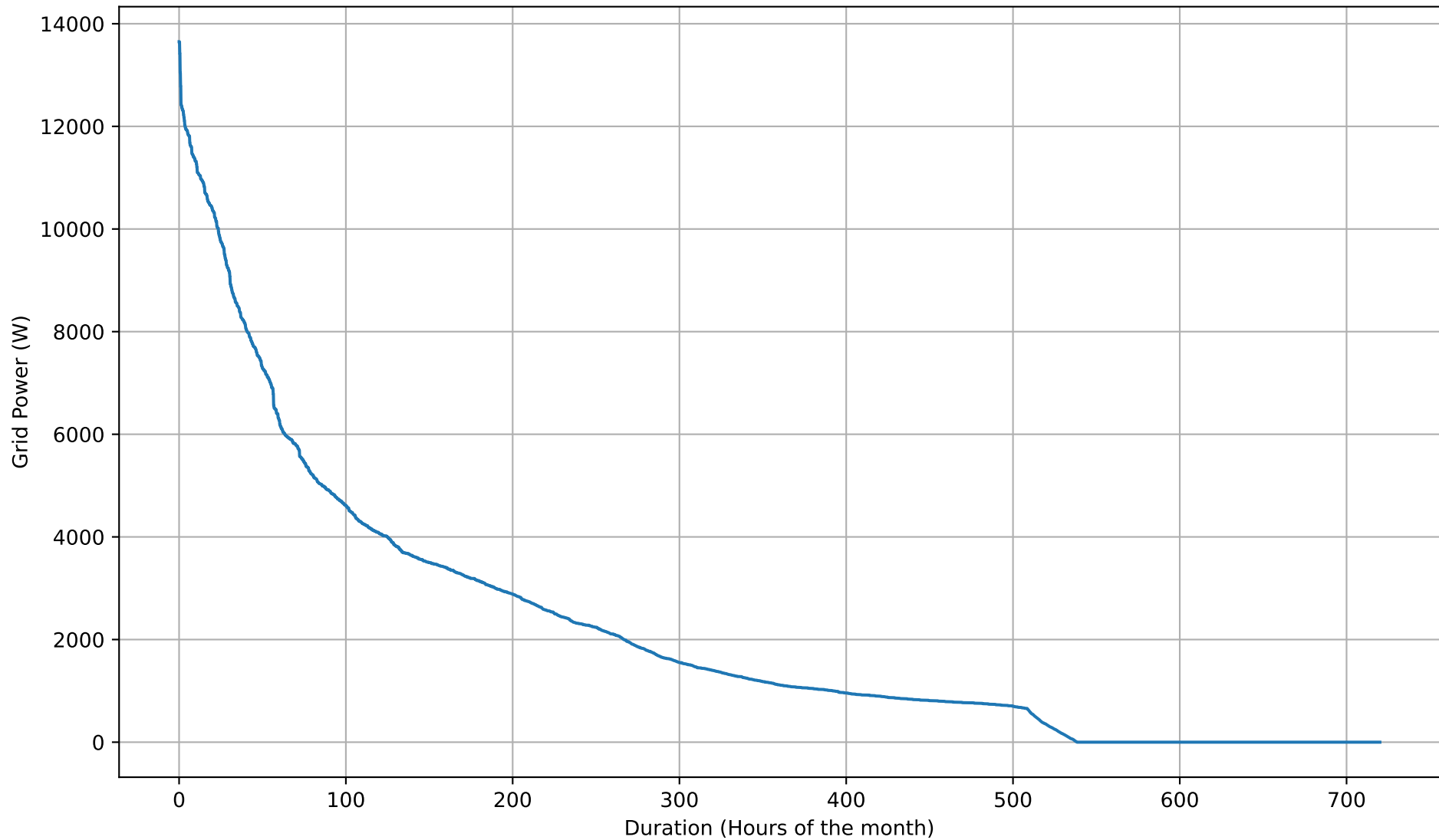
Grid Import Duration Curve - 8kWh - Nov
