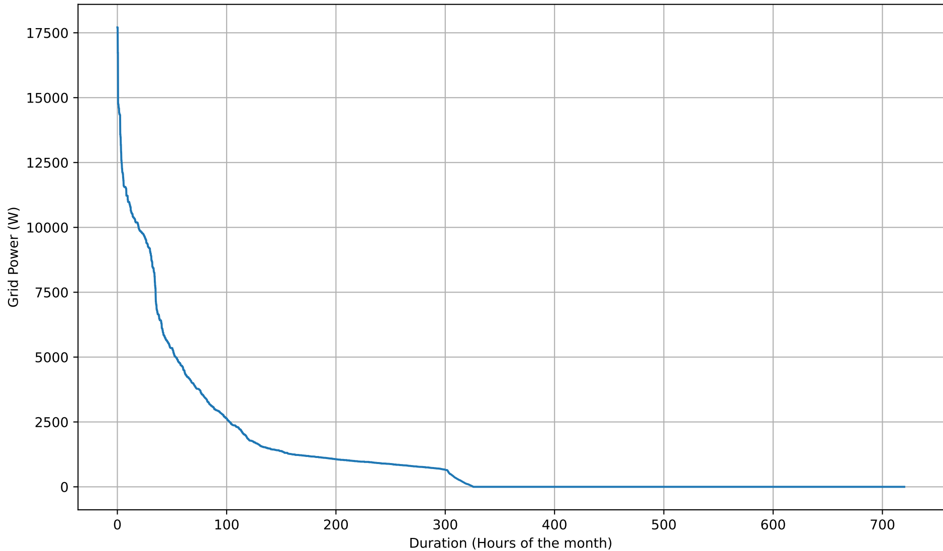
Grid Import Duration Curve - 8kWh - Sep
