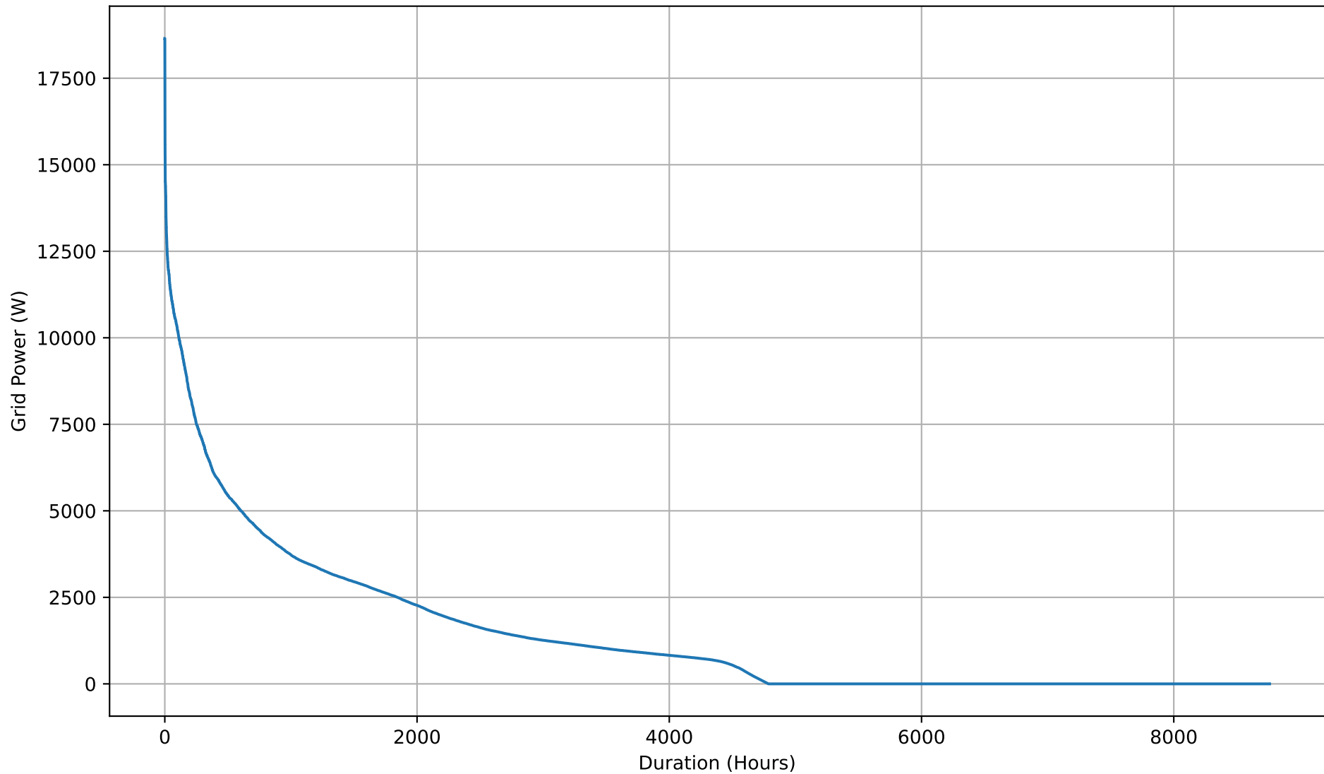
Yearly Grid Import Duration Curve - 8kWh
