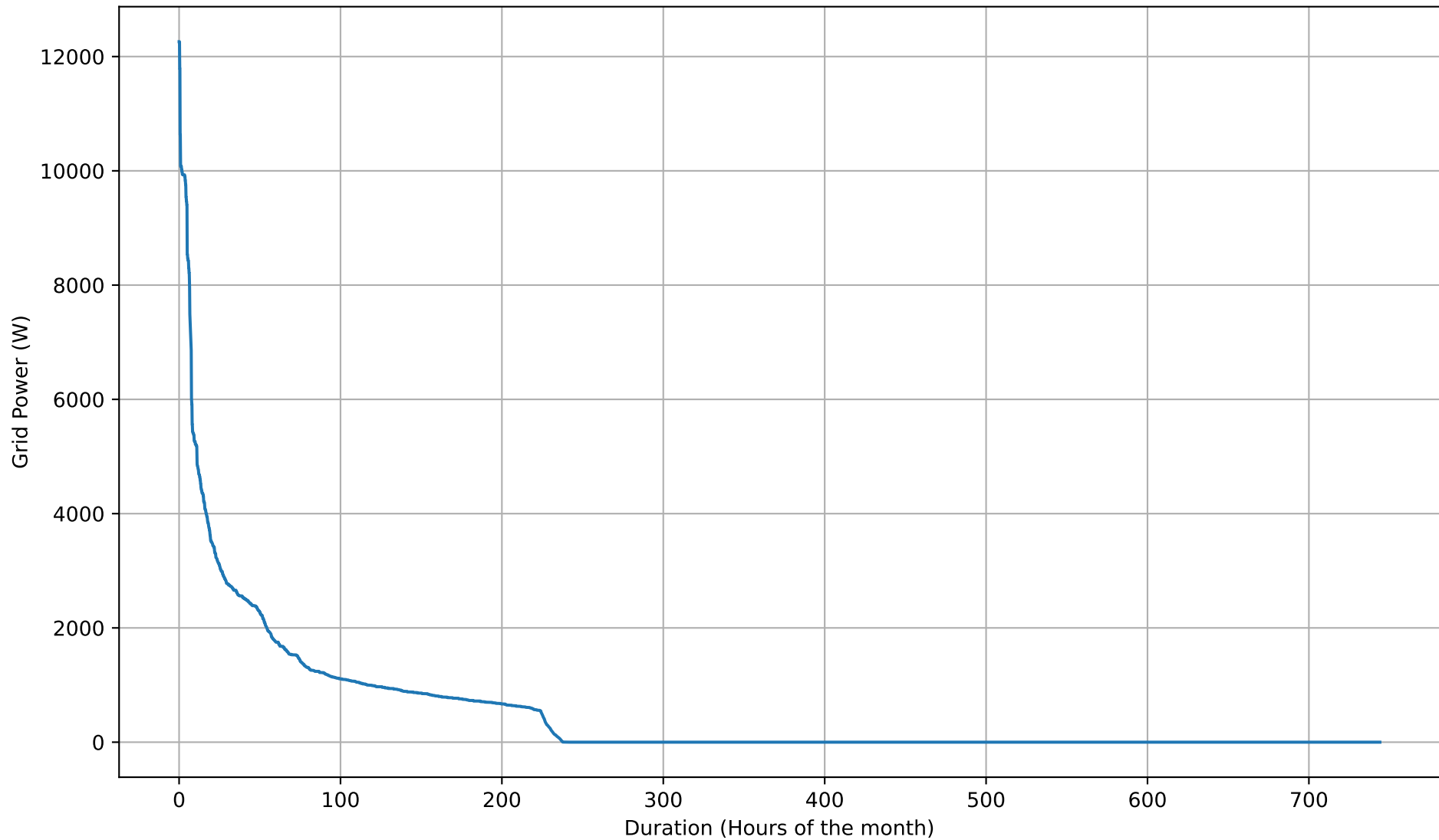
Grid Import Duration Curve - 8kWh - Aug
