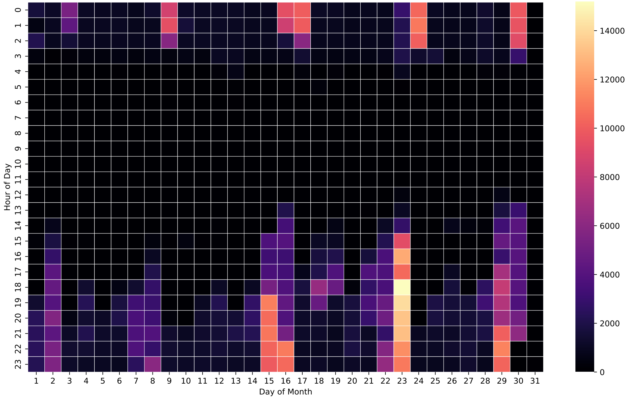
Grid Import Heatmap (Wh/Hour) - 8kWh - Sep
