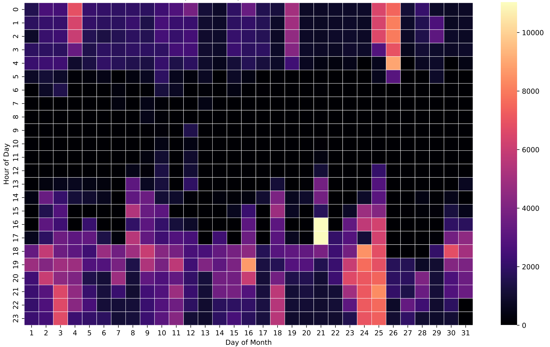
Grid Import Heatmap (Wh/Hour) - 8kWh - Mar
