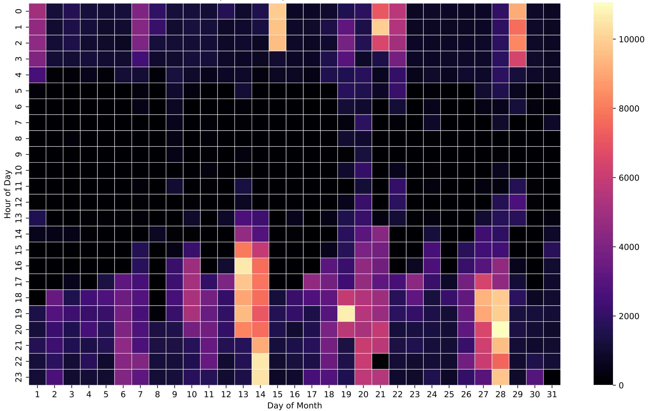
Grid Import Heatmap (Wh/Hour) - 8kWh - Oct
