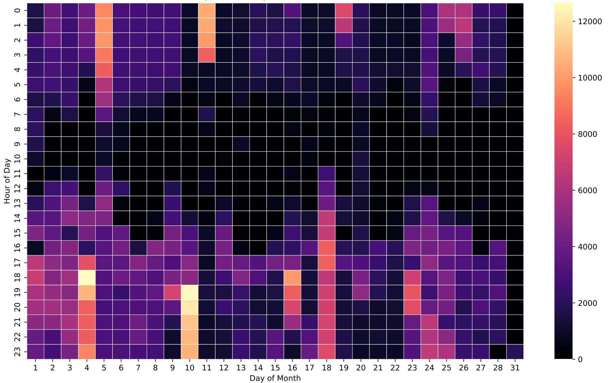
Grid Import Heatmap (Wh/Hour) - 8kWh - Feb
