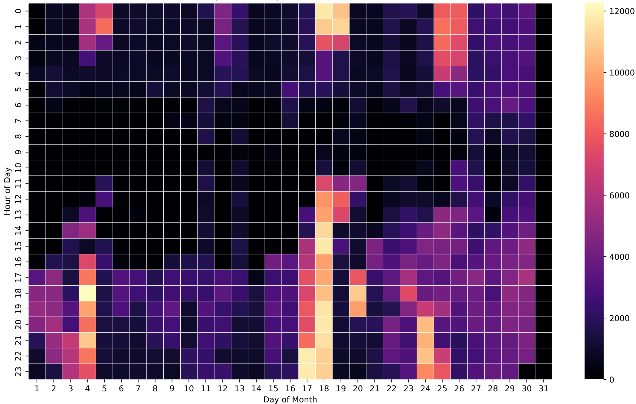
Grid Import Heatmap (Wh/Hour) - 8kWh - Nov
