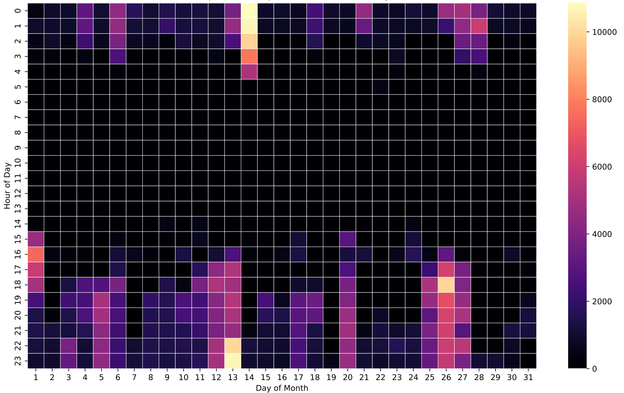
Grid Import Heatmap (Wh/Hour) - 8kWh - May
