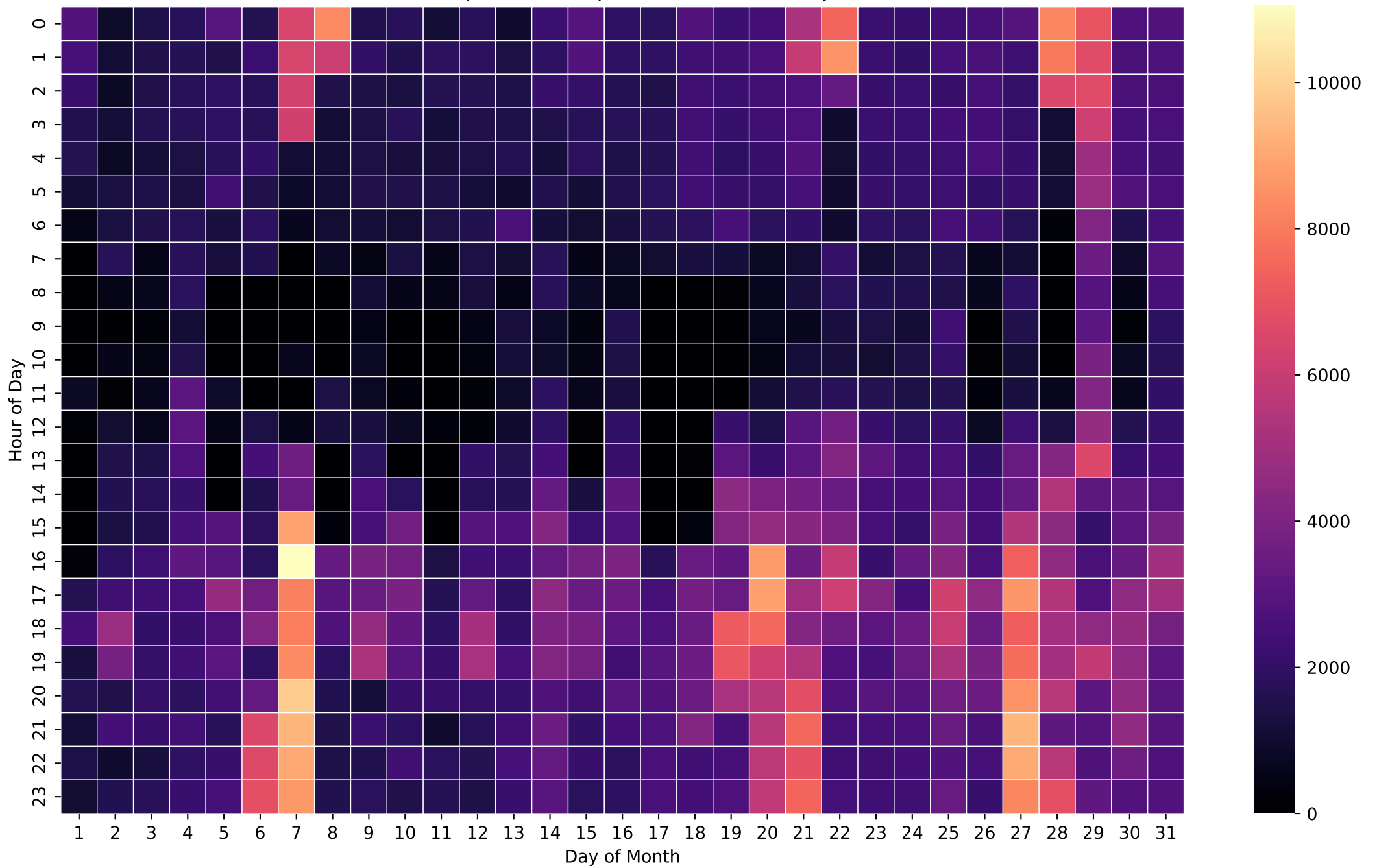
Grid Import Heatmap (Wh/Hour) - 8kWh - Jan
