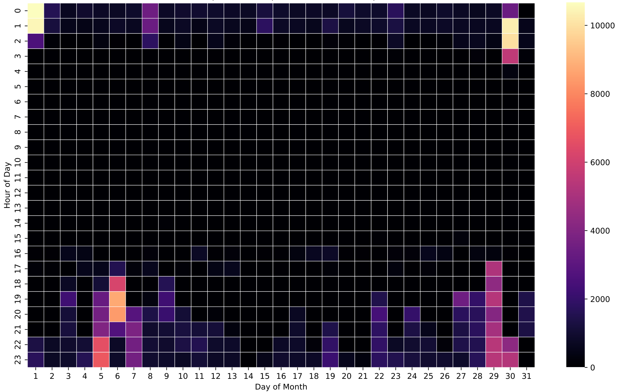
Grid Import Heatmap (Wh/Hour) - 8kWh - Jul
