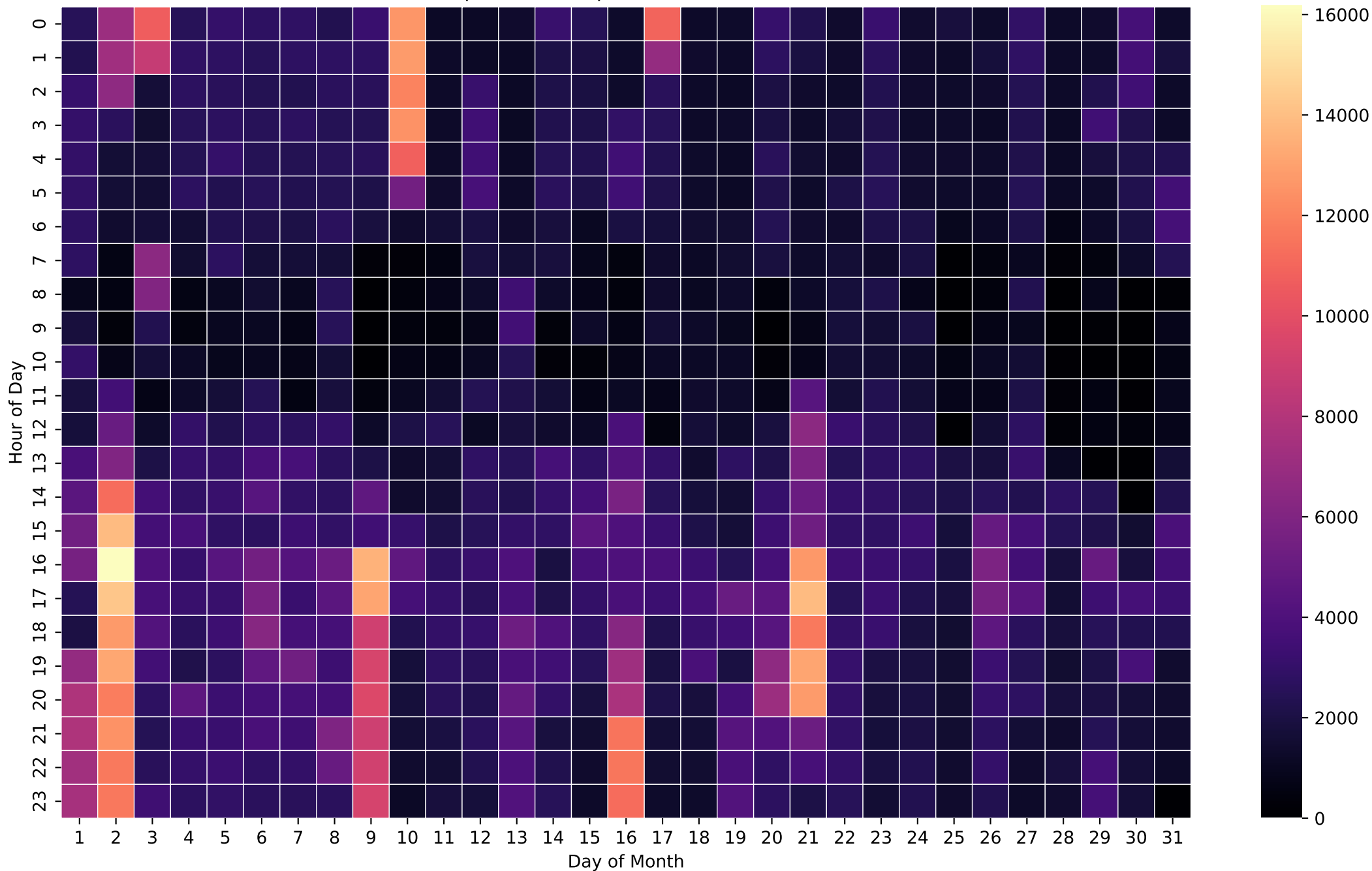
Grid Import Heatmap (Wh/Hour) - 8kWh - Dec
