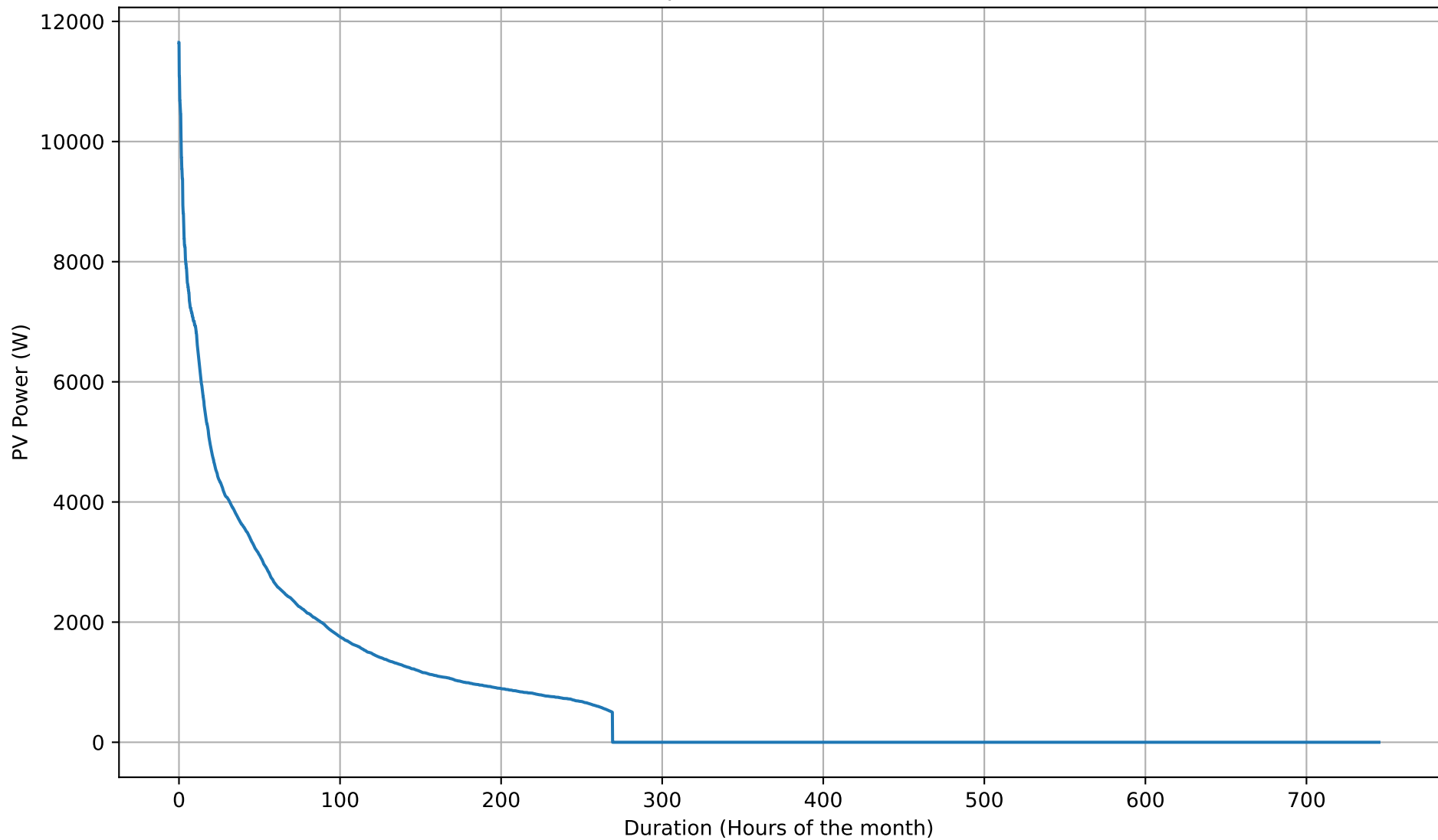
PV Self-Consumption Duration Curve - 8kWh - Oct
