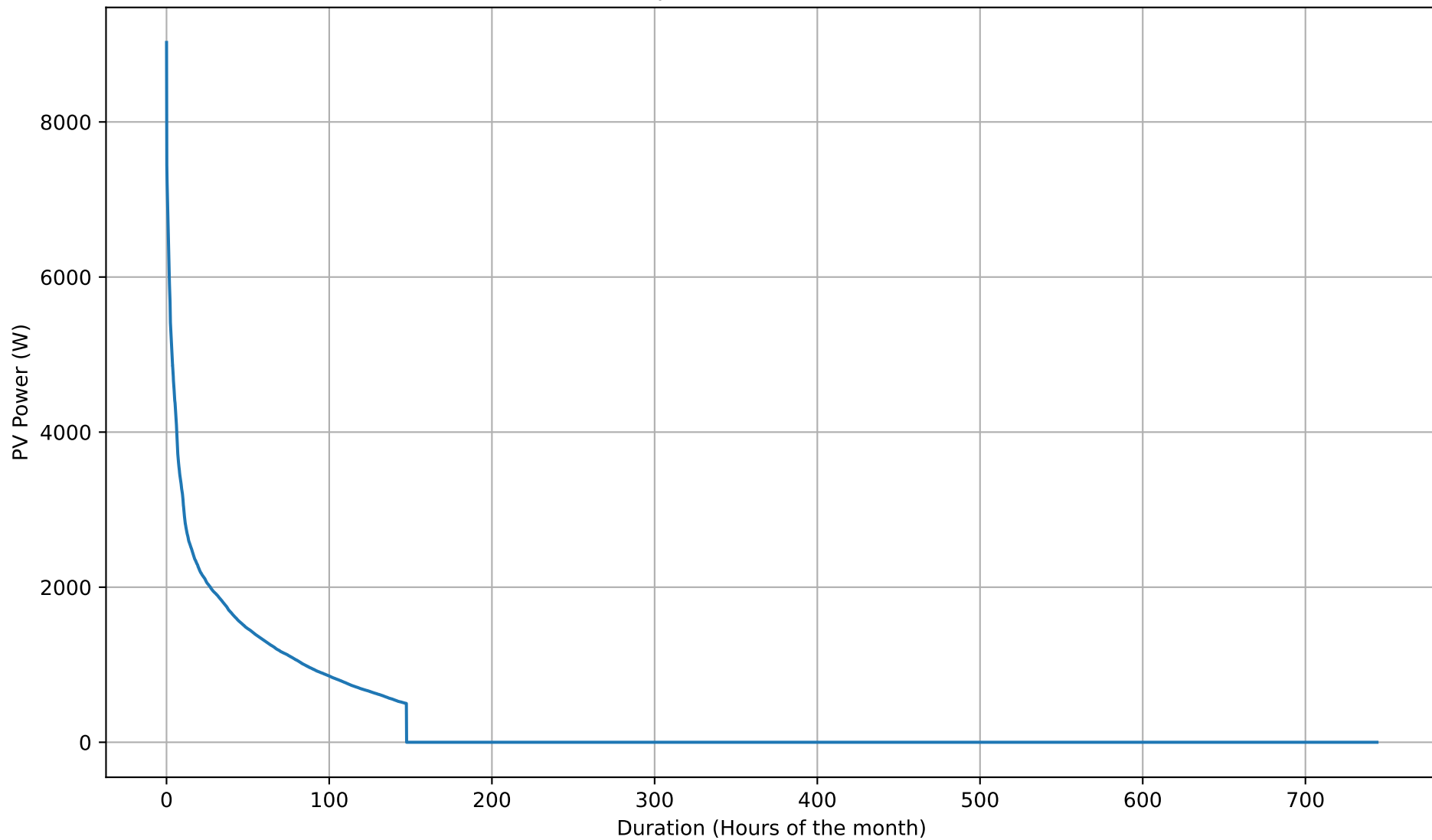
PV Self-Consumption Duration Curve - 8kWh - Dec
