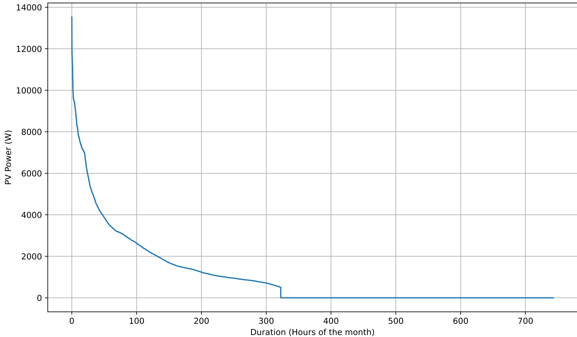
PV Self-Consumption Duration Curve - 8kWh - Mar
