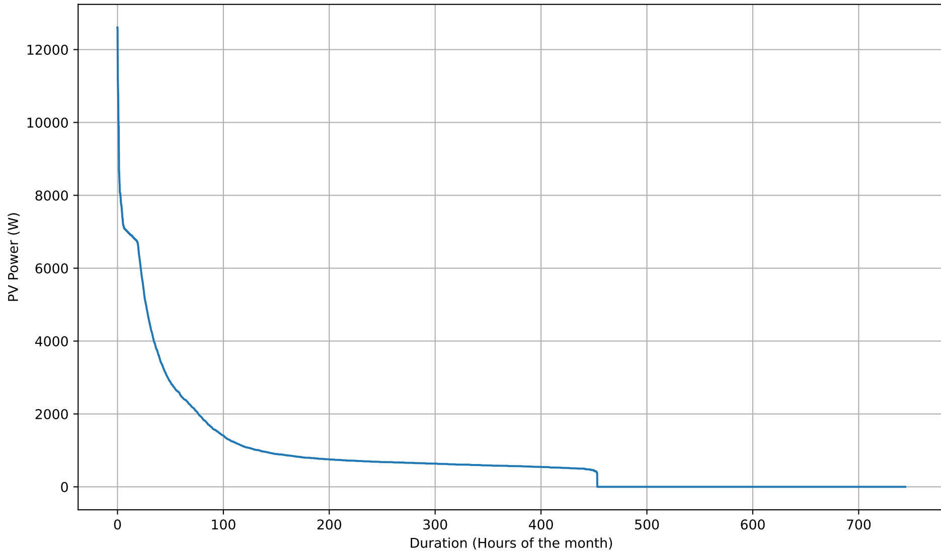
PV Self-Consumption Duration Curve - 8kWh - Jul
