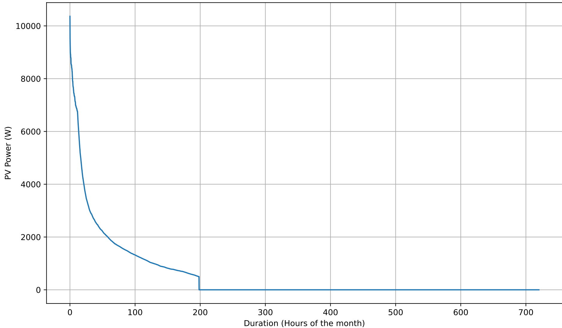
PV Self-Consumption Duration Curve - 8kWh - Nov
