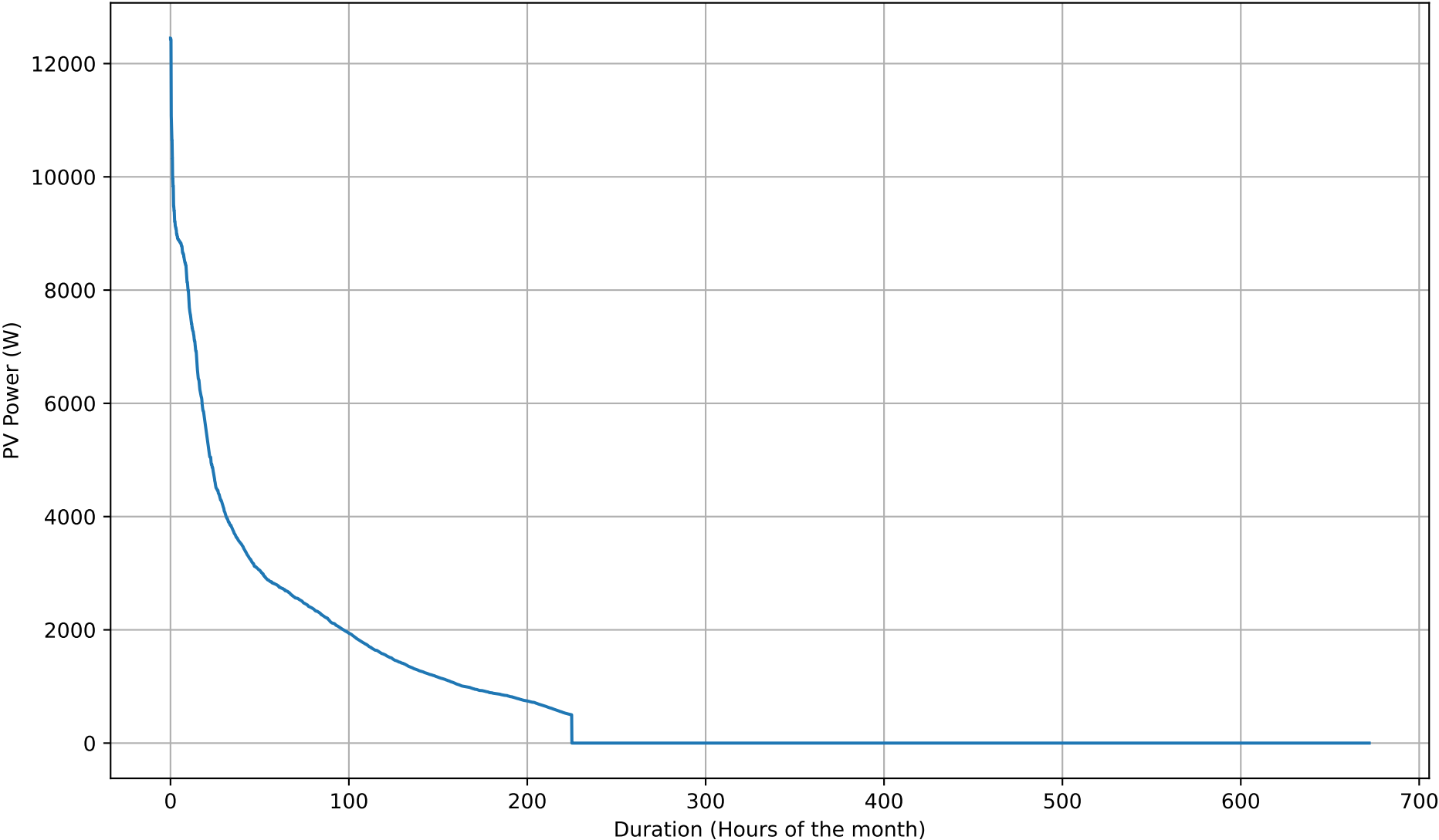
PV Self-Consumption Duration Curve - 8kWh - Feb
