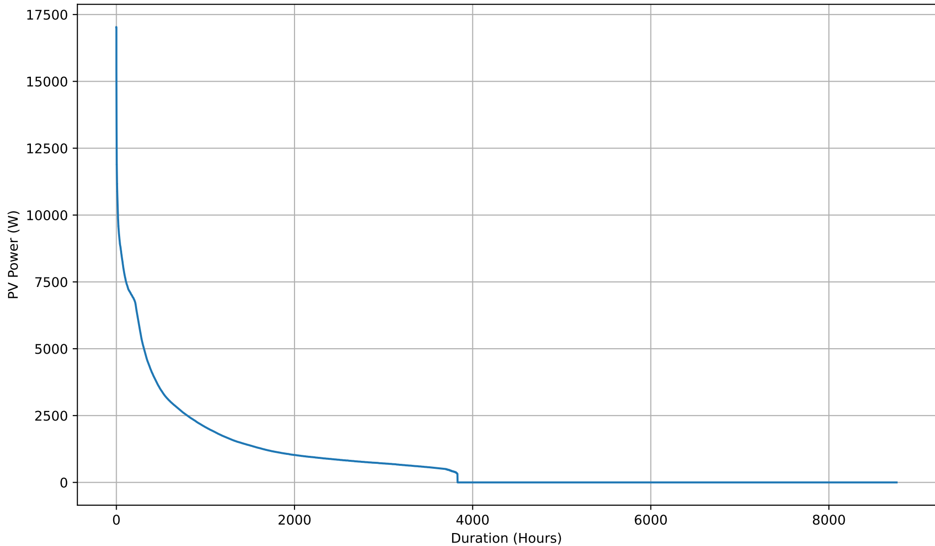
Yearly PV Self-Consumption Duration Curve - 8kWh
