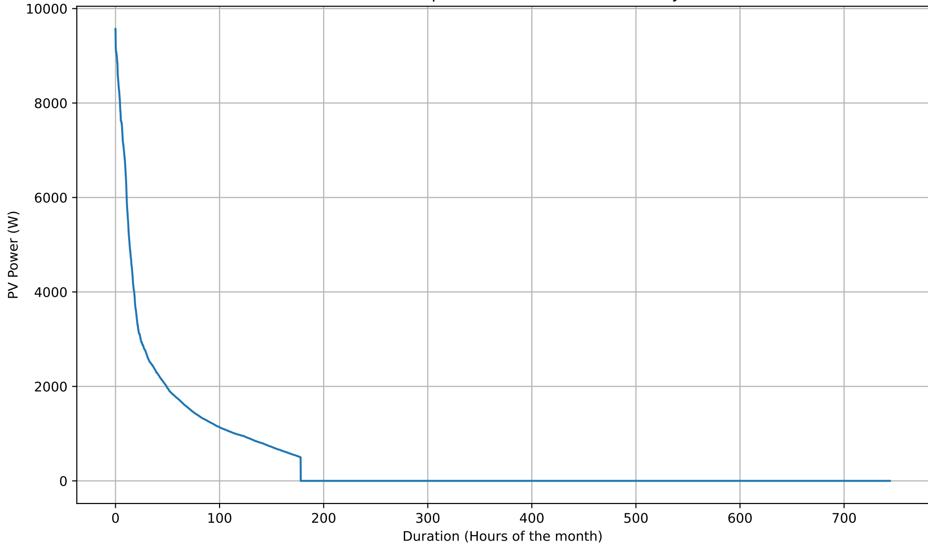
PV Self-Consumption Duration Curve - 8kWh - Jan
