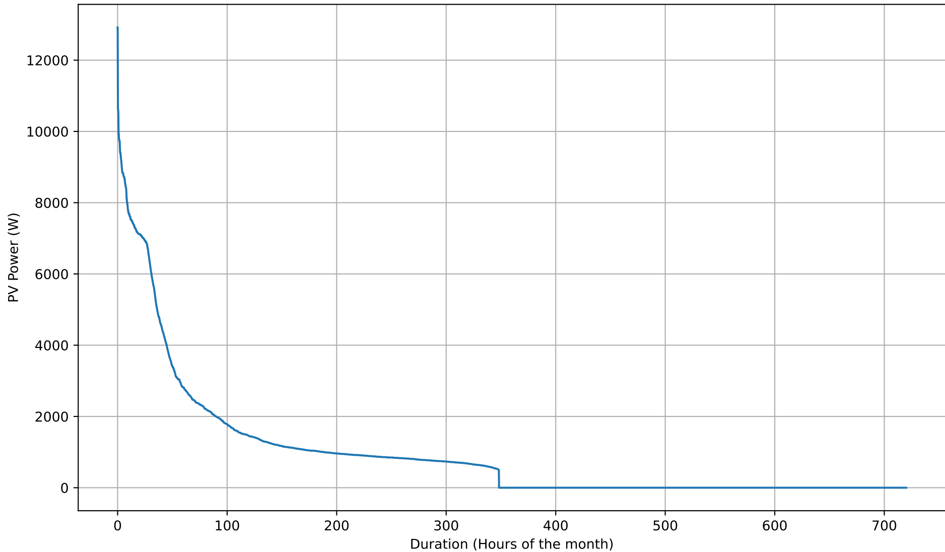
PV Self-Consumption Duration Curve - 8kWh - Sep
