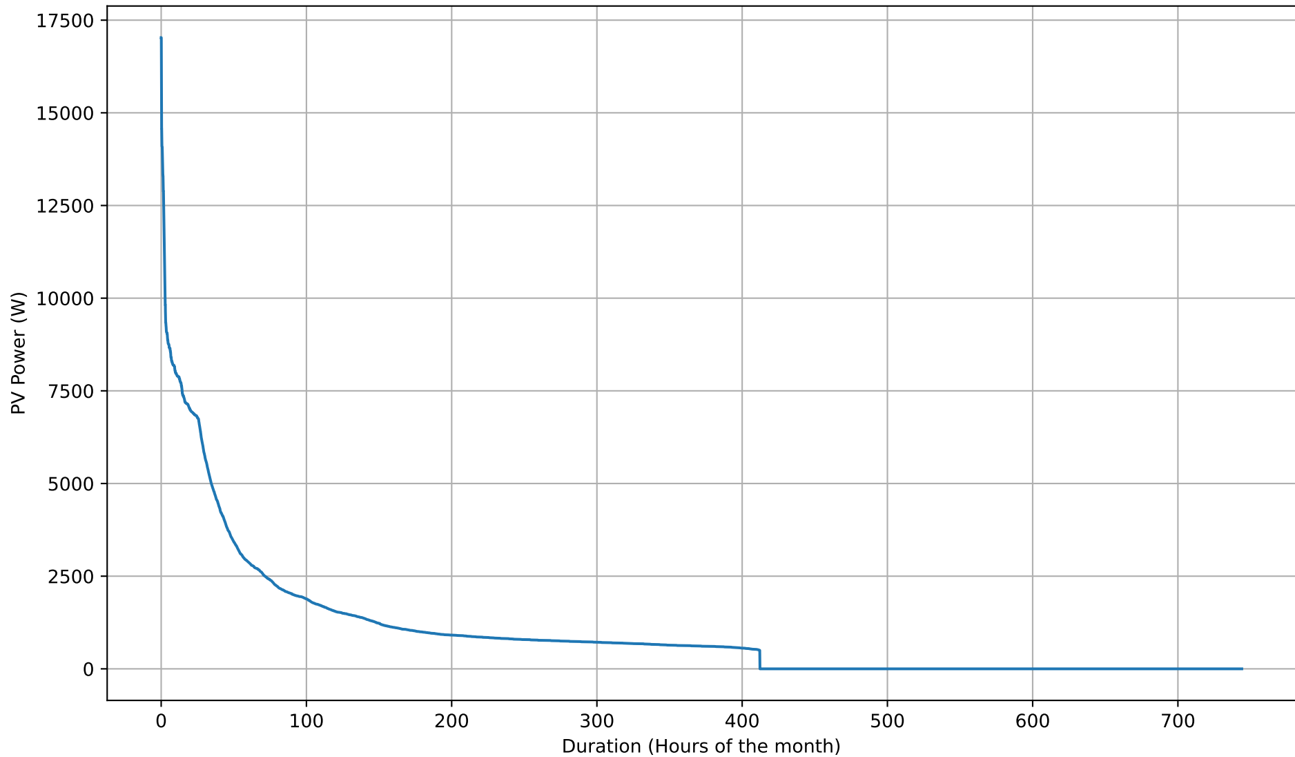
PV Self-Consumption Duration Curve - 8kWh - Aug
