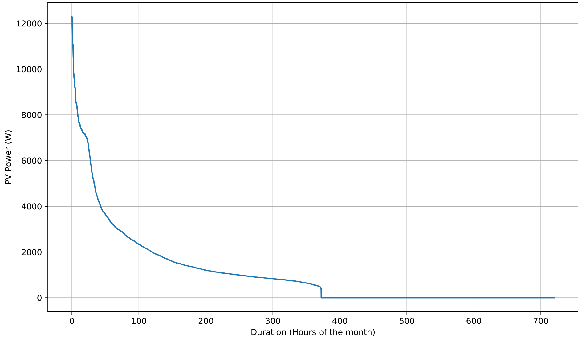
PV Self-Consumption Duration Curve - 8kWh - Apr
