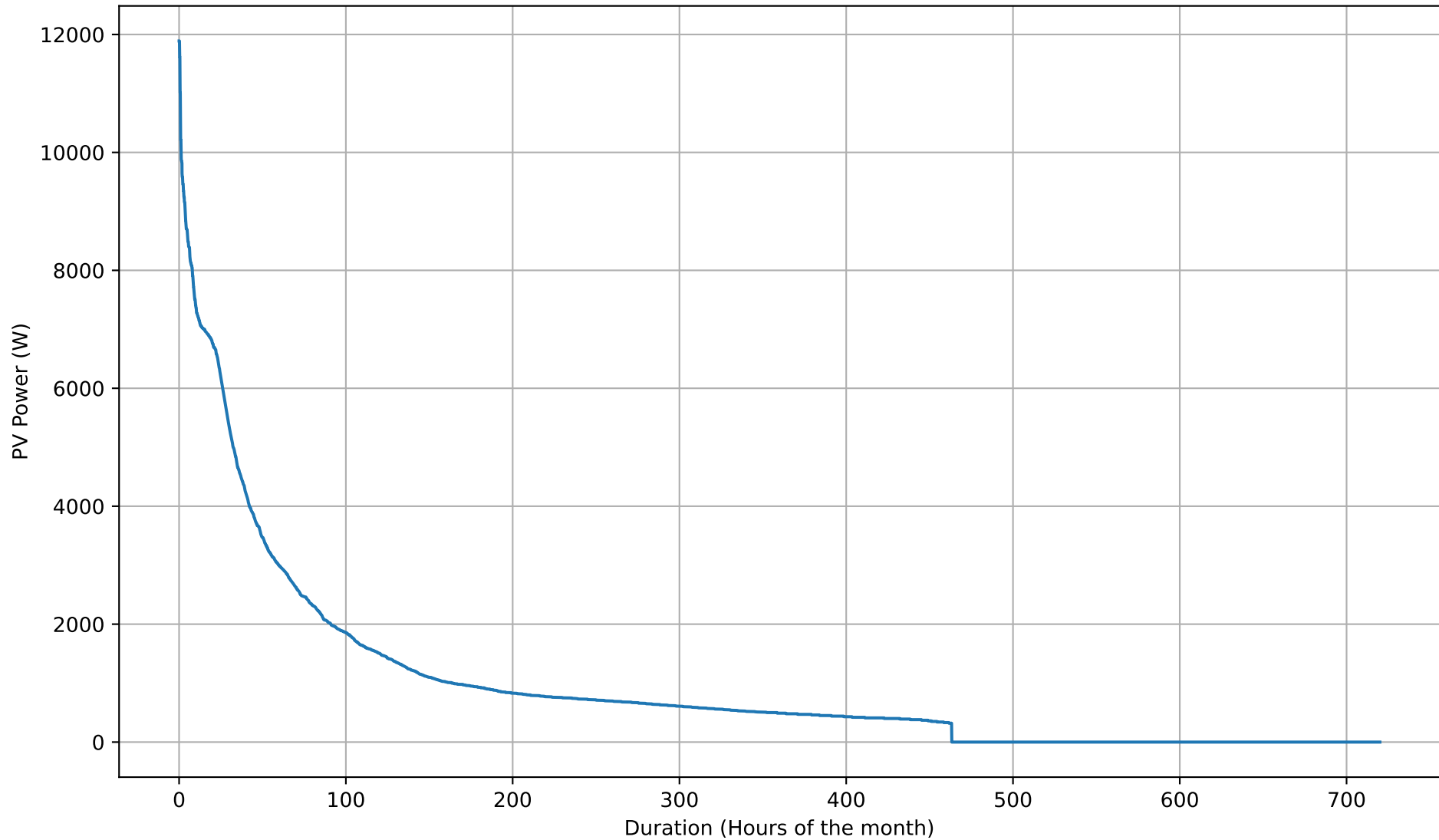
PV Self-Consumption Duration Curve - 8kWh - Jun
