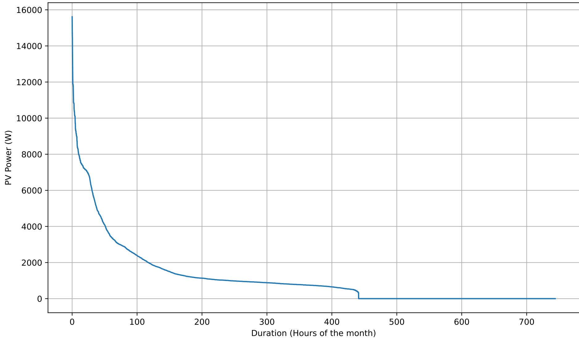
PV Self-Consumption Duration Curve - 8kWh - May
