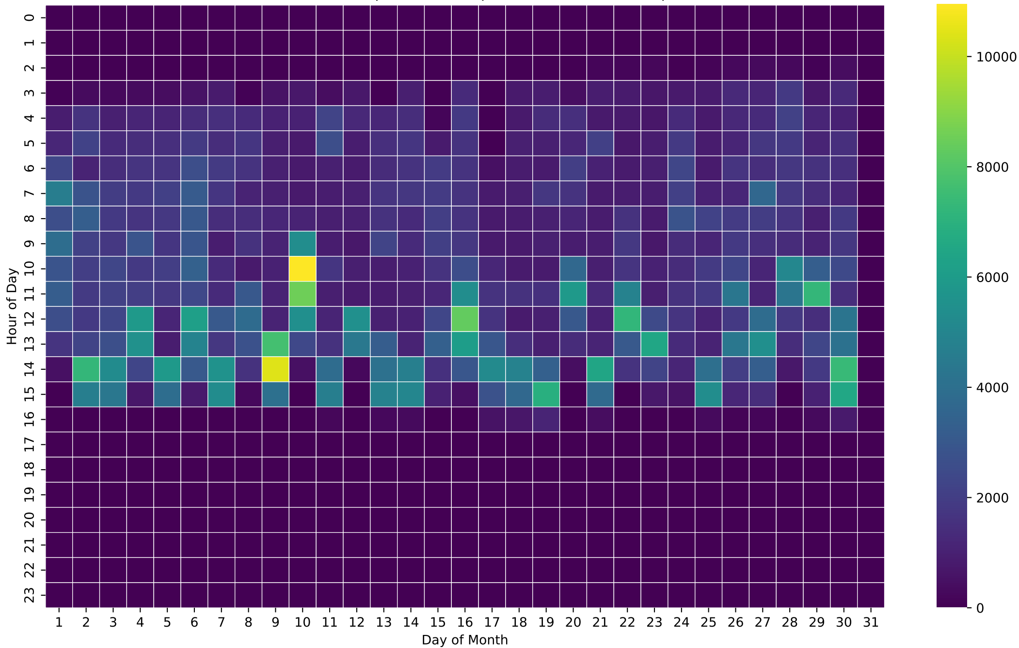
PV Self-Consumption Heatmap (Wh/Hour) - 8kWh - Apr
