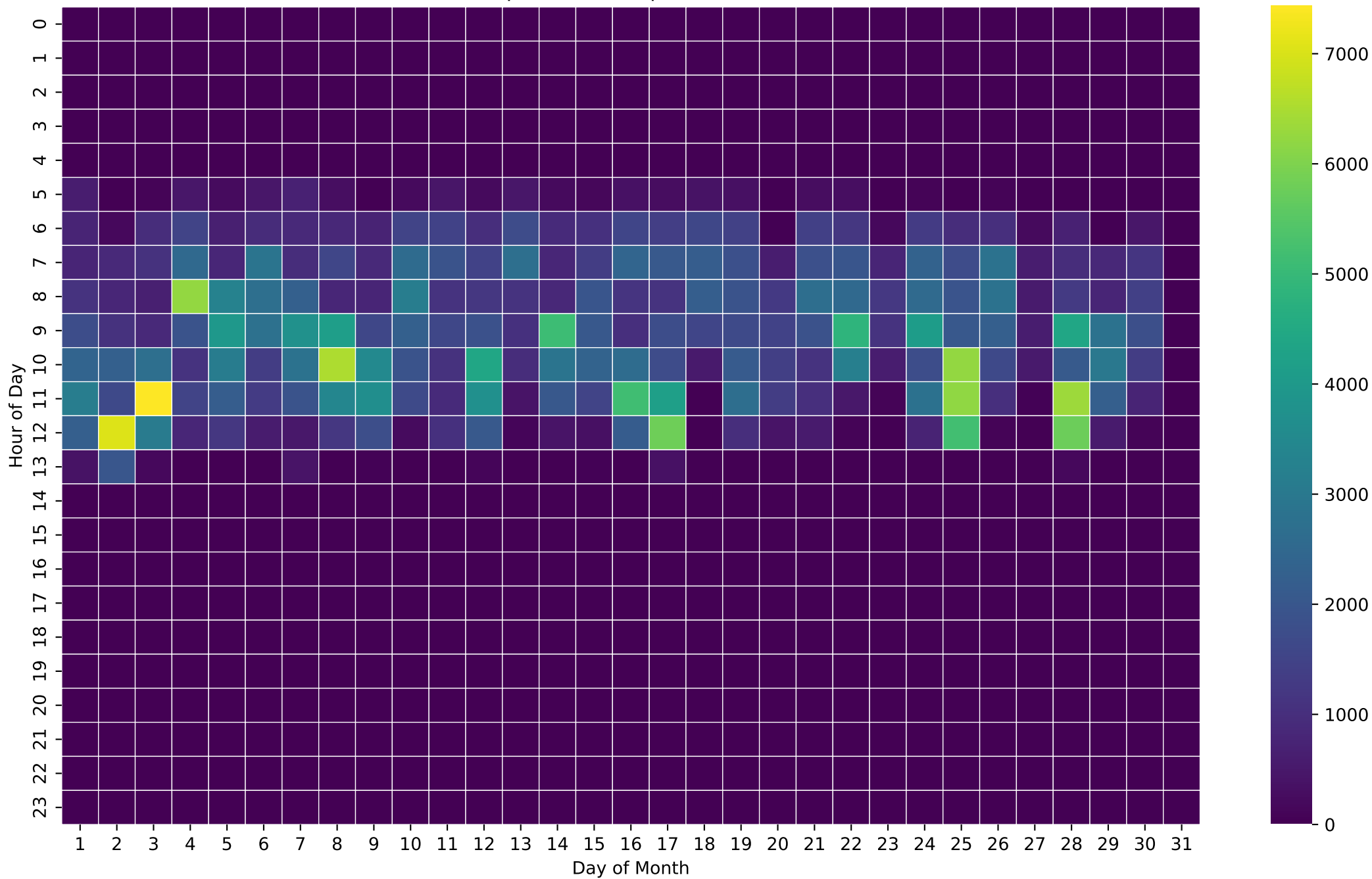
PV Self-Consumption Heatmap (Wh/Hour) - 8kWh - Nov
