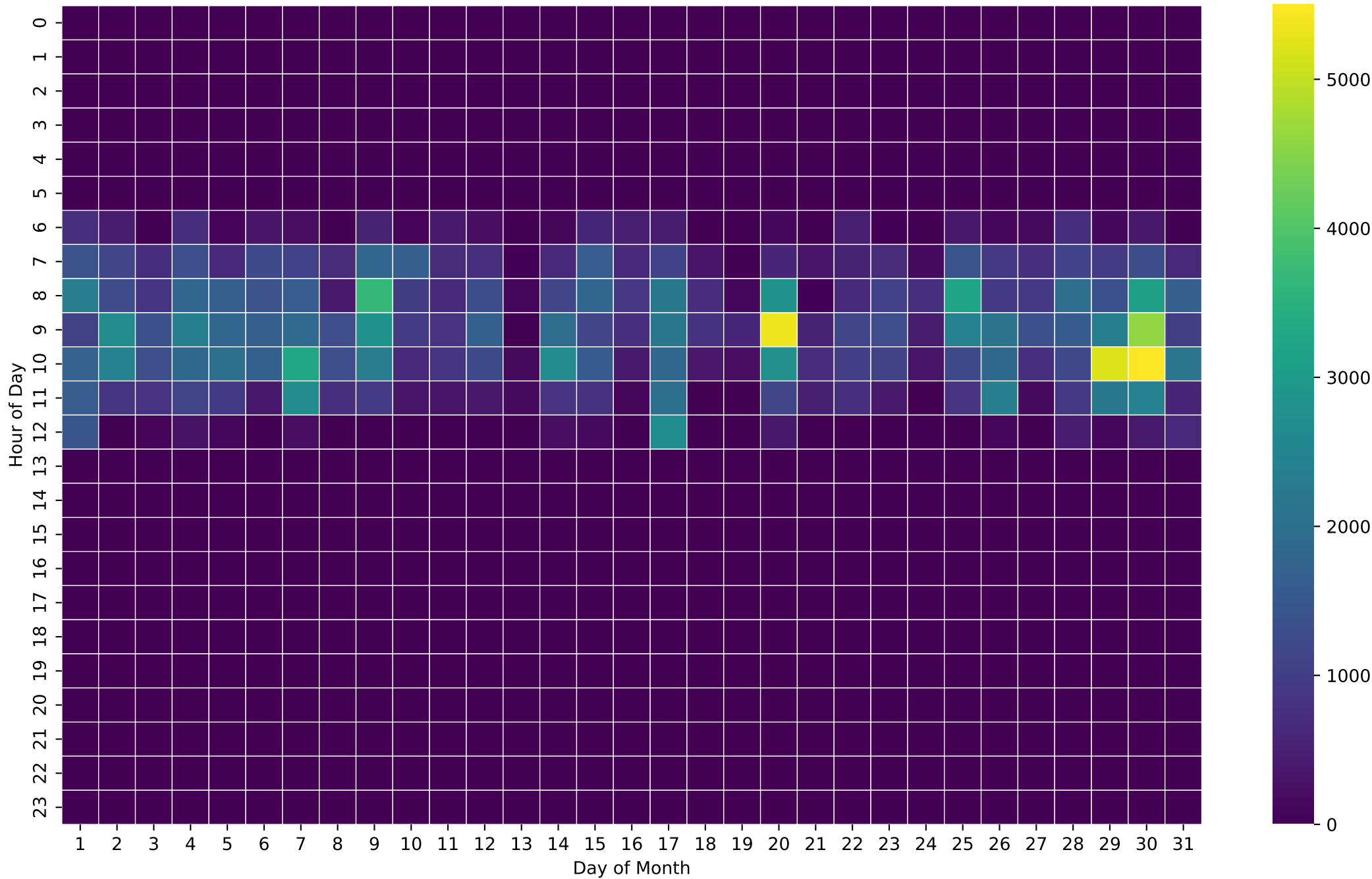
PV Self-Consumption Heatmap (Wh/Hour) - 8kWh - Dec
