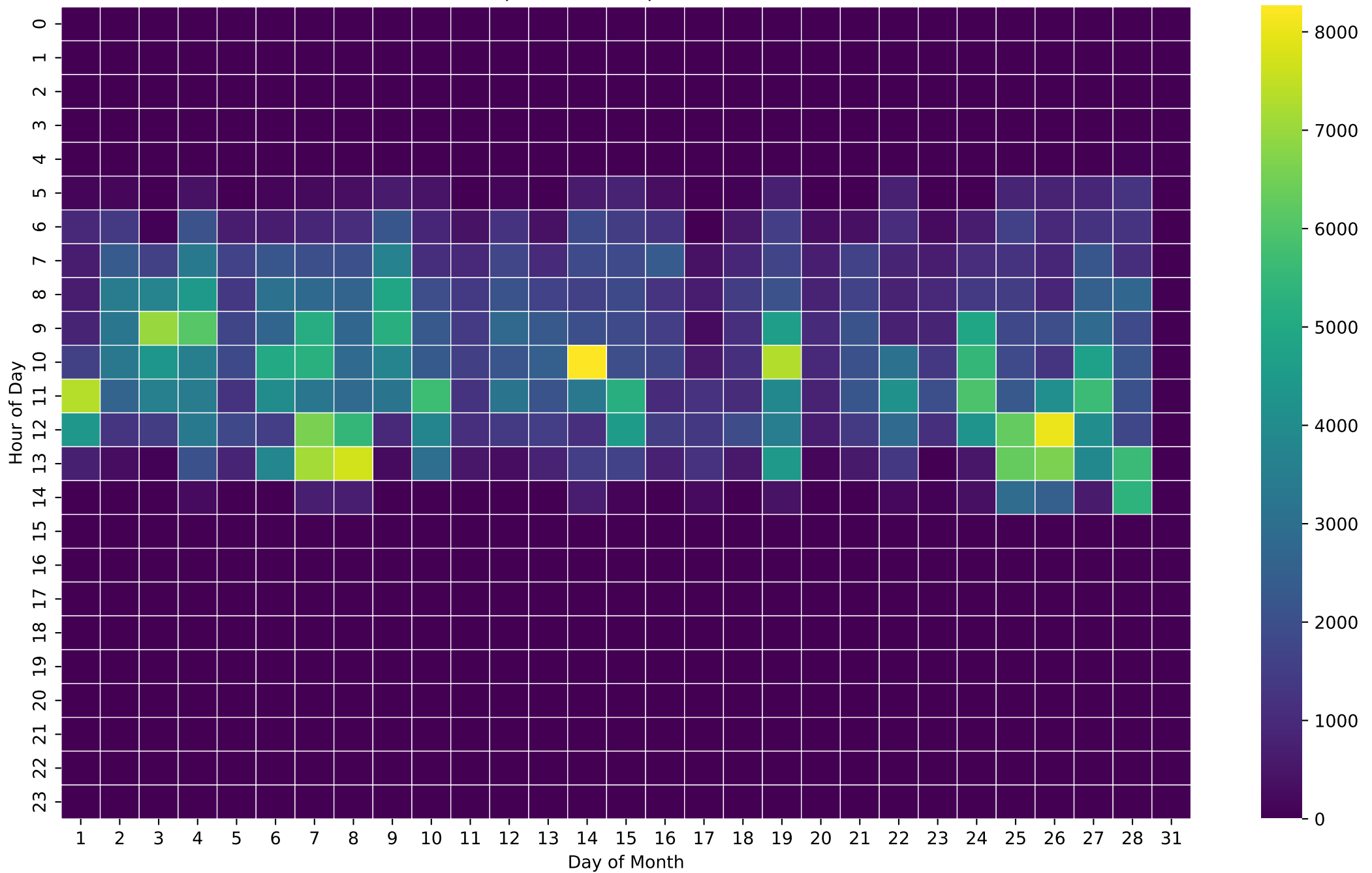
PV Self-Consumption Heatmap (Wh/Hour) - 8kWh - Feb
