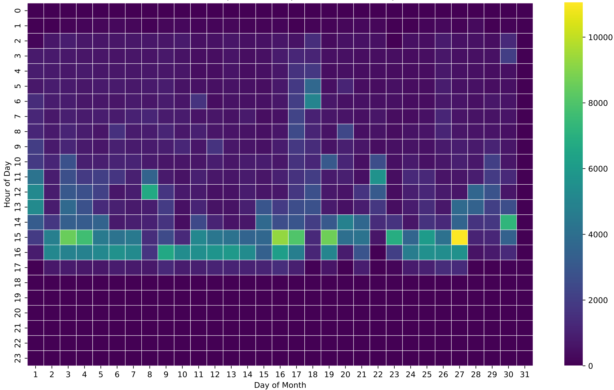
PV Self-Consumption Heatmap (Wh/Hour) - 8kWh - Jun
