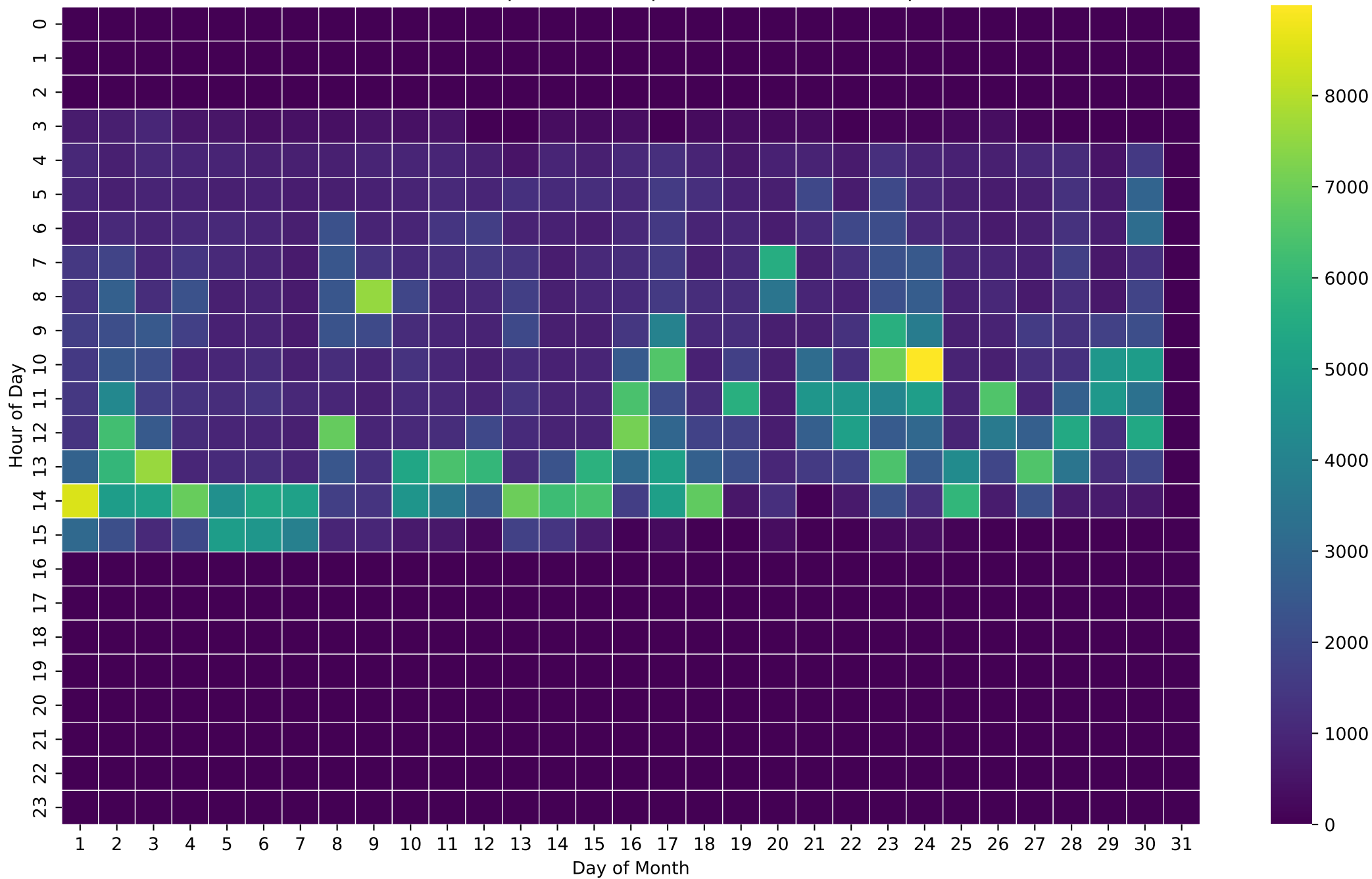
PV Self-Consumption Heatmap (Wh/Hour) - 8kWh - Sep
