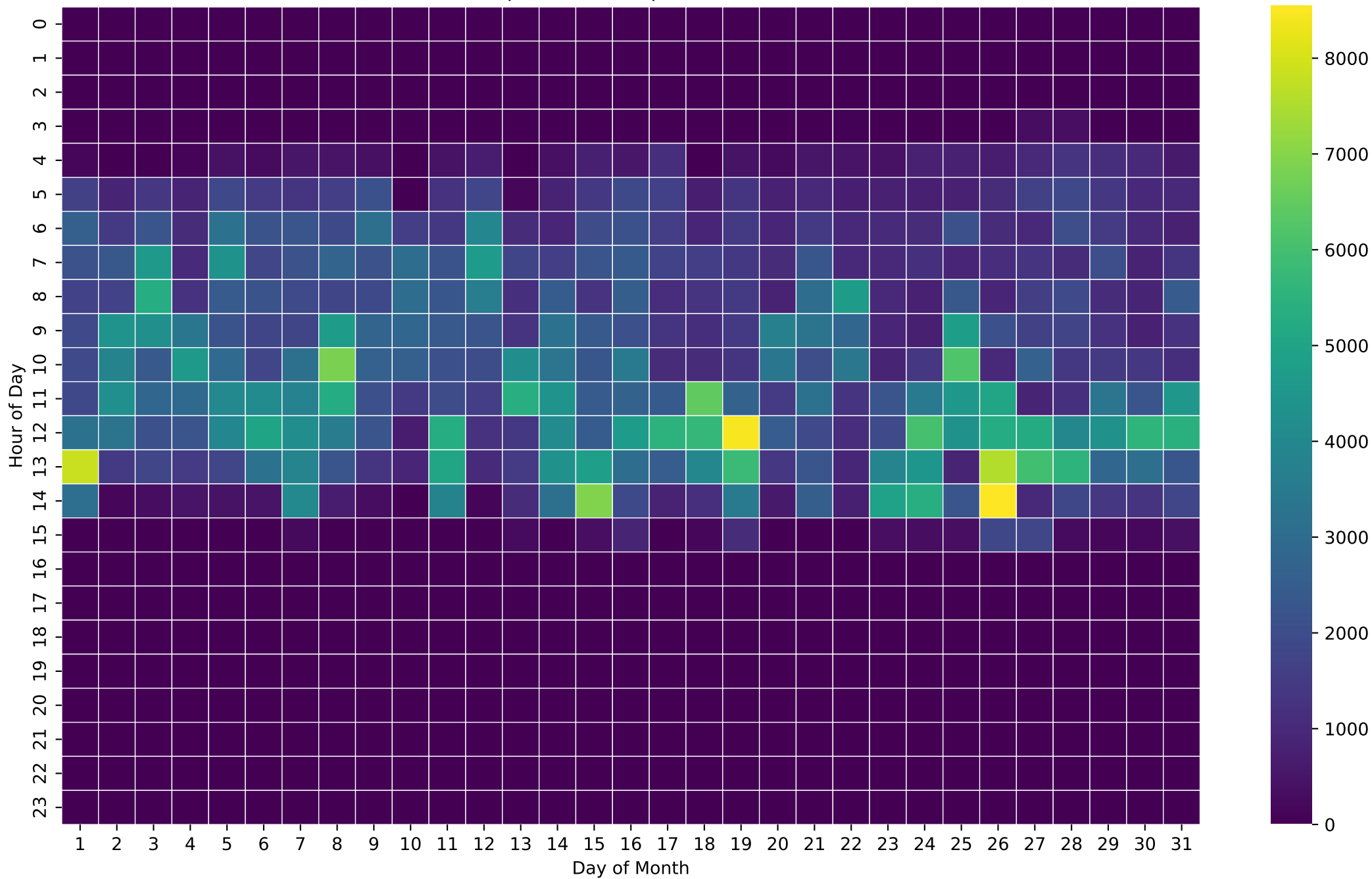
PV Self-Consumption Heatmap (Wh/Hour) - 8kWh - Mar
