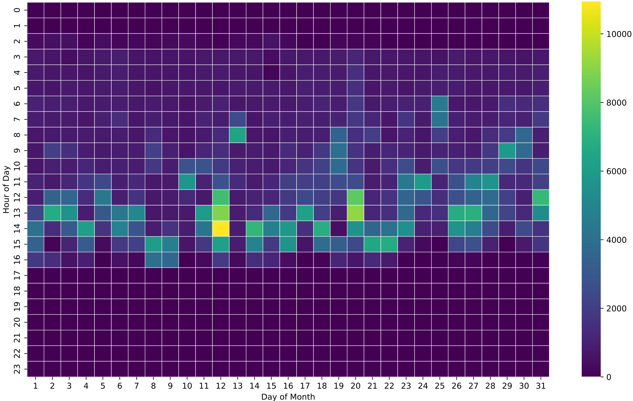
PV Self-Consumption Heatmap (Wh/Hour) - 8kWh - Aug
