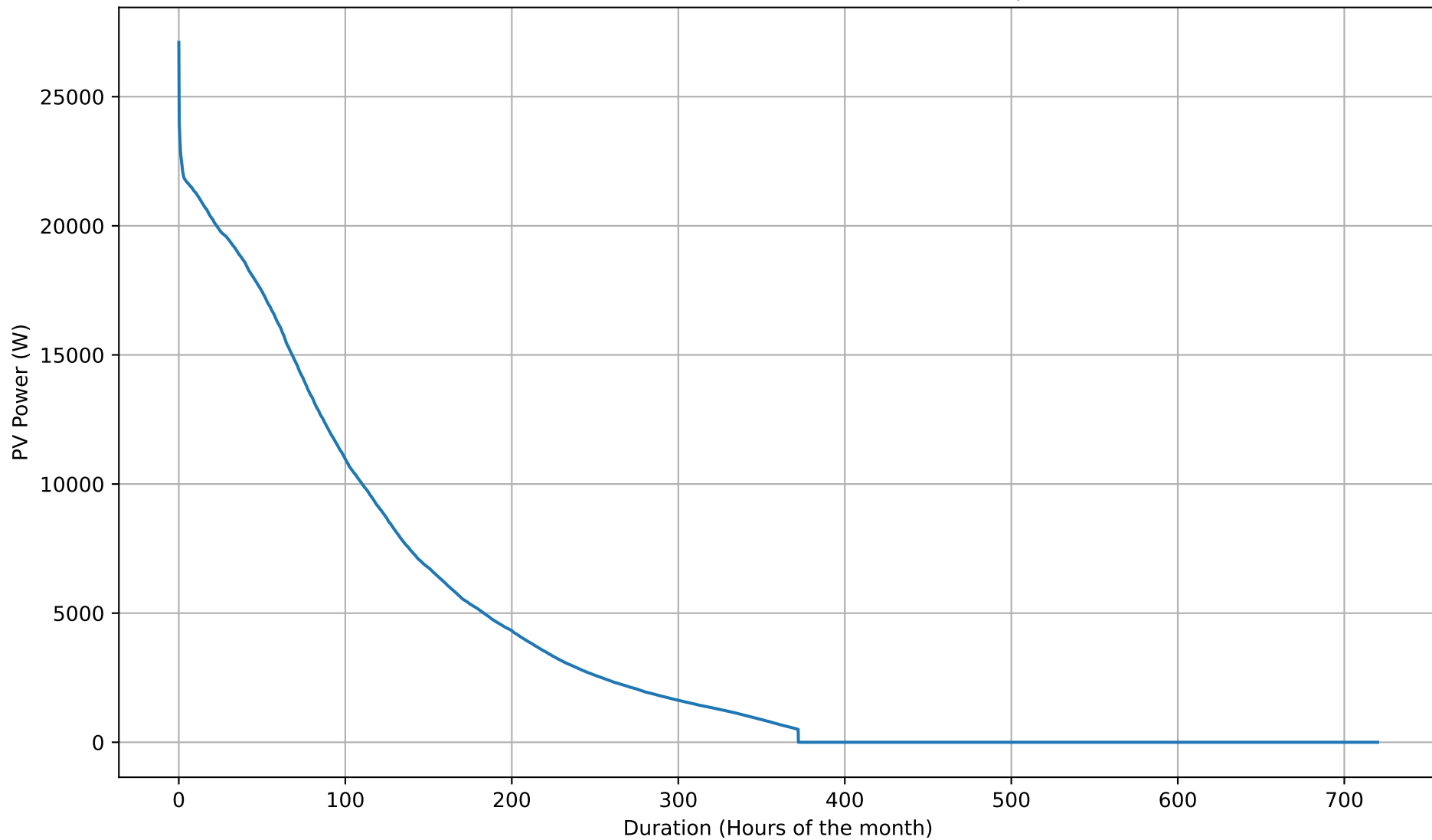
PV Production Duration Curve - 8kWh - Apr
