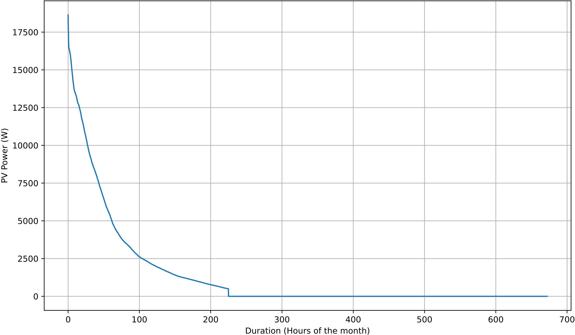
PV Production Duration Curve - 8kWh - Feb
