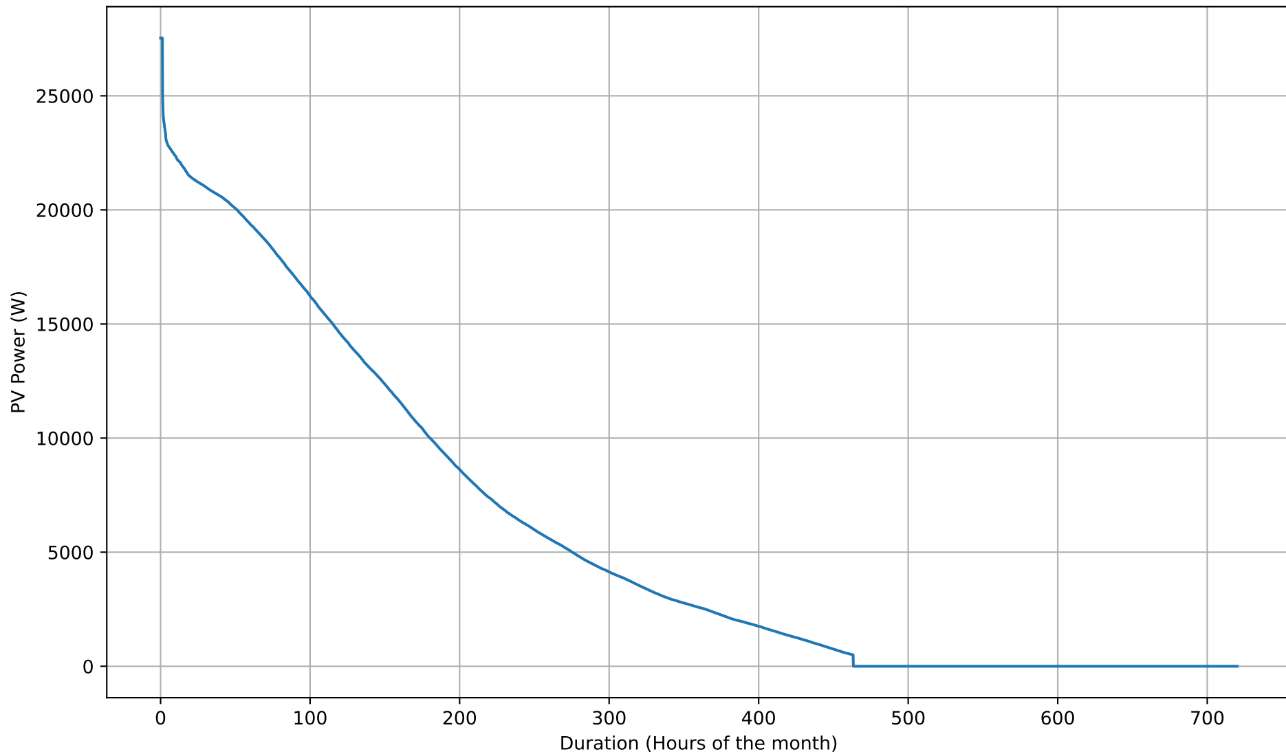
PV Production Duration Curve - 8kWh - Jun
