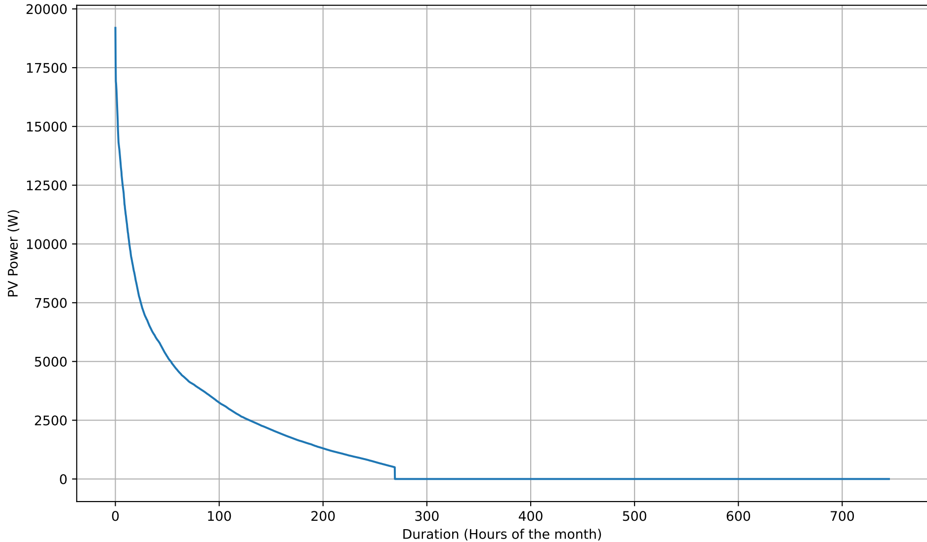
PV Production Duration Curve - 8kWh - Oct
