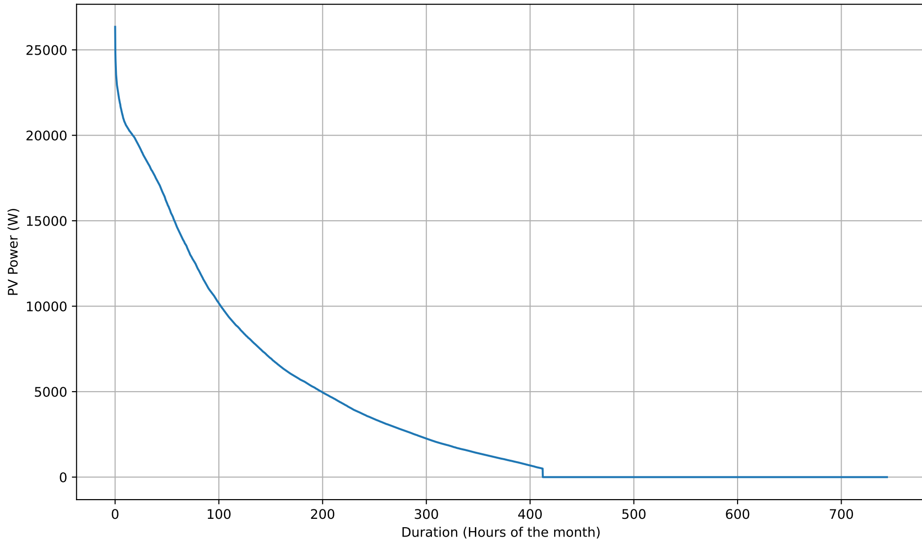
PV Production Duration Curve - 8kWh - Aug
