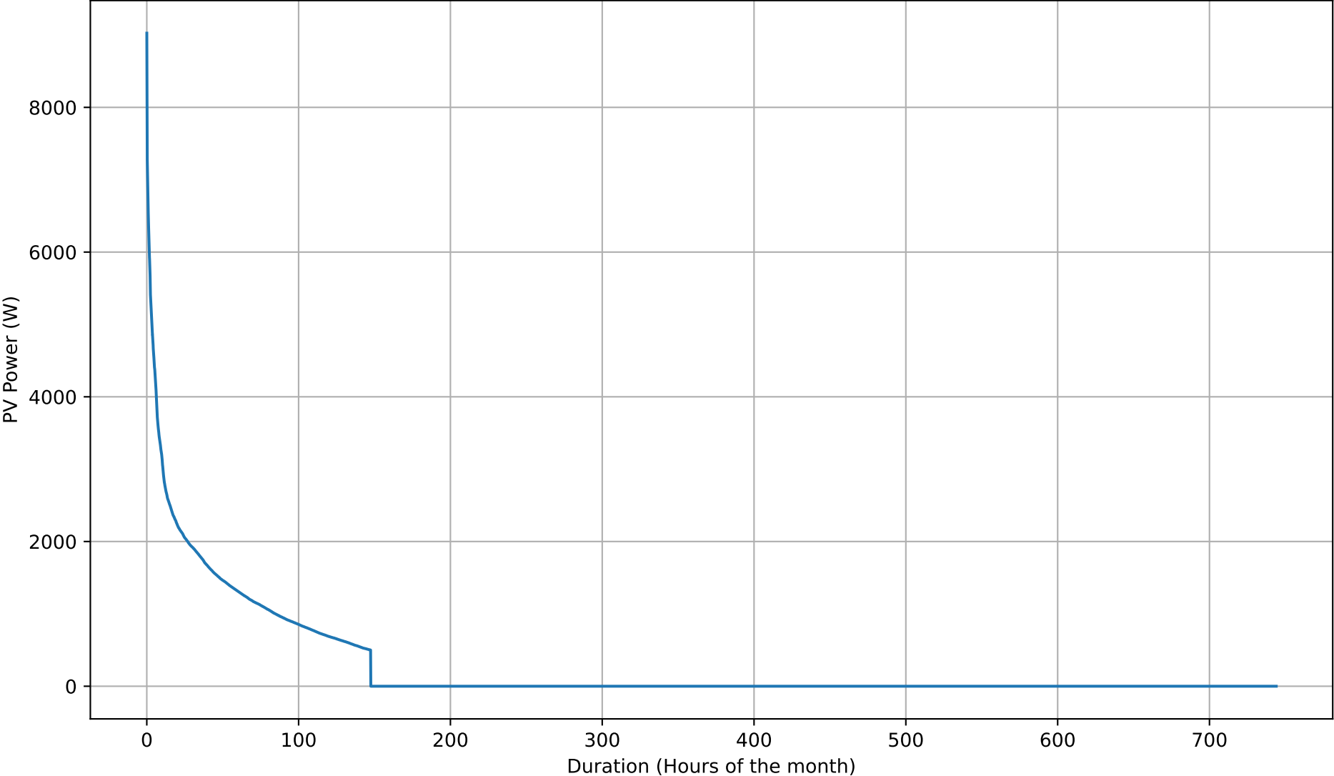
PV Production Duration Curve - 8kWh - Dec
