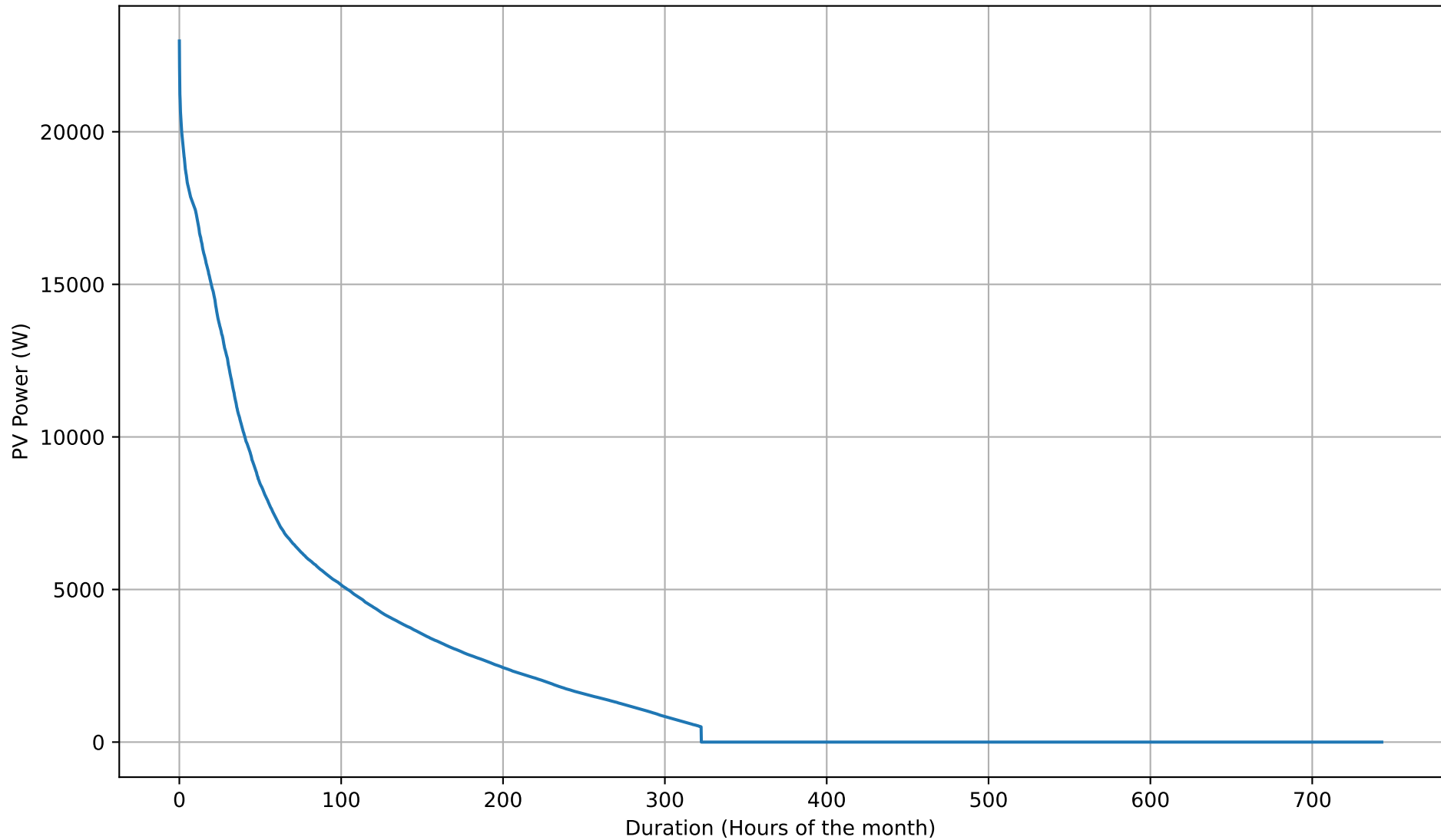
PV Production Duration Curve - 8kWh - Mar
