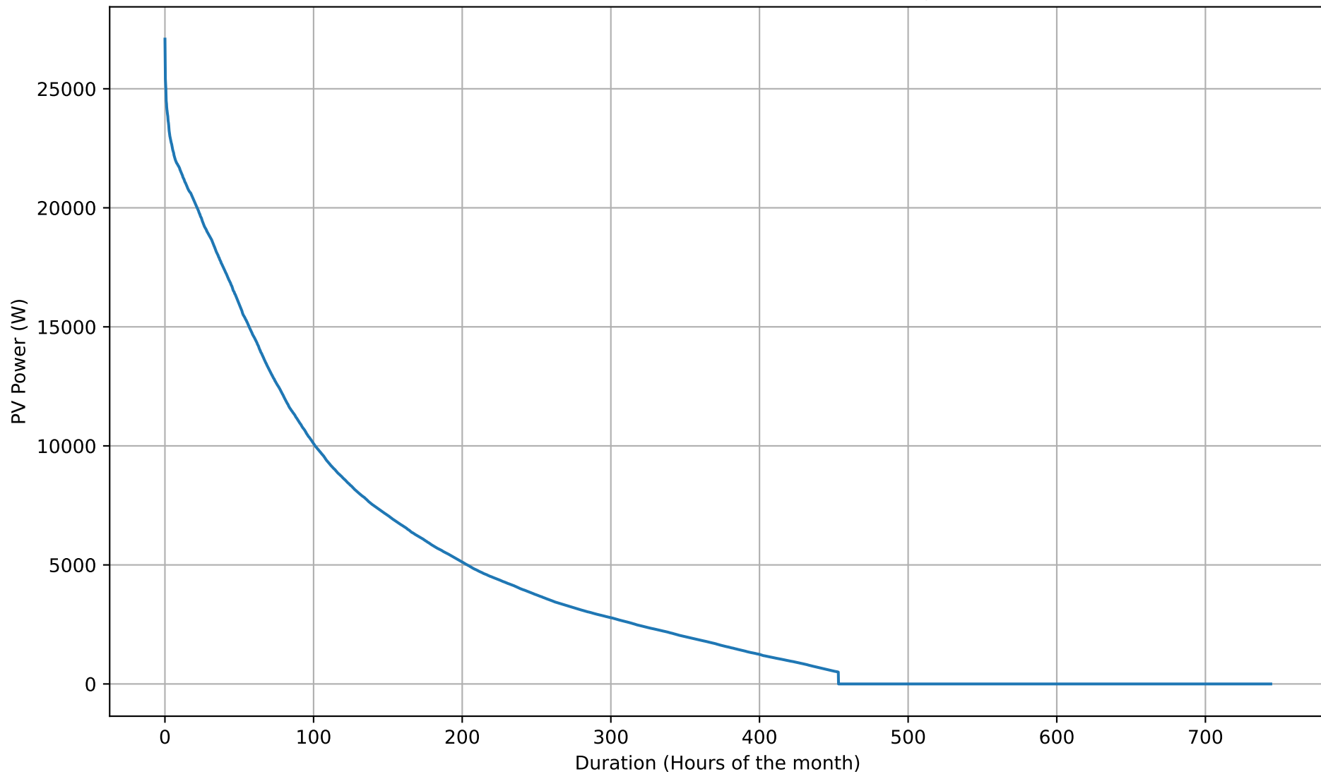
PV Production Duration Curve - 8kWh - Jul
