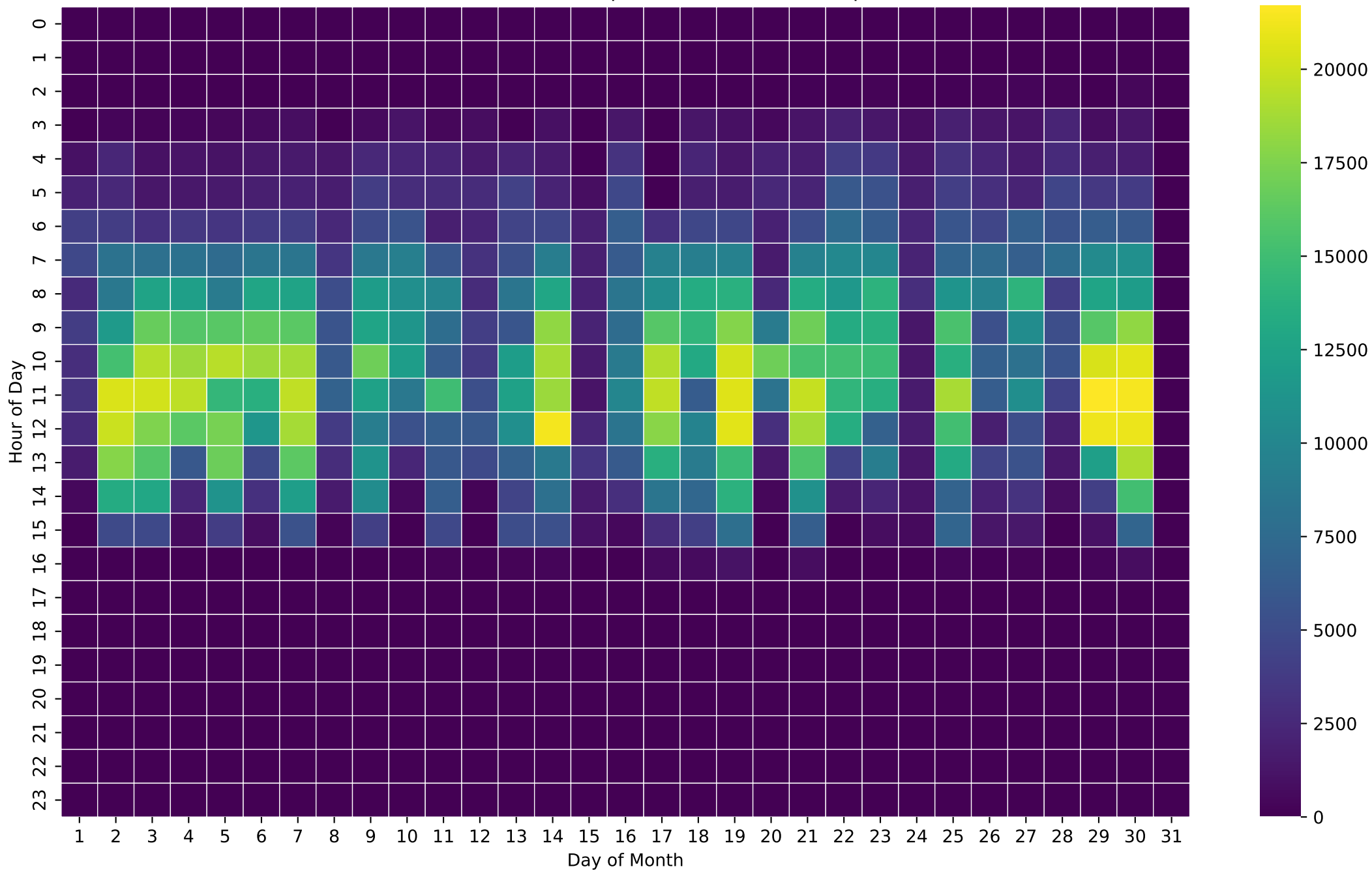
PV Production Heatmap (Wh/Hour) - 8kWh - Apr
