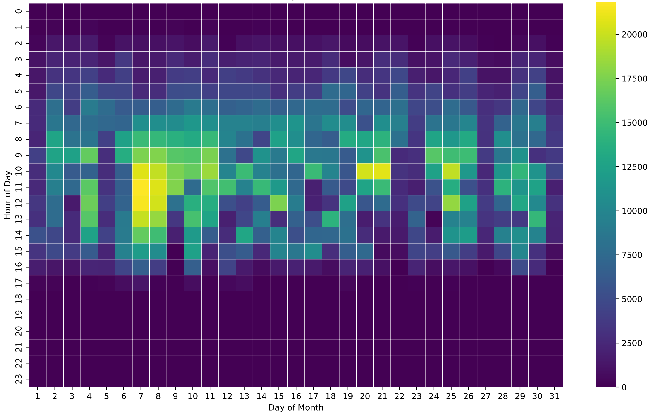
PV Production Heatmap (Wh/Hour) - 8kWh - Jul
