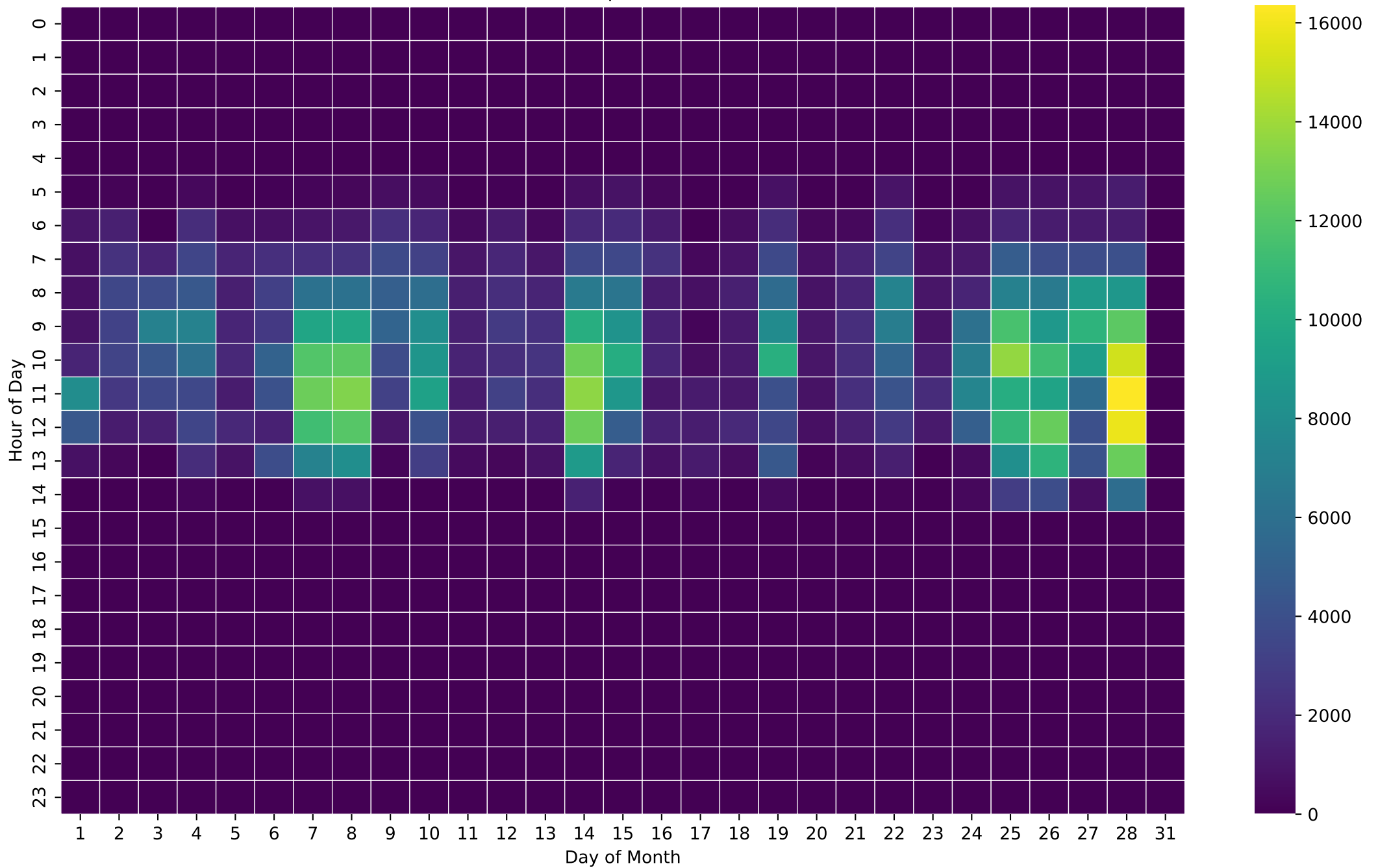
PV Production Heatmap (Wh/Hour) - 8kWh - Feb
