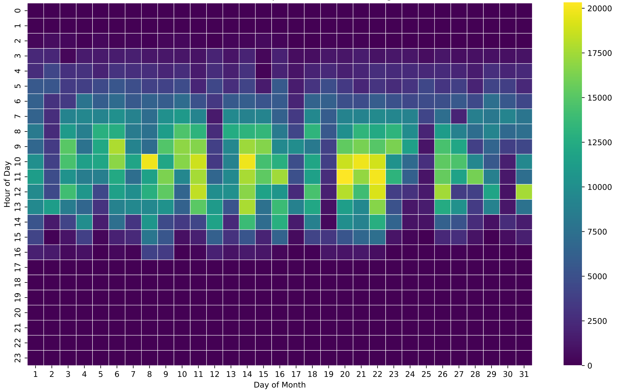
PV Production Heatmap (Wh/Hour) - 8kWh - Aug
