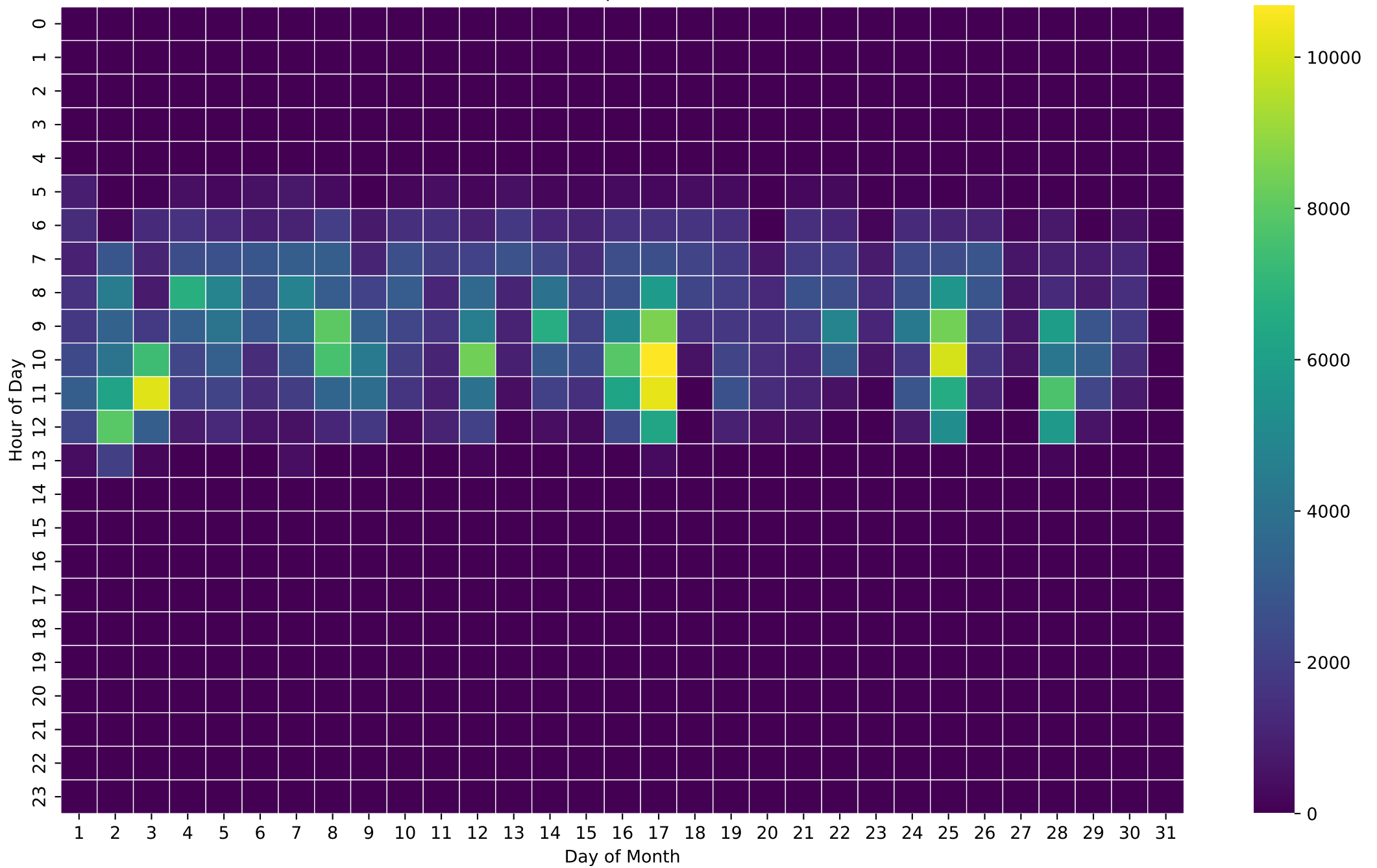
PV Production Heatmap (Wh/Hour) - 8kWh - Nov
