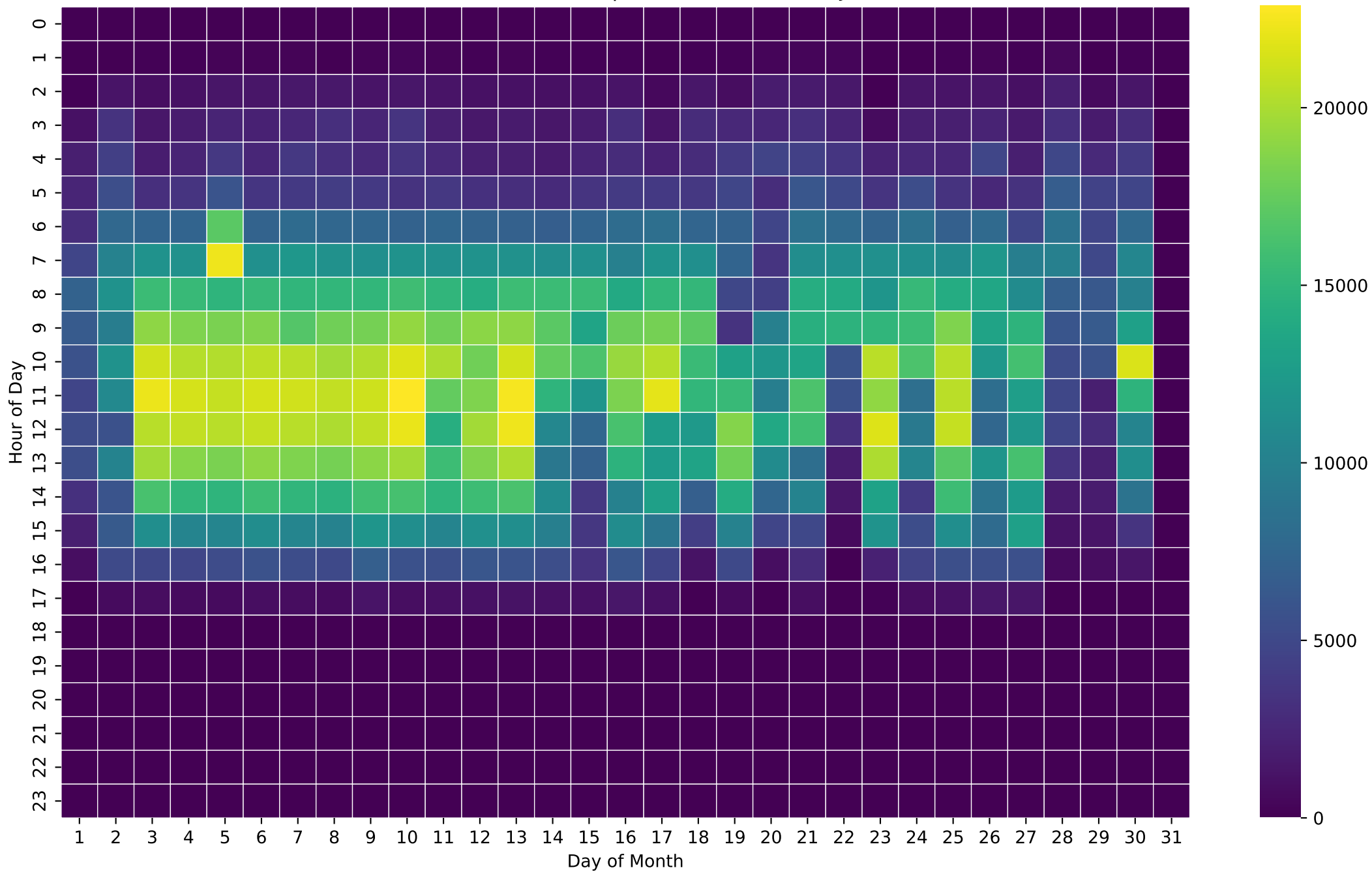
PV Production Heatmap (Wh/Hour) - 8kWh - Jun
