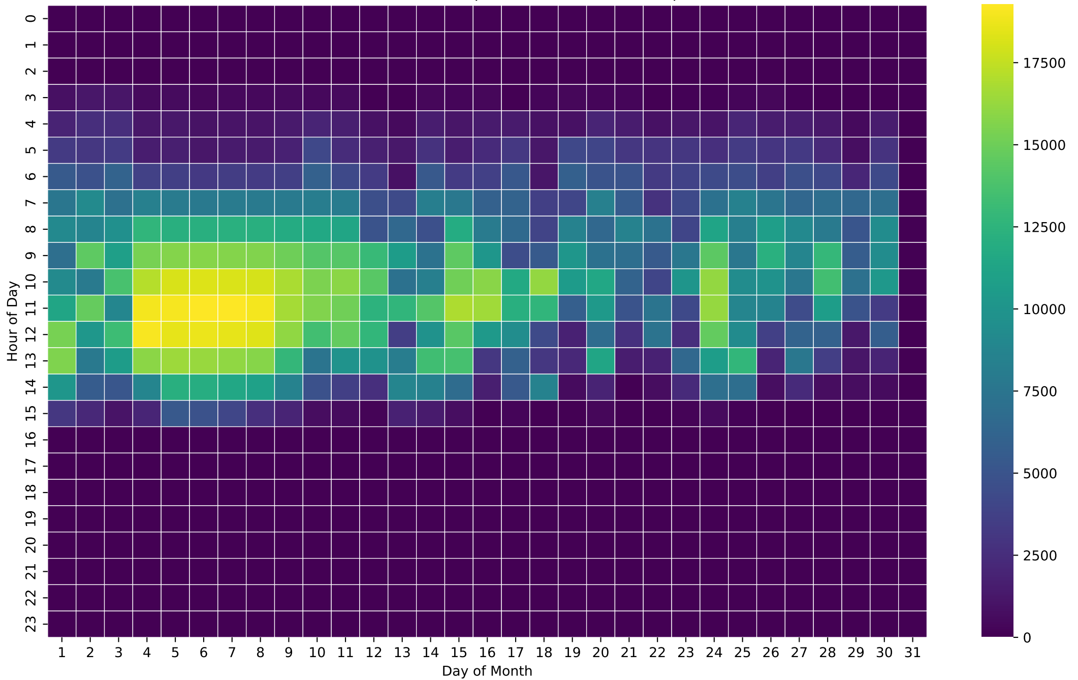
PV Production Heatmap (Wh/Hour) - 8kWh - Sep
