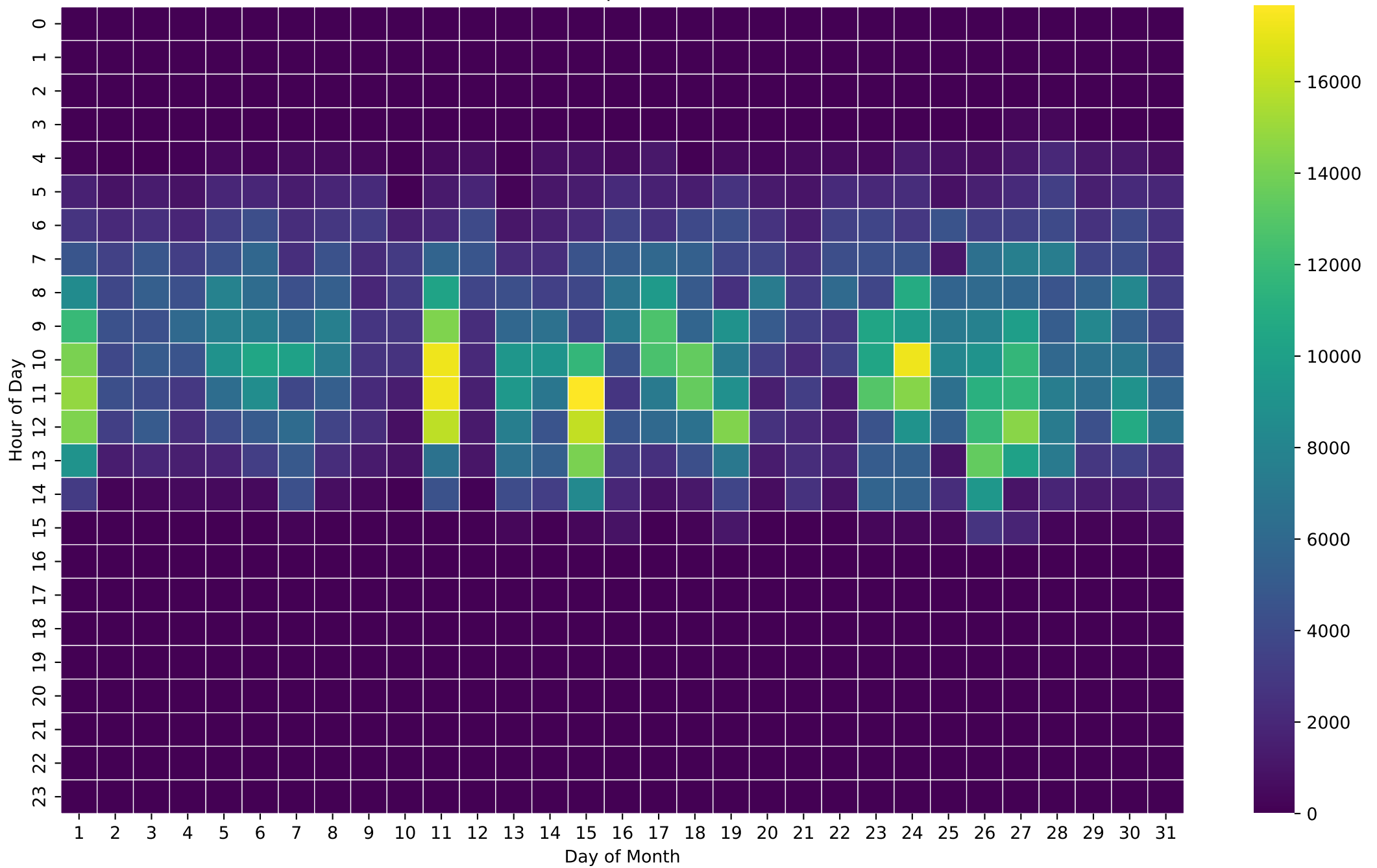
PV Production Heatmap (Wh/Hour) - 8kWh - Mar
