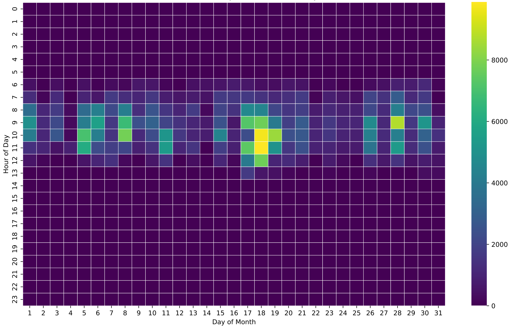
PV Production Heatmap (Wh/Hour) - 8kWh - Jan
