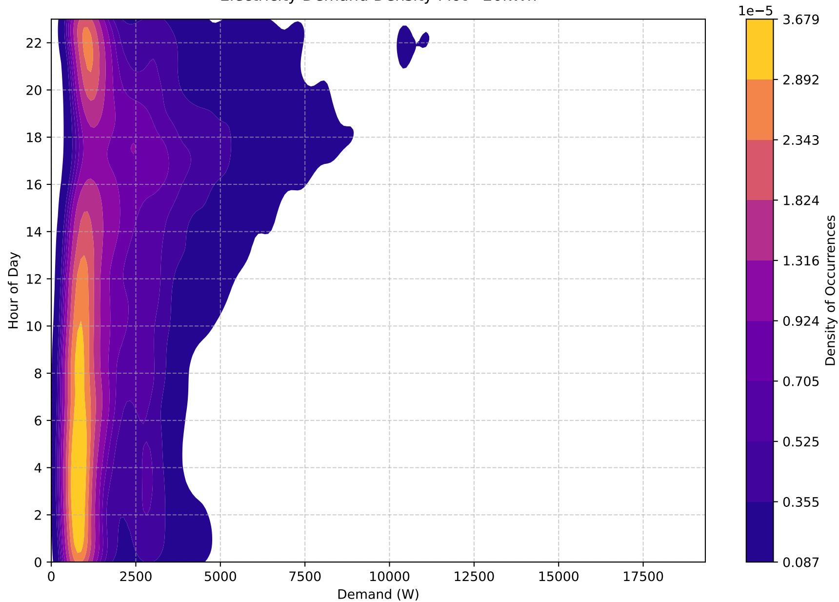
Electricity Demand Density Plot - 20kWh
