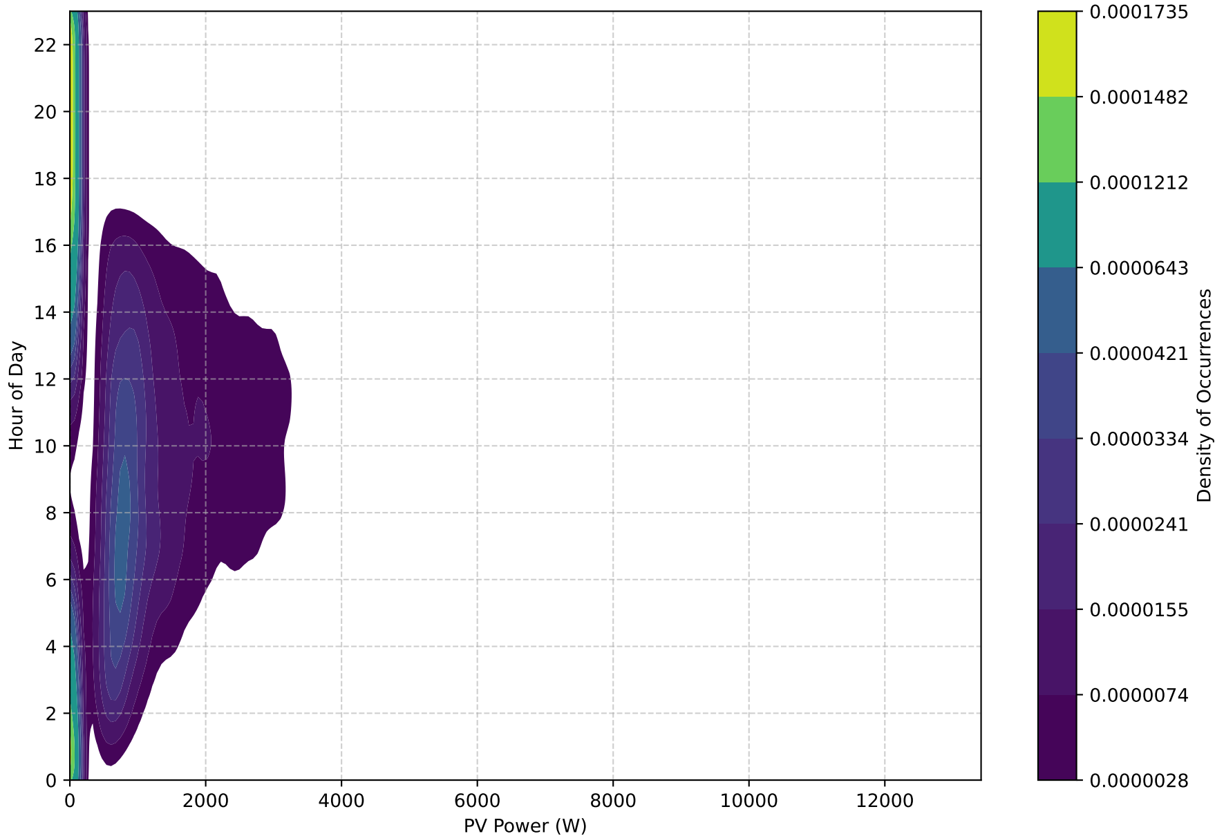
PV Self-Consumption Density Plot - NoBattery
