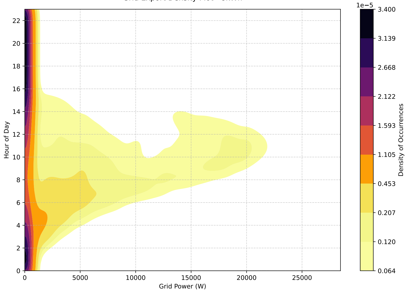
Grid Export Density Plot - 8kWh
