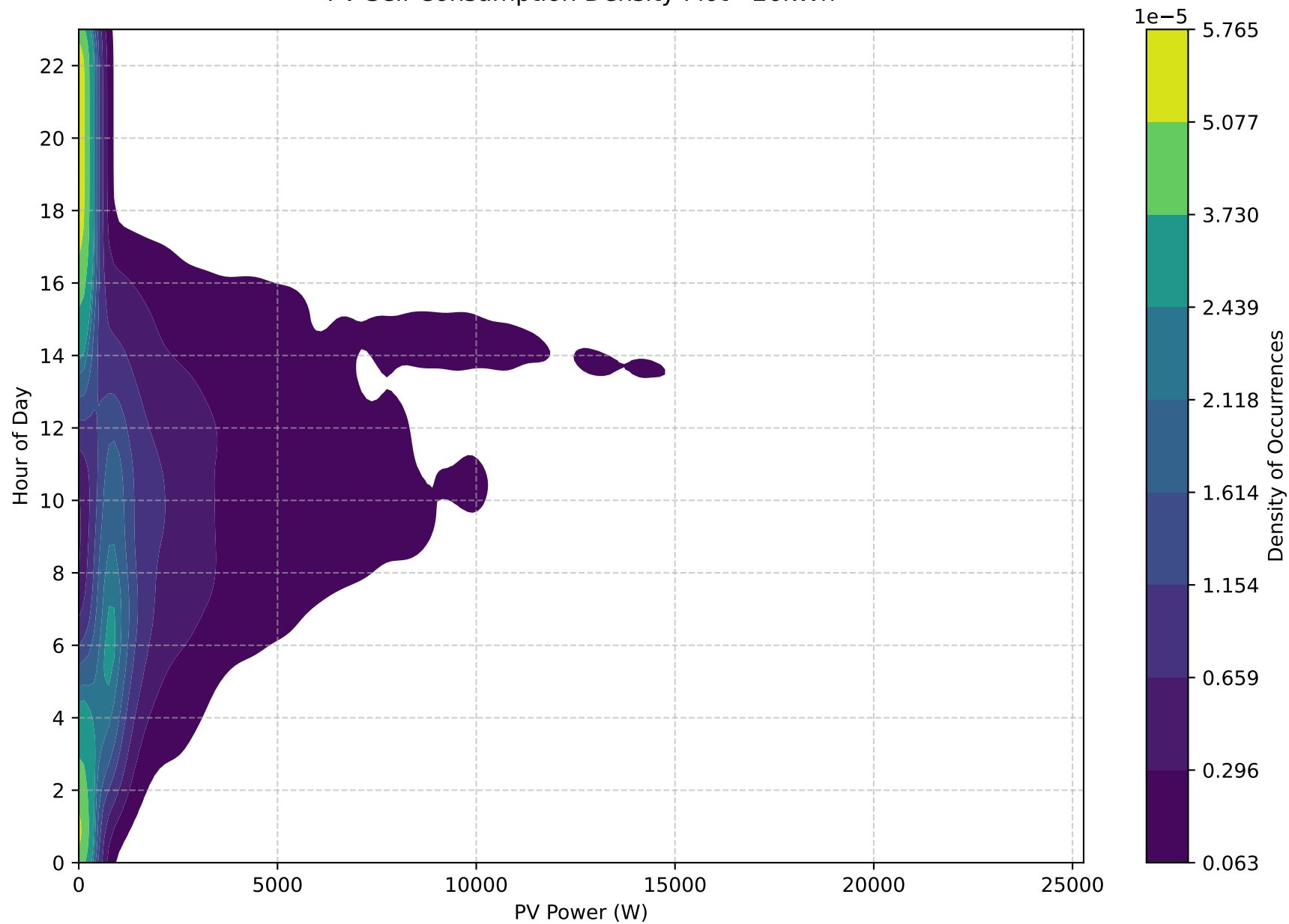
PV Self-Consumption Density Plot - 26kWh
