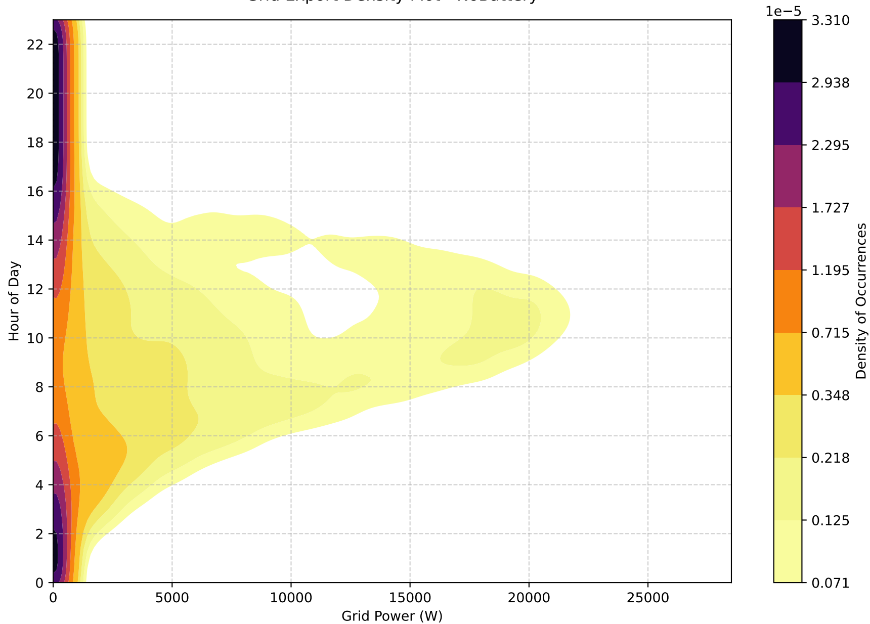
Grid Export Density Plot - NoBattery
