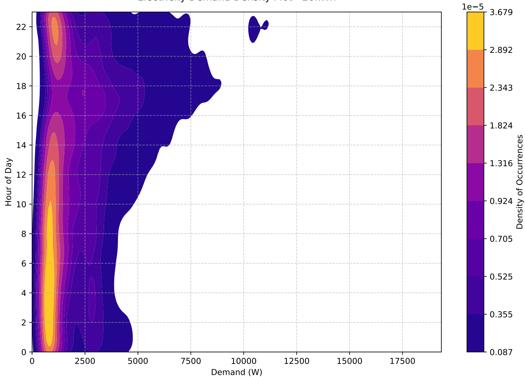
Electricity Demand Density Plot - 26kWh
