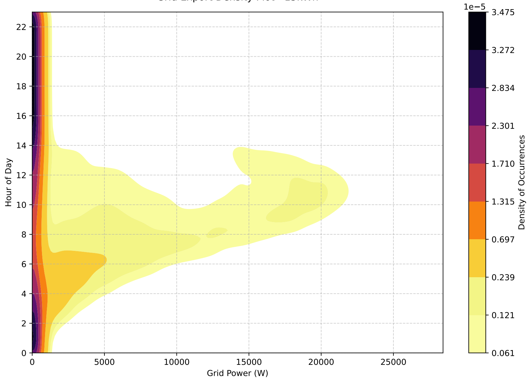
Grid Export Density Plot - 15kWh
