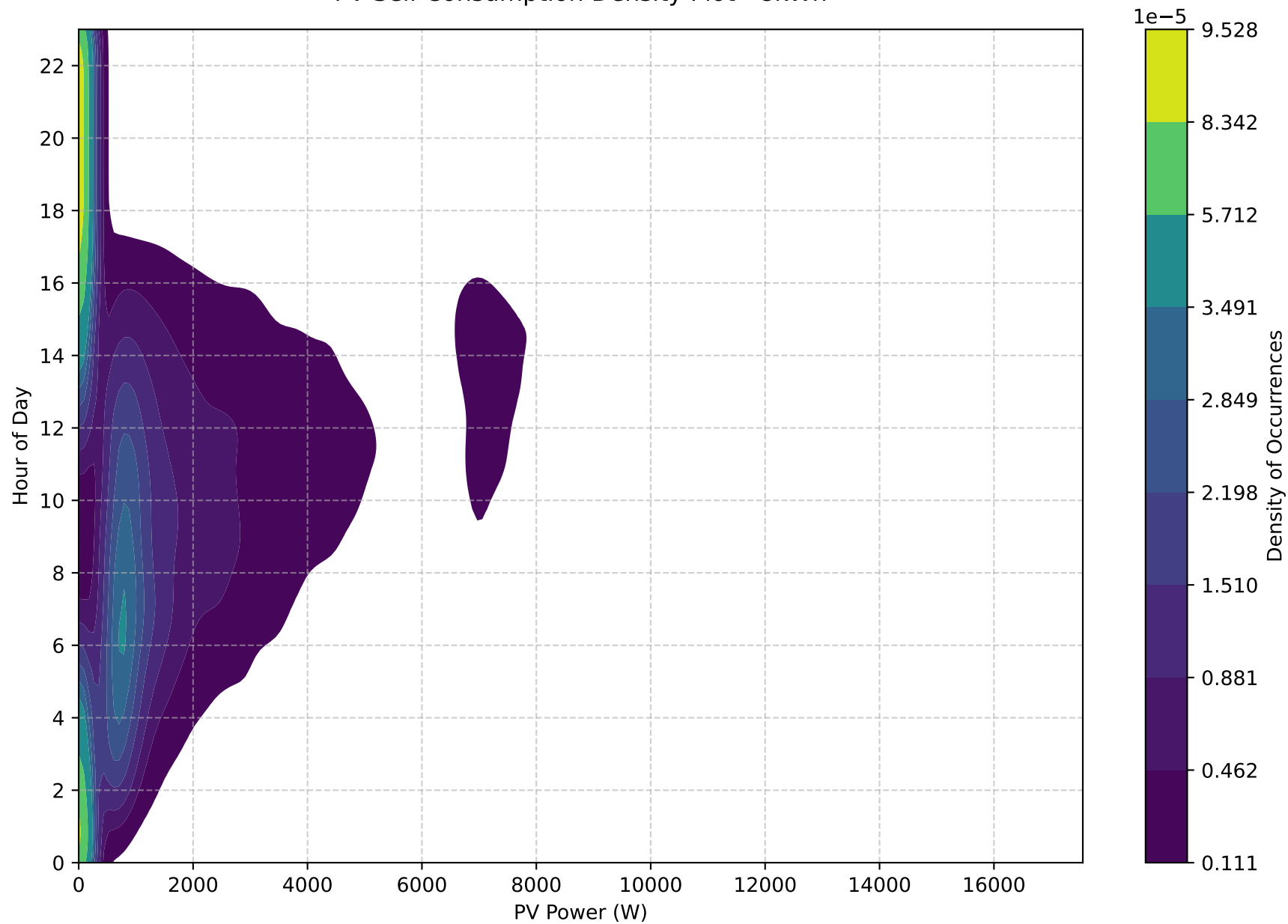
PV Self-Consumption Density Plot - 8kWh
