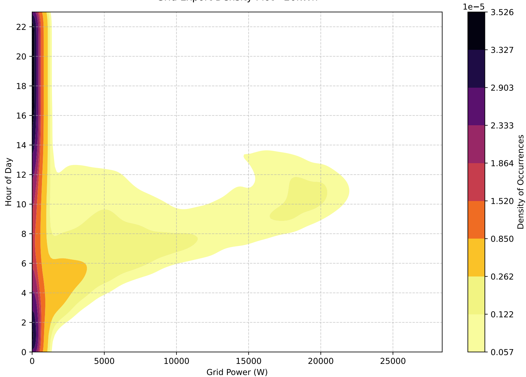
Grid Export Density Plot - 20kWh
