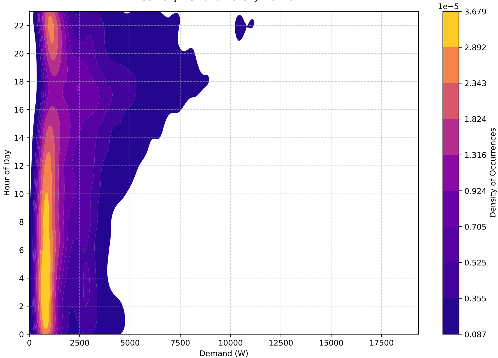
Electricity Demand Density Plot - 5kWh
