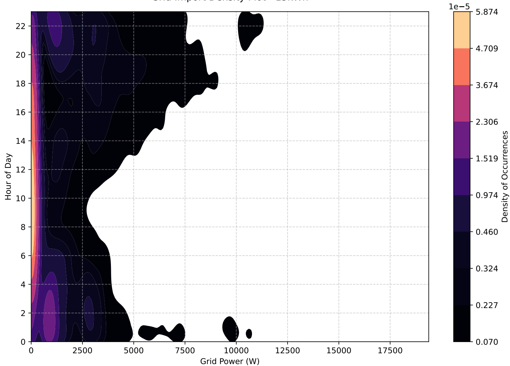
Grid Import Density Plot - 15kWh
