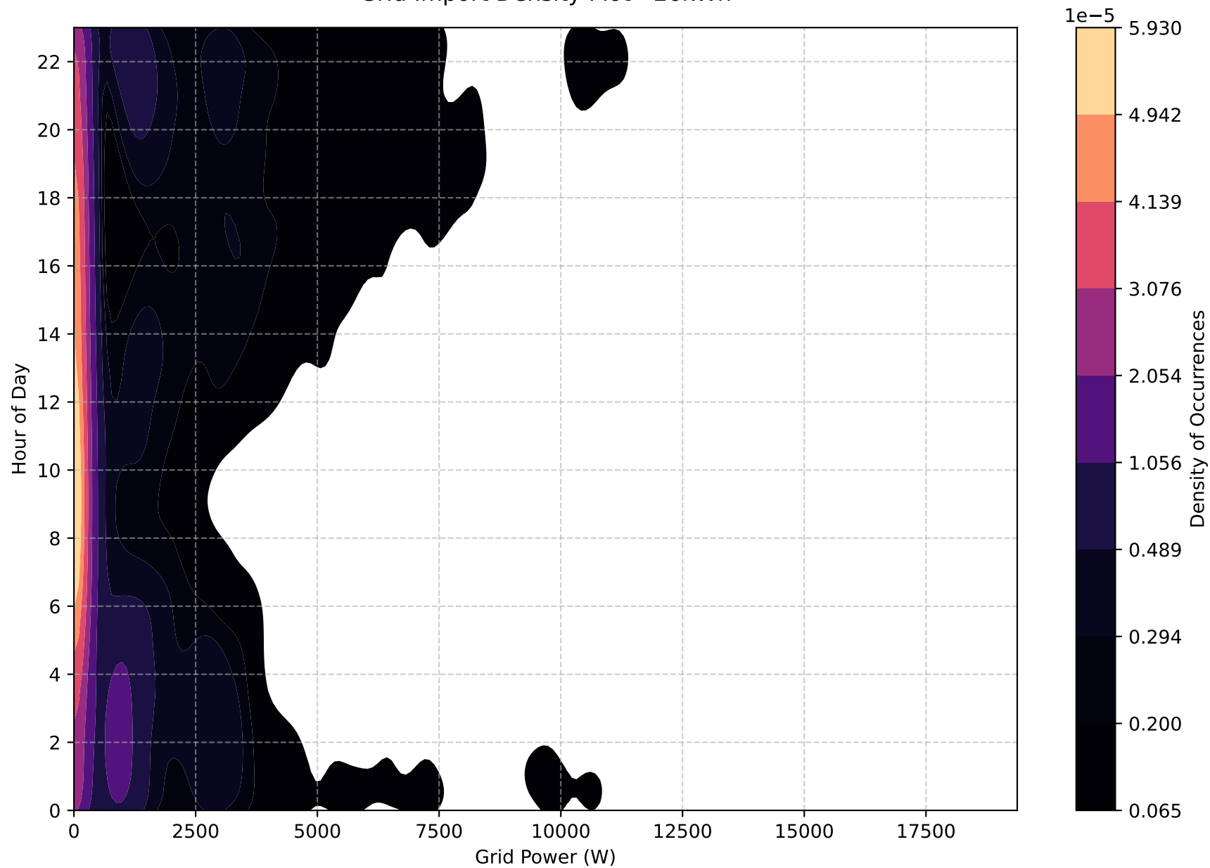
Grid Import Density Plot - 26kWh
