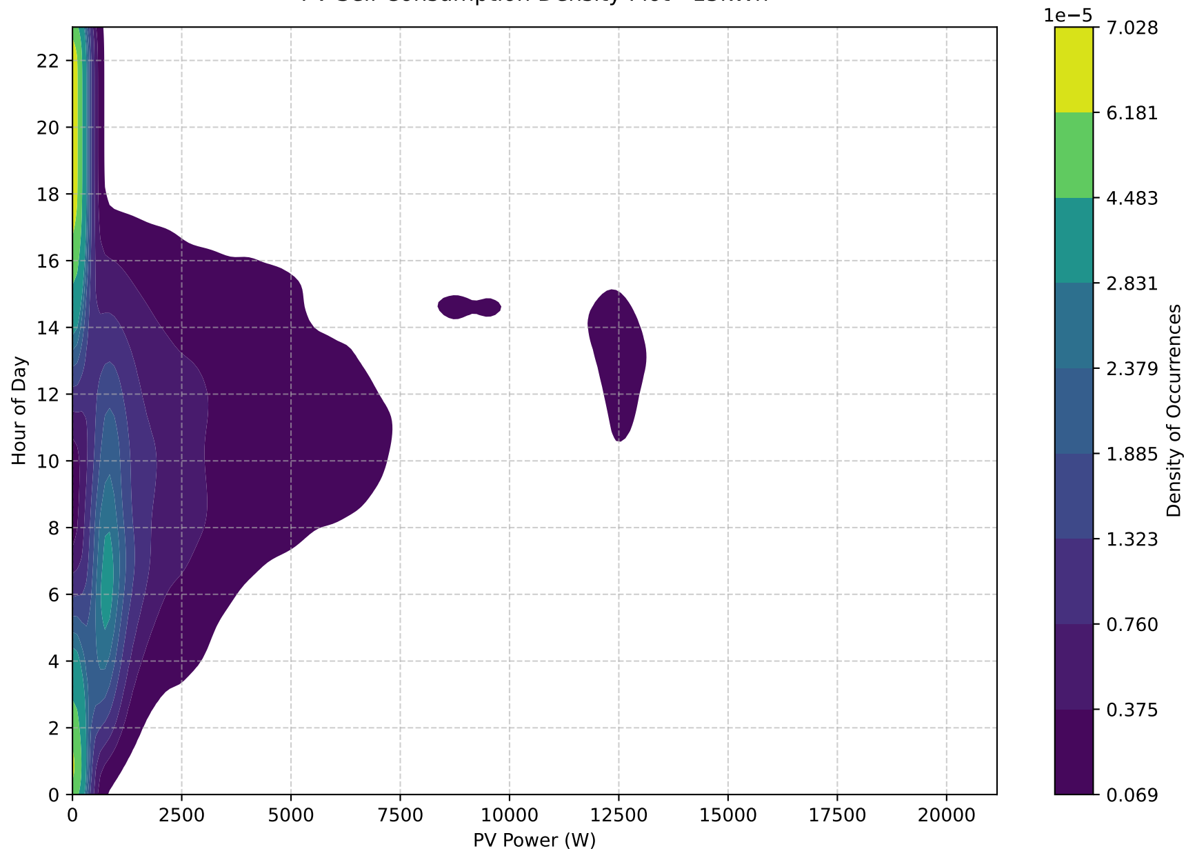
PV Self-Consumption Density Plot - 15kWh
