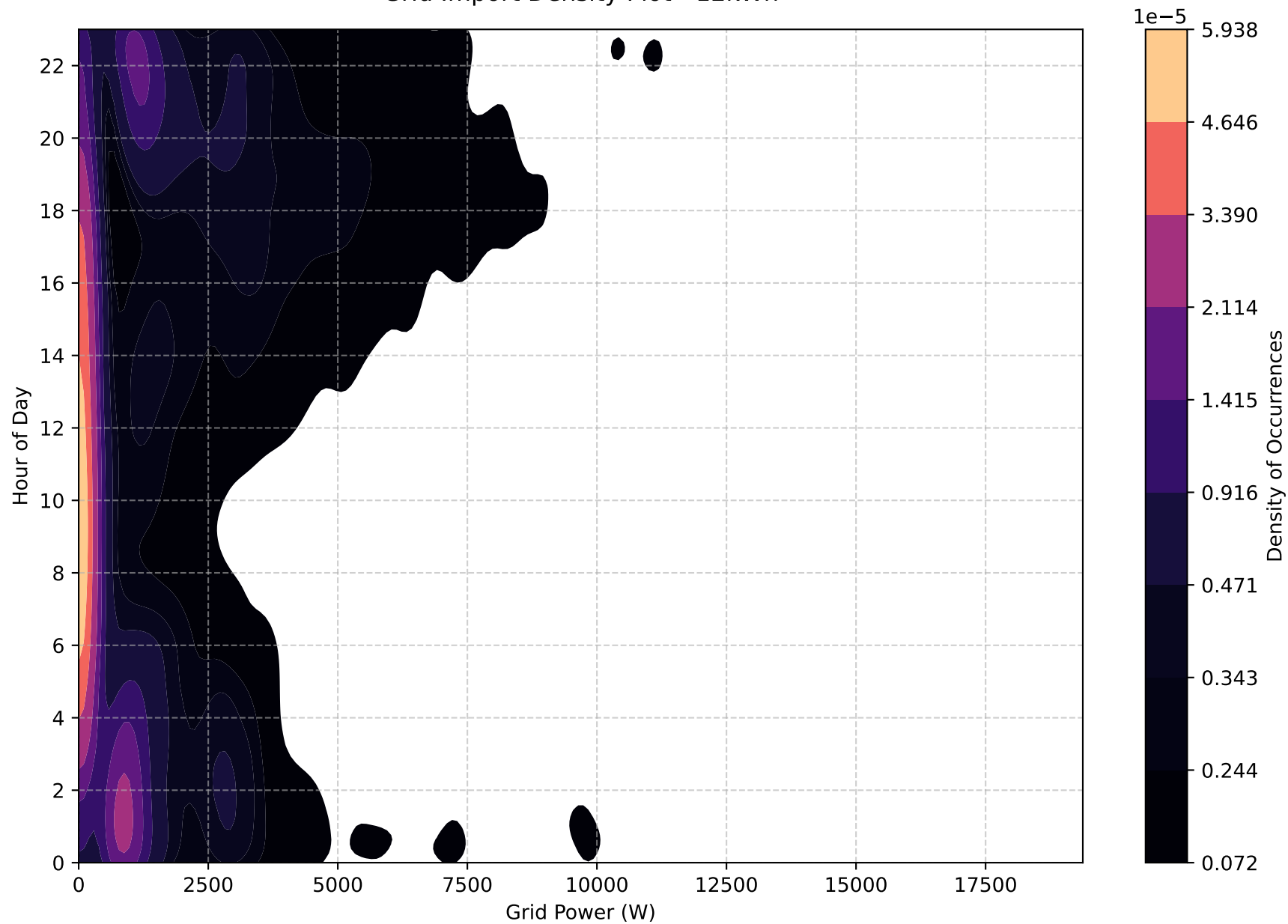
Grid Import Density Plot - 12kWh
