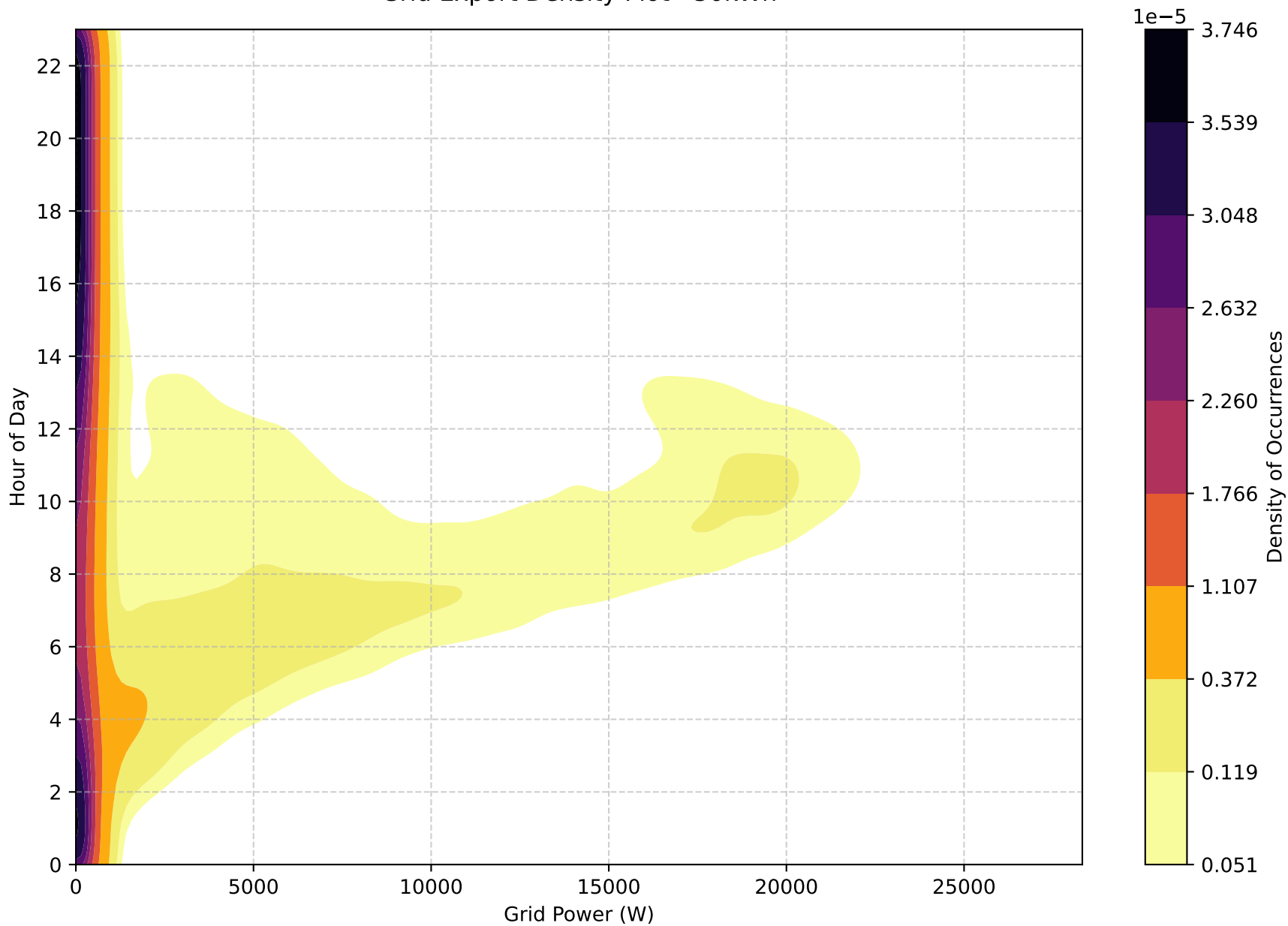
Grid Export Density Plot - 50kWh
