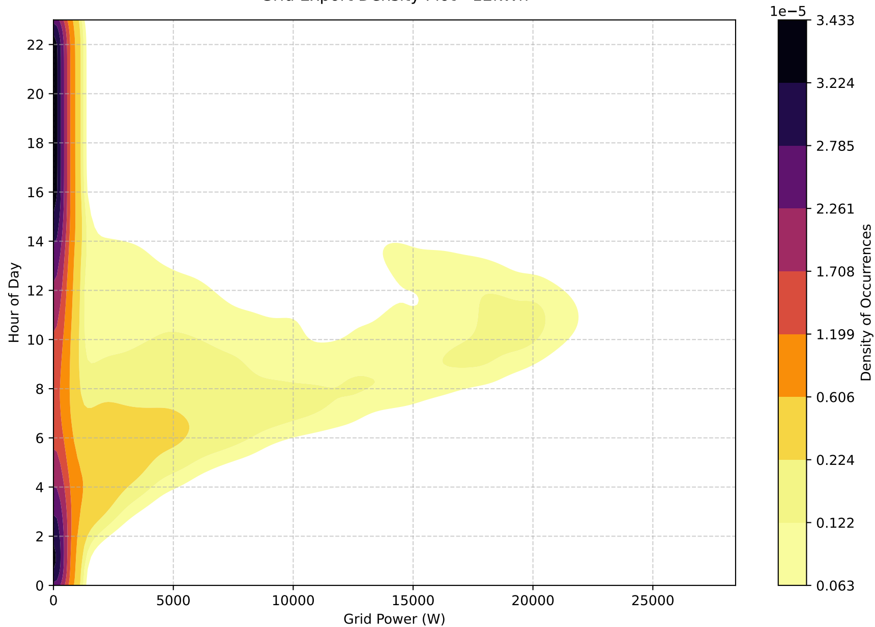
Grid Export Density Plot - 12kWh
