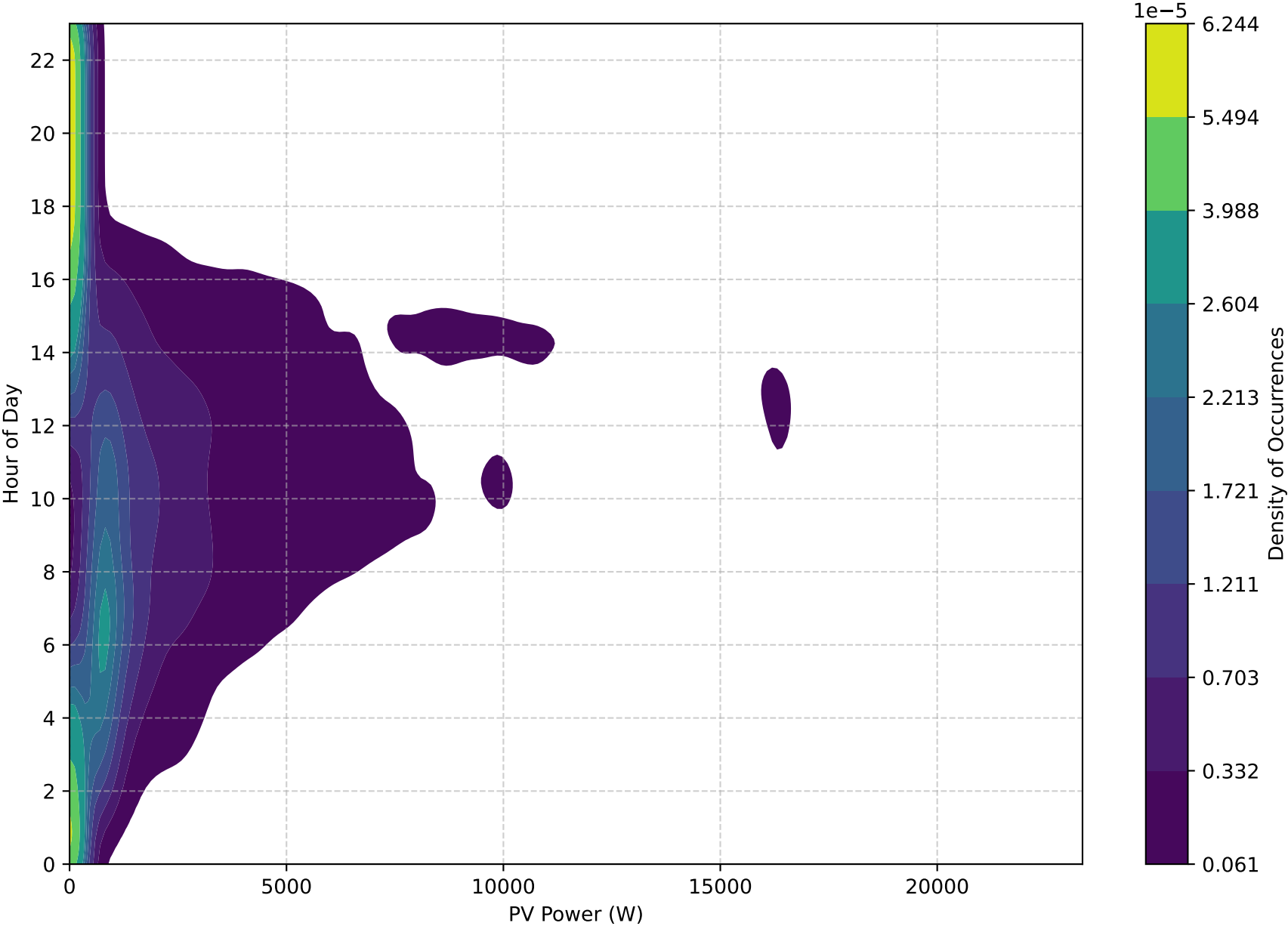
PV Self-Consumption Density Plot - 20kWh
