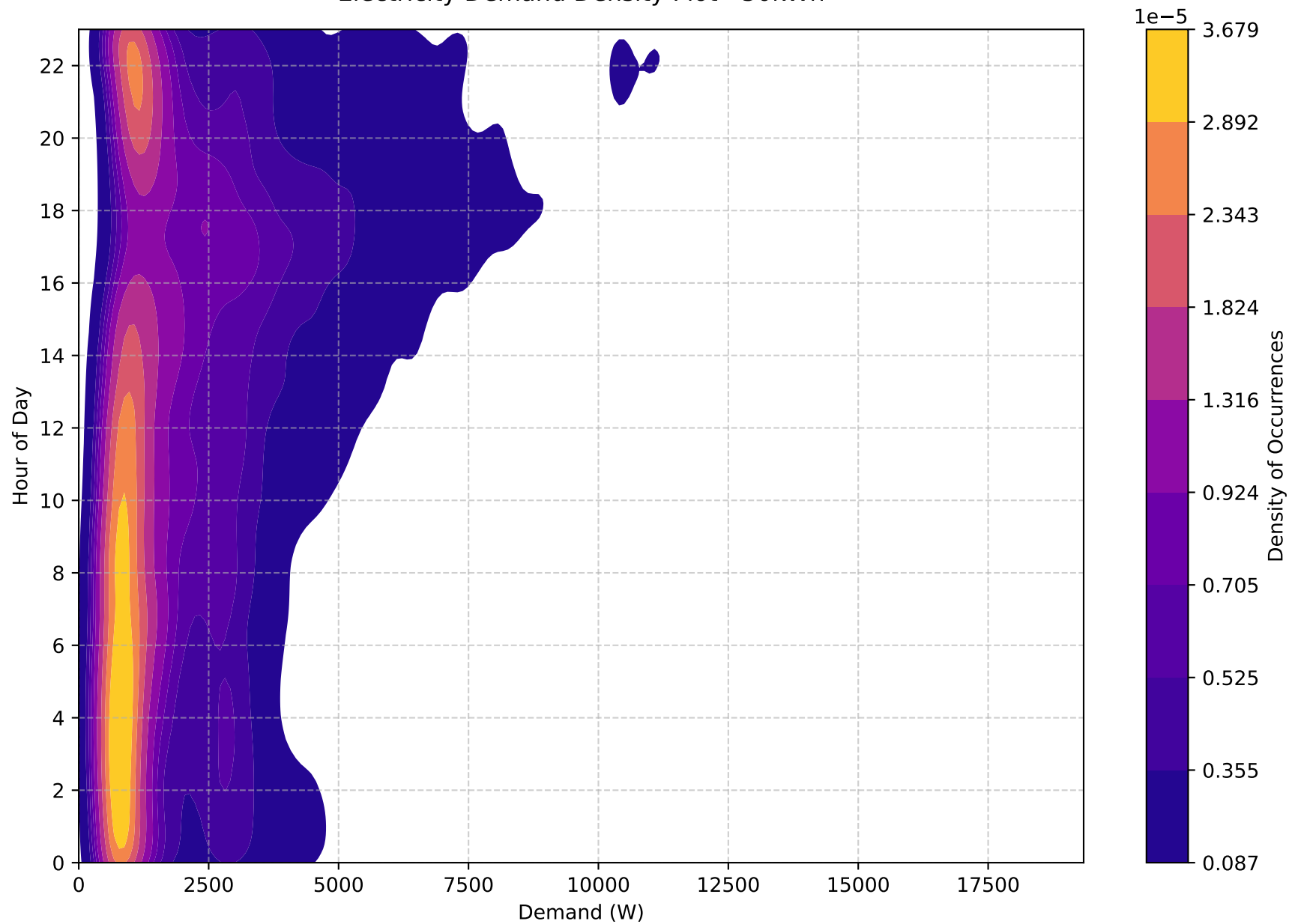
Electricity Demand Density Plot - 50kWh
