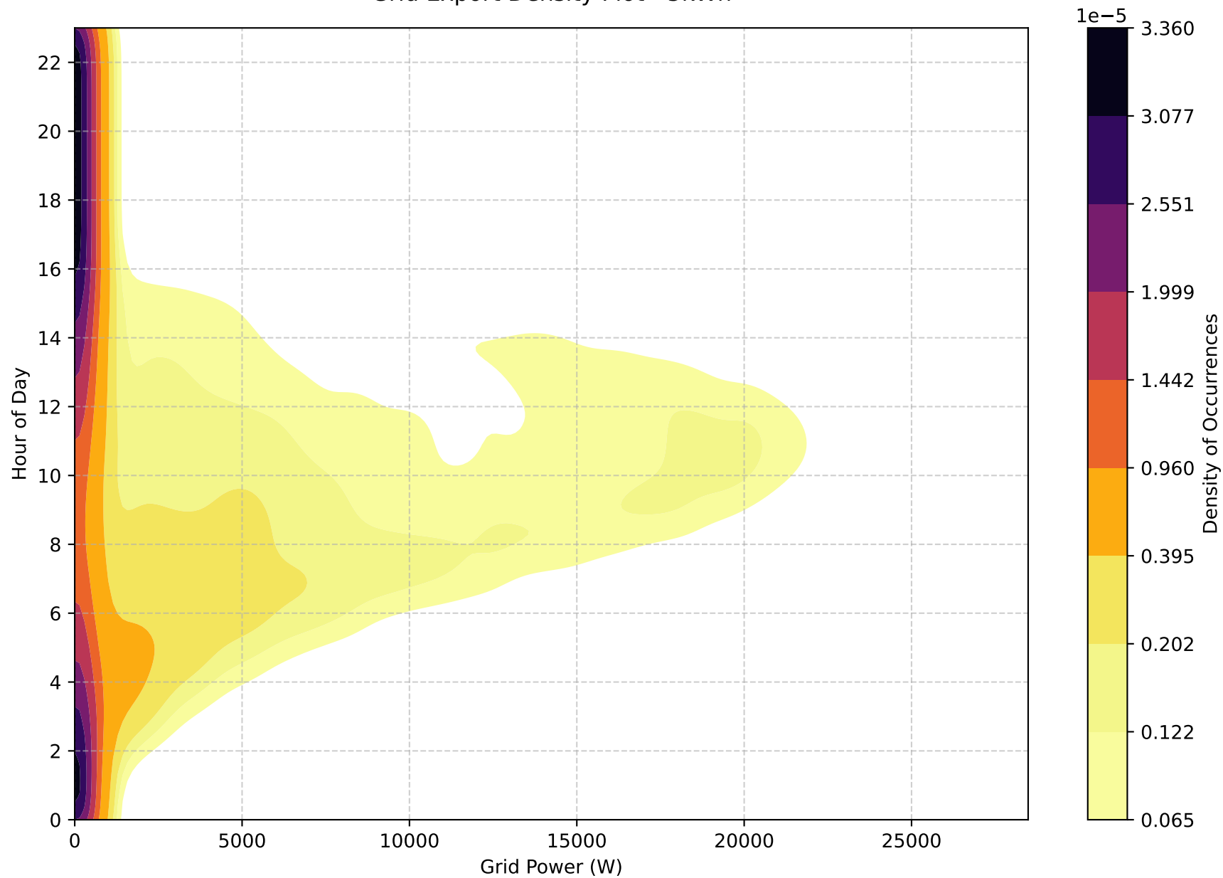
Grid Export Density Plot - 5kWh
