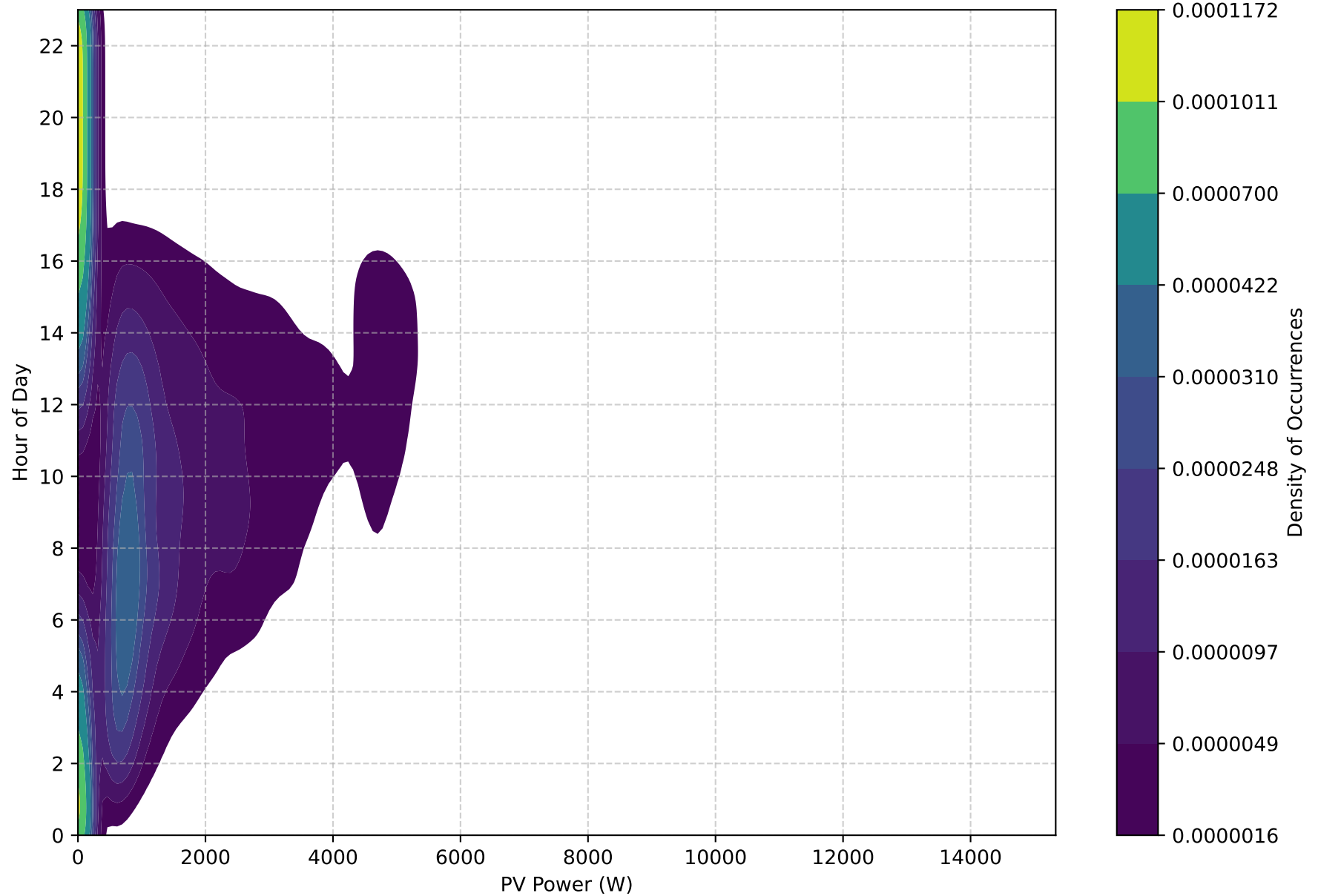
PV Self-Consumption Density Plot - 5kWh
