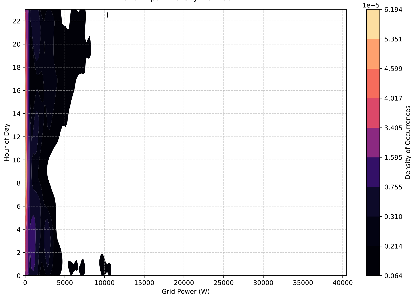
Grid Import Density Plot - 50kWh
