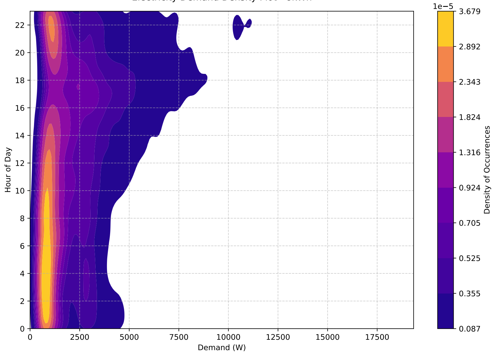
Electricity Demand Density Plot - 8kWh
