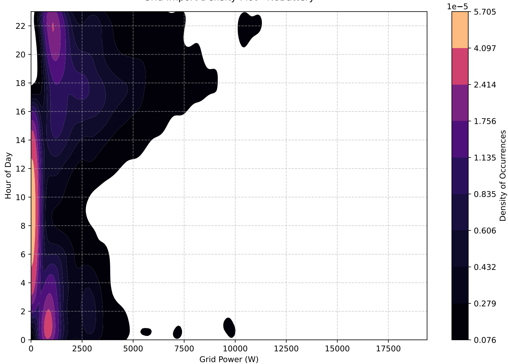
Grid Import Density Plot - NoBattery
