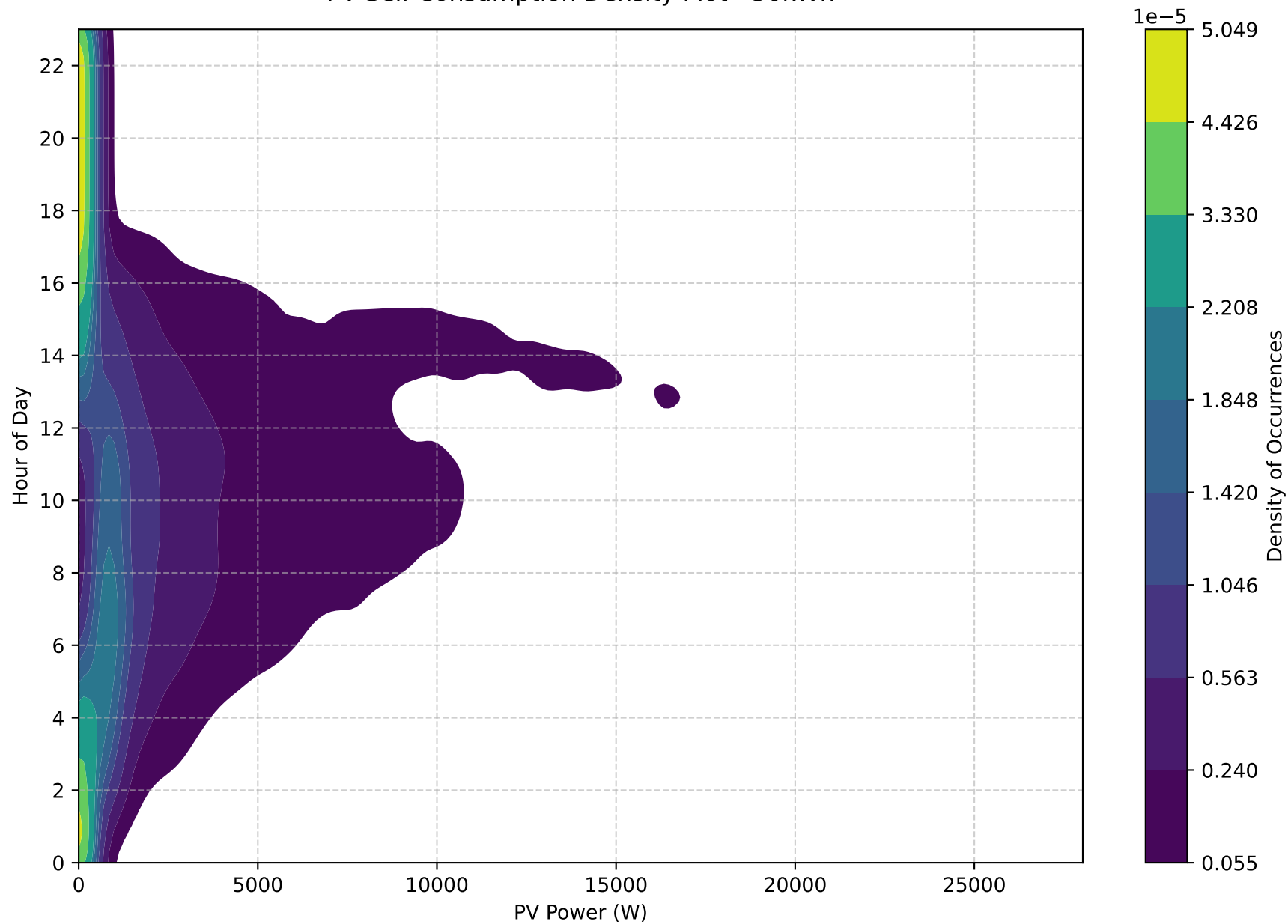
PV Self-Consumption Density Plot - 50kWh
