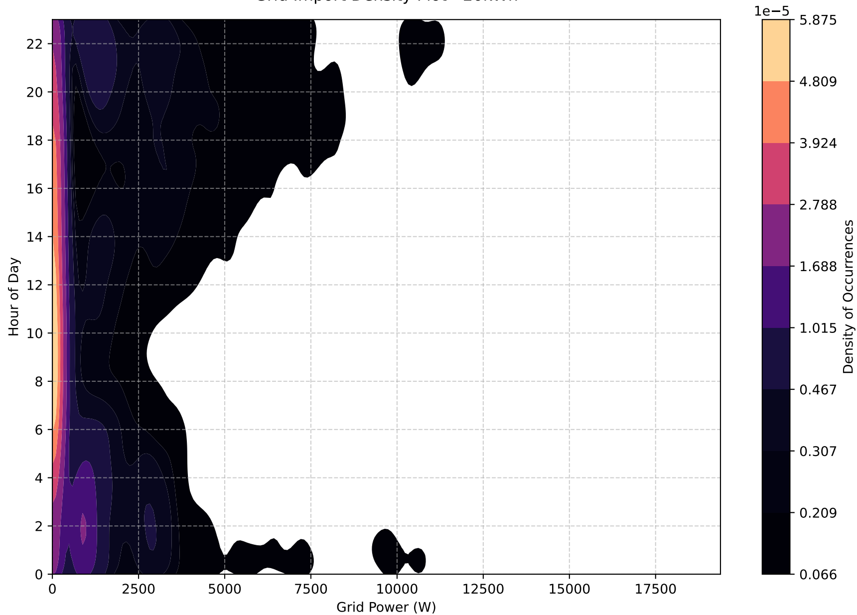
Grid Import Density Plot - 20kWh
