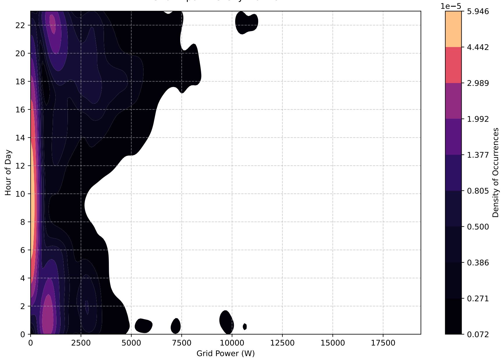
Grid Import Density Plot - 8kWh
