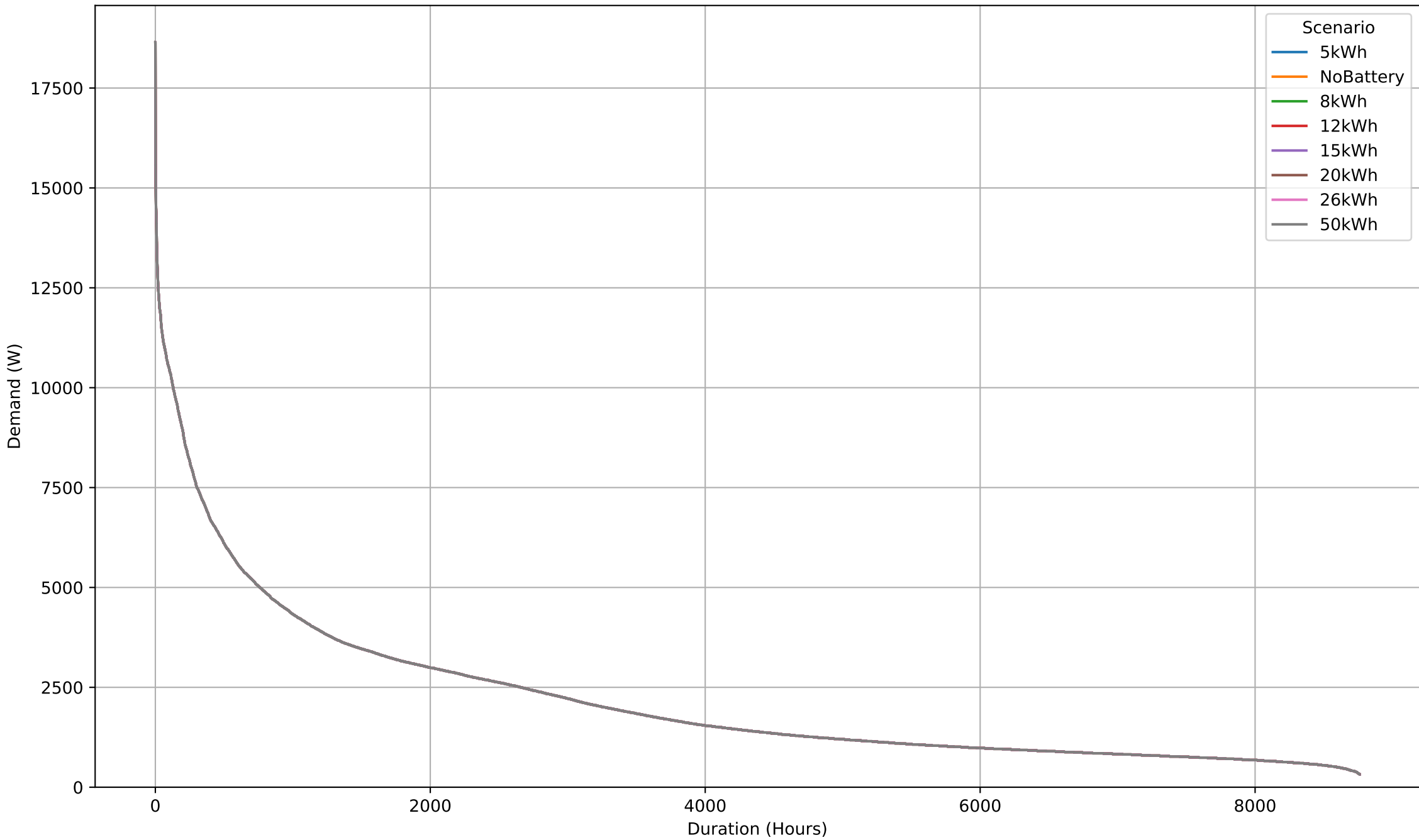
Combined Yearly Electricity Demand Duration Curves for All Scenarios
