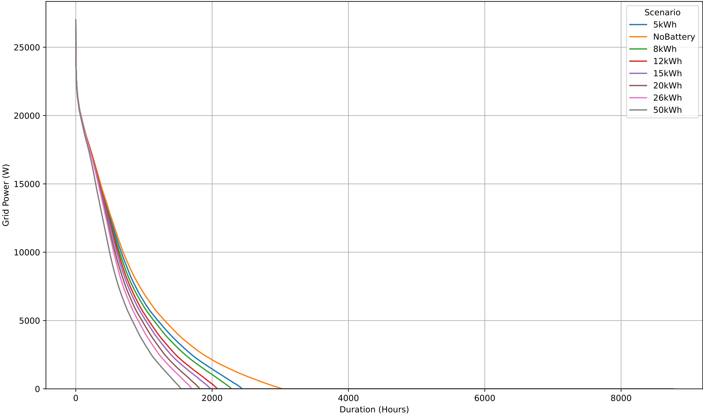
Combined Yearly Grid Export Duration Curves for All Scenarios
