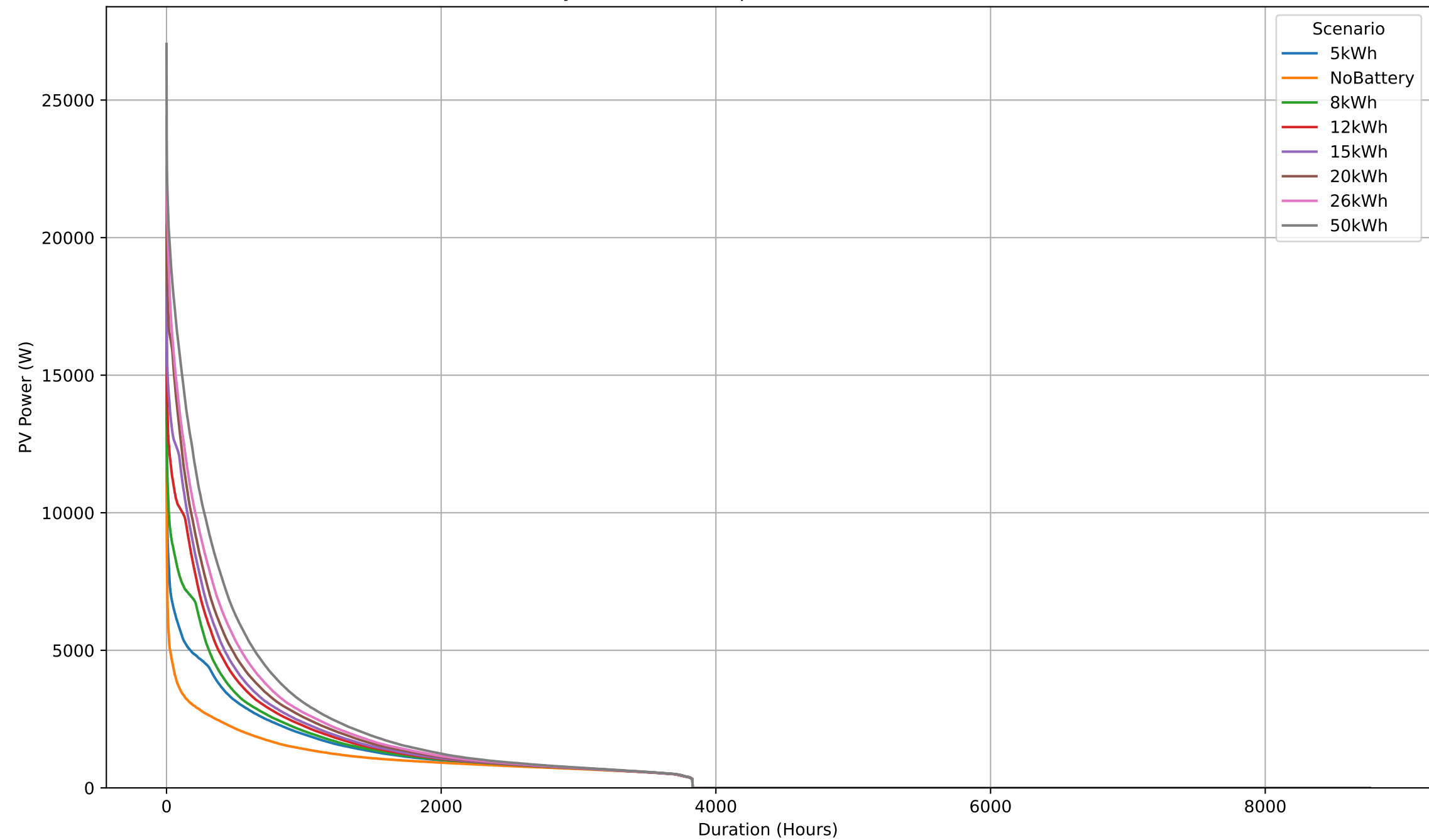
Combined Yearly PV Self-Consumption Duration Curves for All Scenarios
