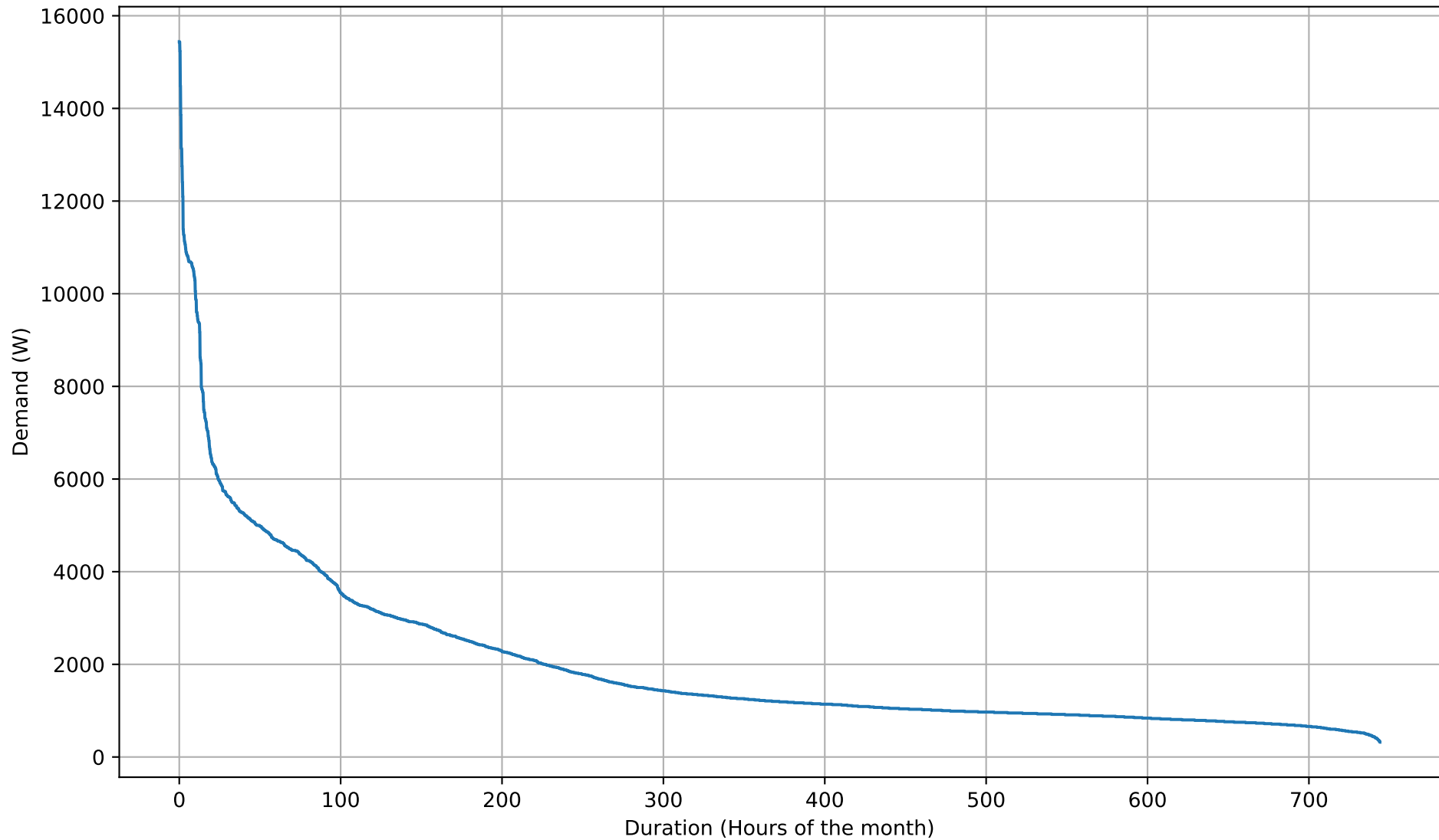
Electricity Demand Duration Curve - NoBattery - May
