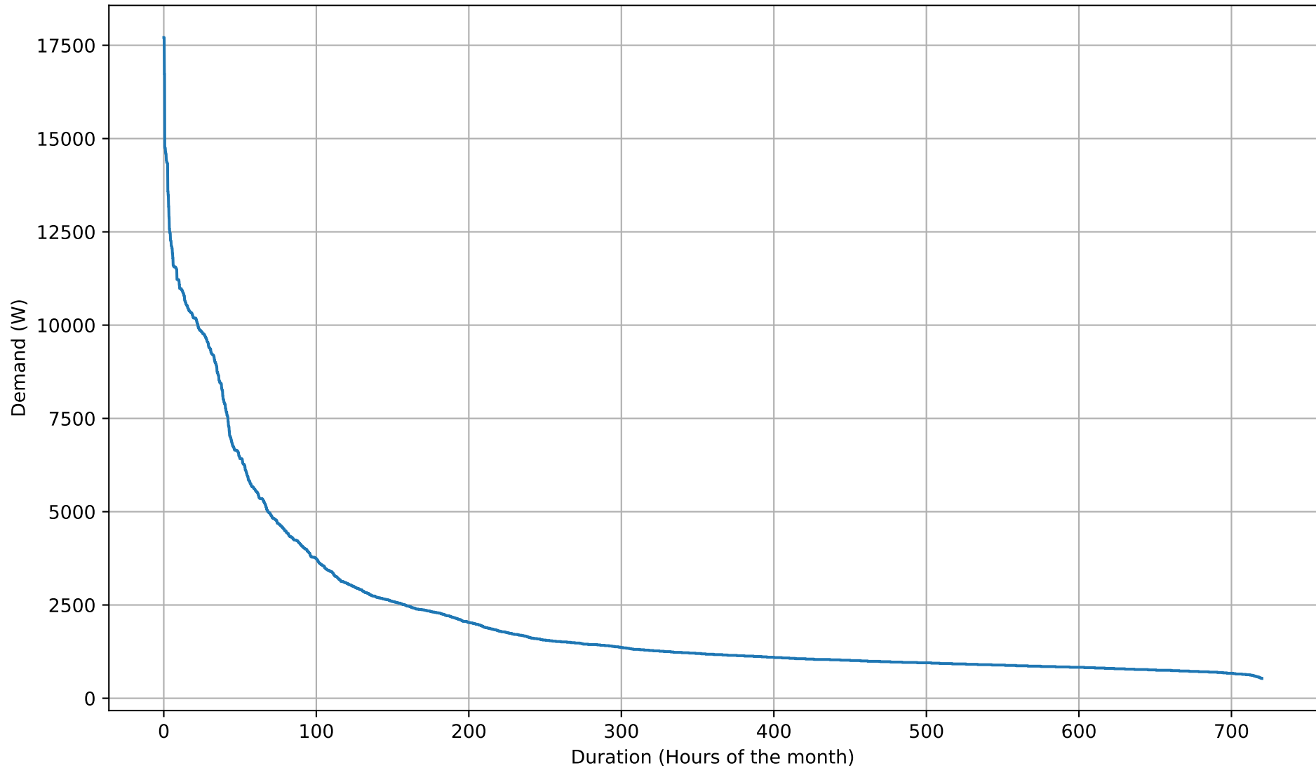
Electricity Demand Duration Curve - NoBattery - Sep
