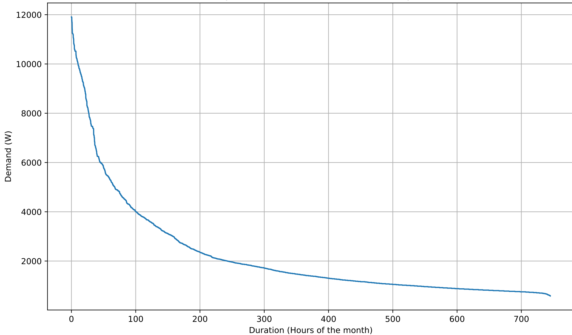
Electricity Demand Duration Curve - NoBattery - Oct
