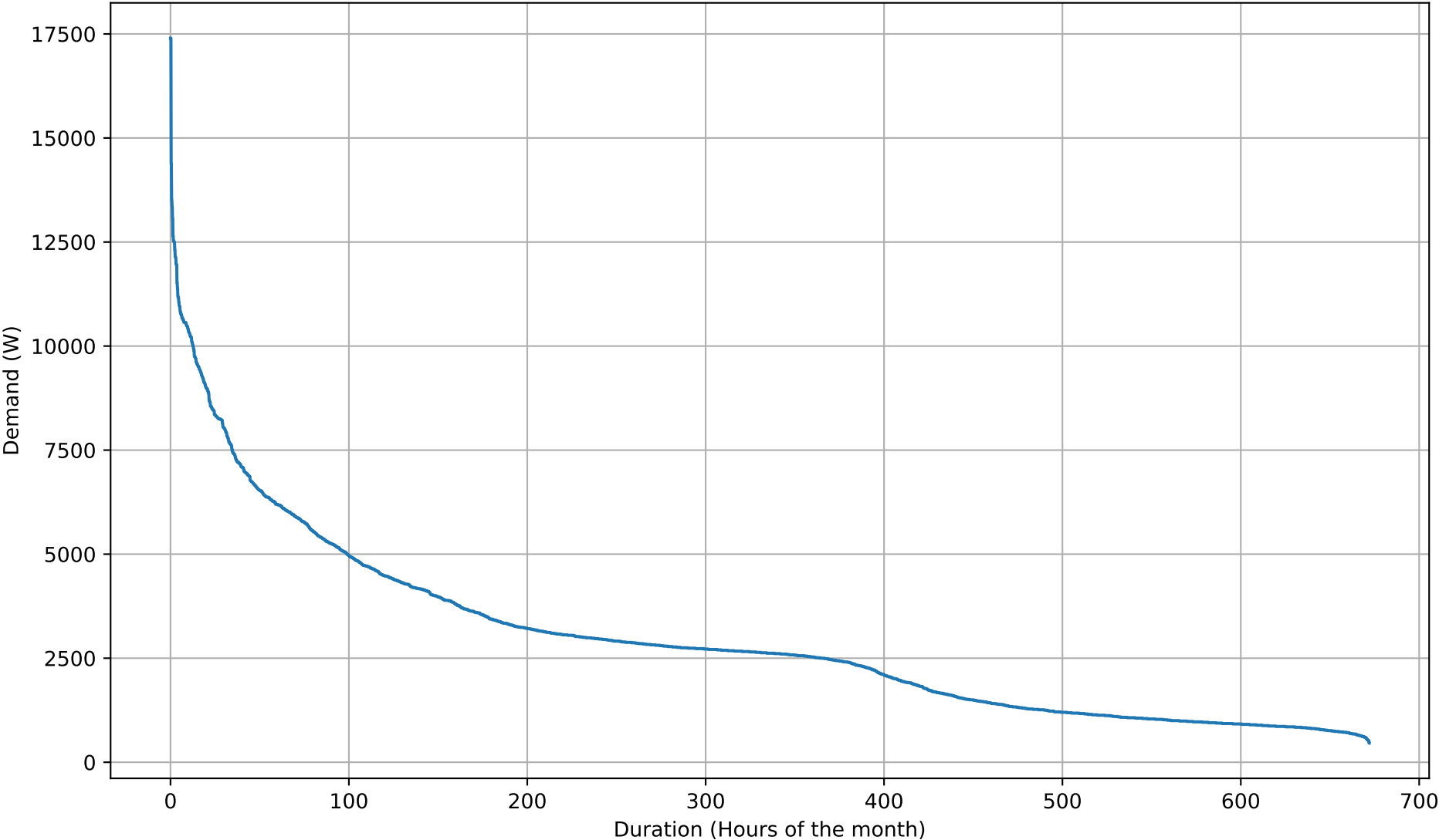
Electricity Demand Duration Curve - NoBattery - Feb
