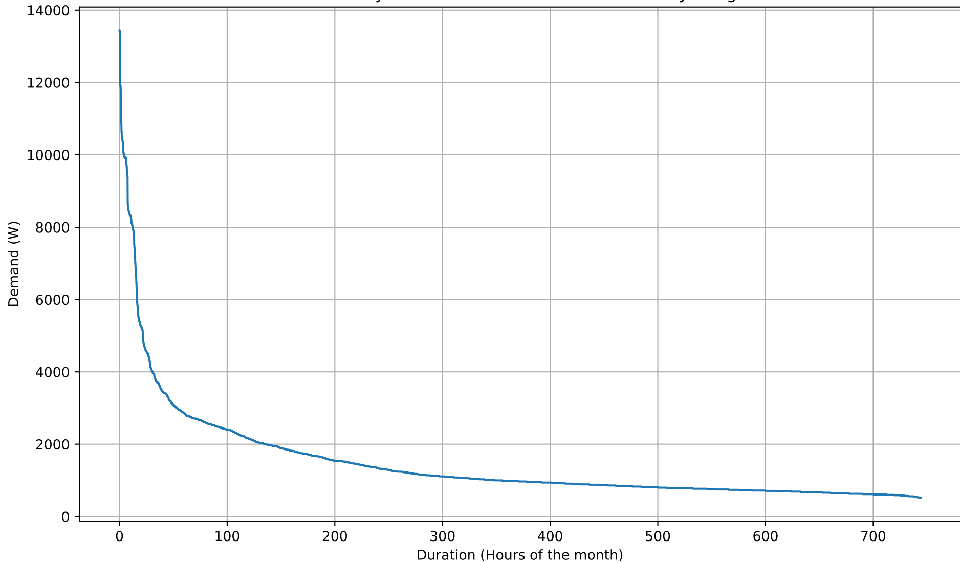
Electricity Demand Duration Curve - NoBattery - Aug
