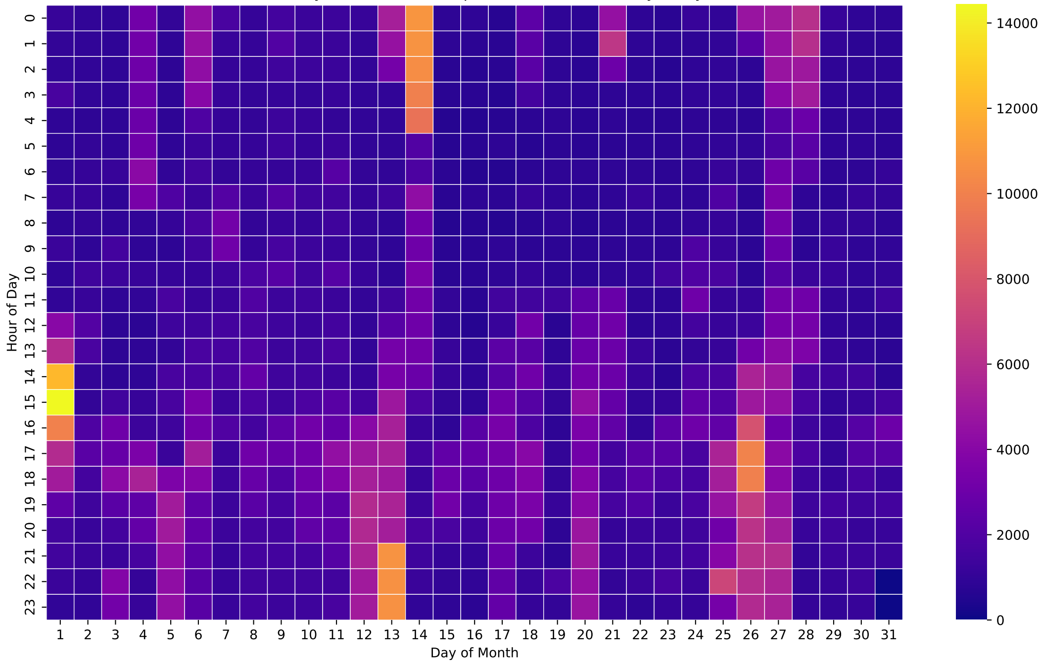
Electricity Demand Heatmap (Wh/Hour) - NoBattery - May
