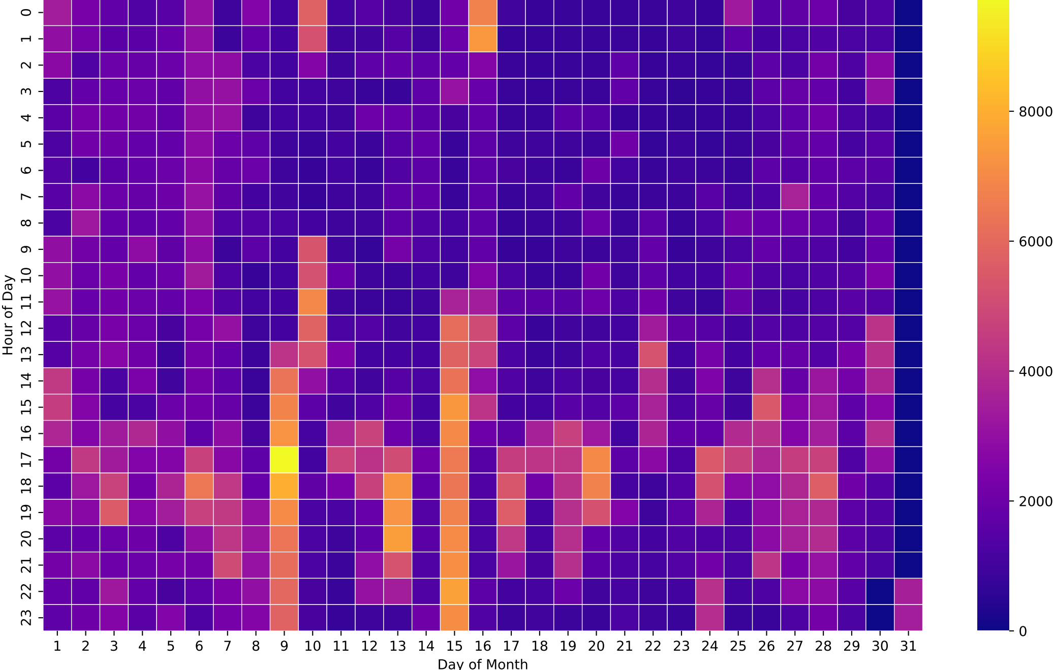
Electricity Demand Heatmap (Wh/Hour) - NoBattery - Apr
