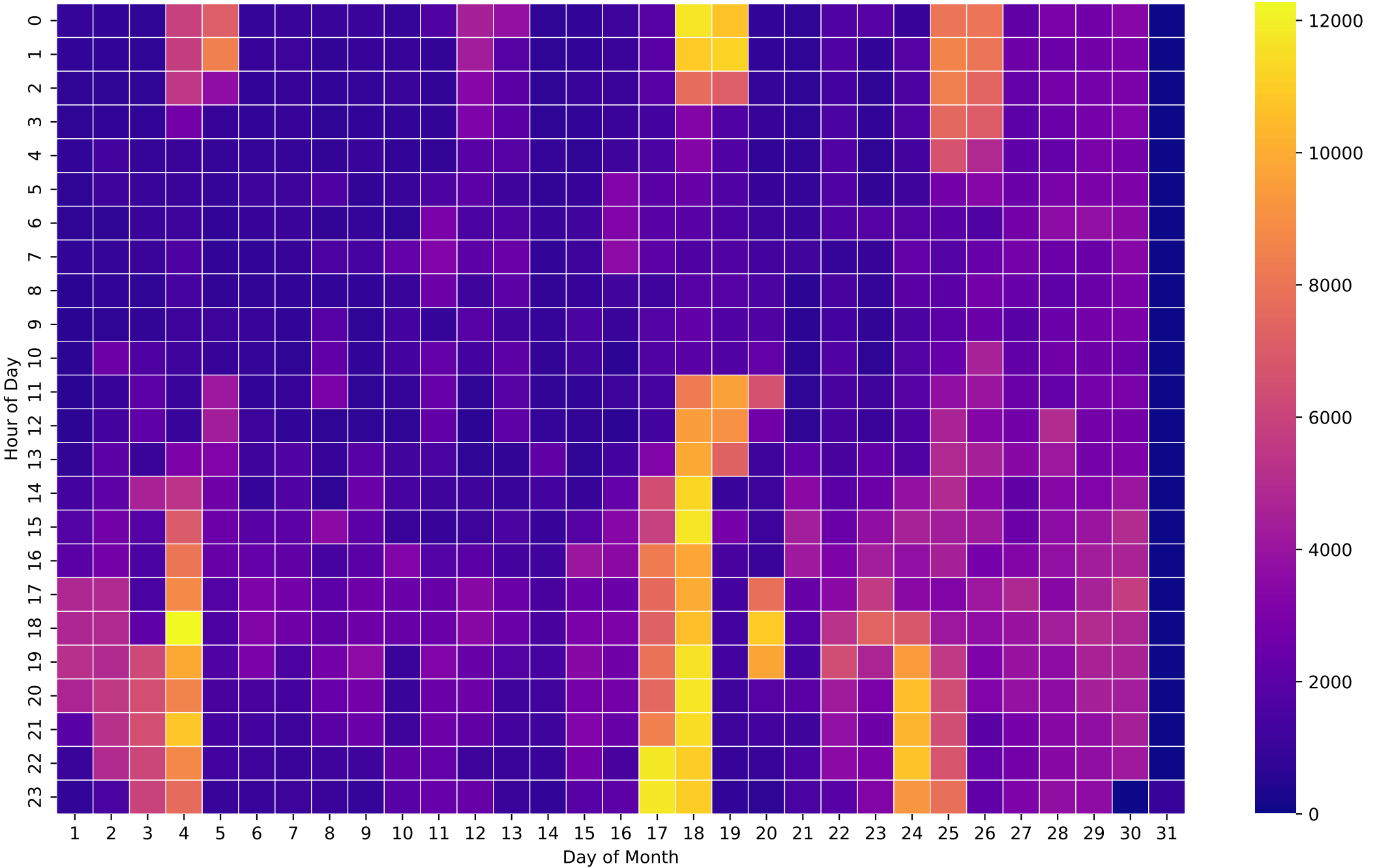
Electricity Demand Heatmap (Wh/Hour) - NoBattery - Nov
