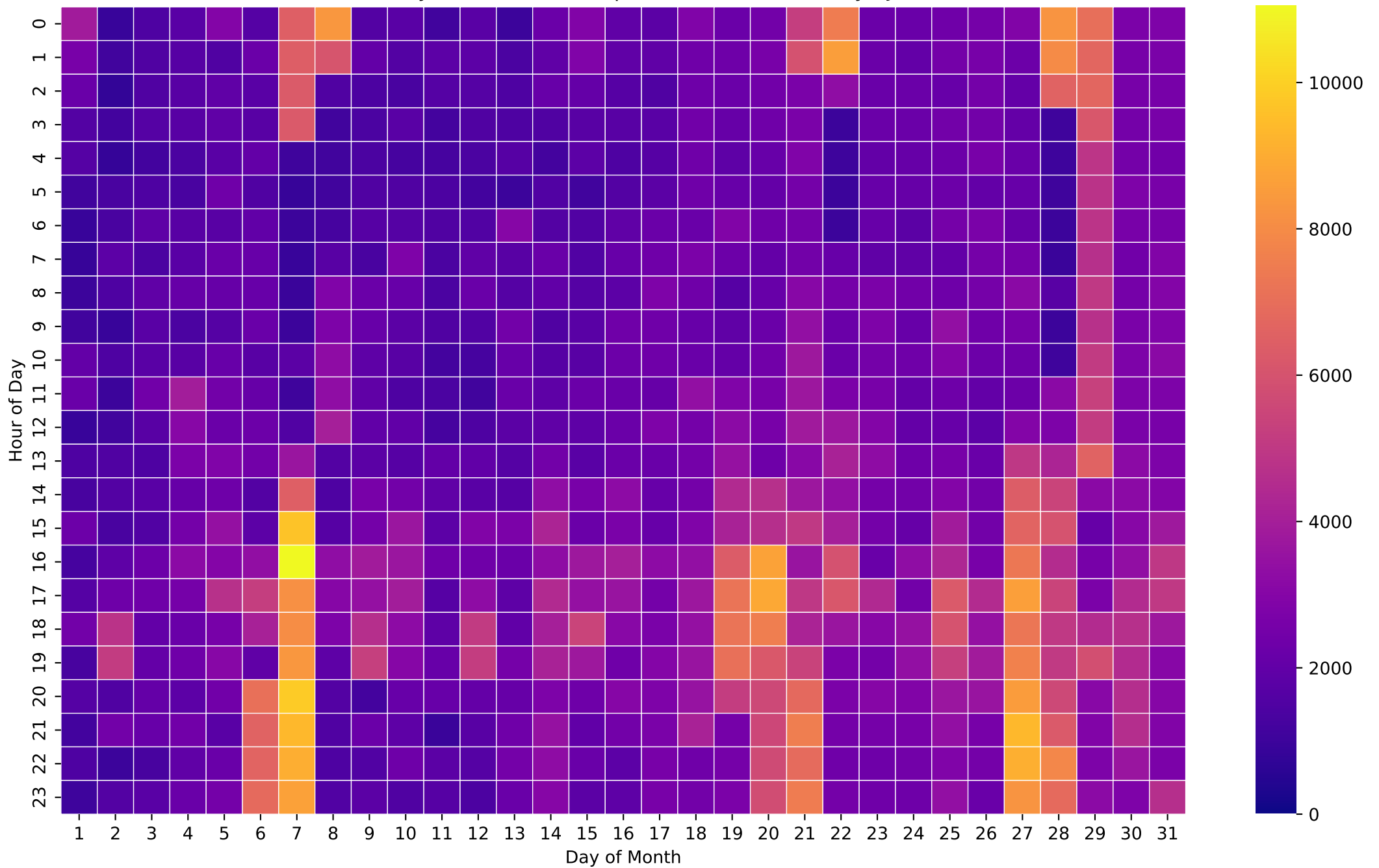
Electricity Demand Heatmap (Wh/Hour) - NoBattery - Jan
