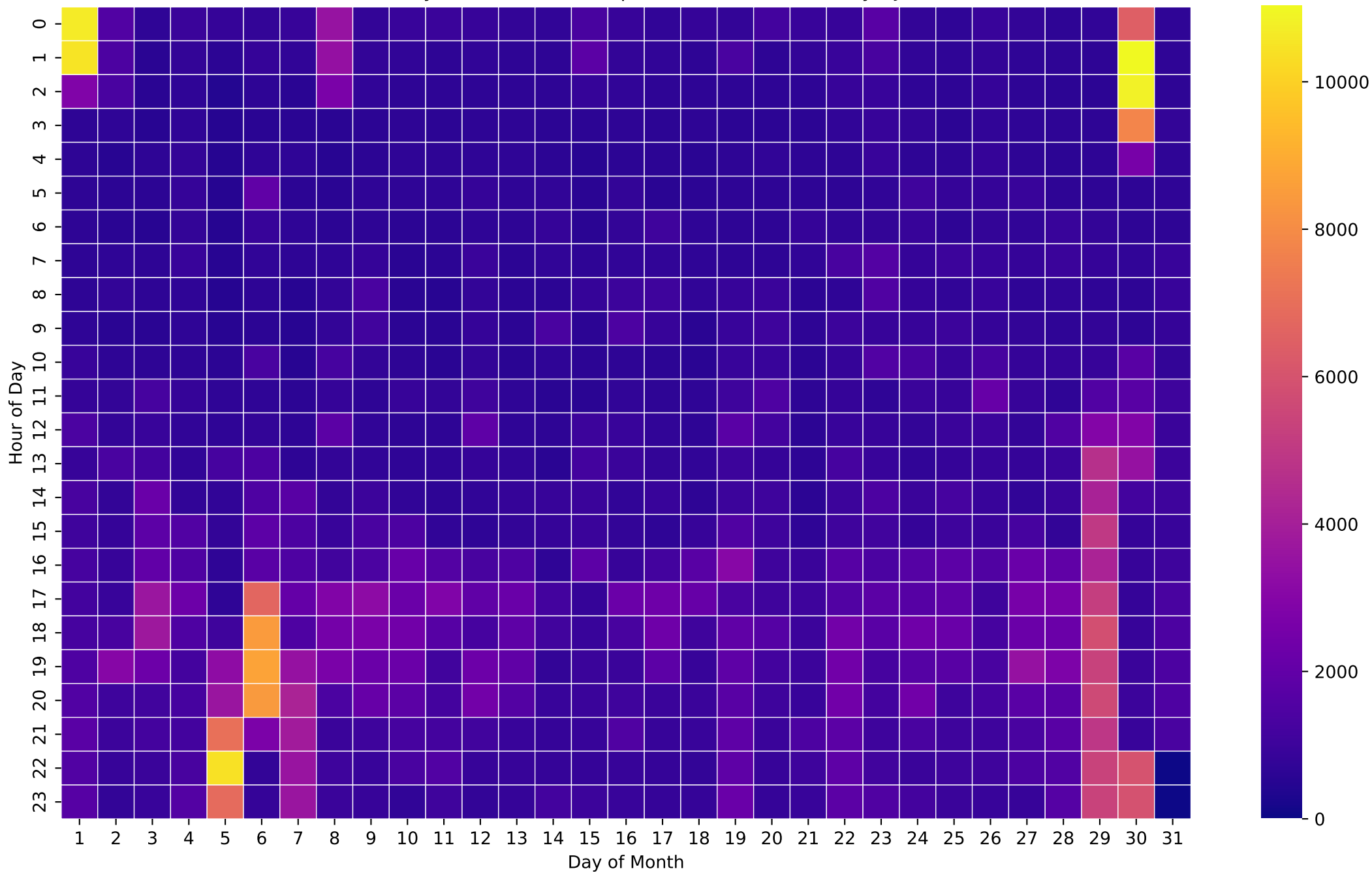
Electricity Demand Heatmap (Wh/Hour) - NoBattery - Jul
