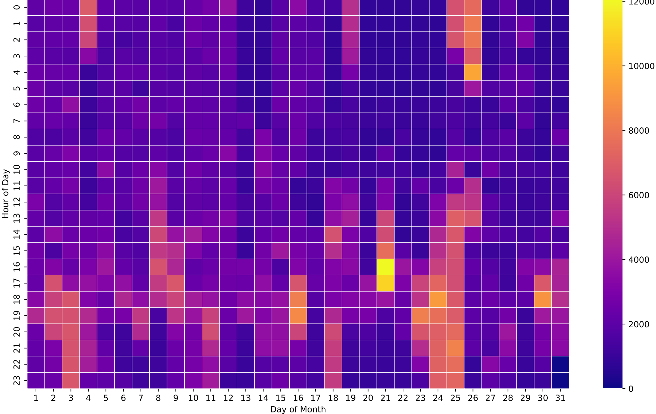
Electricity Demand Heatmap (Wh/Hour) - NoBattery - Mar
