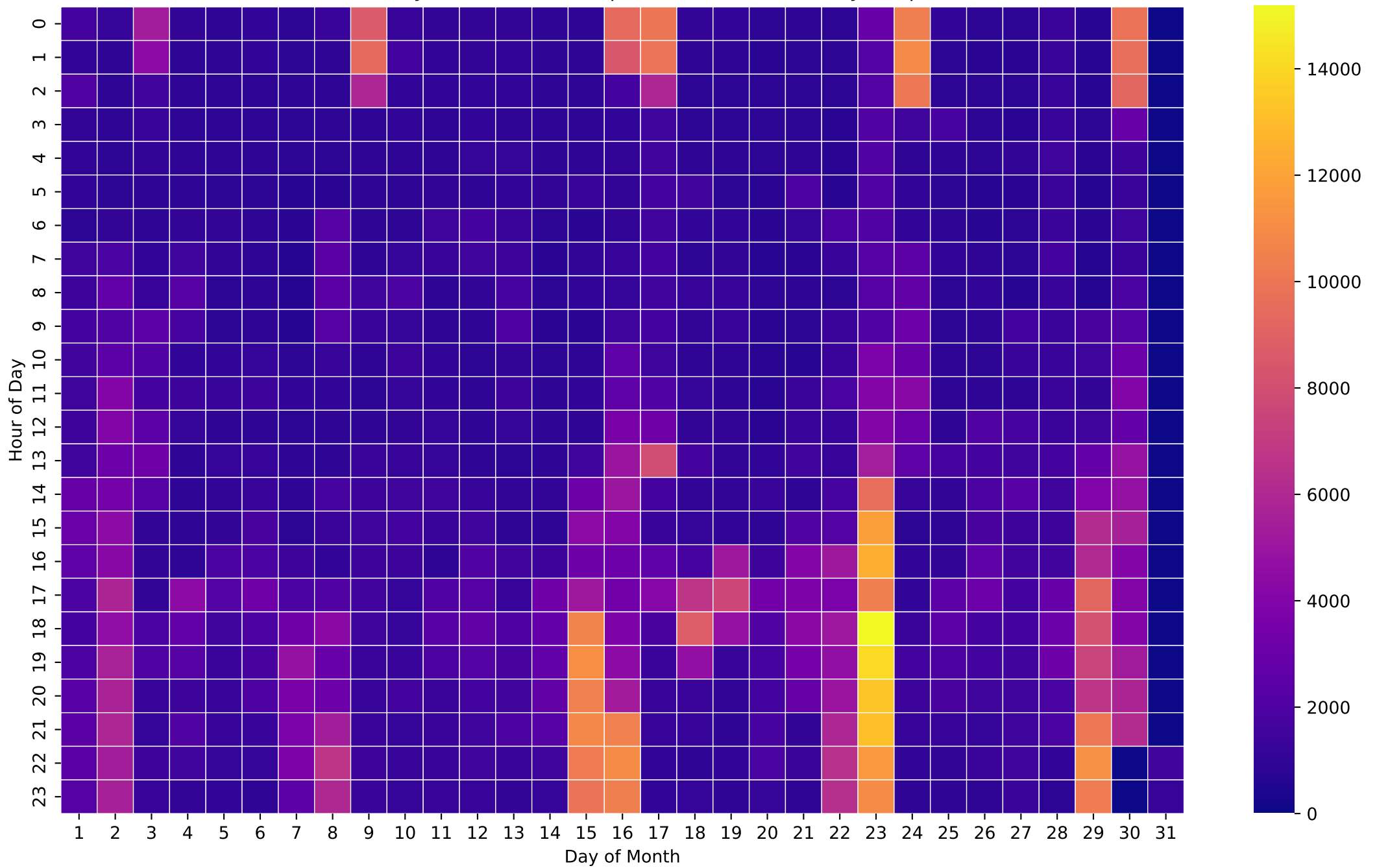
Electricity Demand Heatmap (Wh/Hour) - NoBattery - Sep
