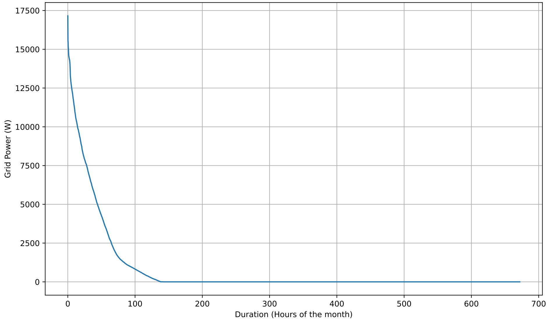
Grid Export Duration Curve - NoBattery - Feb
