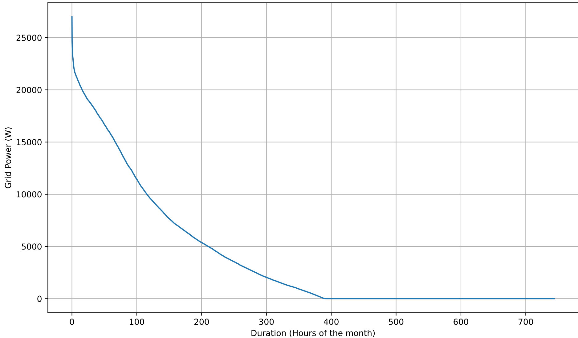
Grid Export Duration Curve - NoBattery - May
