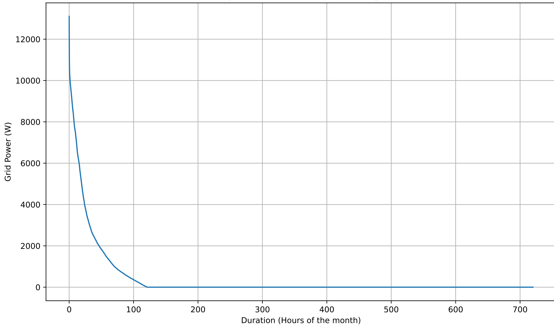
Grid Export Duration Curve - NoBattery - Nov
