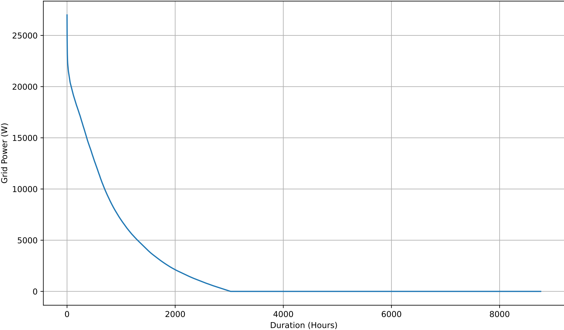
Yearly Grid Export Duration Curve - NoBattery
