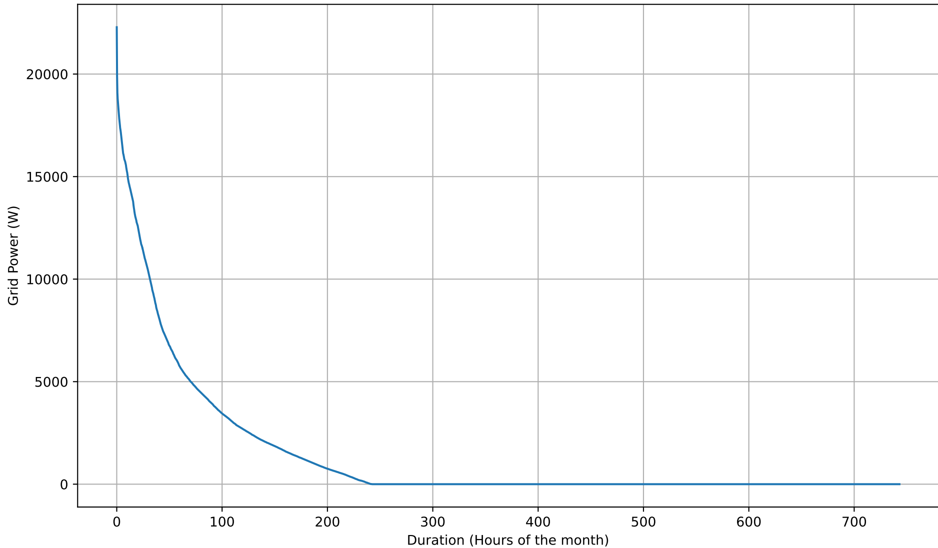
Grid Export Duration Curve - NoBattery - Mar
