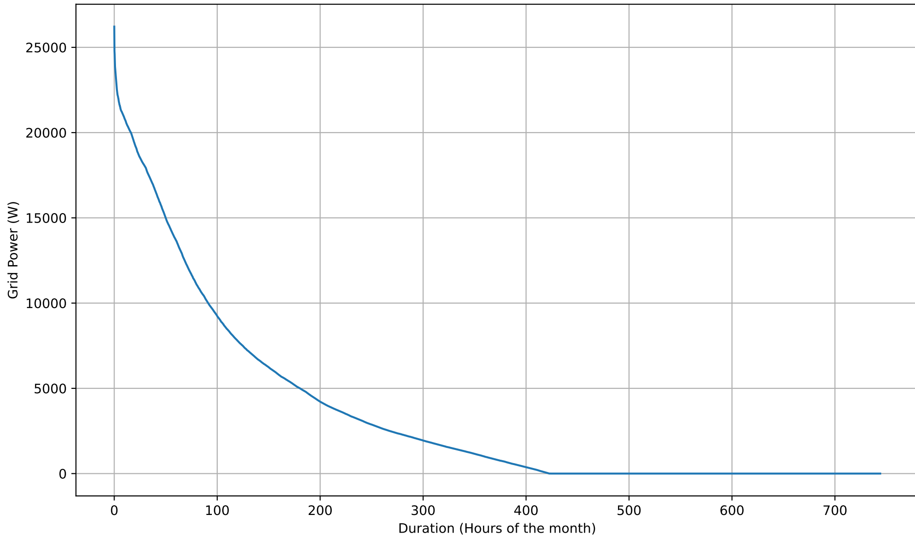
Grid Export Duration Curve - NoBattery - Jul
