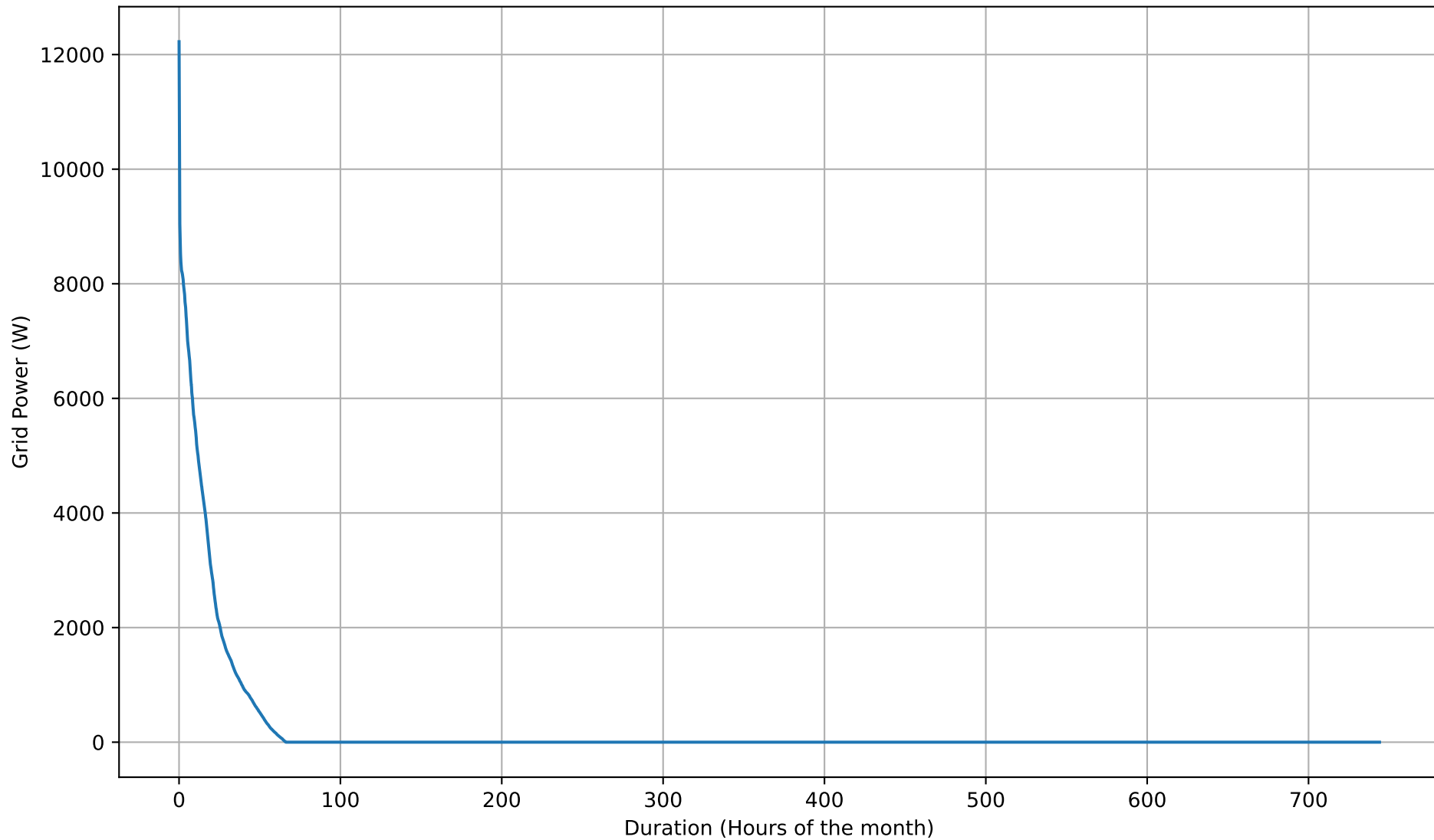
Grid Export Duration Curve - NoBattery - Jan
