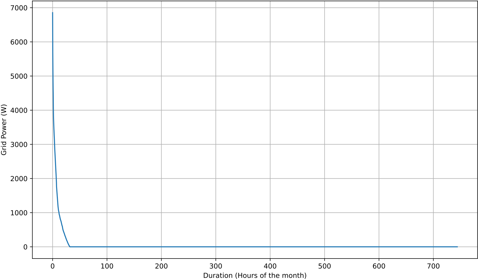
Grid Export Duration Curve - NoBattery - Dec
