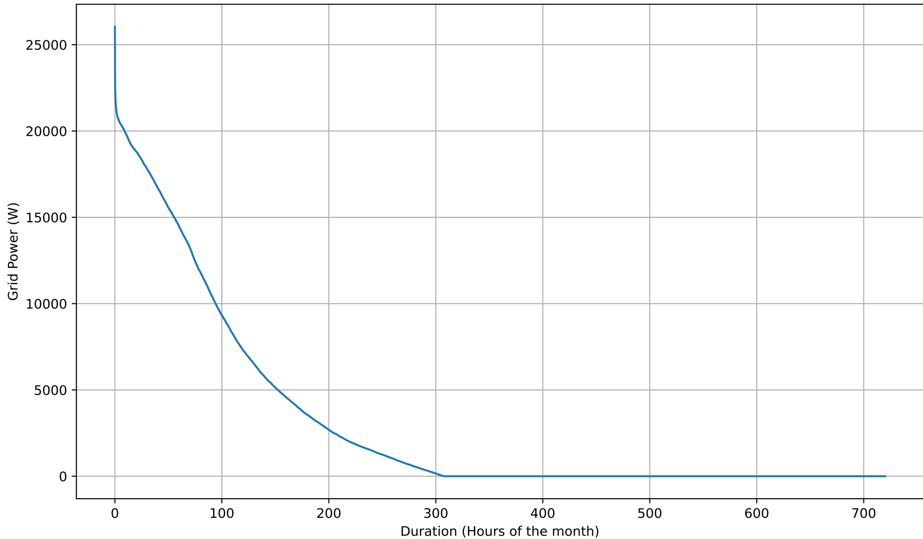
Grid Export Duration Curve - NoBattery - Apr
