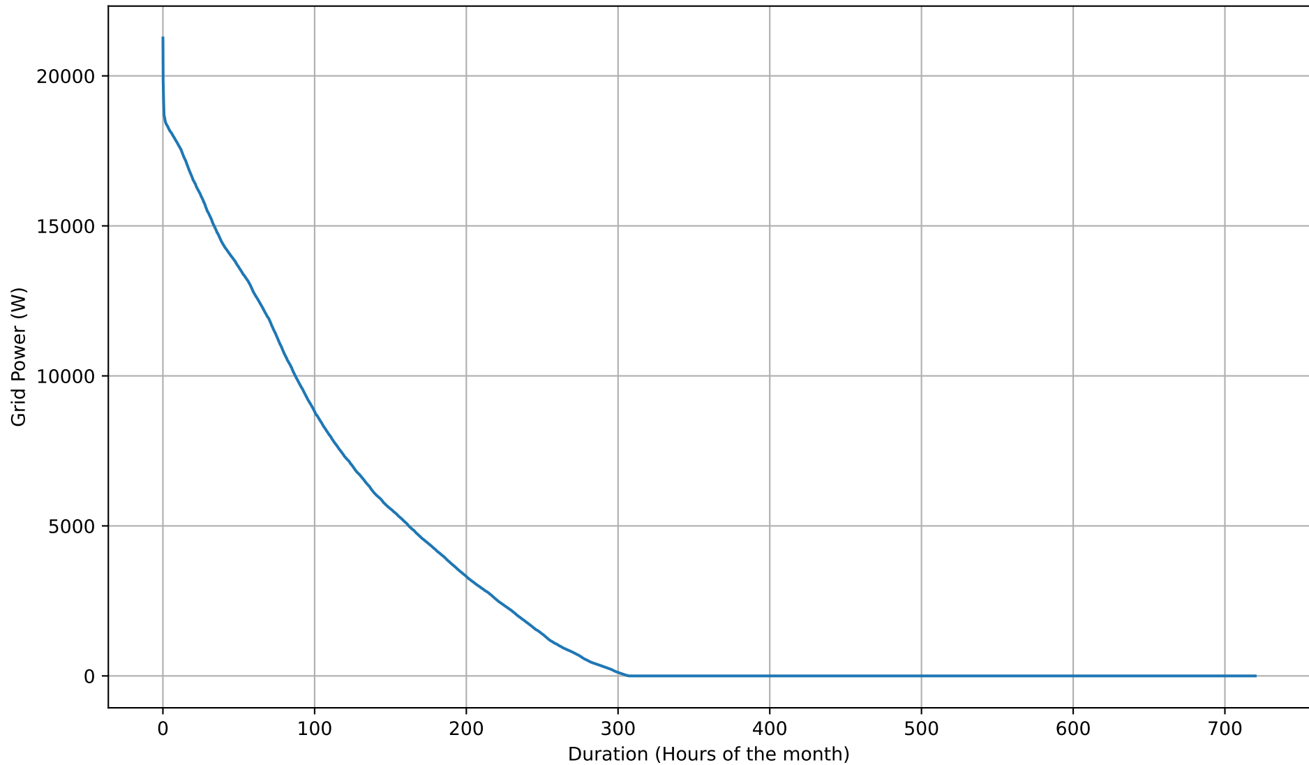
Grid Export Duration Curve - NoBattery - Sep
