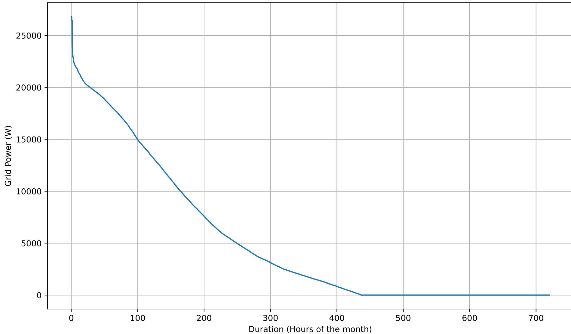
Grid Export Duration Curve - NoBattery - Jun
