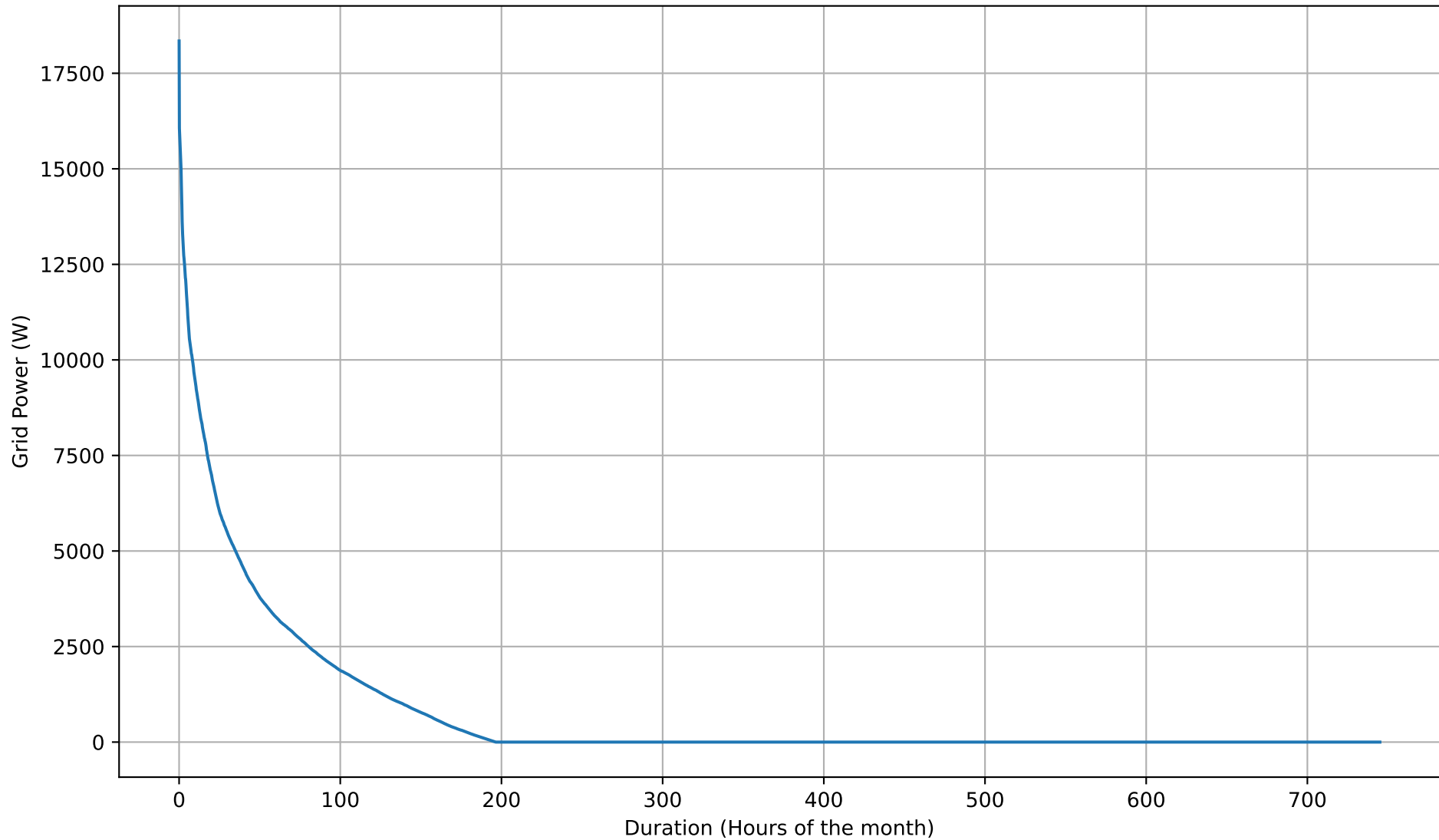
Grid Export Duration Curve - NoBattery - Oct
