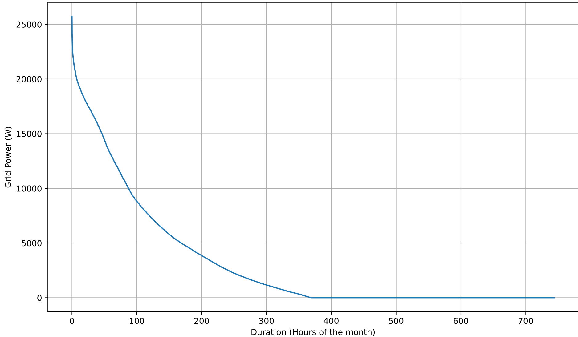
Grid Export Duration Curve - NoBattery - Aug
