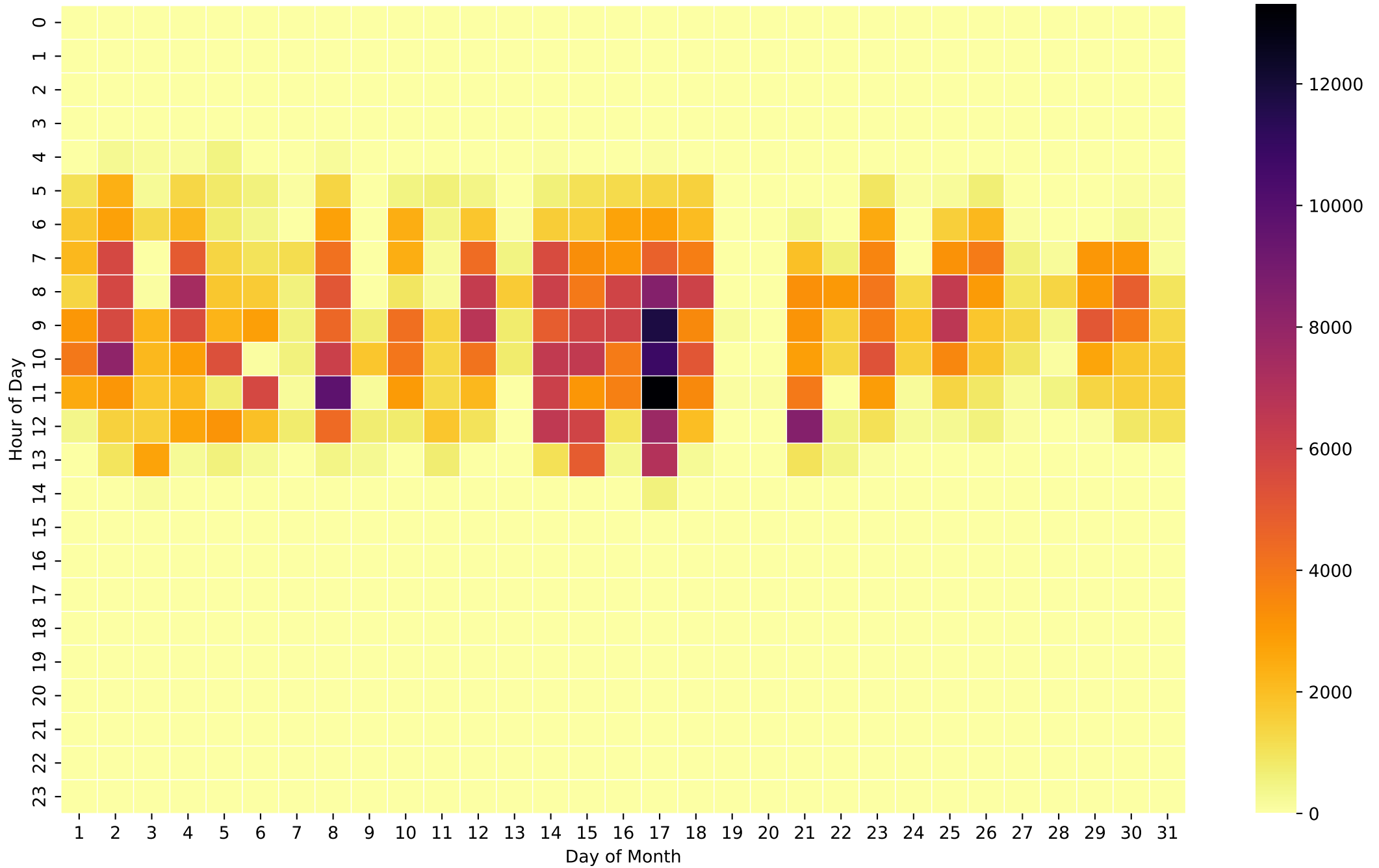
Grid Export Heatmap (Wh/Hour) - NoBattery - Oct
