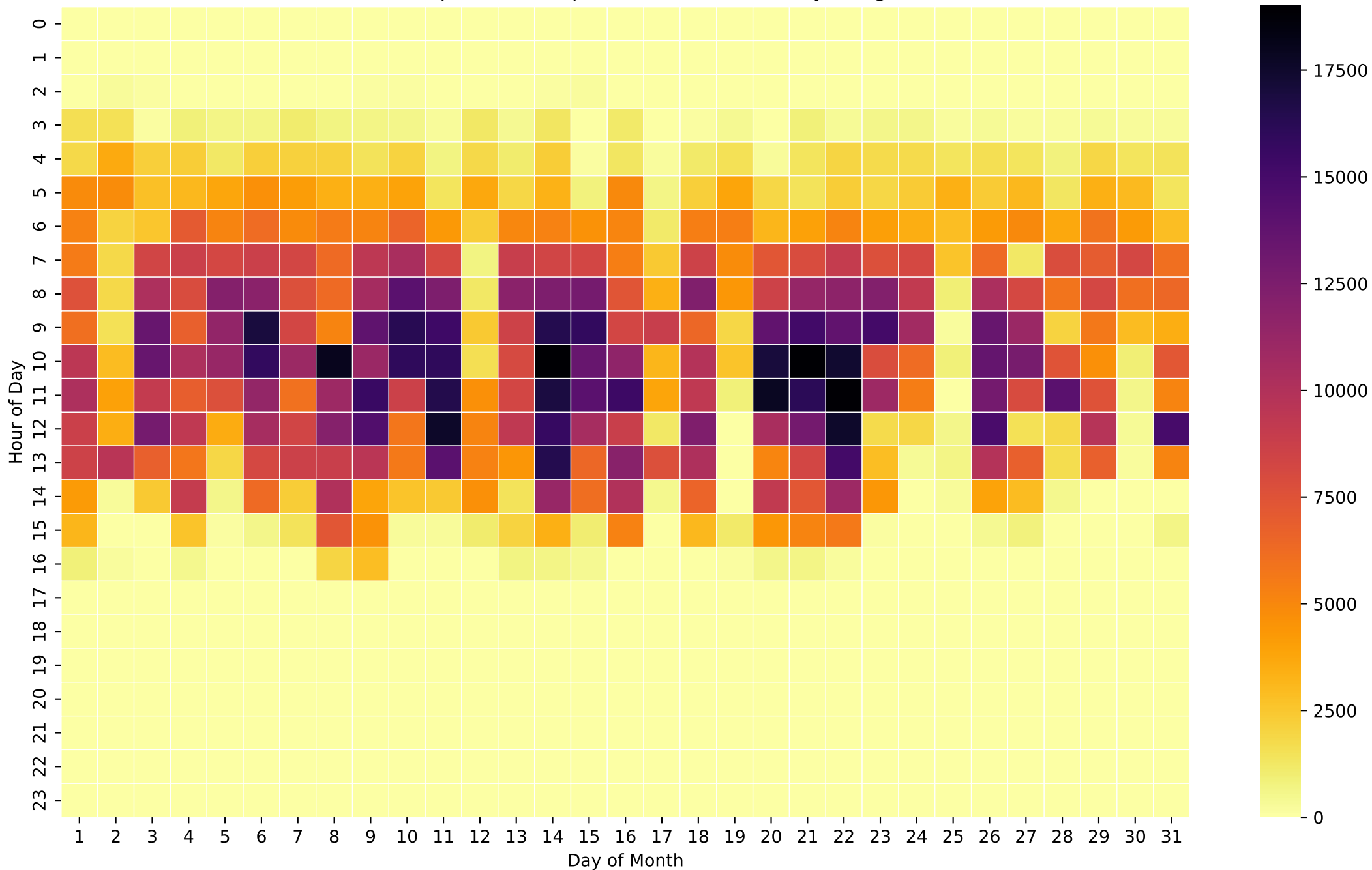
Grid Export Heatmap (Wh/Hour) - NoBattery - Aug
