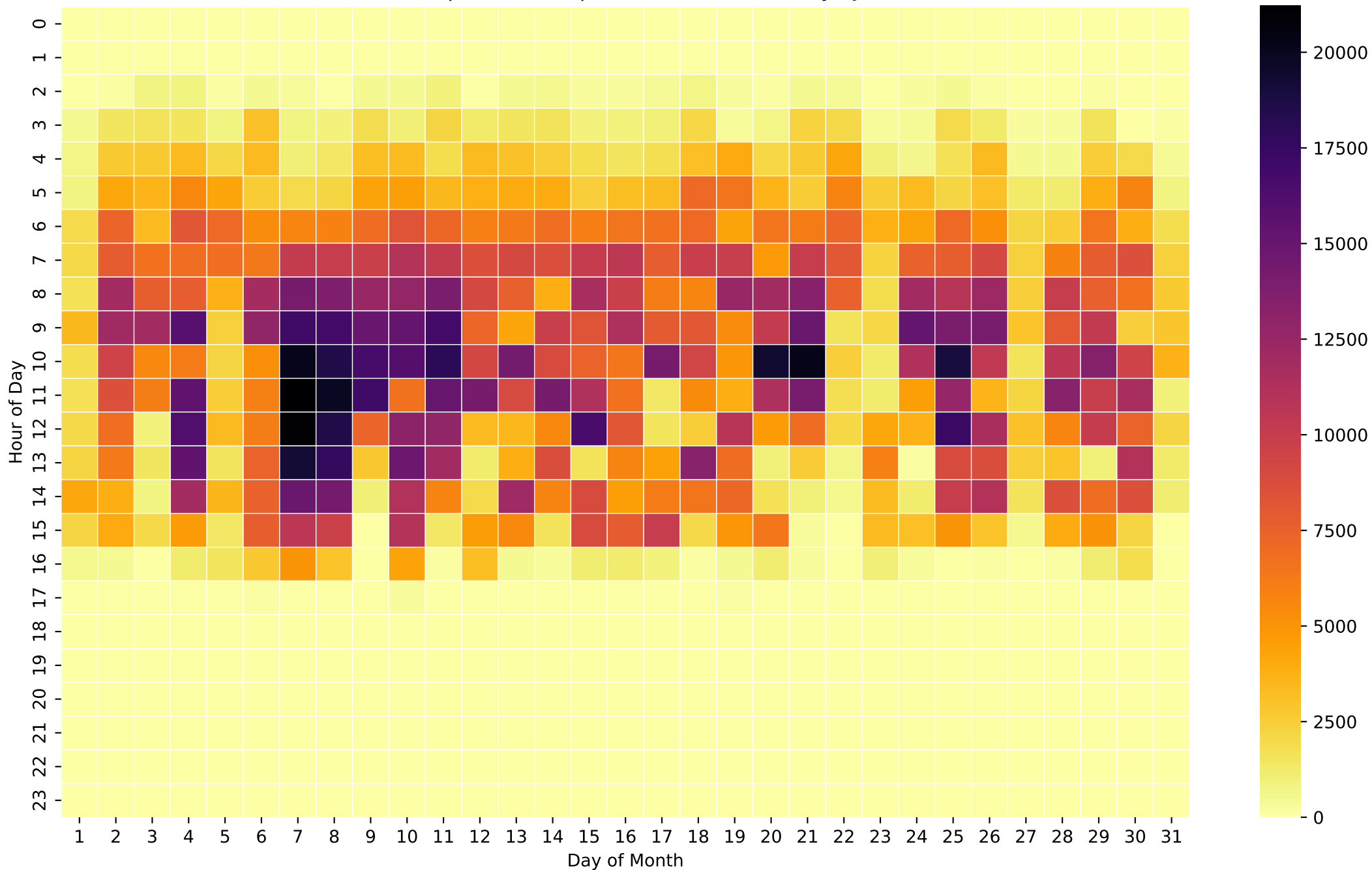
Grid Export Heatmap (Wh/Hour) - NoBattery - Jul
