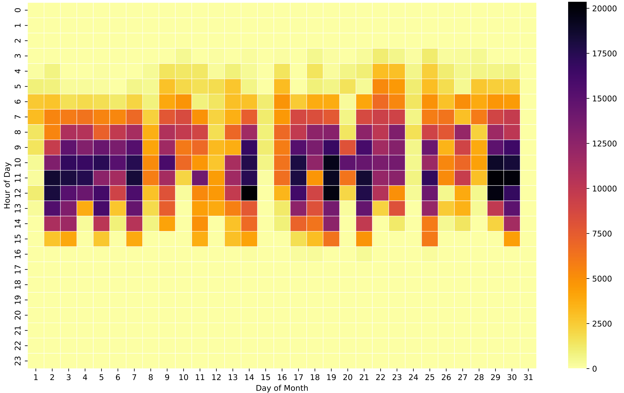
Grid Export Heatmap (Wh/Hour) - NoBattery - Apr
