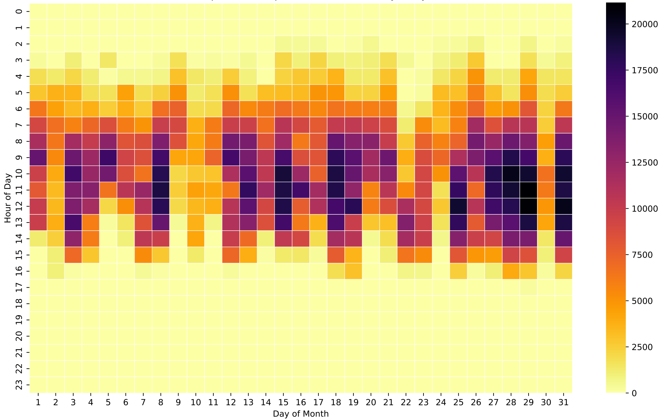
Grid Export Heatmap (Wh/Hour) - NoBattery - May
