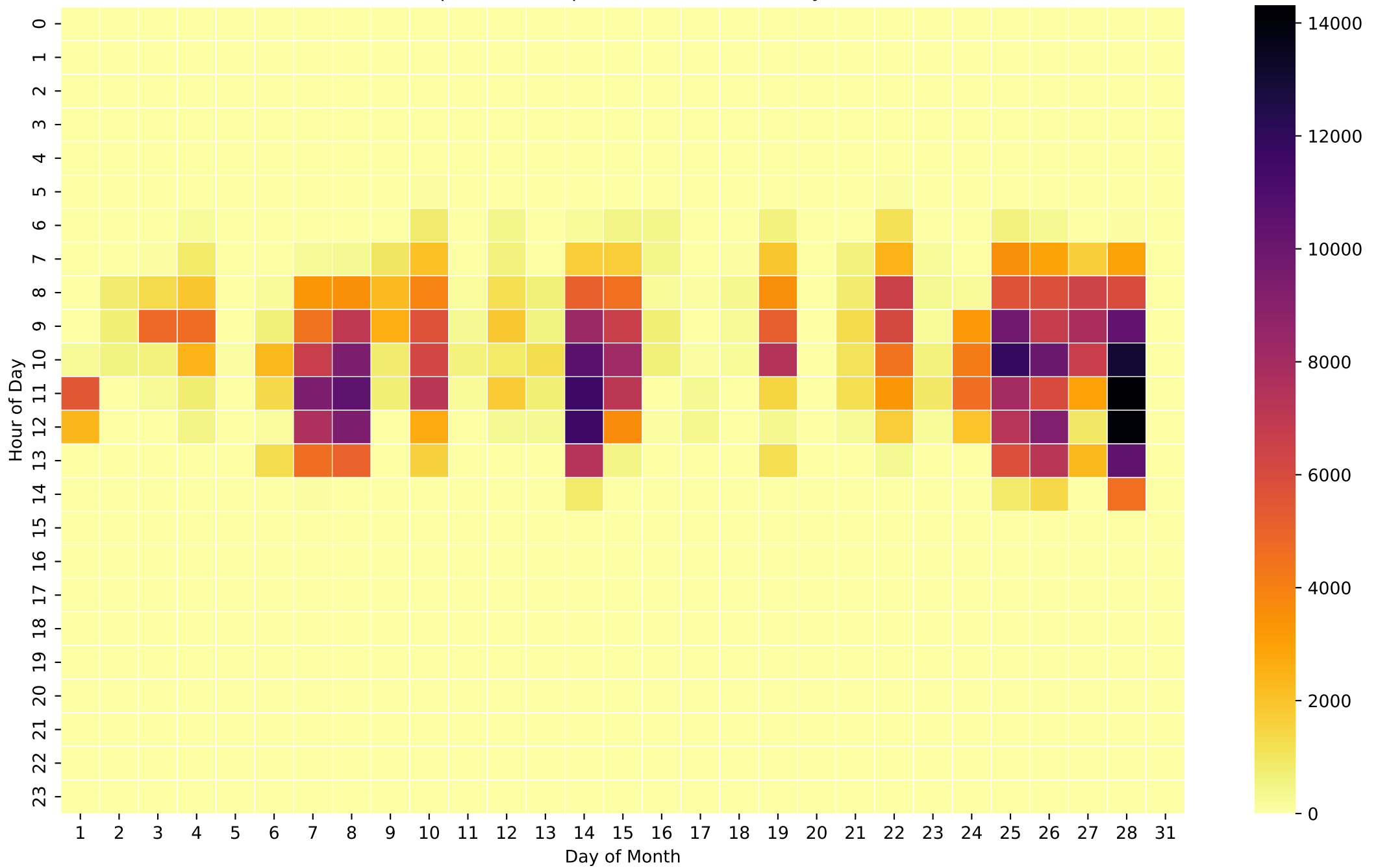
Grid Export Heatmap (Wh/Hour) - NoBattery - Feb
