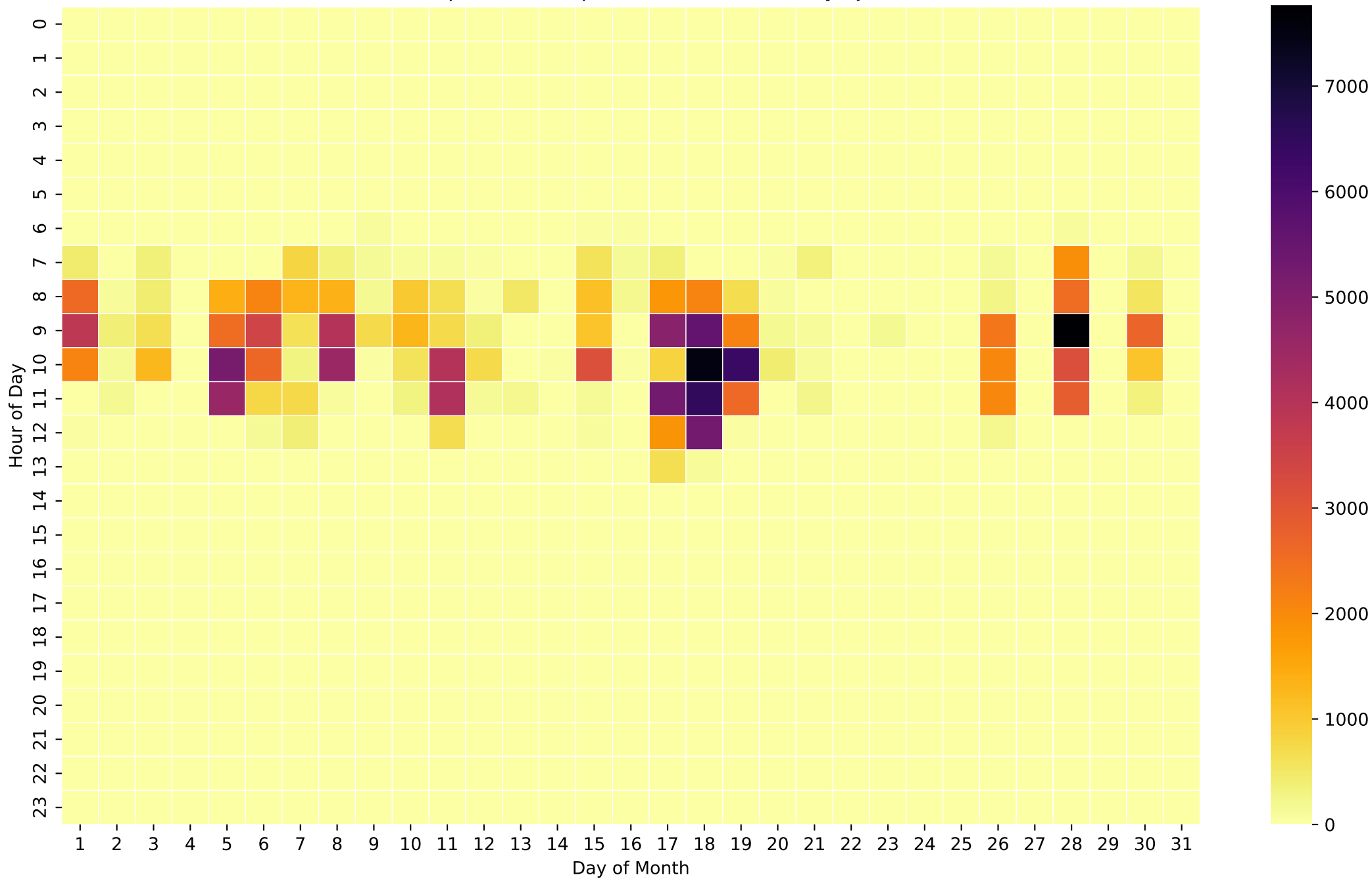
Grid Export Heatmap (Wh/Hour) - NoBattery - Jan
