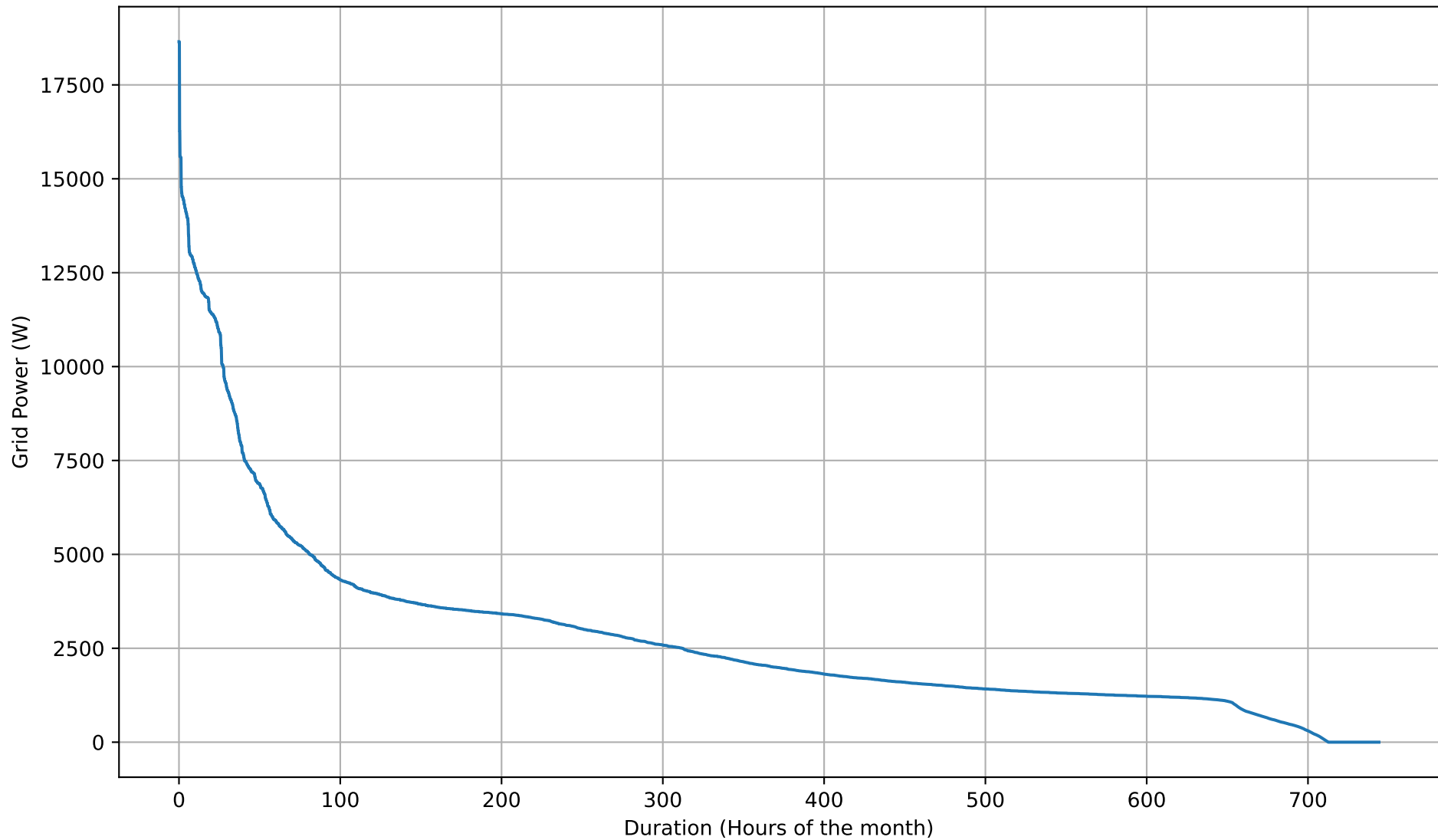
Grid Import Duration Curve - NoBattery - Dec
