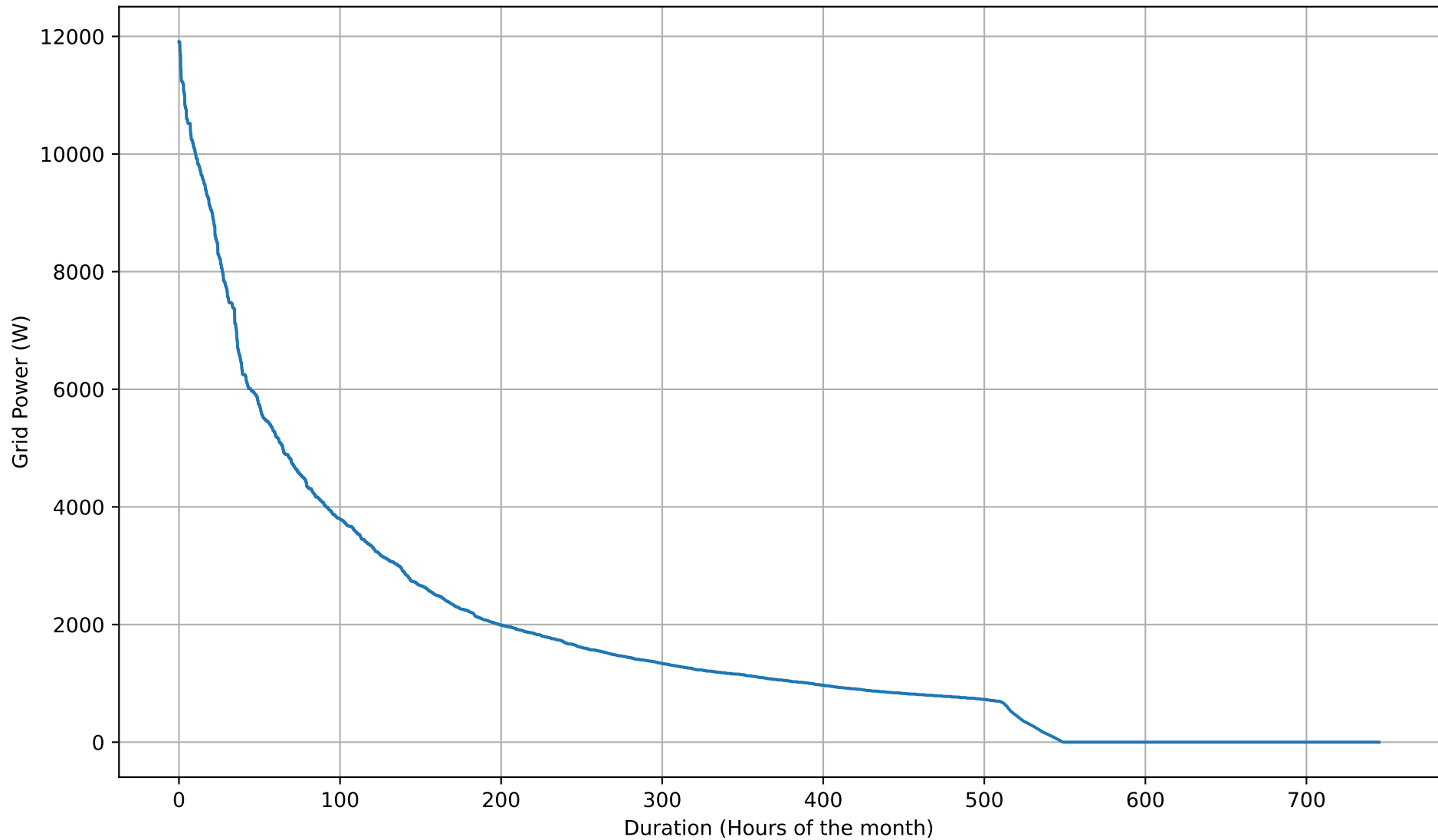
Grid Import Duration Curve - NoBattery - Oct
