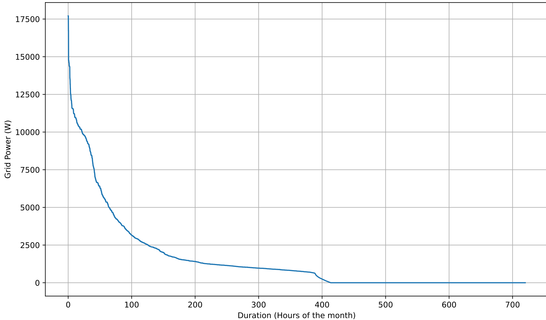
Grid Import Duration Curve - NoBattery - Sep
