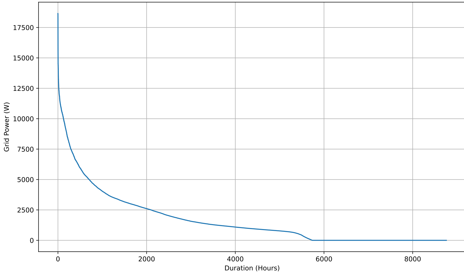
Yearly Grid Import Duration Curve - NoBattery
