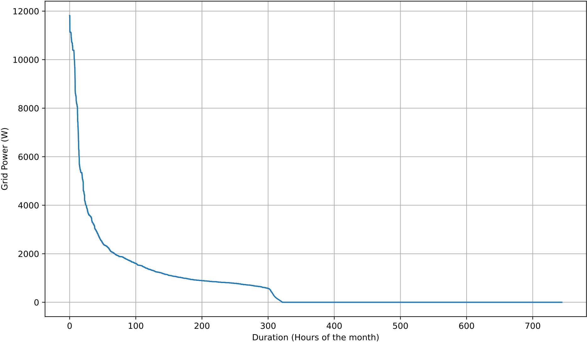
Grid Import Duration Curve - NoBattery - Jul
