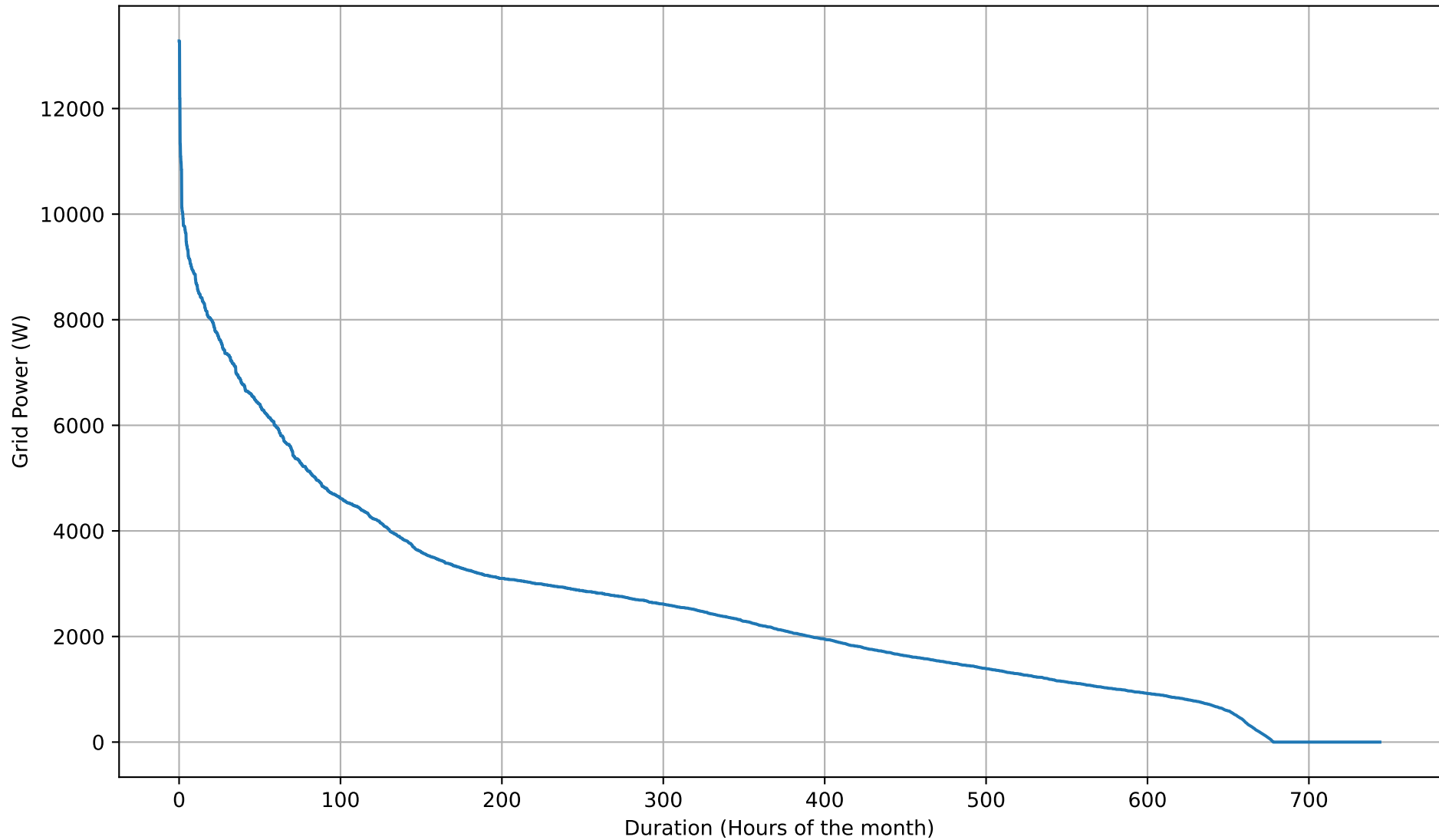
Grid Import Duration Curve - NoBattery - Jan
