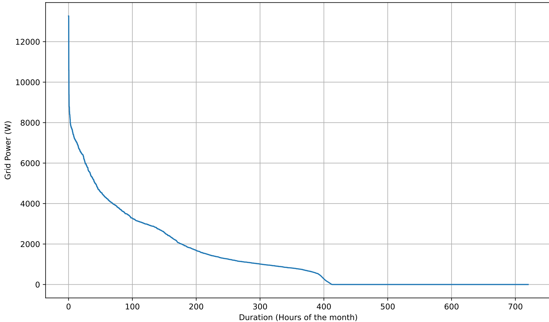
Grid Import Duration Curve - NoBattery - Apr
