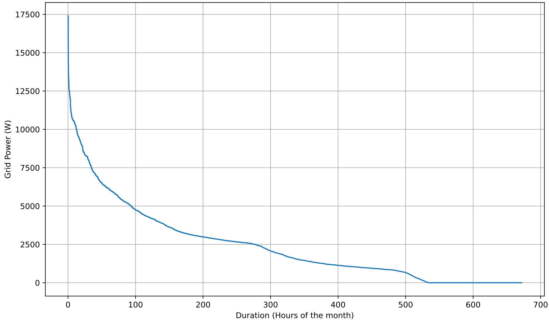
Grid Import Duration Curve - NoBattery - Feb
