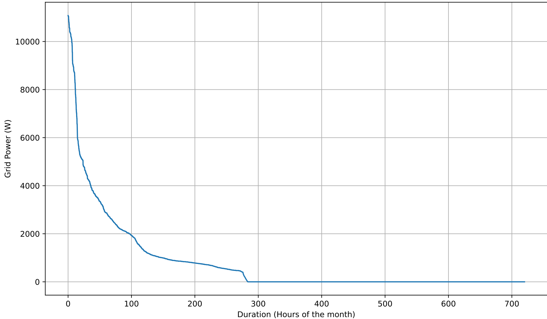
Grid Import Duration Curve - NoBattery - Jun
