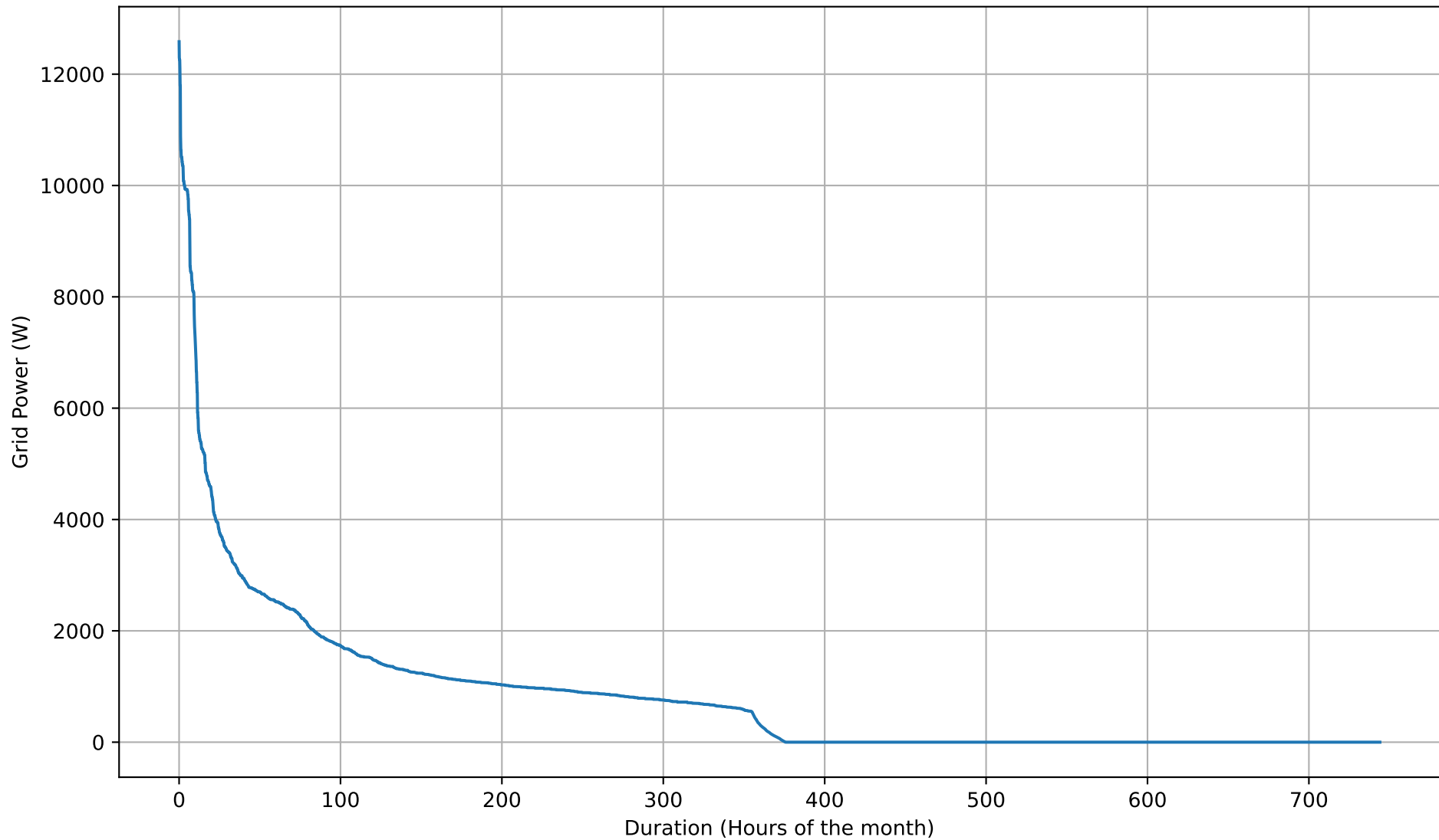
Grid Import Duration Curve - NoBattery - Aug
