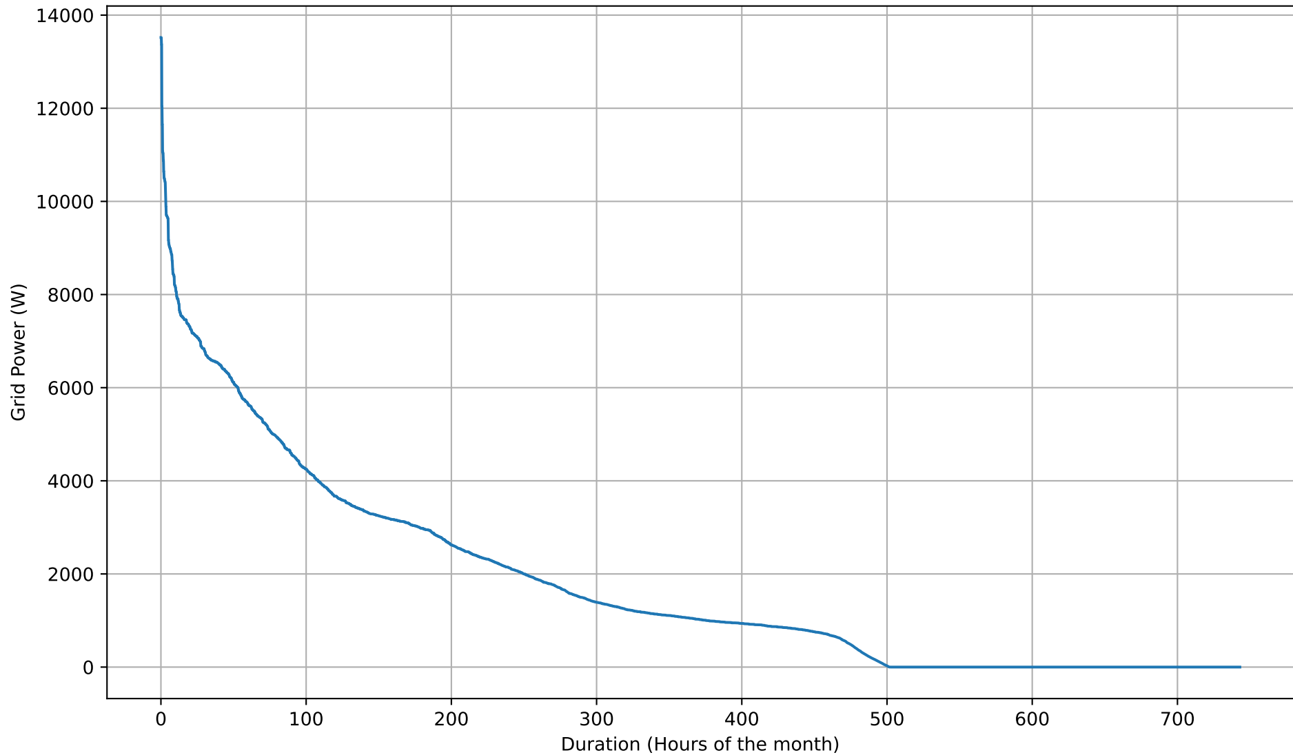
Grid Import Duration Curve - NoBattery - Mar
