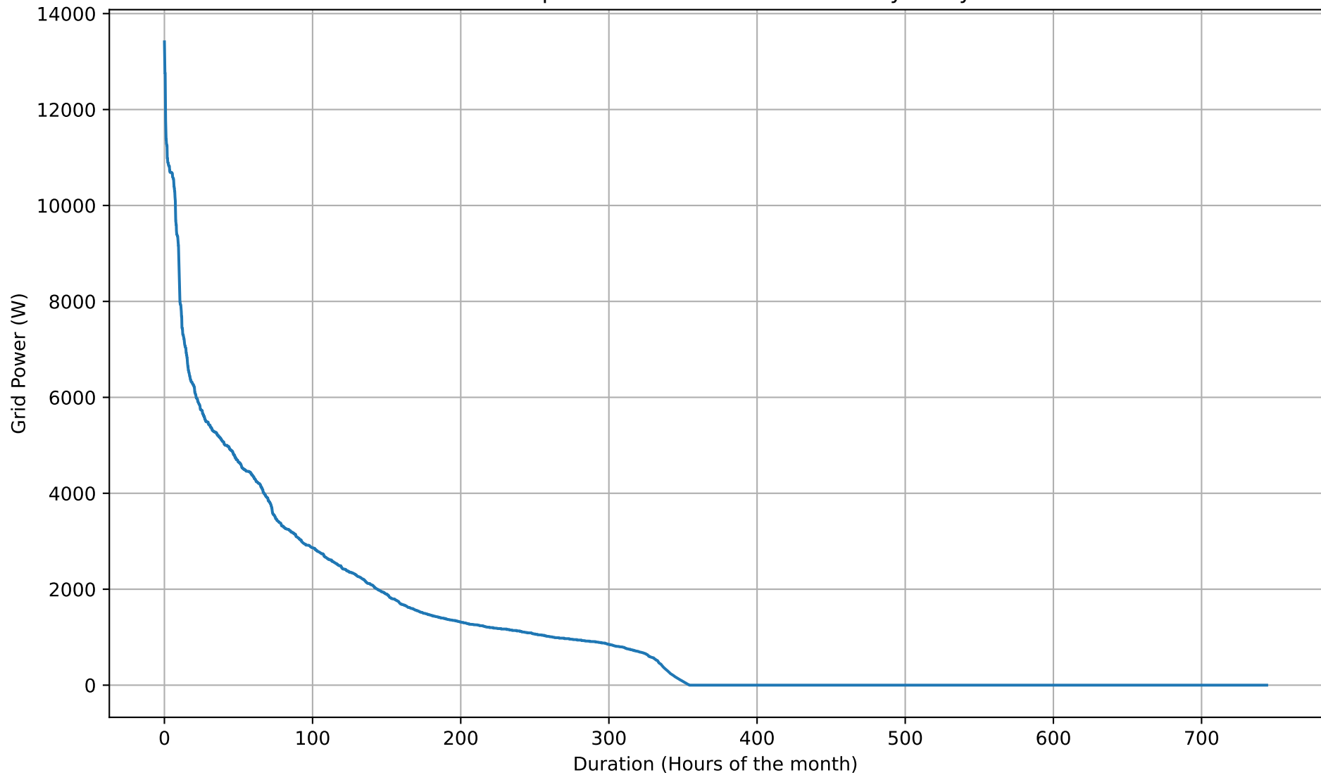
Grid Import Duration Curve - NoBattery - May
