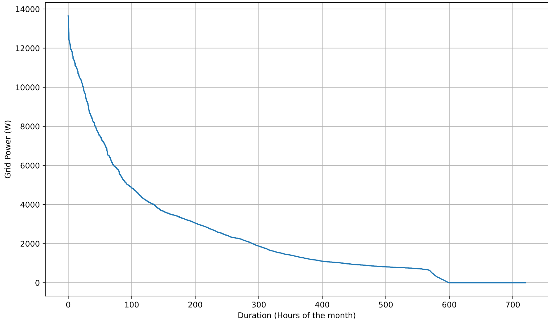
Grid Import Duration Curve - NoBattery - Nov
