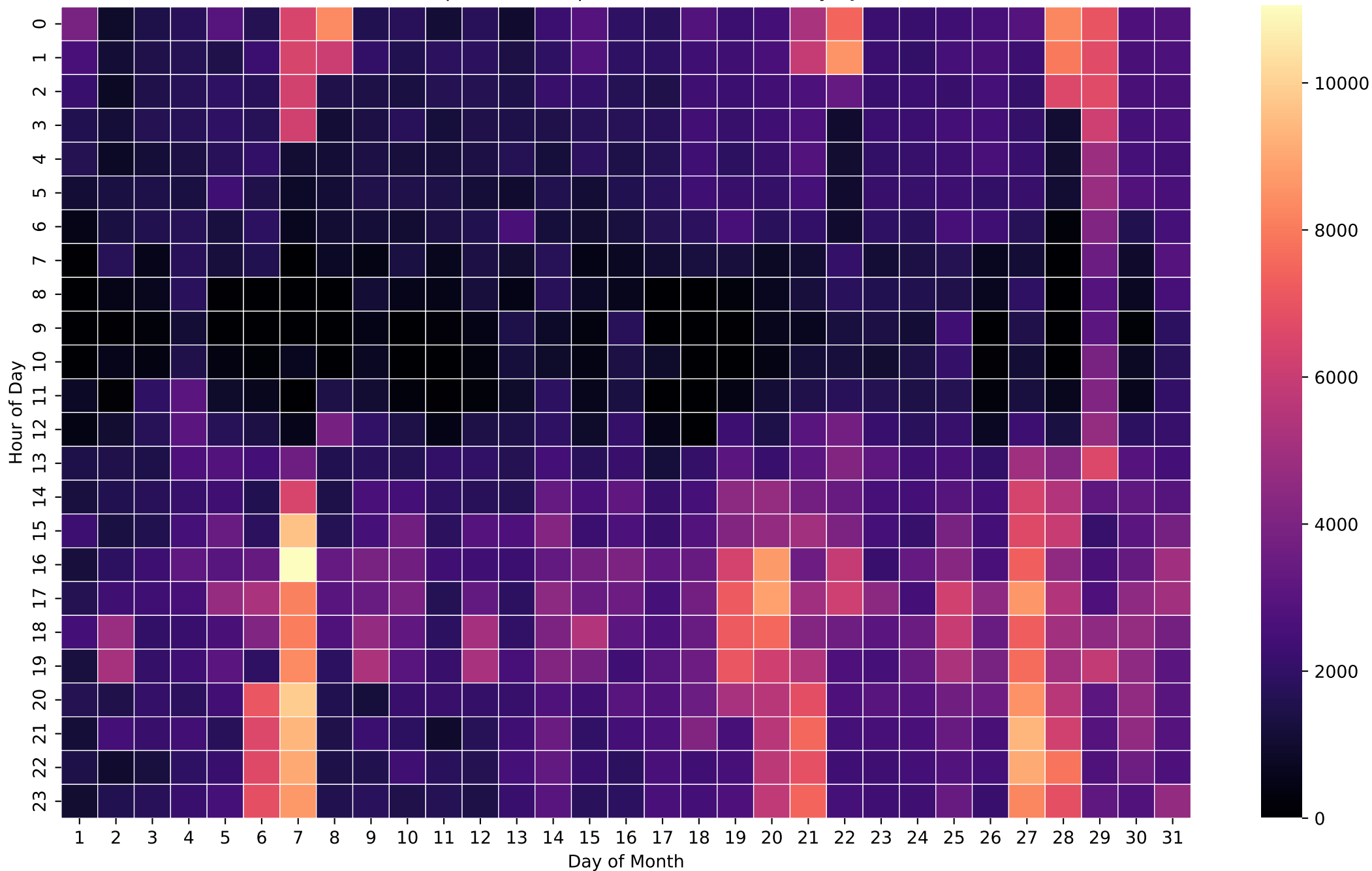
Grid Import Heatmap (Wh/Hour) - NoBattery - Jan
