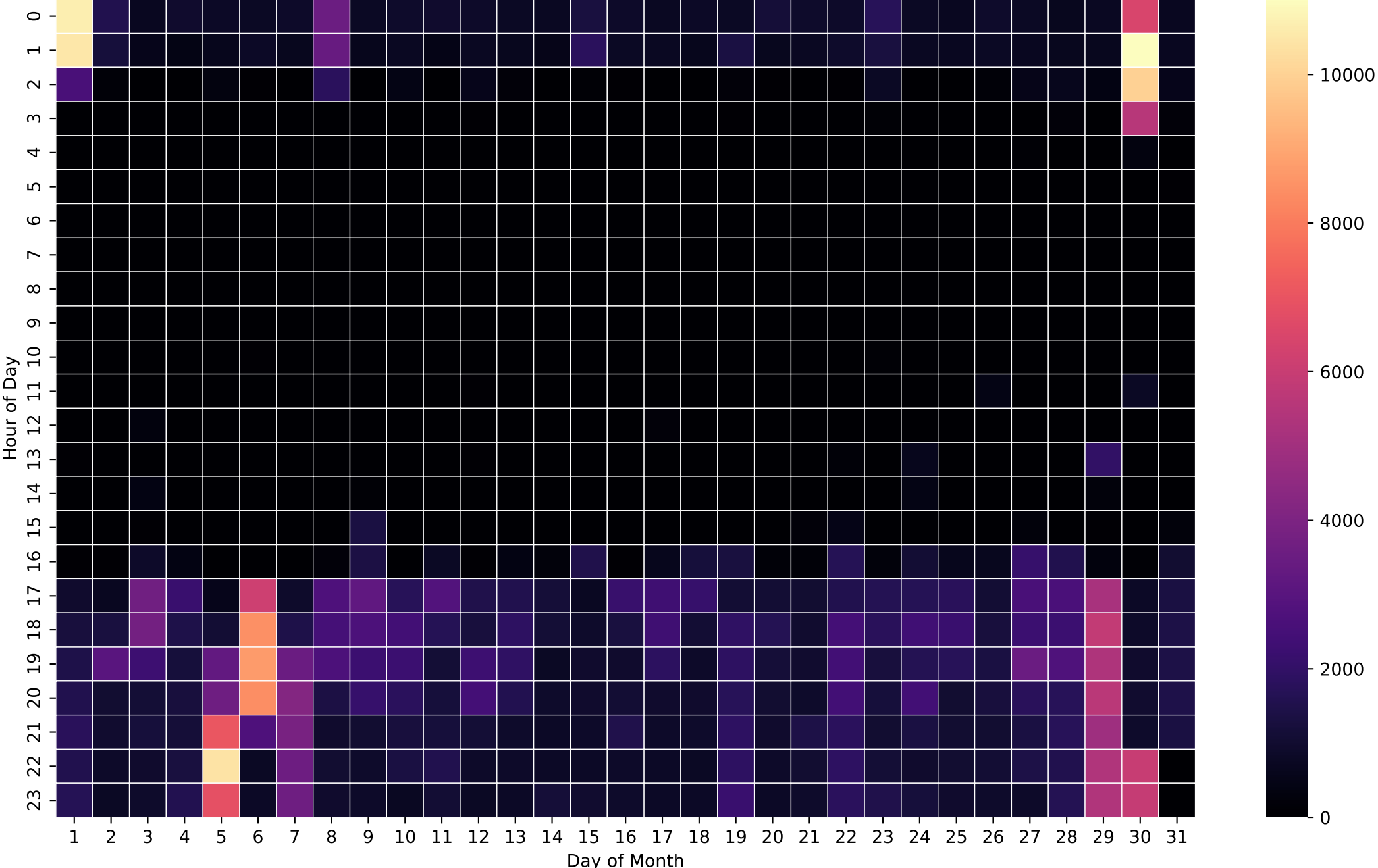
Grid Import Heatmap (Wh/Hour) - NoBattery - Jul
