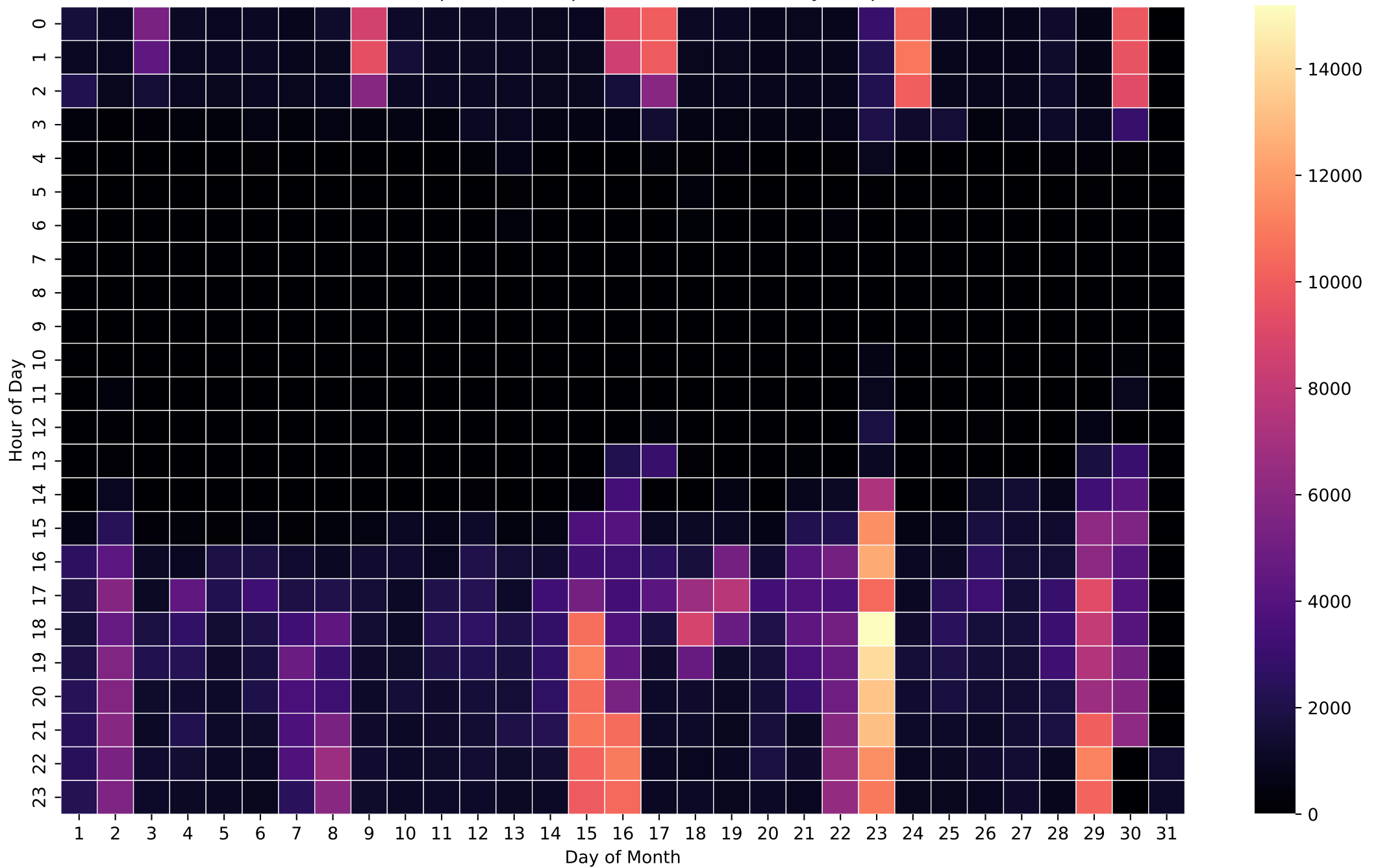
Grid Import Heatmap (Wh/Hour) - NoBattery - Sep
