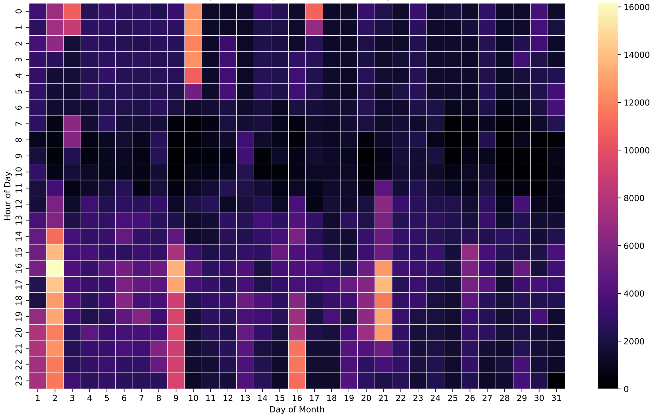
Grid Import Heatmap (Wh/Hour) - NoBattery - Dec
