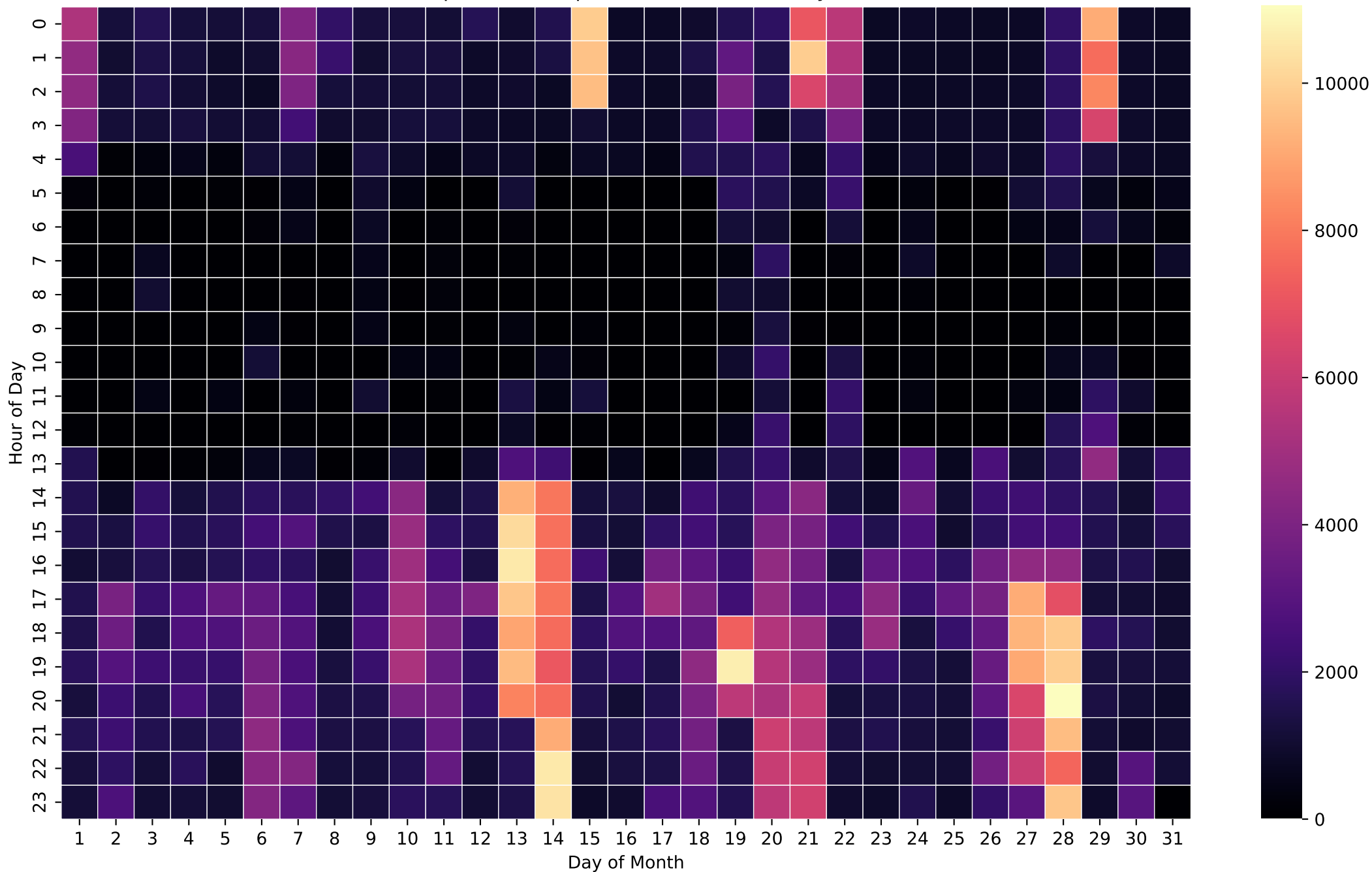
Grid Import Heatmap (Wh/Hour) - NoBattery - Oct
