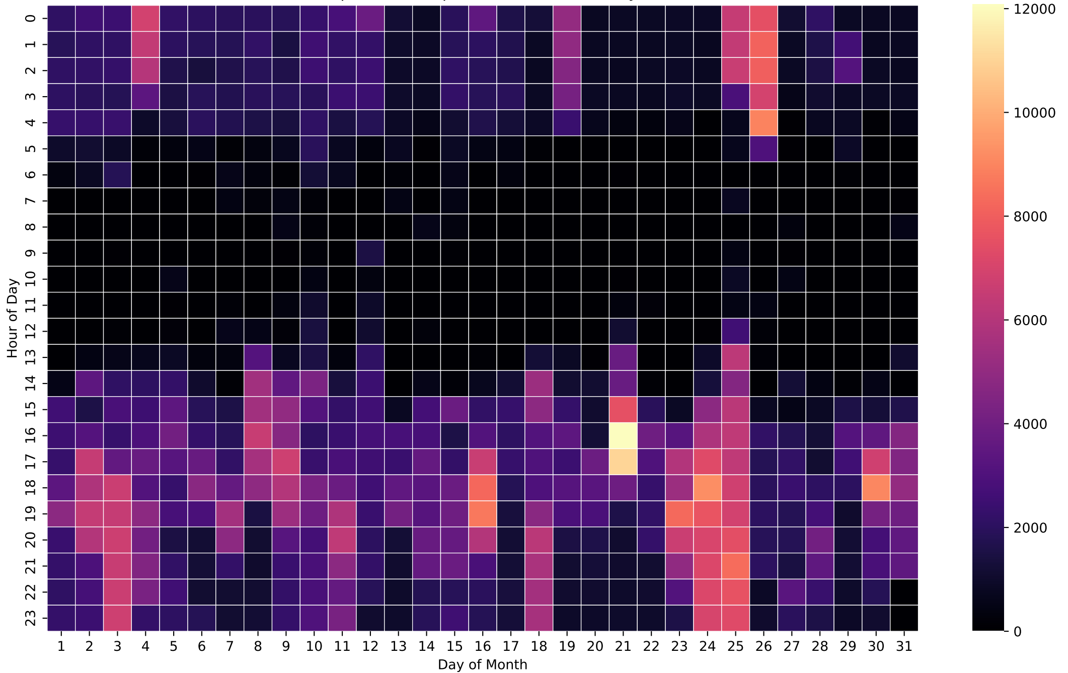
Grid Import Heatmap (Wh/Hour) - NoBattery - Mar
