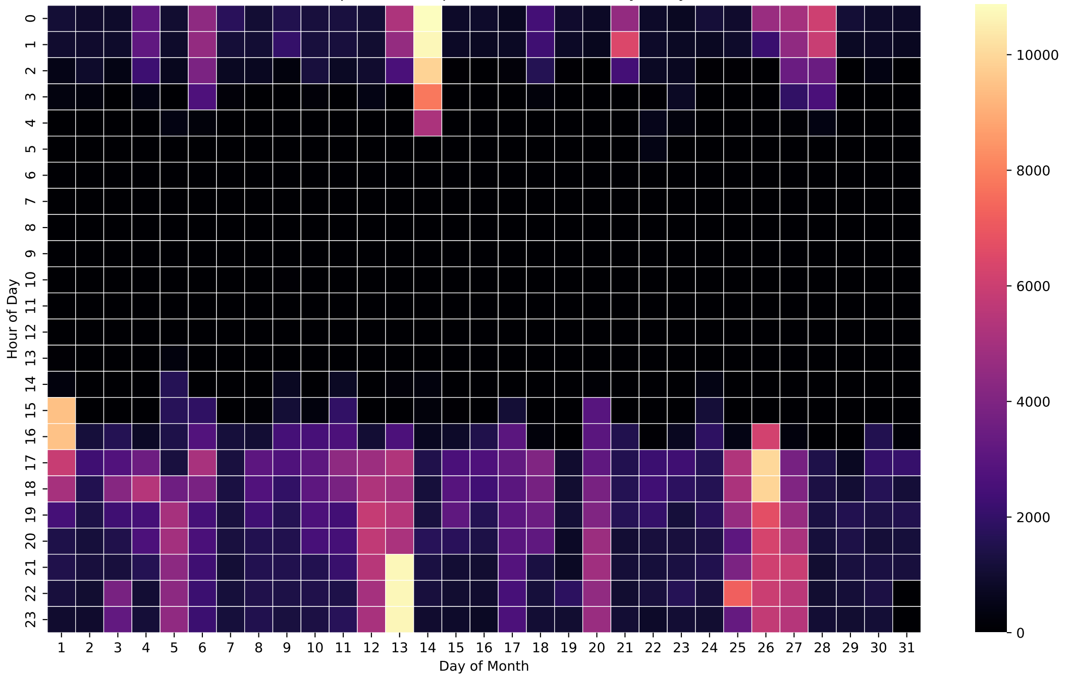
Grid Import Heatmap (Wh/Hour) - NoBattery - May
