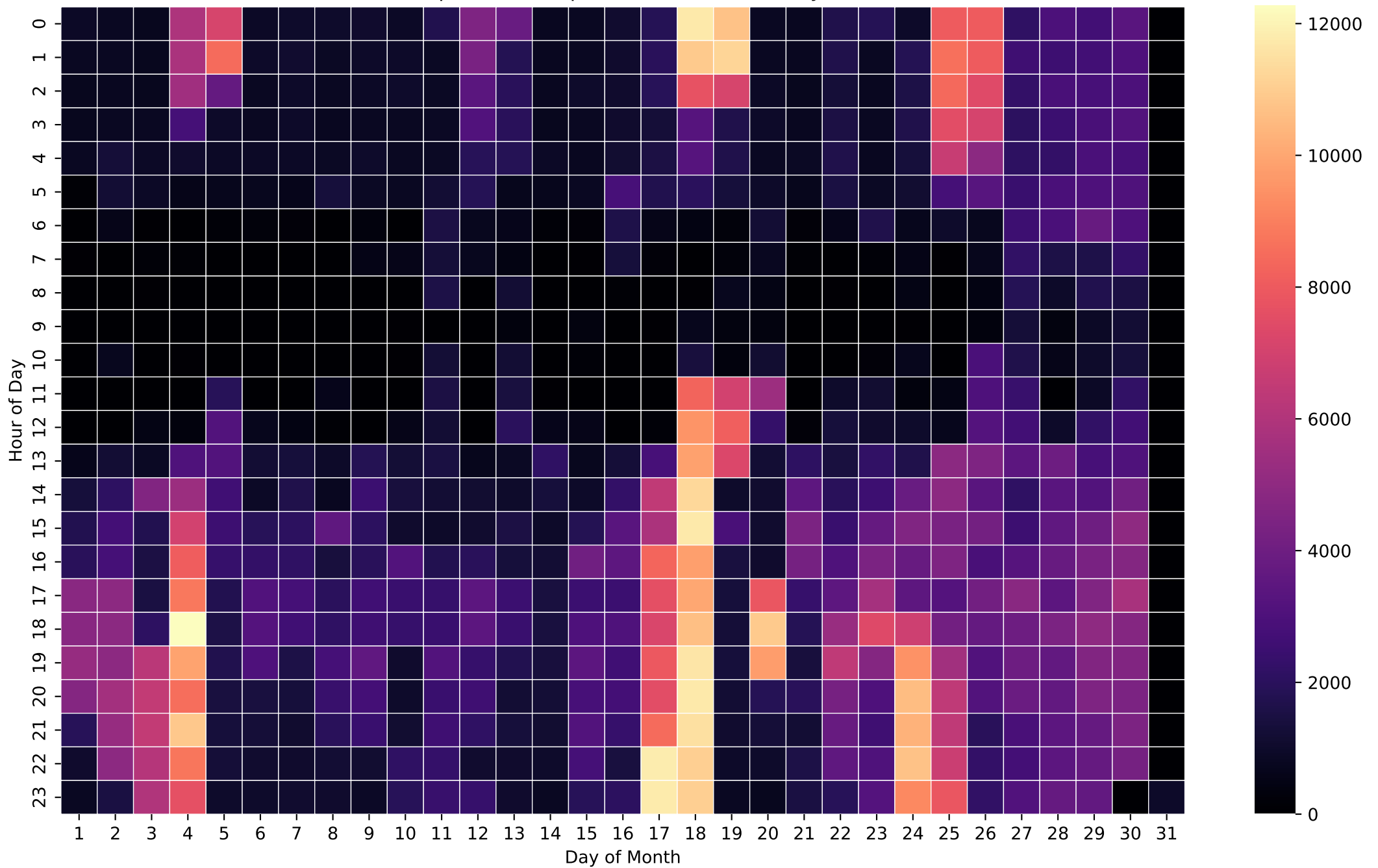
Grid Import Heatmap (Wh/Hour) - NoBattery - Nov
