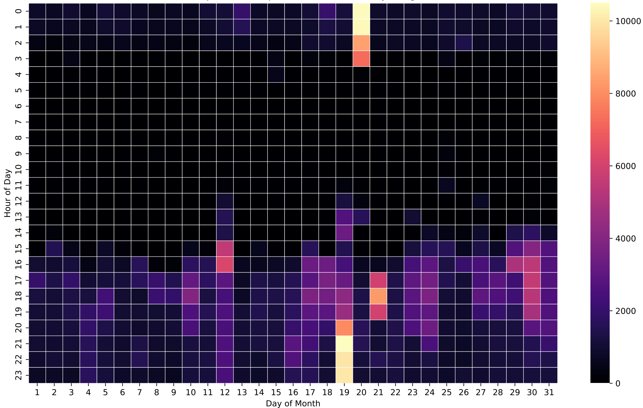
Grid Import Heatmap (Wh/Hour) - NoBattery - Aug
