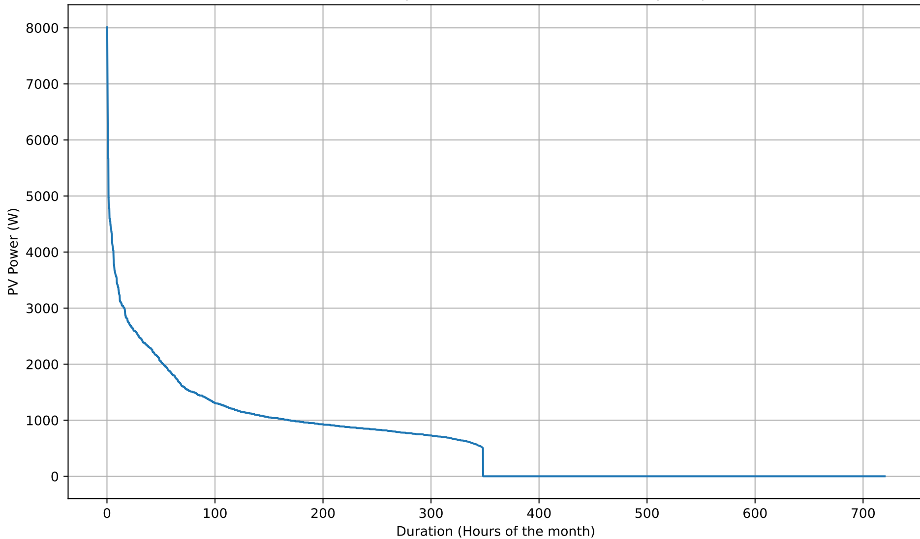
PV Self-Consumption Duration Curve - NoBattery - Sep
