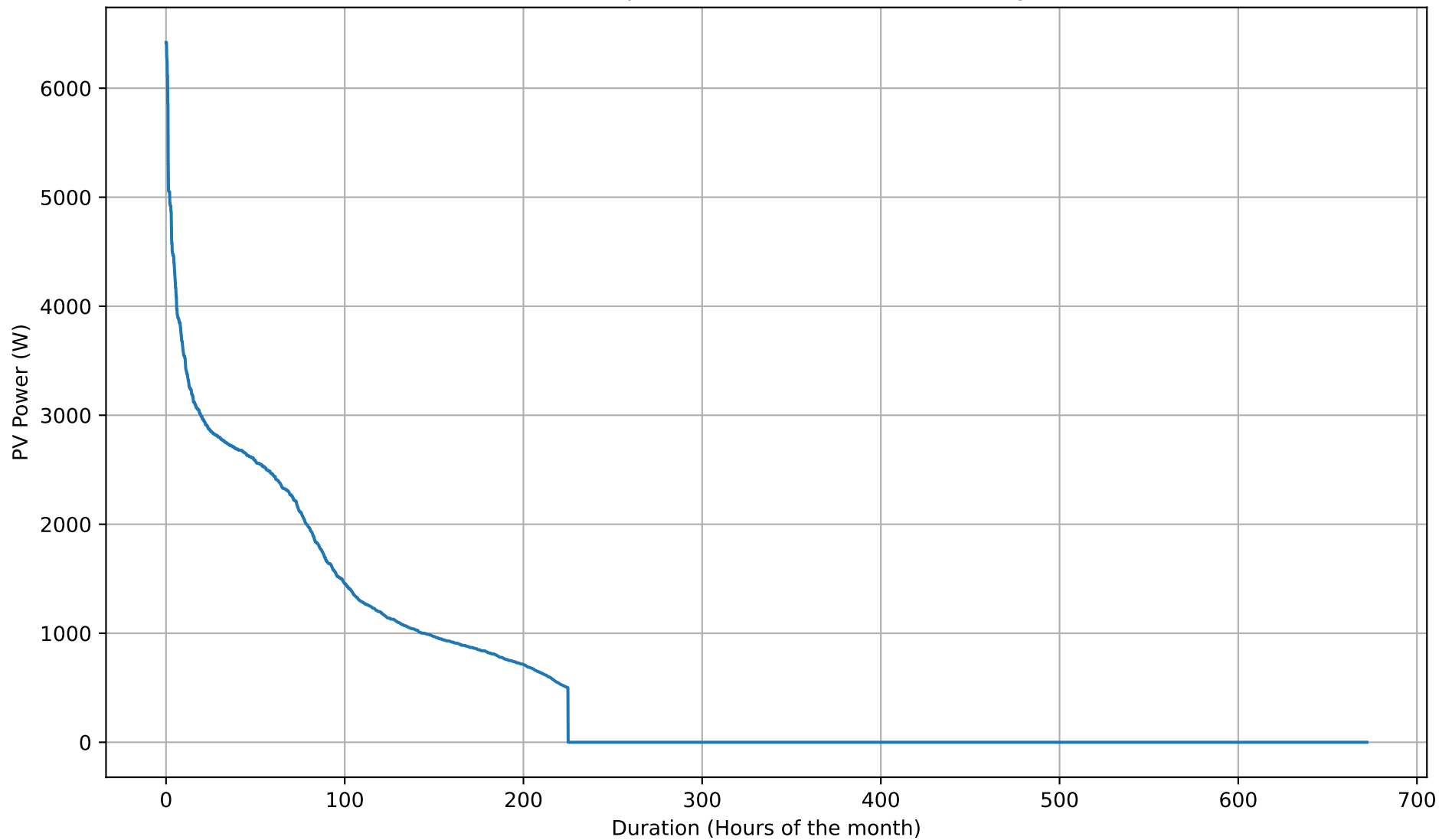
PV Self-Consumption Duration Curve - NoBattery - Feb
