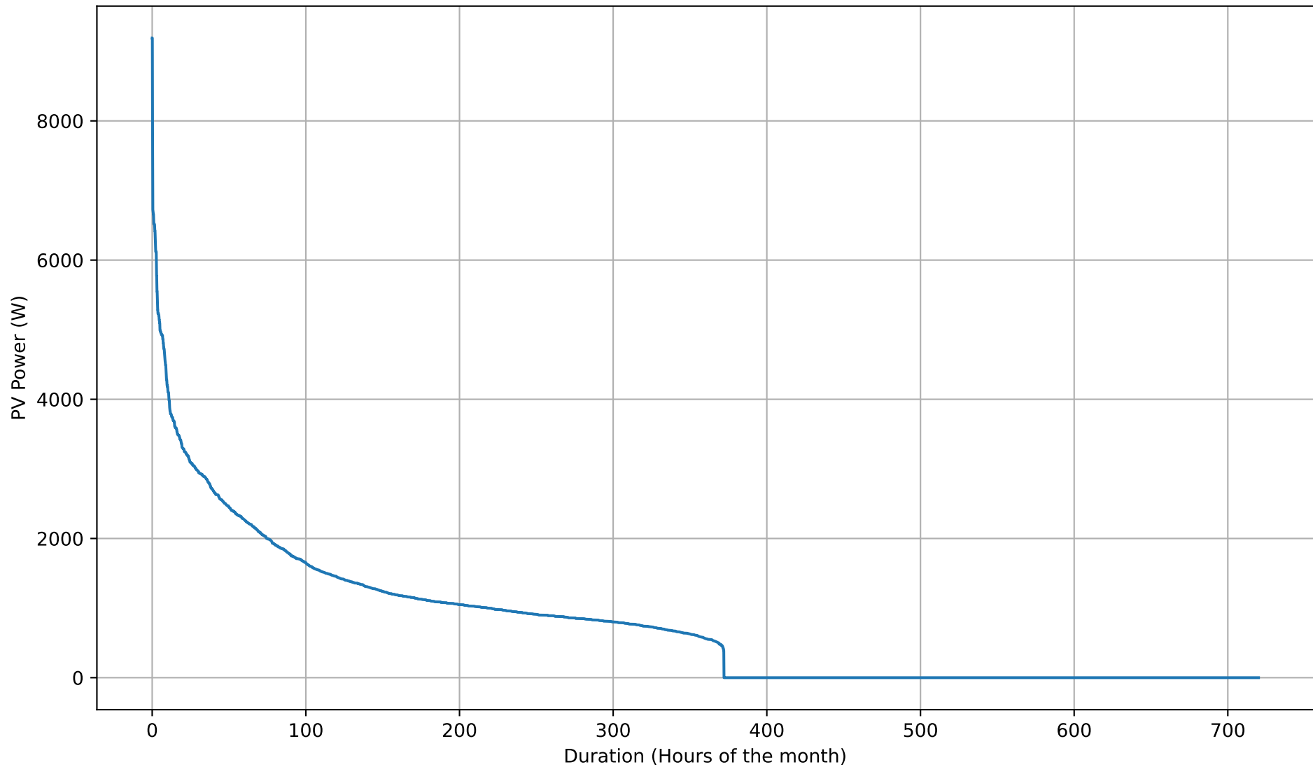
PV Self-Consumption Duration Curve - NoBattery - Apr
