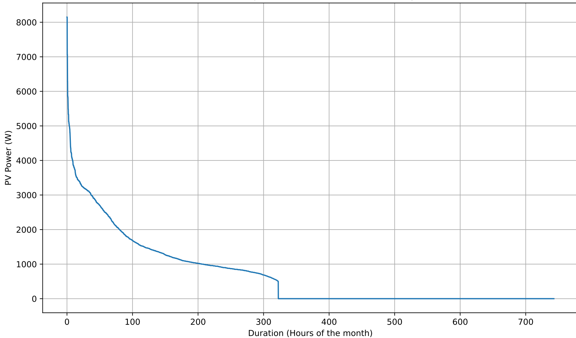
PV Self-Consumption Duration Curve - NoBattery - Mar
