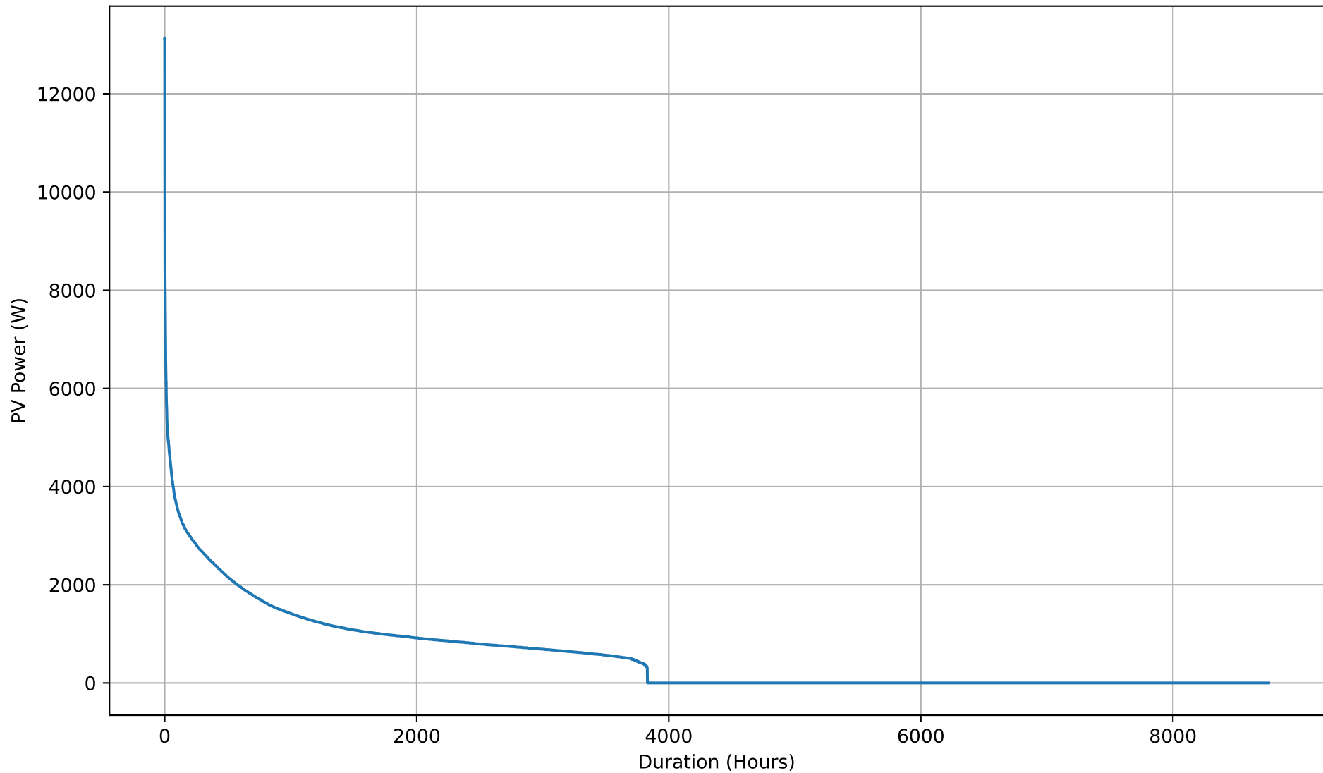
Yearly PV Self-Consumption Duration Curve - NoBattery
