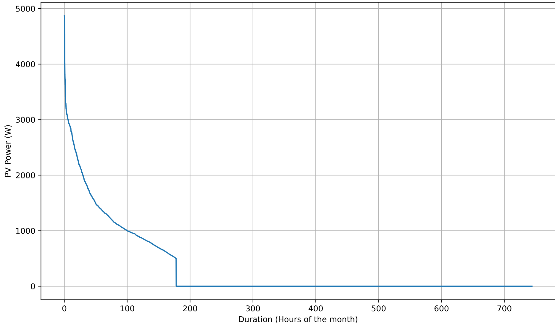
PV Self-Consumption Duration Curve - NoBattery - Jan
