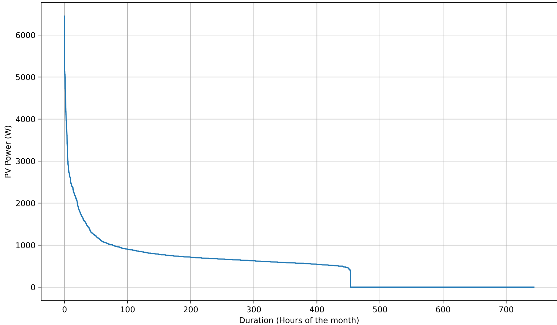
PV Self-Consumption Duration Curve - NoBattery - Jul
