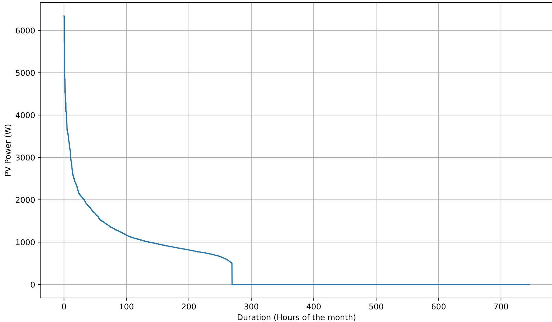
PV Self-Consumption Duration Curve - NoBattery - Oct
