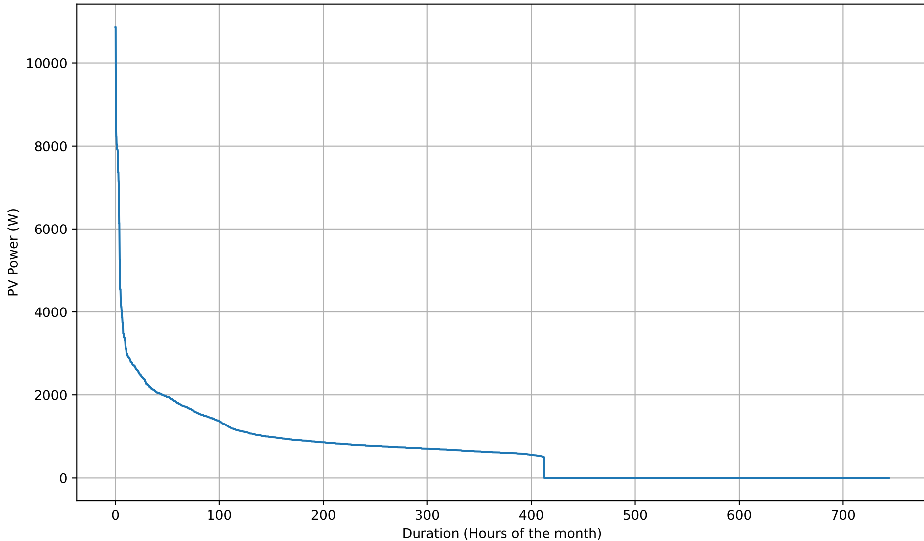
PV Self-Consumption Duration Curve - NoBattery - Aug
