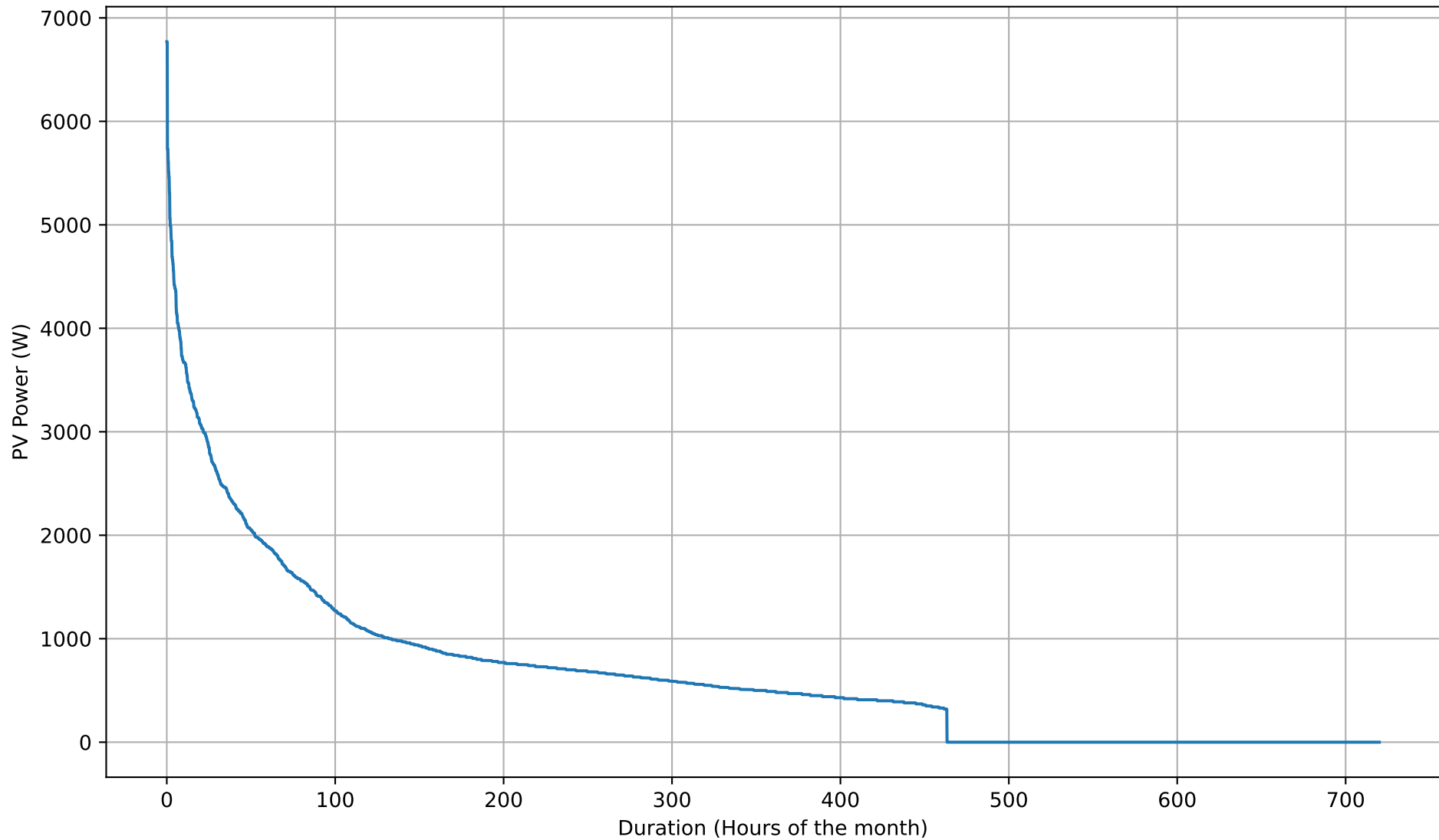
PV Self-Consumption Duration Curve - NoBattery - Jun
