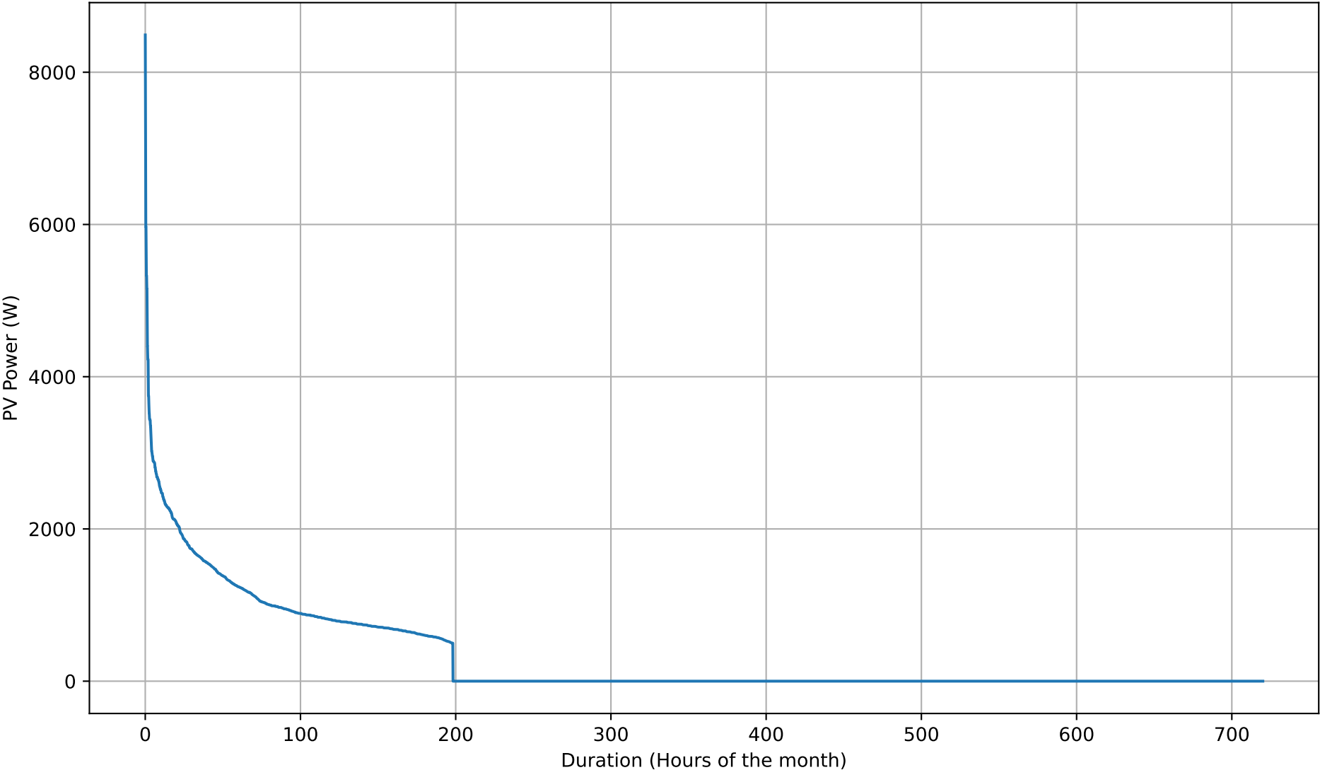
PV Self-Consumption Duration Curve - NoBattery - Nov
