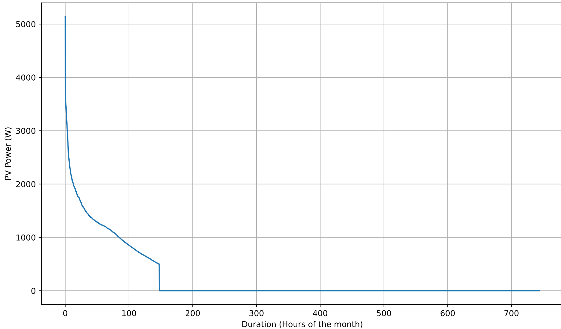
PV Self-Consumption Duration Curve - NoBattery - Dec
