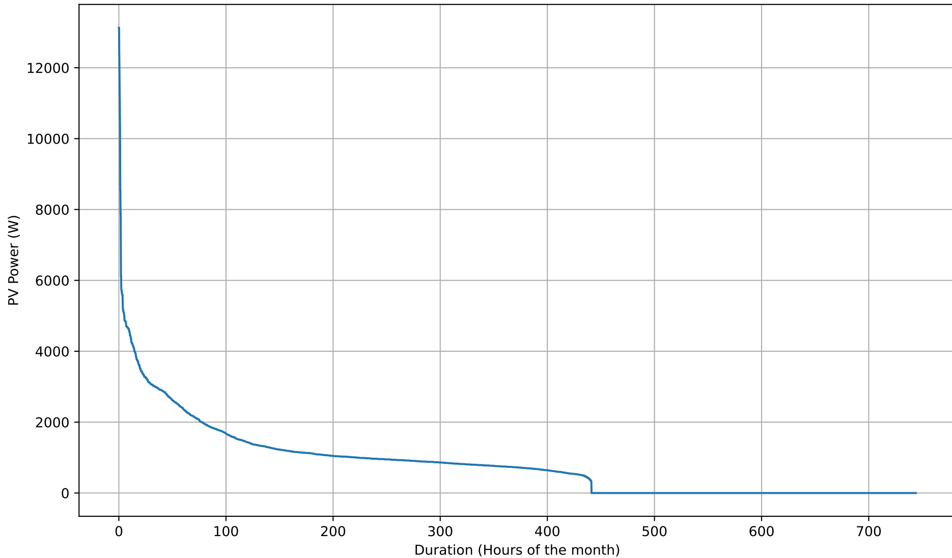
PV Self-Consumption Duration Curve - NoBattery - May
