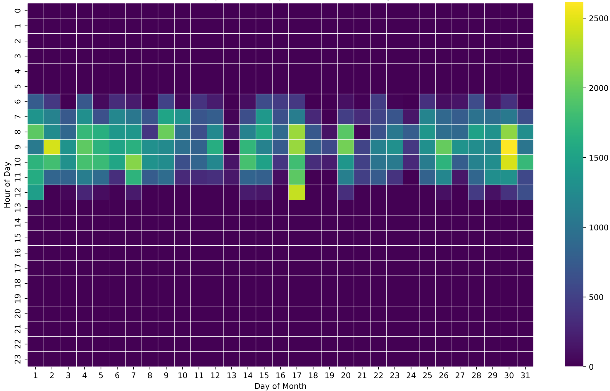
PV Self-Consumption Heatmap (Wh/Hour) - NoBattery - Dec
