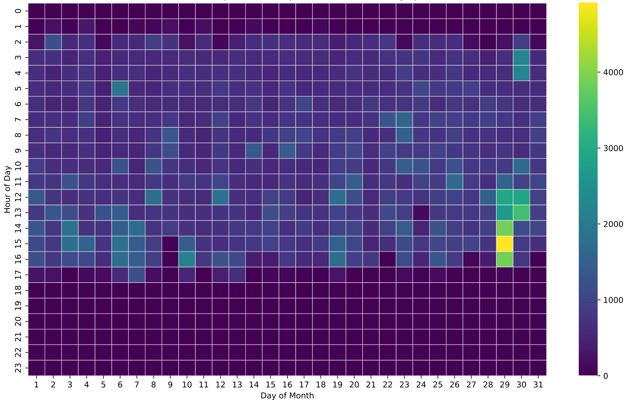
PV Self-Consumption Heatmap (Wh/Hour) - NoBattery - Jul
