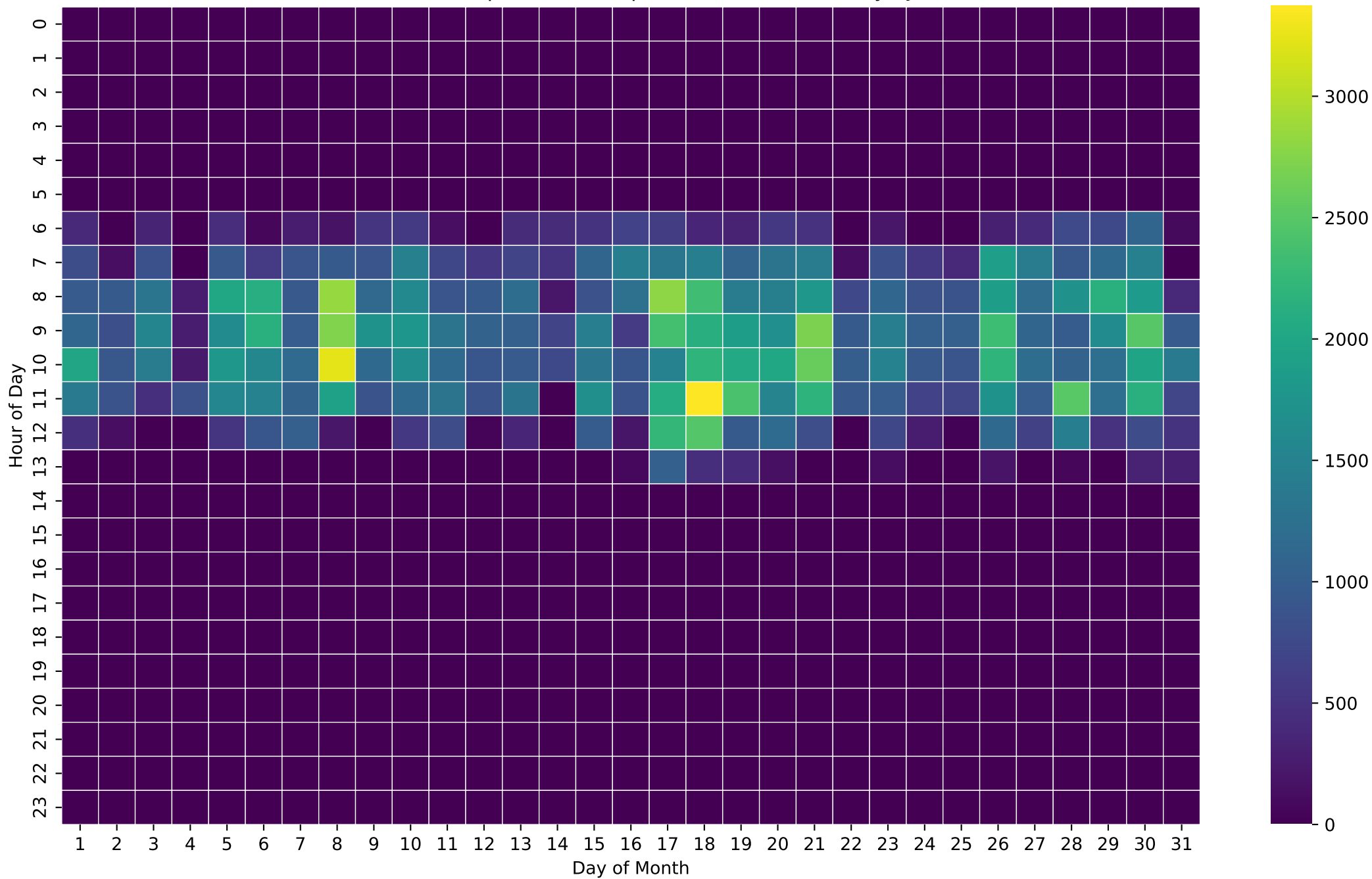
PV Self-Consumption Heatmap (Wh/Hour) - NoBattery - Jan
