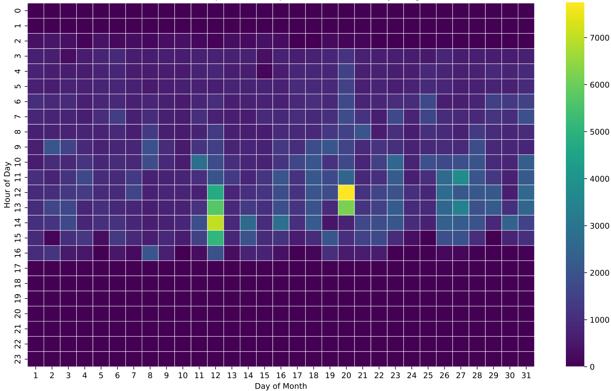
PV Self-Consumption Heatmap (Wh/Hour) - NoBattery - Aug
