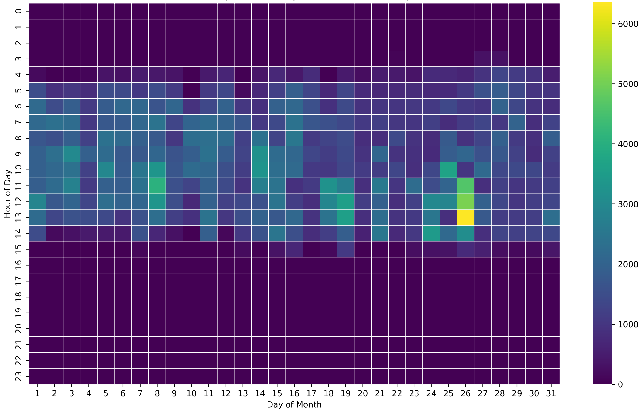
PV Self-Consumption Heatmap (Wh/Hour) - NoBattery - Mar
