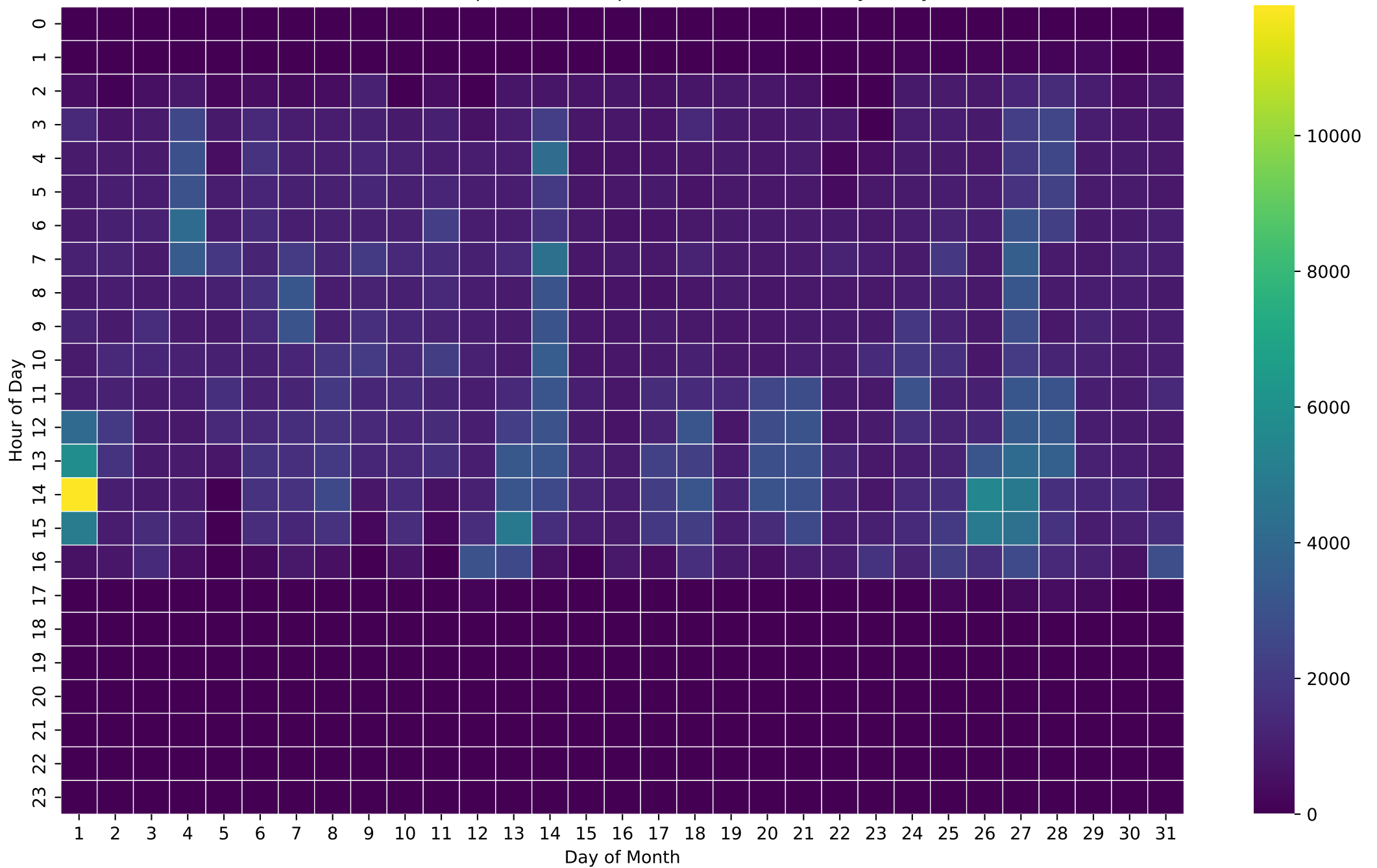
PV Self-Consumption Heatmap (Wh/Hour) - NoBattery - May
