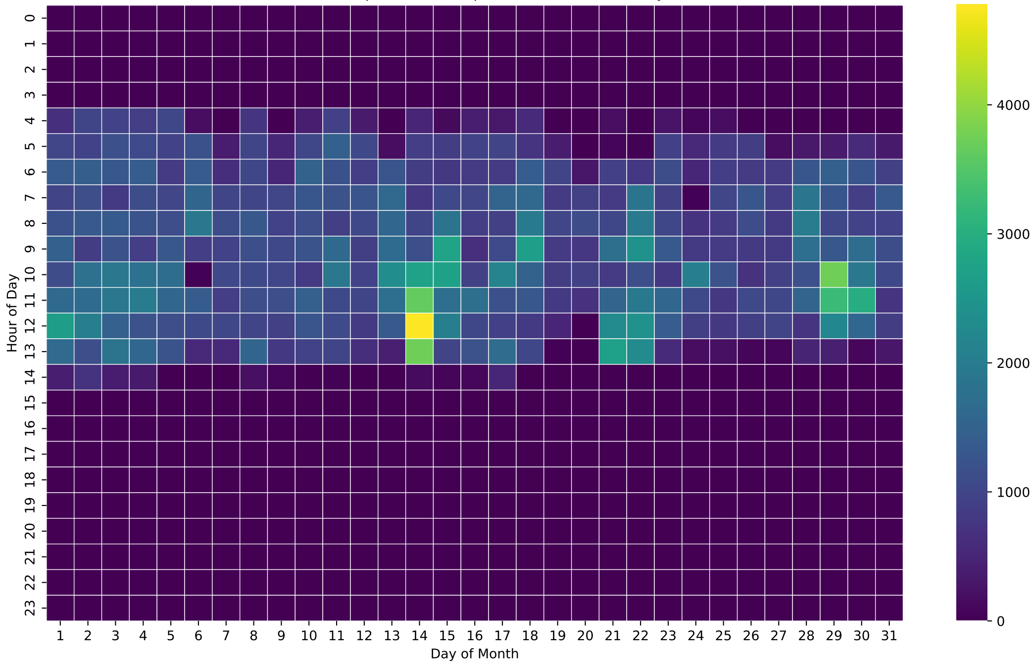
PV Self-Consumption Heatmap (Wh/Hour) - NoBattery - Oct
