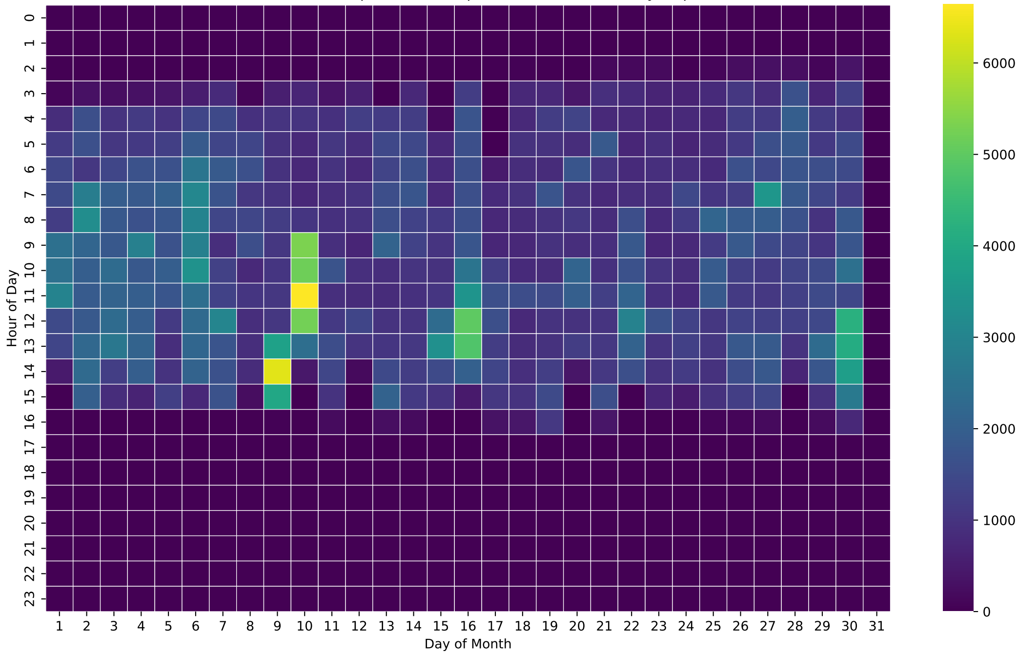
PV Self-Consumption Heatmap (Wh/Hour) - NoBattery - Apr
