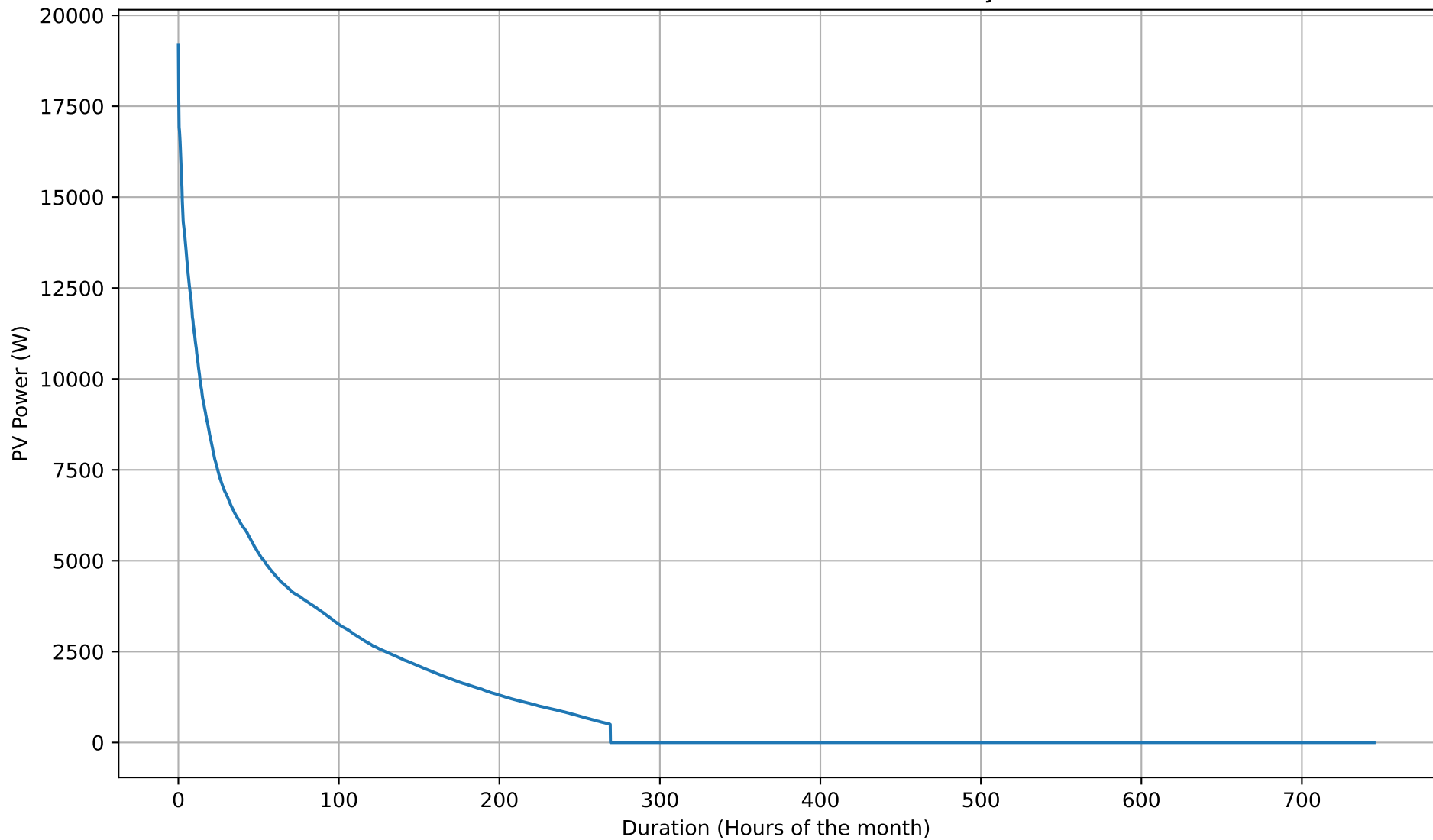
PV Production Duration Curve - NoBattery - Oct
