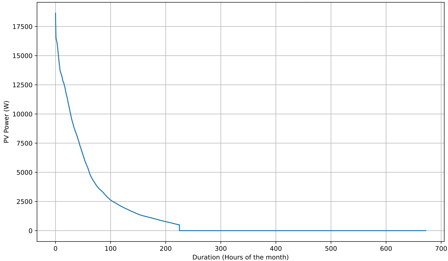
PV Production Duration Curve - NoBattery - Feb
