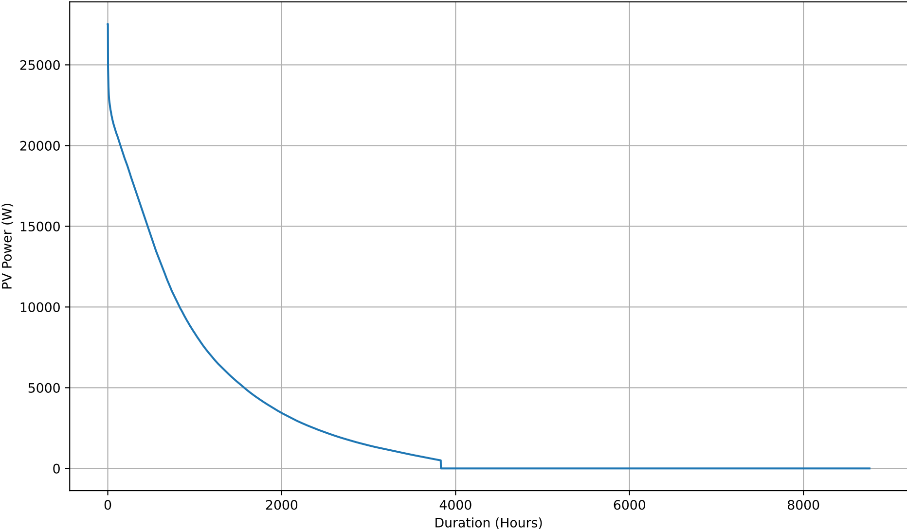
Yearly PV Production Duration Curve - NoBattery
