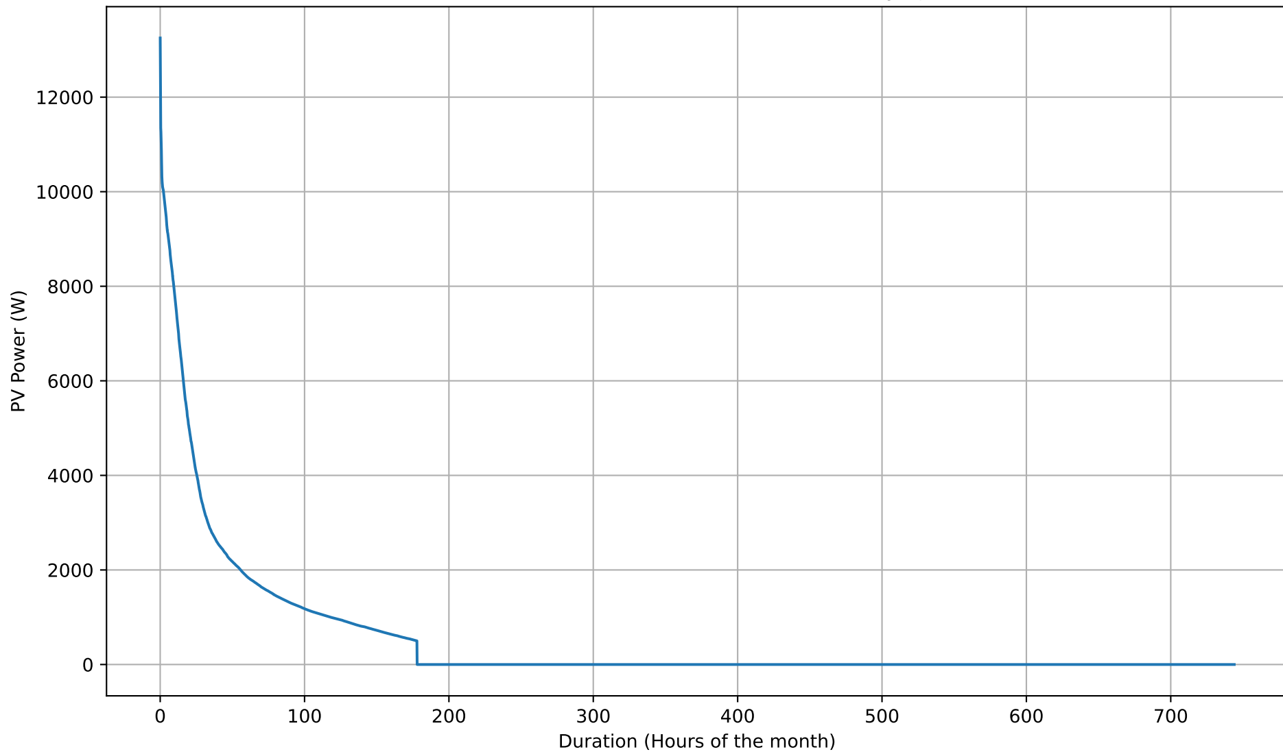
PV Production Duration Curve - NoBattery - Jan
