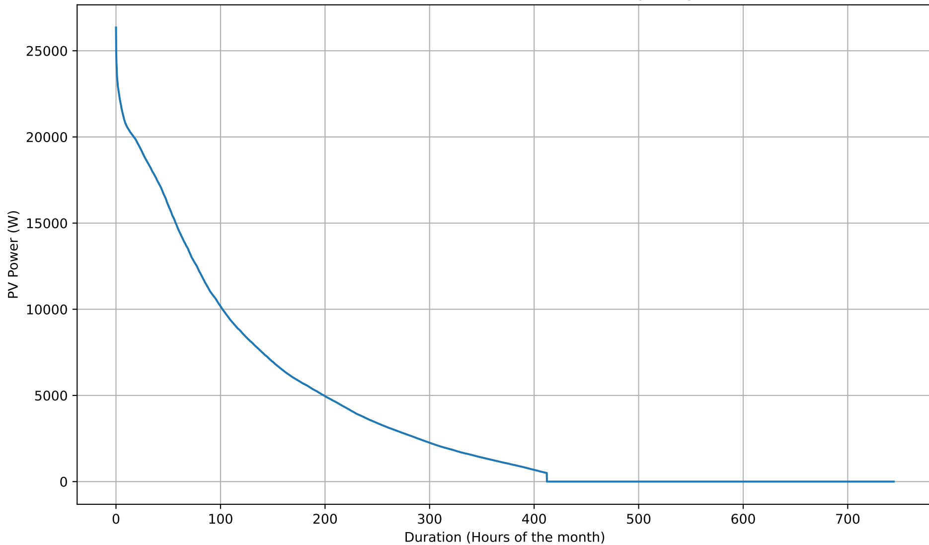
PV Production Duration Curve - NoBattery - Aug
