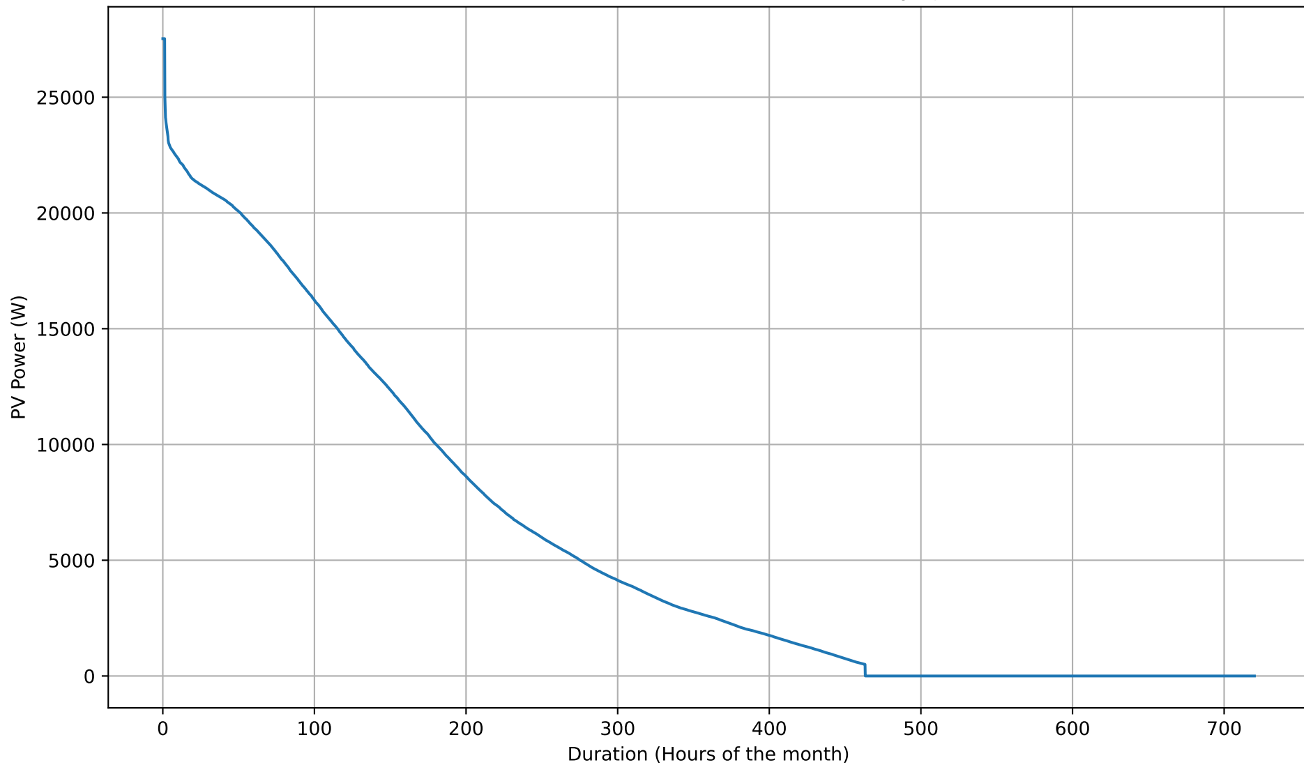
PV Production Duration Curve - NoBattery - Jun
