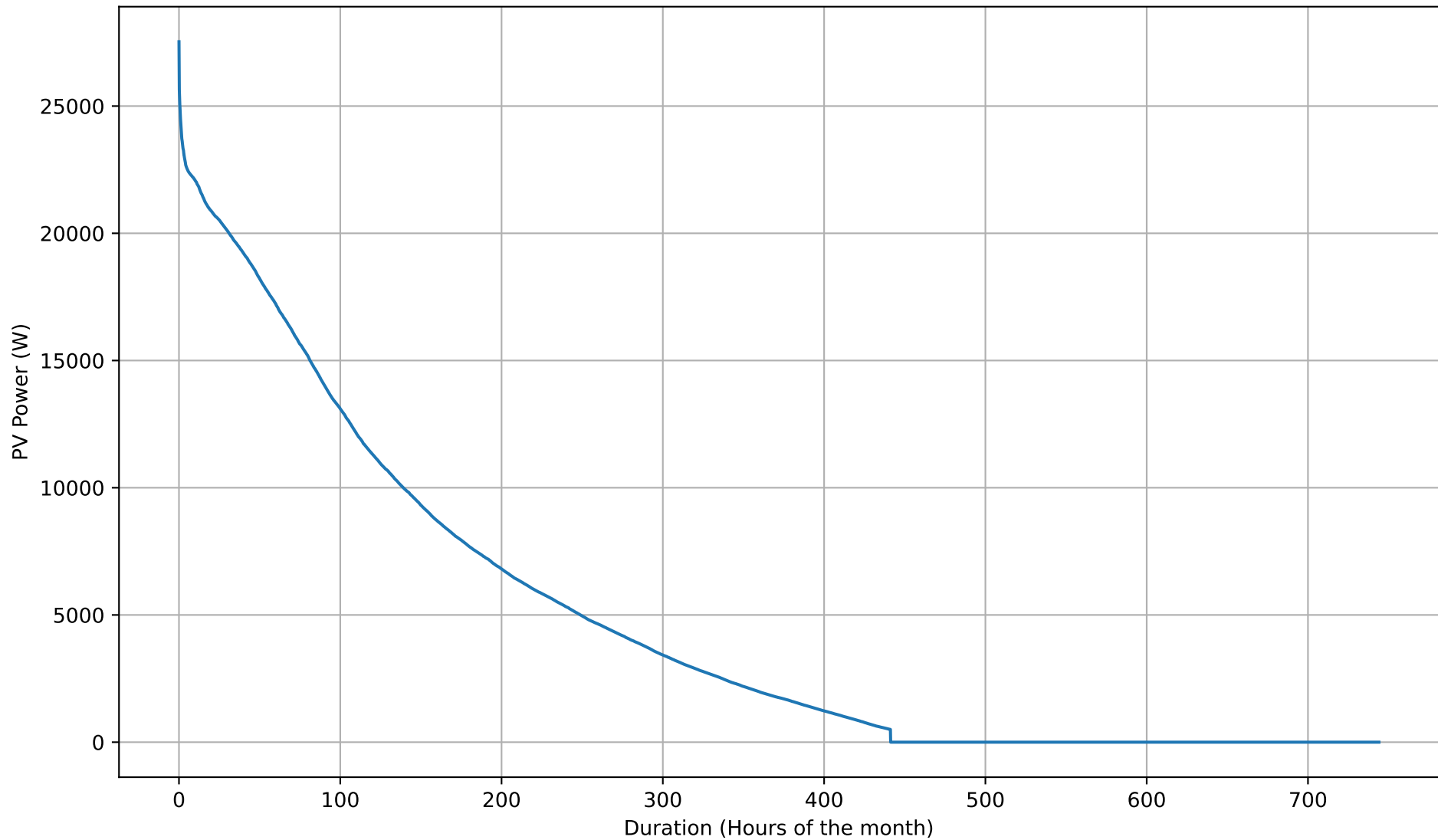
PV Production Duration Curve - NoBattery - May
