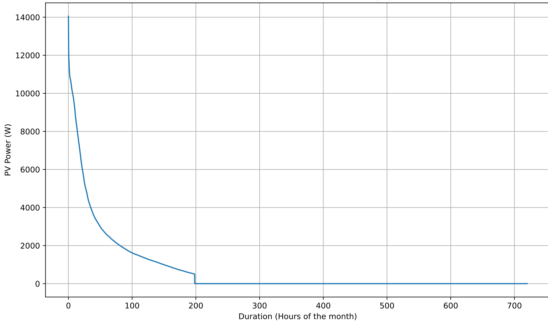
PV Production Duration Curve - NoBattery - Nov
