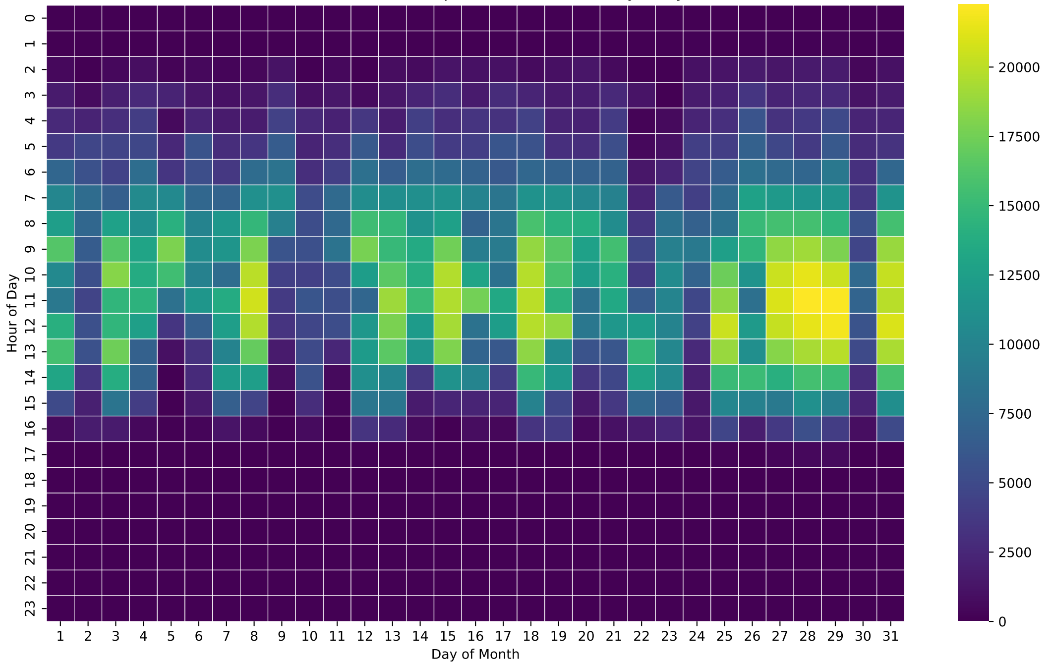
PV Production Heatmap (Wh/Hour) - NoBattery - May
