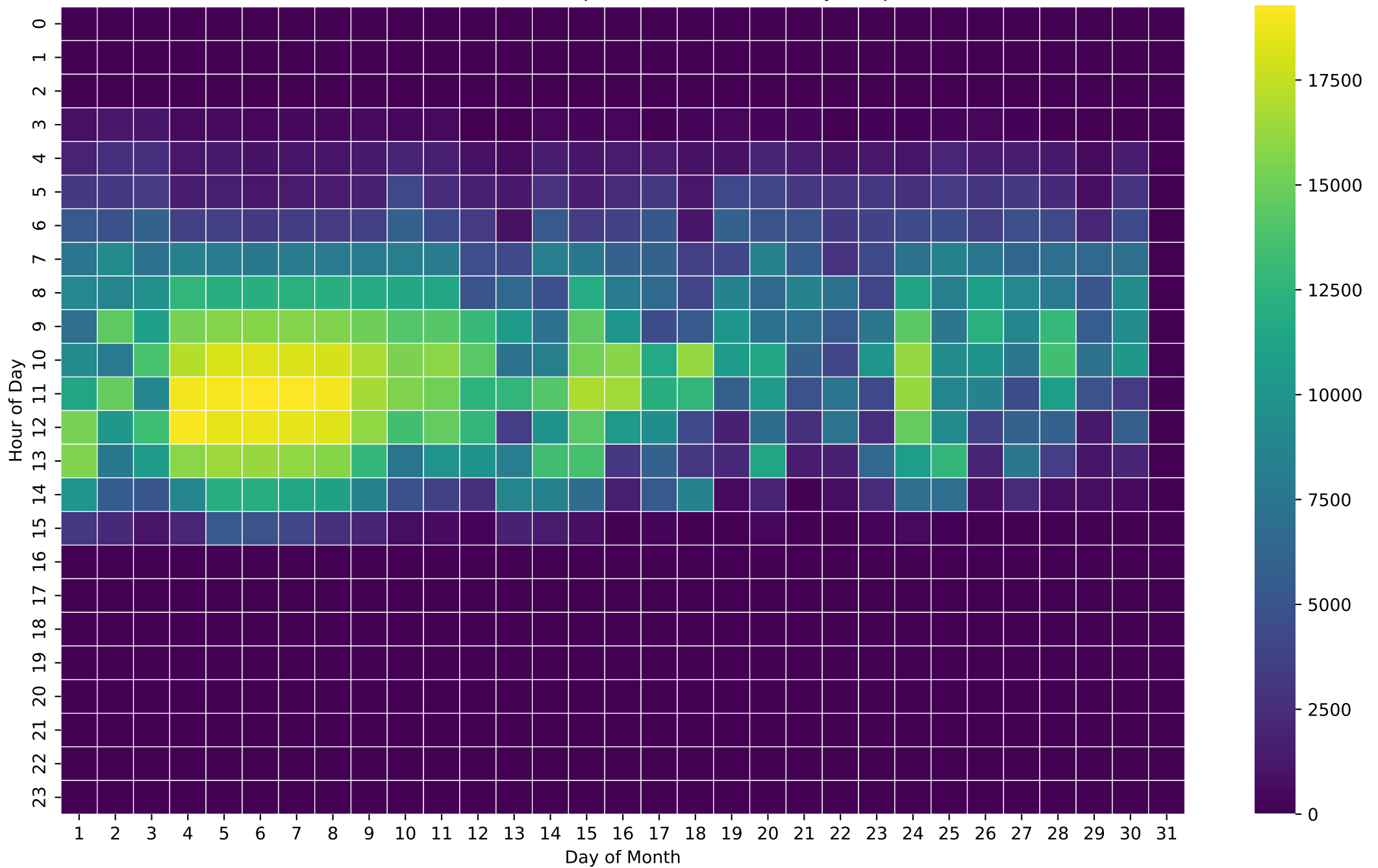
PV Production Heatmap (Wh/Hour) - NoBattery - Sep
