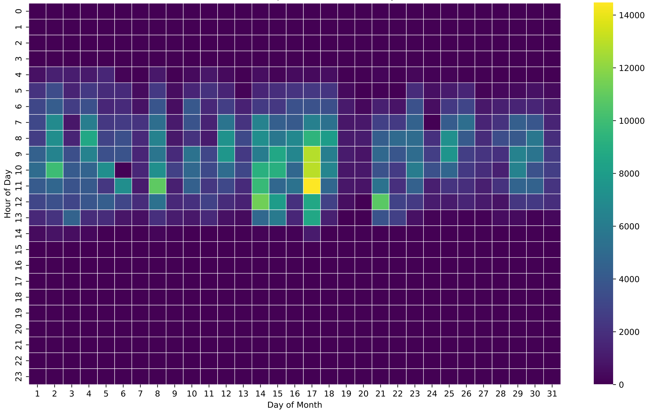
PV Production Heatmap (Wh/Hour) - NoBattery - Oct
