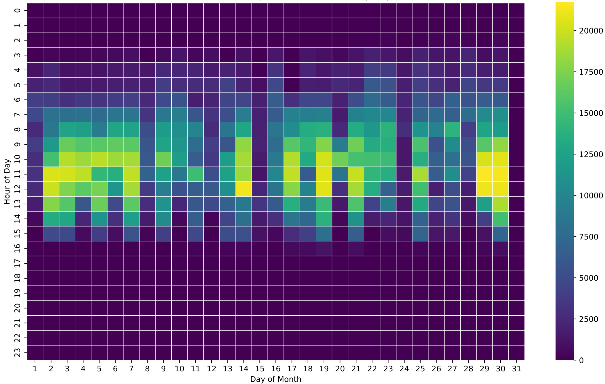
PV Production Heatmap (Wh/Hour) - NoBattery - Apr
