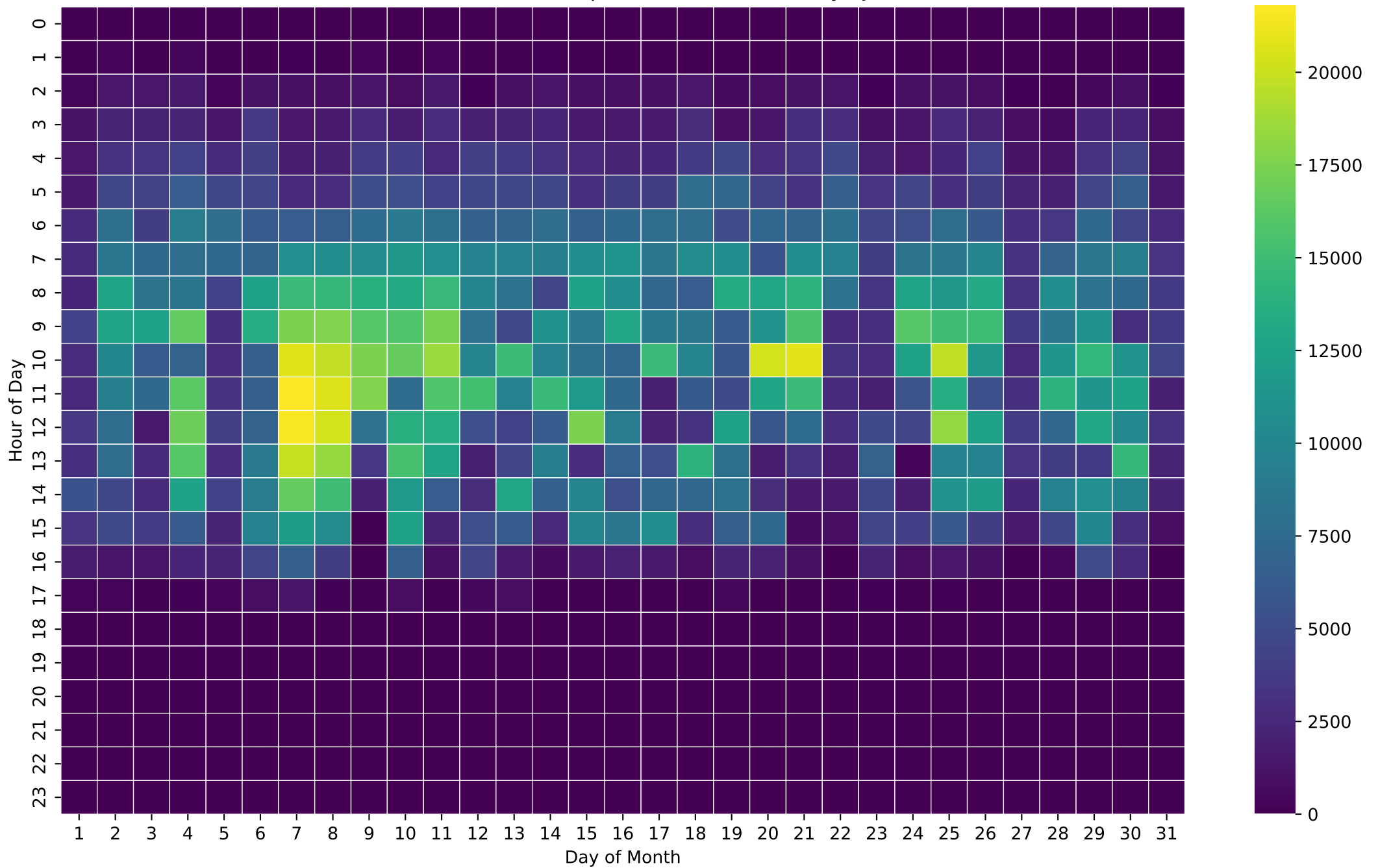
PV Production Heatmap (Wh/Hour) - NoBattery - Jul
