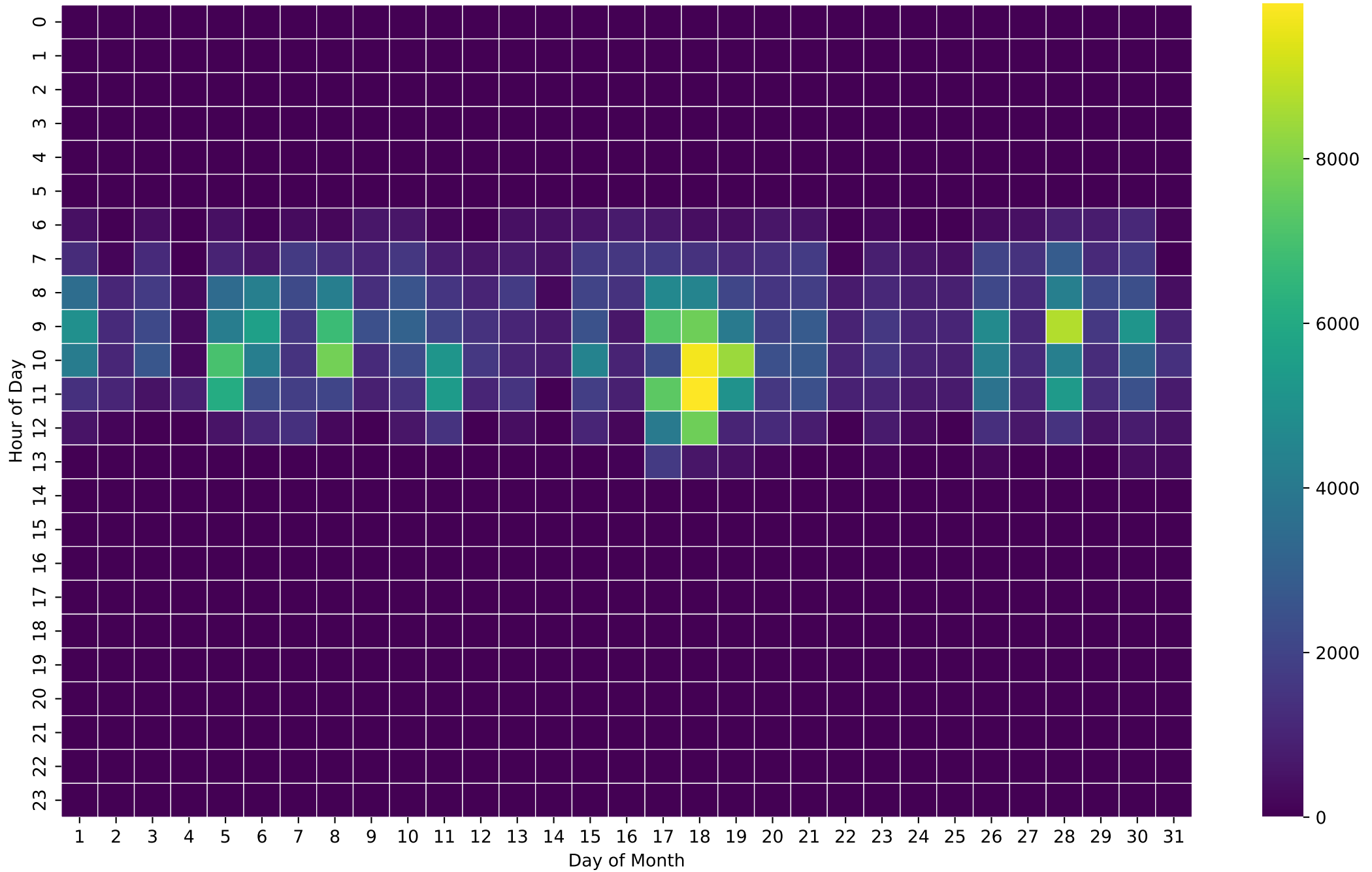
PV Production Heatmap (Wh/Hour) - NoBattery - Jan
