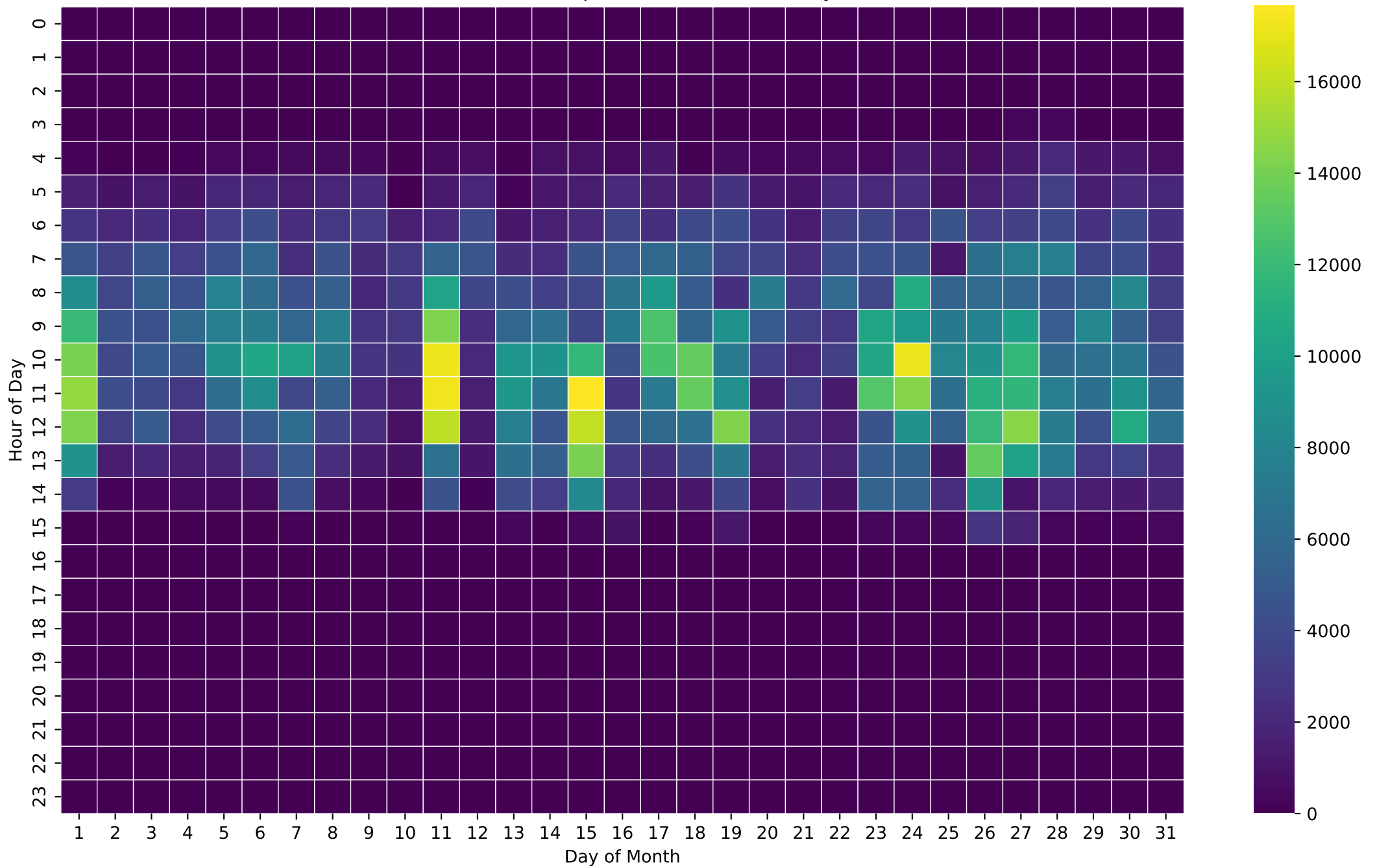
PV Production Heatmap (Wh/Hour) - NoBattery - Mar
