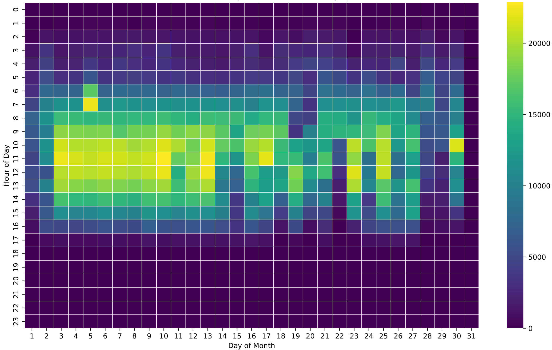
PV Production Heatmap (Wh/Hour) - NoBattery - Jun
