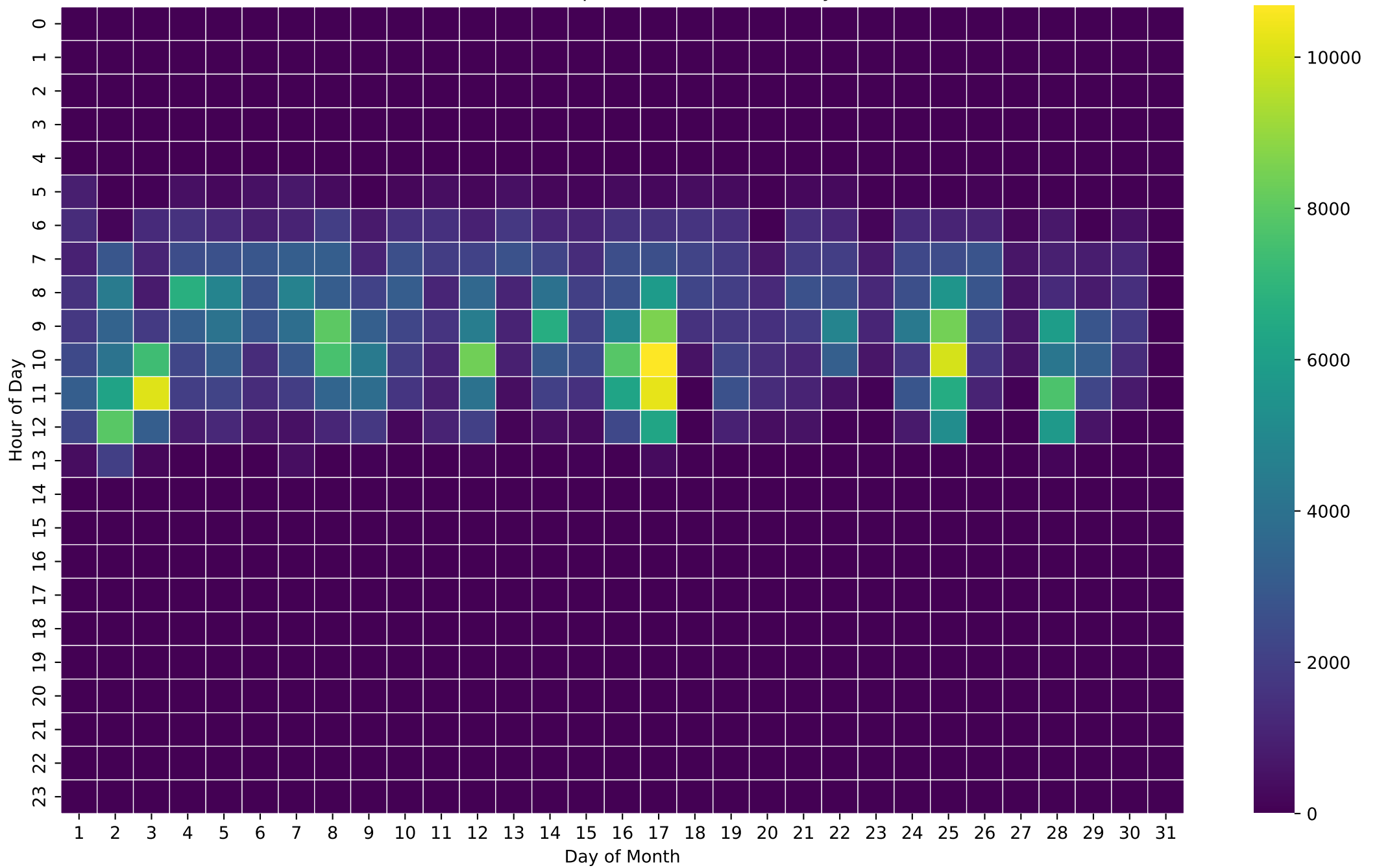
PV Production Heatmap (Wh/Hour) - NoBattery - Nov
