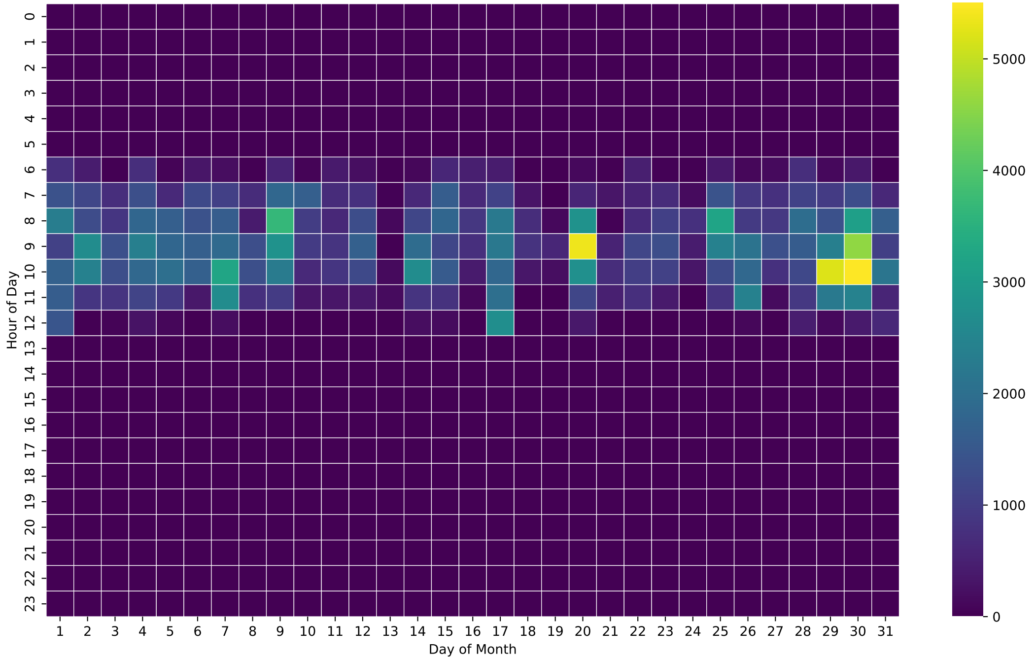
PV Production Heatmap (Wh/Hour) - NoBattery - Dec
