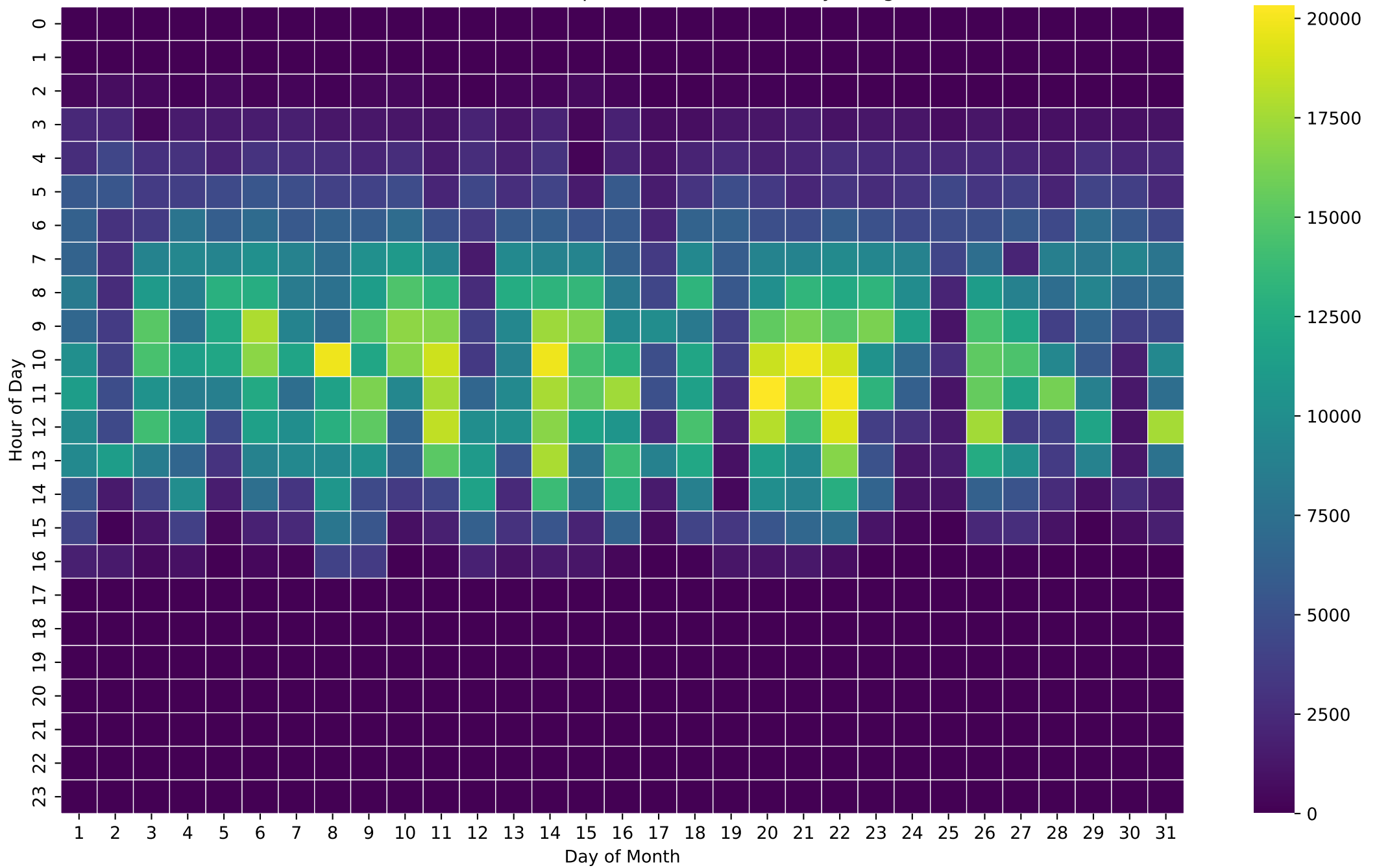
PV Production Heatmap (Wh/Hour) - NoBattery - Aug
