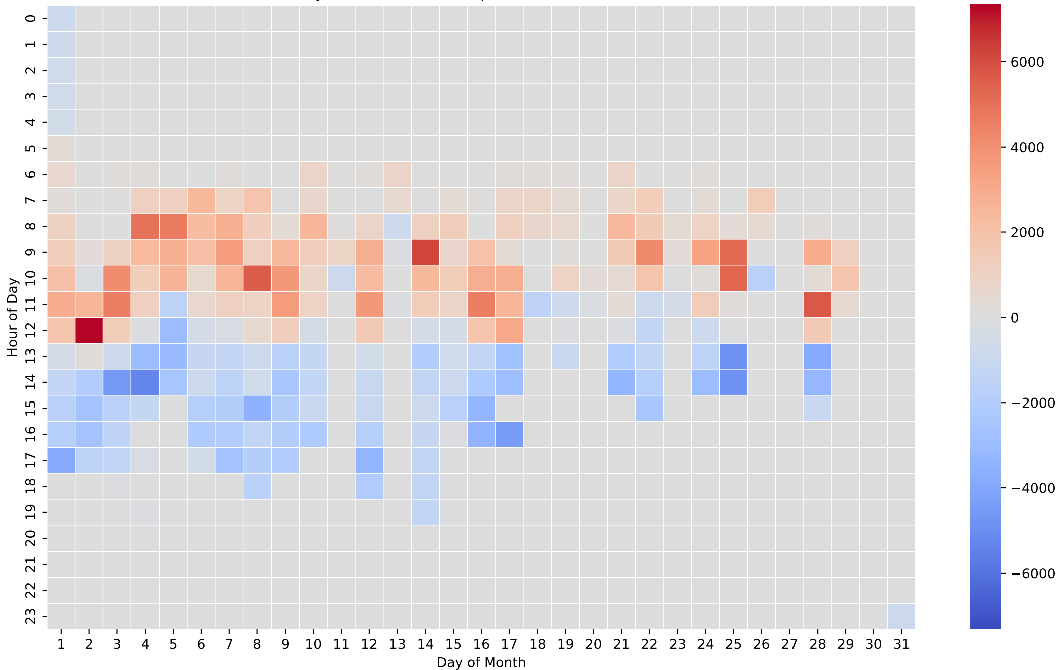
Battery Net Power Heatmap (Wh/Hour) - 12kWh - Nov
