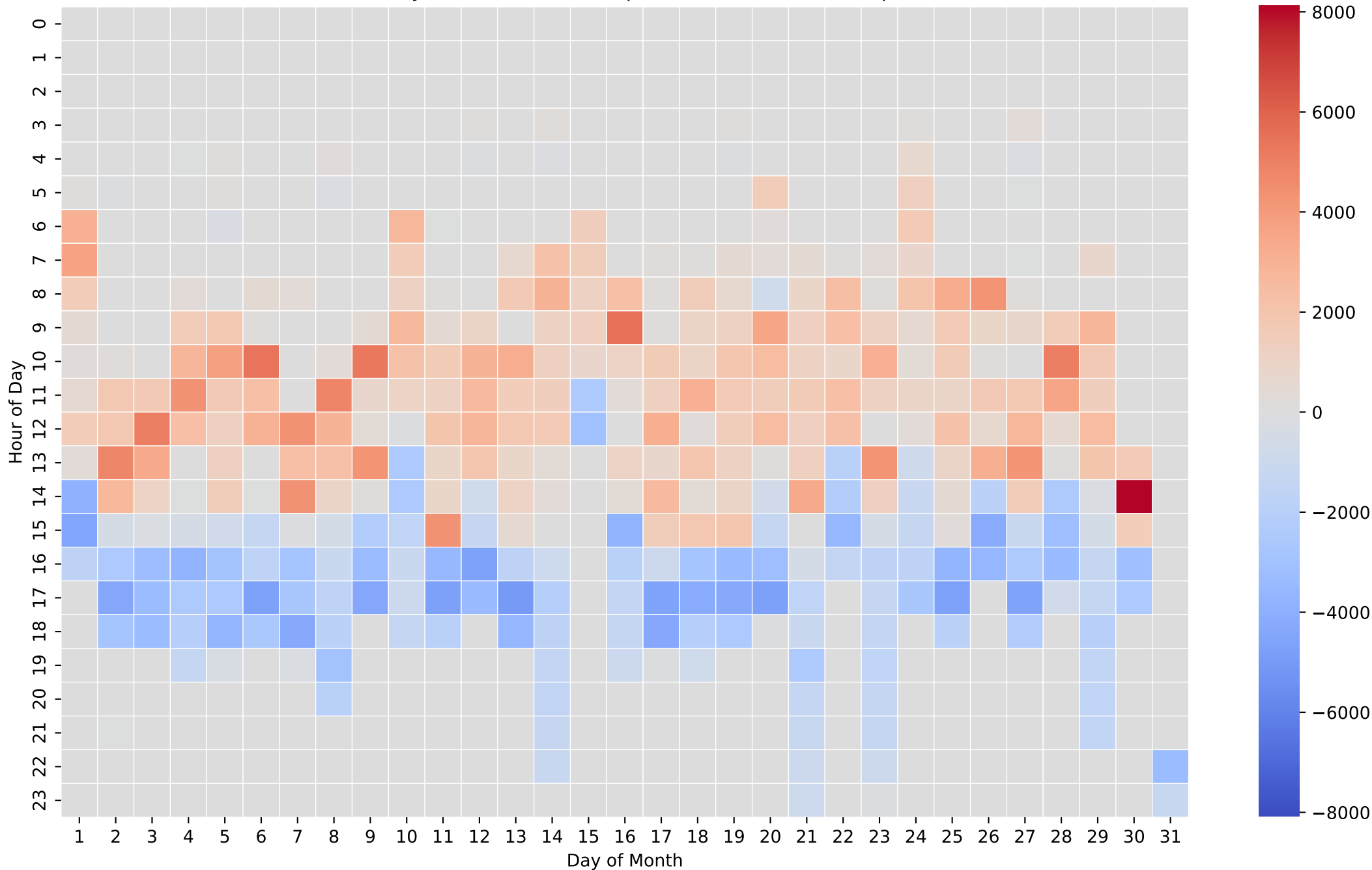
Battery Net Power Heatmap (Wh/Hour) - 12kWh - Apr
