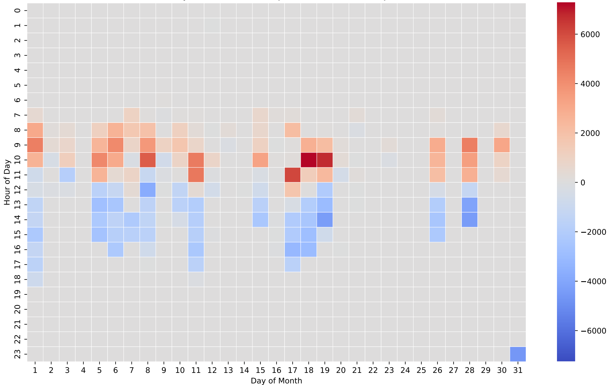
Battery Net Power Heatmap (Wh/Hour) - 12kWh - Jan
