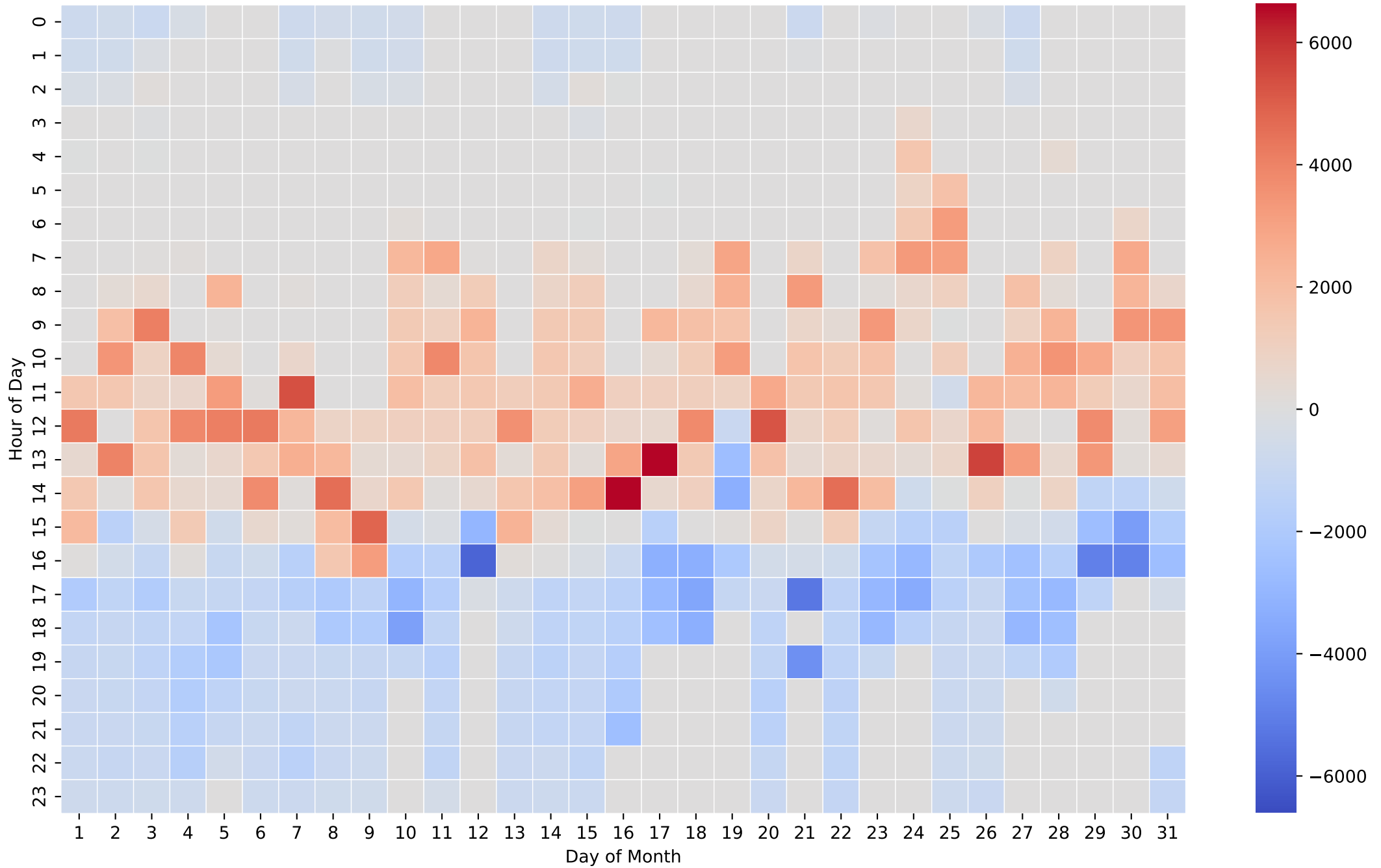
Battery Net Power Heatmap (Wh/Hour) - 12kWh - Aug
