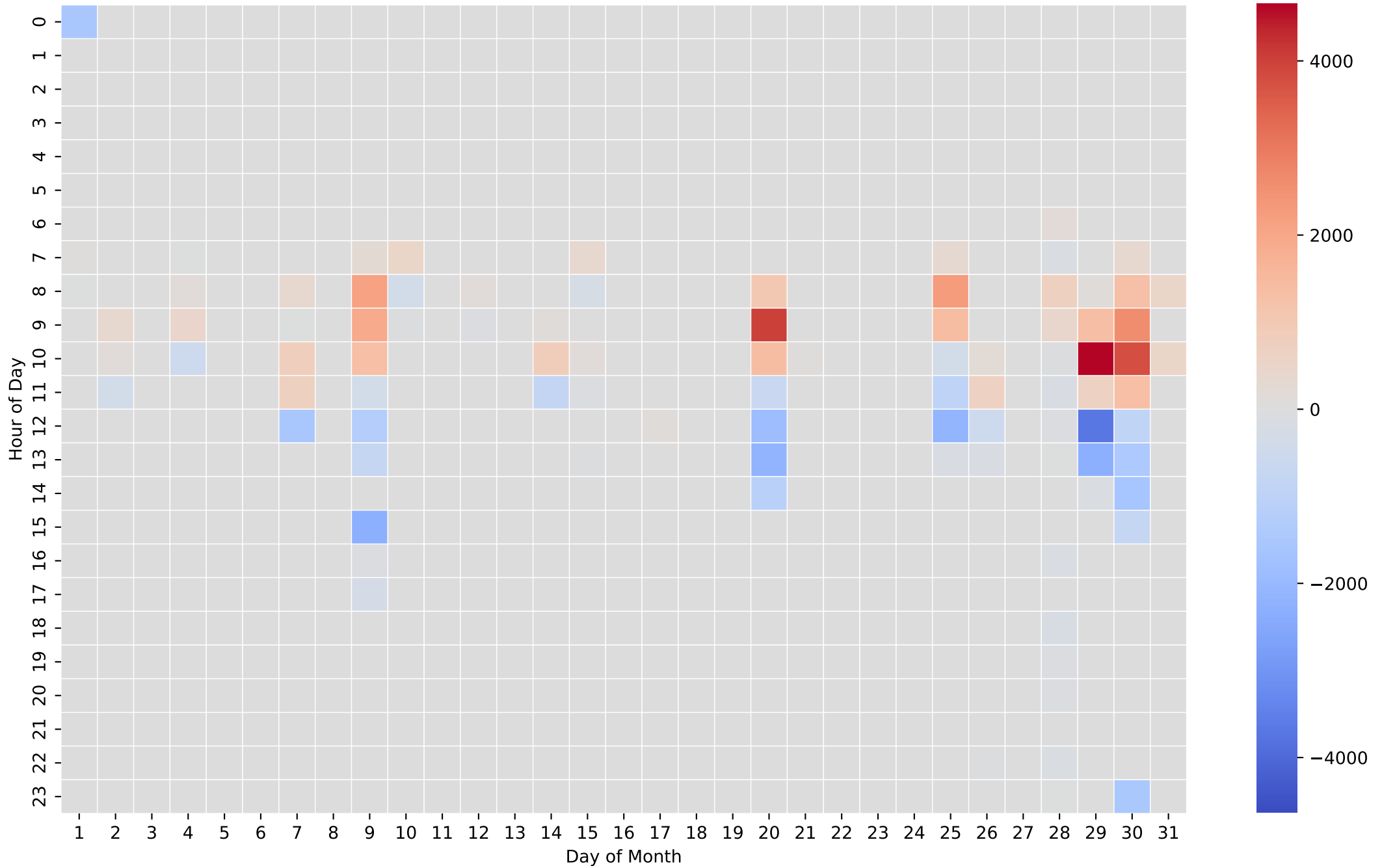
Battery Net Power Heatmap (Wh/Hour) - 12kWh - Dec
