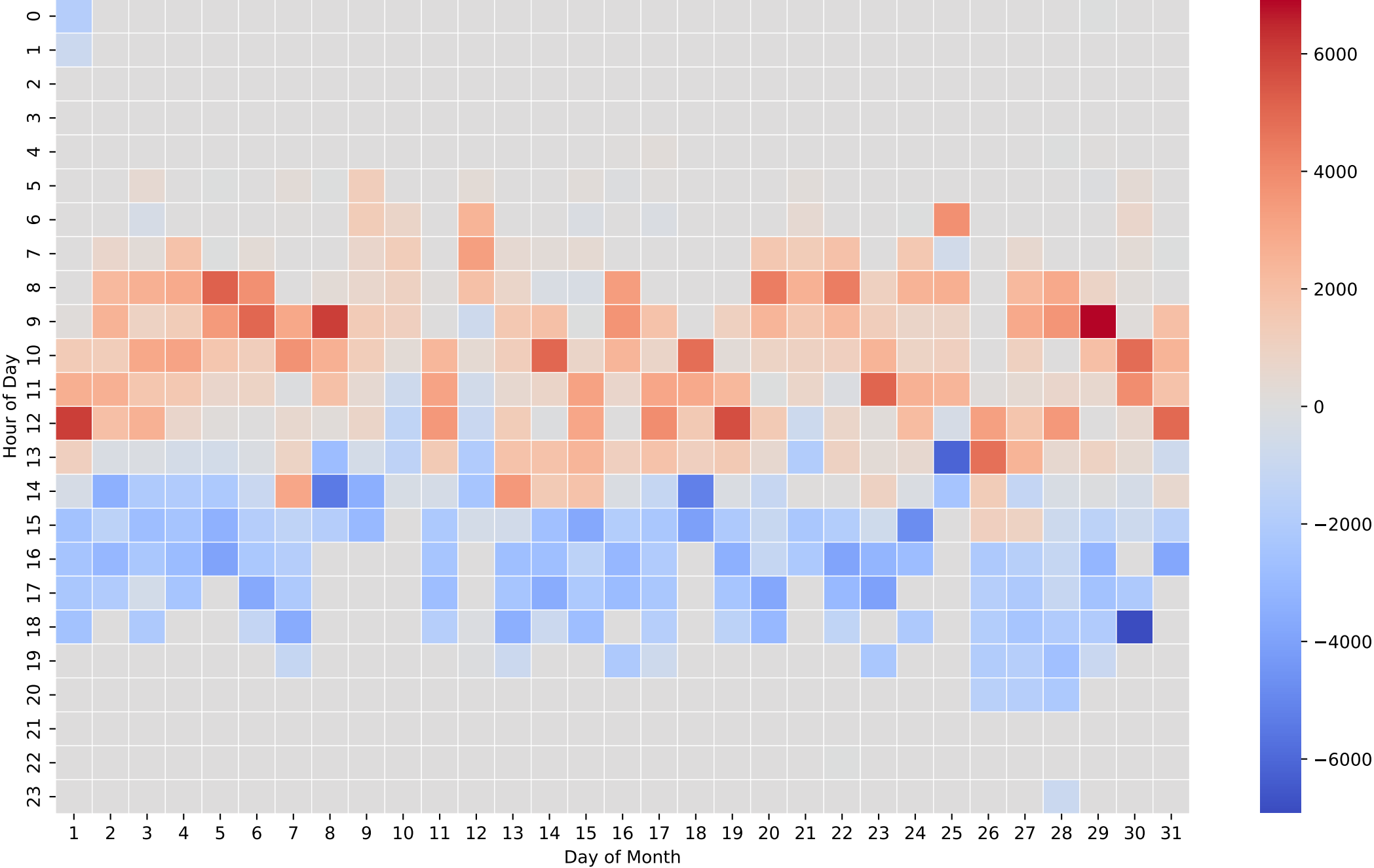
Battery Net Power Heatmap (Wh/Hour) - 12kWh - Mar
