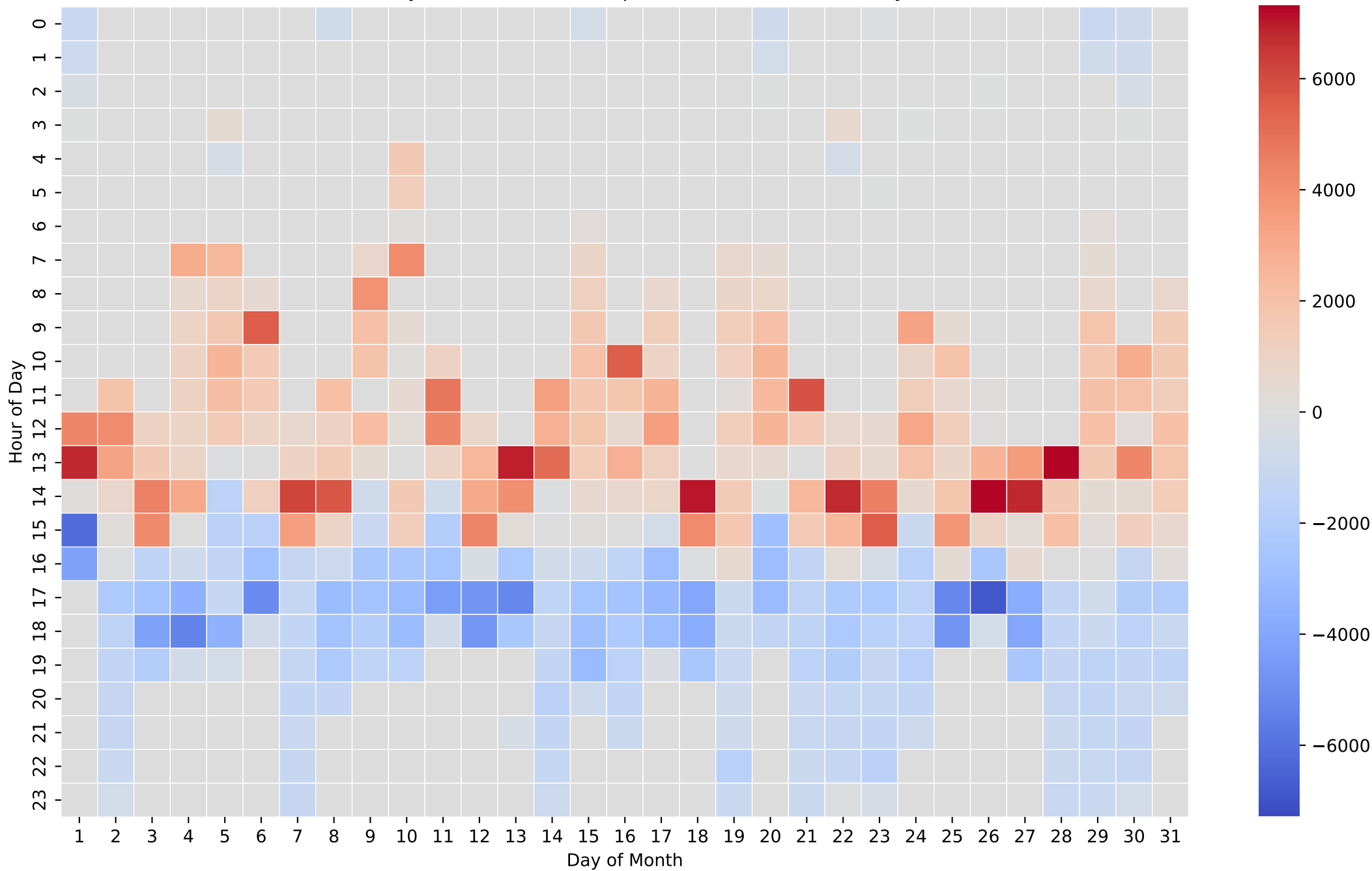
Battery Net Power Heatmap (Wh/Hour) - 12kWh - May
