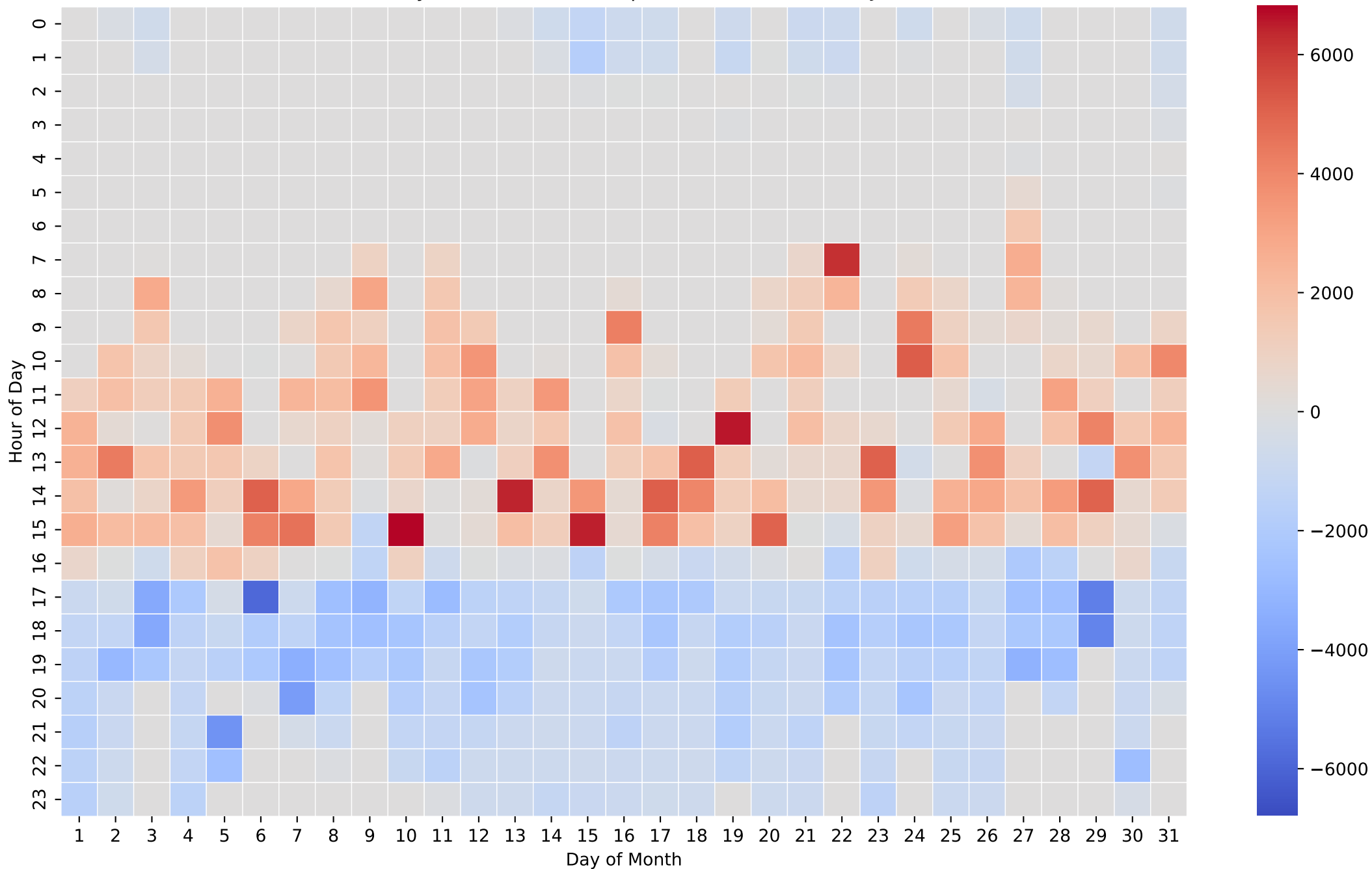
Battery Net Power Heatmap (Wh/Hour) - 12kWh - Jul
