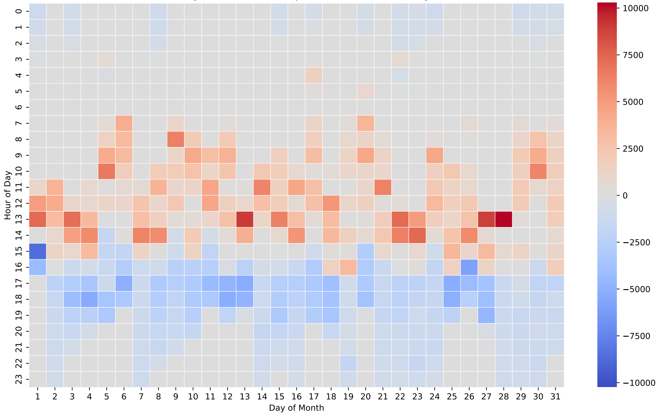
Battery Net Power Heatmap (Wh/Hour) - 15kWh - May
