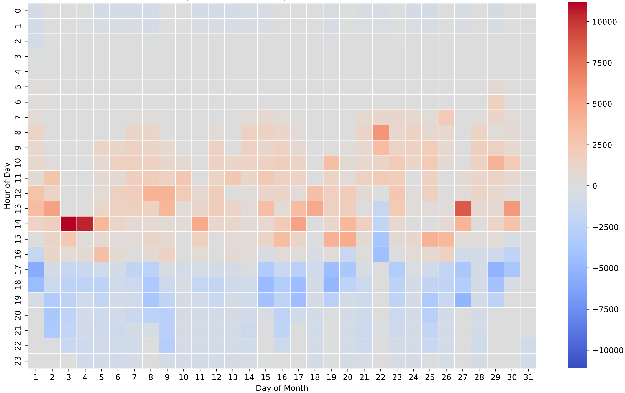
Battery Net Power Heatmap (Wh/Hour) - 15kWh - Jun
