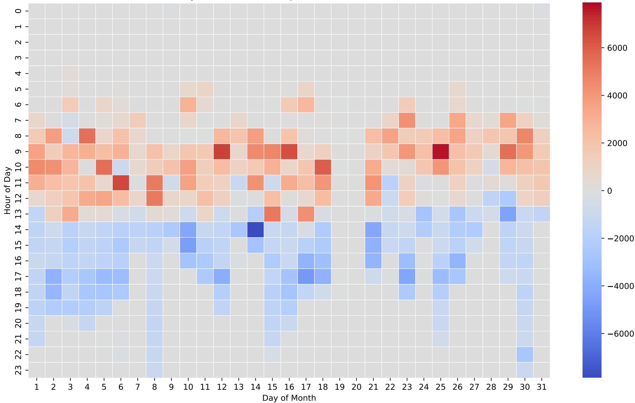
Battery Net Power Heatmap (Wh/Hour) - 15kWh - Oct
