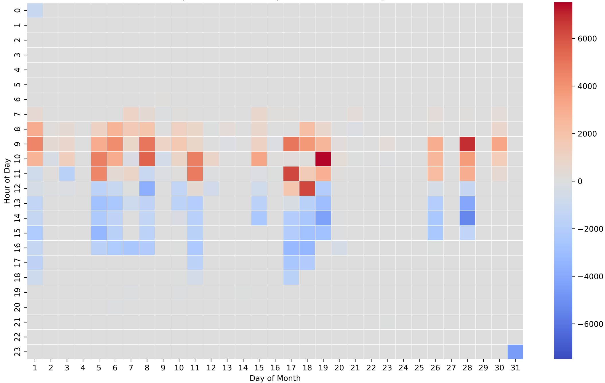
Battery Net Power Heatmap (Wh/Hour) - 15kWh - Jan
