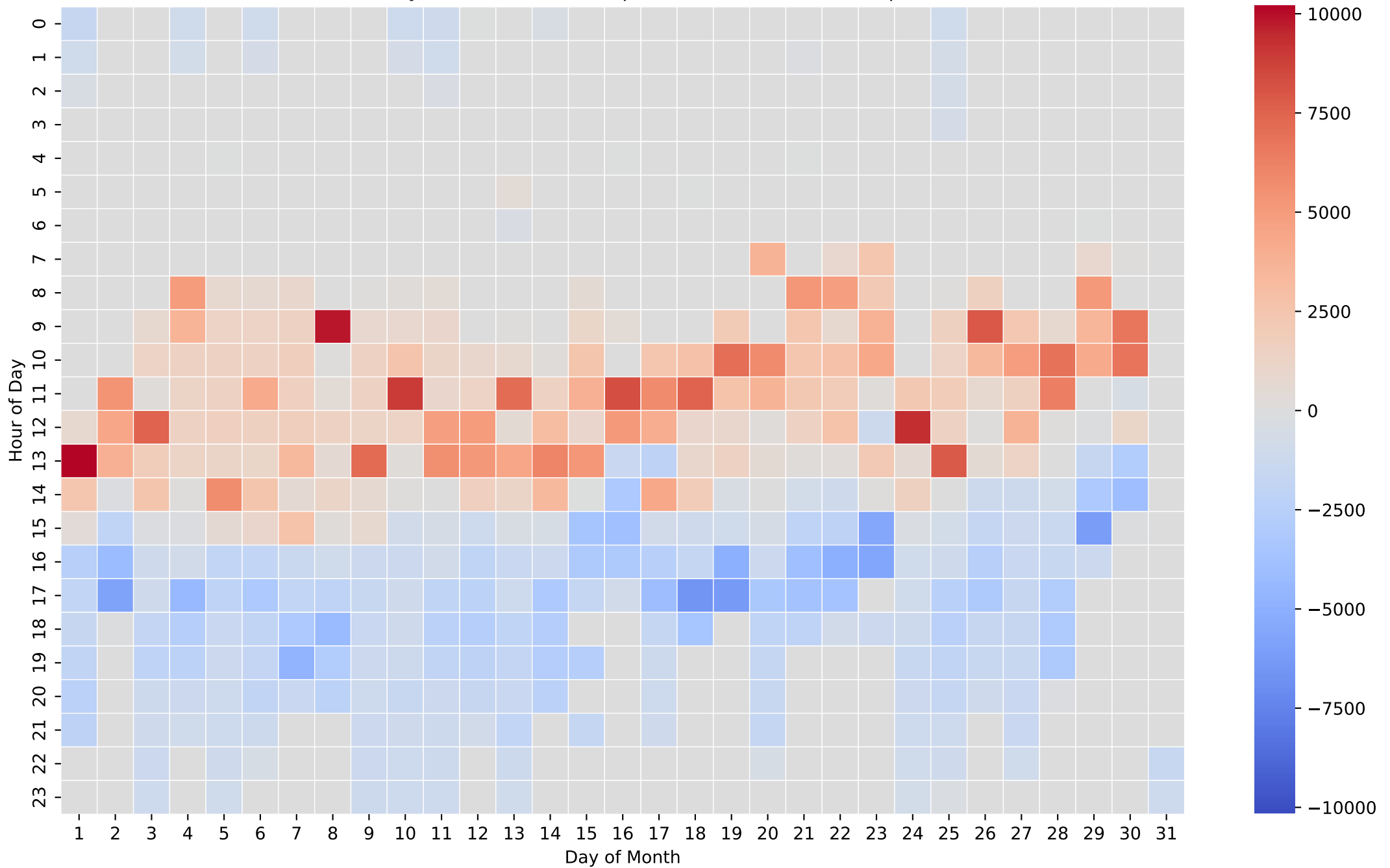
Battery Net Power Heatmap (Wh/Hour) - 15kWh - Sep
