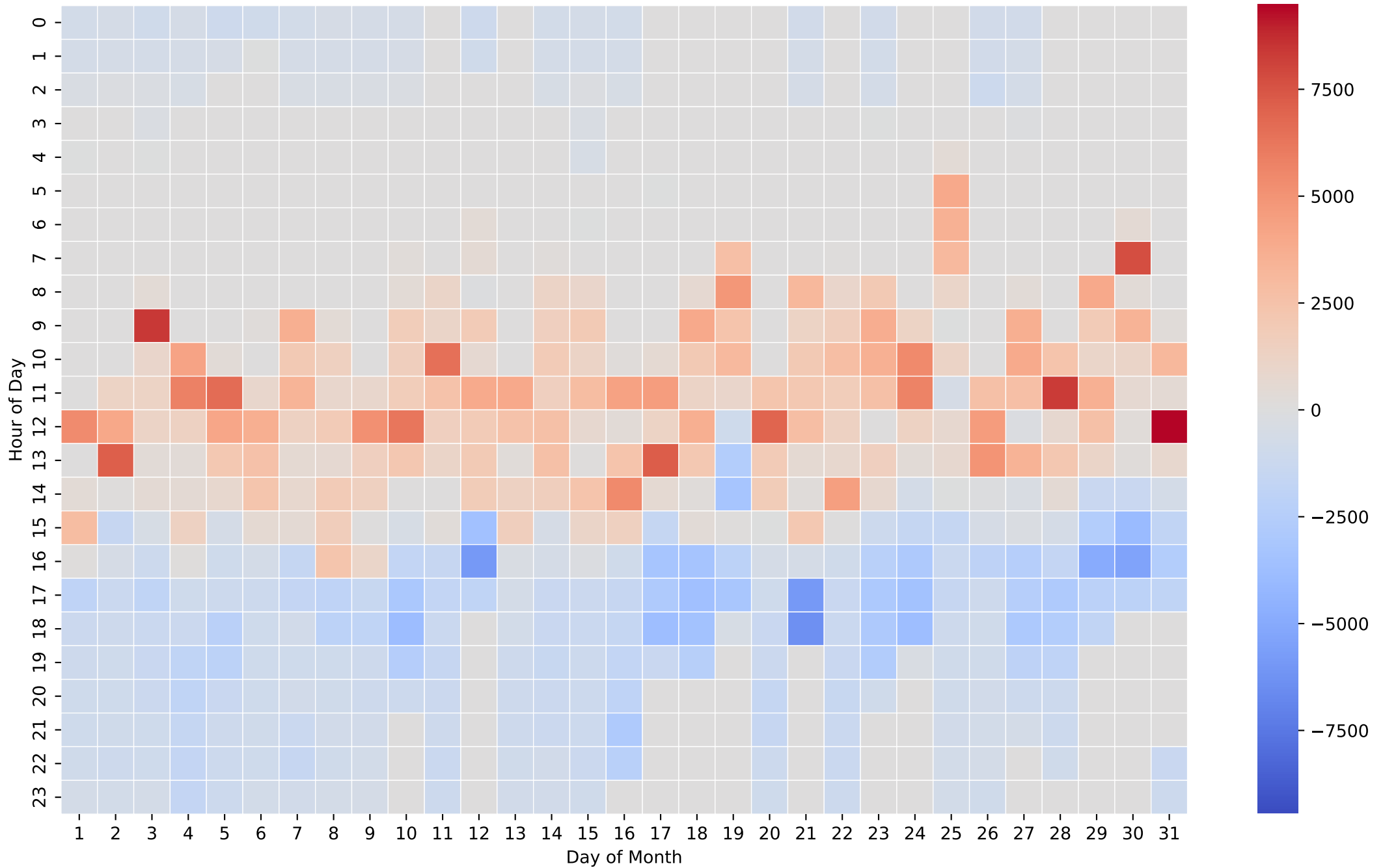
Battery Net Power Heatmap (Wh/Hour) - 15kWh - Aug
