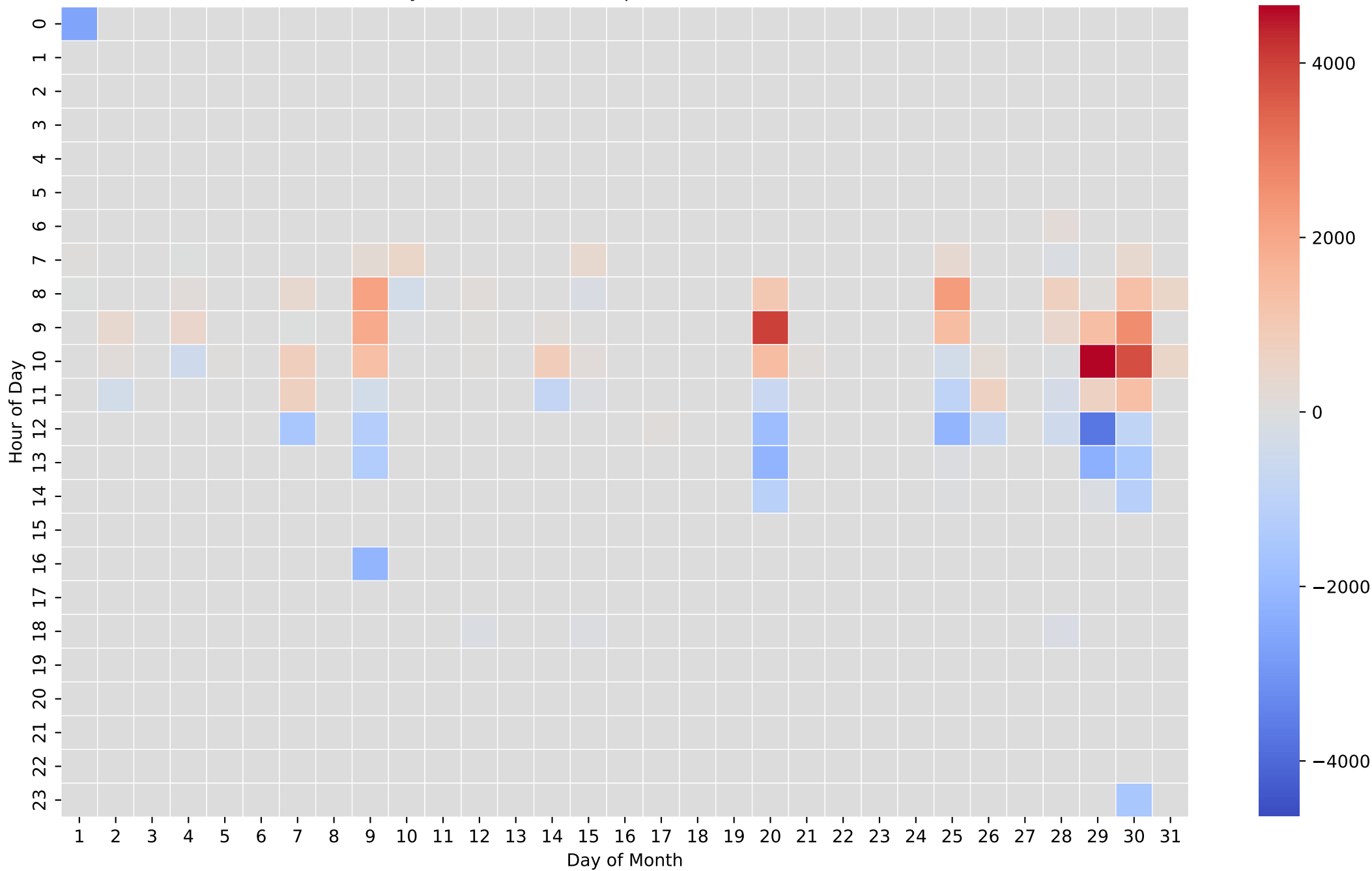
Battery Net Power Heatmap (Wh/Hour) - 15kWh - Dec
