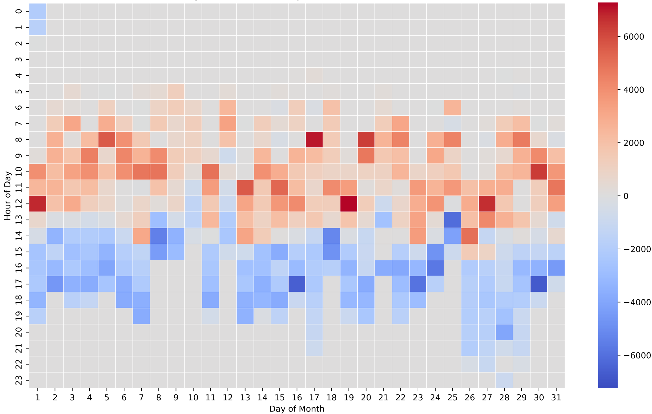
Battery Net Power Heatmap (Wh/Hour) - 15kWh - Mar
