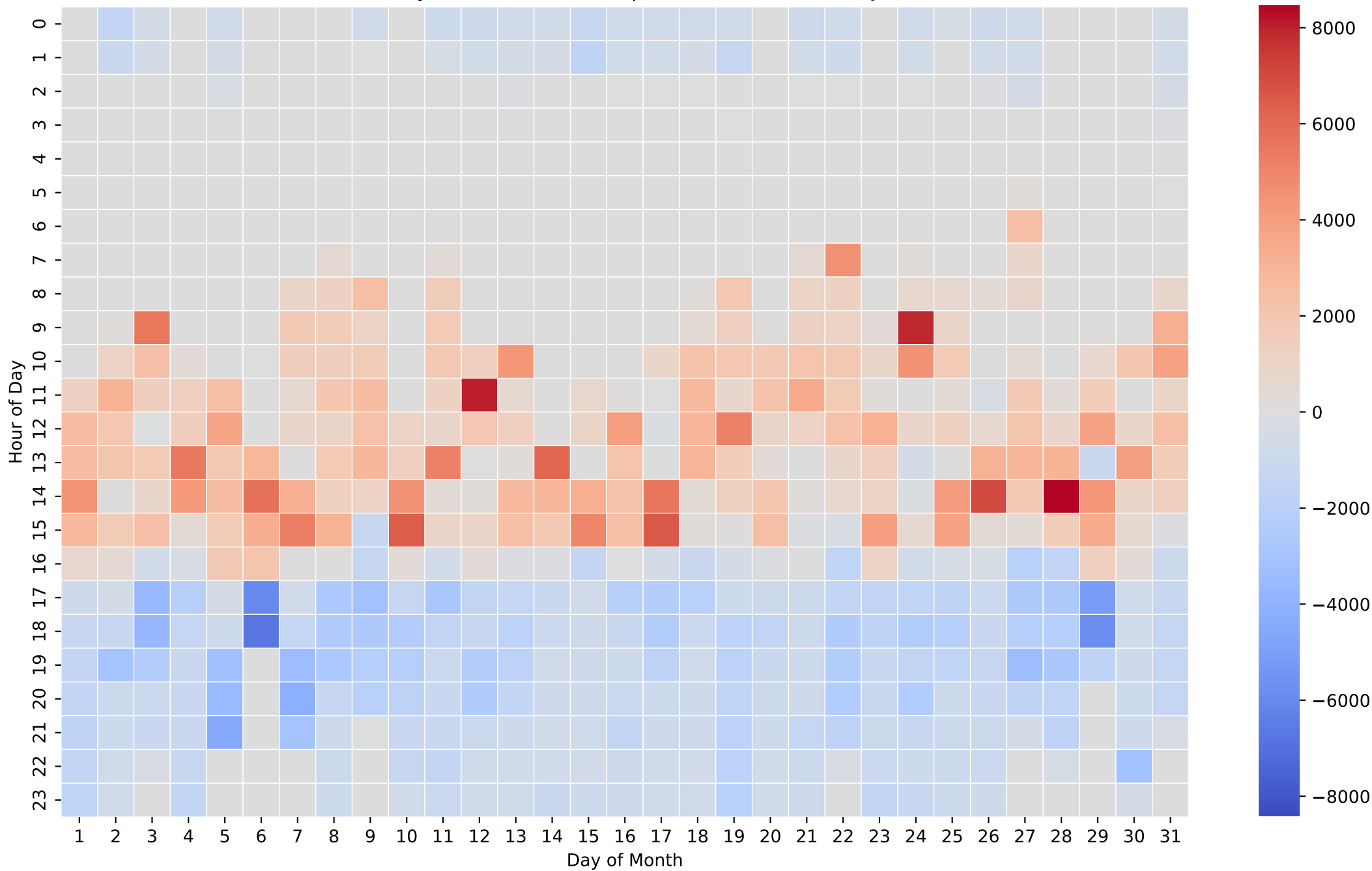
Battery Net Power Heatmap (Wh/Hour) - 15kWh - Jul
