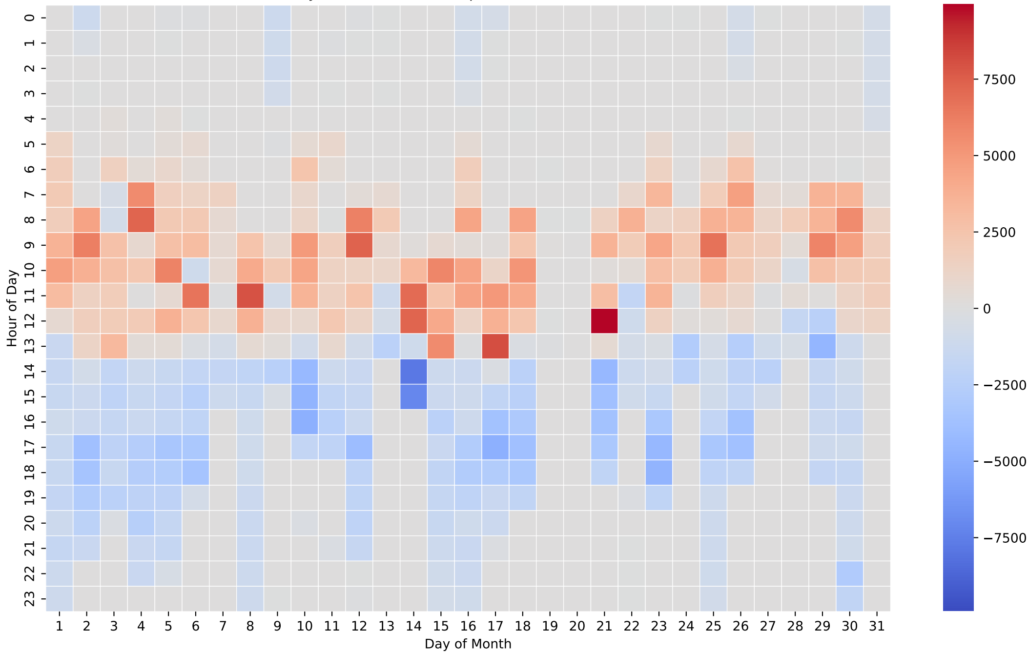
Battery Net Power Heatmap (Wh/Hour) - 20kWh - Oct
