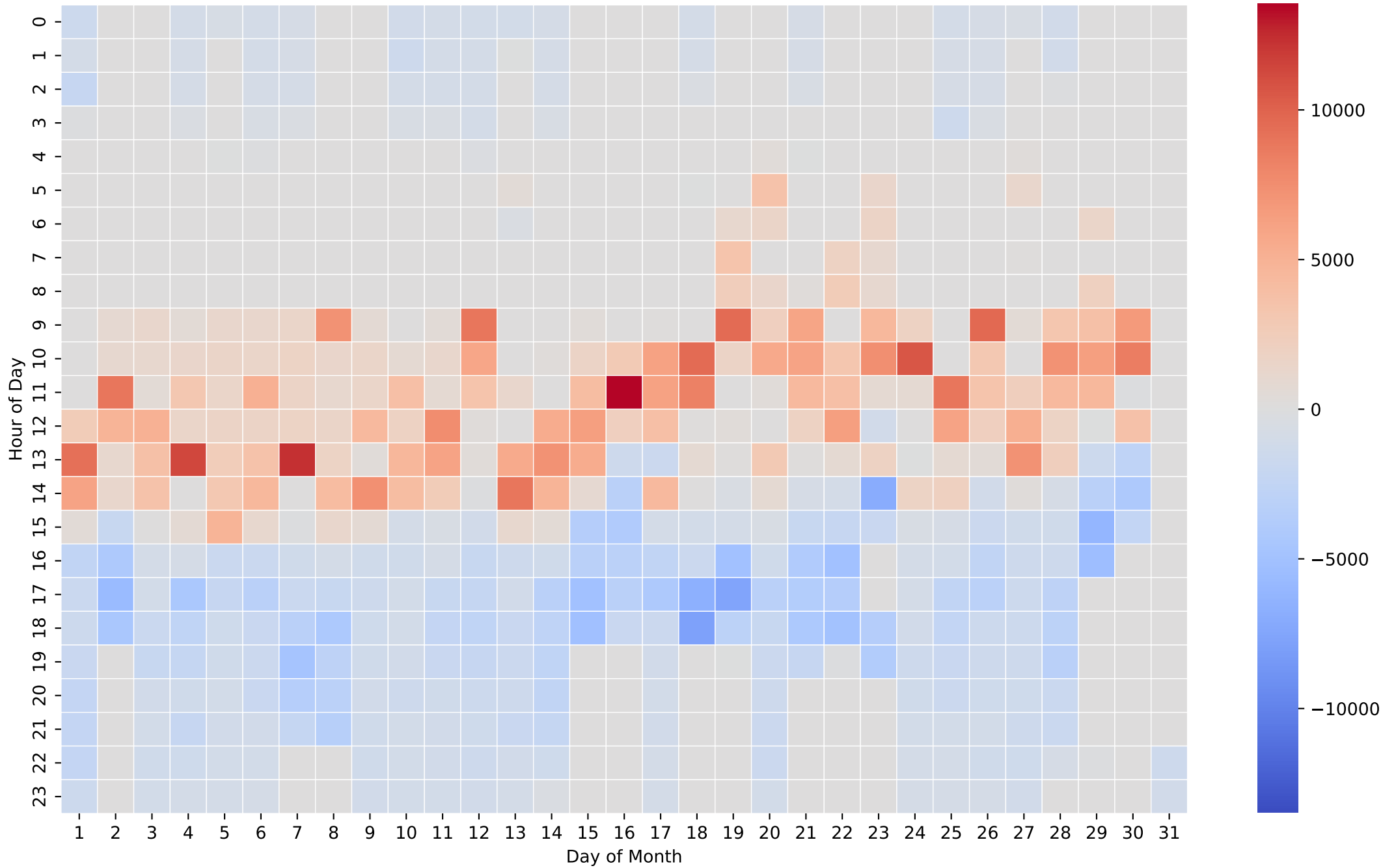
Battery Net Power Heatmap (Wh/Hour) - 20kWh - Sep
