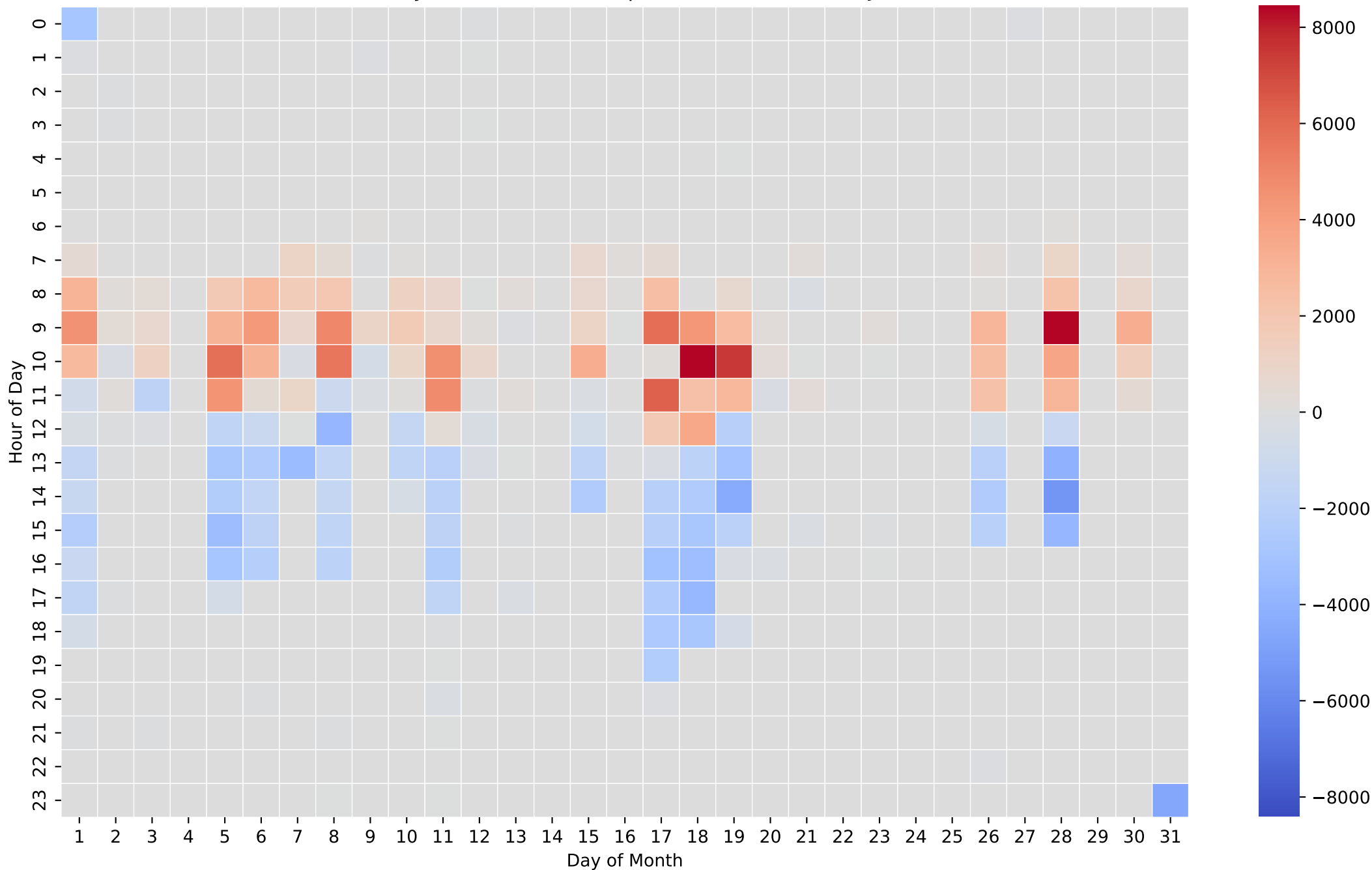
Battery Net Power Heatmap (Wh/Hour) - 20kWh - Jan
