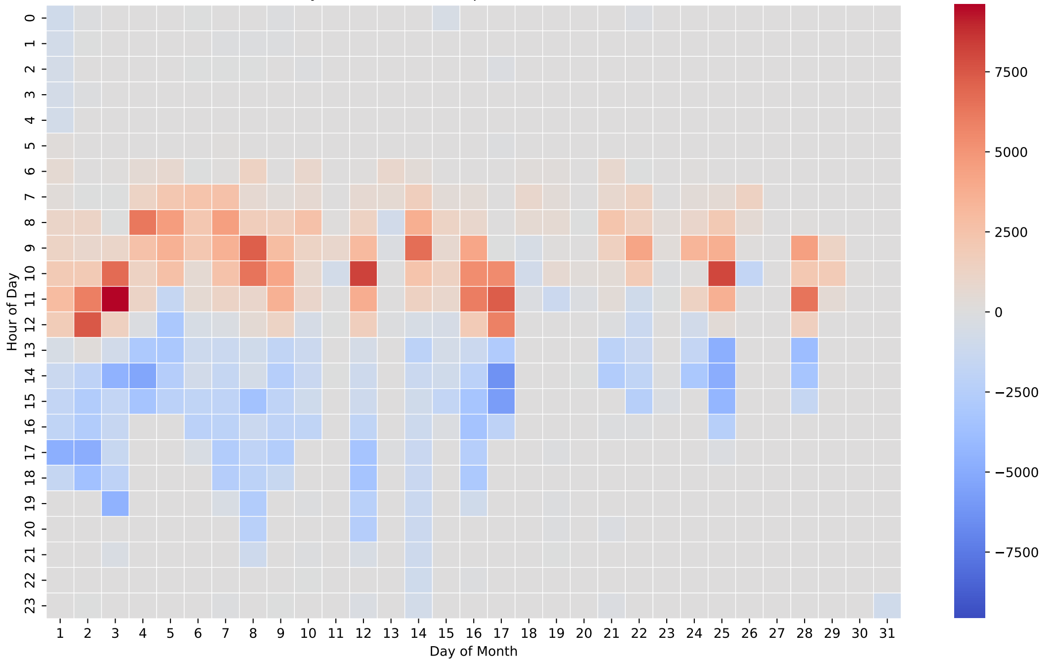
Battery Net Power Heatmap (Wh/Hour) - 20kWh - Nov
