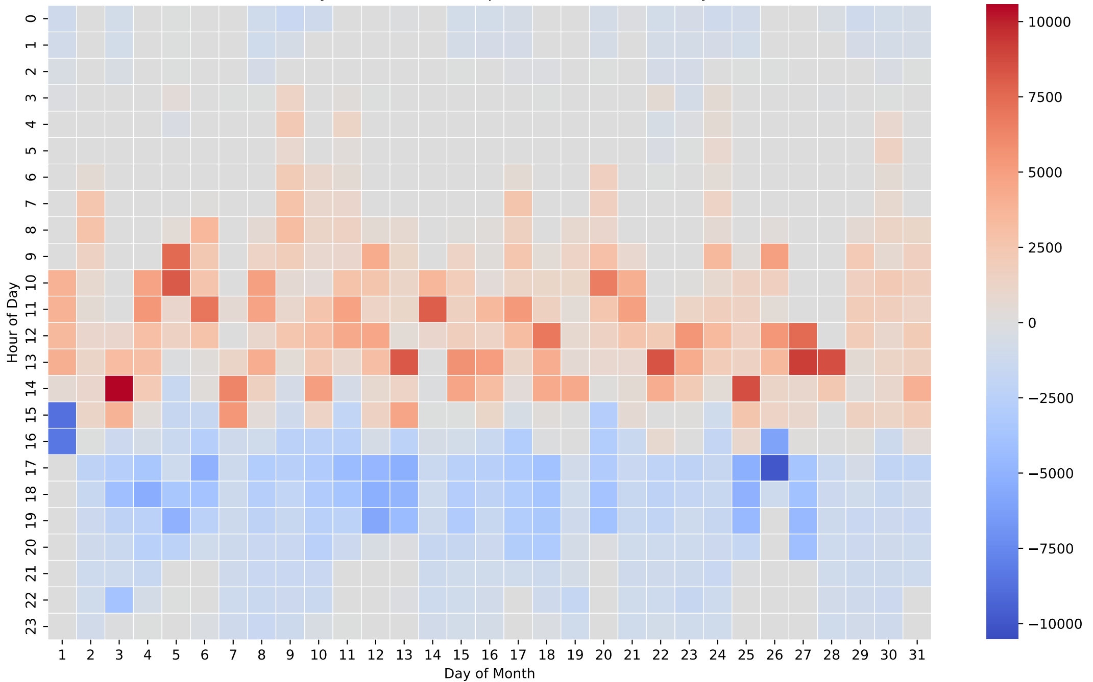
Battery Net Power Heatmap (Wh/Hour) - 20kWh - May
