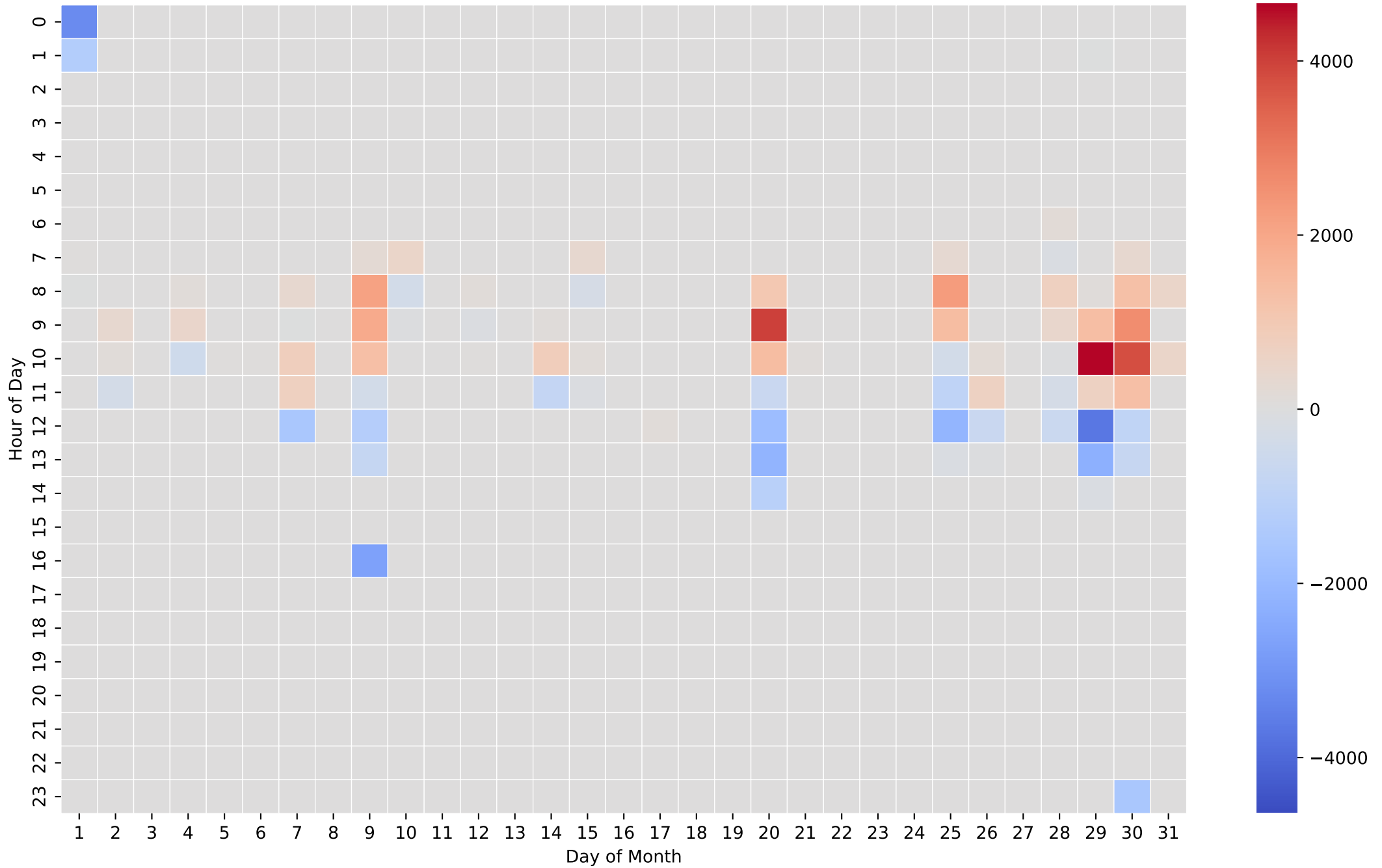
Battery Net Power Heatmap (Wh/Hour) - 20kWh - Dec
