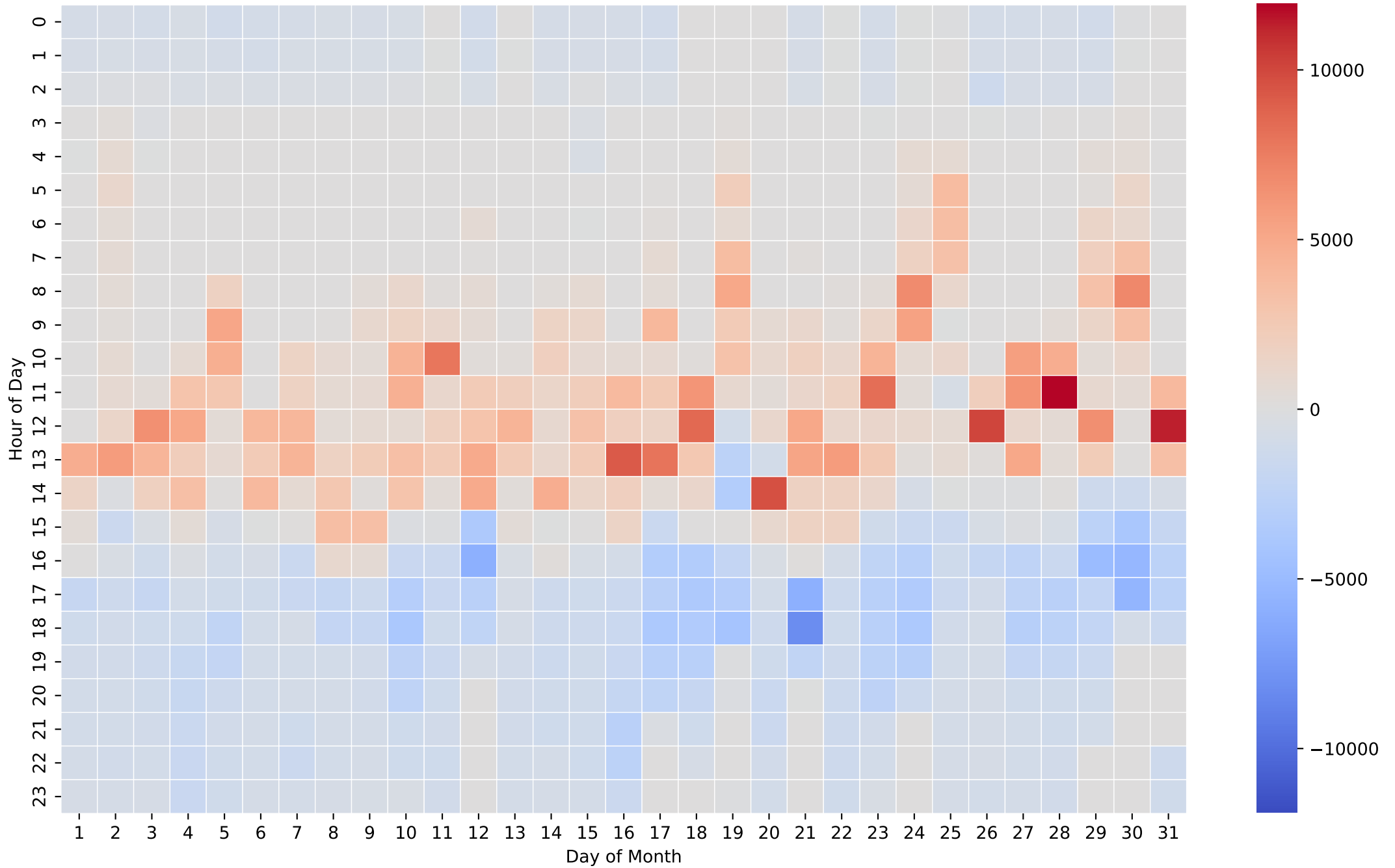
Battery Net Power Heatmap (Wh/Hour) - 20kWh - Aug
