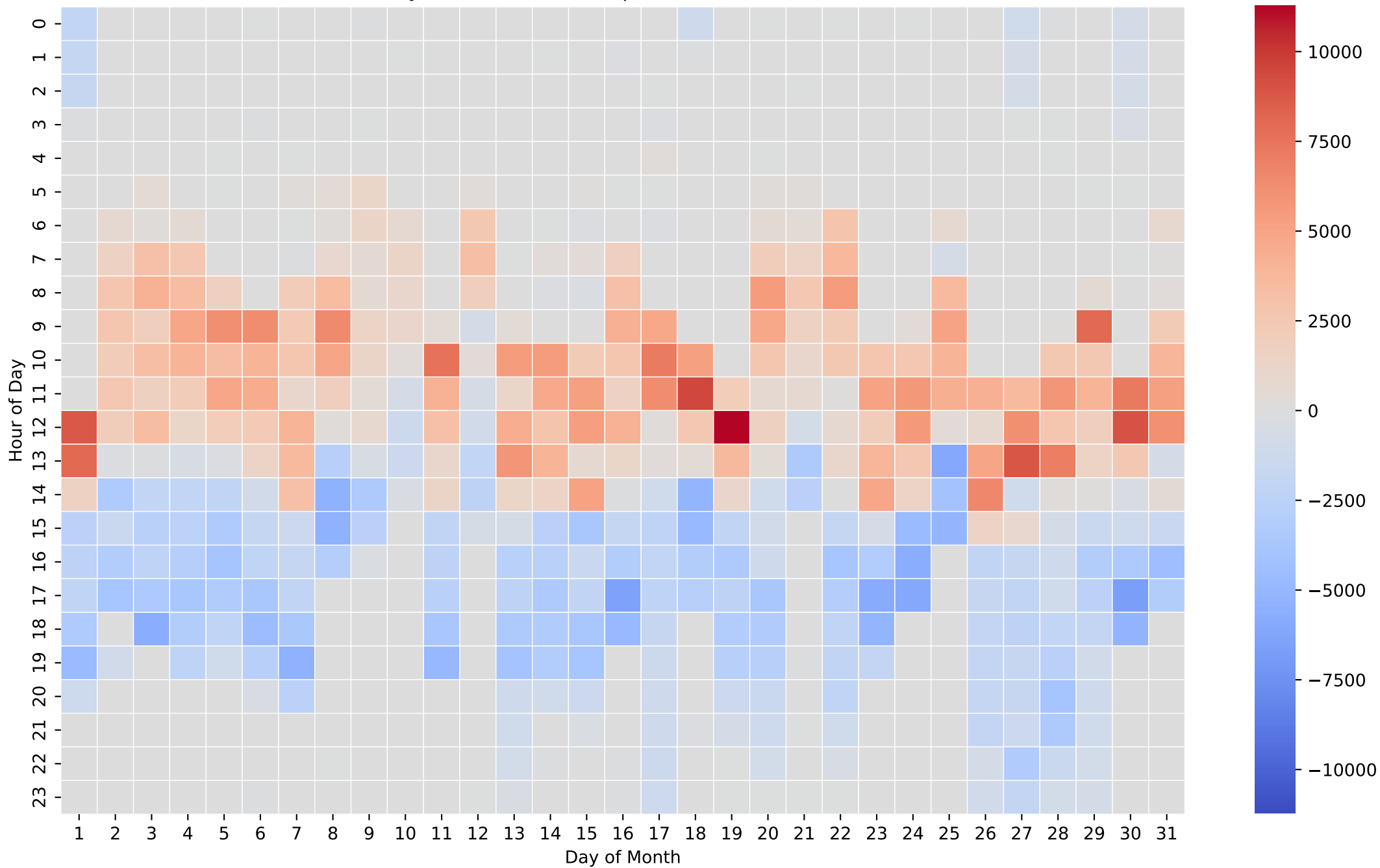
Battery Net Power Heatmap (Wh/Hour) - 20kWh - Mar
