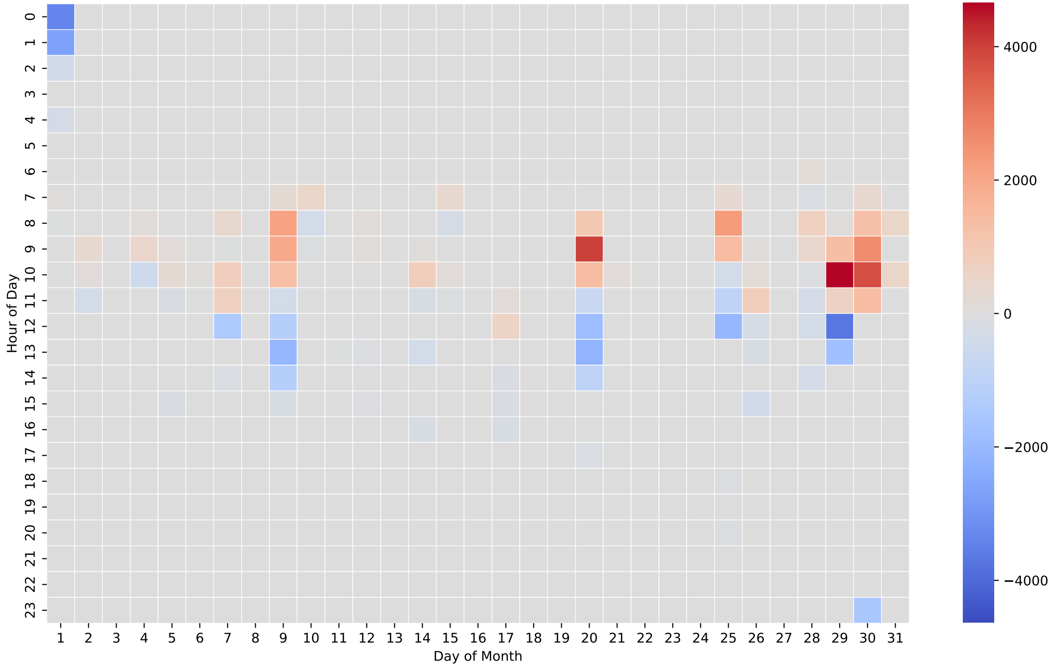
Battery Net Power Heatmap (Wh/Hour) - 26kWh - Dec
