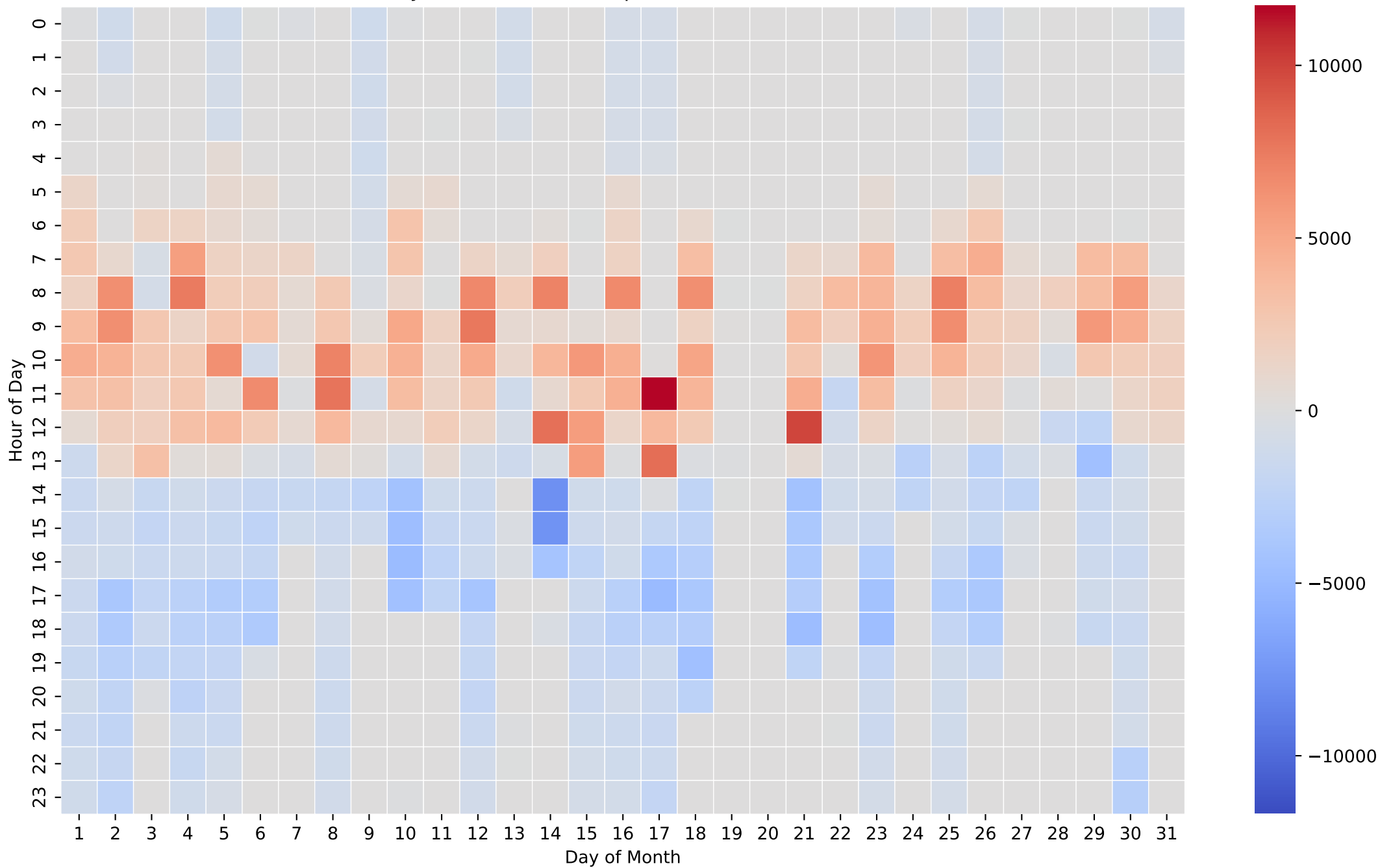
Battery Net Power Heatmap (Wh/Hour) - 26kWh - Oct
