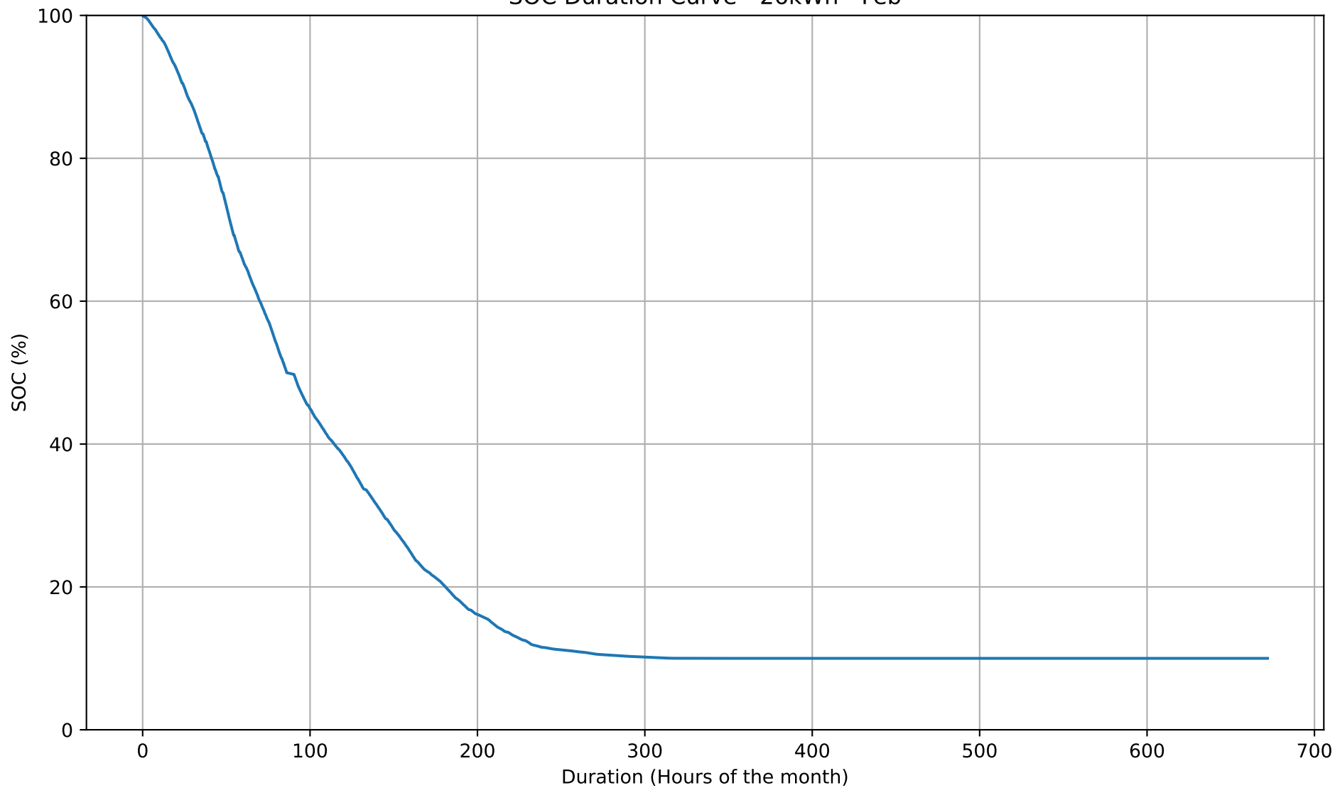
SOC Duration Curve - 26kWh - Feb
