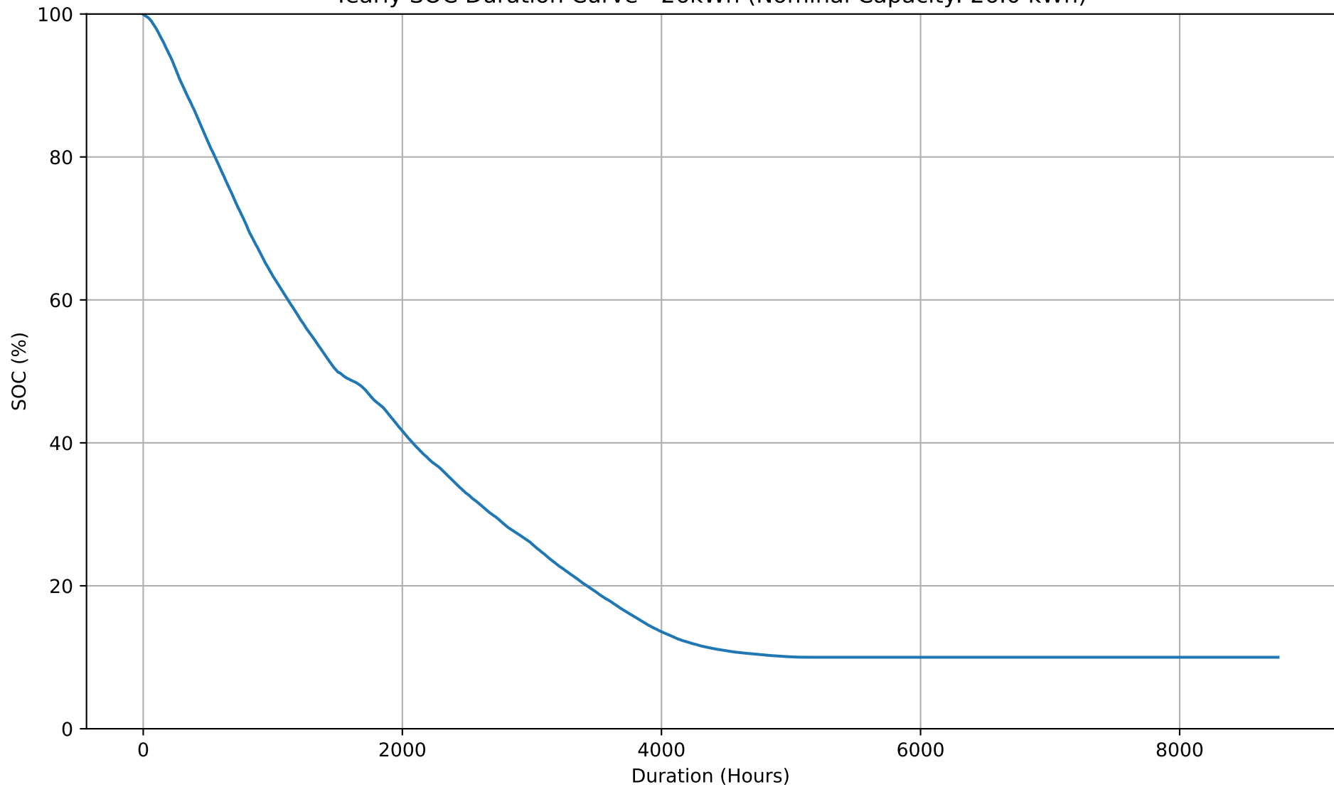
Yearly SOC Duration Curve - 26kWh (Nominal Capacity: 26.0 kWh)
