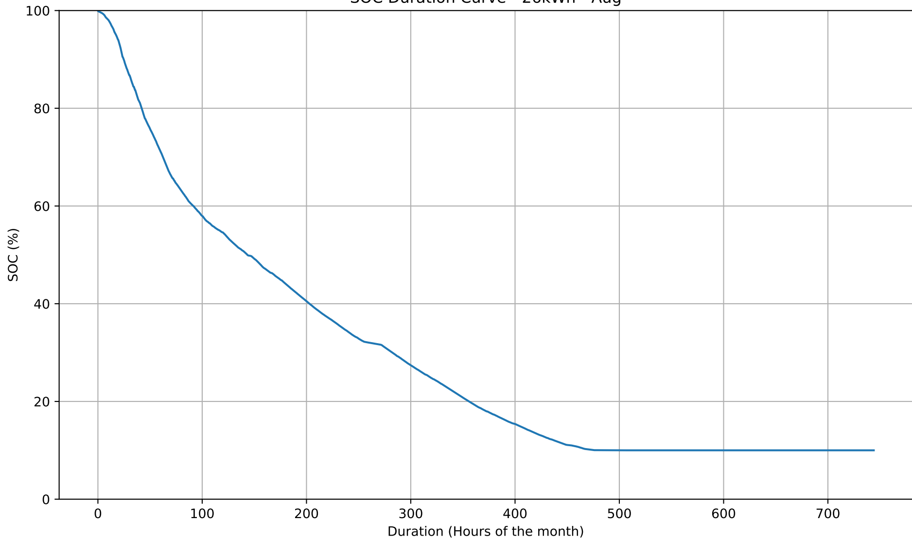
SOC Duration Curve - 26kWh - Aug
