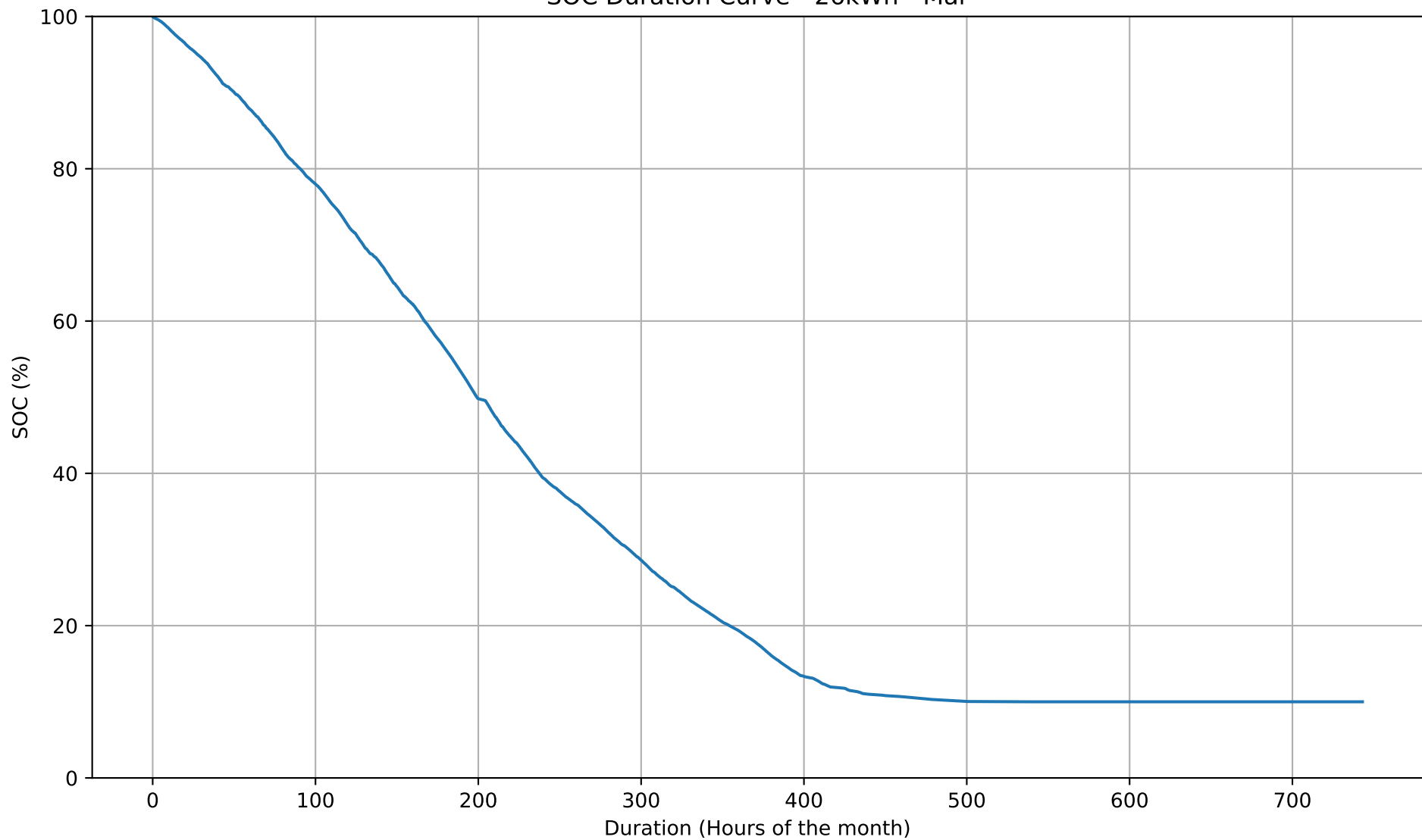
SOC Duration Curve - 26kWh - Mar
