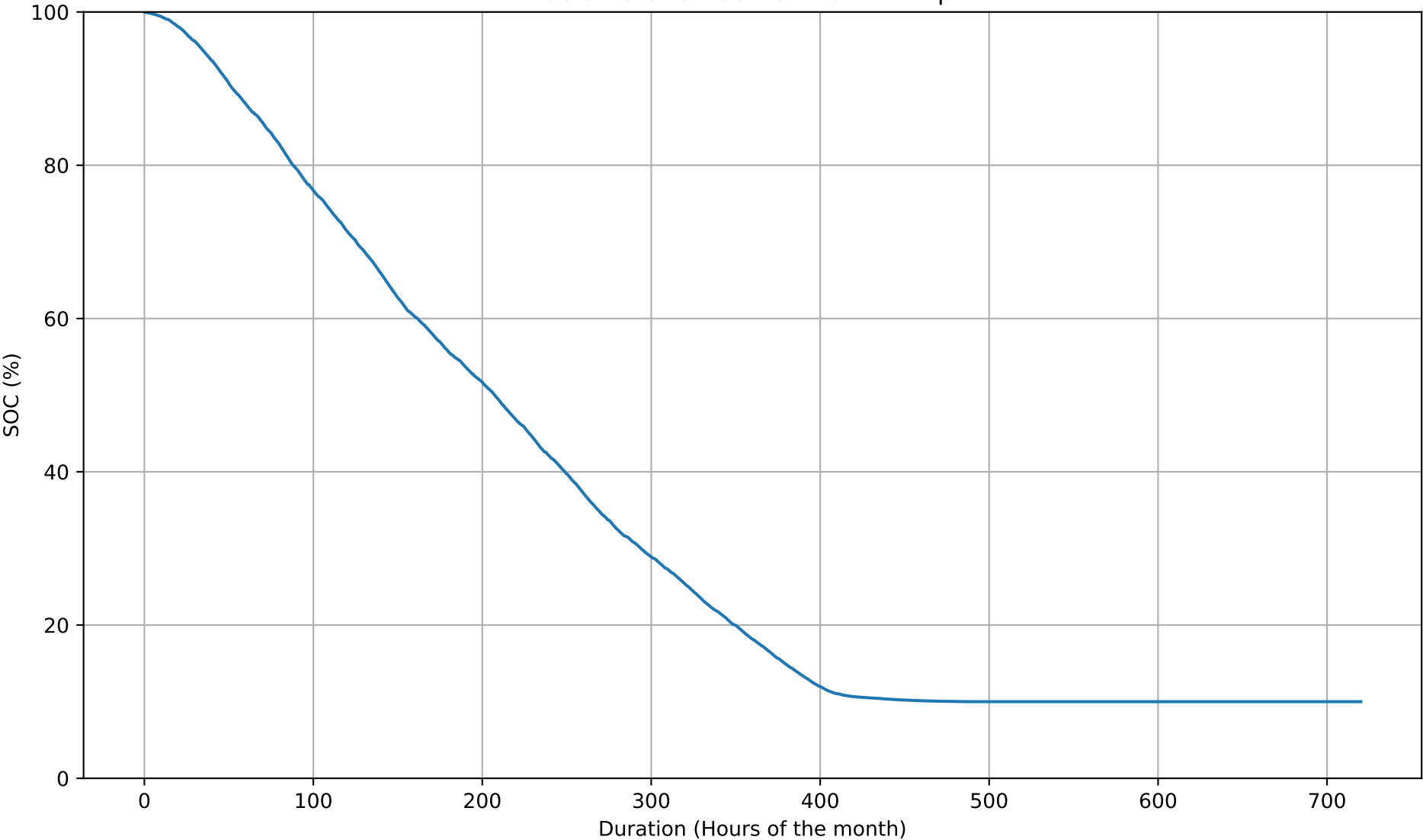
SOC Duration Curve - 26kWh - Apr
