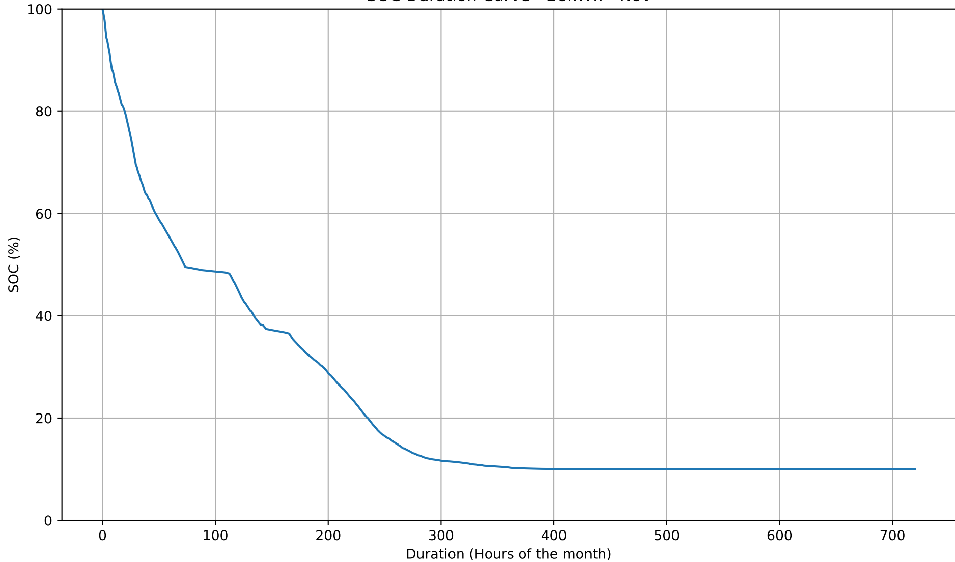
SOC Duration Curve - 26kWh - Nov
