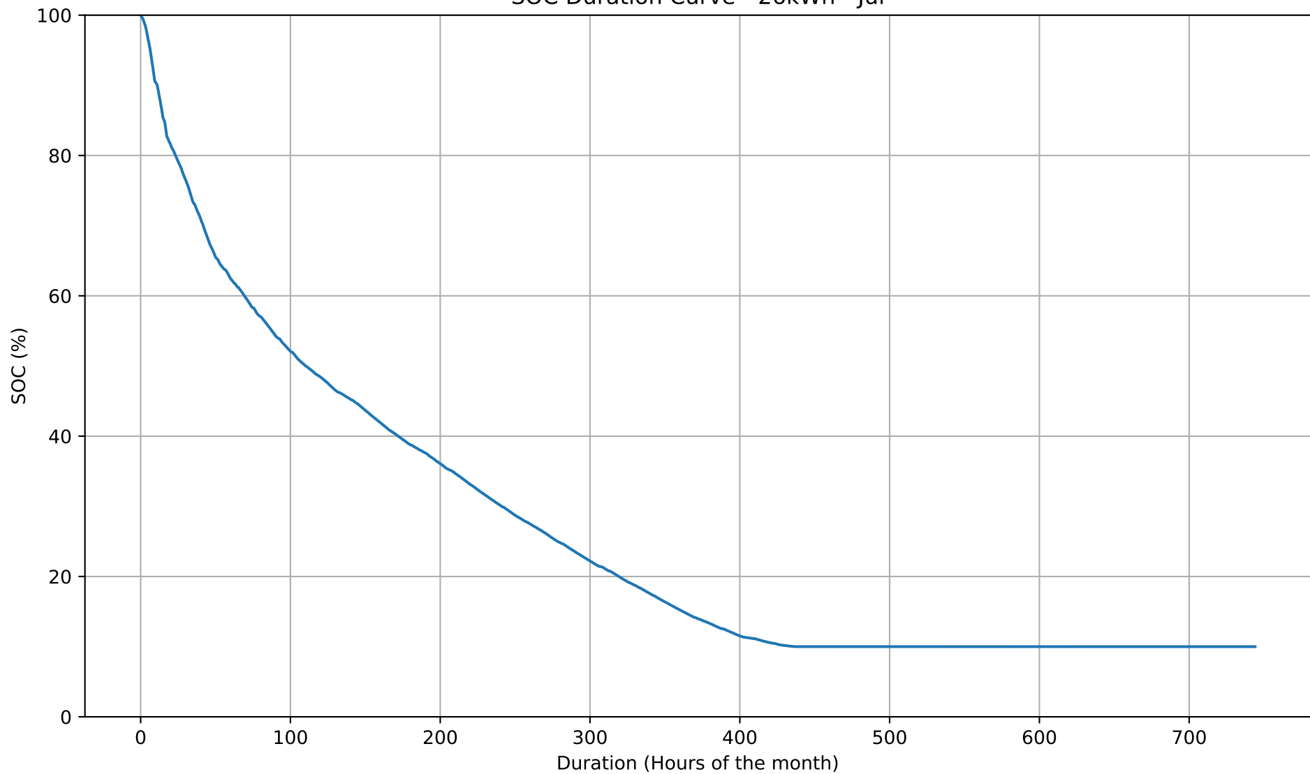
SOC Duration Curve - 26kWh - Jul
