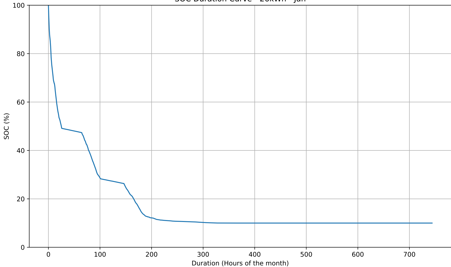
SOC Duration Curve - 26kWh - Jan
