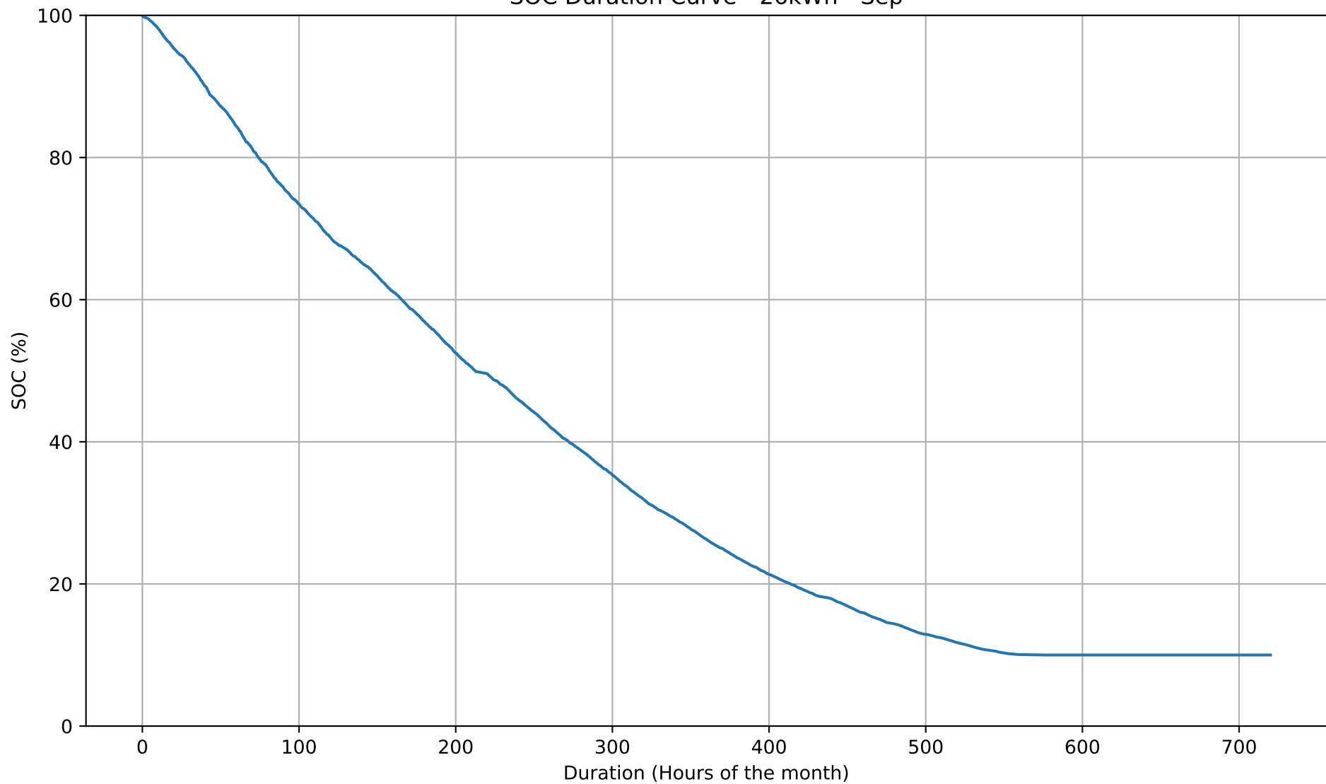
SOC Duration Curve - 26kWh - Sep
