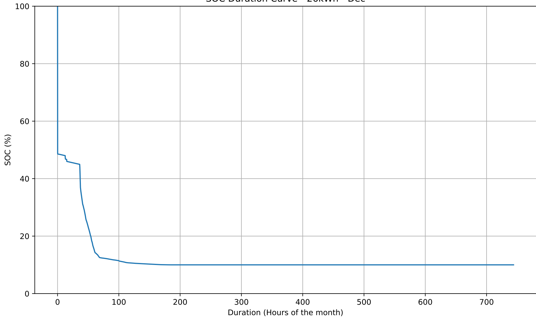
SOC Duration Curve - 26kWh - Dec
