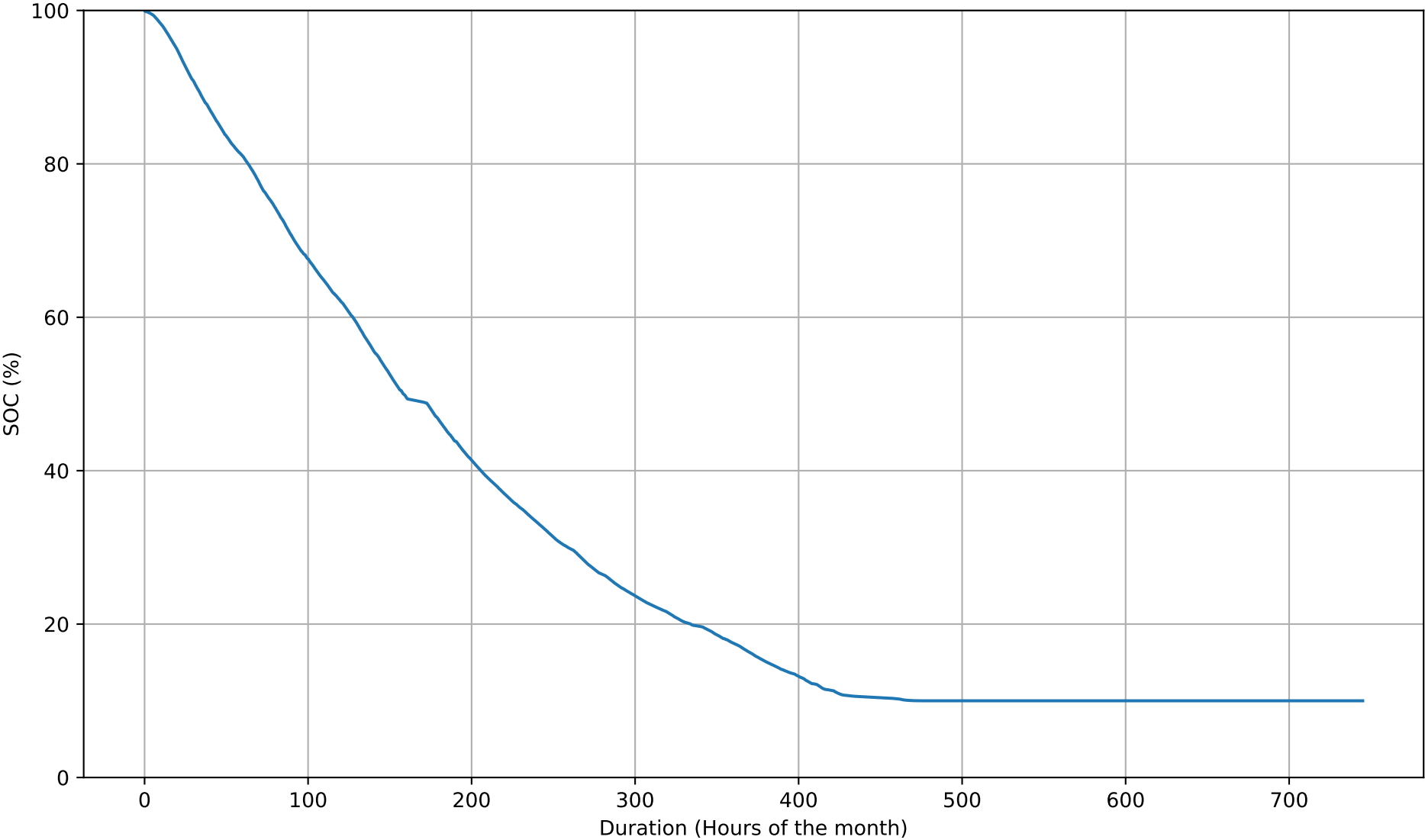
SOC Duration Curve - 26kWh - Oct
