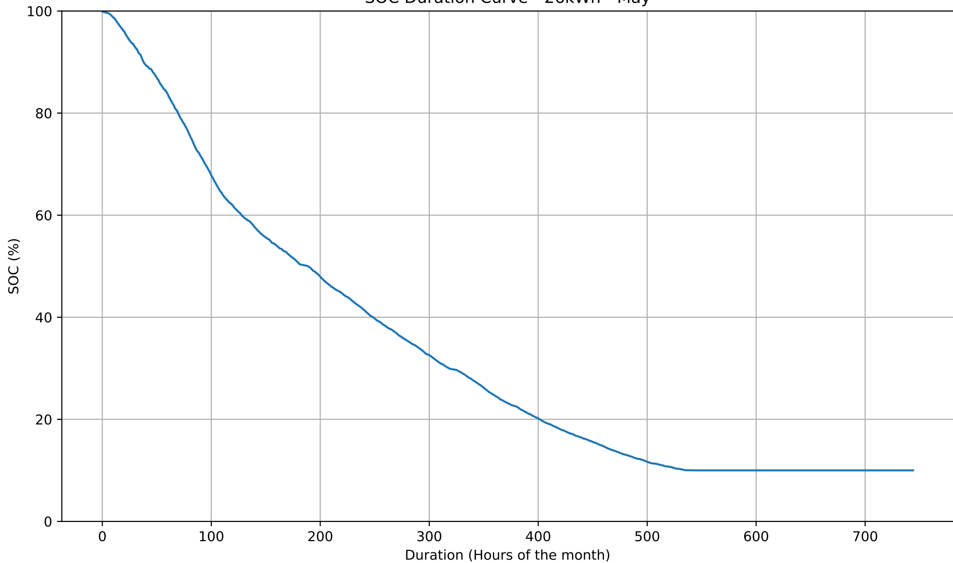
SOC Duration Curve - 26kWh - May
