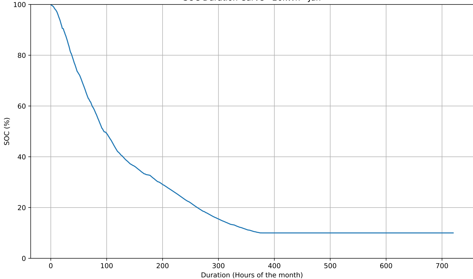
SOC Duration Curve - 26kWh - Jun
