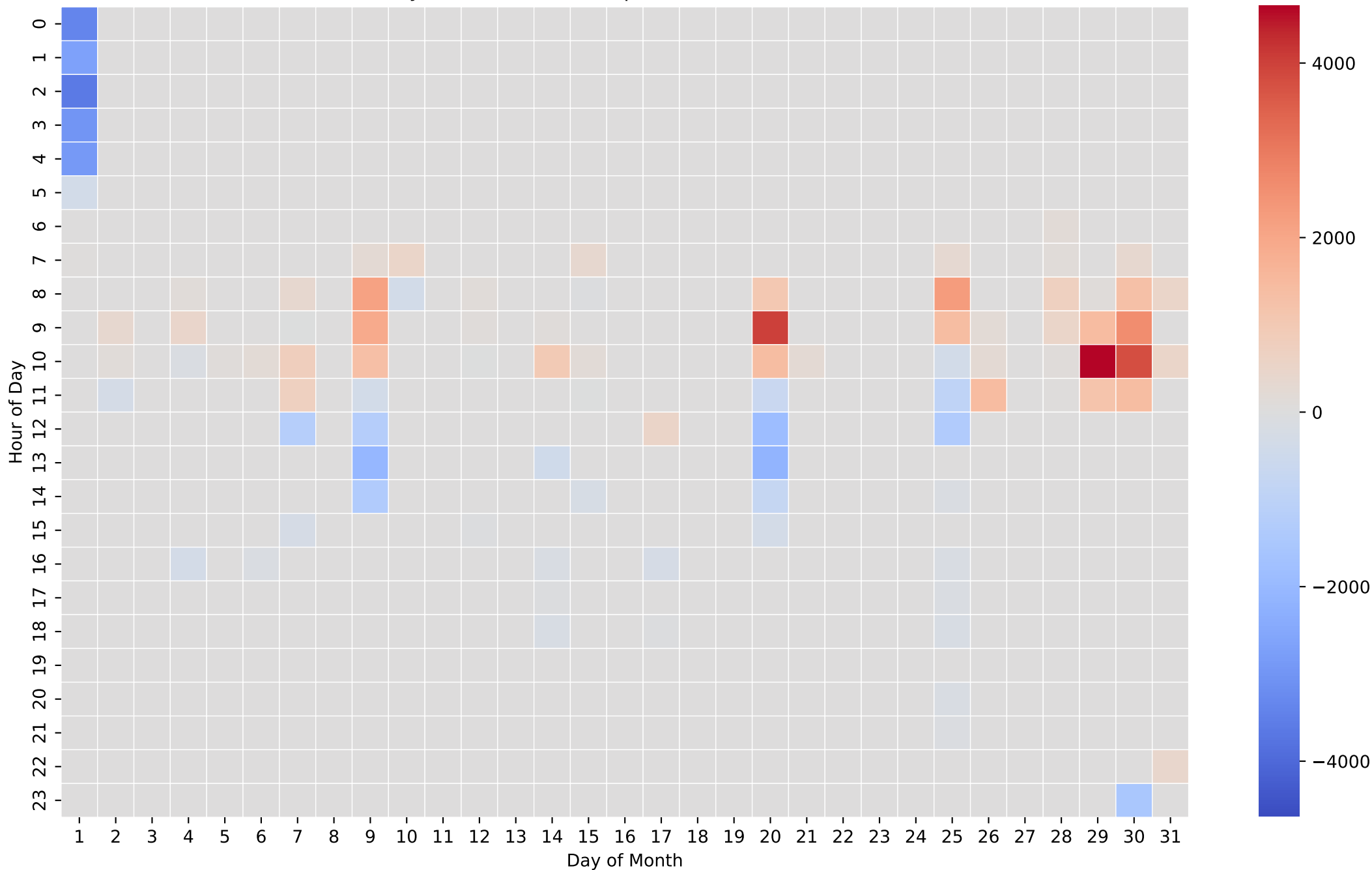
Battery Net Power Heatmap (Wh/Hour) - 50kWh - Dec
