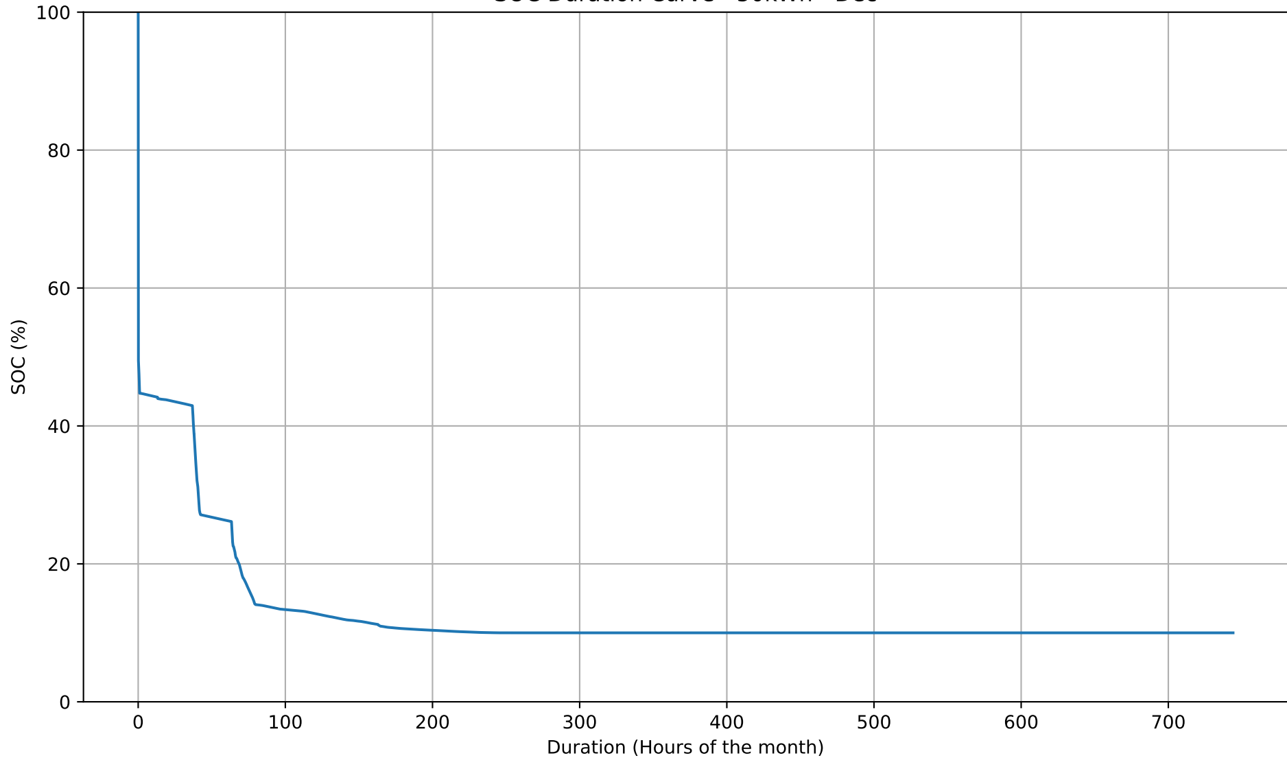
SOC Duration Curve - 50kWh - Dec
