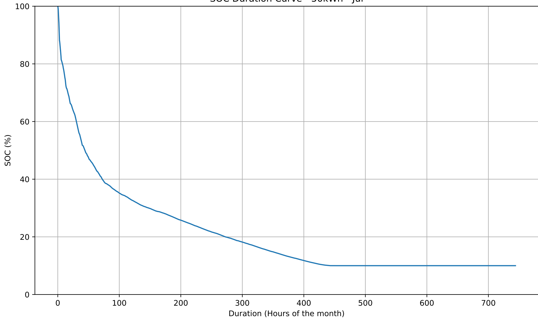
SOC Duration Curve - 50kWh - Jul
