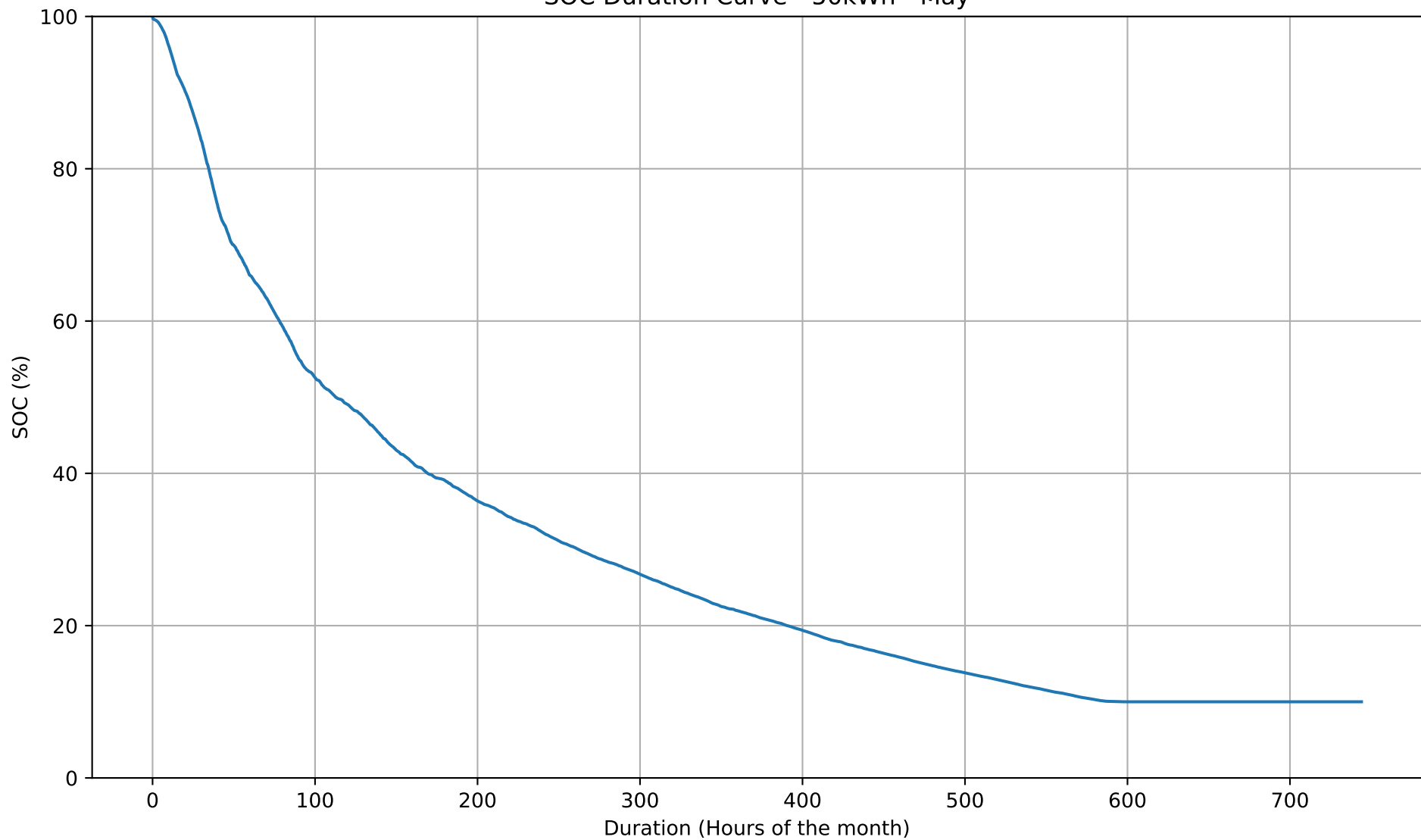
SOC Duration Curve - 50kWh - May
