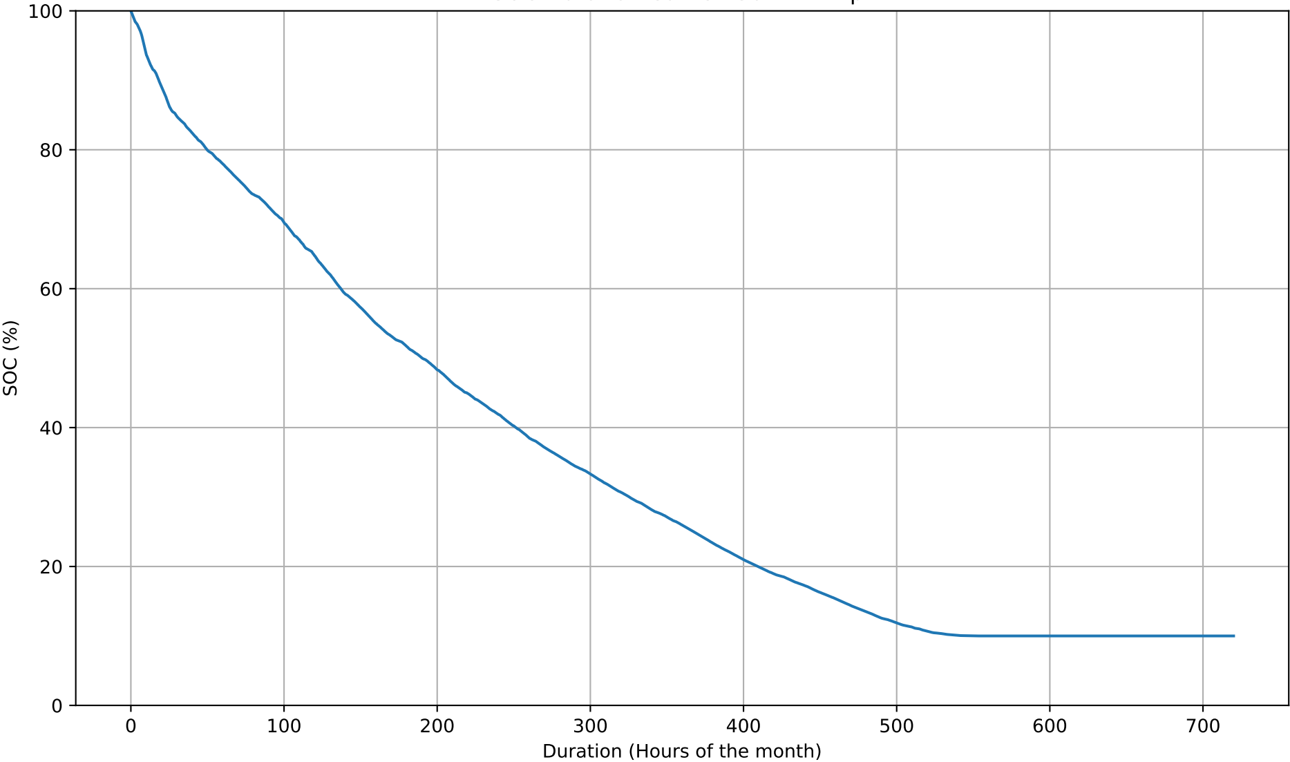
SOC Duration Curve - 50kWh - Apr
