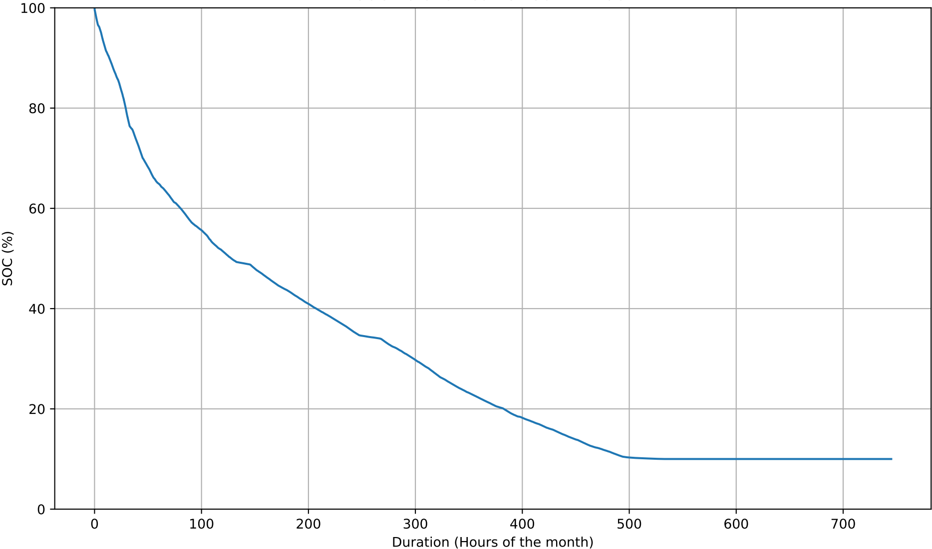
SOC Duration Curve - 50kWh - Oct
