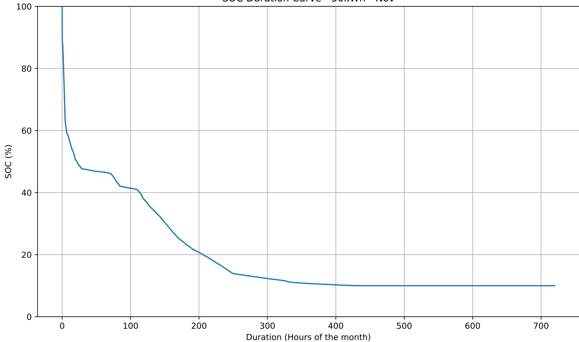
SOC Duration Curve - 50kWh - Nov
