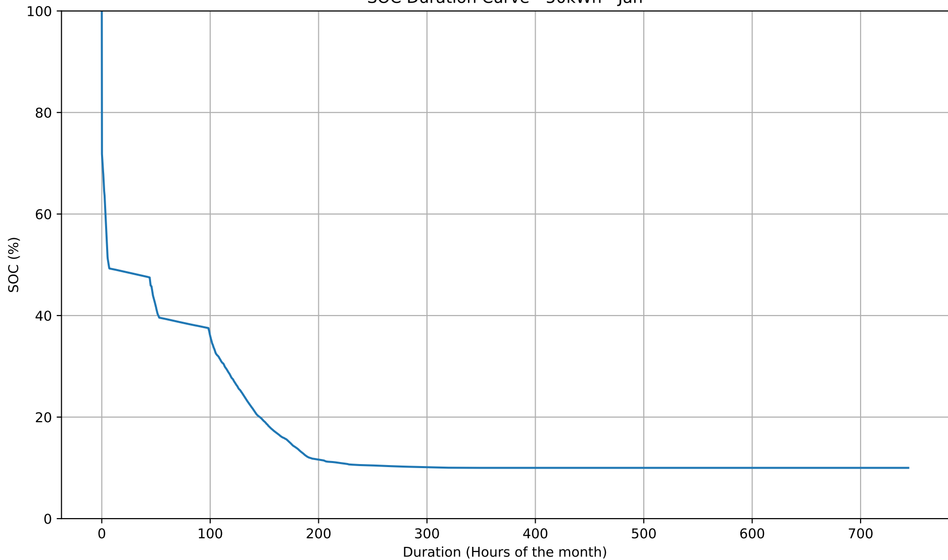
SOC Duration Curve - 50kWh - Jan
