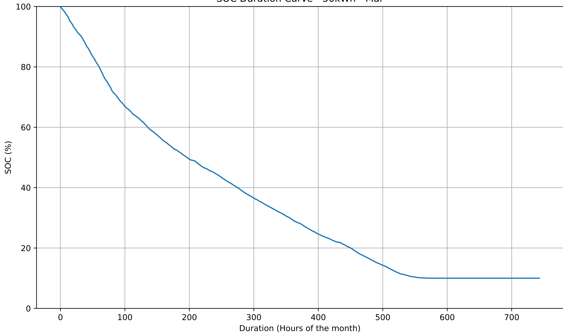
SOC Duration Curve - 50kWh - Mar
