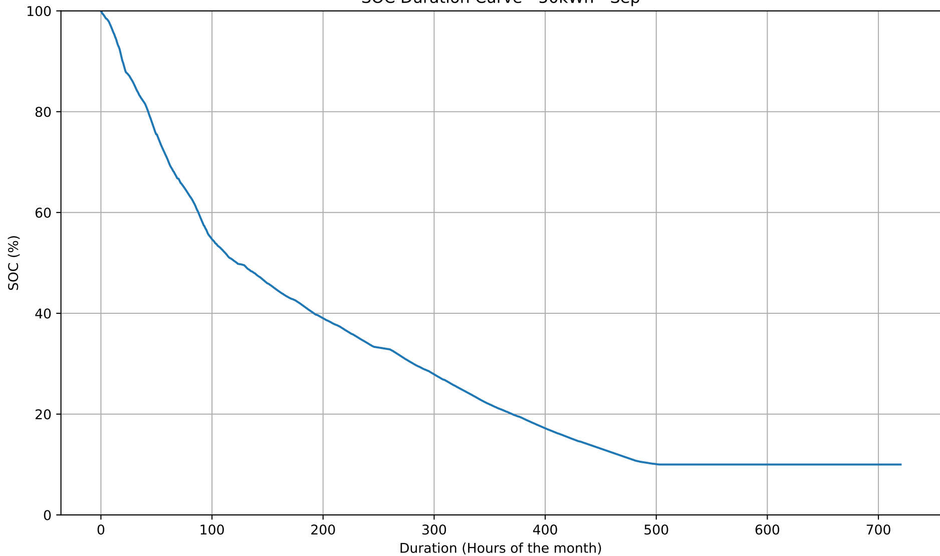
SOC Duration Curve - 50kWh - Sep
