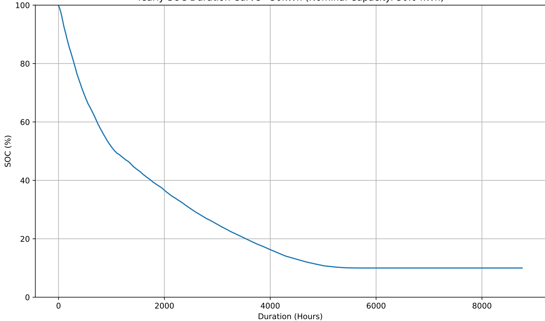
Yearly SOC Duration Curve - 50kWh (Nominal Capacity: 50.0 kWh)
