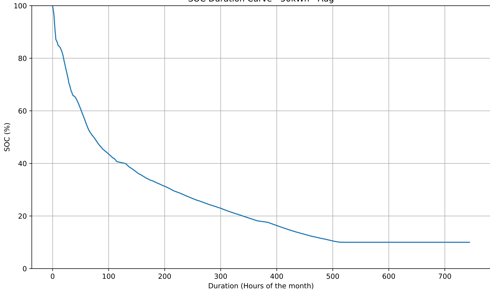
SOC Duration Curve - 50kWh - Aug
