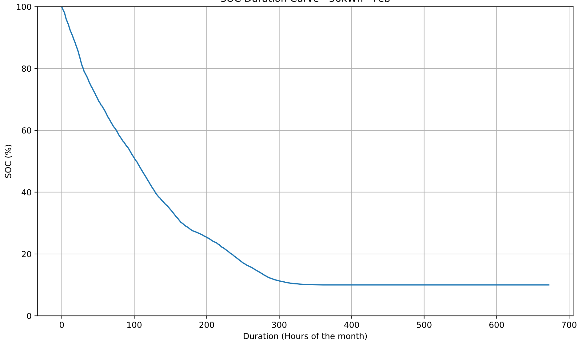
SOC Duration Curve - 50kWh - Feb
