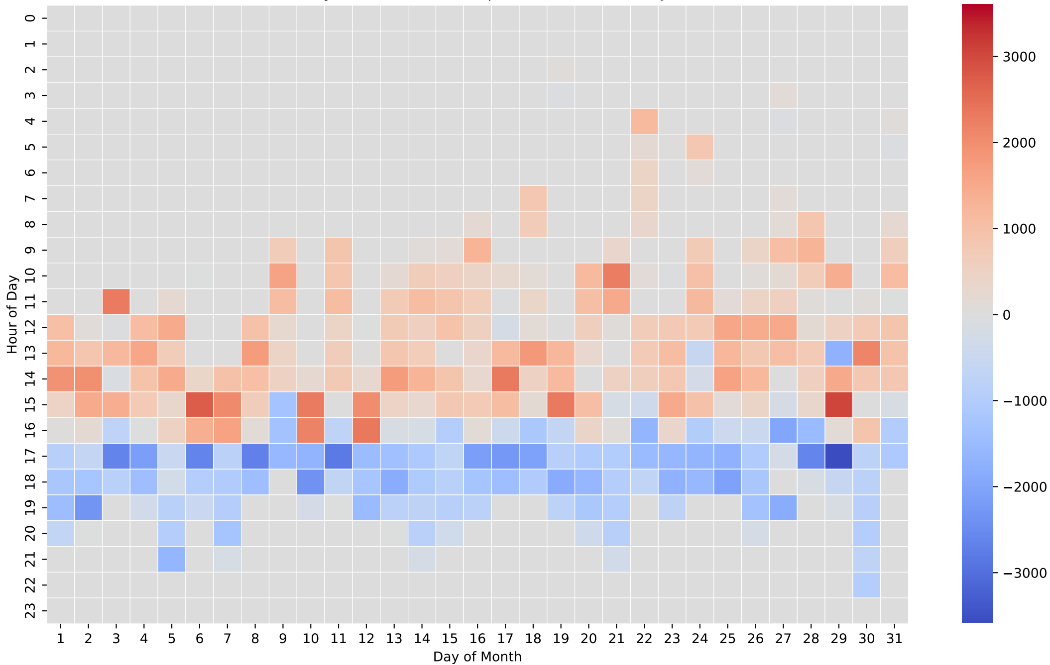
Battery Net Power Heatmap (Wh/Hour) - 5kWh - Jul
