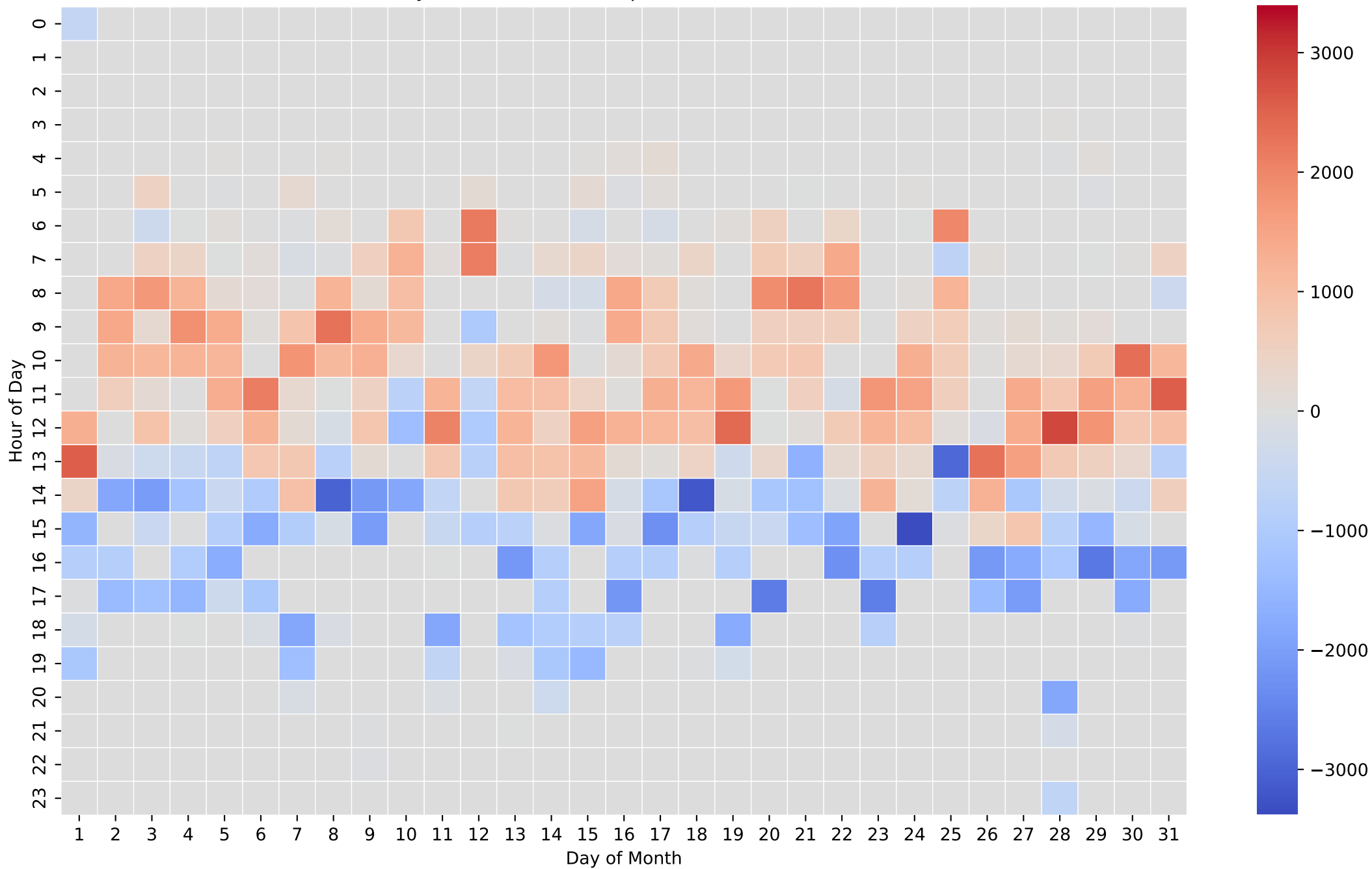
Battery Net Power Heatmap (Wh/Hour) - 5kWh - Mar
