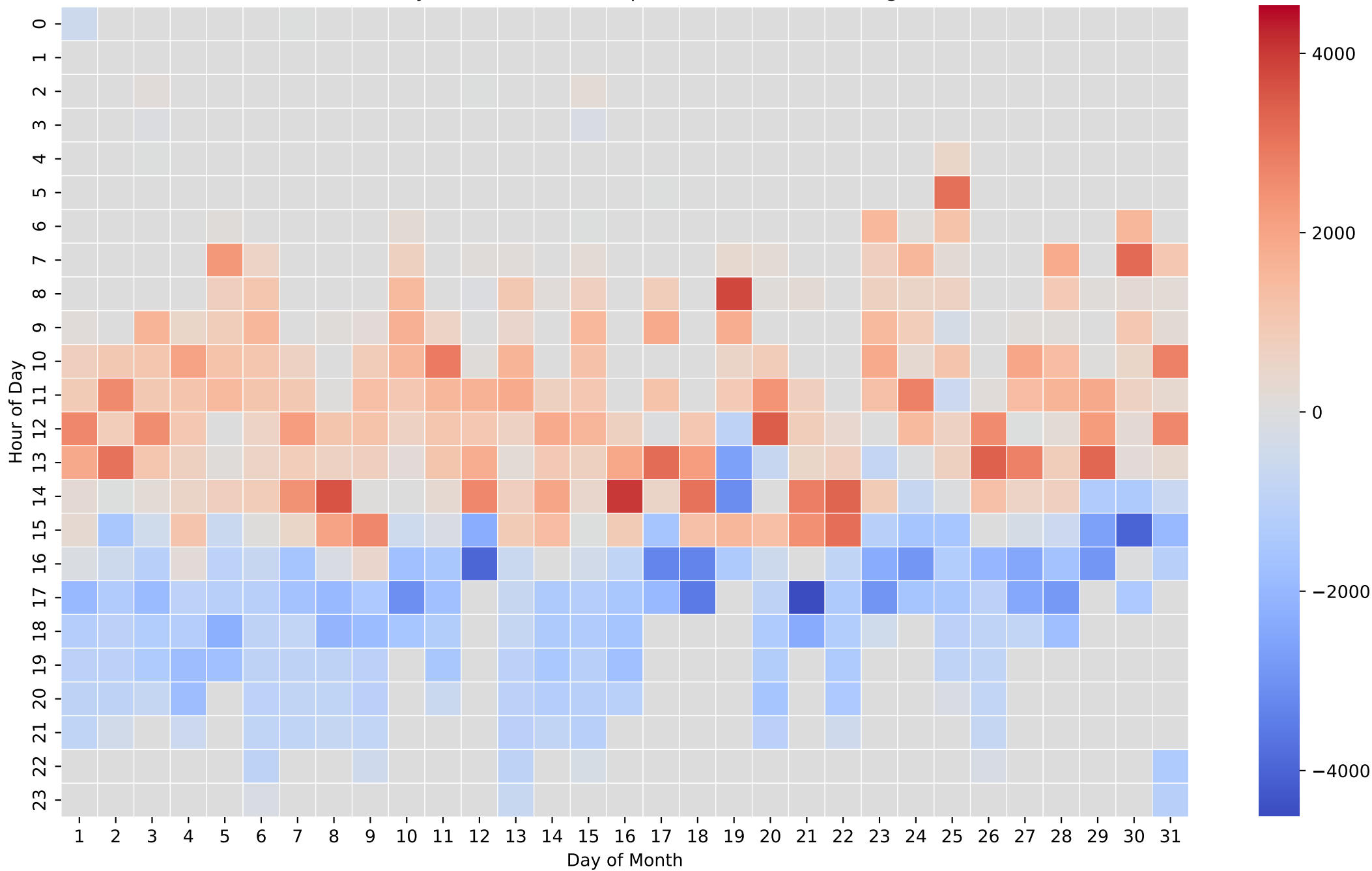
Battery Net Power Heatmap (Wh/Hour) - 8kWh - Aug
