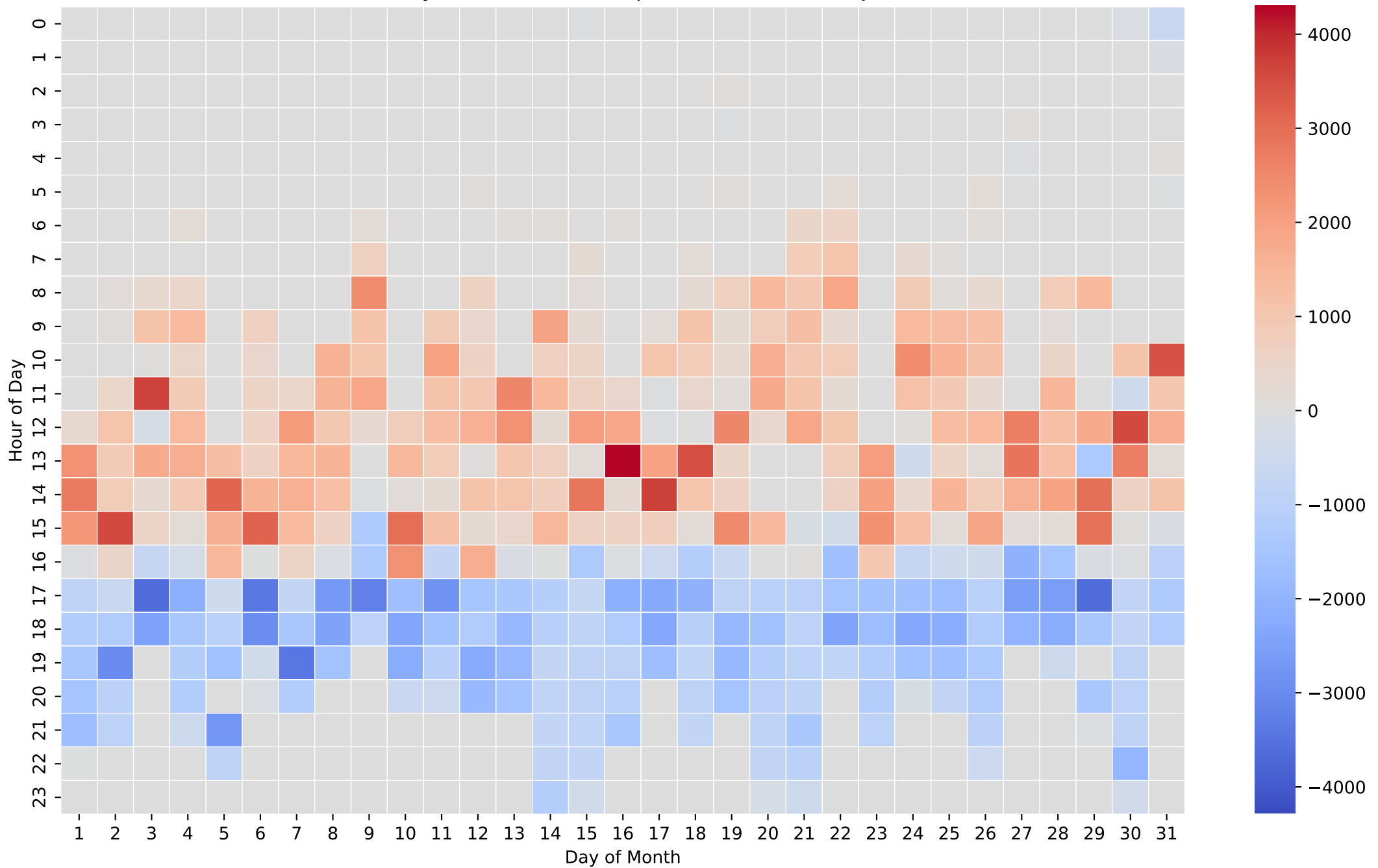
Battery Net Power Heatmap (Wh/Hour) - 8kWh - Jul
